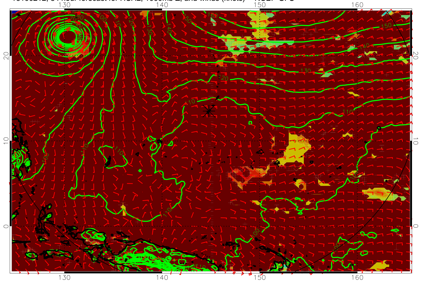
16100212, 84 hour forecast for HCAL, 1000mb Z, and winds (knots) -- NCEP GFS
