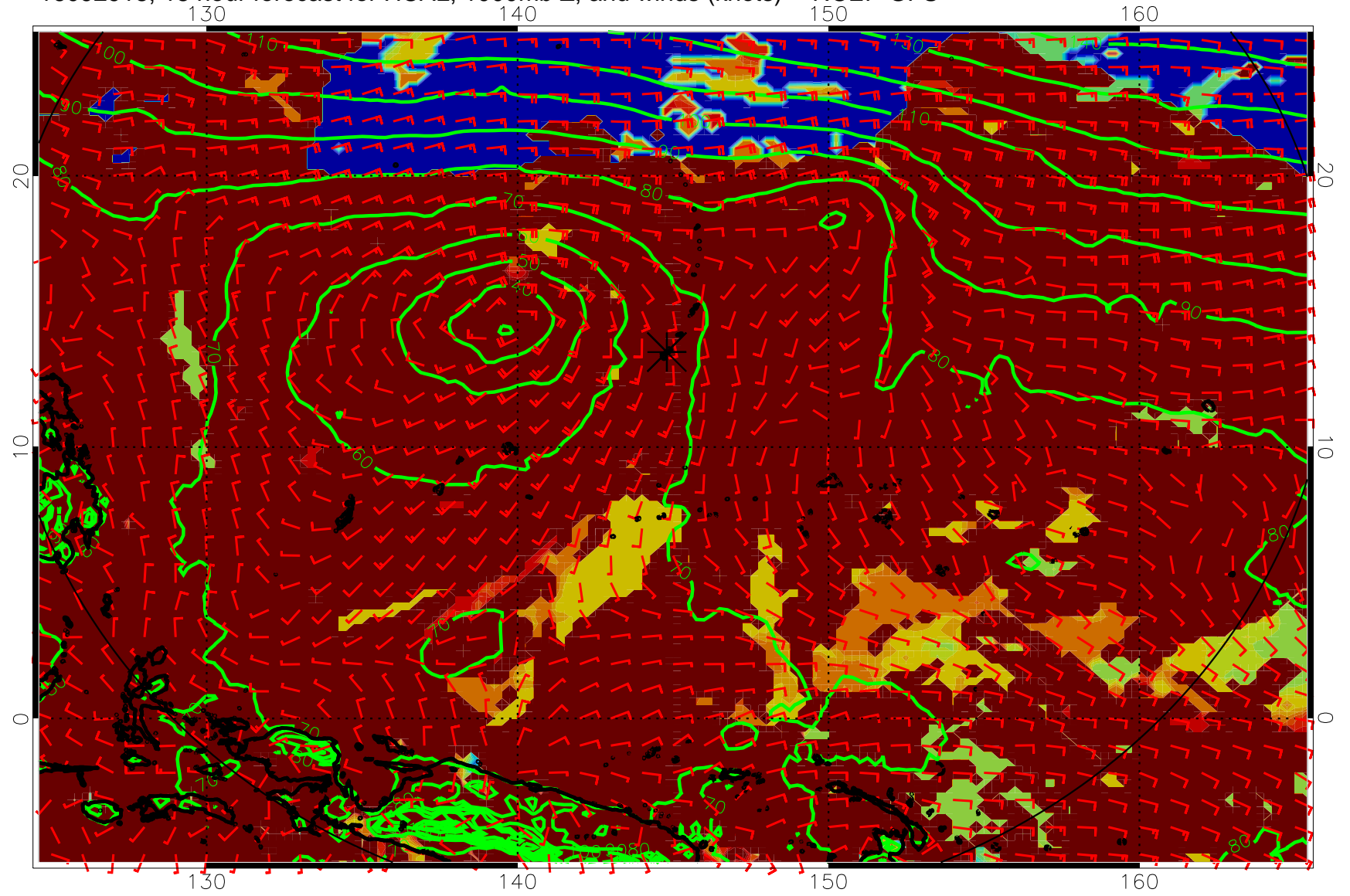
16092918, 18 hour forecast for HCAL, 1000mb Z, and winds (knots) -- NCEP GFS
