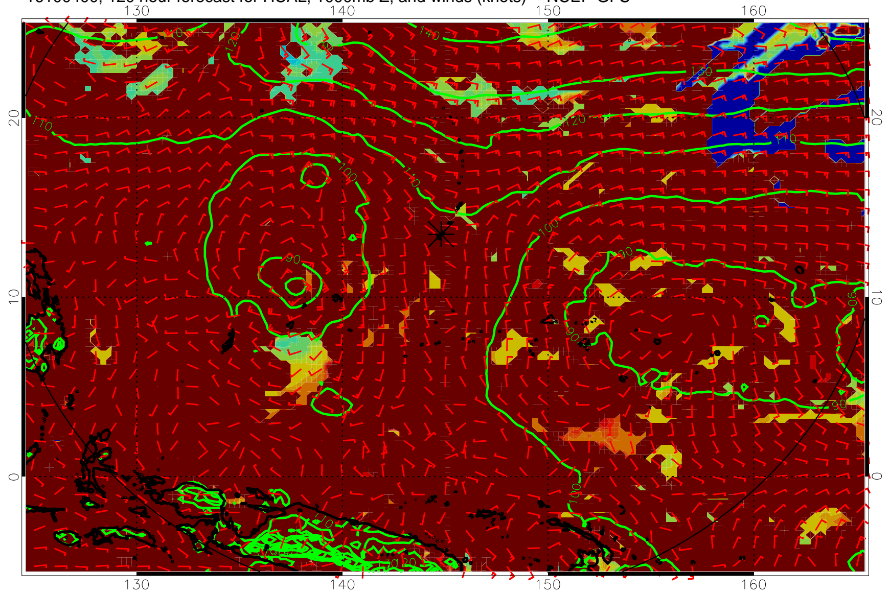
16100400, 120 hour forecast for HCAL, 1000mb Z, and winds (knots) -- NCEP GFS
