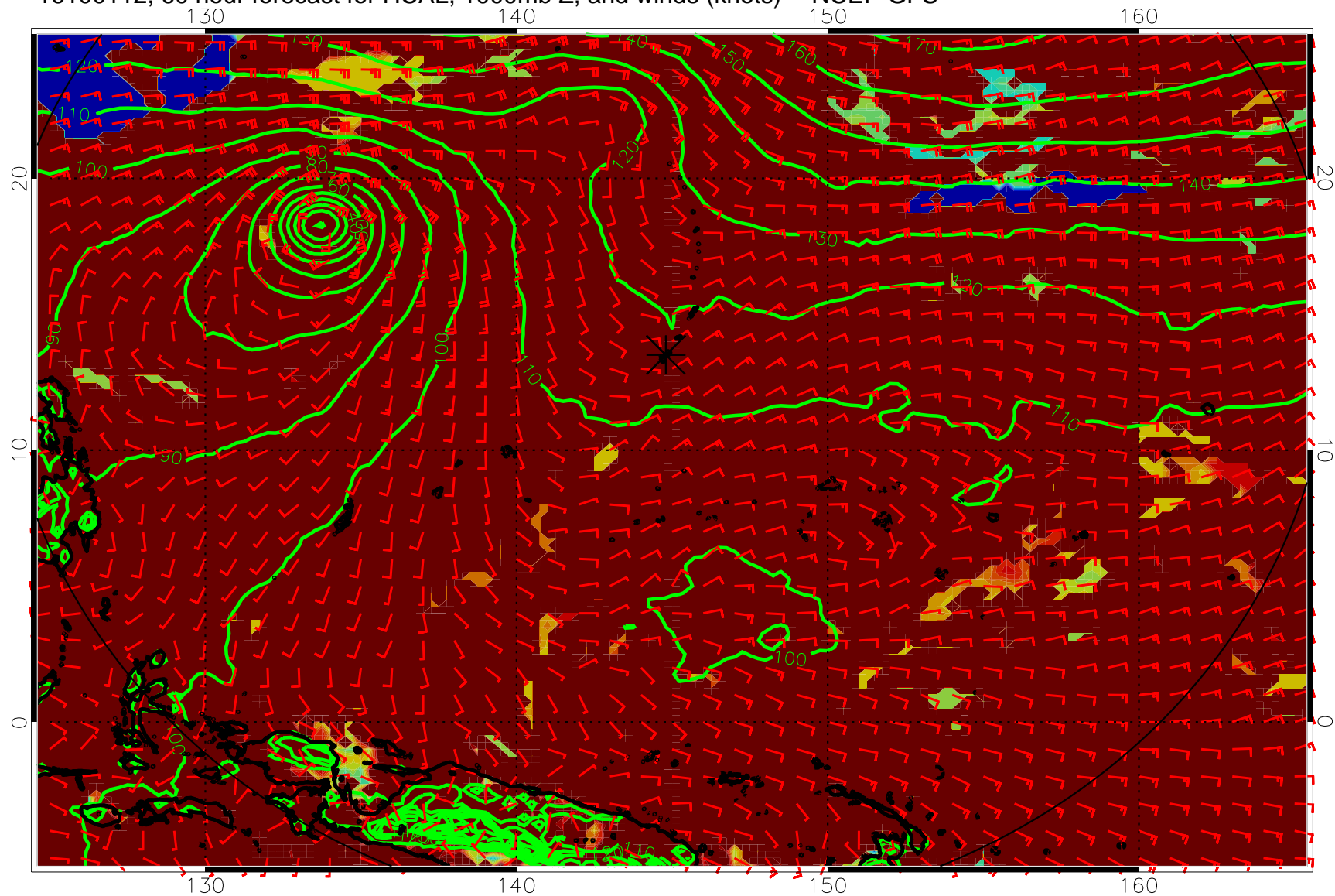
16100112, 60 hour forecast for HCAL, 1000mb Z, and winds (knots) -- NCEP GFS
