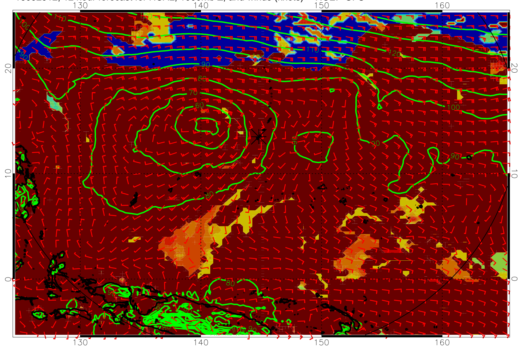
16092912, 12 hour forecast for HCAL, 1000mb Z, and winds (knots) -- NCEP GFS
