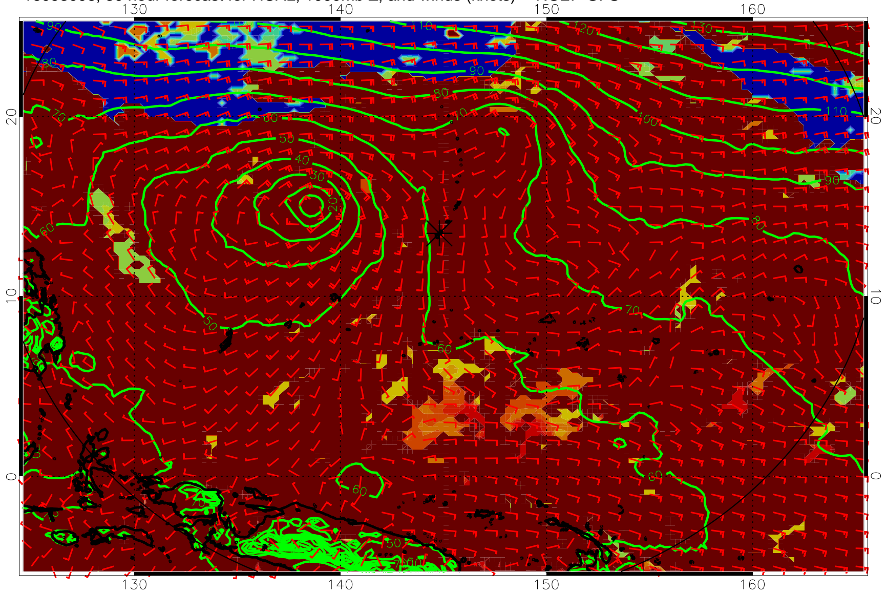
16093006, 30 hour forecast for HCAL, 1000mb Z, and winds (knots) -- NCEP GFS
