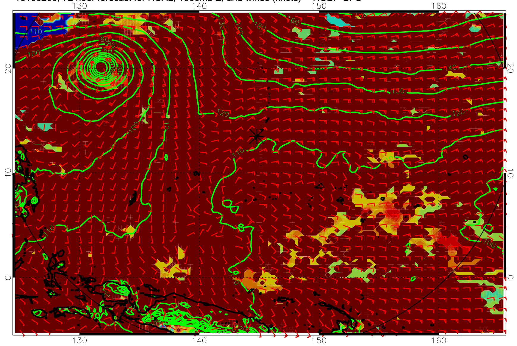
16100200, 72 hour forecast for HCAL, 1000mb Z, and winds (knots) -- NCEP GFS
