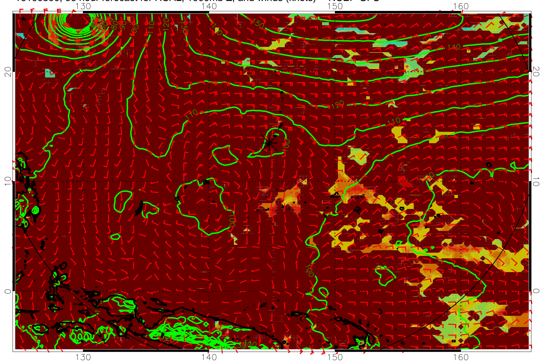
16100300, 96 hour forecast for HCAL, 1000mb Z, and winds (knots) -- NCEP GFS
