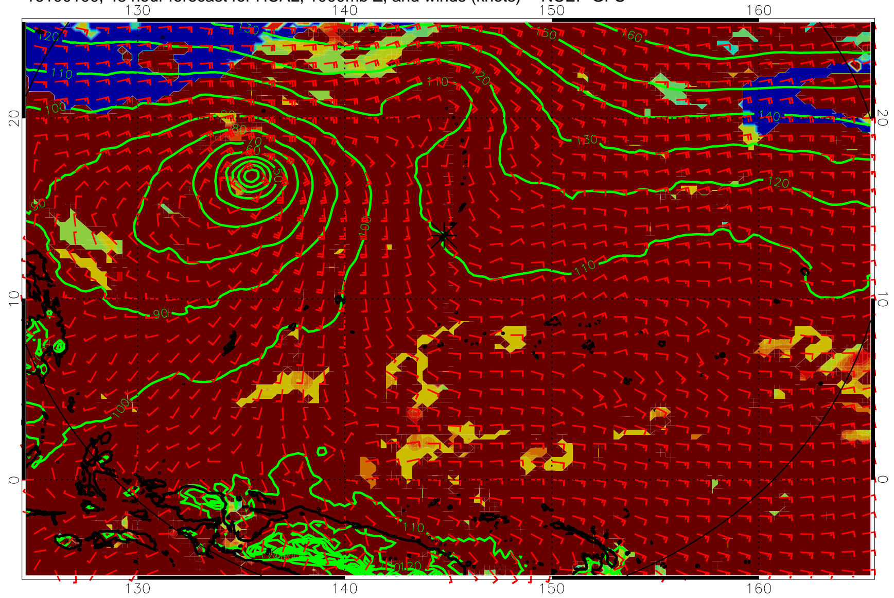
16100100, 48 hour forecast for HCAL, 1000mb Z, and winds (knots) -- NCEP GFS
