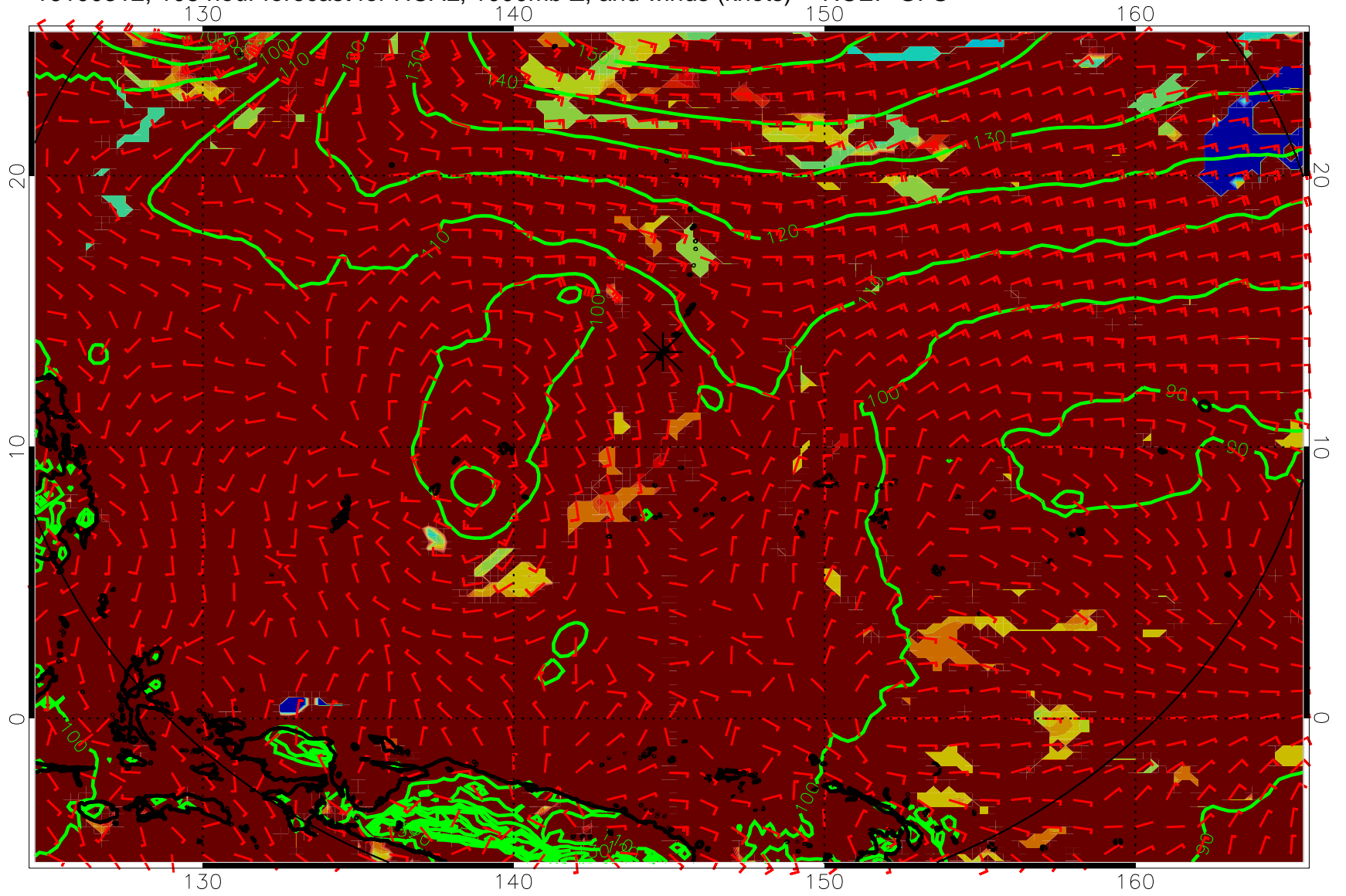
16100312, 108 hour forecast for HCAL, 1000mb Z, and winds (knots) -- NCEP GFS
