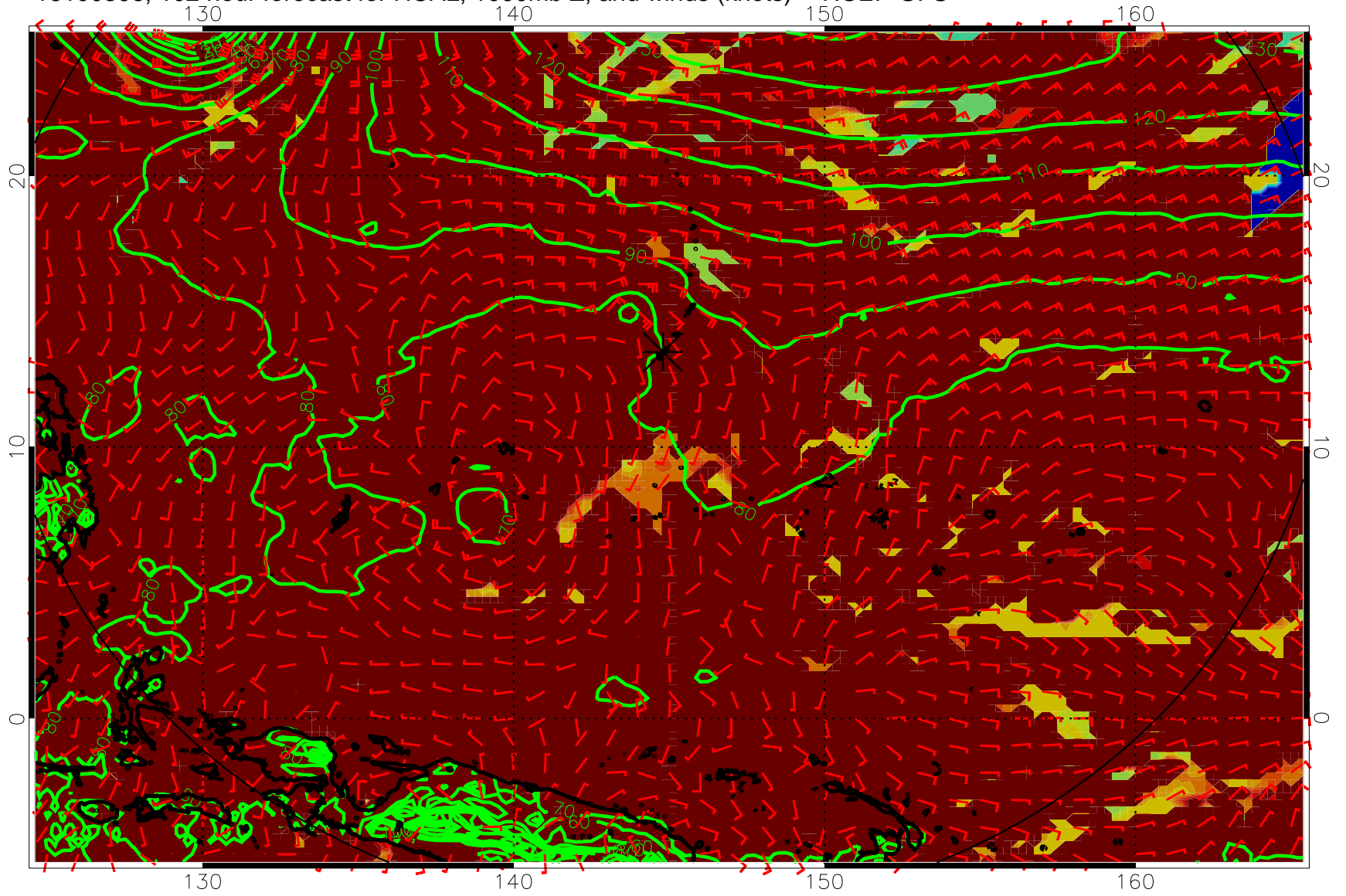
16100306, 102 hour forecast for HCAL, 1000mb Z, and winds (knots) -- NCEP GFS
