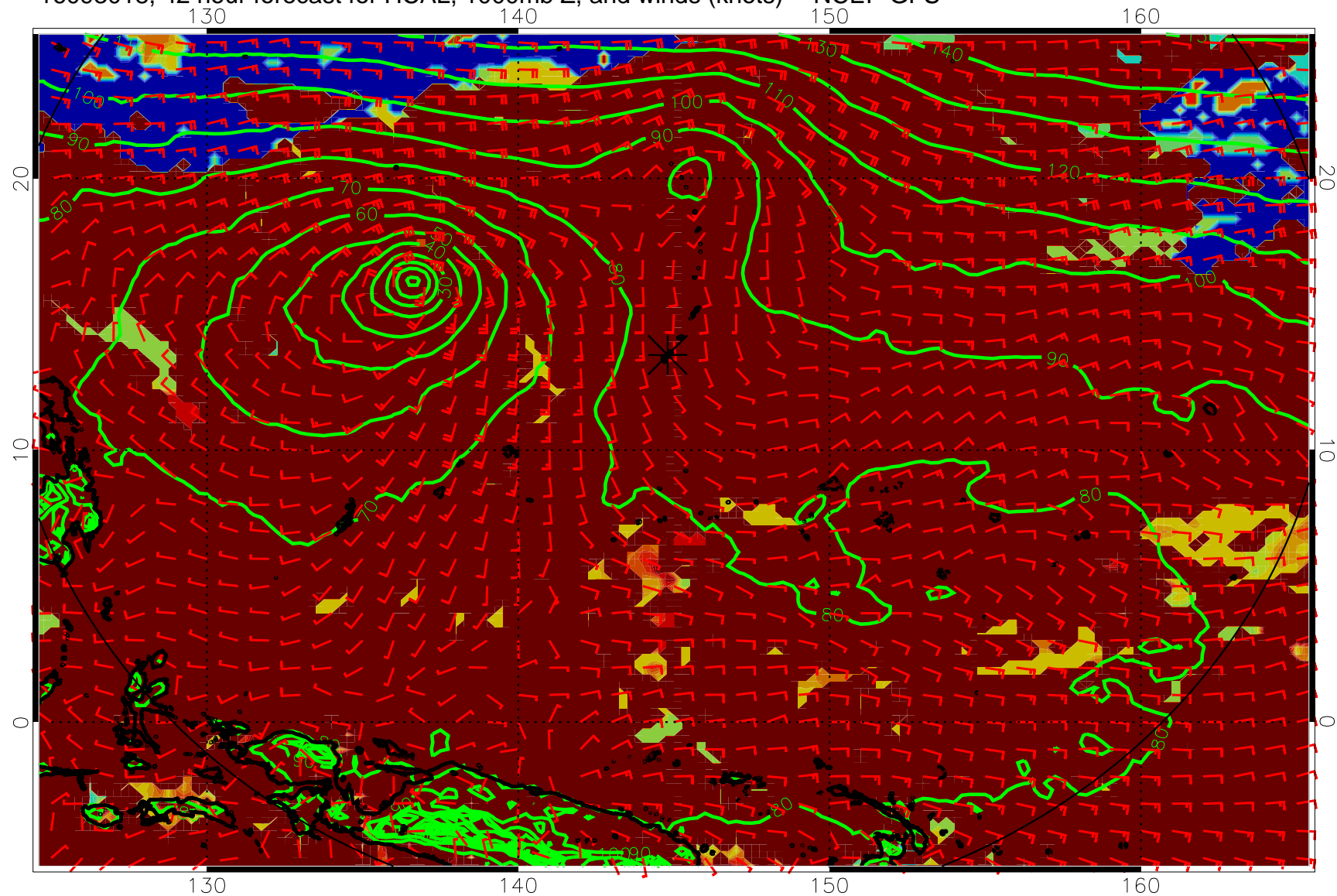
16093018, 42 hour forecast for HCAL, 1000mb Z, and winds (knots) -- NCEP GFS
