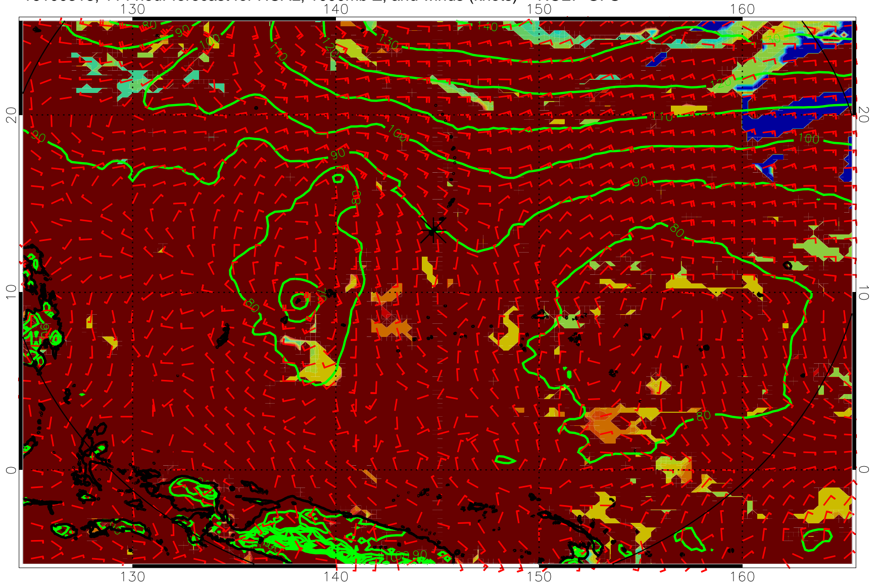
16100318, 114 hour forecast for HCAL, 1000mb Z, and winds (knots) -- NCEP GFS
