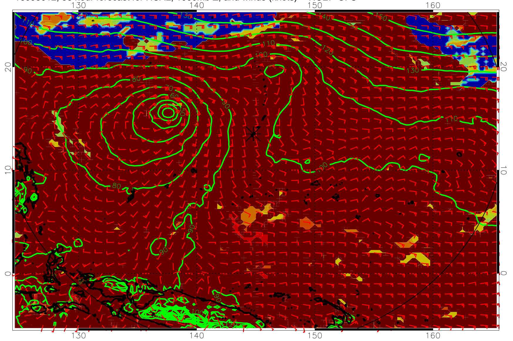
16093012, 36 hour forecast for HCAL, 1000mb Z, and winds (knots) -- NCEP GFS
