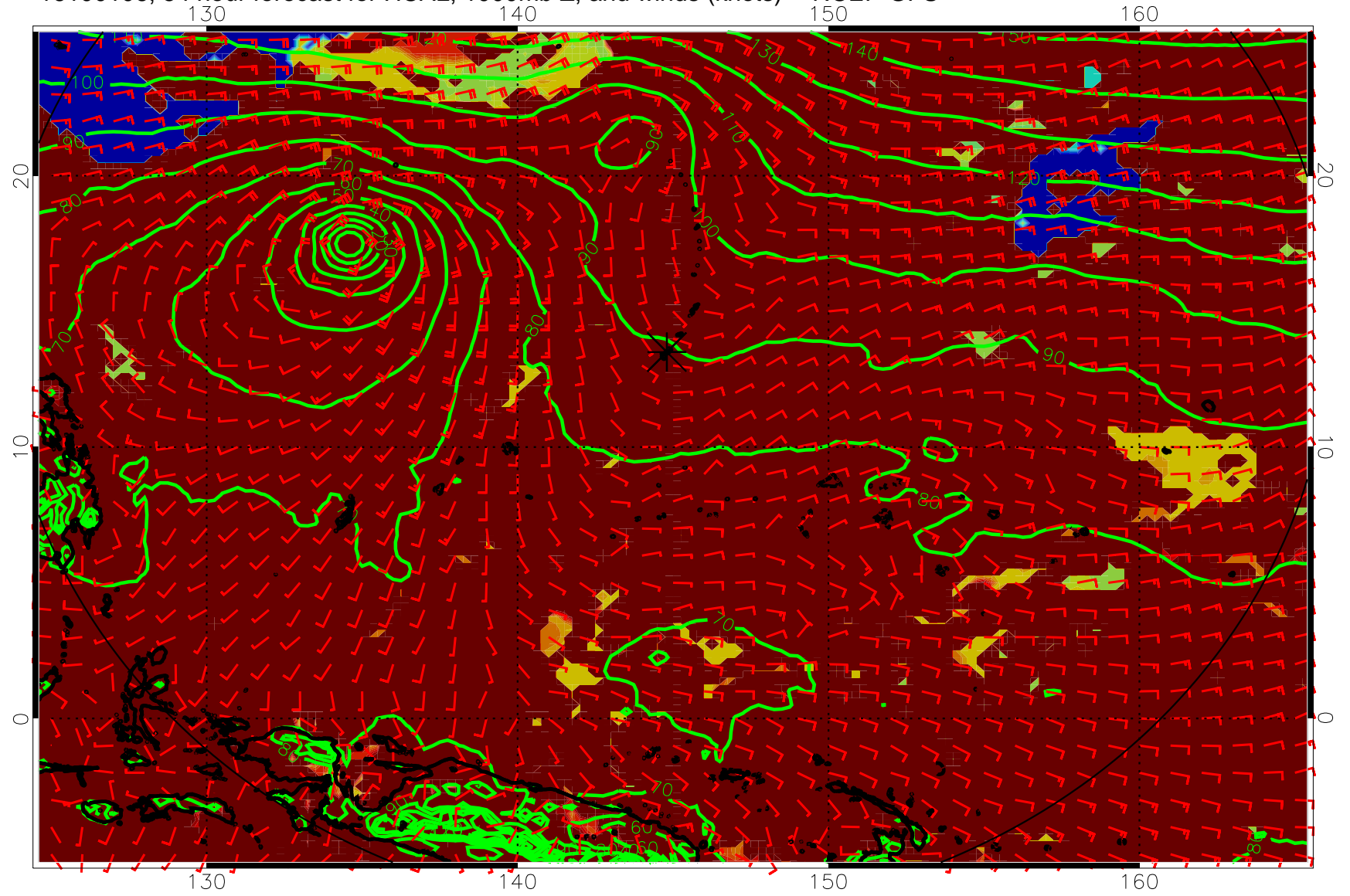
16100106, 54 hour forecast for HCAL, 1000mb Z, and winds (knots) -- NCEP GFS
