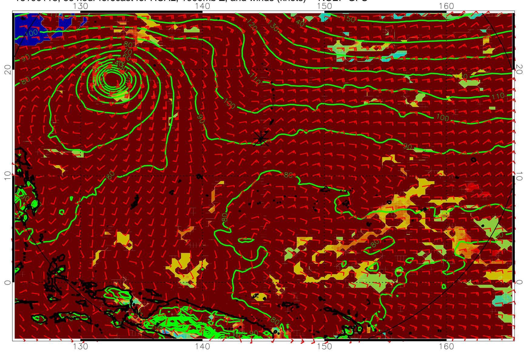
16100118, 66 hour forecast for HCAL, 1000mb Z, and winds (knots) -- NCEP GFS
