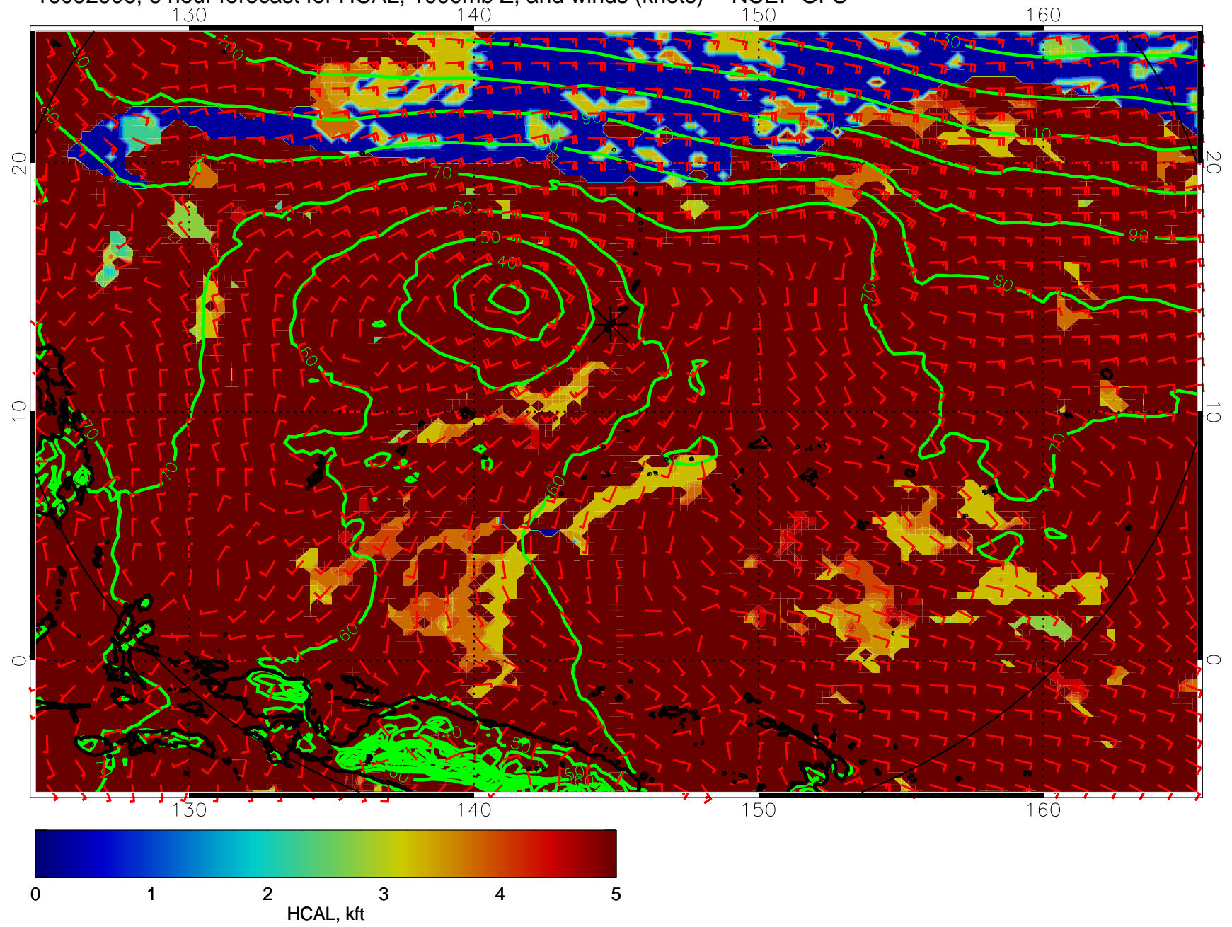
16092906, 6 hour forecast for HCAL, 1000mb Z, and winds (knots) -- NCEP GFS
