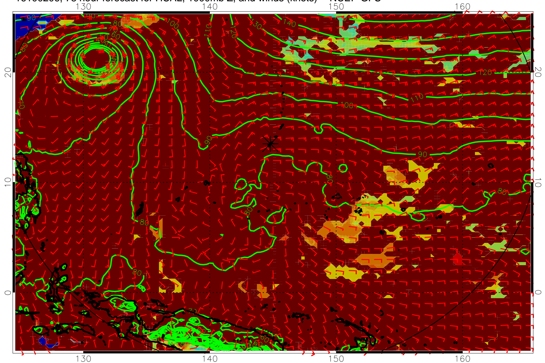
16100206, 78 hour forecast for HCAL, 1000mb Z, and winds (knots) -- NCEP GFS
