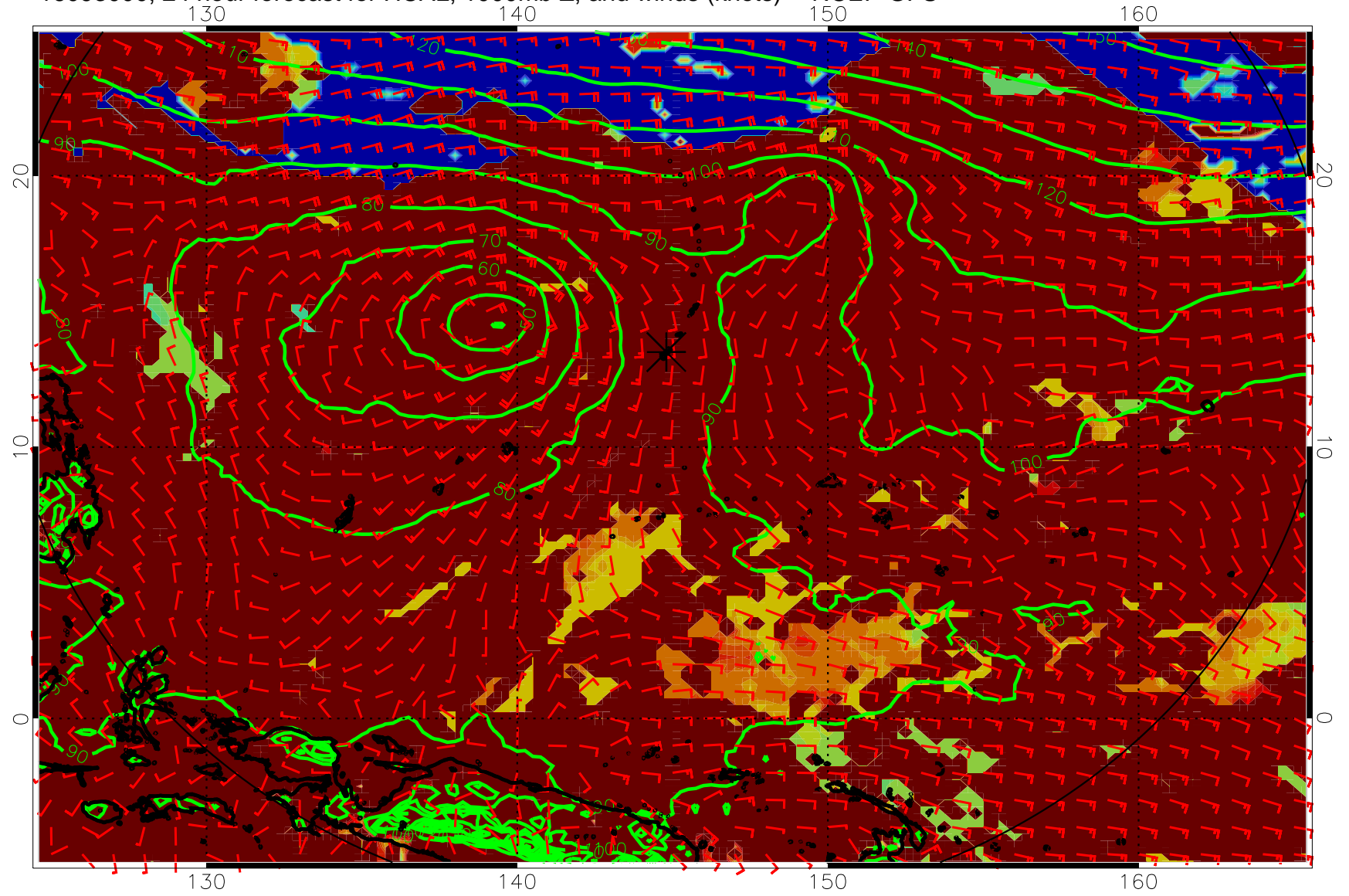
16093000, 24 hour forecast for HCAL, 1000mb Z, and winds (knots) -- NCEP GFS
