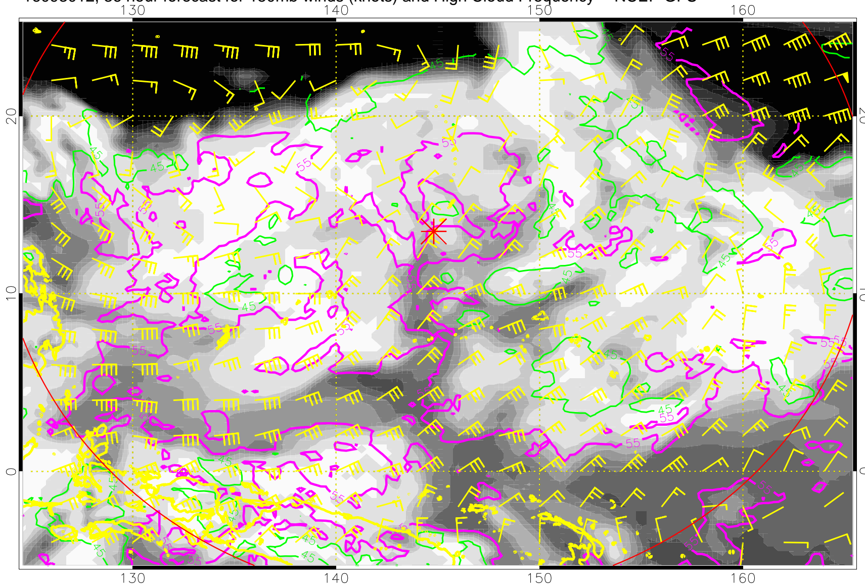
16093012, 36 hour forecast for 150mb winds (knots) and High Cloud Frequency -- NCEP GFS
