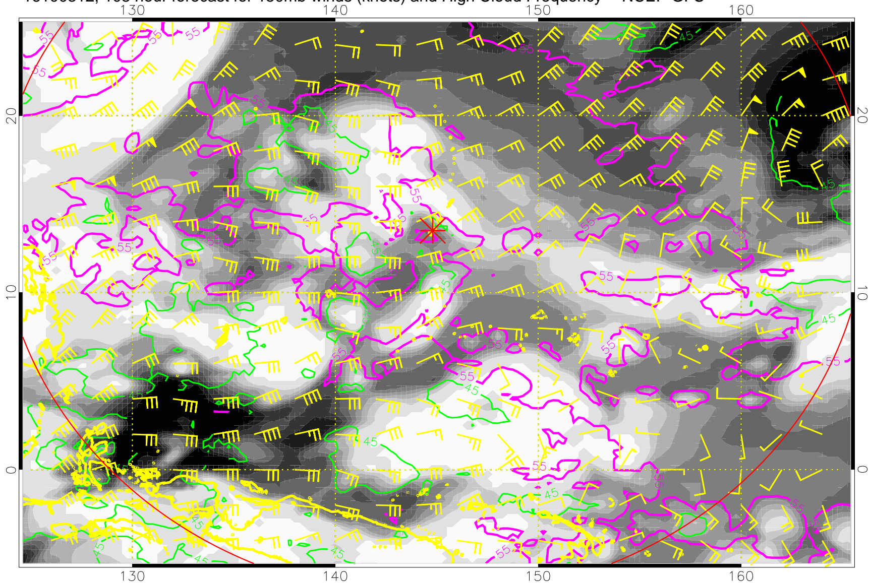
16100312, 108 hour forecast for 150mb winds (knots) and High Cloud Frequency -- NCEP GFS
