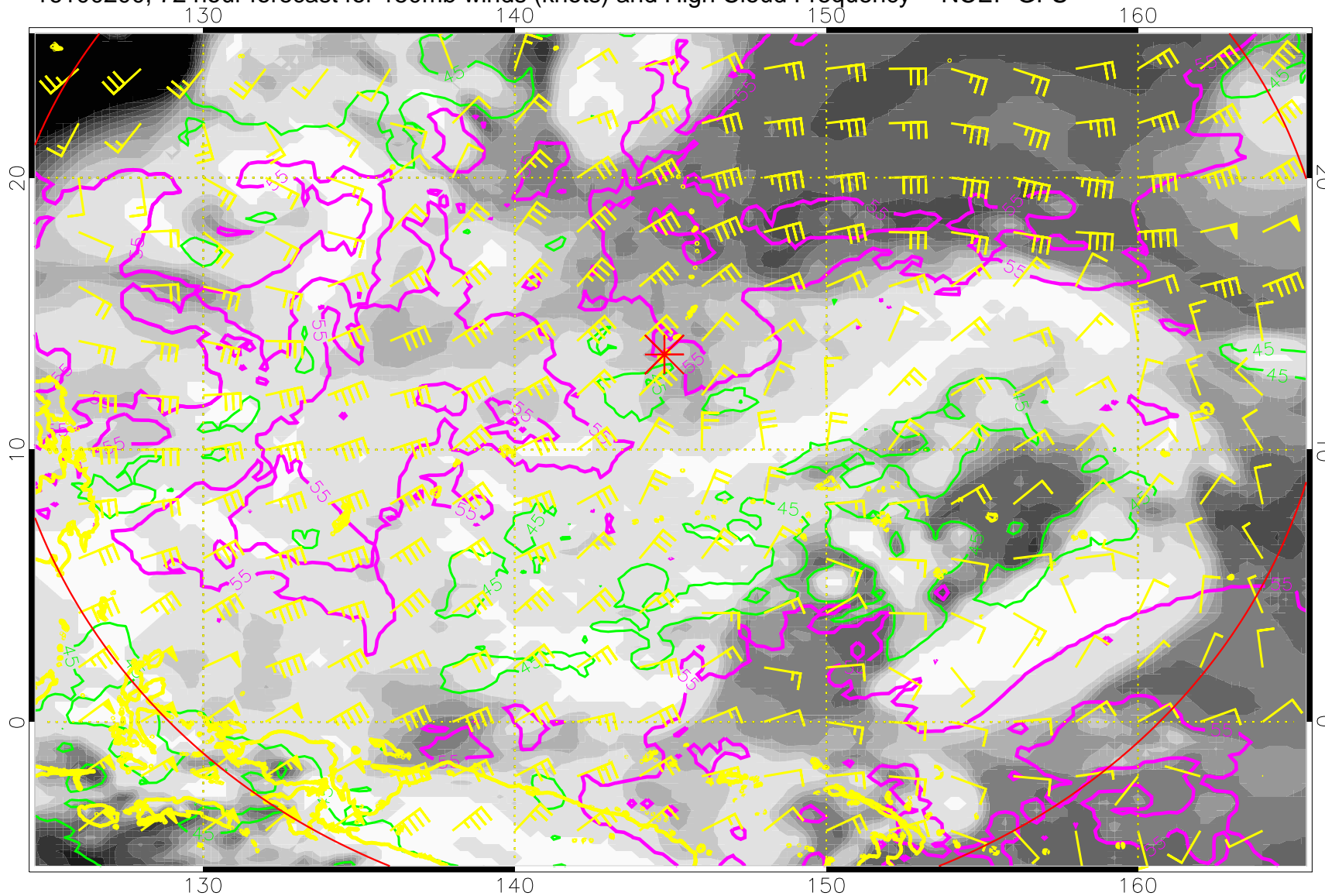
16100200, 72 hour forecast for 150mb winds (knots) and High Cloud Frequency -- NCEP GFS
