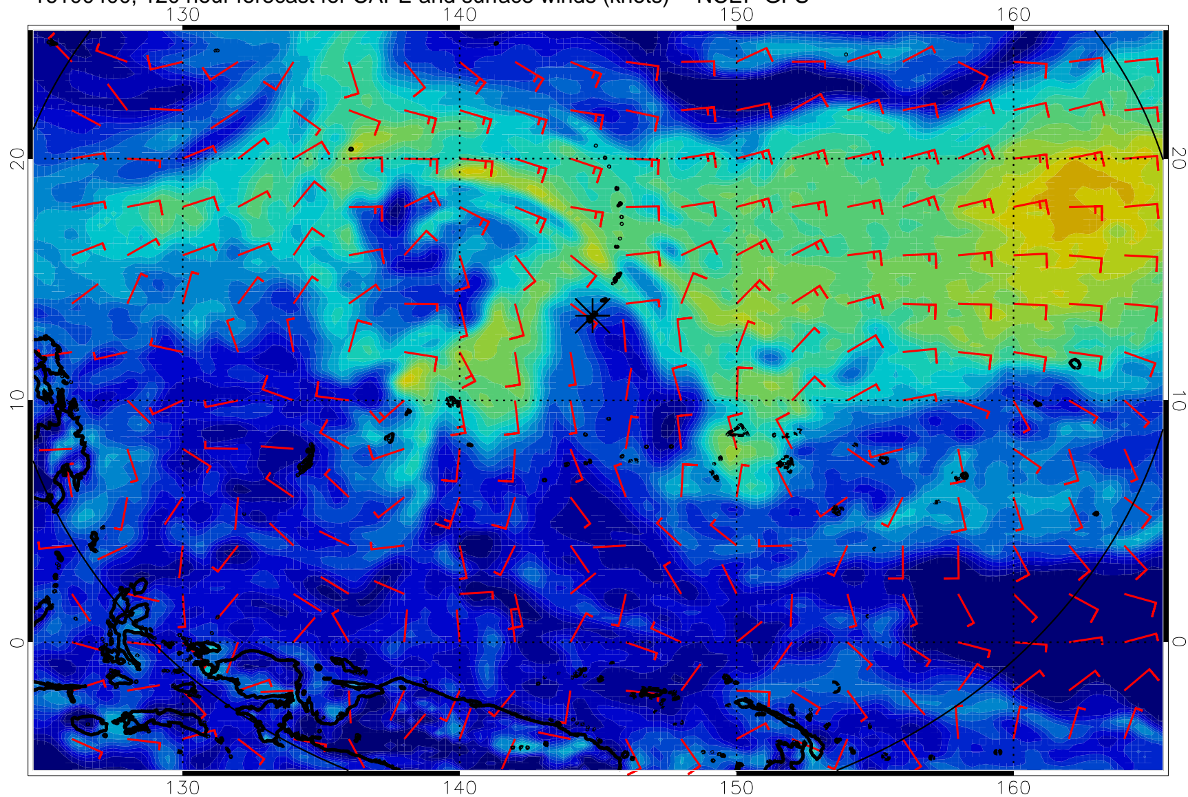
16100400, 120 hour forecast for CAPE and surface winds (knots) -- NCEP GFS
