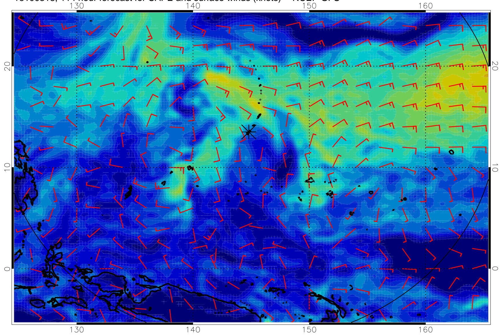
16100318, 114 hour forecast for CAPE and surface winds (knots) -- NCEP GFS
