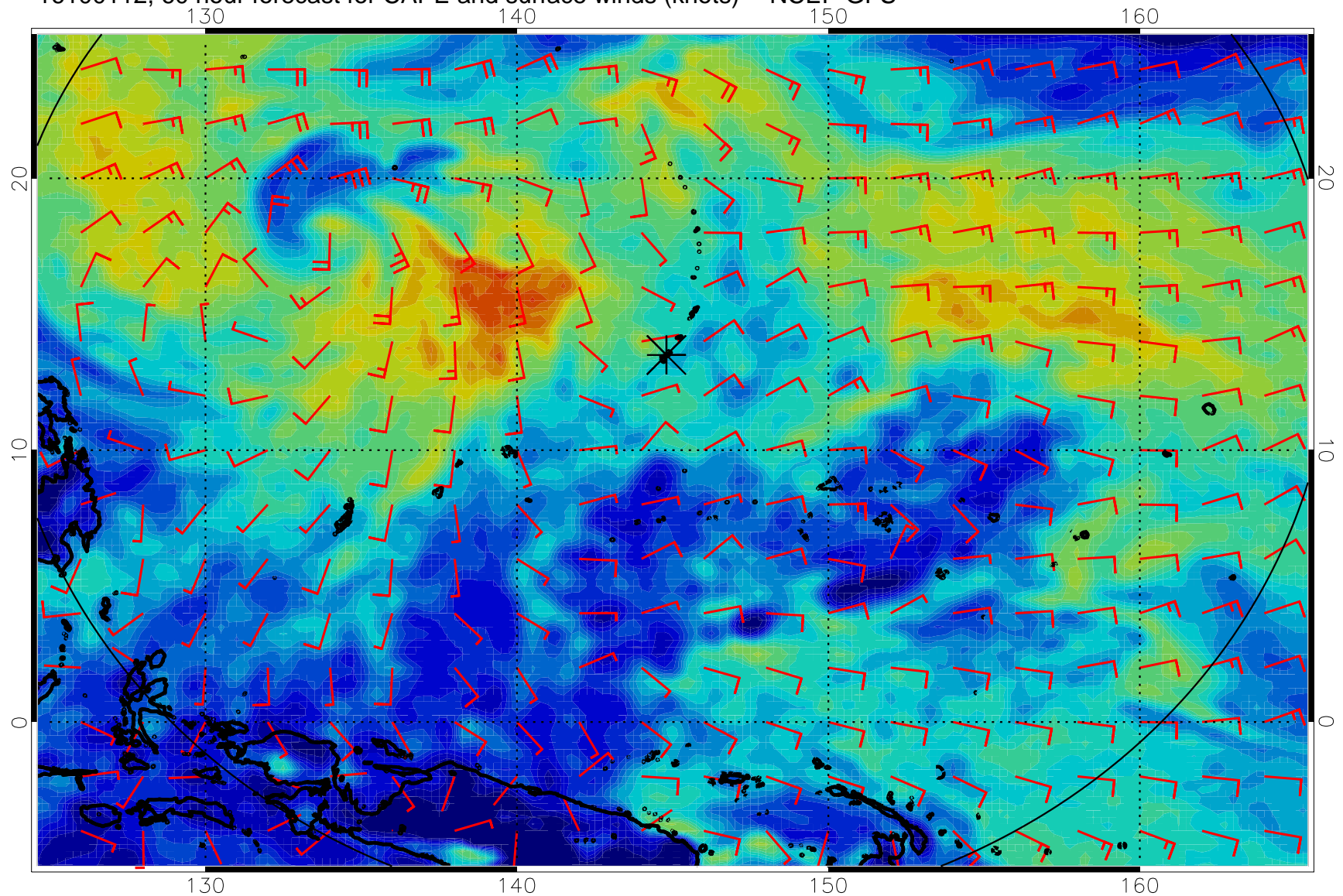
16100112, 60 hour forecast for CAPE and surface winds (knots) -- NCEP GFS
