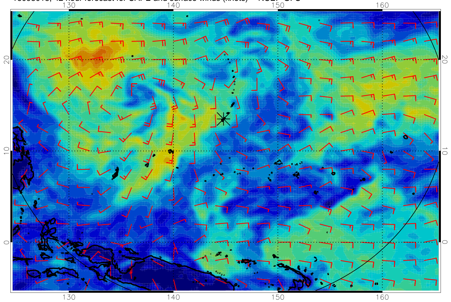
16093018, 42 hour forecast for CAPE and surface winds (knots) -- NCEP GFS
