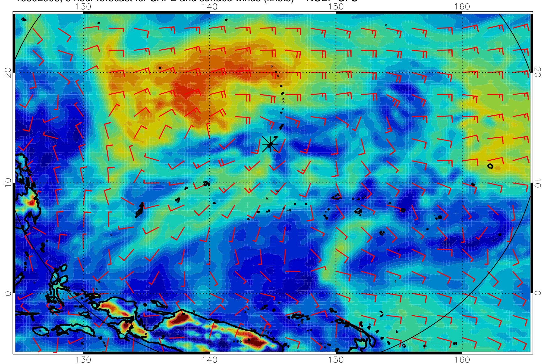
16092906, 6 hour forecast for CAPE and surface winds (knots) -- NCEP GFS
