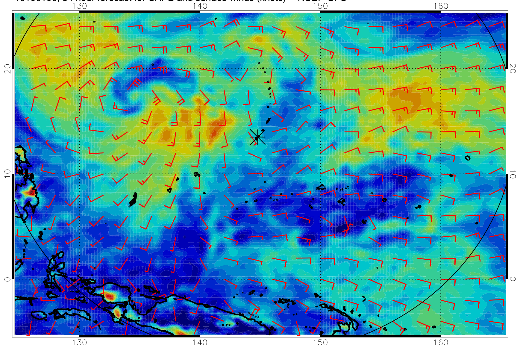
16100106, 54 hour forecast for CAPE and surface winds (knots) -- NCEP GFS
