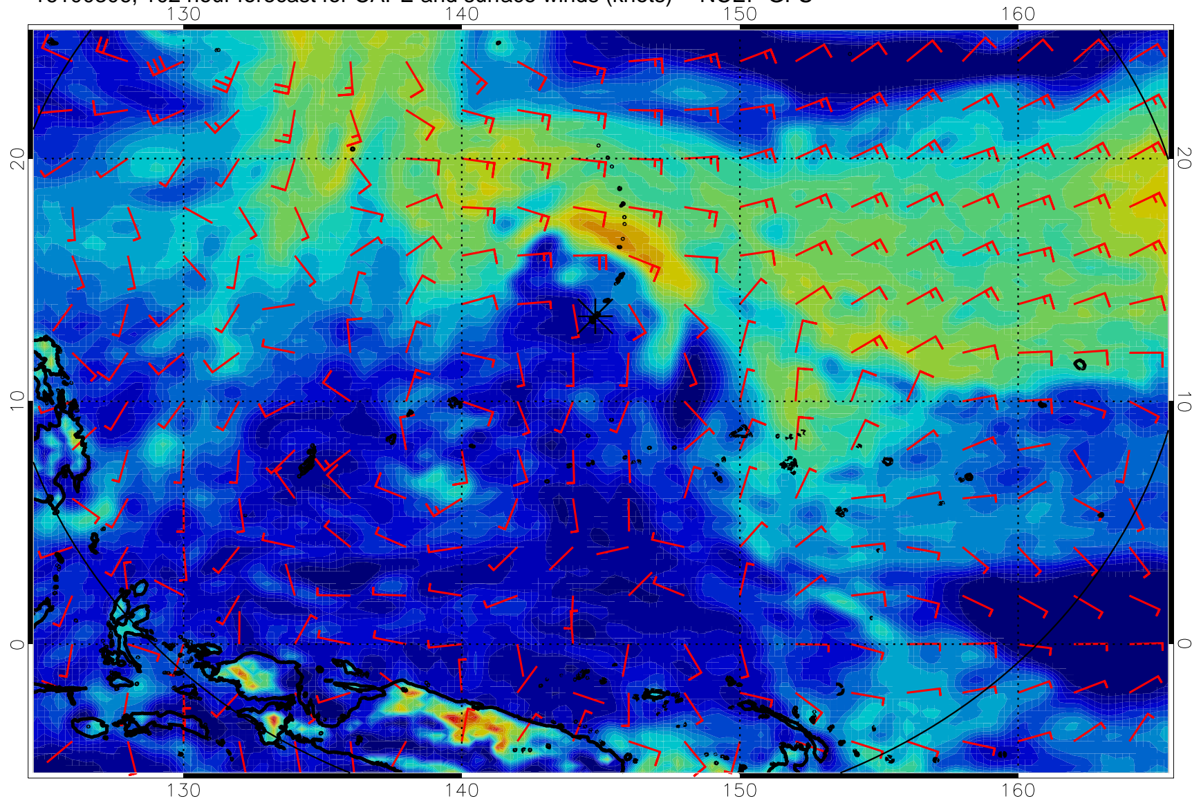
16100306, 102 hour forecast for CAPE and surface winds (knots) -- NCEP GFS
