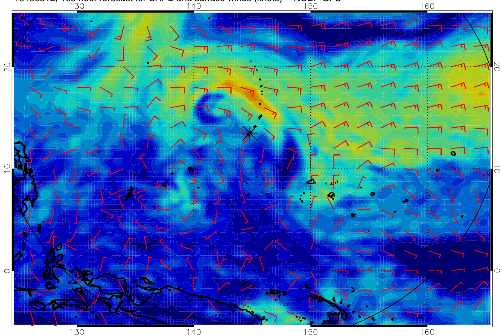
16100312, 108 hour forecast for CAPE and surface winds (knots) -- NCEP GFS
