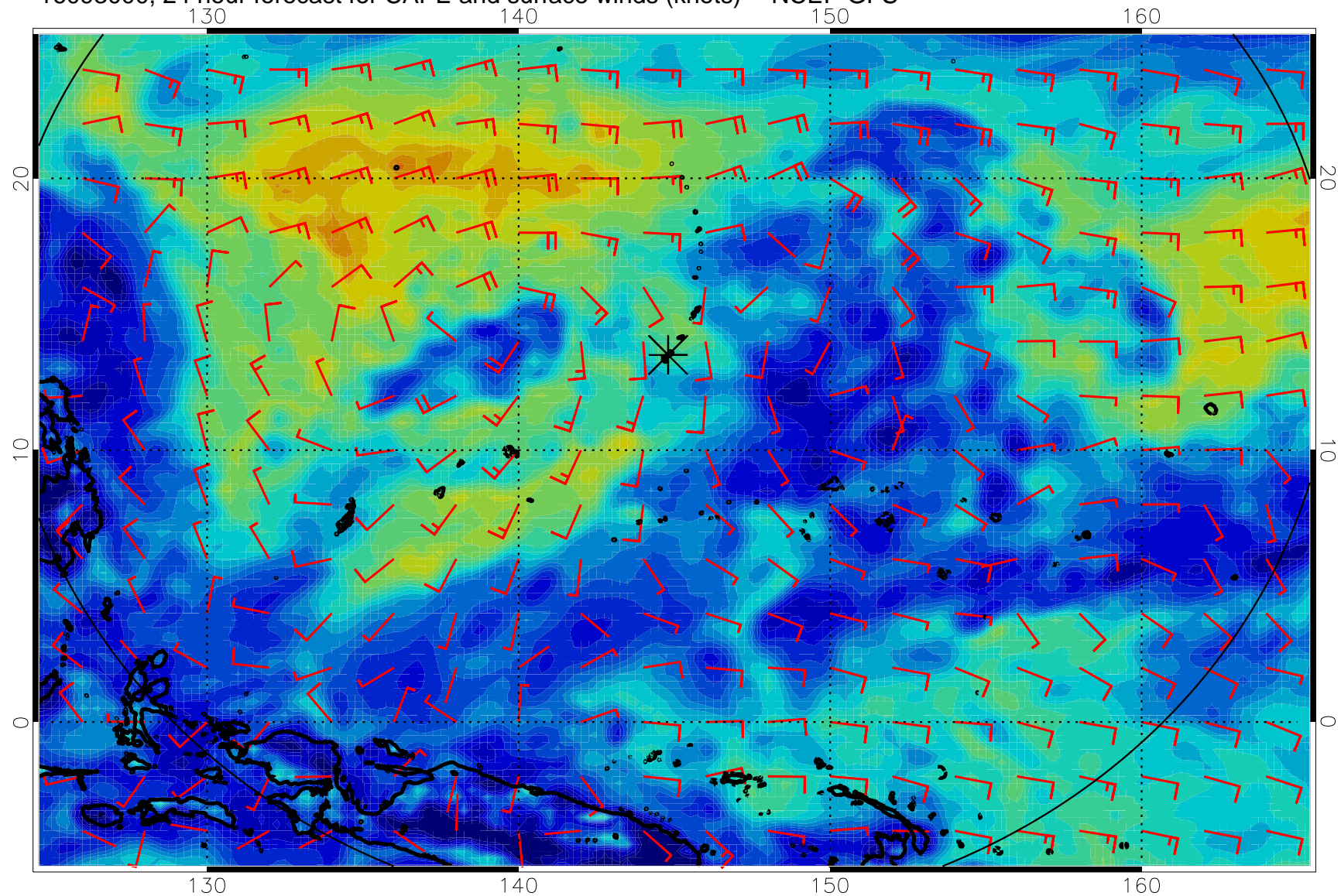
16093000, 24 hour forecast for CAPE and surface winds (knots) -- NCEP GFS
