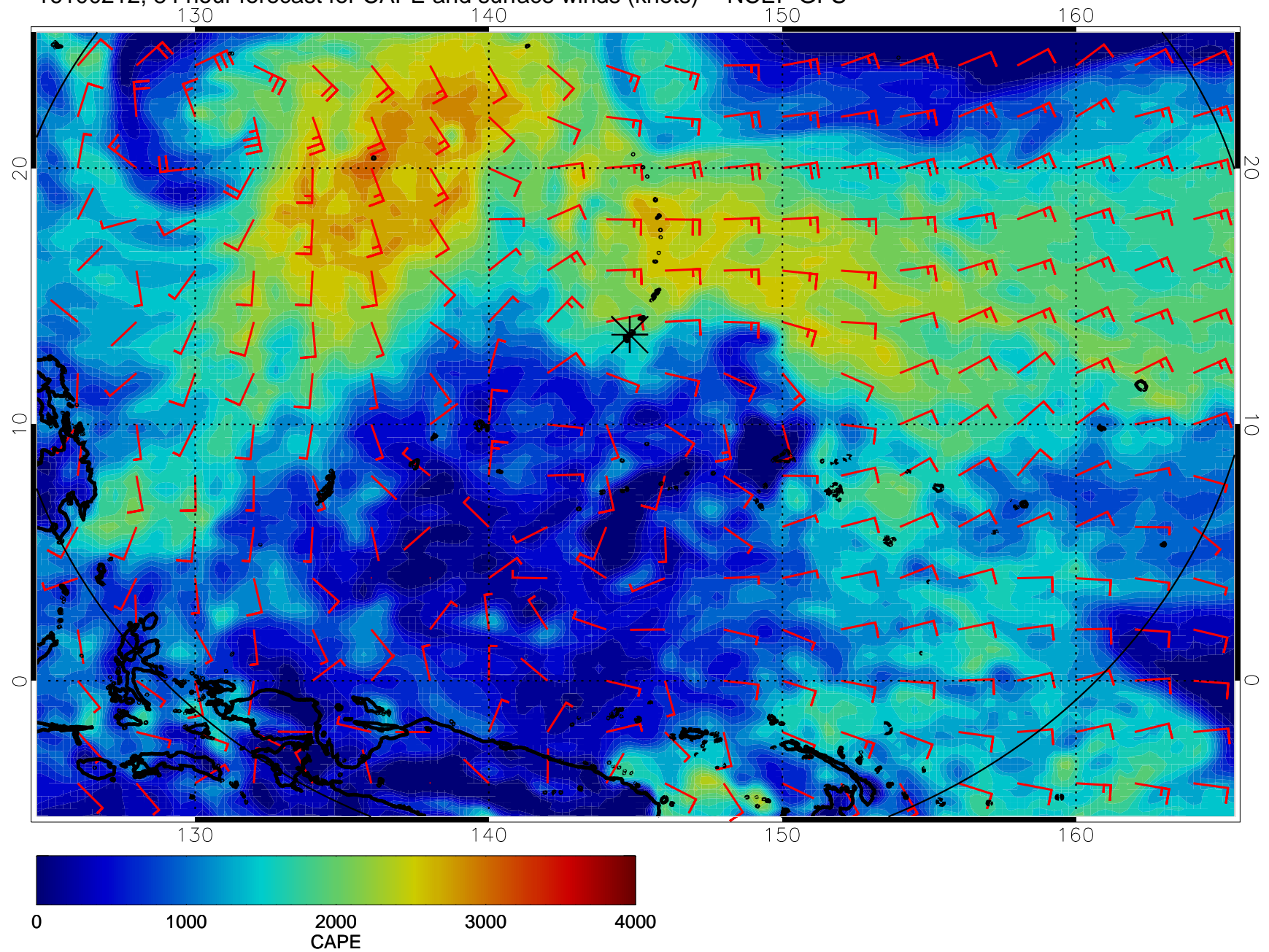
16100212, 84 hour forecast for CAPE and surface winds (knots) -- NCEP GFS
