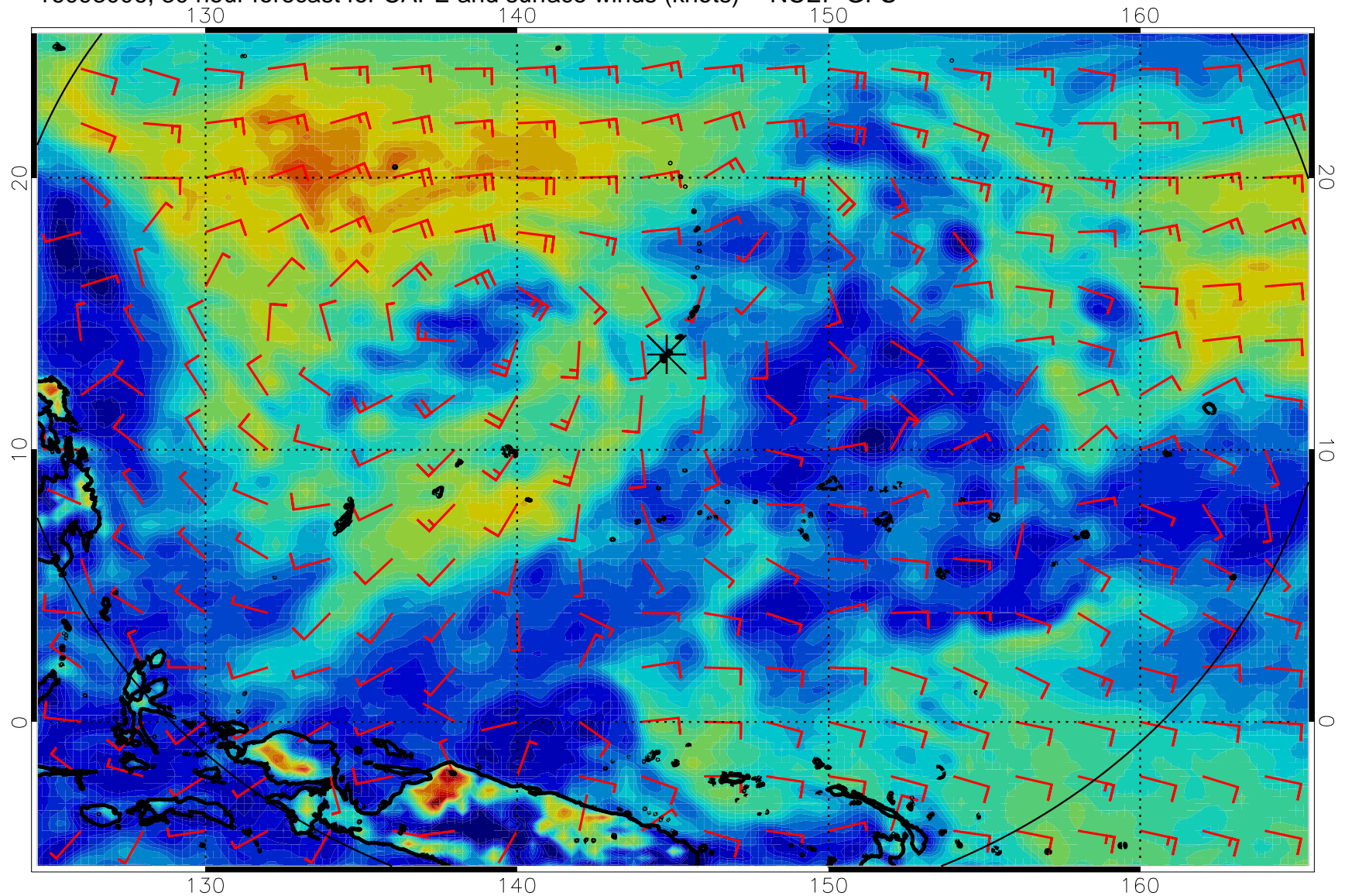
16093006, 30 hour forecast for CAPE and surface winds (knots) -- NCEP GFS
