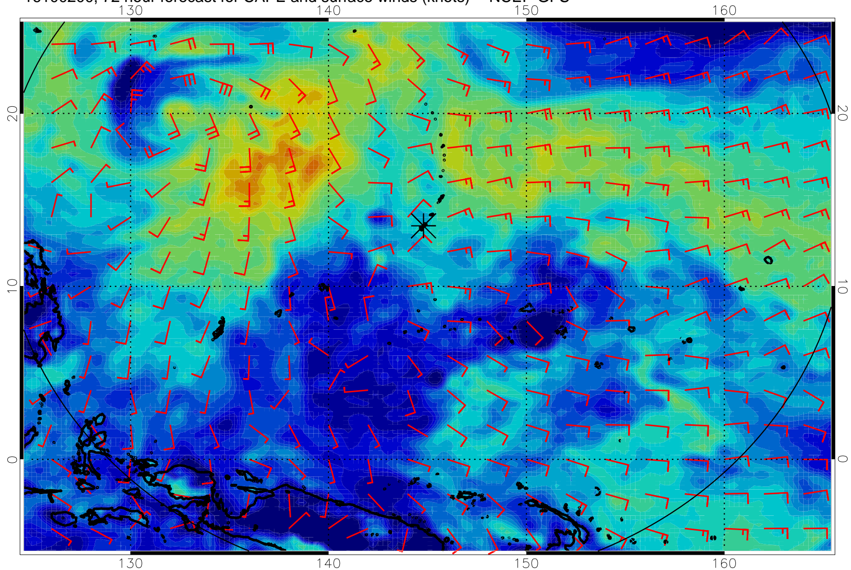
16100200, 72 hour forecast for CAPE and surface winds (knots) -- NCEP GFS
