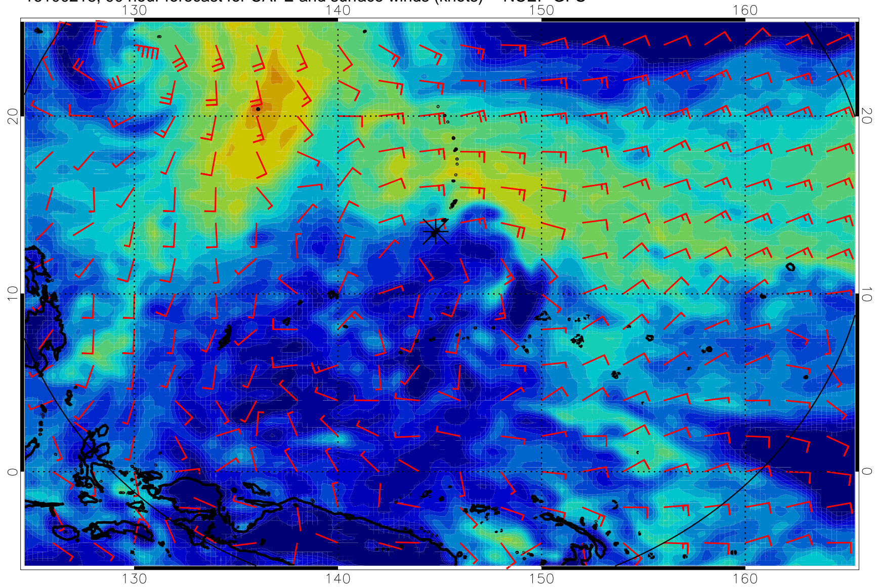
16100218, 90 hour forecast for CAPE and surface winds (knots) -- NCEP GFS
