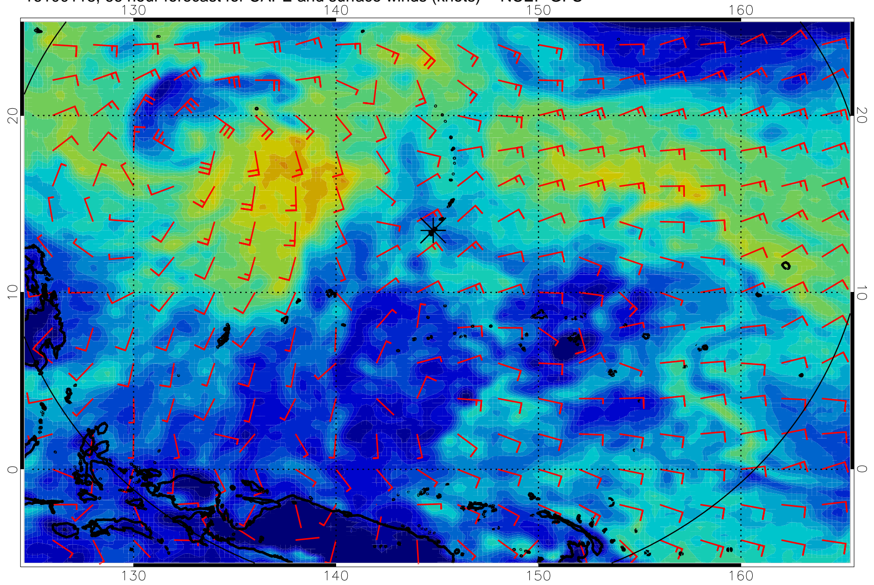
16100118, 66 hour forecast for CAPE and surface winds (knots) -- NCEP GFS
