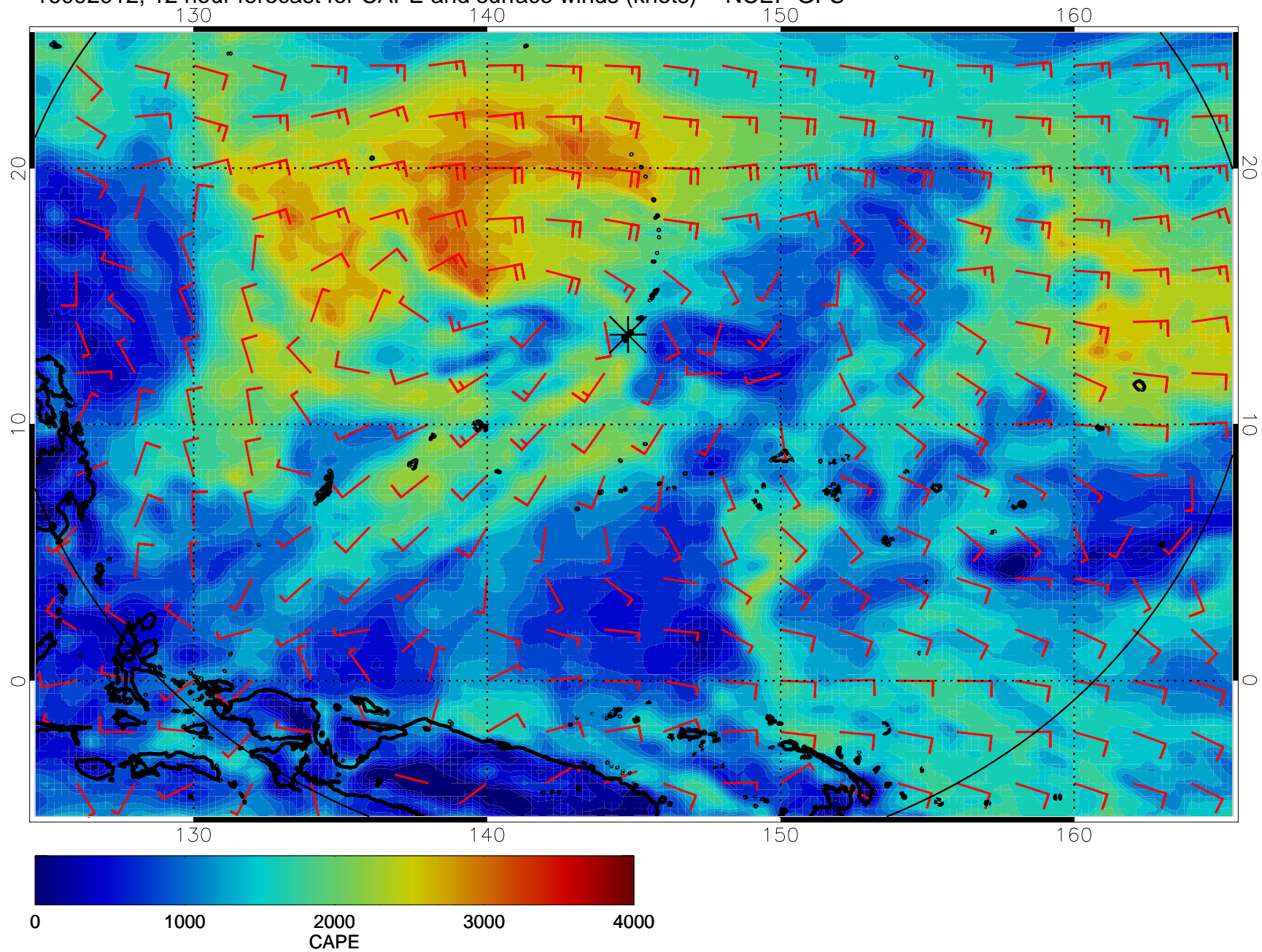
16092912, 12 hour forecast for CAPE and surface winds (knots) -- NCEP GFS
