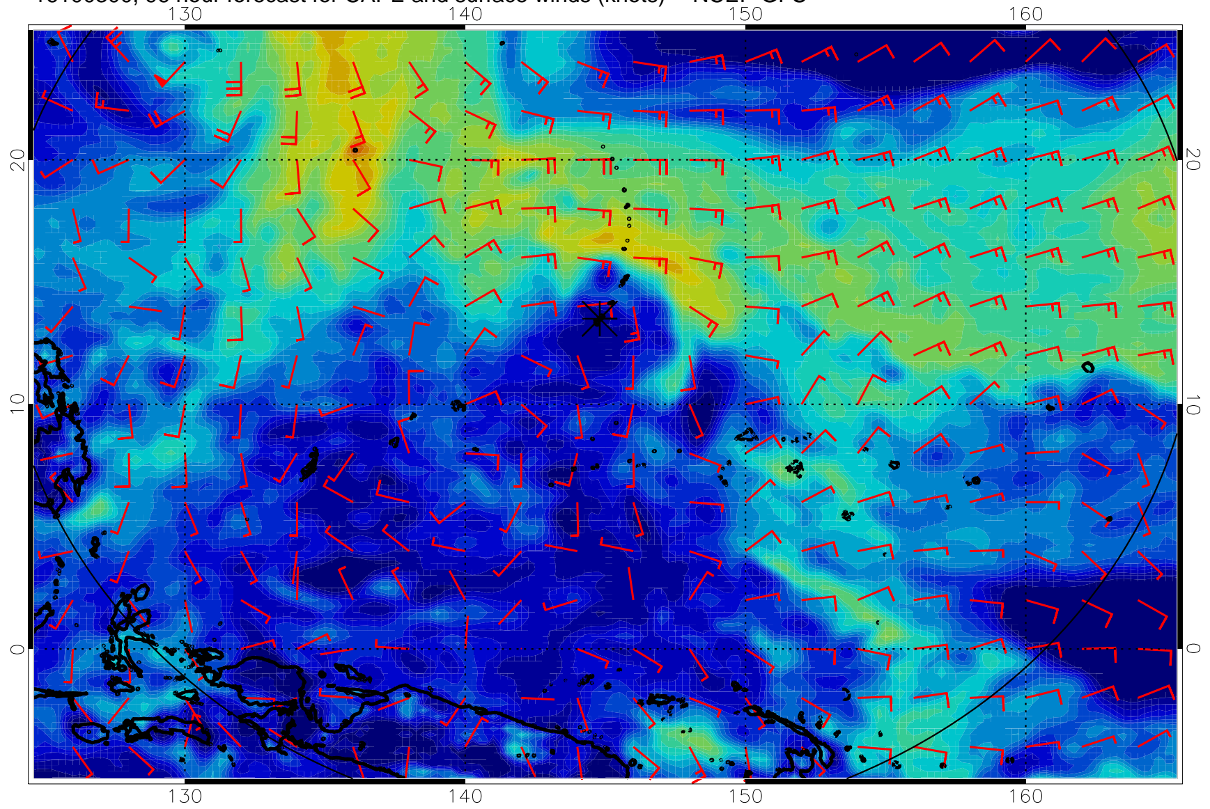
16100300, 96 hour forecast for CAPE and surface winds (knots) -- NCEP GFS
