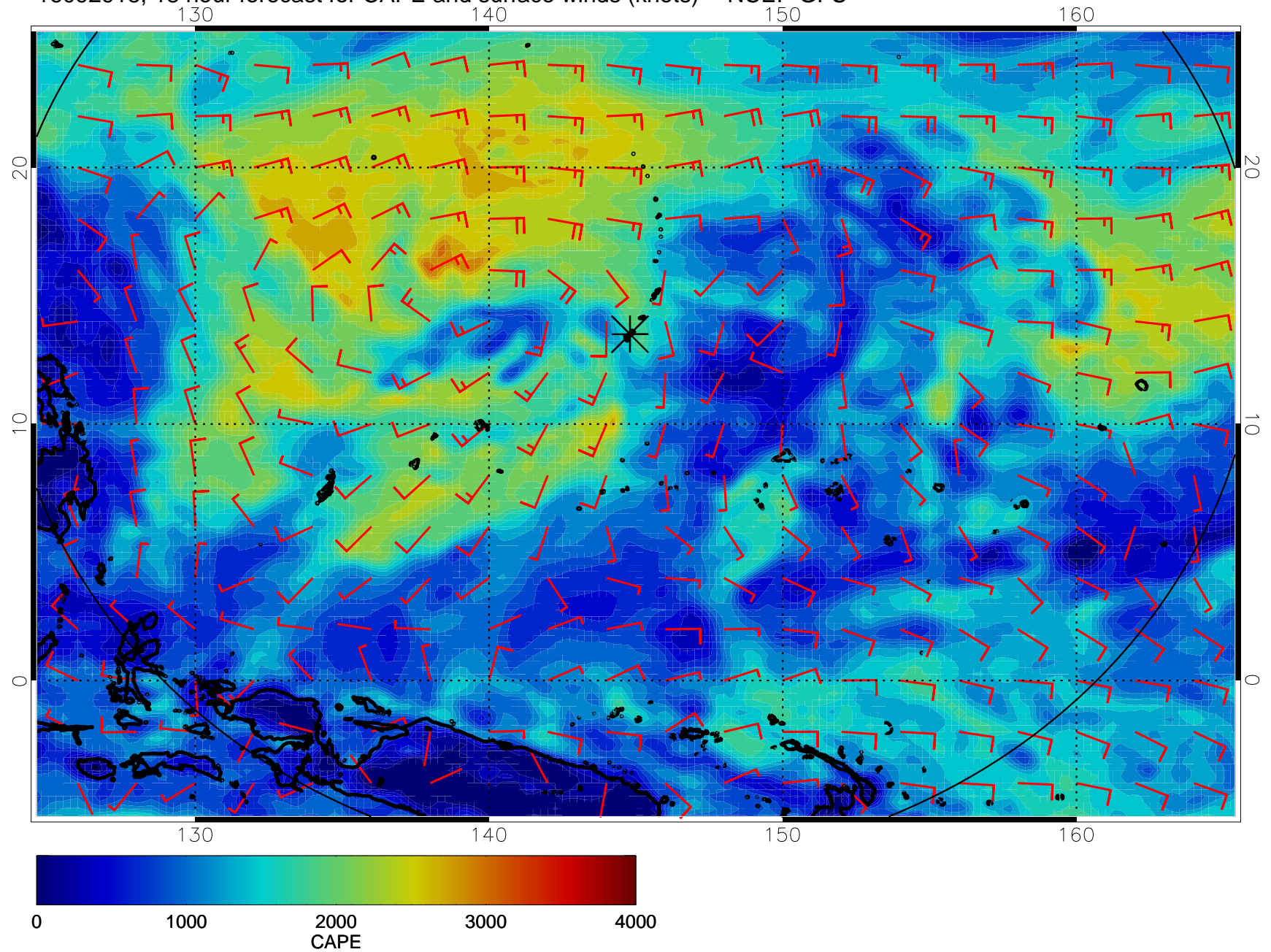
16092918, 18 hour forecast for CAPE and surface winds (knots) -- NCEP GFS
