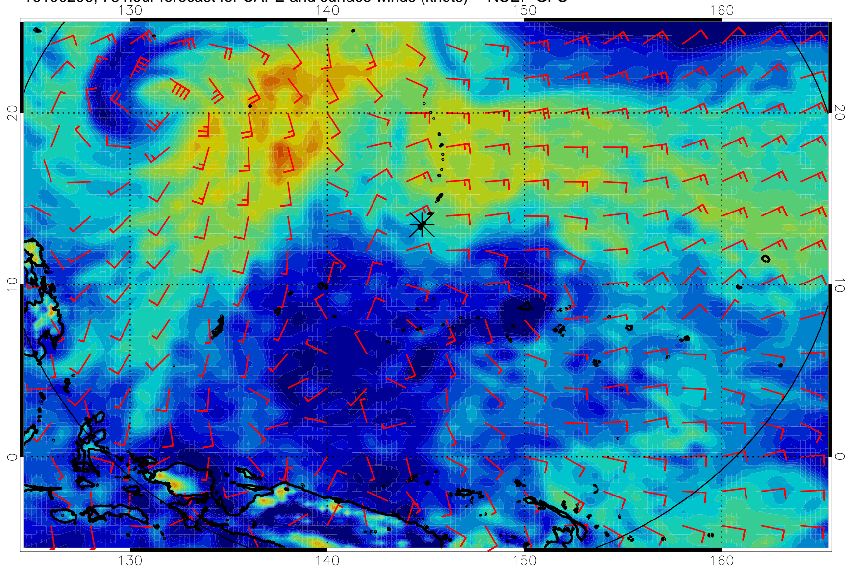
16100206, 78 hour forecast for CAPE and surface winds (knots) -- NCEP GFS
