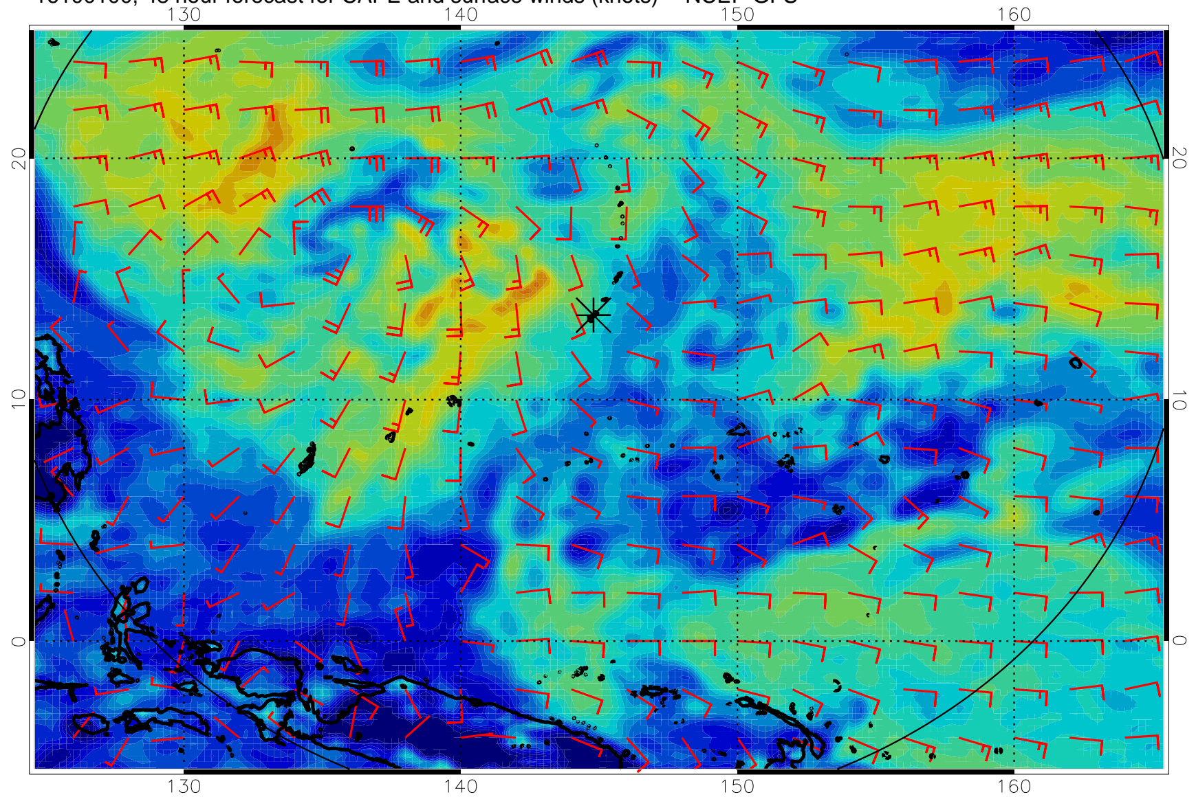
16100100, 48 hour forecast for CAPE and surface winds (knots) -- NCEP GFS
