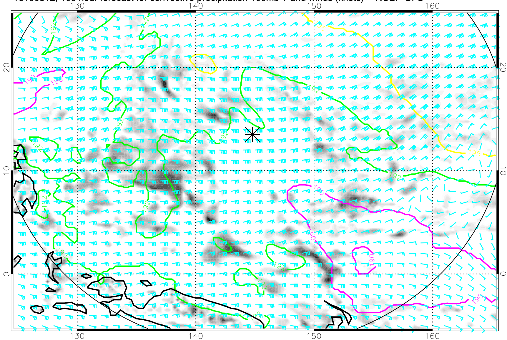
16100312, 108 hour forecast for convective precipitation 100mb T and winds (knots) -- NCEP GFS
