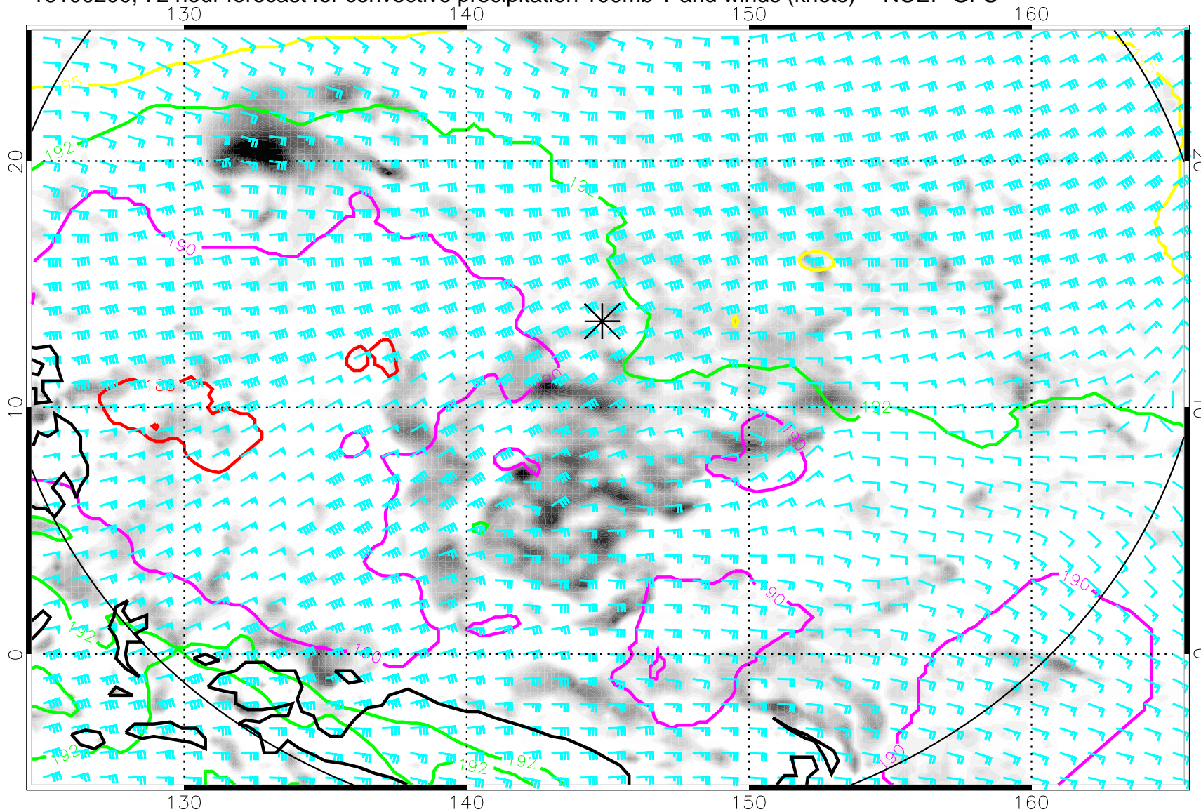
16100200, 72 hour forecast for convective precipitation 100mb T and winds (knots) -- NCEP GFS
