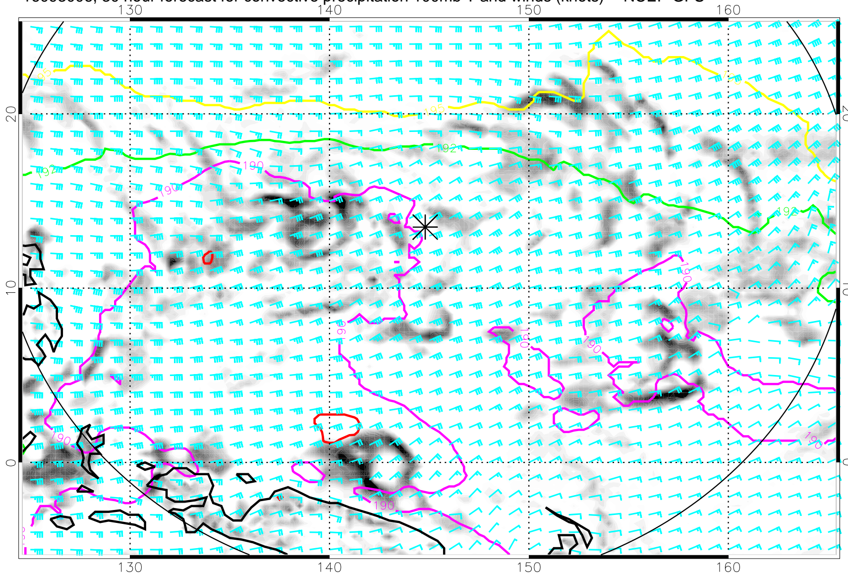
16093006, 30 hour forecast for convective precipitation 100mb T and winds (knots) -- NCEP GFS
