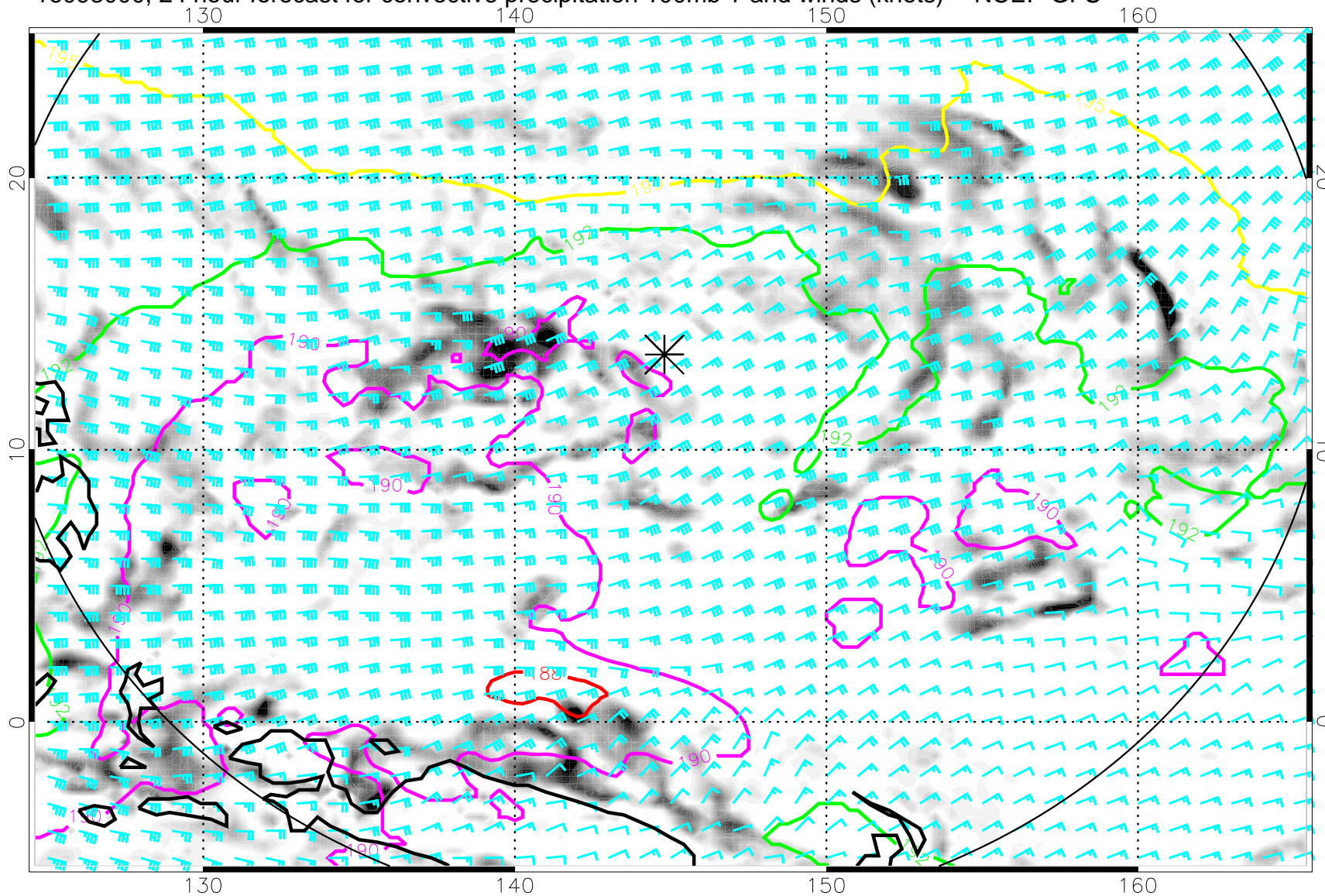
16093000, 24 hour forecast for convective precipitation 100mb T and winds (knots) -- NCEP GFS
