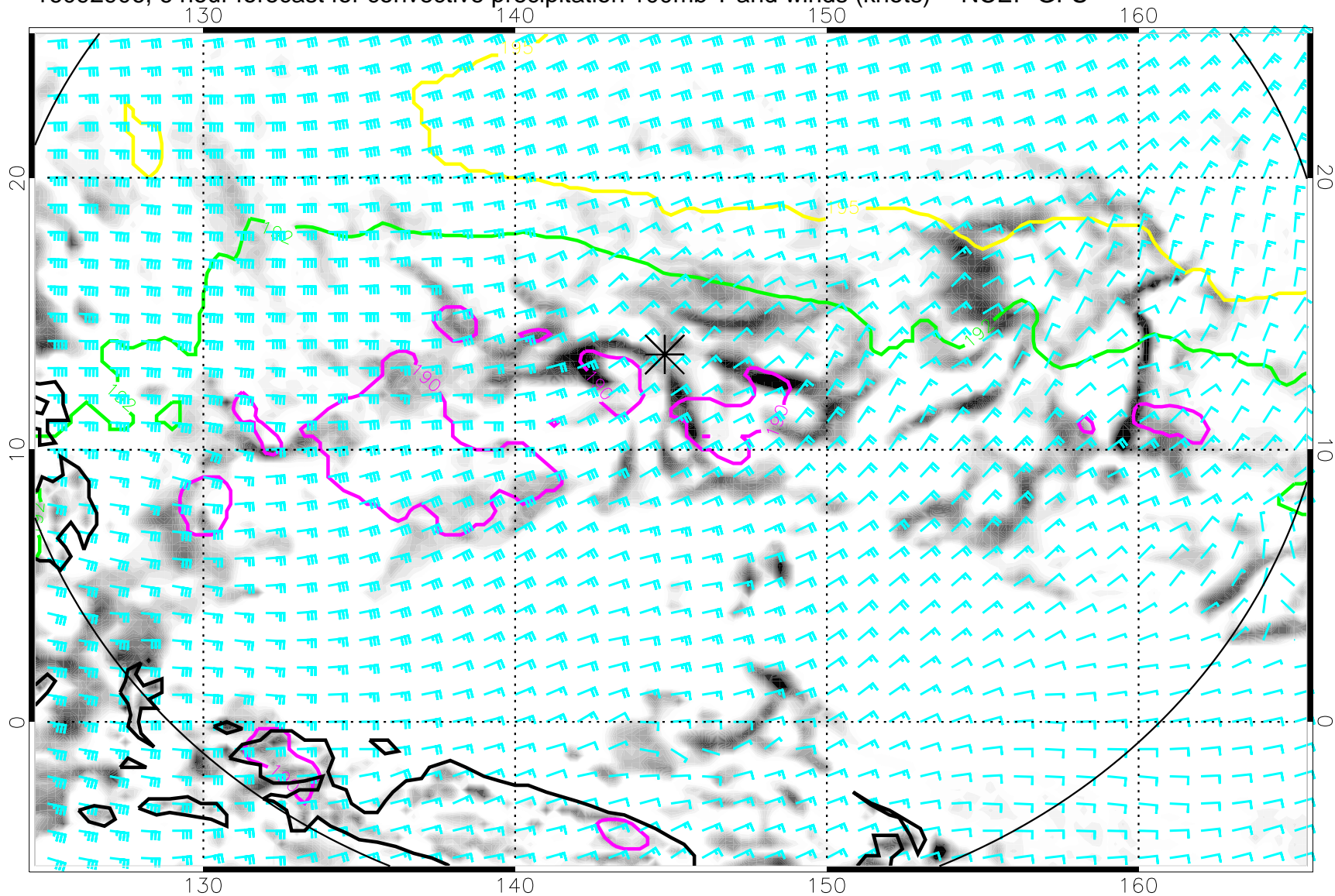
16092906, 6 hour forecast for convective precipitation 100mb T and winds (knots) -- NCEP GFS
