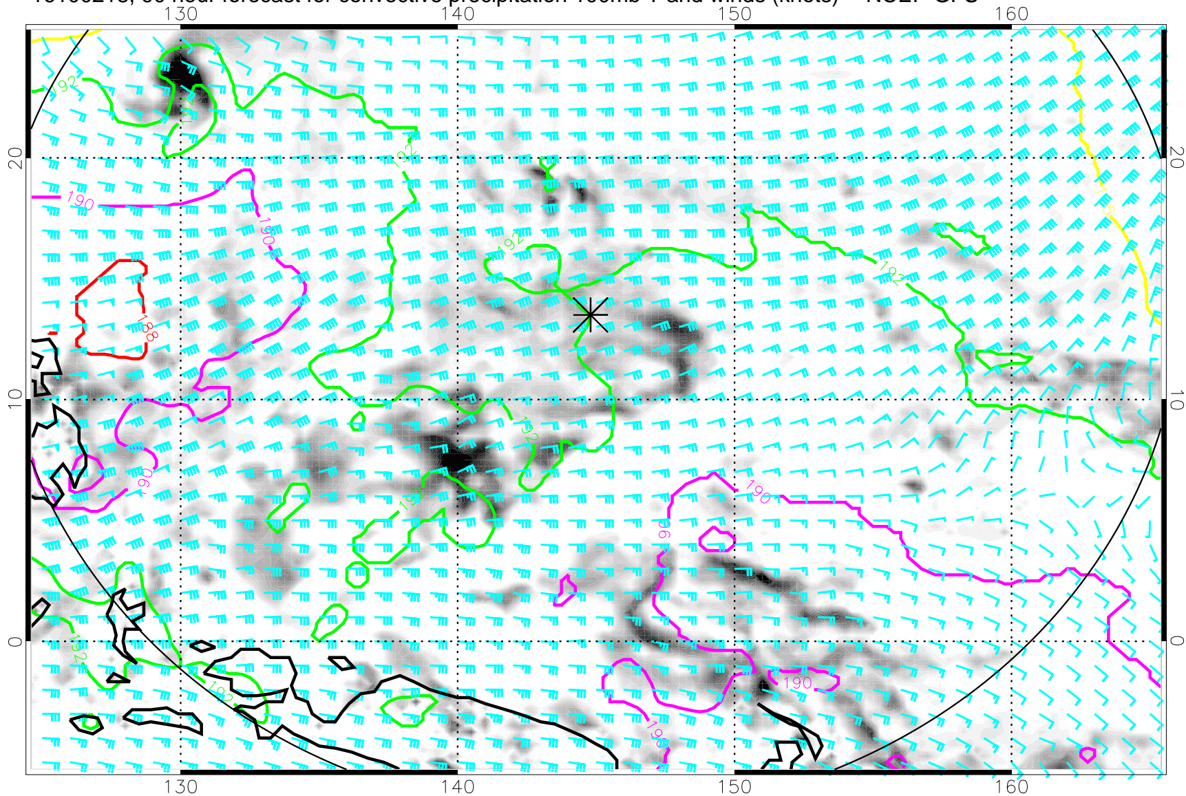
16100218, 90 hour forecast for convective precipitation 100mb T and winds (knots) -- NCEP GFS
