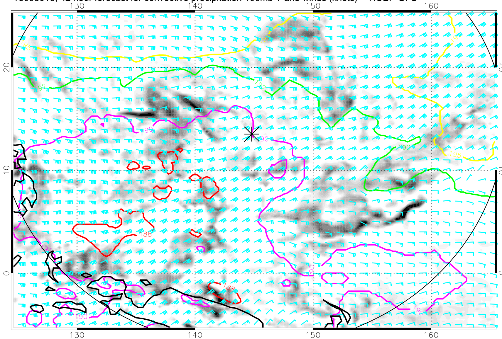
16093018, 42 hour forecast for convective precipitation 100mb T and winds (knots) -- NCEP GFS
