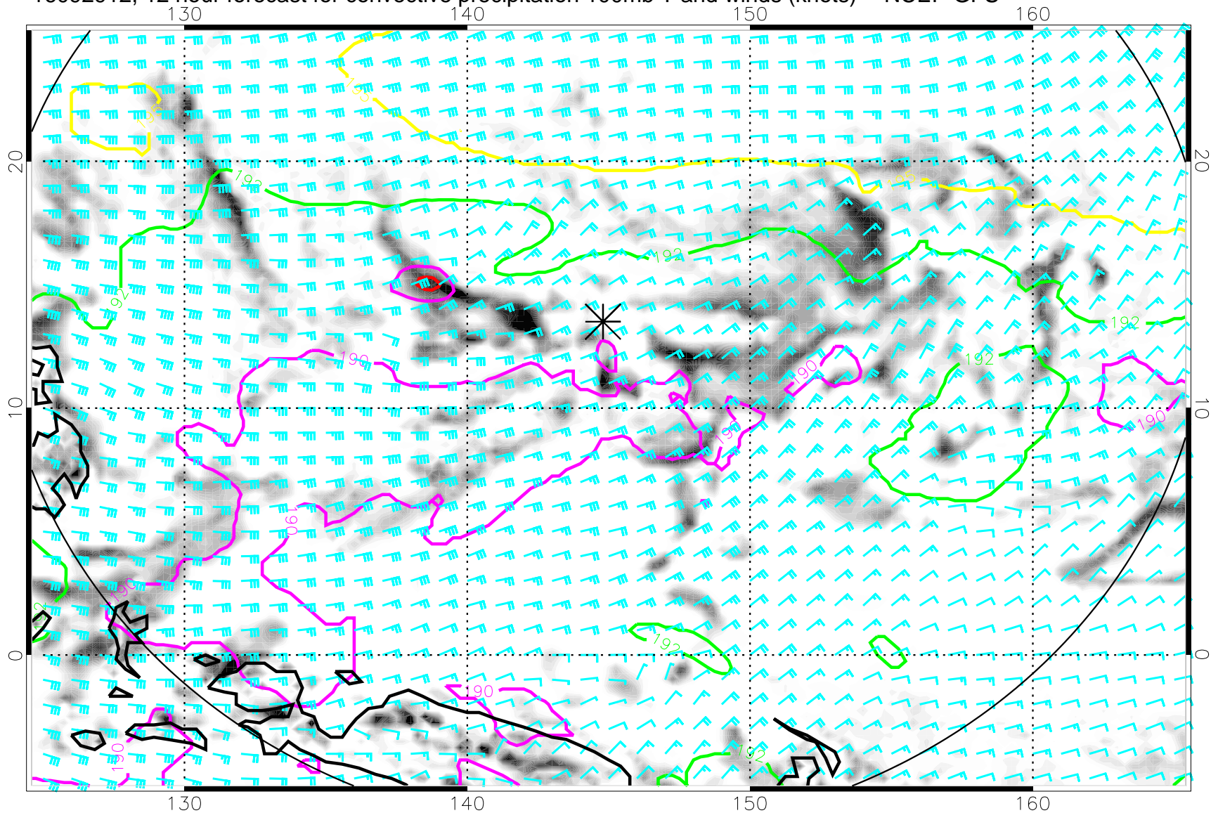
16092912, 12 hour forecast for convective precipitation 100mb T and winds (knots) -- NCEP GFS
