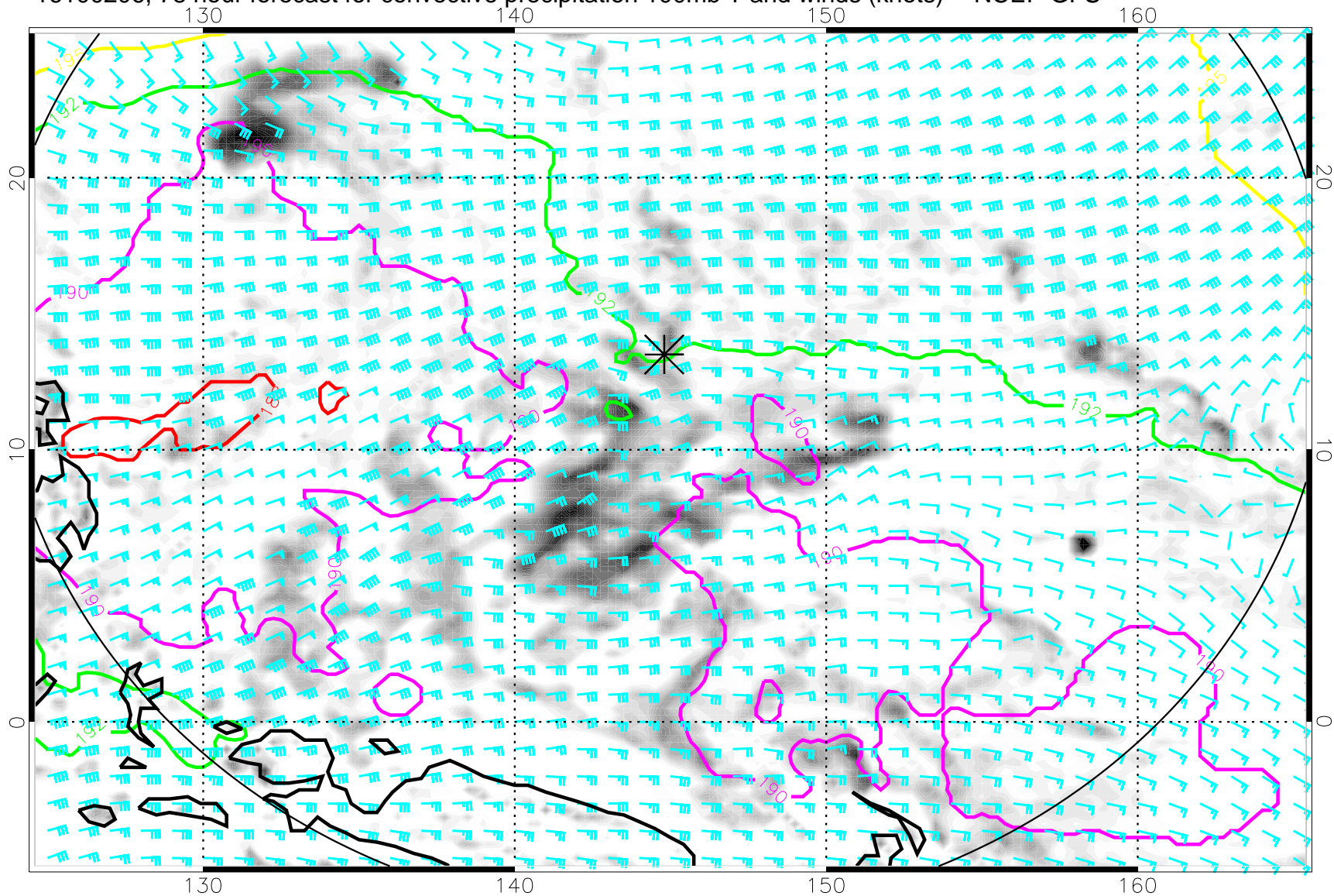
16100206, 78 hour forecast for convective precipitation 100mb T and winds (knots) -- NCEP GFS
