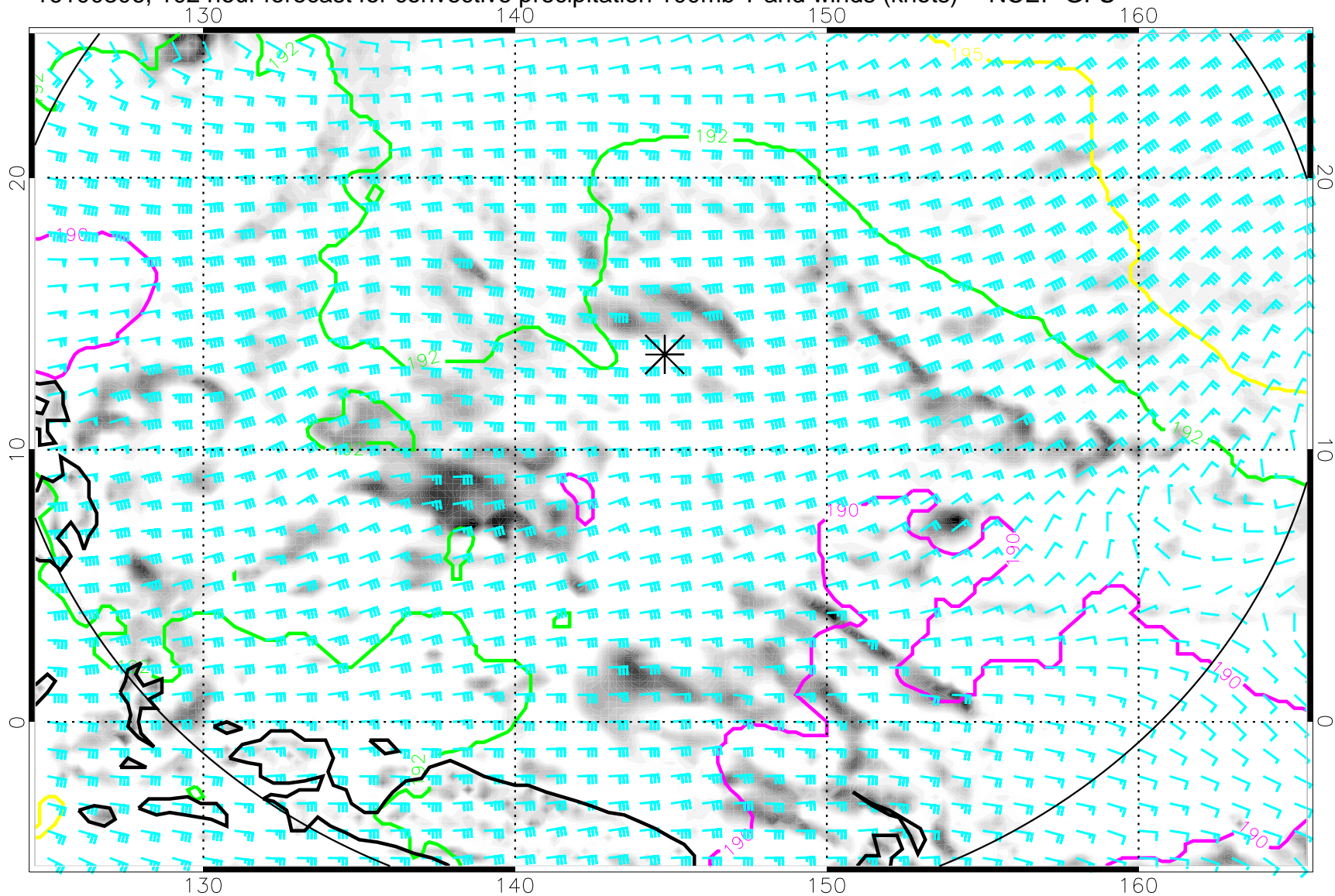
16100306, 102 hour forecast for convective precipitation 100mb T and winds (knots) -- NCEP GFS
