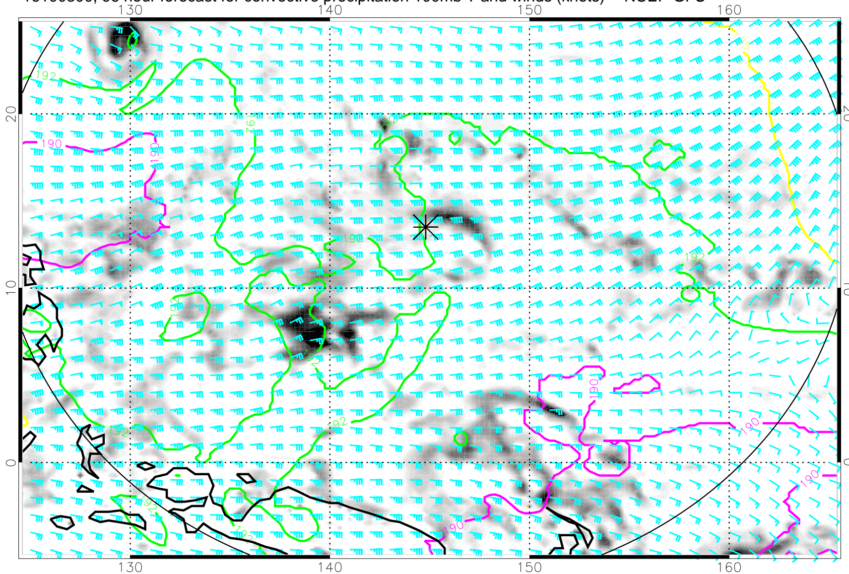
16100300, 96 hour forecast for convective precipitation 100mb T and winds (knots) -- NCEP GFS
