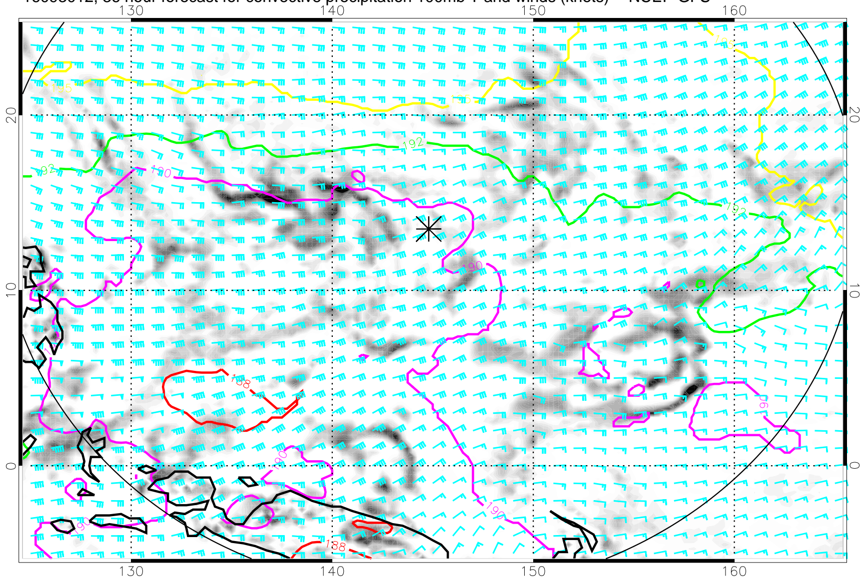
16093012, 36 hour forecast for convective precipitation 100mb T and winds (knots) -- NCEP GFS
