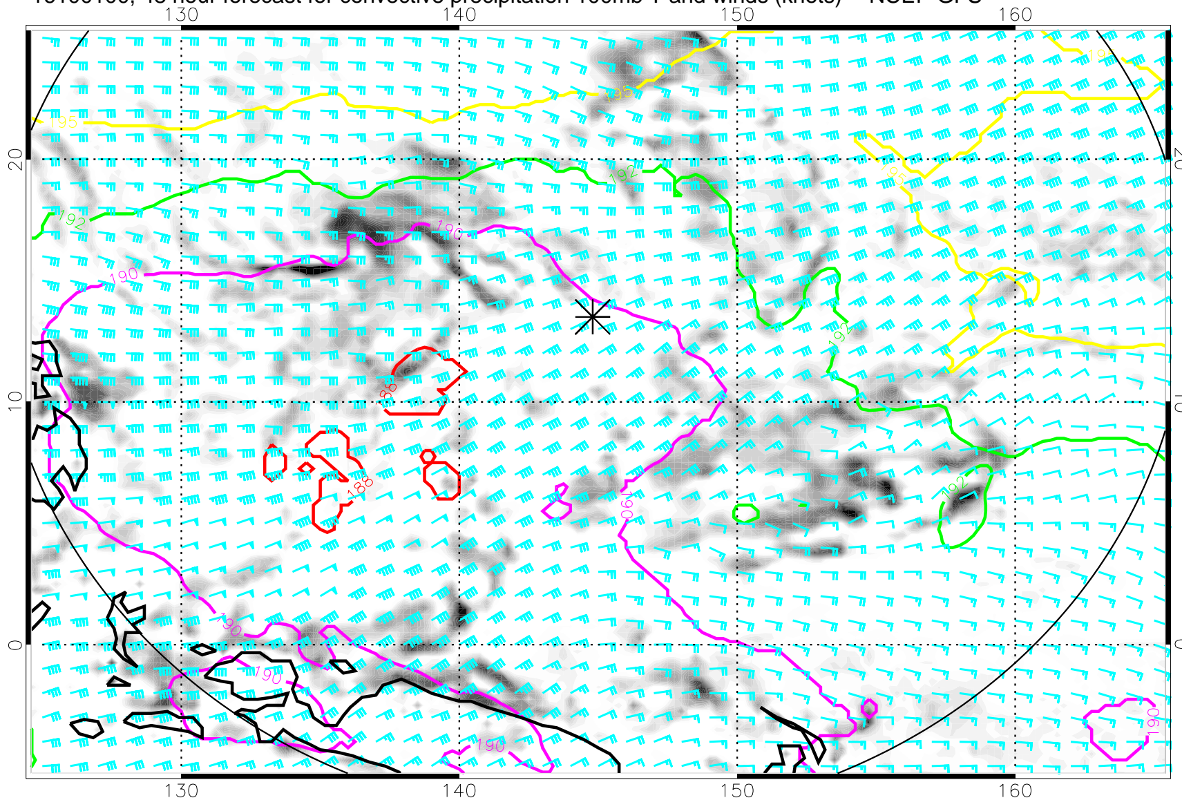
16100100, 48 hour forecast for convective precipitation 100mb T and winds (knots) -- NCEP GFS
