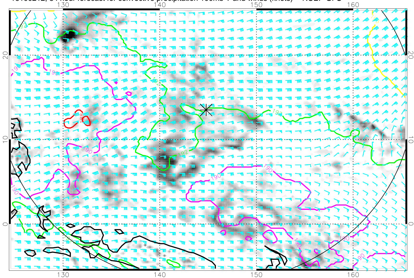
16100212, 84 hour forecast for convective precipitation 100mb T and winds (knots) -- NCEP GFS
