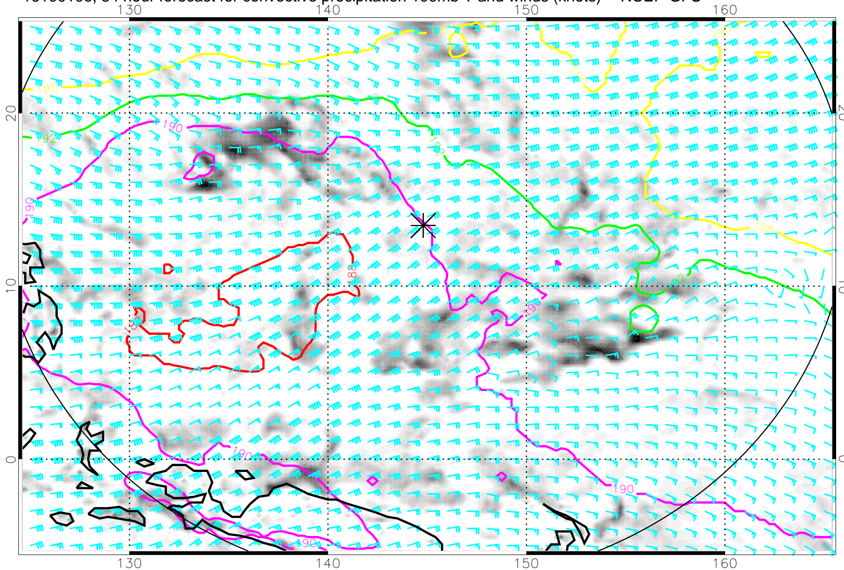
16100106, 54 hour forecast for convective precipitation 100mb T and winds (knots) -- NCEP GFS
