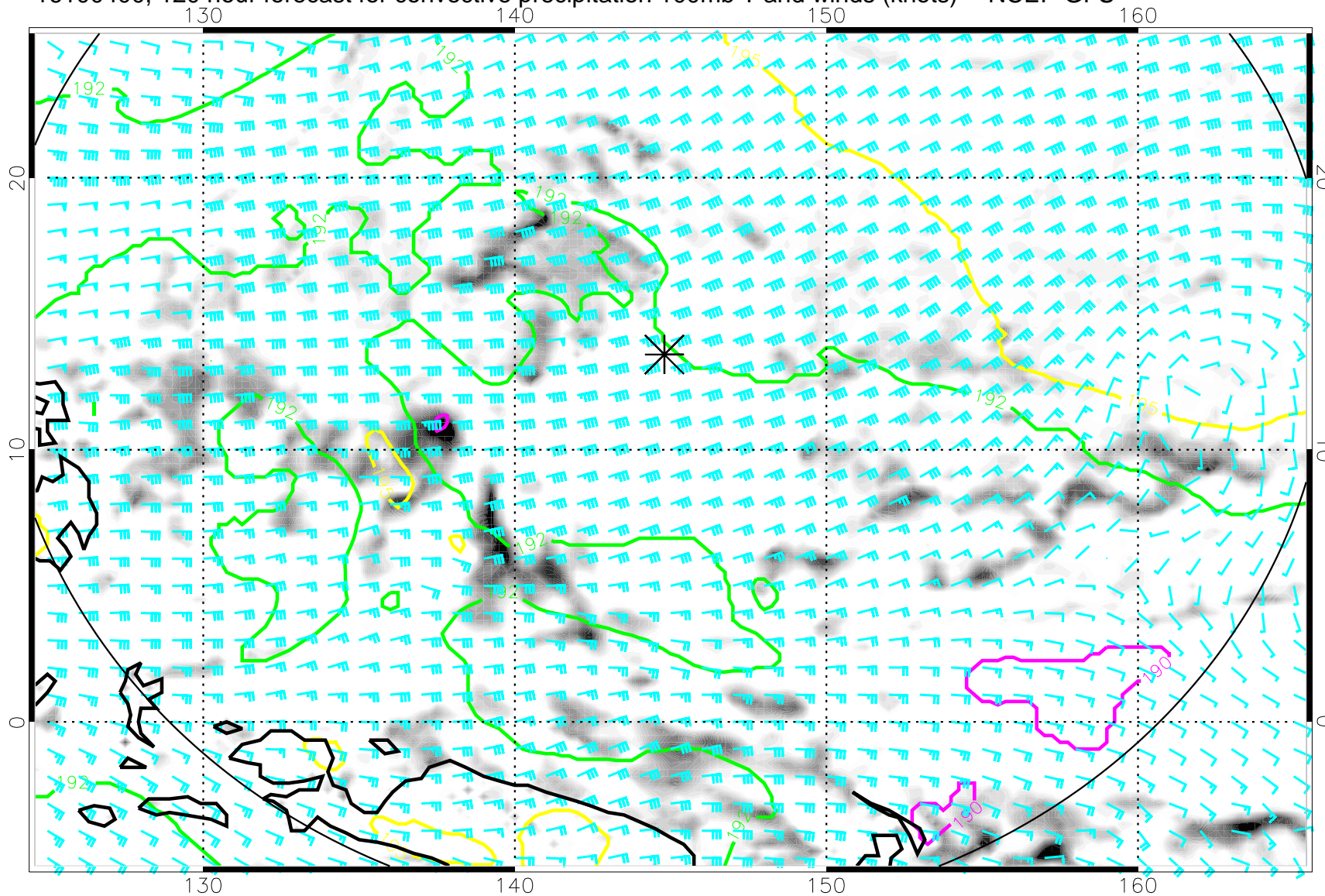
16100400, 120 hour forecast for convective precipitation 100mb T and winds (knots) -- NCEP GFS
