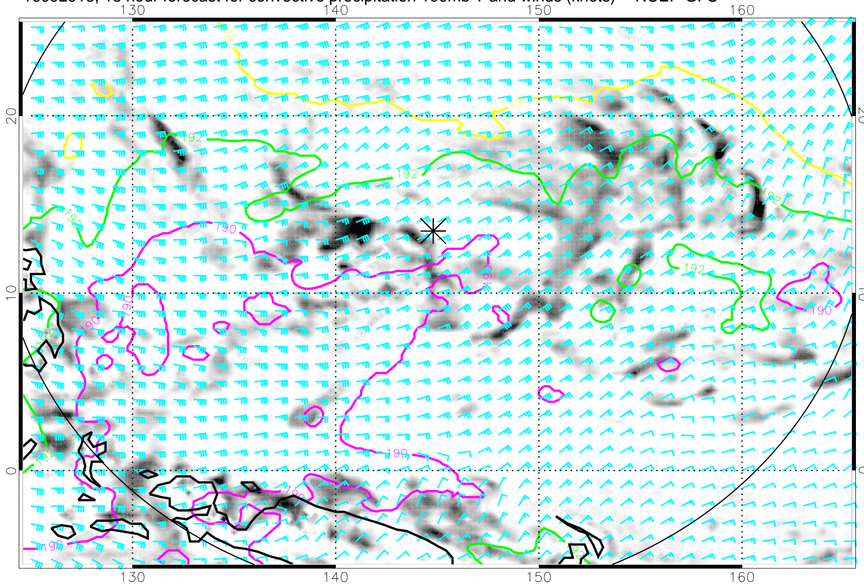
16092918, 18 hour forecast for convective precipitation 100mb T and winds (knots) -- NCEP GFS
