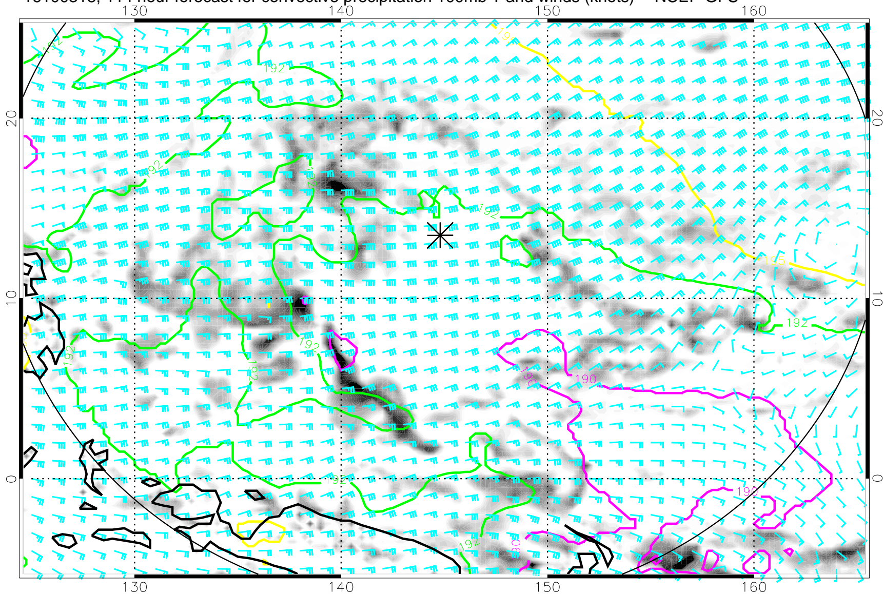
16100318, 114 hour forecast for convective precipitation 100mb T and winds (knots) -- NCEP GFS
