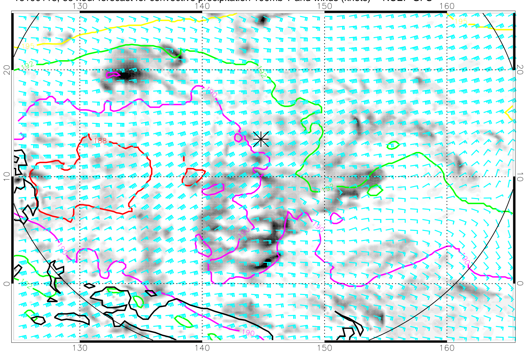
16100118, 66 hour forecast for convective precipitation 100mb T and winds (knots) -- NCEP GFS
