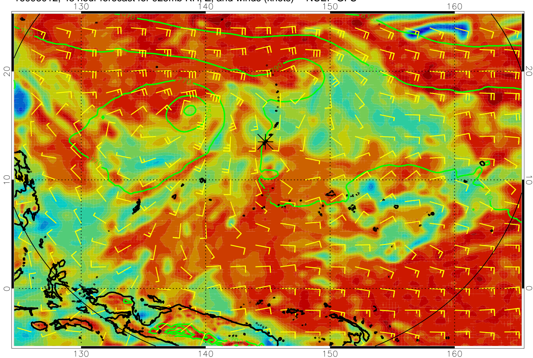
16093012, 48 hour forecast for 925mb RH, Z, and winds (knots) -- NCEP GFS
