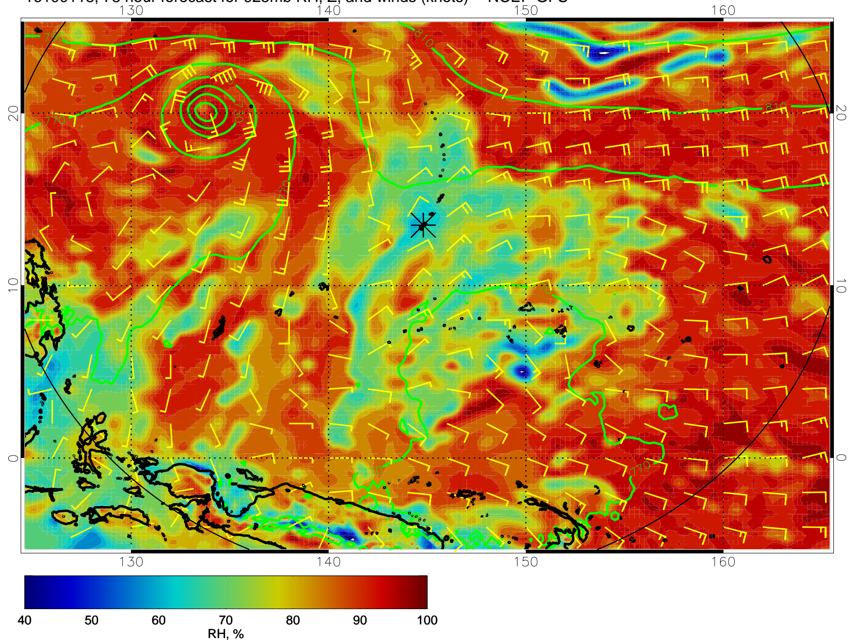
16100118, 78 hour forecast for 925mb RH, Z, and winds (knots) -- NCEP GFS
