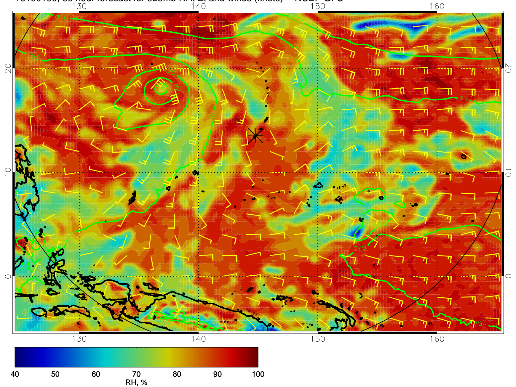
16100100, 60 hour forecast for 925mb RH, Z, and winds (knots) -- NCEP GFS
