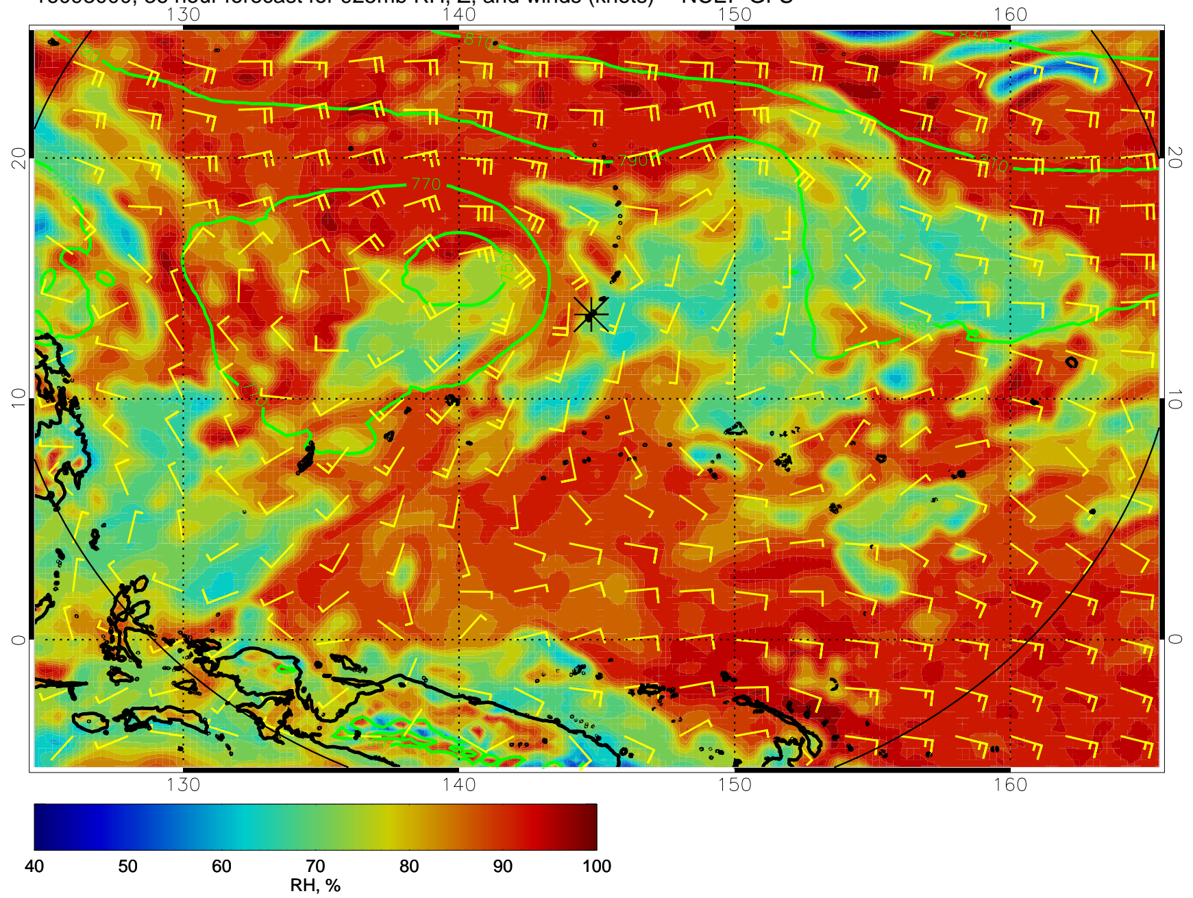
16093000, 36 hour forecast for 925mb RH, Z, and winds (knots) -- NCEP GFS
