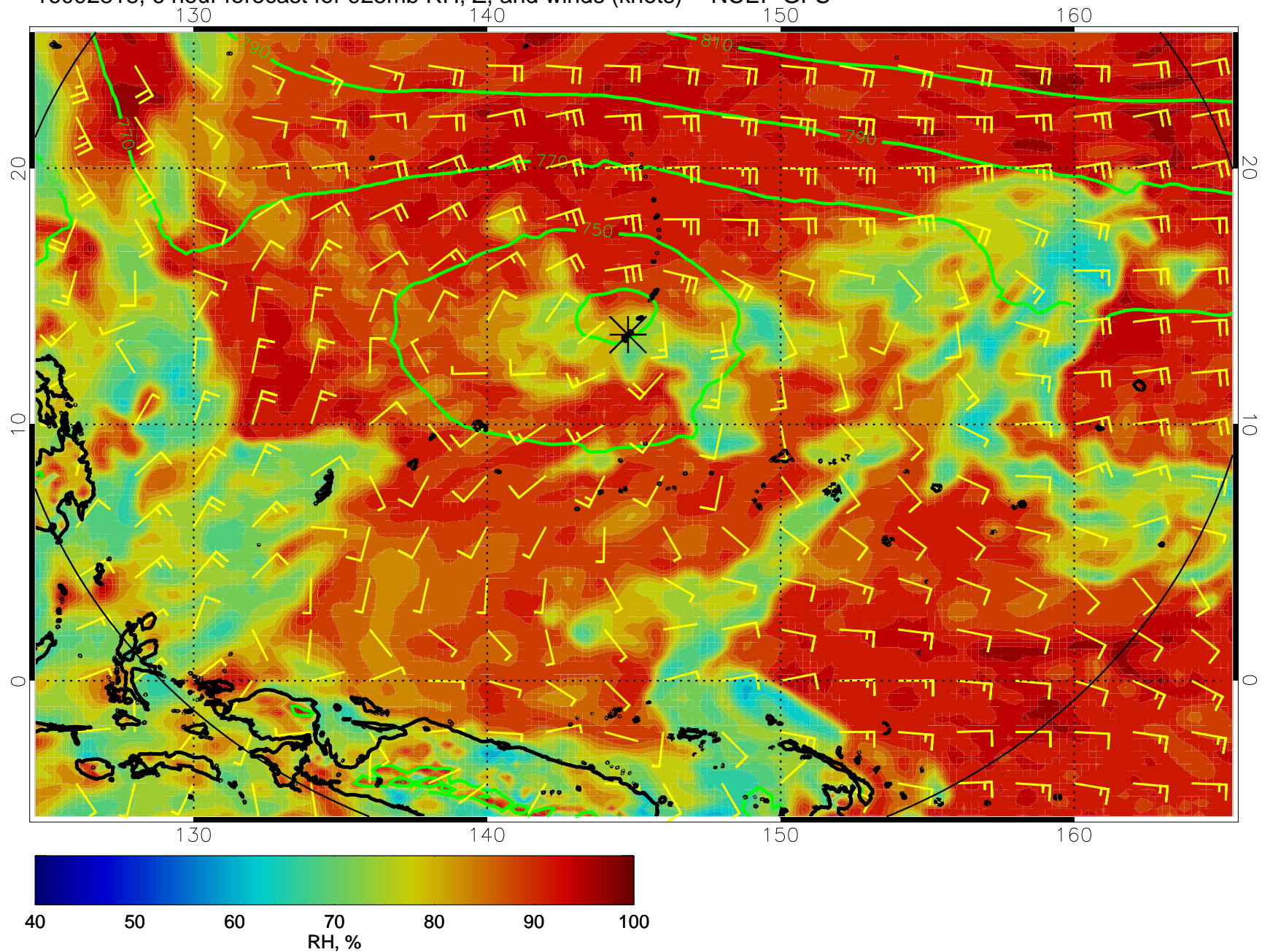
16092818, 6 hour forecast for 925mb RH, Z, and winds (knots) -- NCEP GFS
