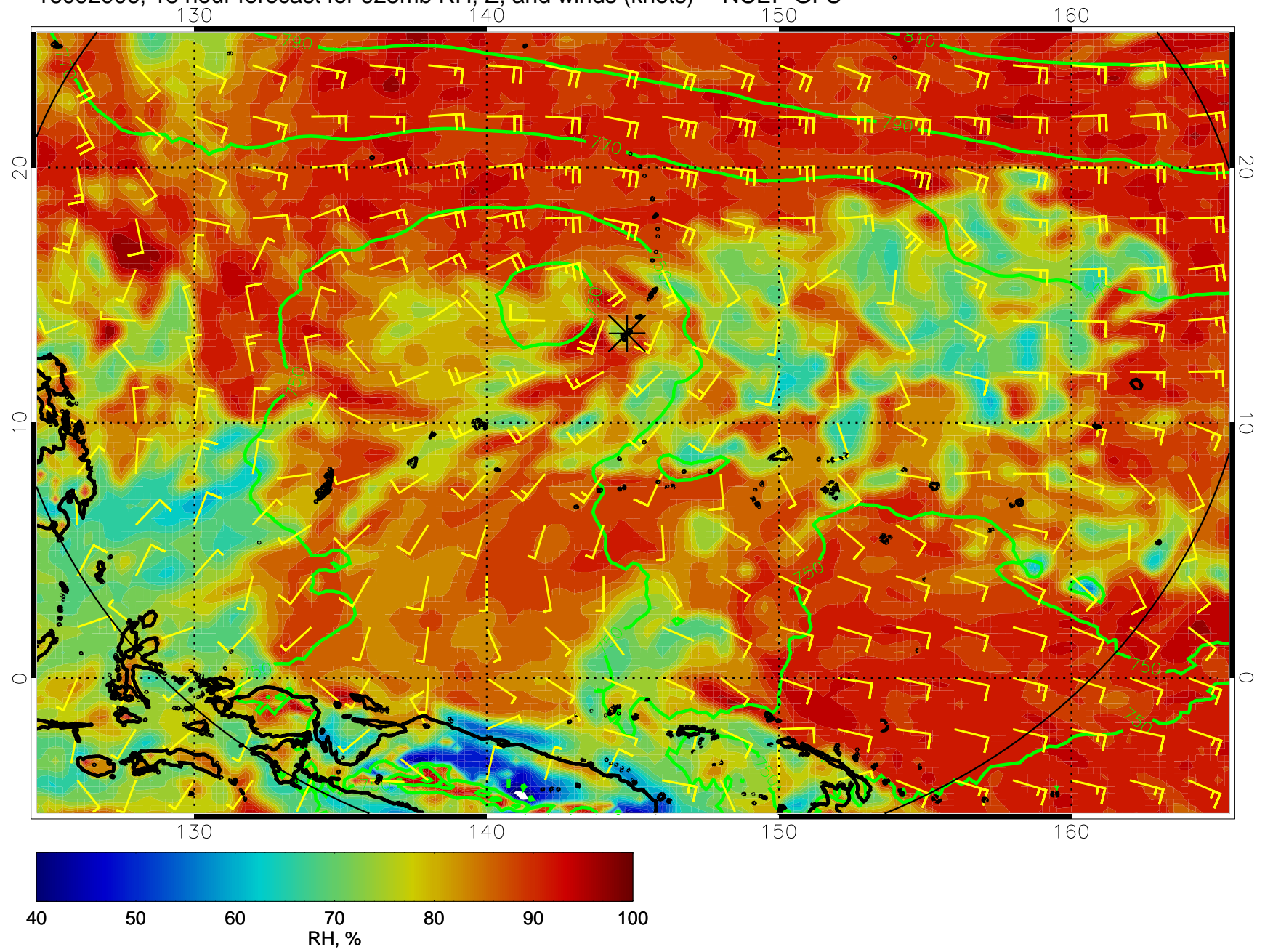
16092906, 18 hour forecast for 925mb RH, Z, and winds (knots) -- NCEP GFS
