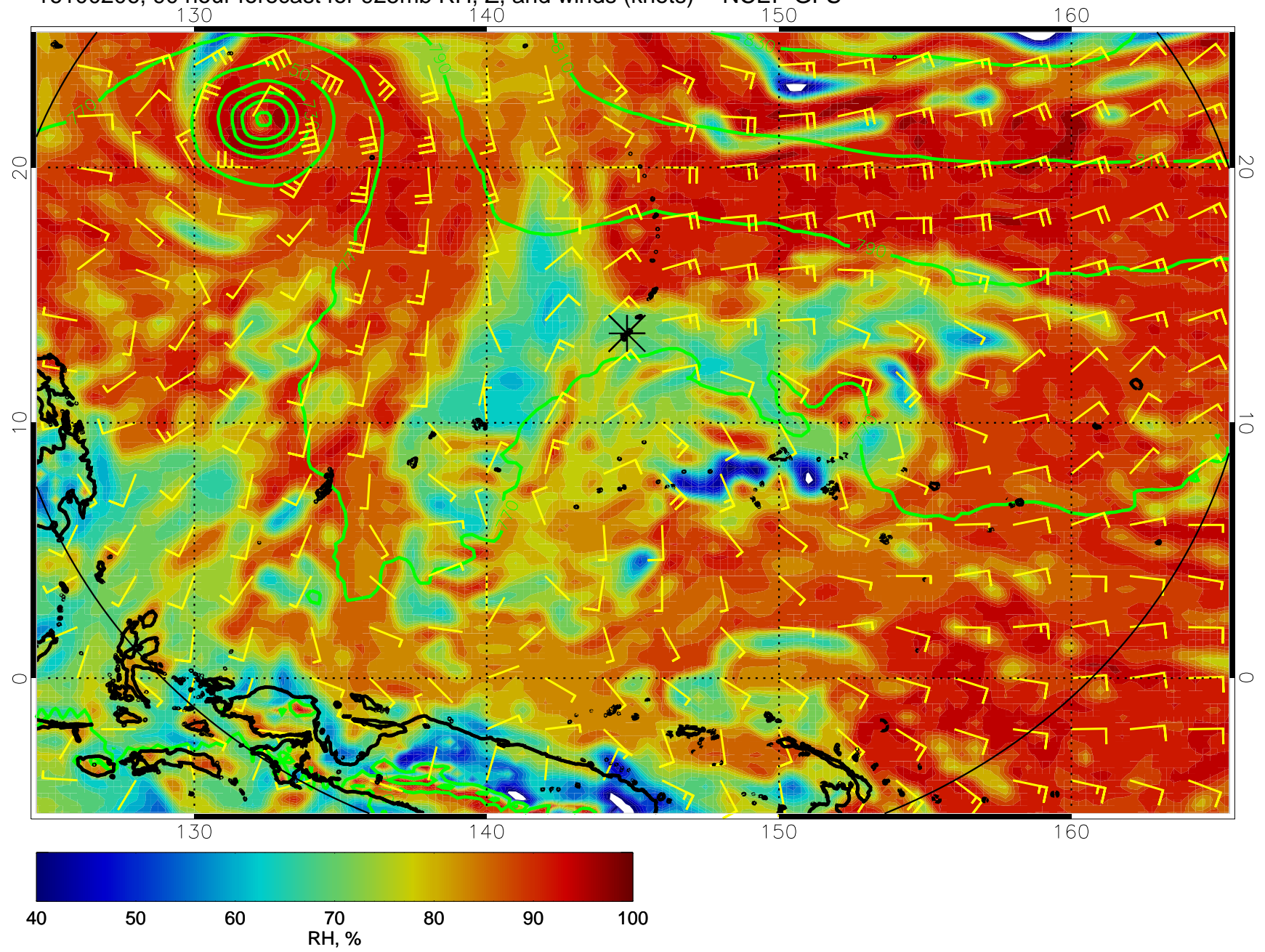
16100206, 90 hour forecast for 925mb RH, Z, and winds (knots) -- NCEP GFS
