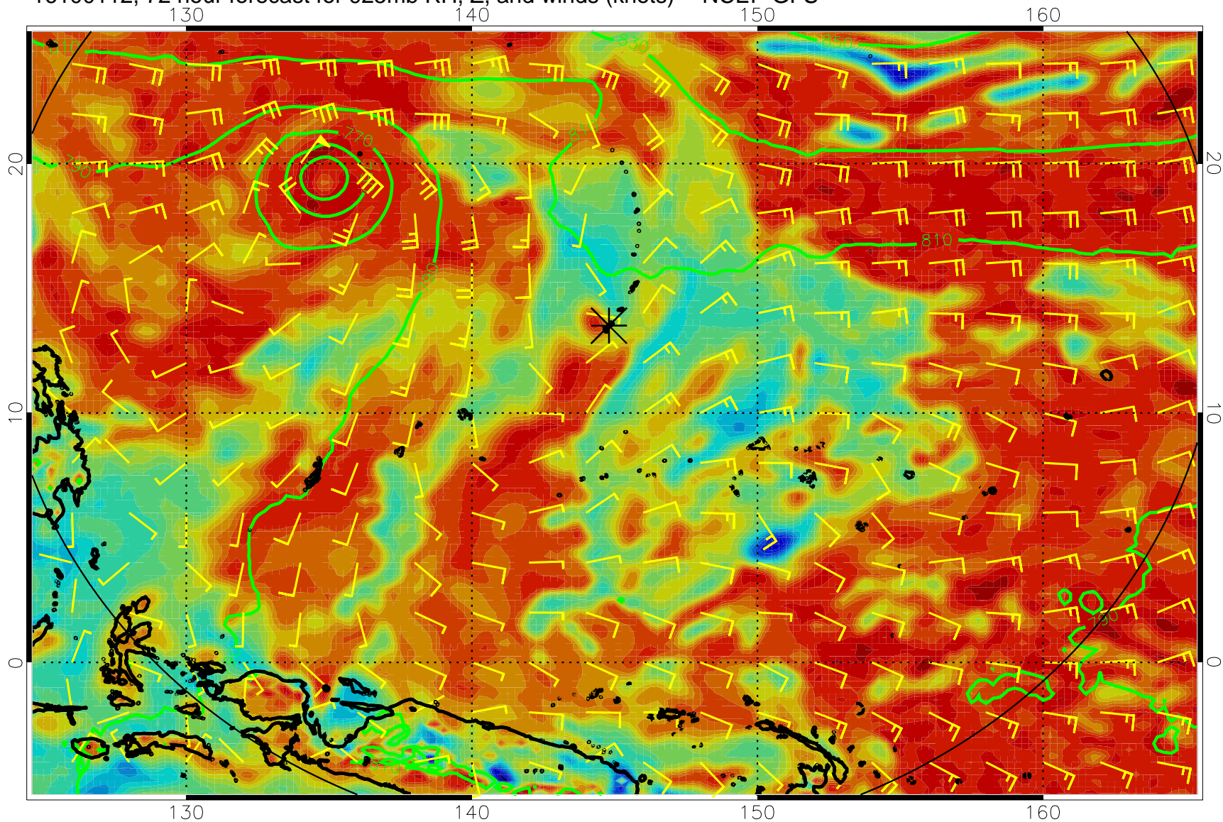
16100112, 72 hour forecast for 925mb RH, Z, and winds (knots) -- NCEP GFS
