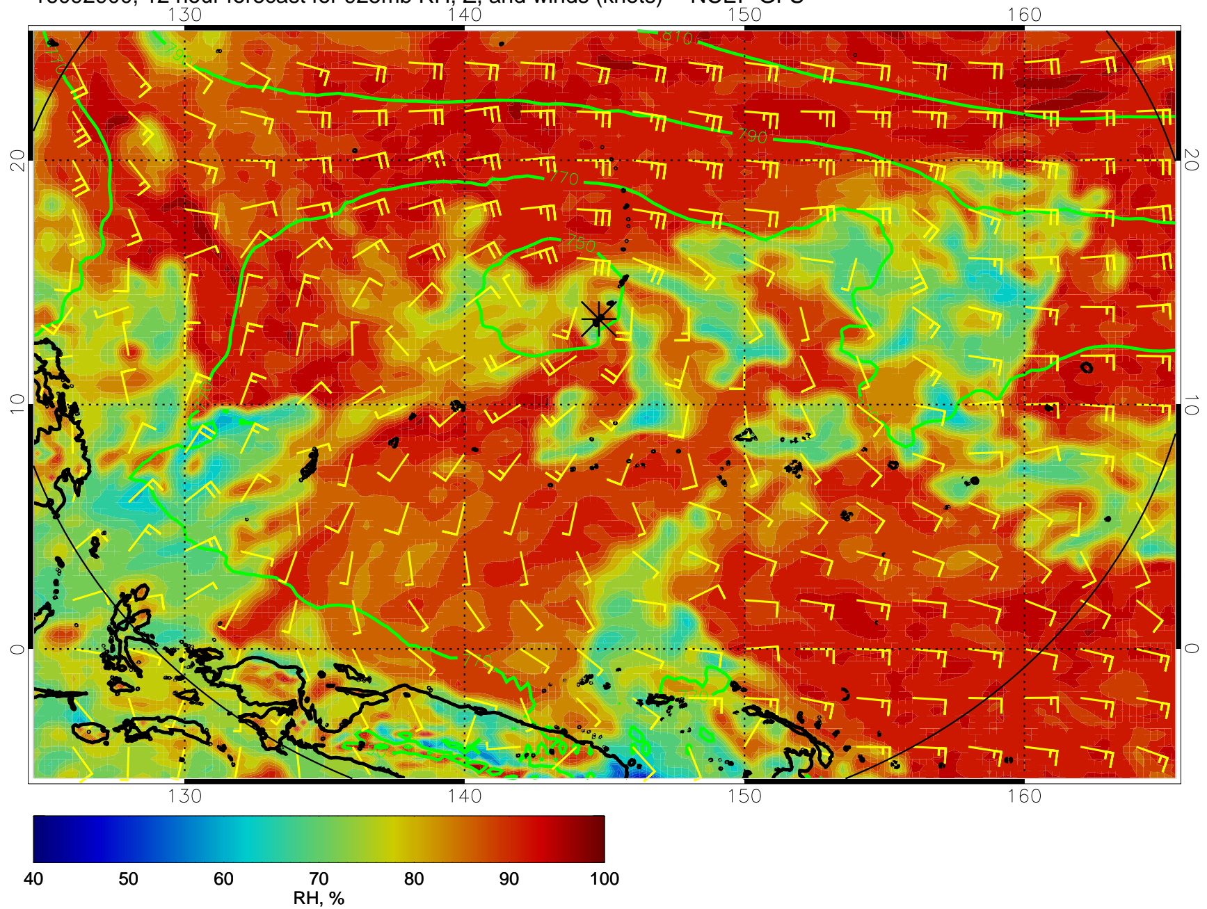
16092900, 12 hour forecast for 925mb RH, Z, and winds (knots) -- NCEP GFS
