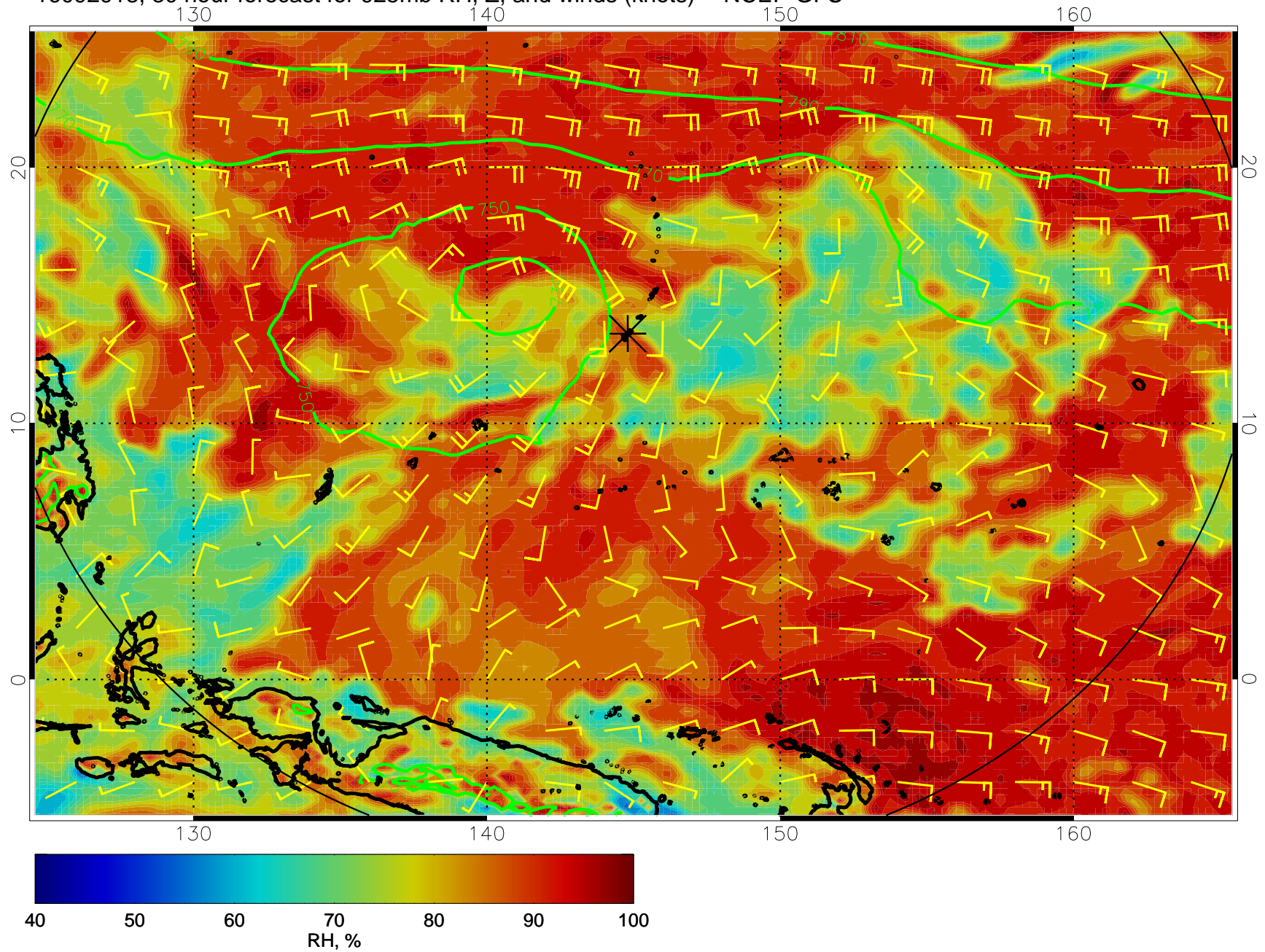
16092918, 30 hour forecast for 925mb RH, Z, and winds (knots) -- NCEP GFS
