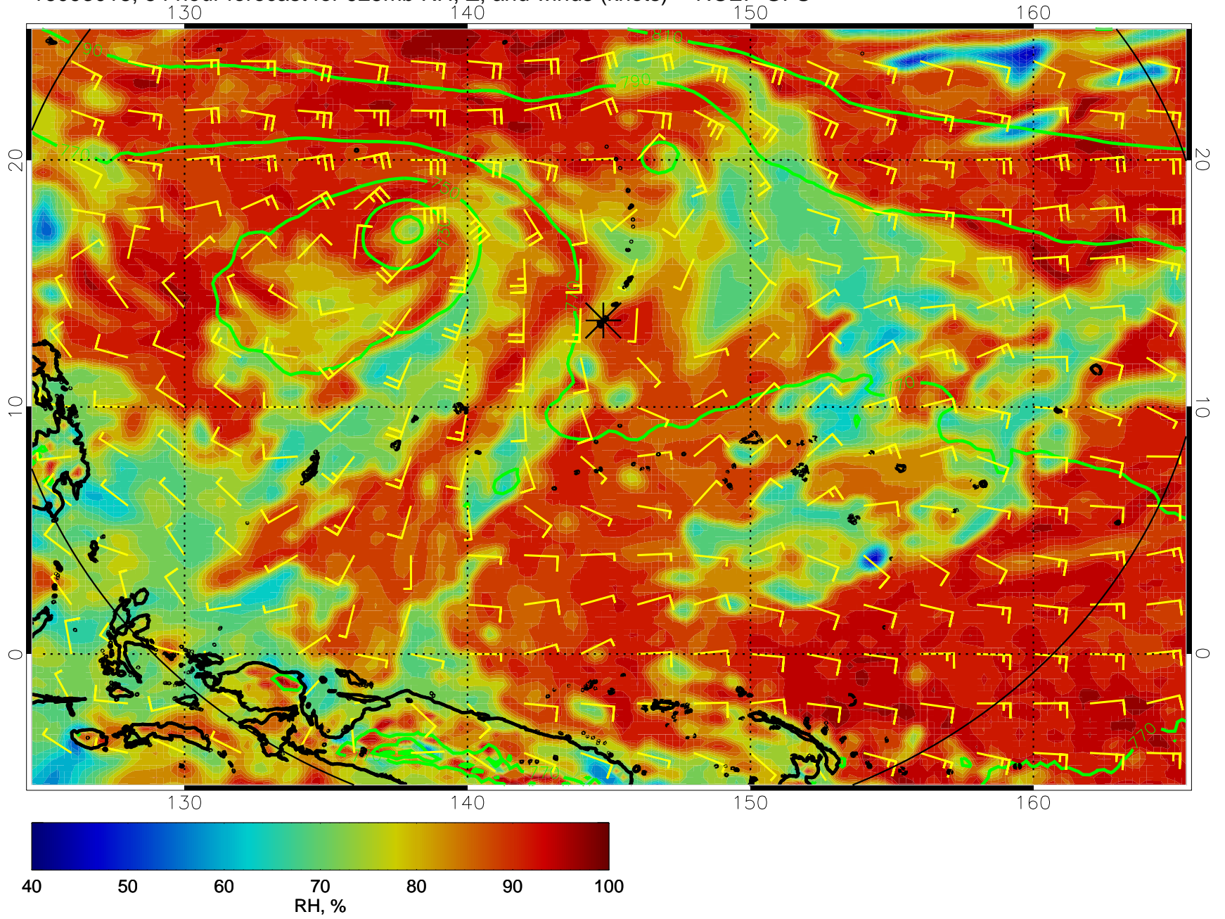
16093018, 54 hour forecast for 925mb RH, Z, and winds (knots) -- NCEP GFS
