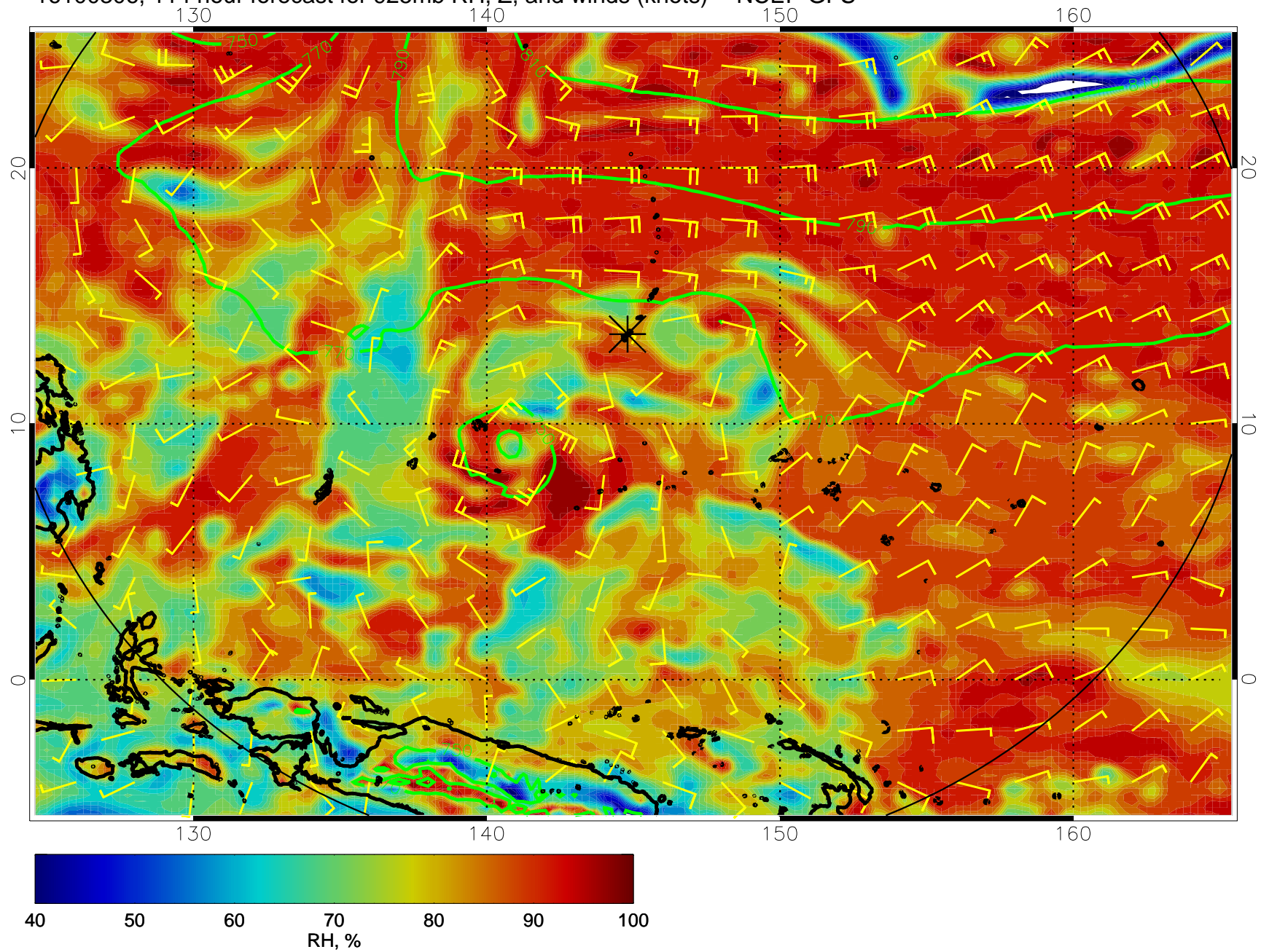
16100306, 114 hour forecast for 925mb RH, Z, and winds (knots) -- NCEP GFS
