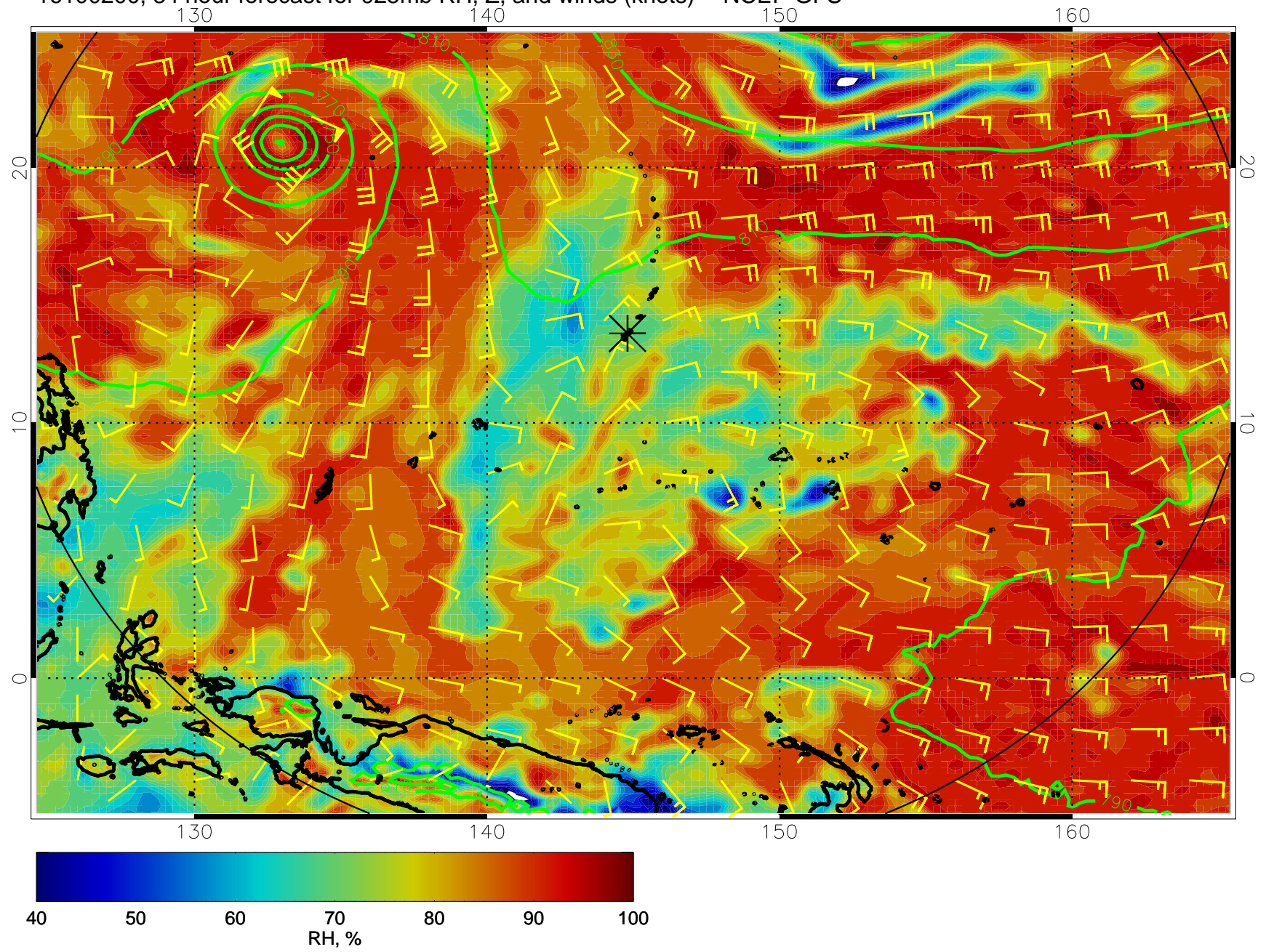
16100200, 84 hour forecast for 925mb RH, Z, and winds (knots) -- NCEP GFS
