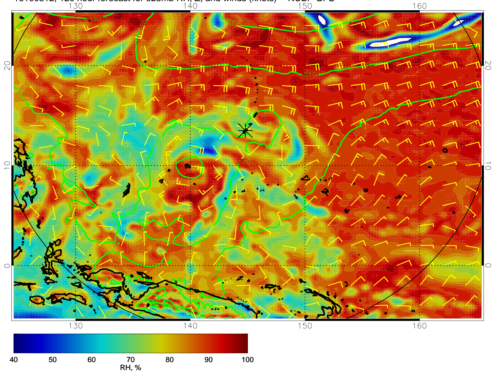
16100312, 120 hour forecast for 925mb RH, Z, and winds (knots) -- NCEP GFS
