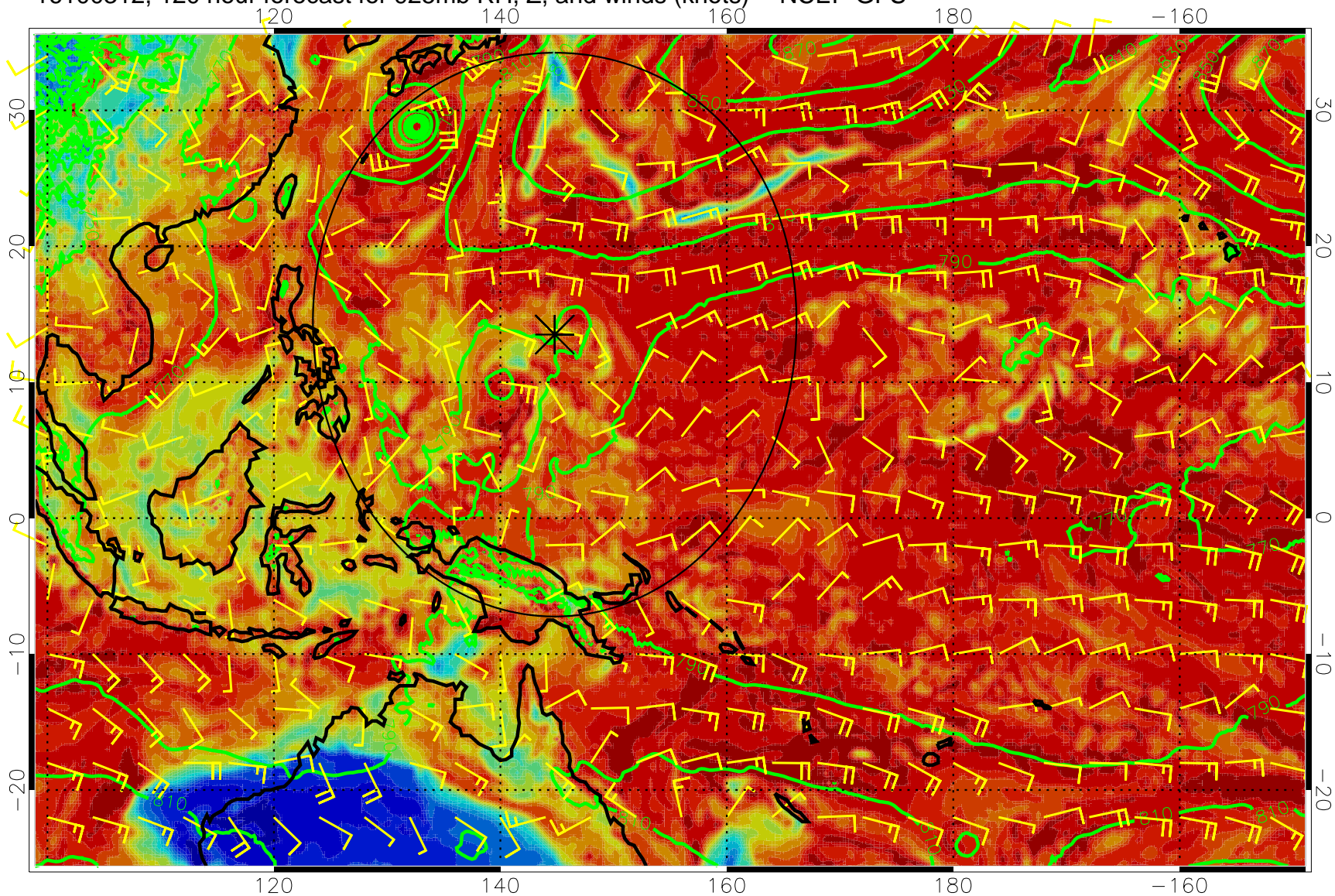
16100312, 120 hour forecast for 925mb RH, Z, and winds (knots) -- NCEP GFS
