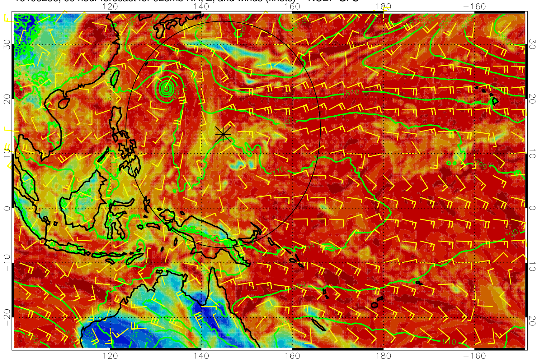
16100206, 90 hour forecast for 925mb RH, Z, and winds (knots) -- NCEP GFS
