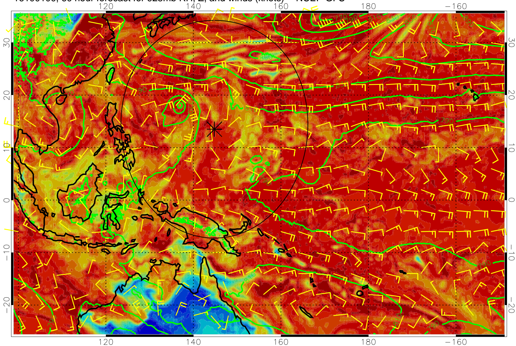
16100100, 60 hour forecast for 925mb RH, Z, and winds (knots) -- NCEP GFS
