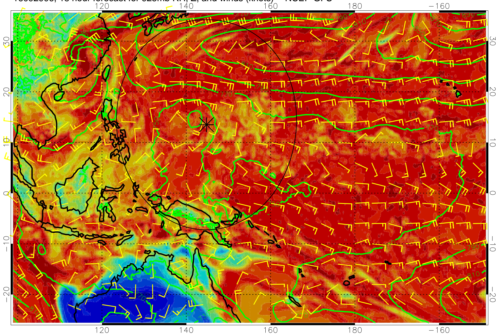
16092906, 18 hour forecast for 925mb RH, Z, and winds (knots) -- NCEP GFS
