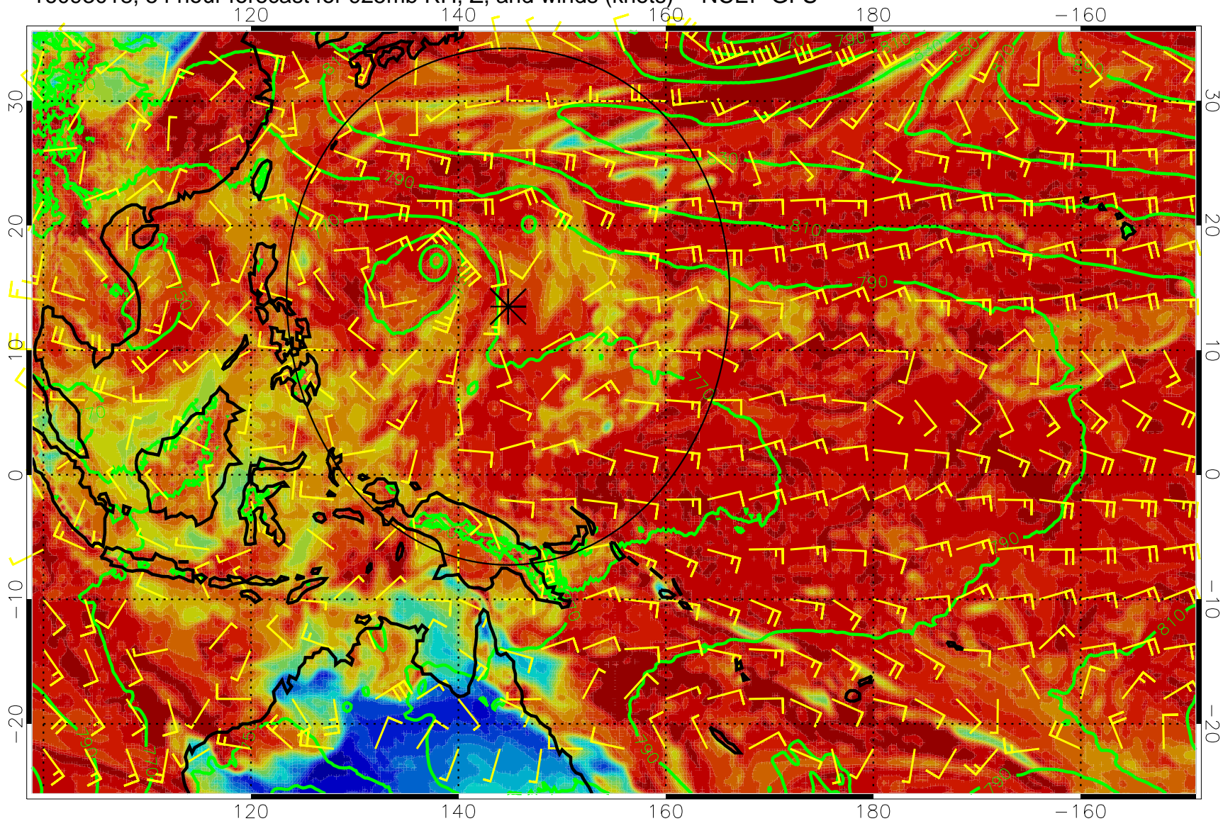
16093018, 54 hour forecast for 925mb RH, Z, and winds (knots) -- NCEP GFS
