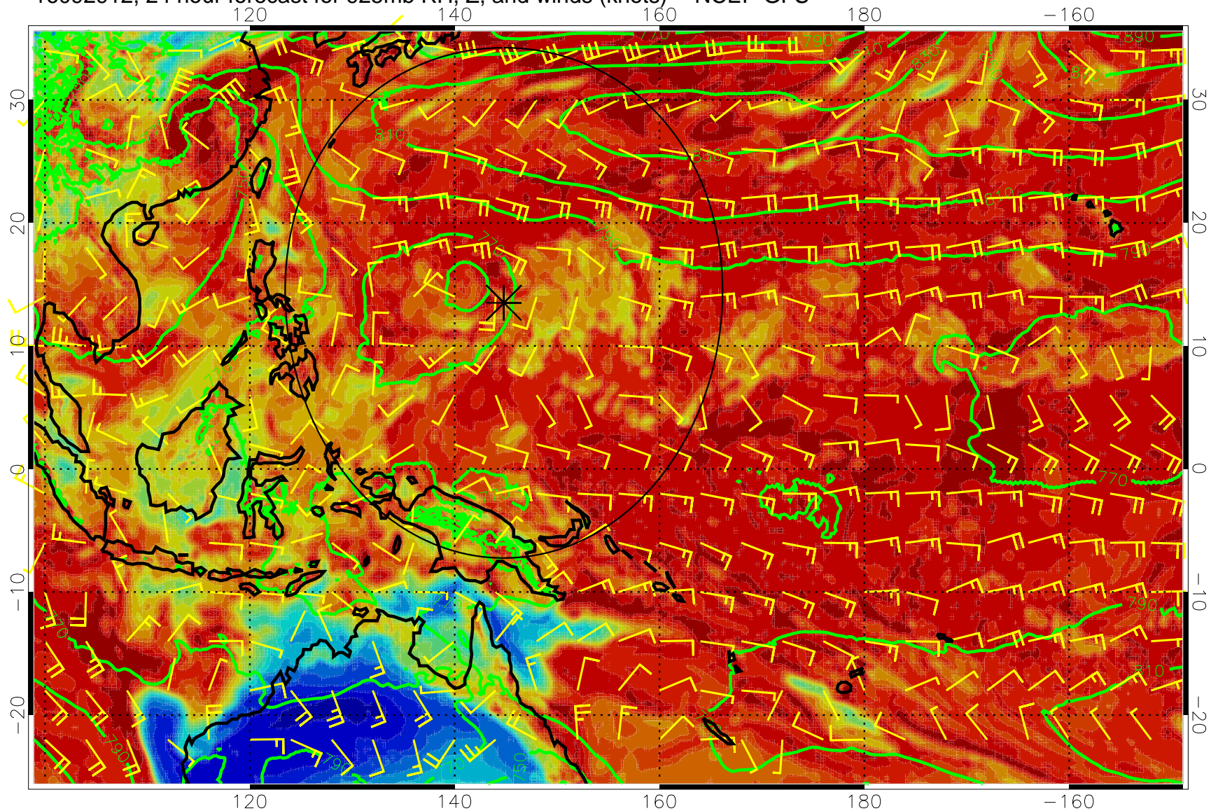
16092912, 24 hour forecast for 925mb RH, Z, and winds (knots) -- NCEP GFS
