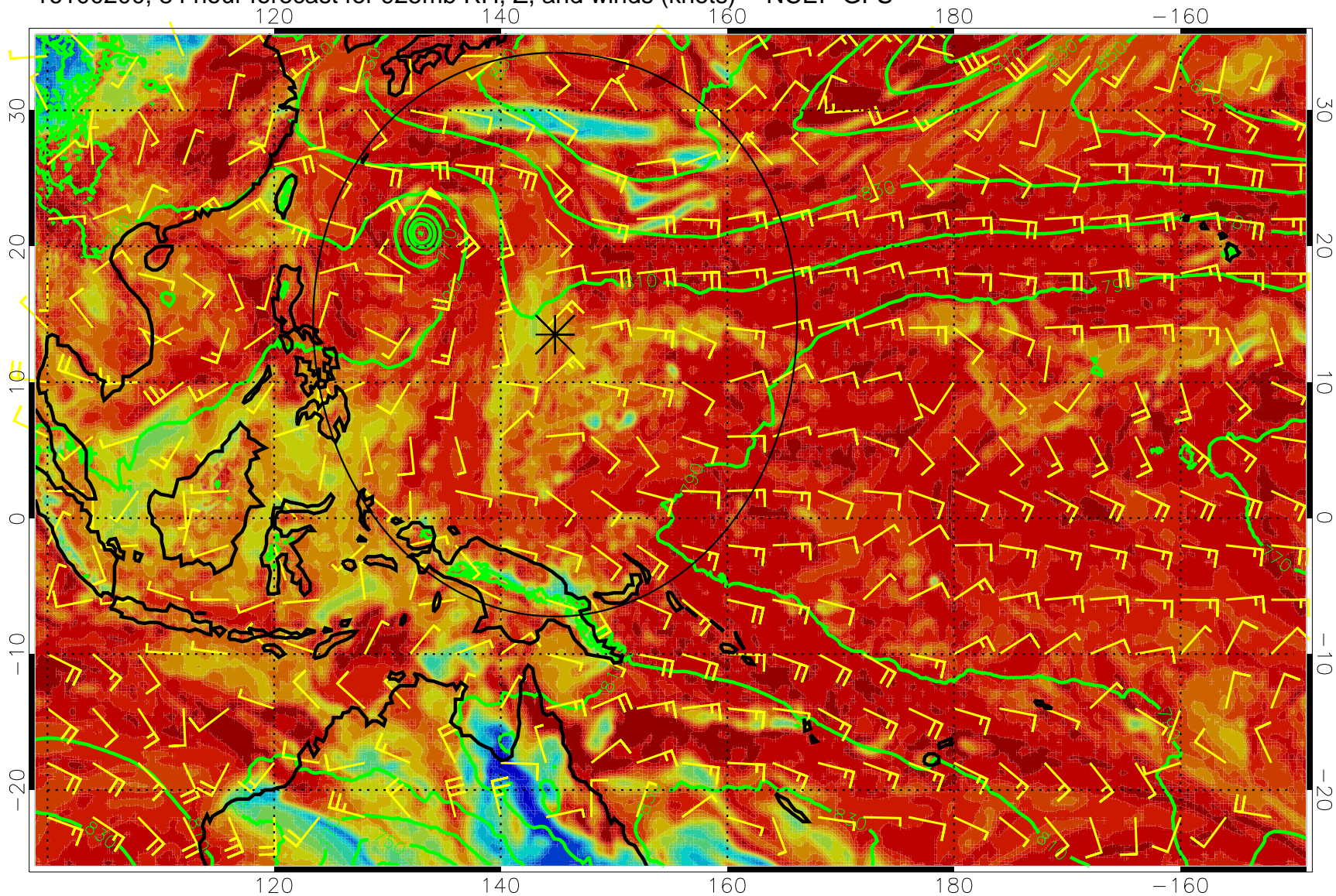
16100200, 84 hour forecast for 925mb RH, Z, and winds (knots) -- NCEP GFS
