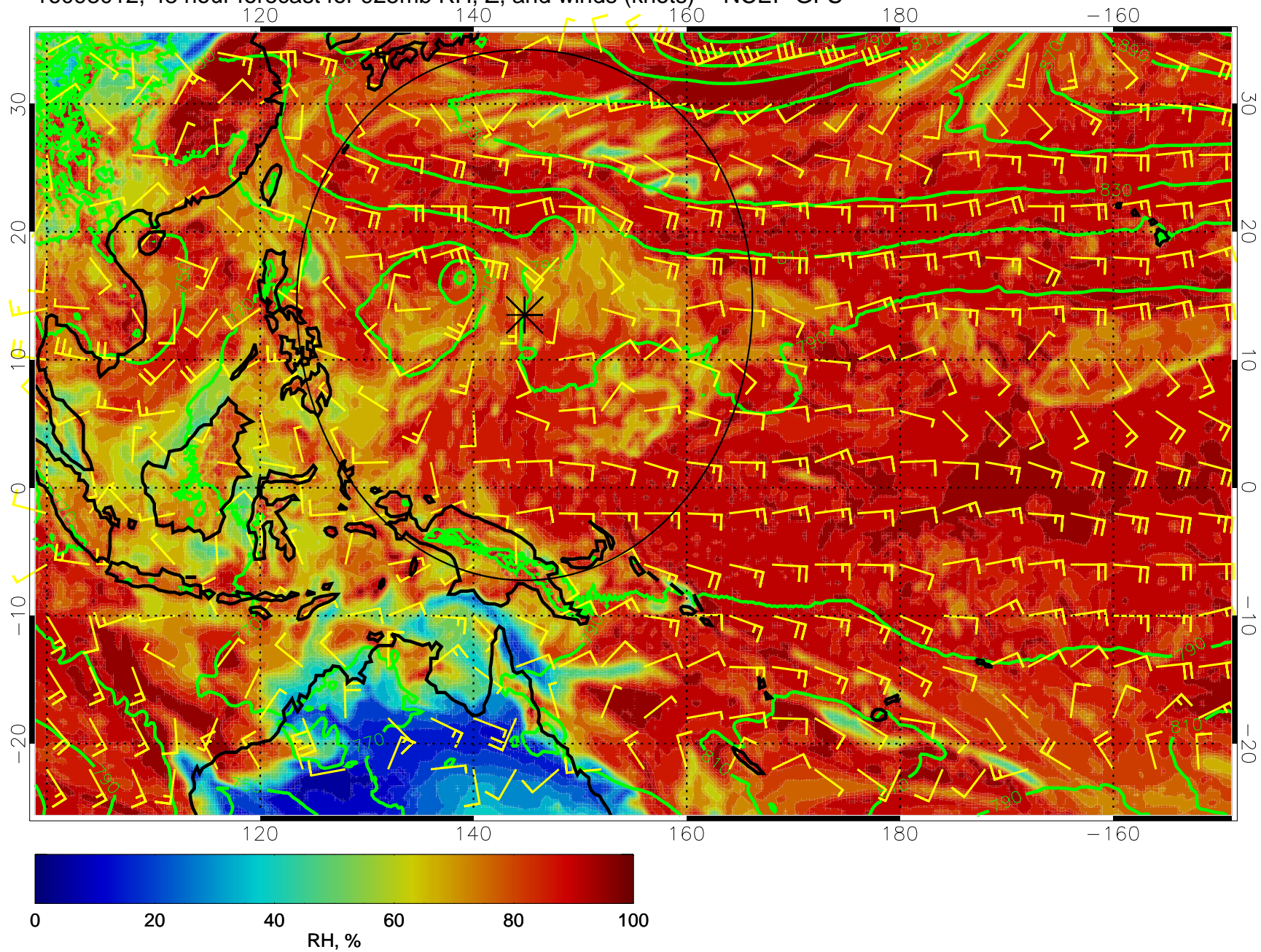
16093012, 48 hour forecast for 925mb RH, Z, and winds (knots) -- NCEP GFS
