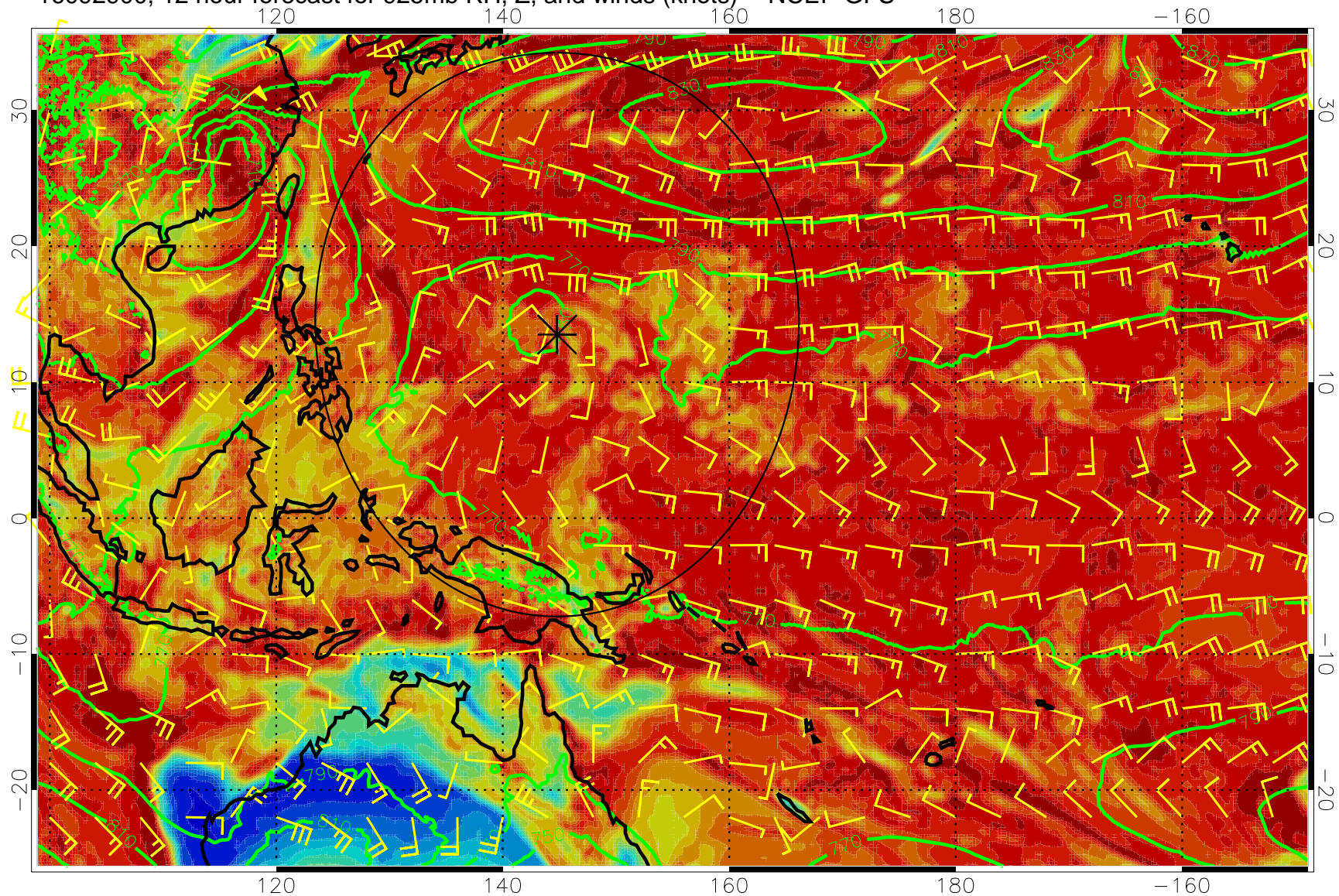
16092900, 12 hour forecast for 925mb RH, Z, and winds (knots) -- NCEP GFS
