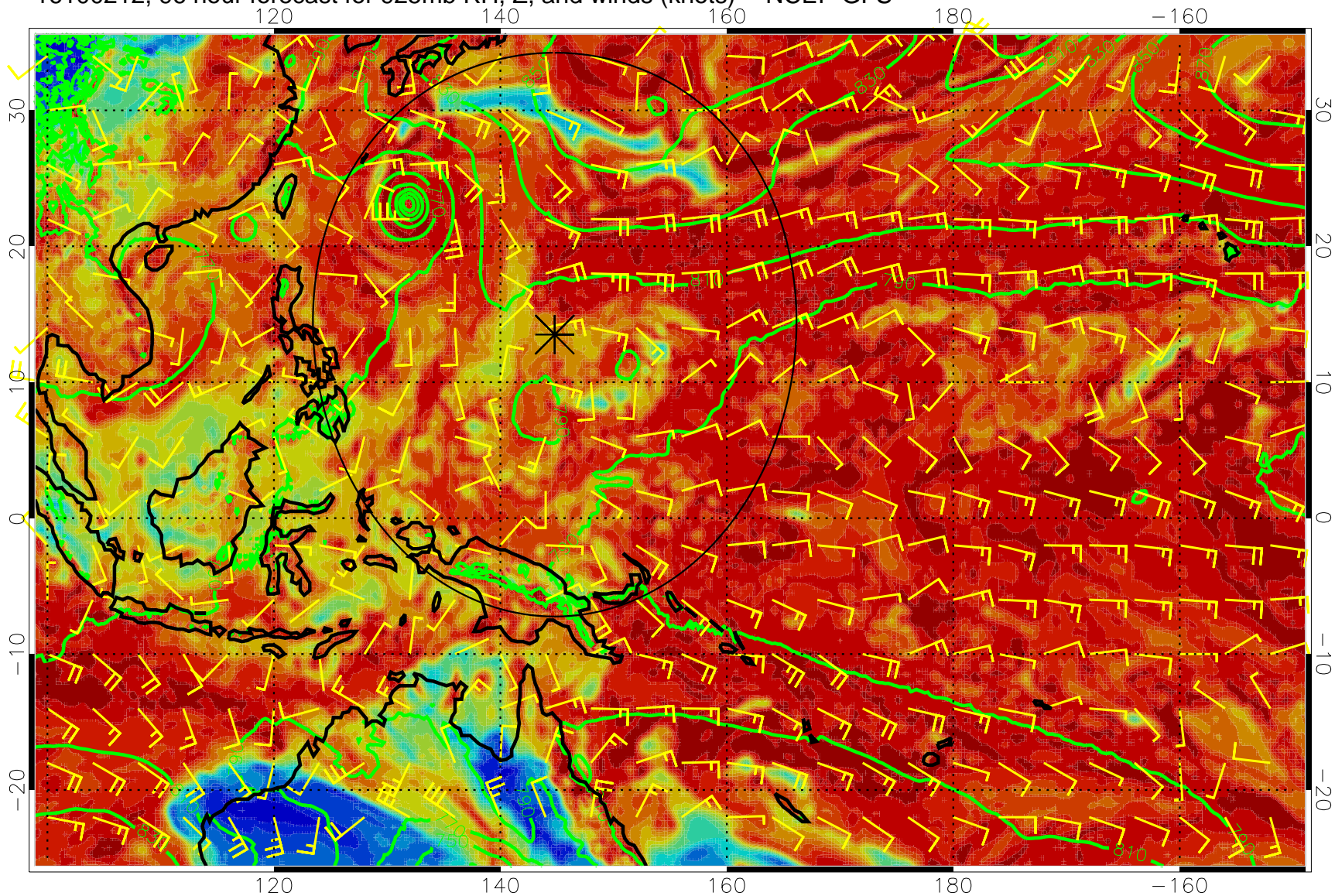
16100212, 96 hour forecast for 925mb RH, Z, and winds (knots) -- NCEP GFS
