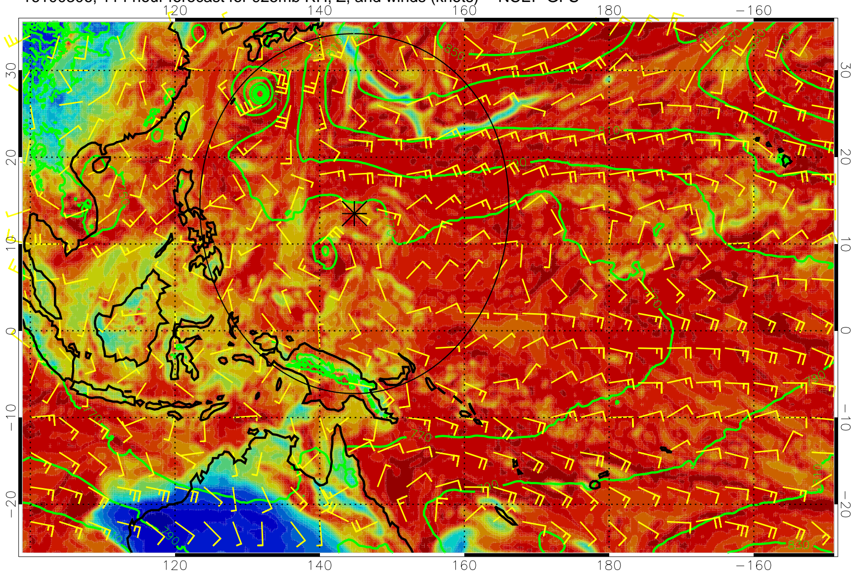
16100306, 114 hour forecast for 925mb RH, Z, and winds (knots) -- NCEP GFS
