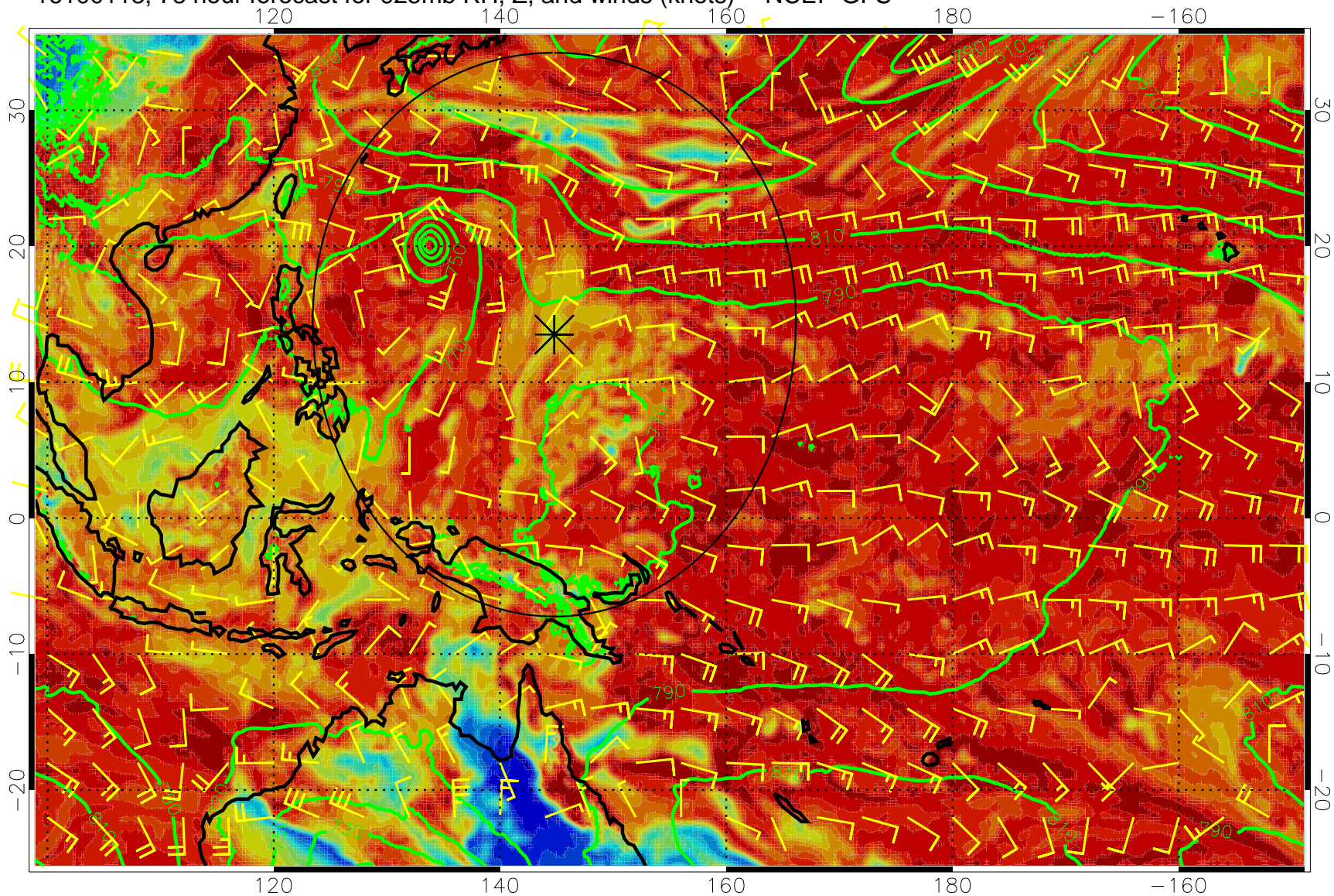
16100118, 78 hour forecast for 925mb RH, Z, and winds (knots) -- NCEP GFS
