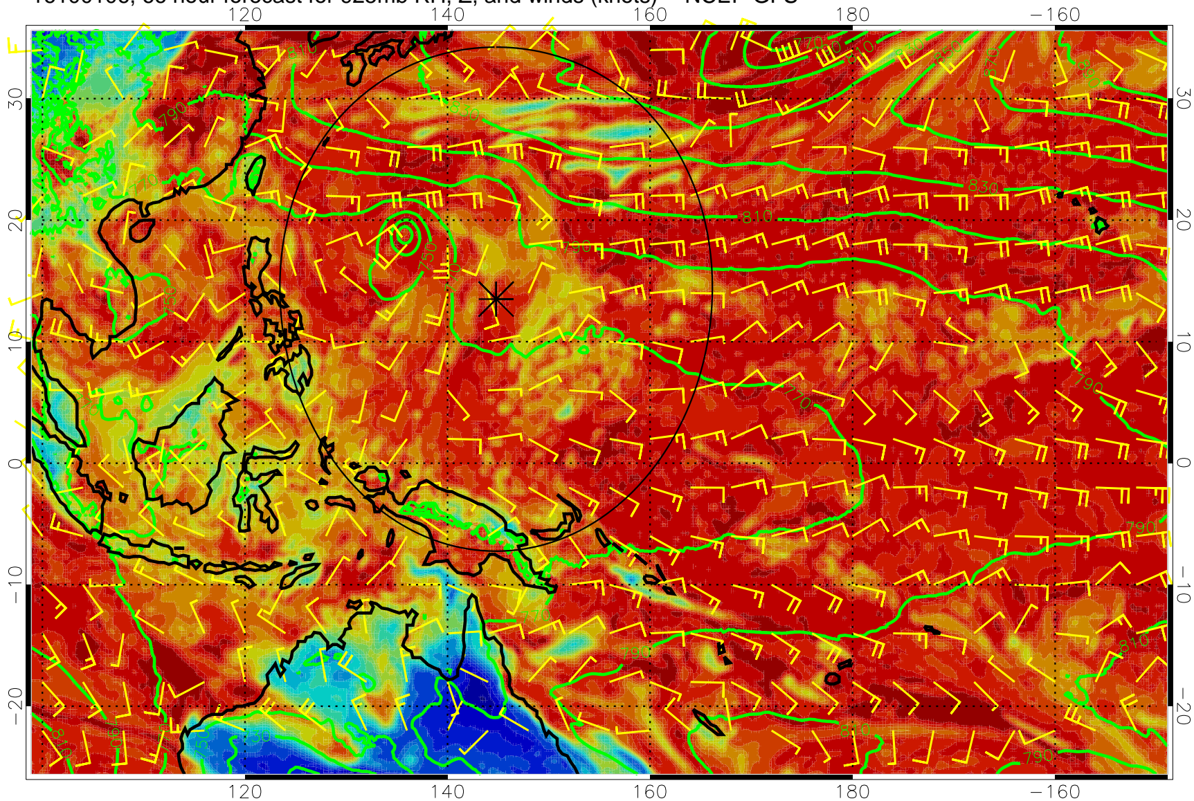
16100106, 66 hour forecast for 925mb RH, Z, and winds (knots) -- NCEP GFS
