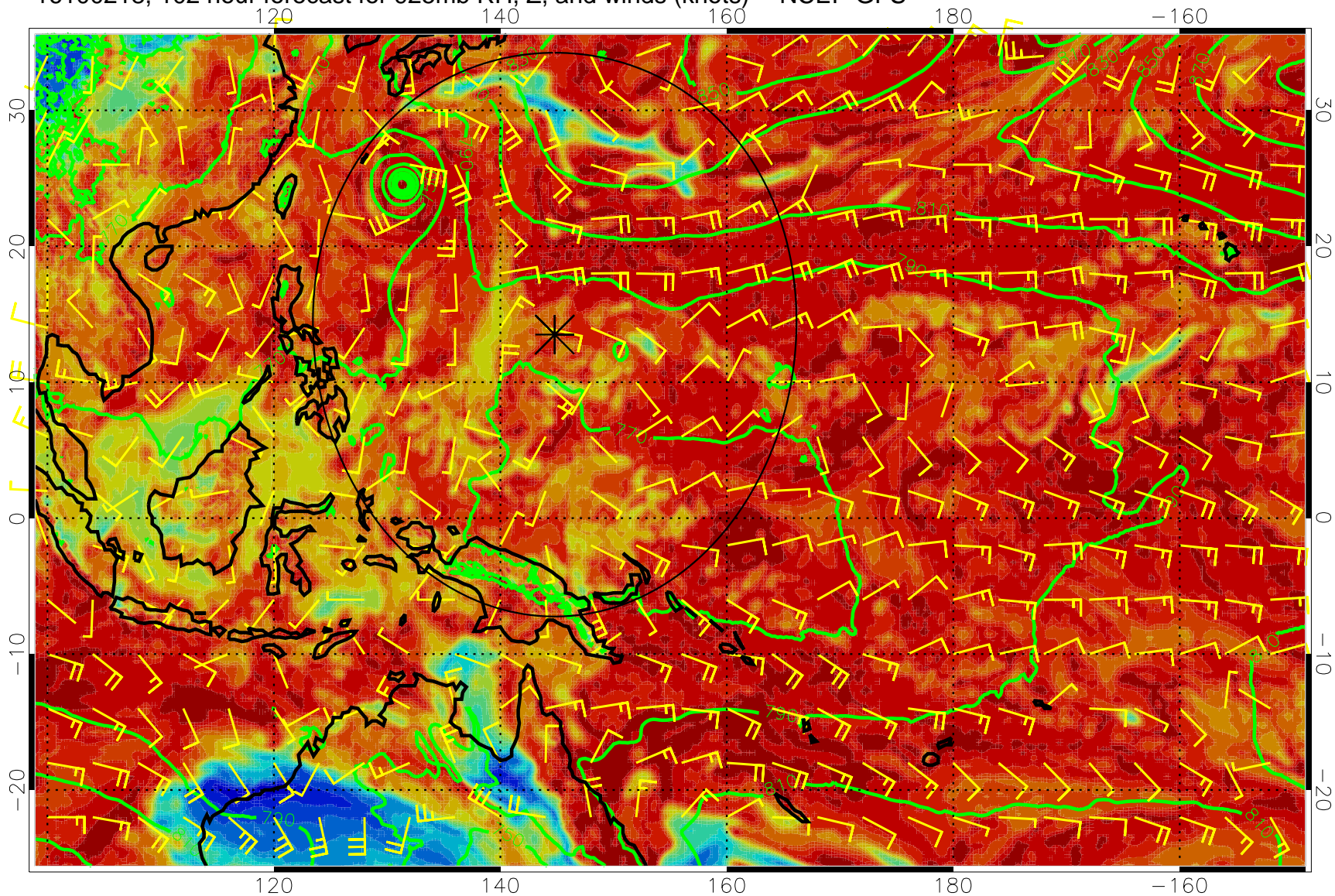
16100218, 102 hour forecast for 925mb RH, Z, and winds (knots) -- NCEP GFS
