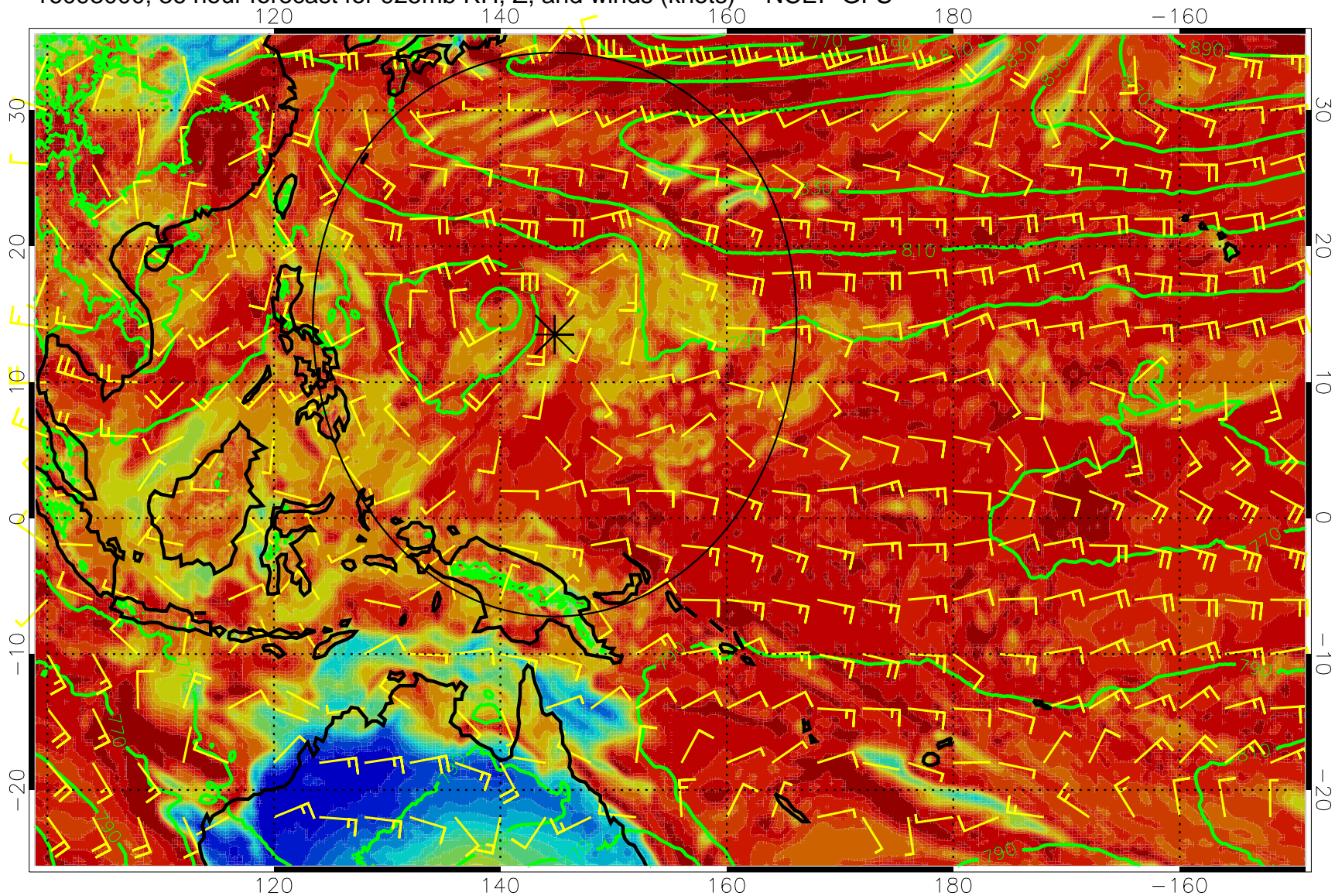
16093000, 36 hour forecast for 925mb RH, Z, and winds (knots) -- NCEP GFS
