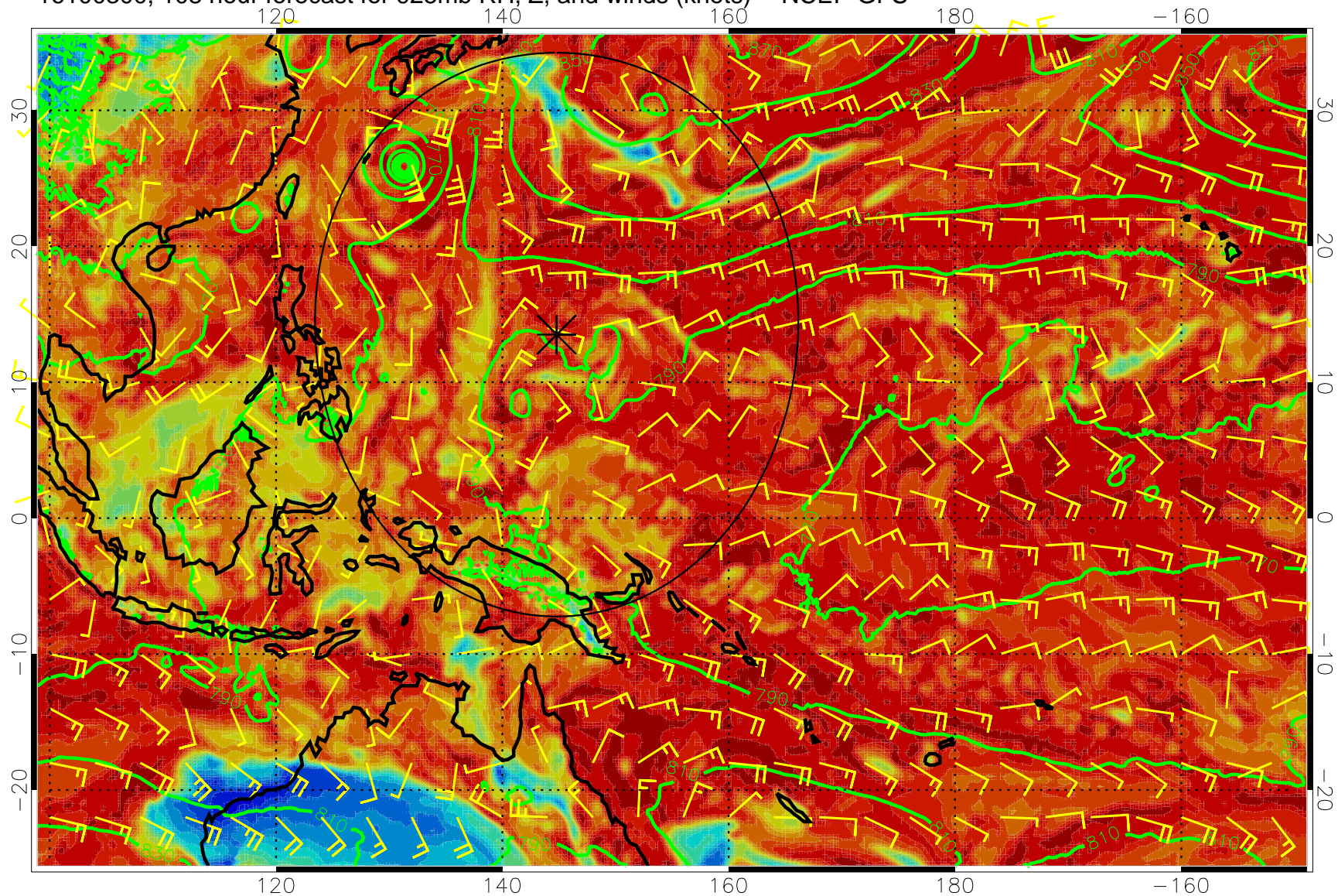
16100300, 108 hour forecast for 925mb RH, Z, and winds (knots) -- NCEP GFS
