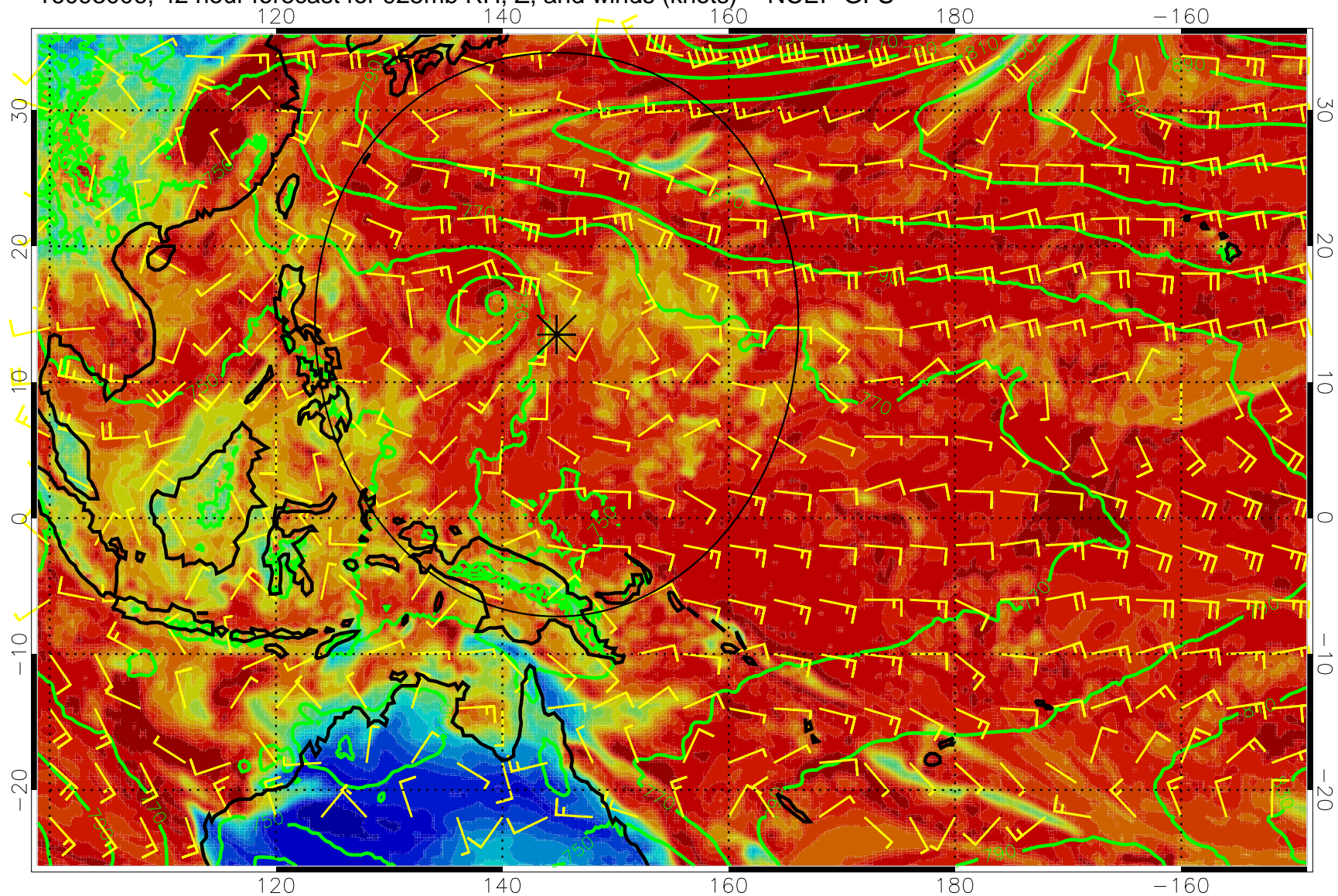
16093006, 42 hour forecast for 925mb RH, Z, and winds (knots) -- NCEP GFS
