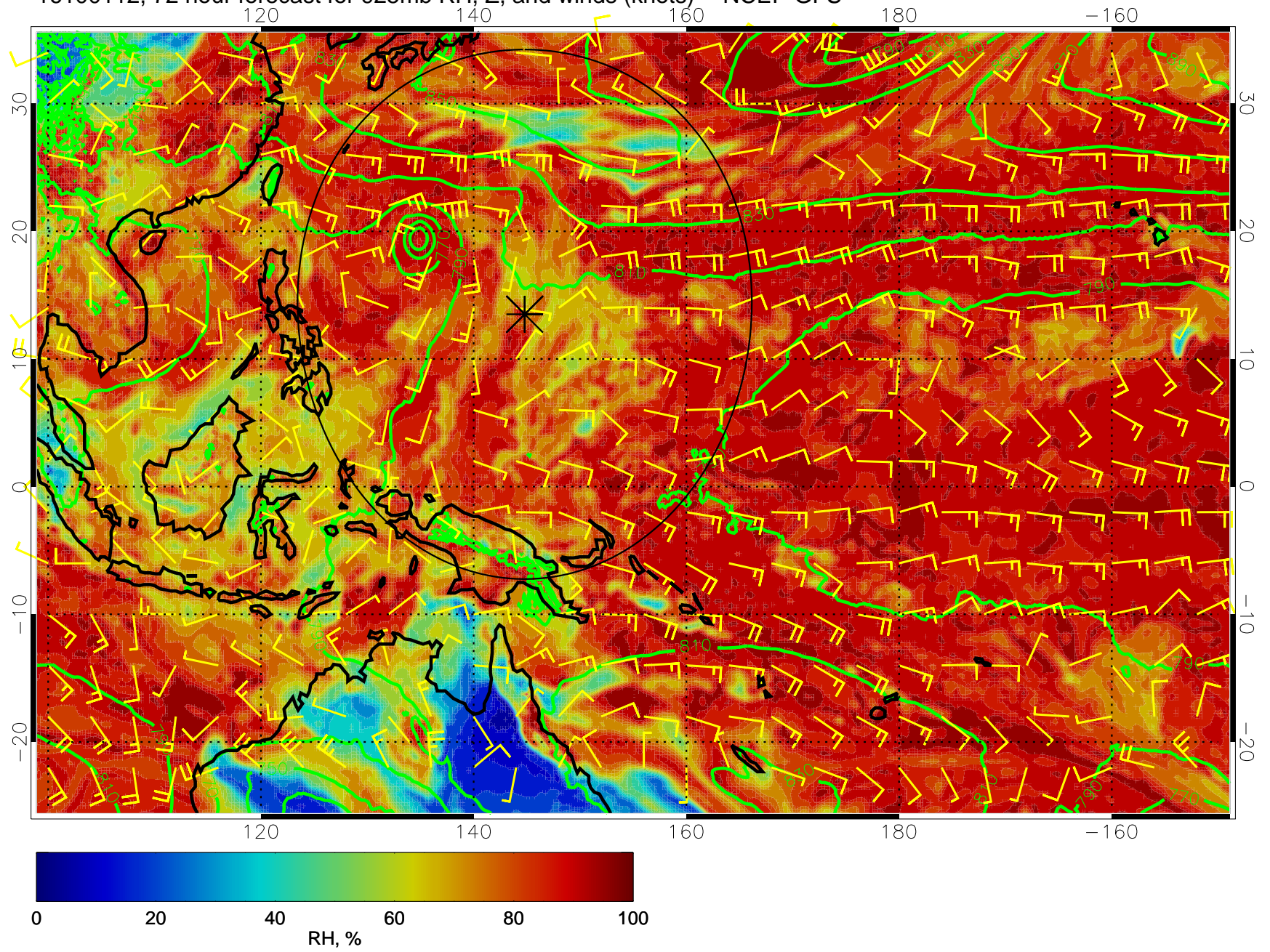
16100112, 72 hour forecast for 925mb RH, Z, and winds (knots) -- NCEP GFS
