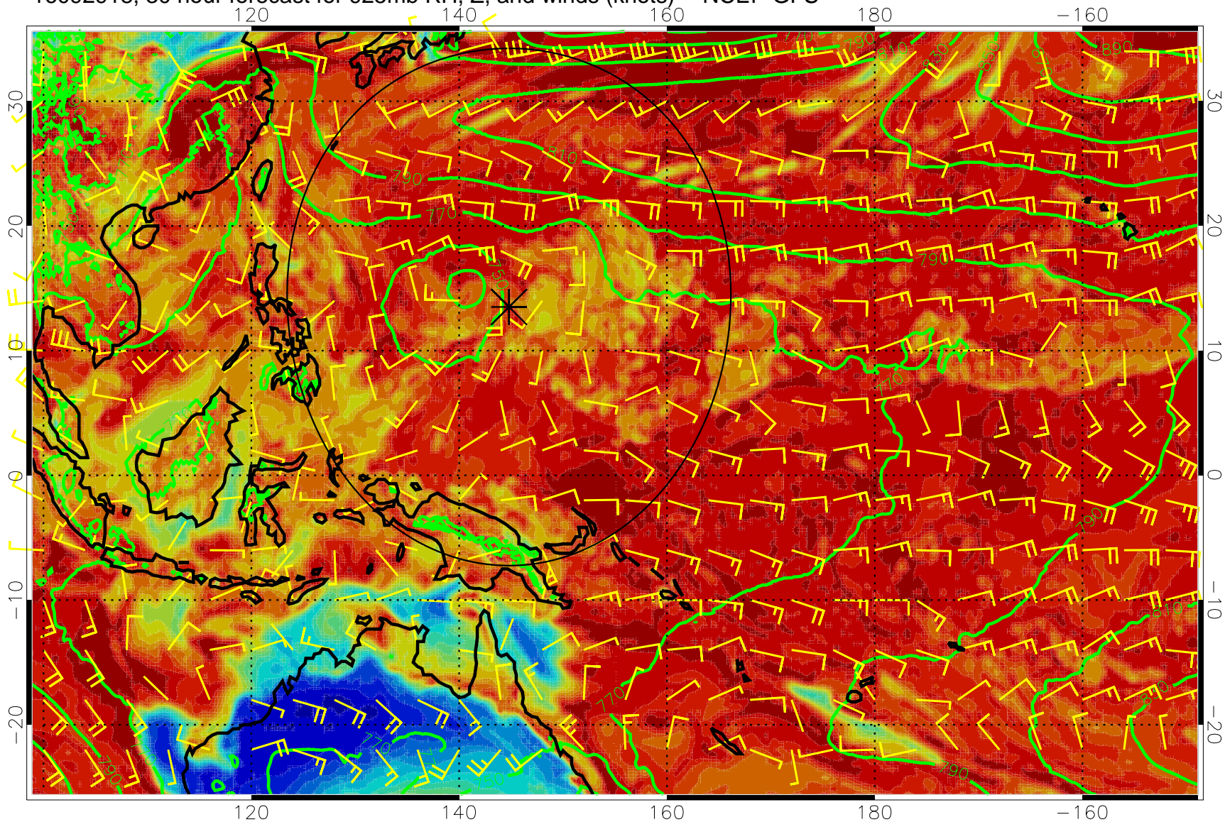
16092918, 30 hour forecast for 925mb RH, Z, and winds (knots) -- NCEP GFS
