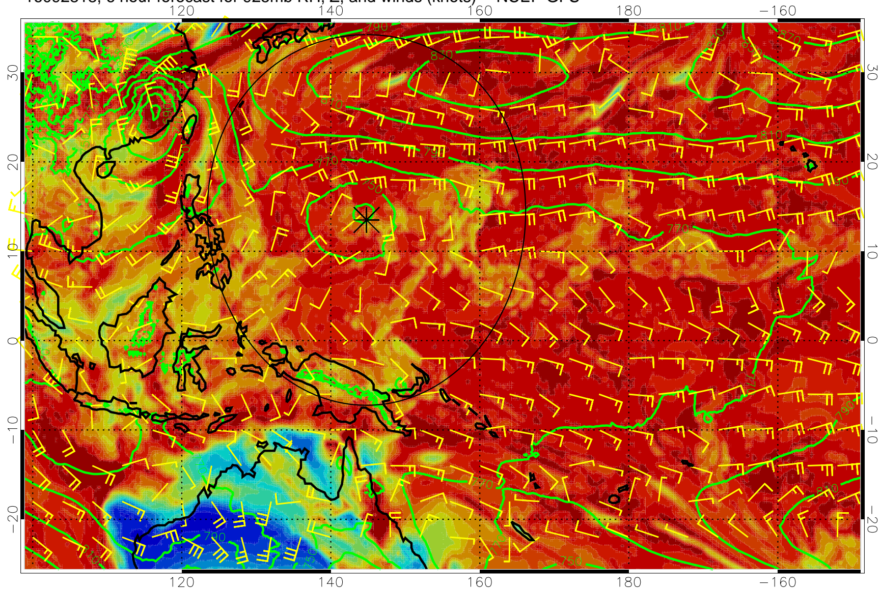
16092818, 6 hour forecast for 925mb RH, Z, and winds (knots) -- NCEP GFS
