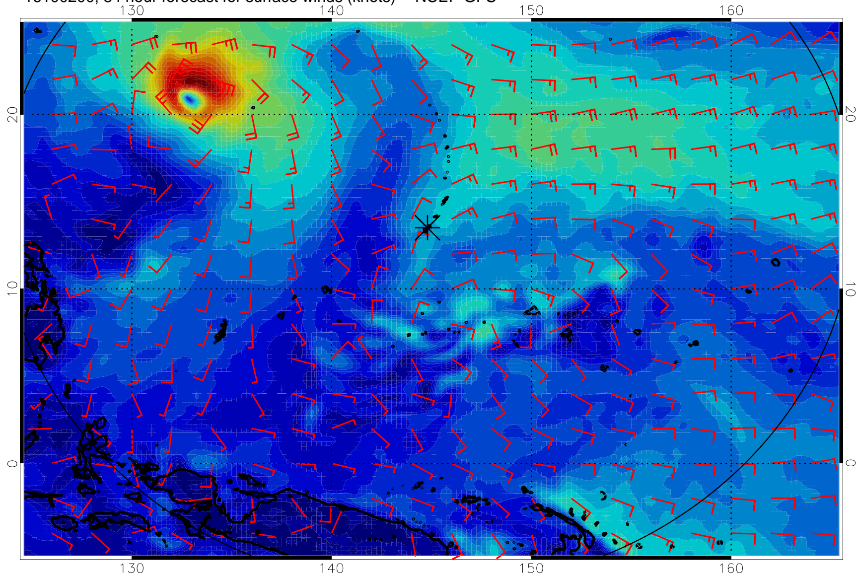
16100200, 84 hour forecast for surface winds (knots) -- NCEP GFS
