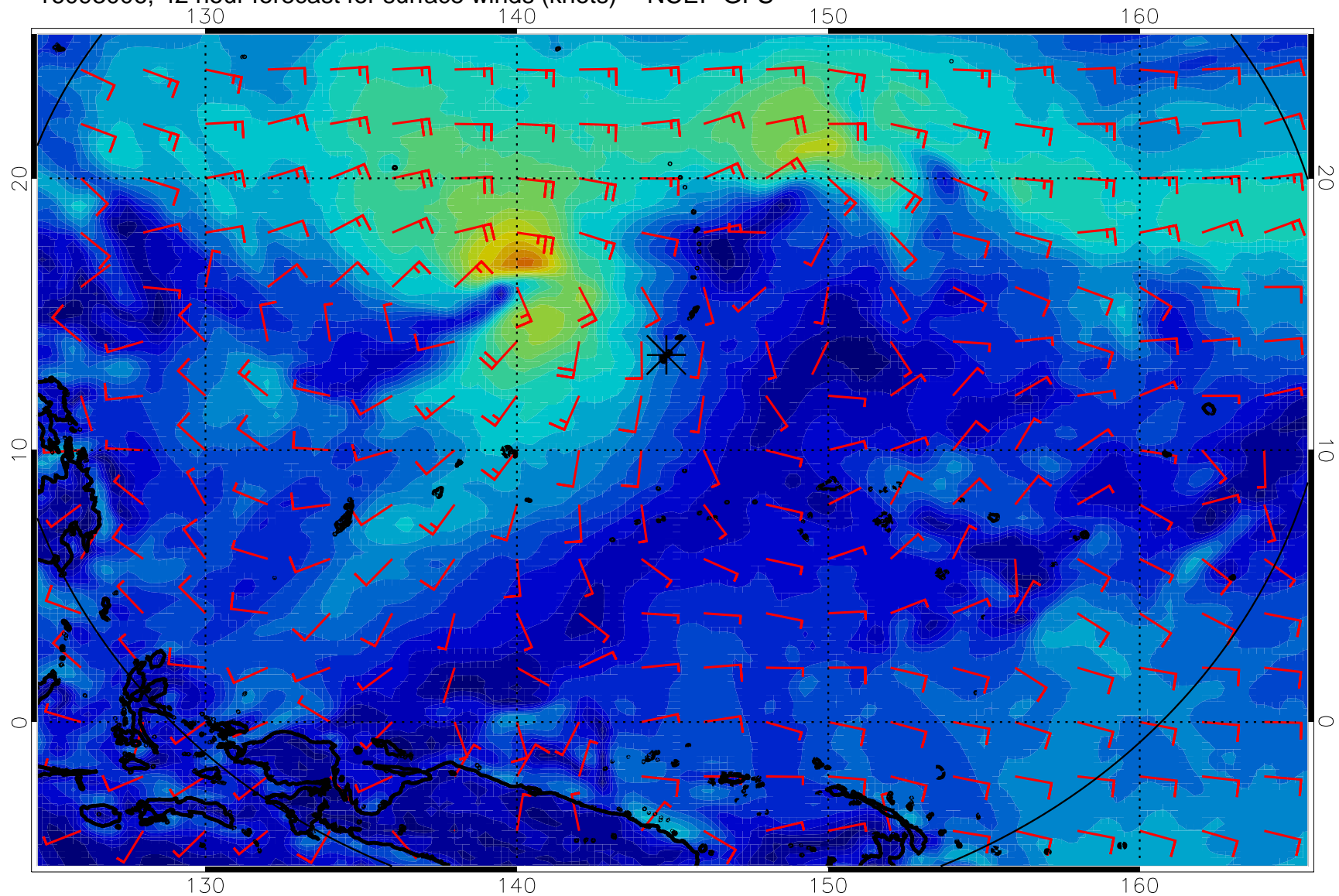
16093006, 42 hour forecast for surface winds (knots) -- NCEP GFS
