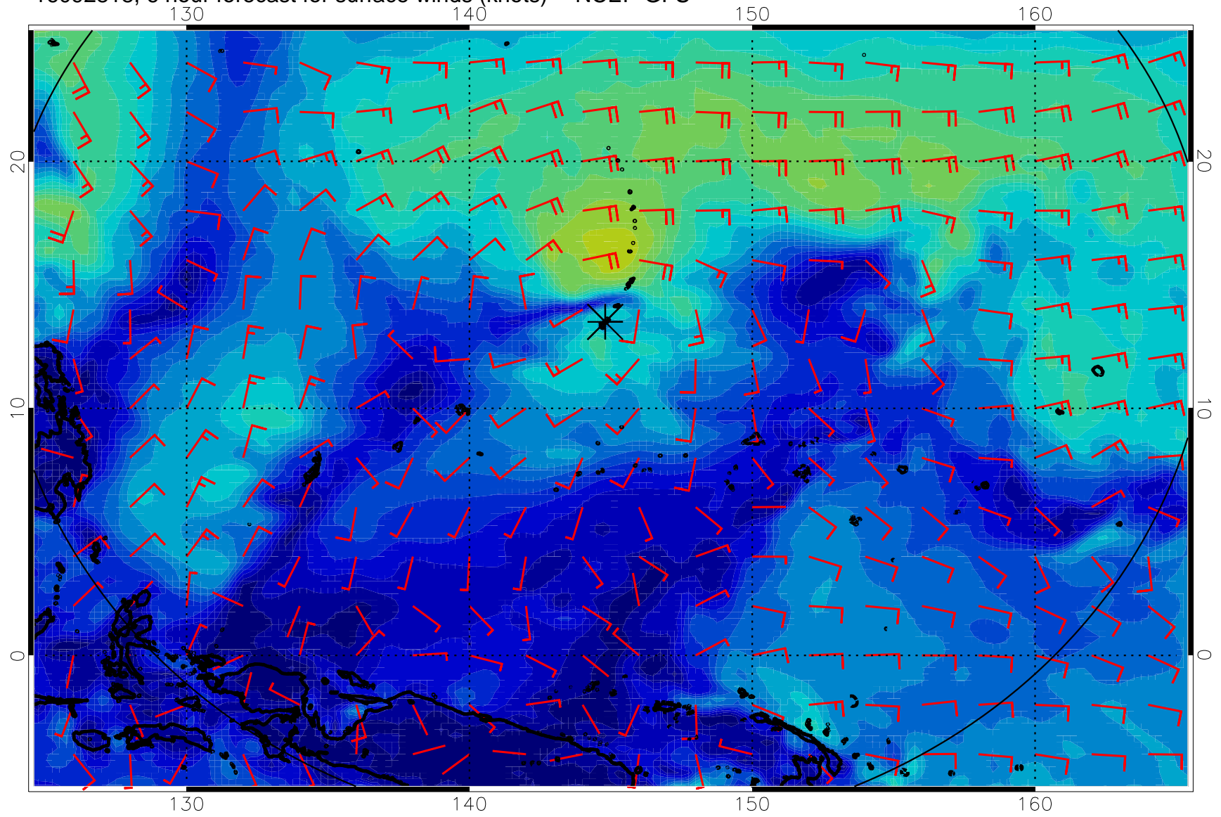
16092818, 6 hour forecast for surface winds (knots) -- NCEP GFS
