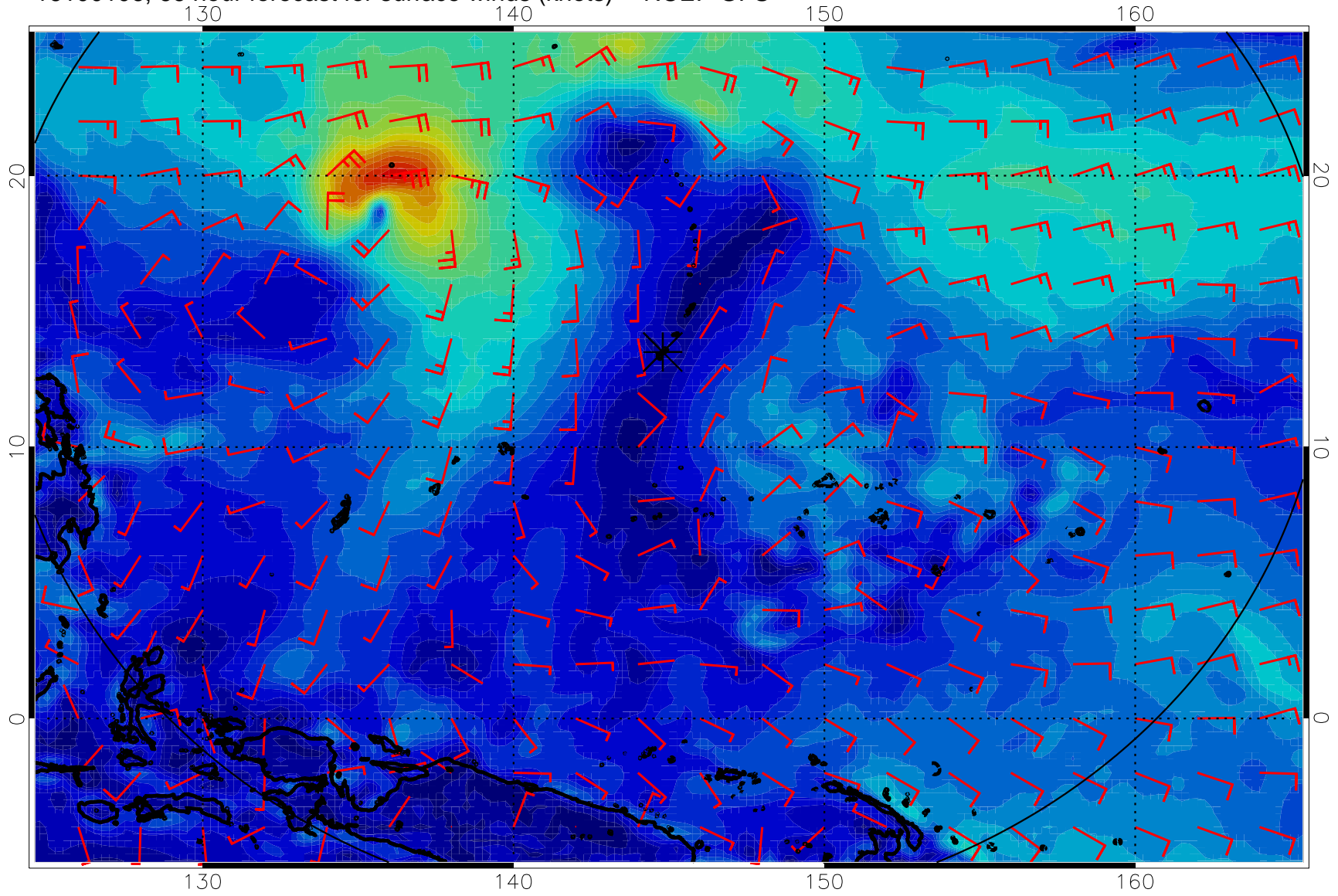
16100106, 66 hour forecast for surface winds (knots) -- NCEP GFS
