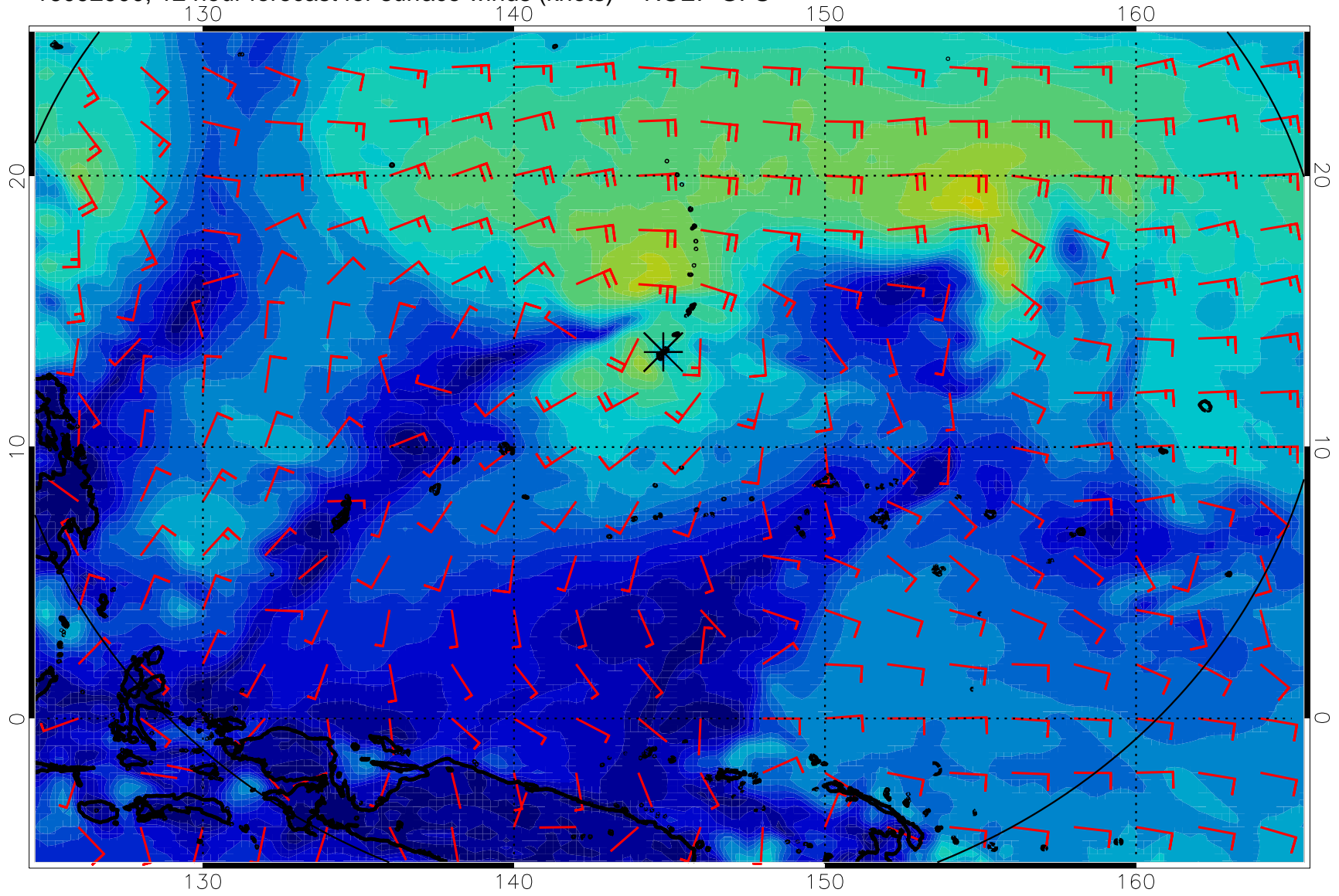
16092900, 12 hour forecast for surface winds (knots) -- NCEP GFS
