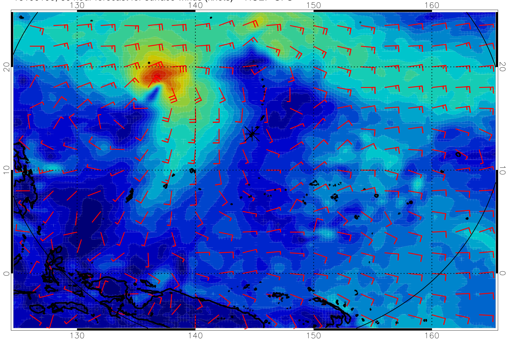
16100100, 60 hour forecast for surface winds (knots) -- NCEP GFS
