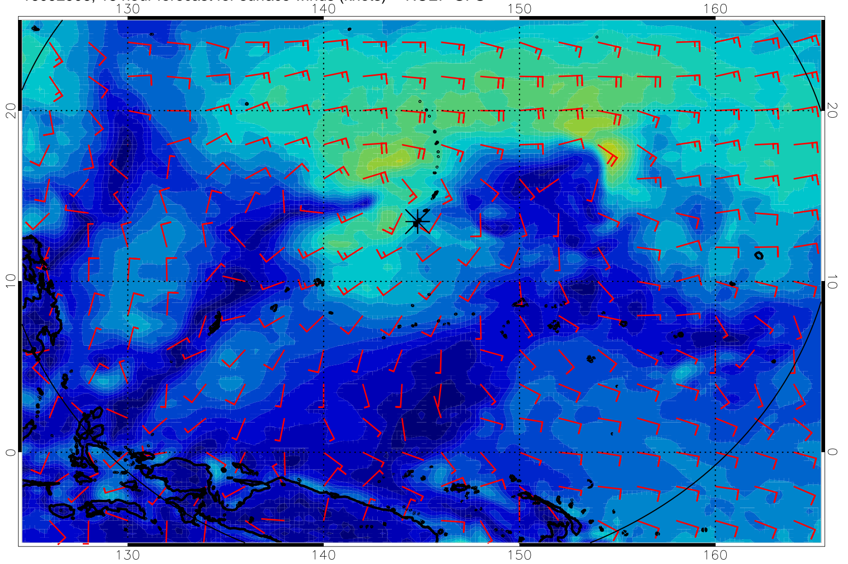
16092906, 18 hour forecast for surface winds (knots) -- NCEP GFS
