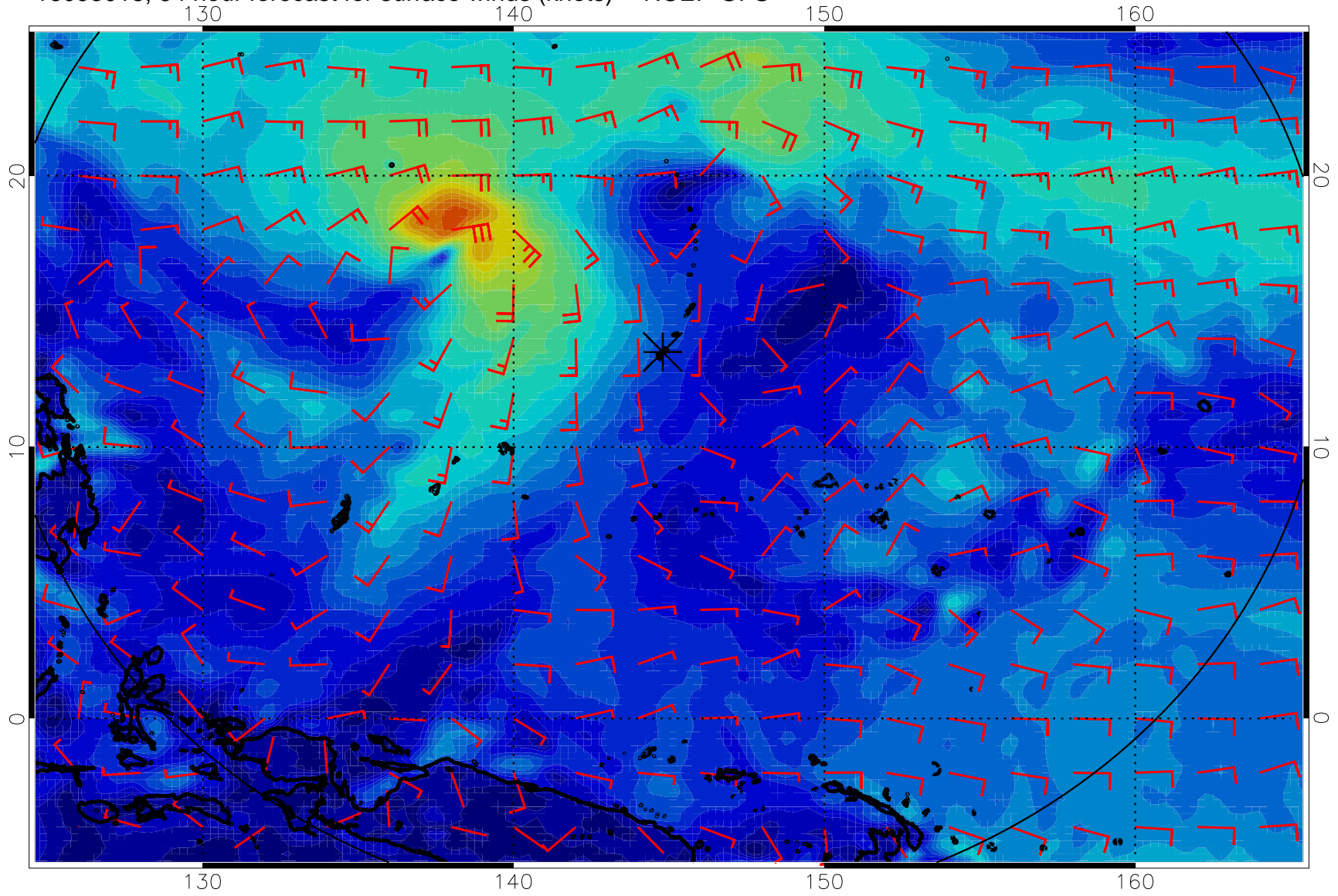
16093018, 54 hour forecast for surface winds (knots) -- NCEP GFS
