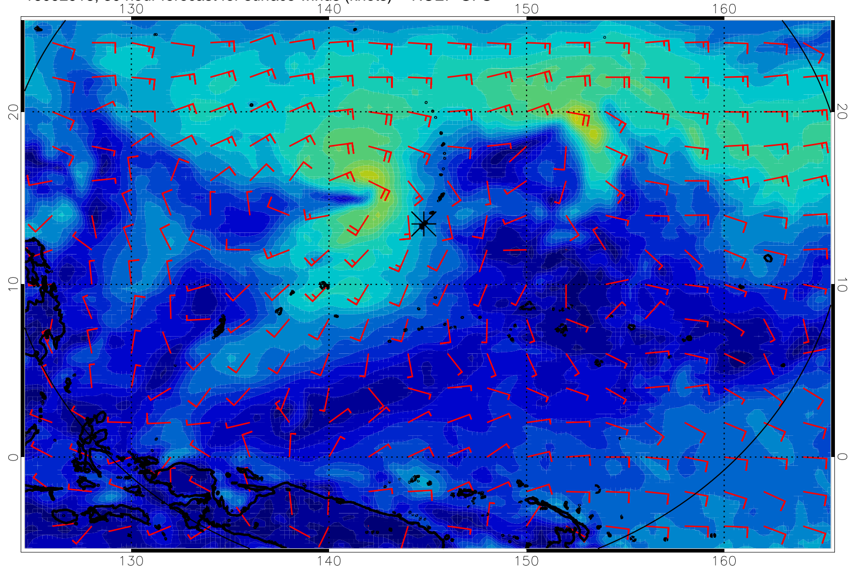
16092918, 30 hour forecast for surface winds (knots) -- NCEP GFS
