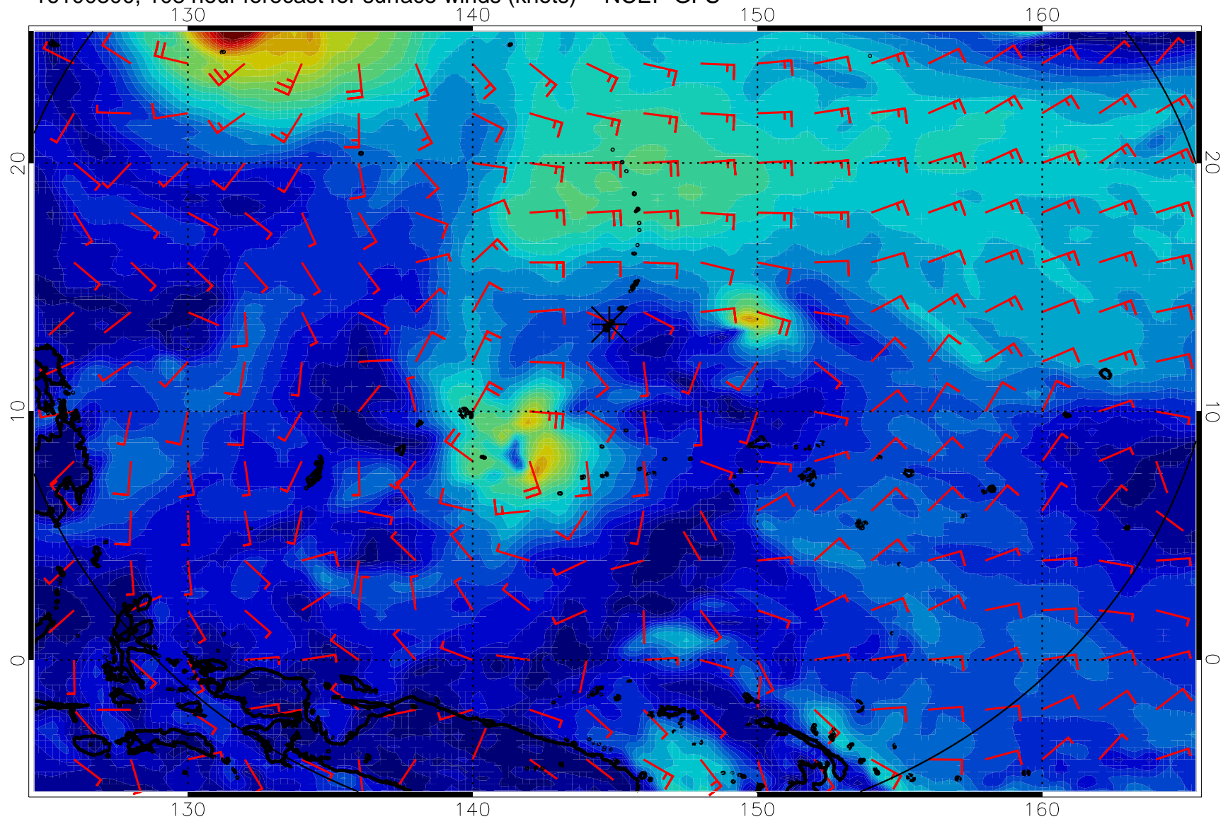
16100300, 108 hour forecast for surface winds (knots) -- NCEP GFS
