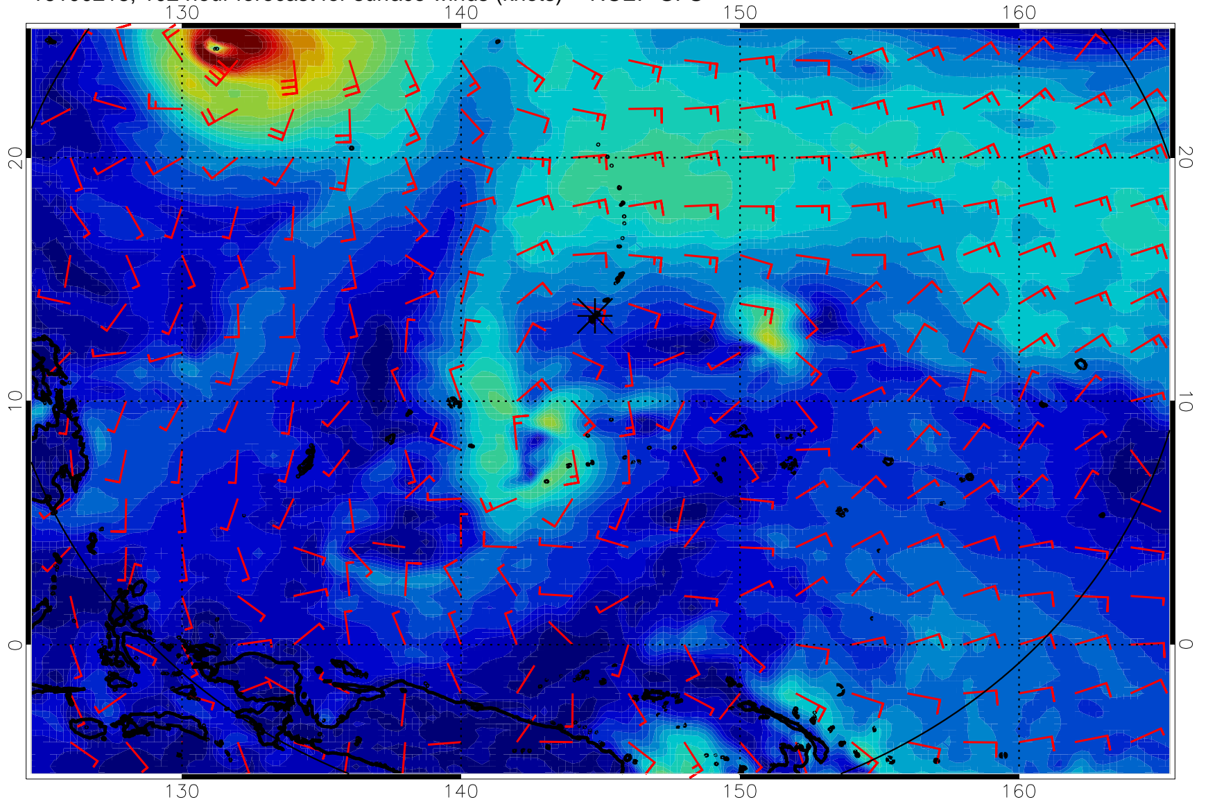
16100218, 102 hour forecast for surface winds (knots) -- NCEP GFS
