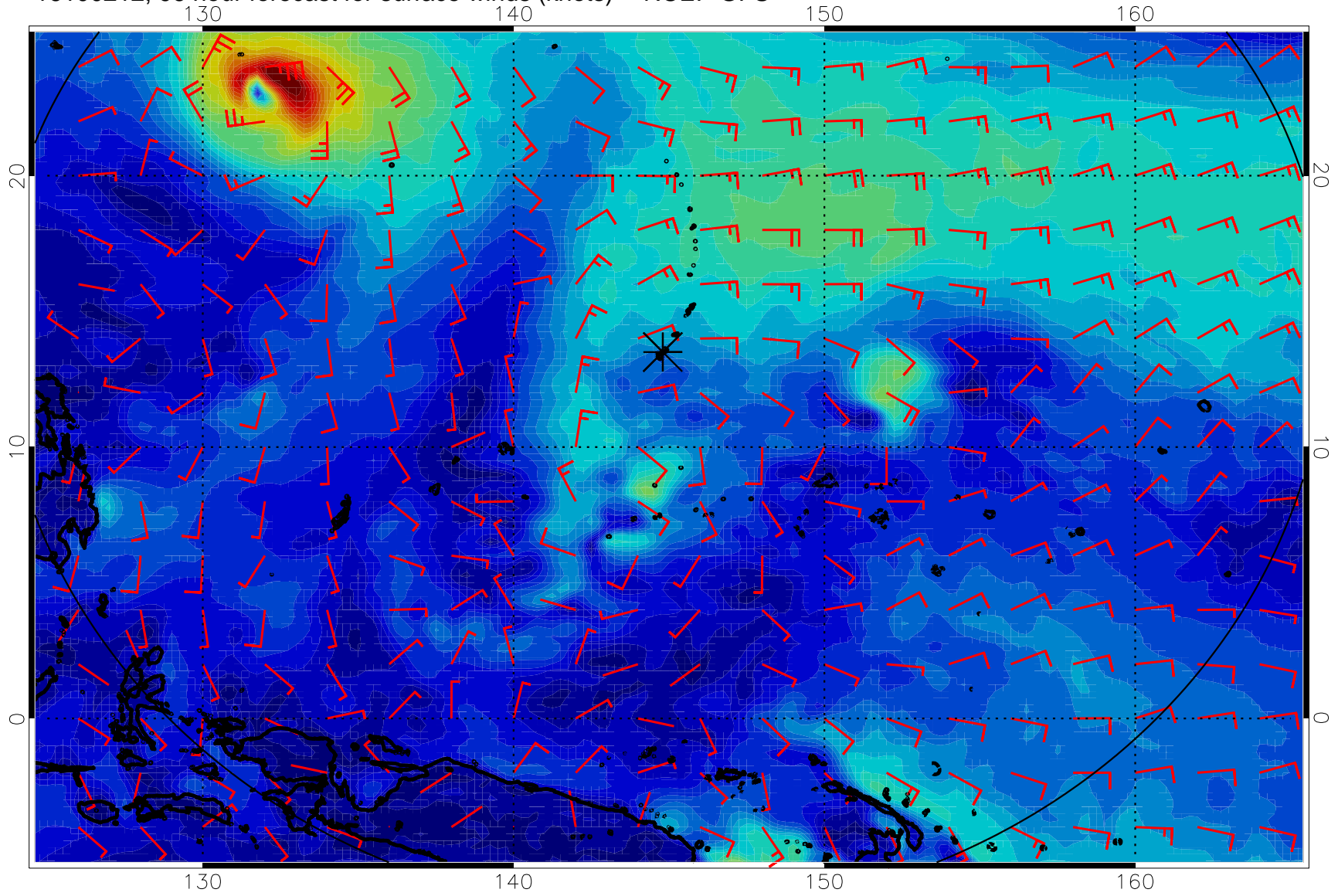
16100212, 96 hour forecast for surface winds (knots) -- NCEP GFS
