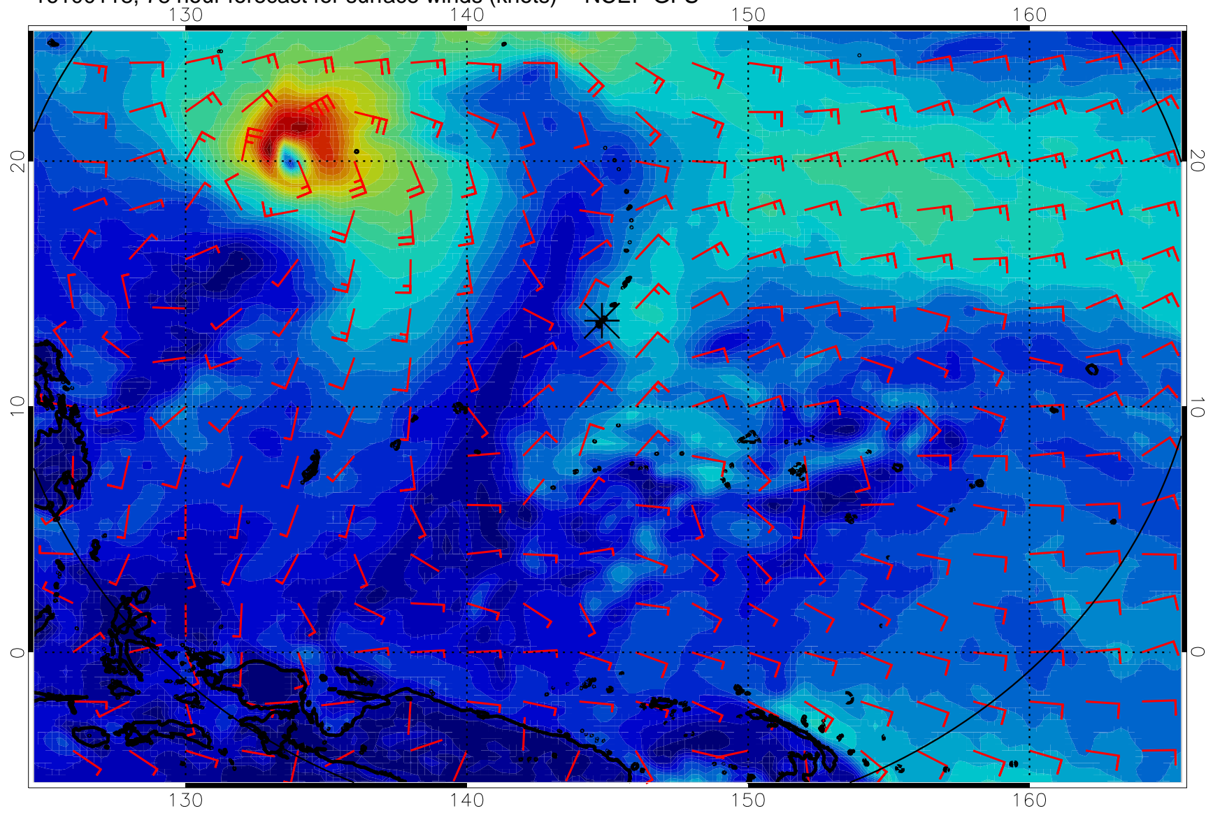
16100118, 78 hour forecast for surface winds (knots) -- NCEP GFS
