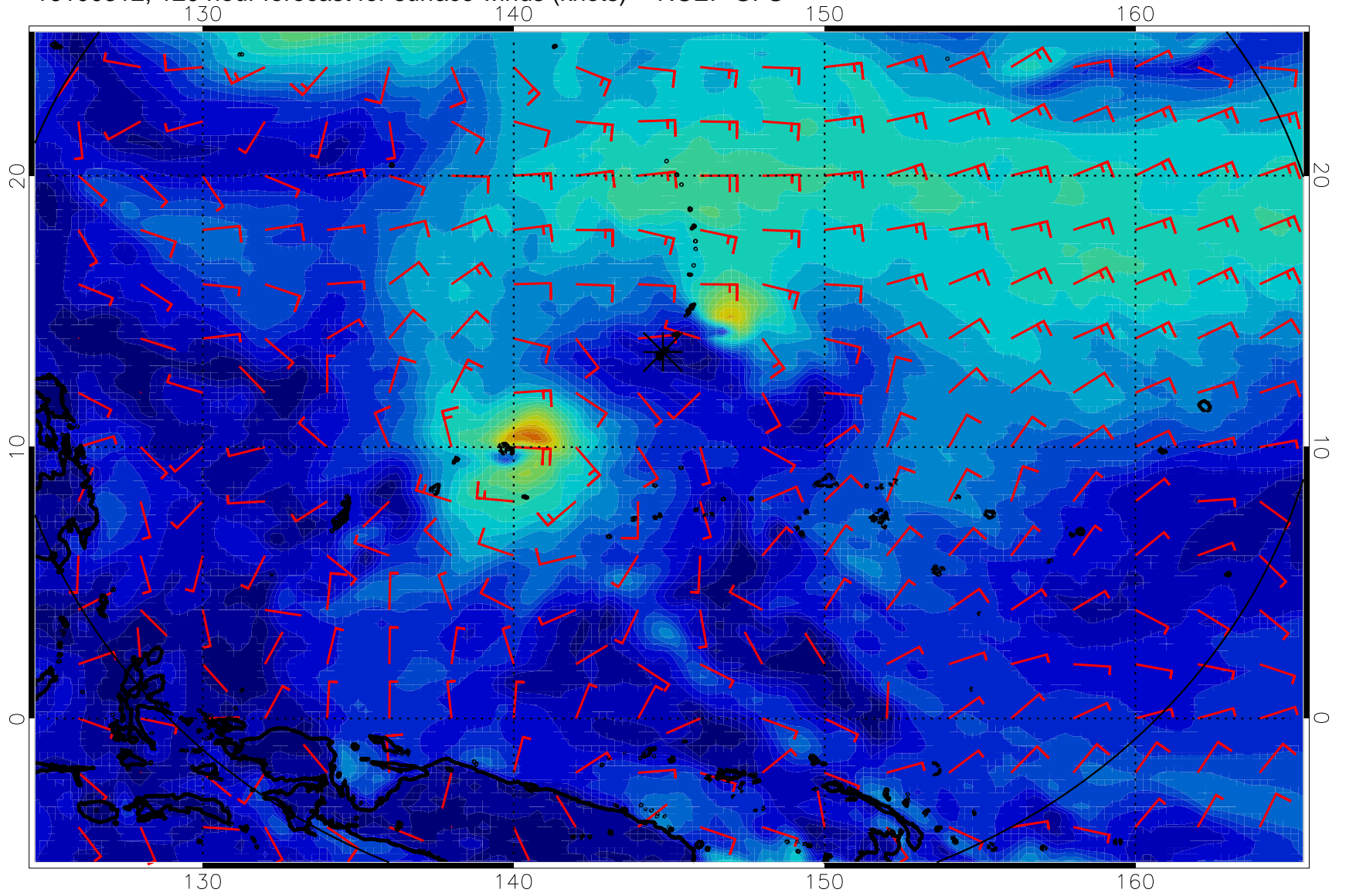
16100312, 120 hour forecast for surface winds (knots) -- NCEP GFS
