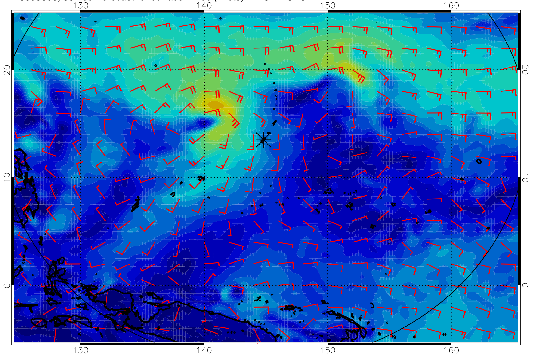
16093000, 36 hour forecast for surface winds (knots) -- NCEP GFS
