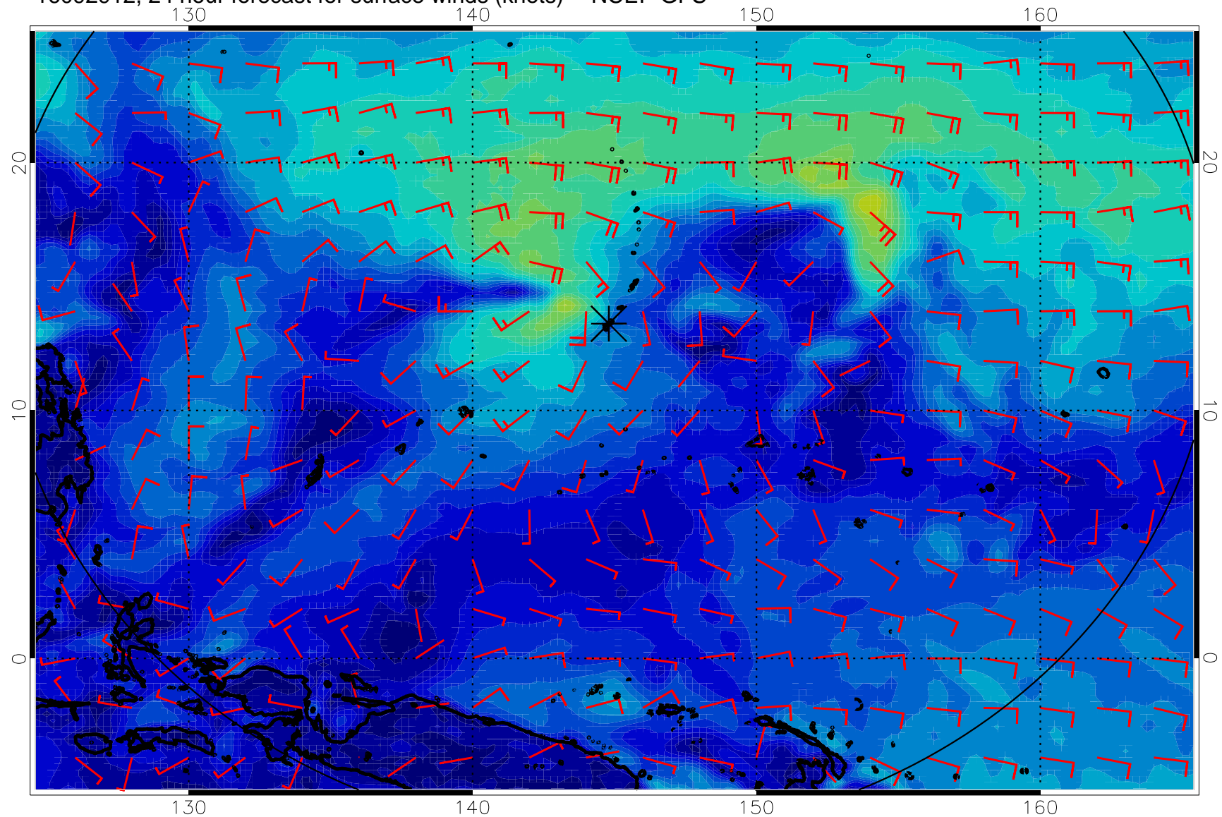
16092912, 24 hour forecast for surface winds (knots) -- NCEP GFS
