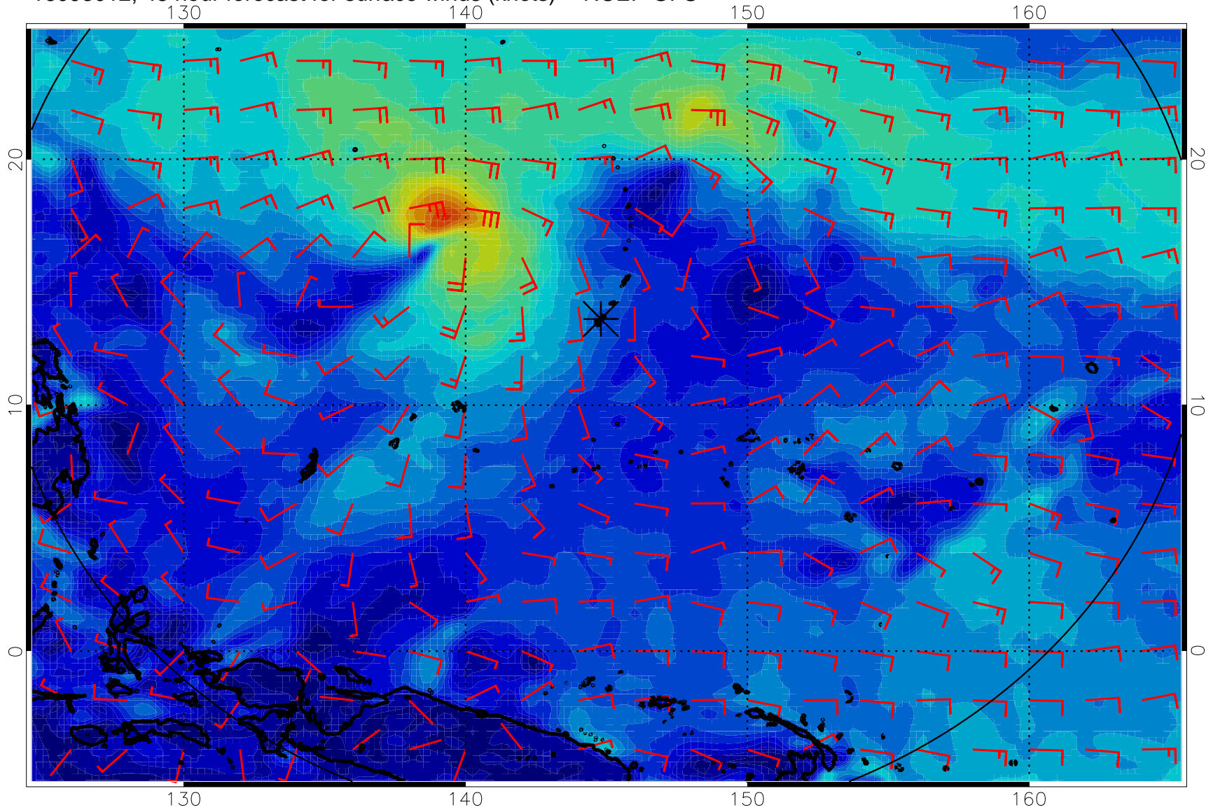
16093012, 48 hour forecast for surface winds (knots) -- NCEP GFS
