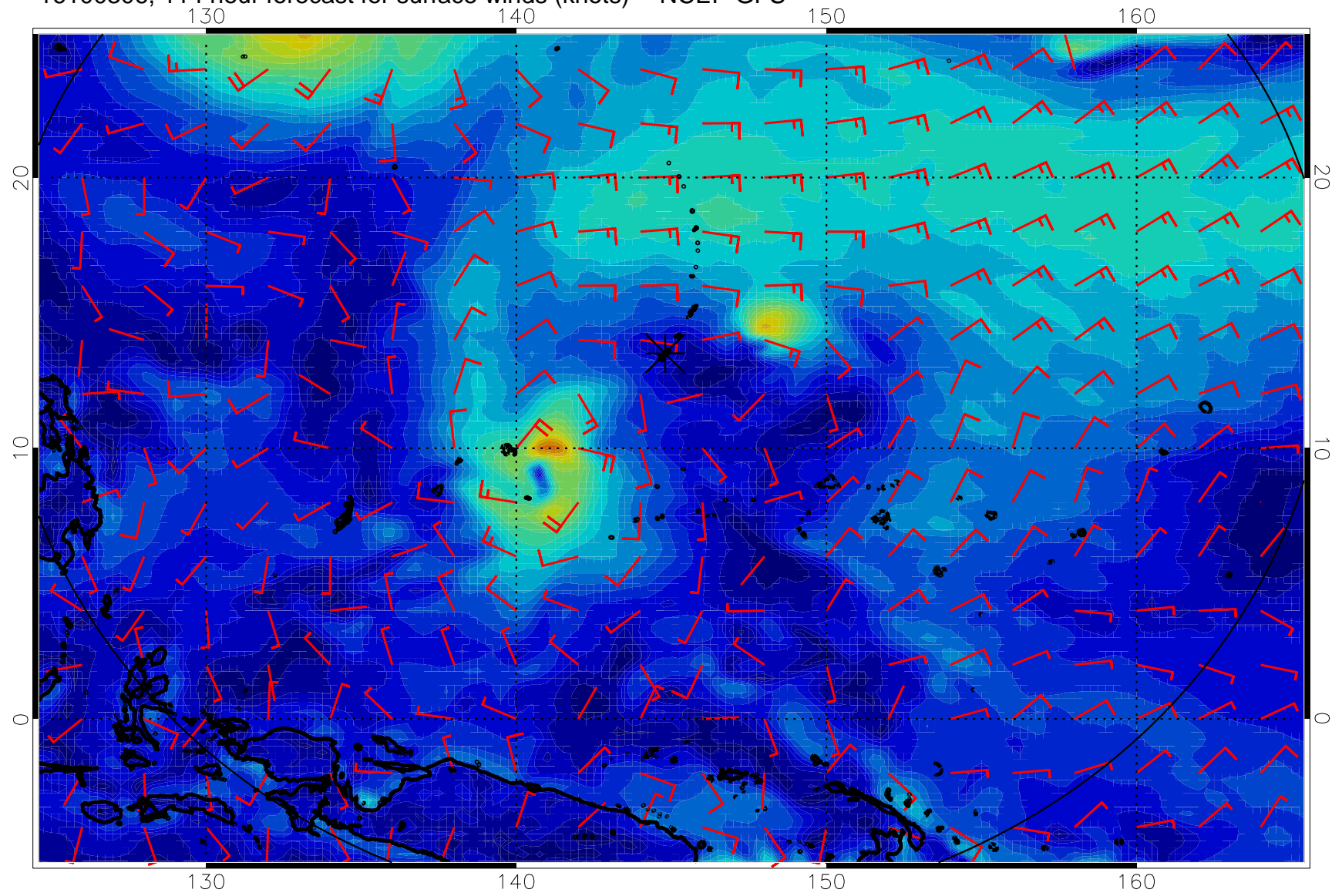
16100306, 114 hour forecast for surface winds (knots) -- NCEP GFS
