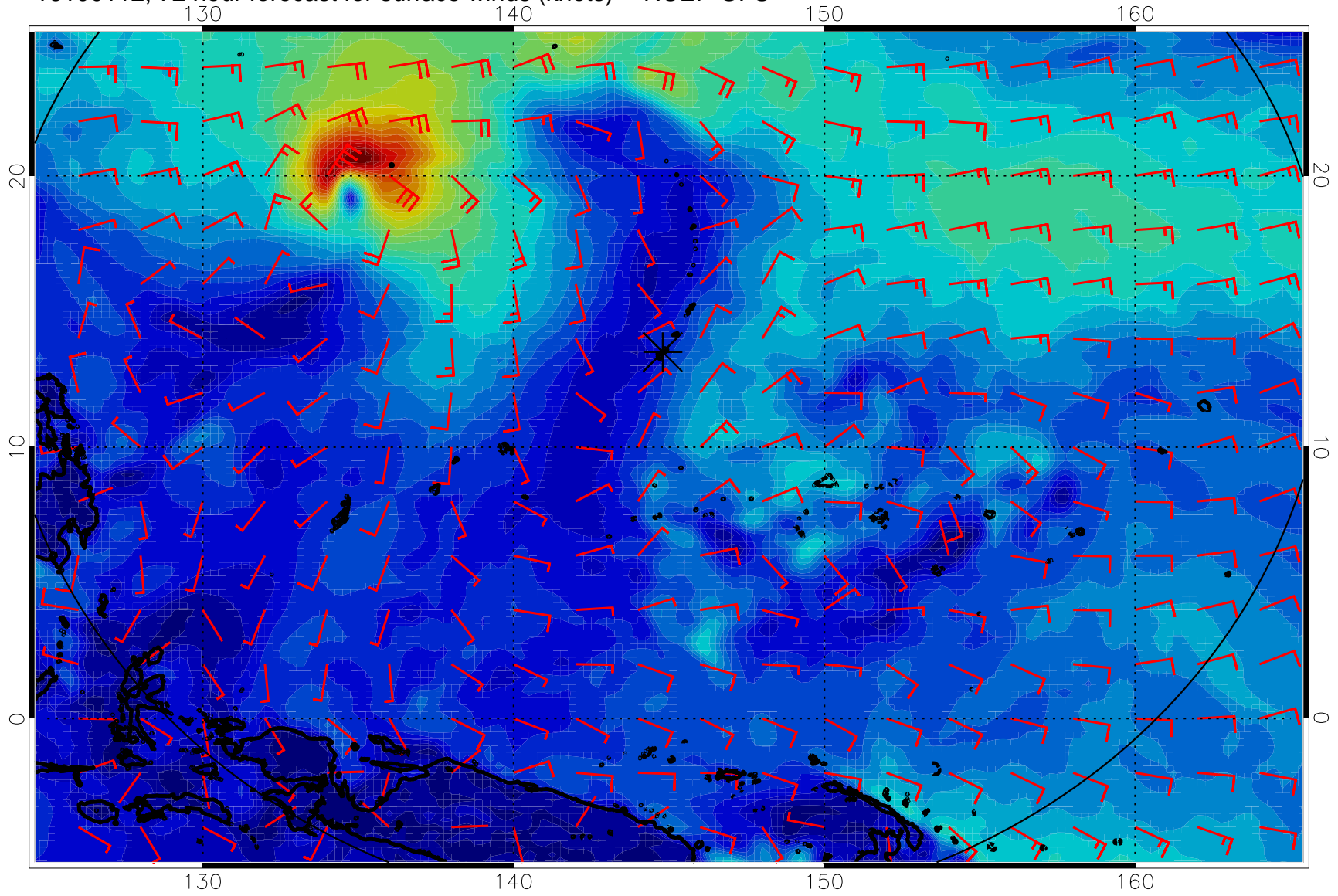
16100112, 72 hour forecast for surface winds (knots) -- NCEP GFS
