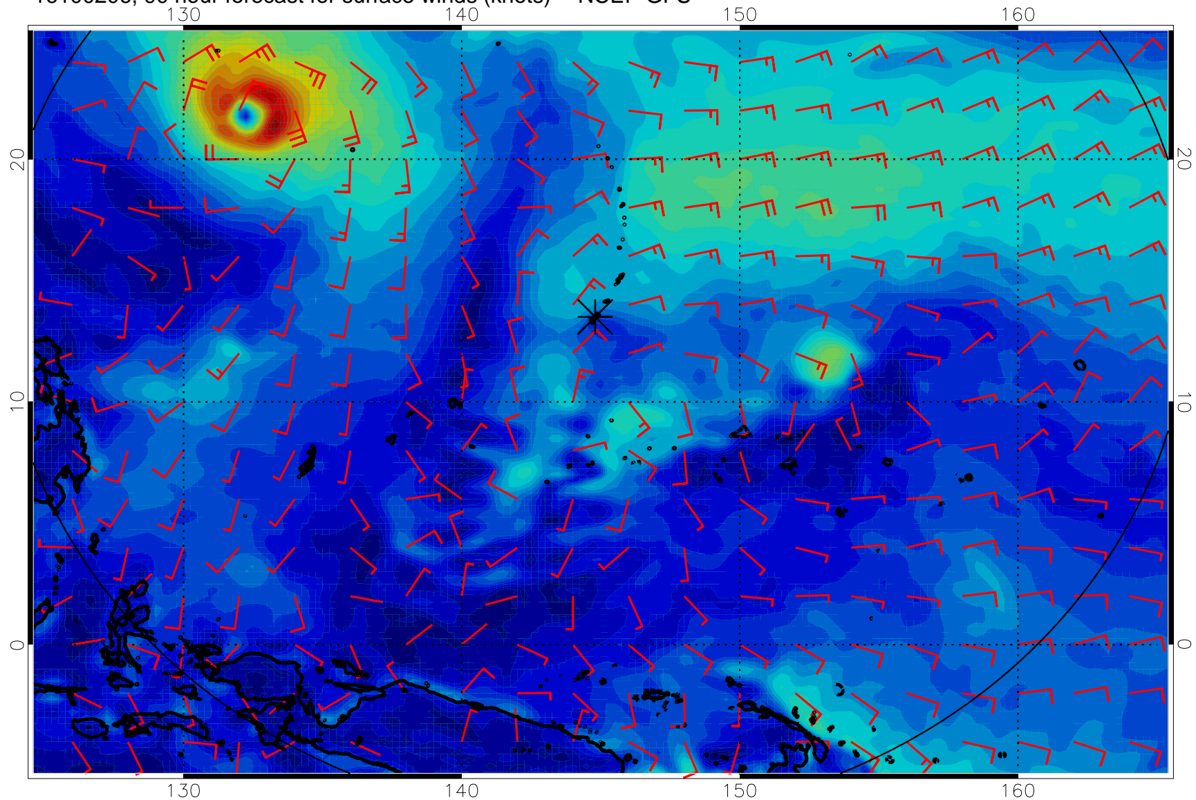
16100206, 90 hour forecast for surface winds (knots) -- NCEP GFS
