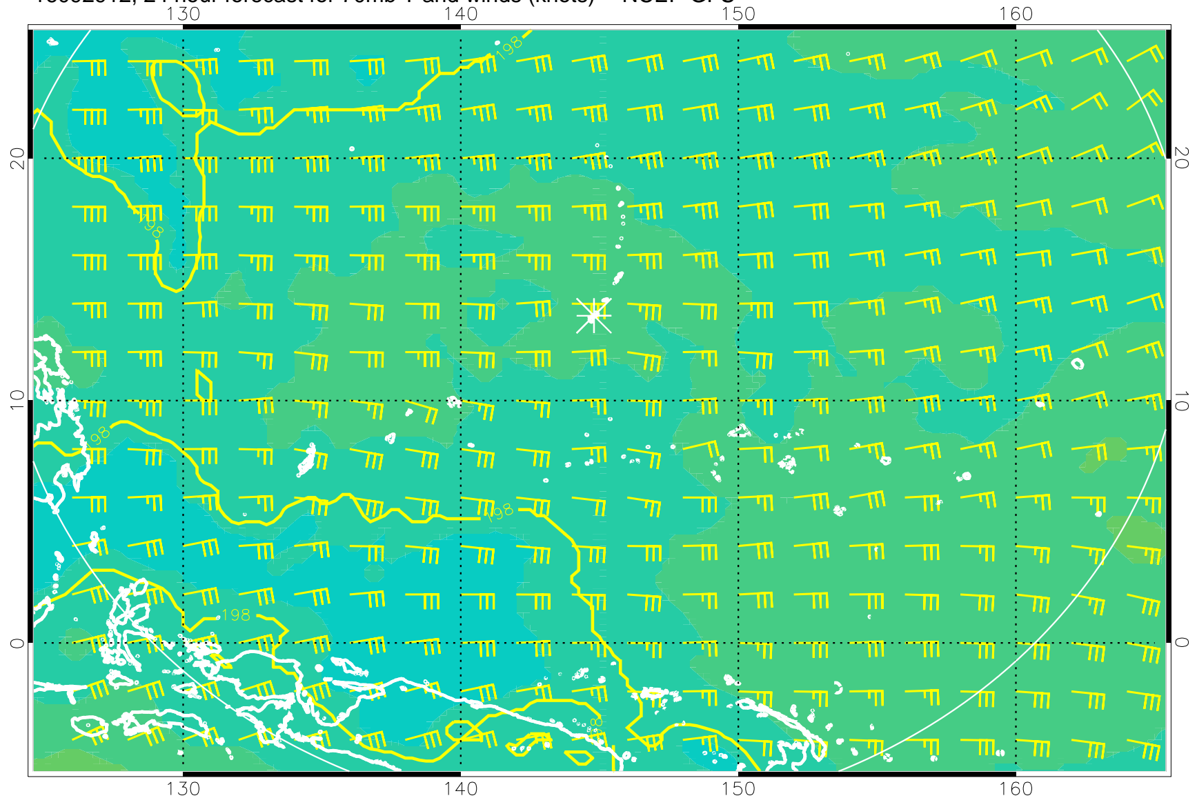
16092912, 24 hour forecast for 70mb T and winds (knots) -- NCEP GFS
