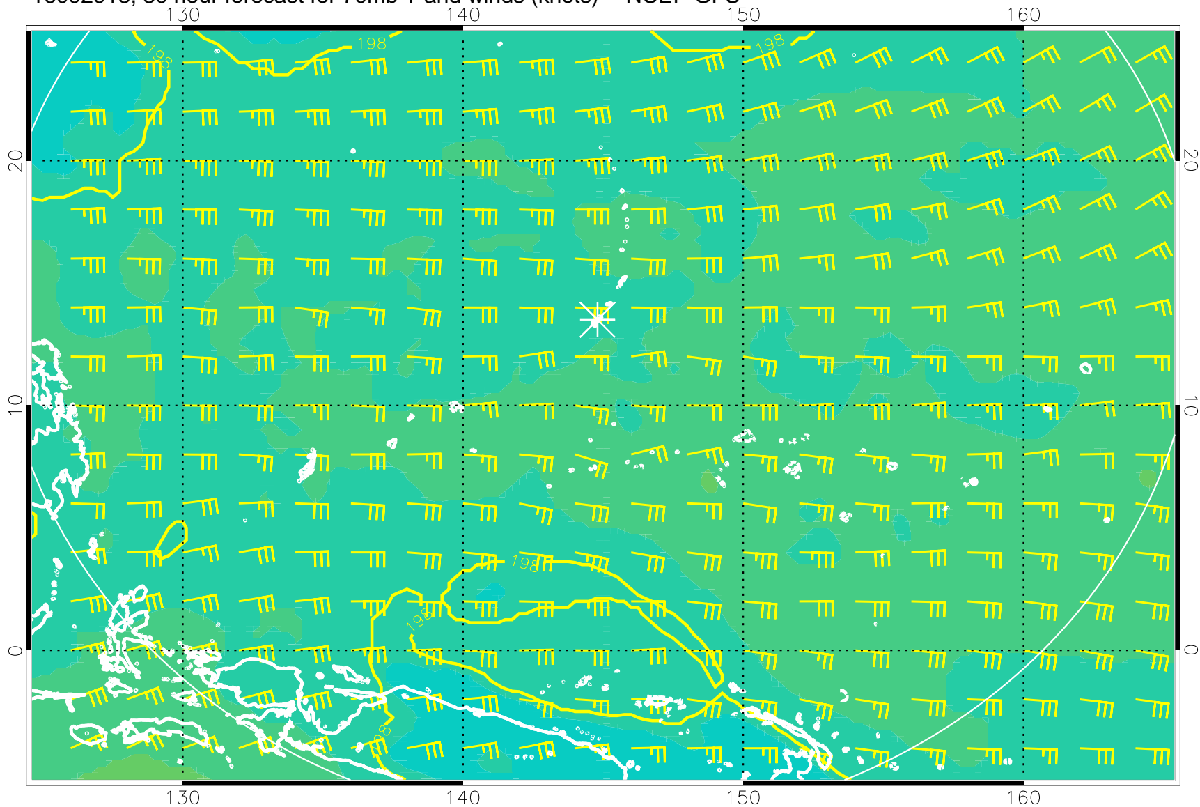
16092918, 30 hour forecast for 70mb T and winds (knots) -- NCEP GFS
