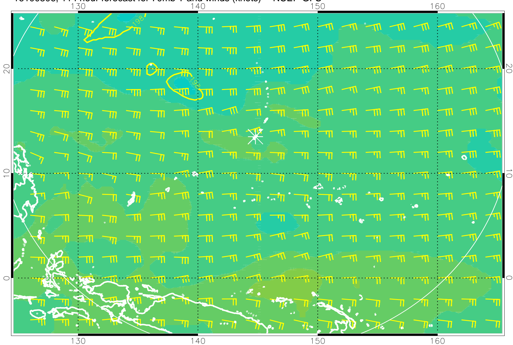
16100306, 114 hour forecast for 70mb T and winds (knots) -- NCEP GFS
