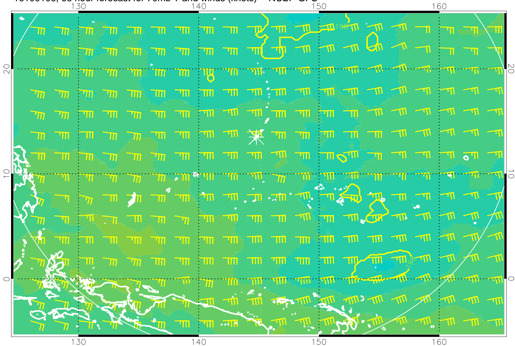
16100106, 66 hour forecast for 70mb T and winds (knots) -- NCEP GFS
