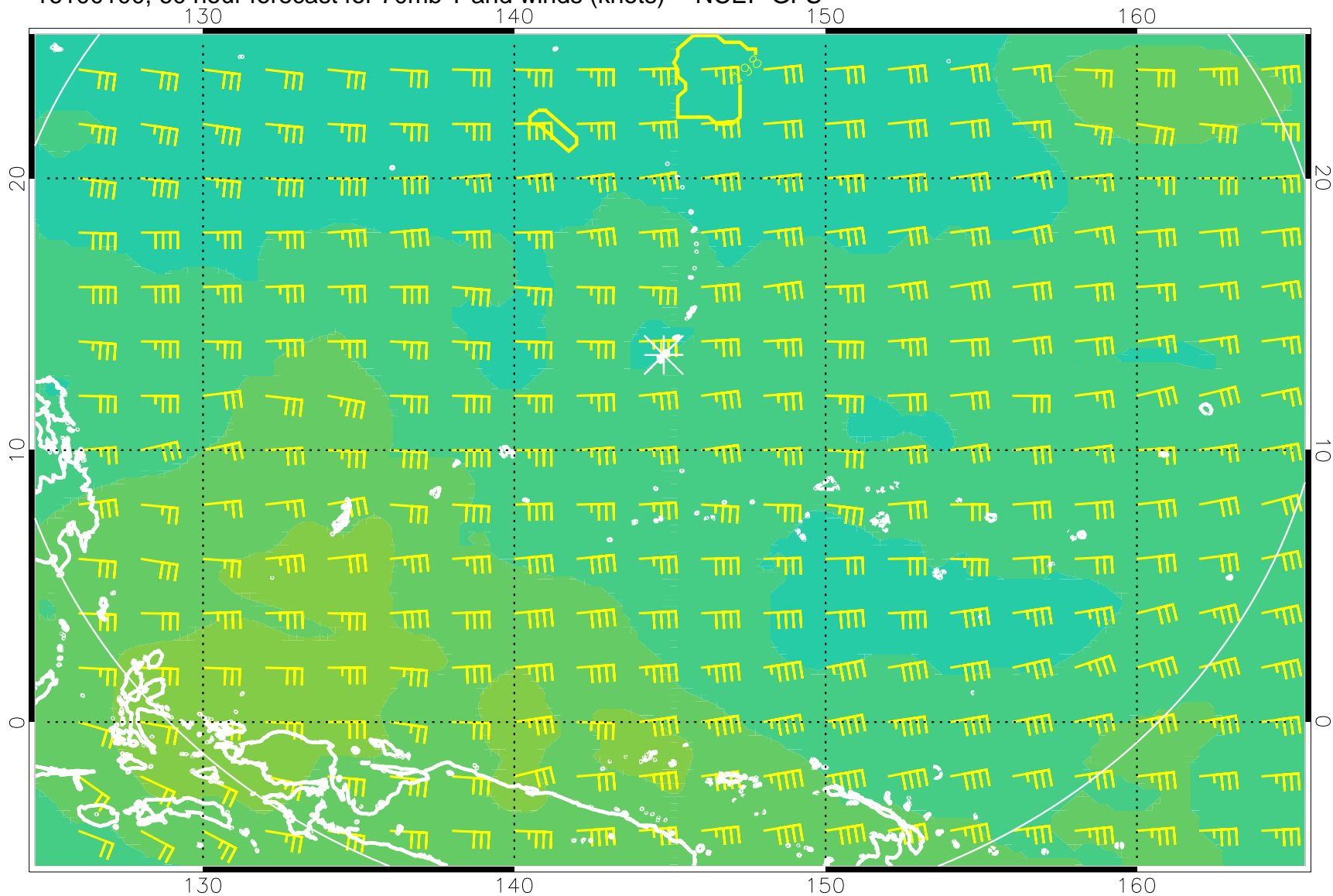
16100100, 60 hour forecast for 70mb T and winds (knots) -- NCEP GFS
