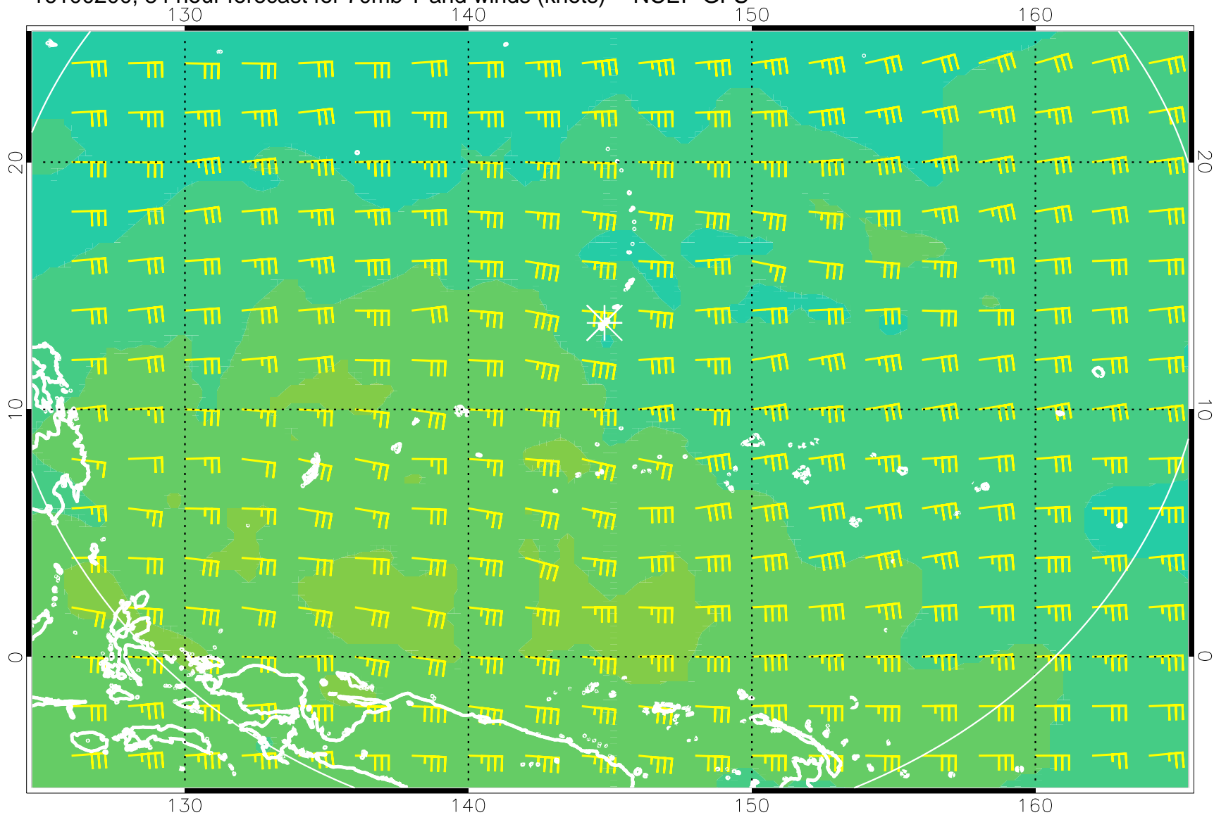
16100200, 84 hour forecast for 70mb T and winds (knots) -- NCEP GFS
