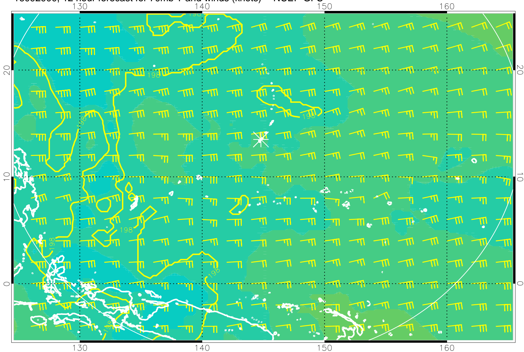
16092900, 12 hour forecast for 70mb T and winds (knots) -- NCEP GFS
