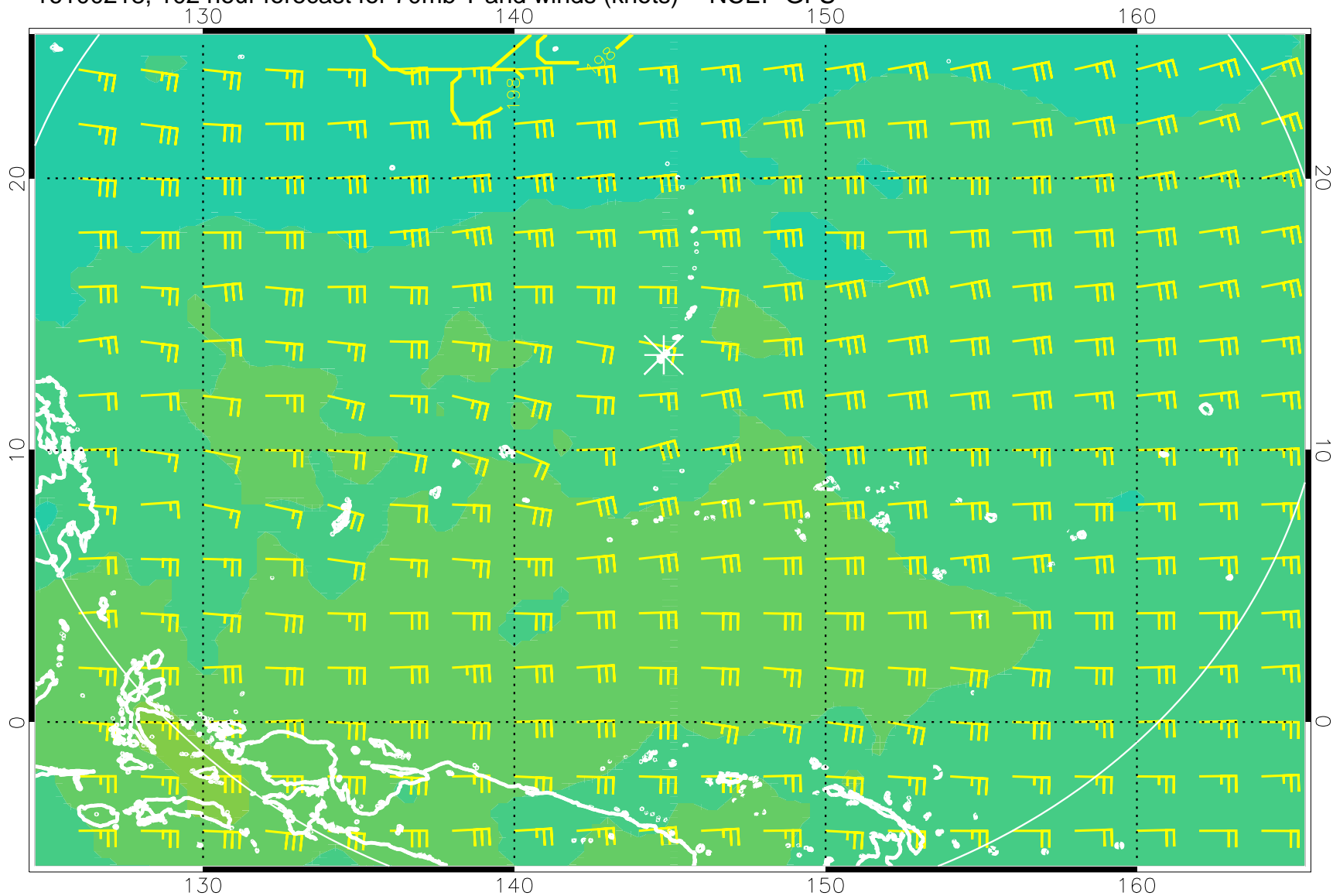
16100218, 102 hour forecast for 70mb T and winds (knots) -- NCEP GFS
