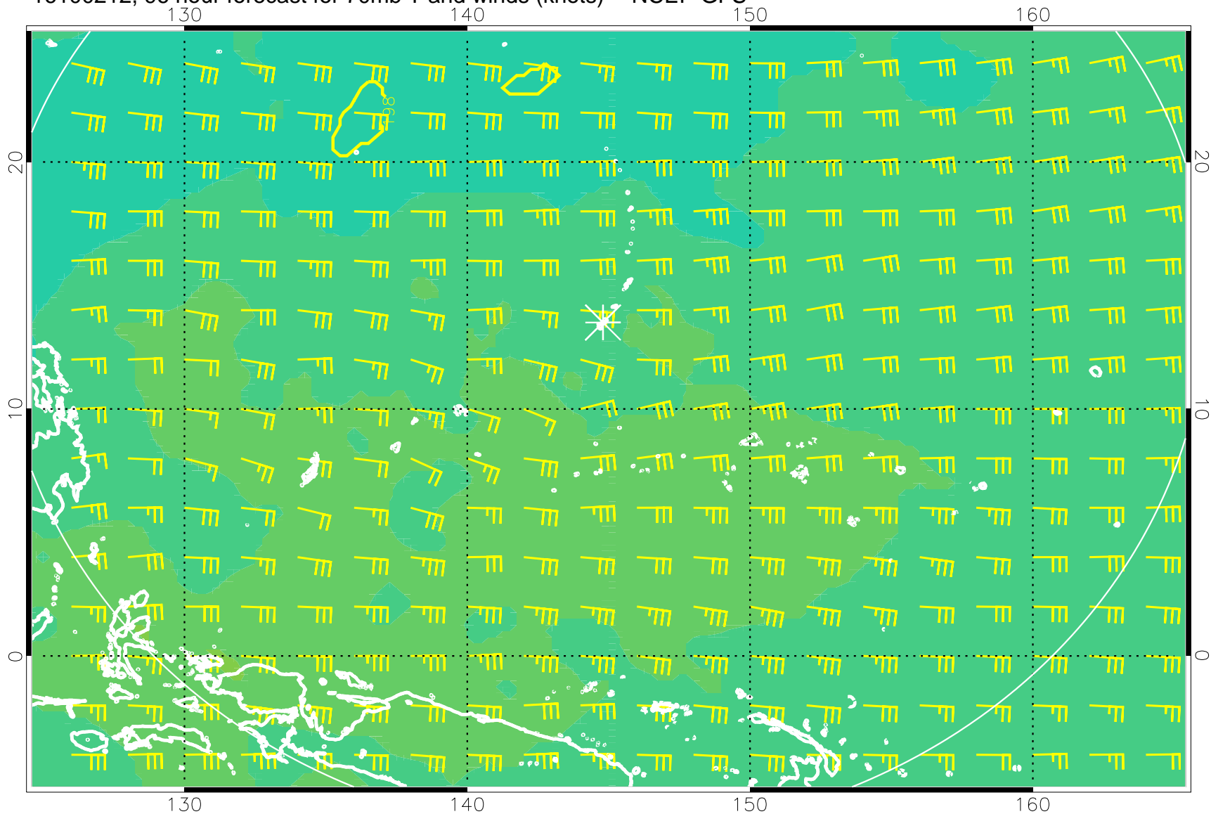
16100212, 96 hour forecast for 70mb T and winds (knots) -- NCEP GFS
