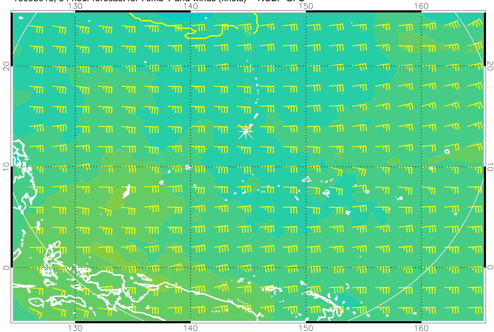
16093018, 54 hour forecast for 70mb T and winds (knots) -- NCEP GFS
