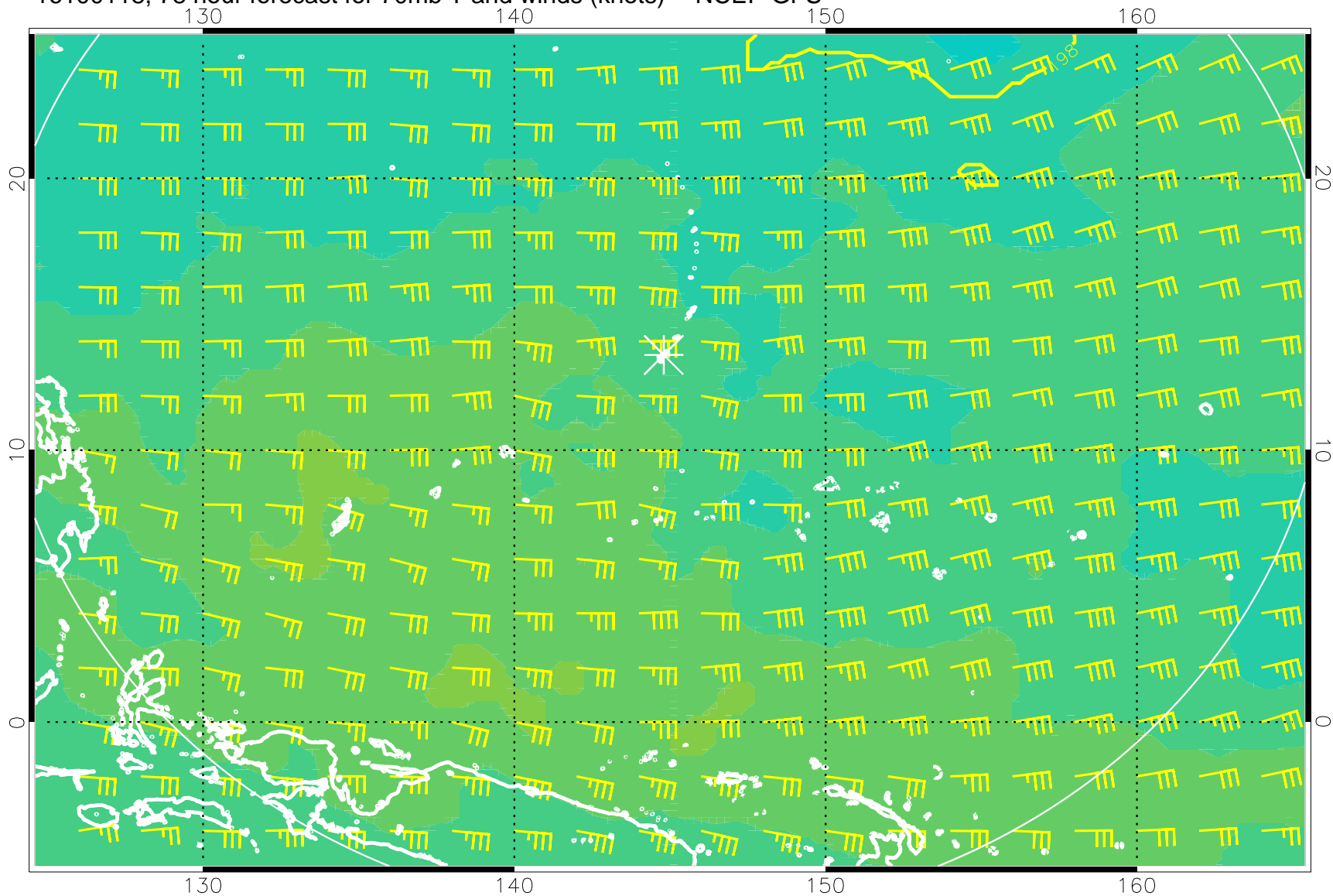
16100118, 78 hour forecast for 70mb T and winds (knots) -- NCEP GFS
