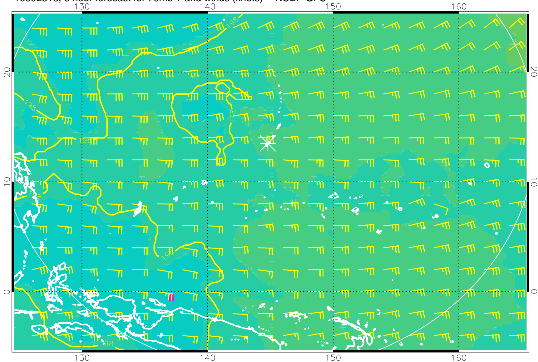
16092818, 6 hour forecast for 70mb T and winds (knots) -- NCEP GFS
