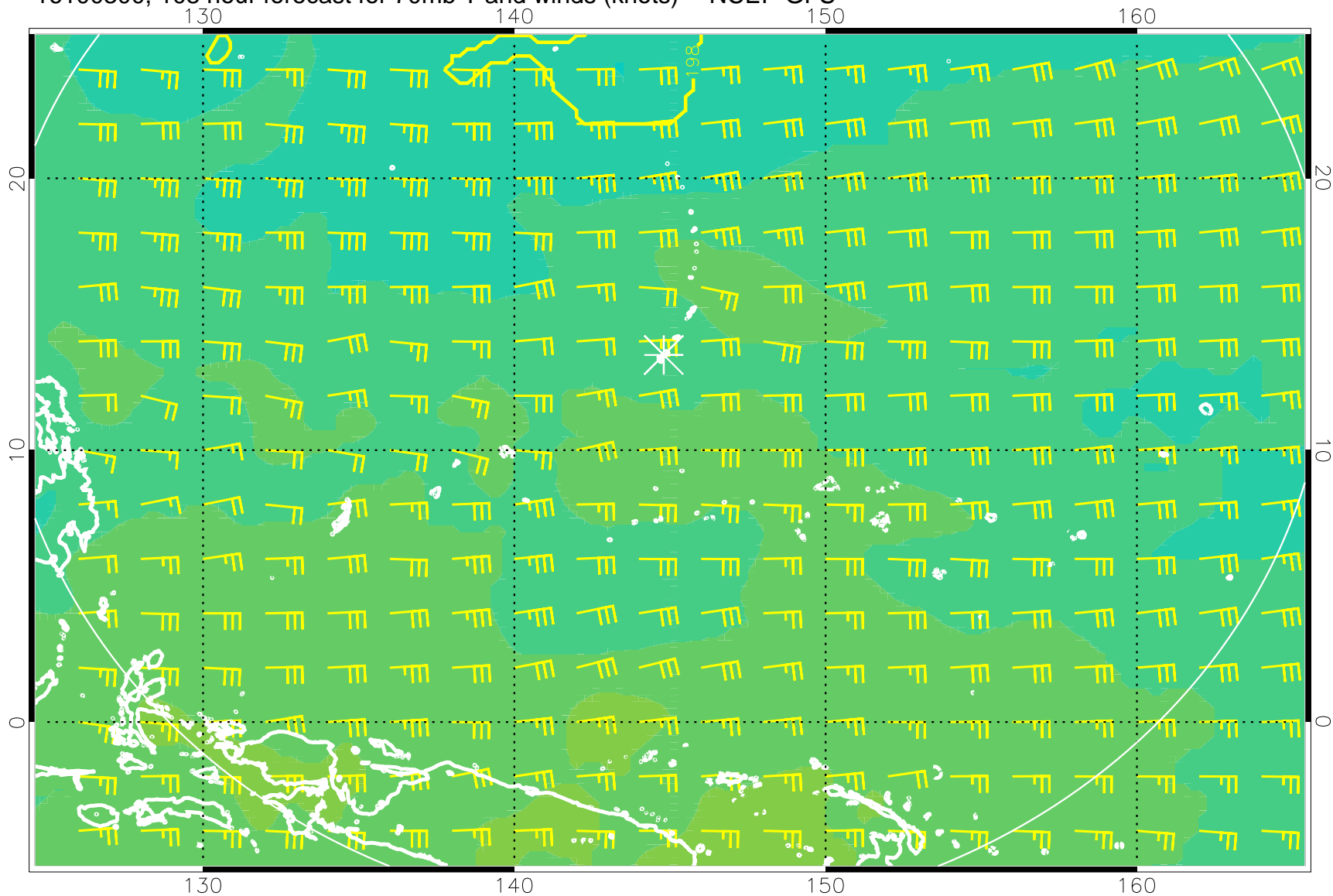
16100300, 108 hour forecast for 70mb T and winds (knots) -- NCEP GFS
