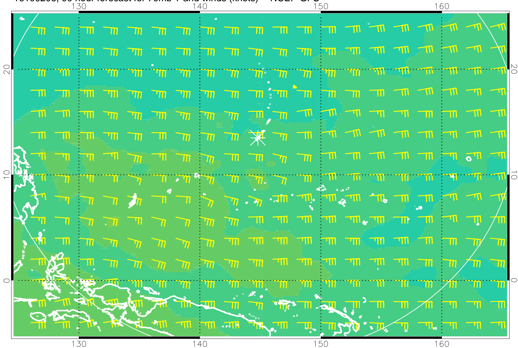
16100206, 90 hour forecast for 70mb T and winds (knots) -- NCEP GFS
