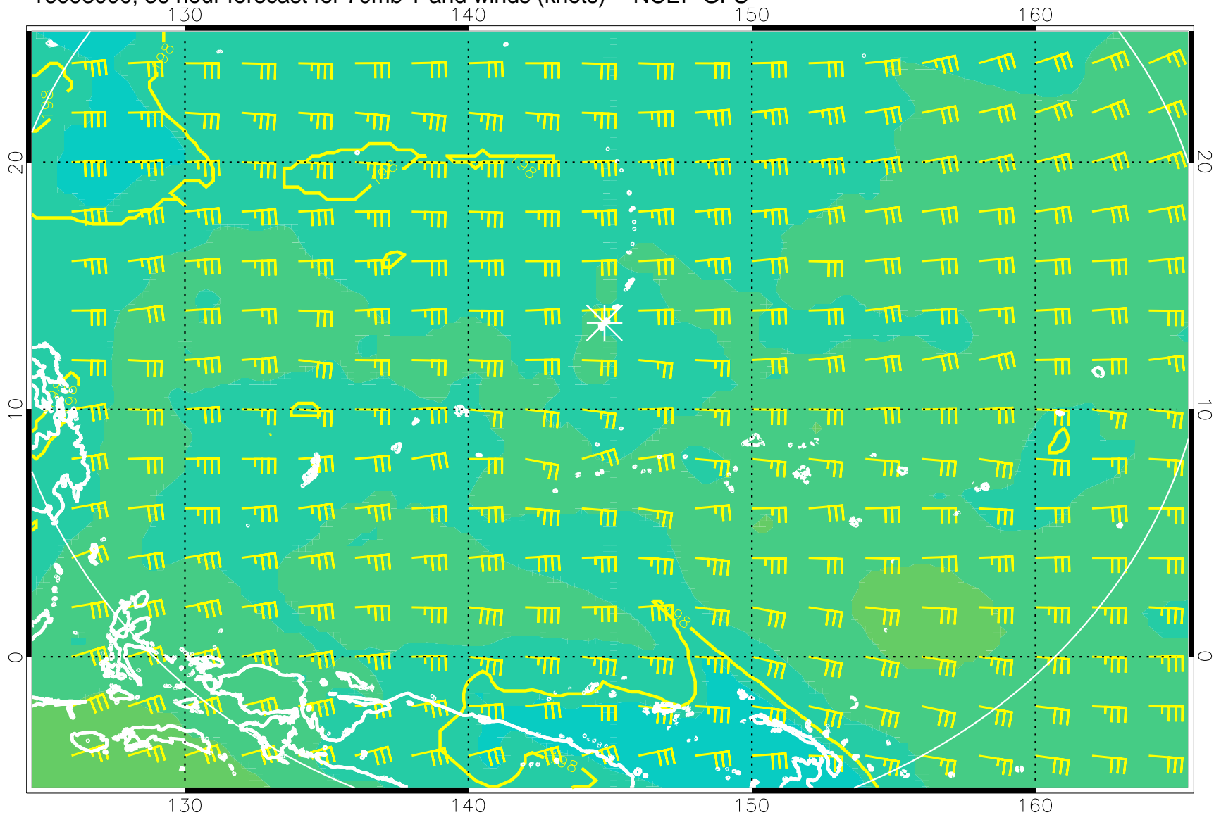
16093000, 36 hour forecast for 70mb T and winds (knots) -- NCEP GFS
