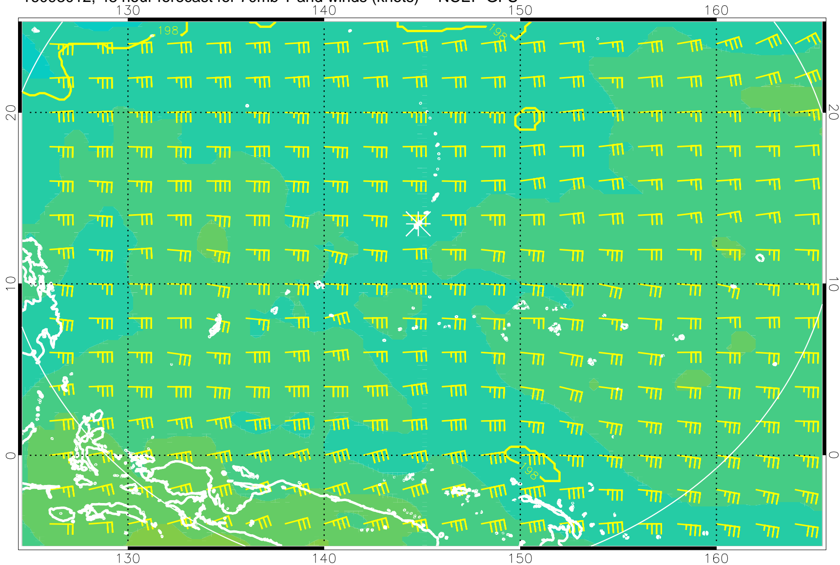
16093012, 48 hour forecast for 70mb T and winds (knots) -- NCEP GFS
