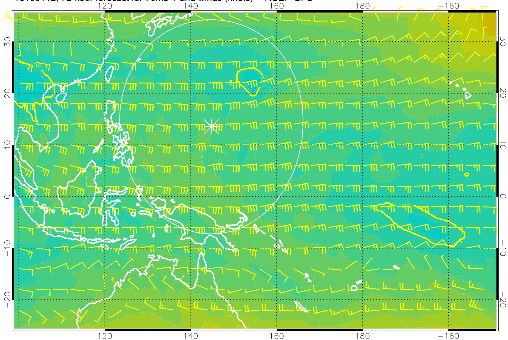
16100112, 72 hour forecast for 70mb T and winds (knots) -- NCEP GFS
