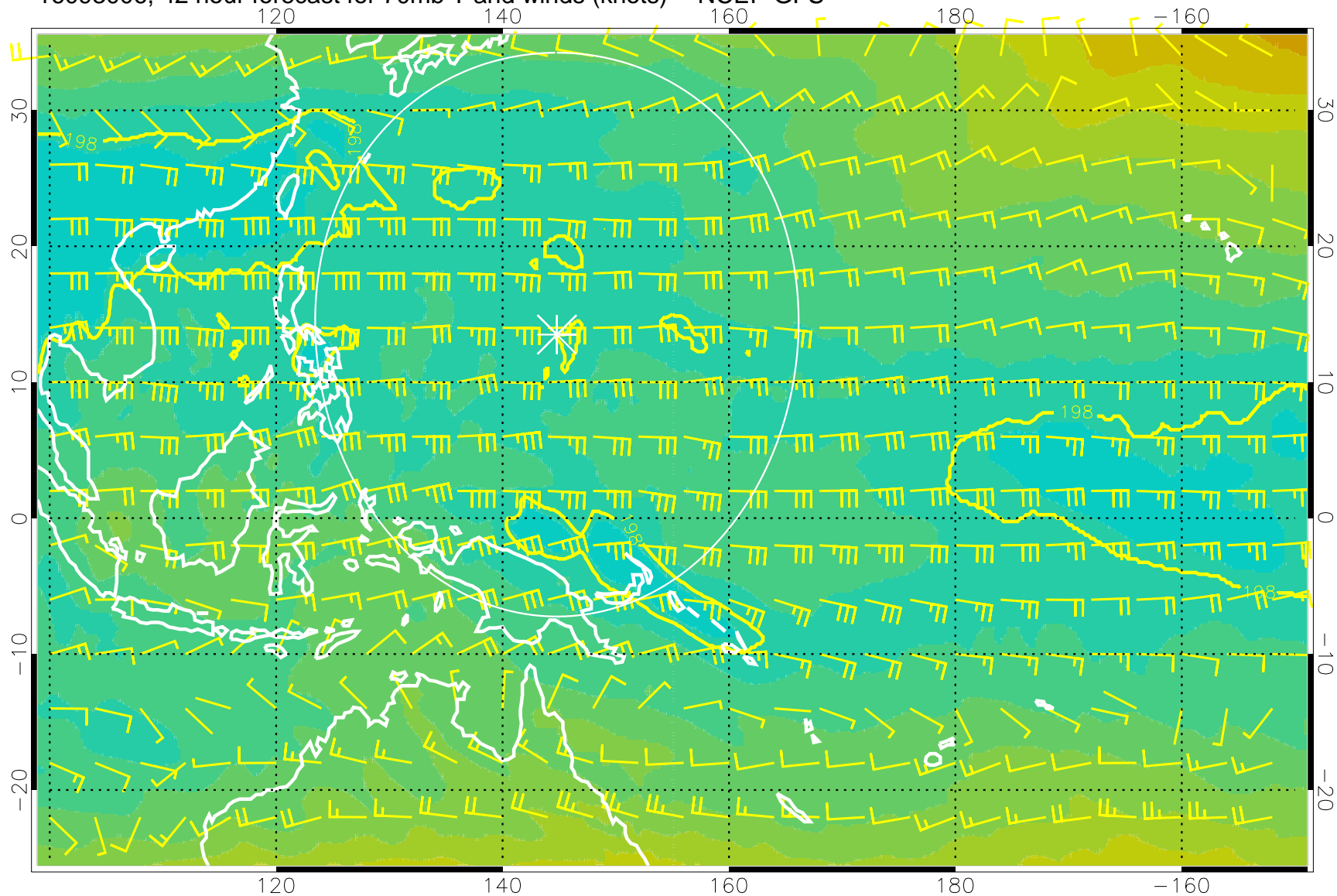
16093006, 42 hour forecast for 70mb T and winds (knots) -- NCEP GFS
