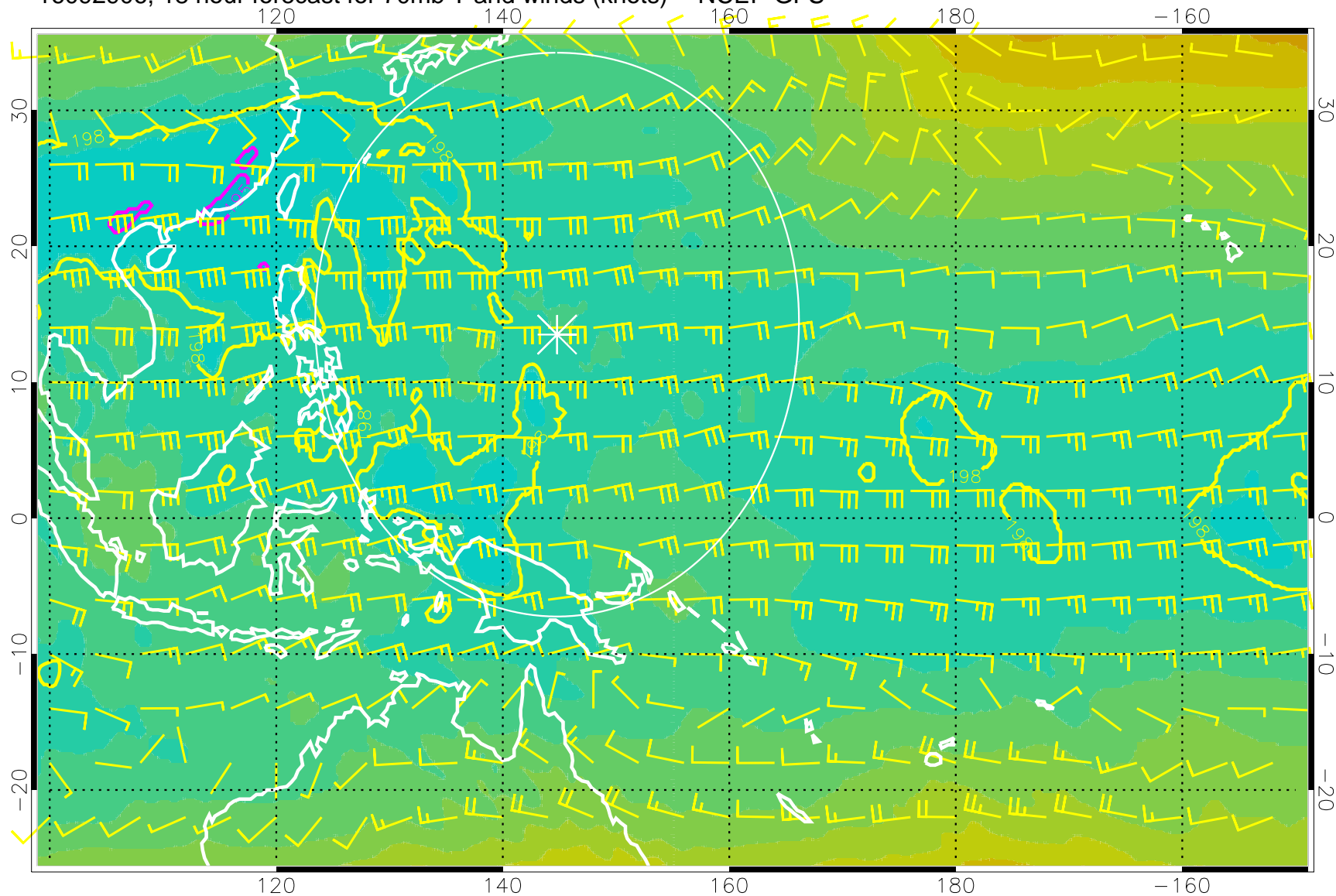
16092906, 18 hour forecast for 70mb T and winds (knots) -- NCEP GFS
