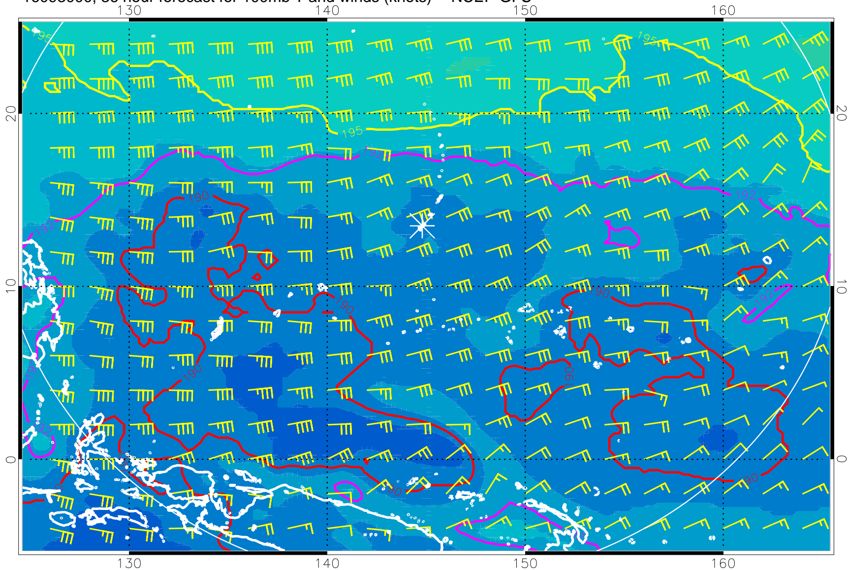
16093000, 36 hour forecast for 100mb T and winds (knots) -- NCEP GFS
