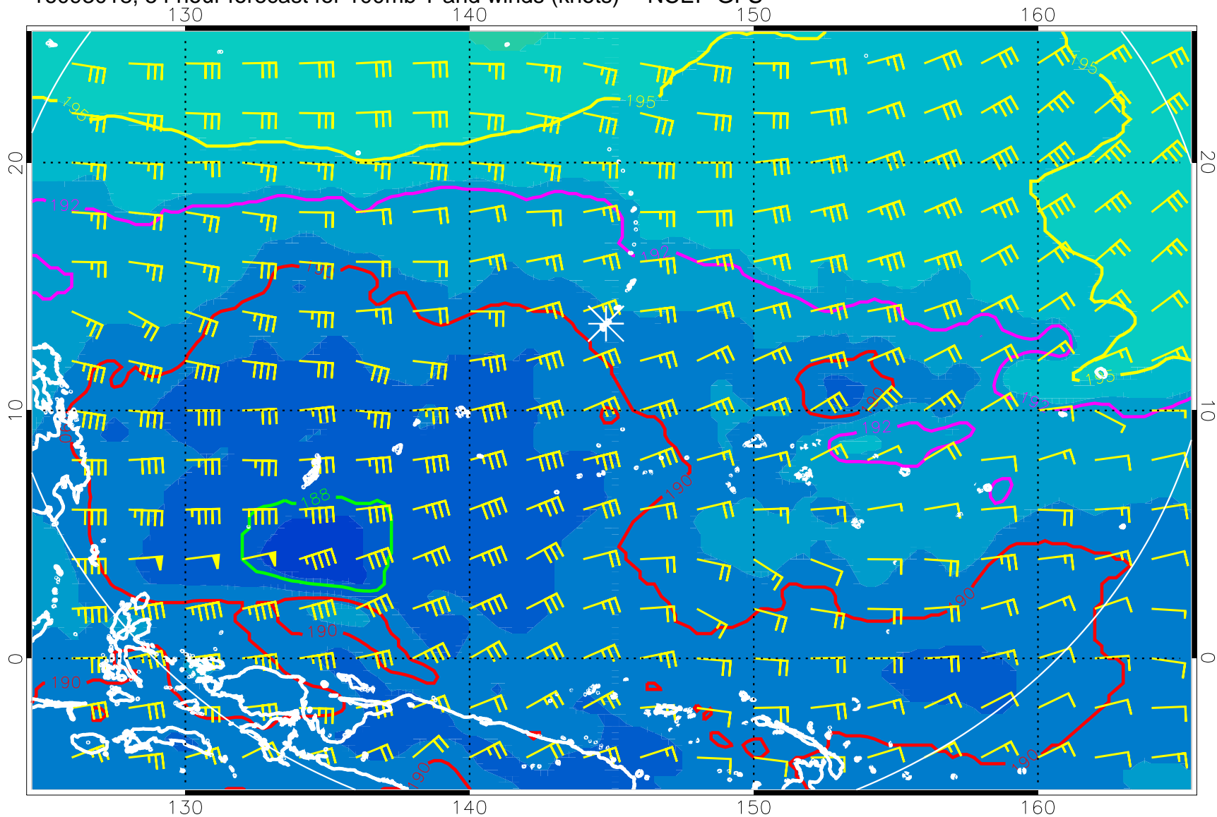
16093018, 54 hour forecast for 100mb T and winds (knots) -- NCEP GFS
