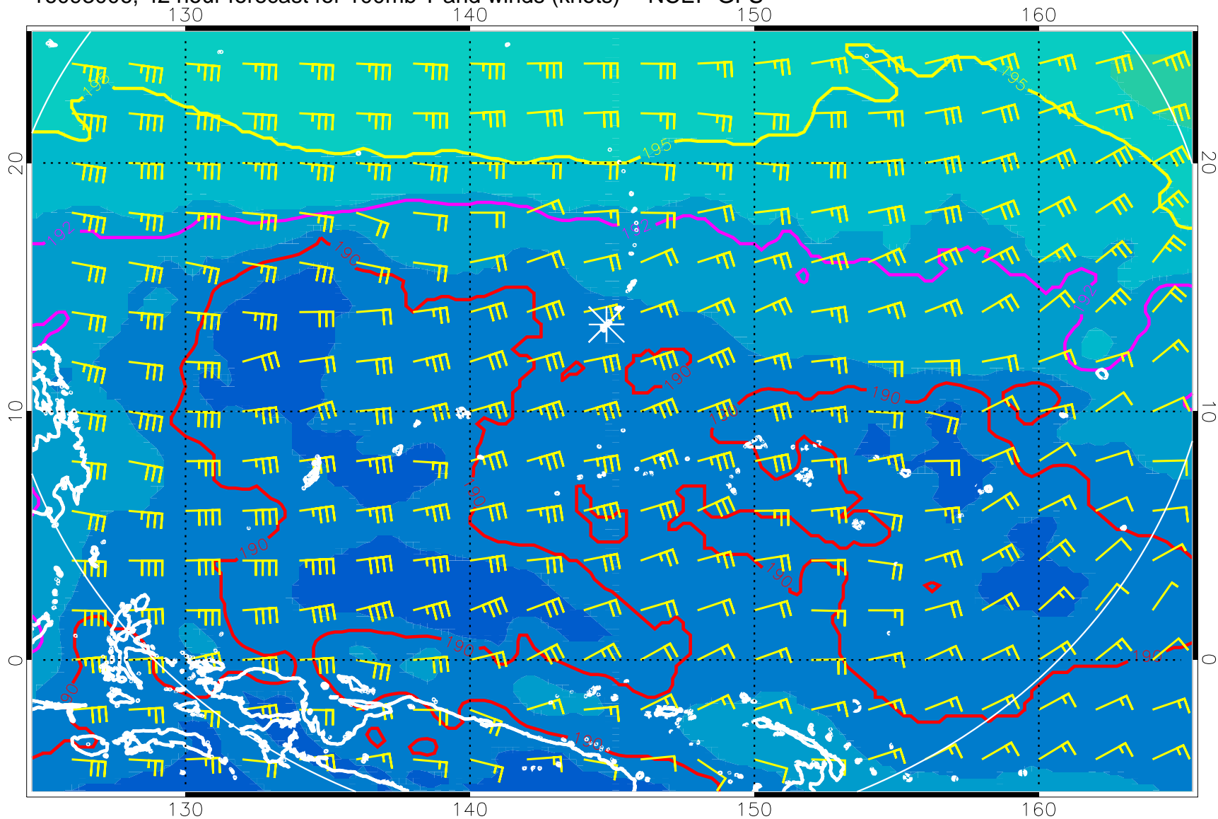
16093006, 42 hour forecast for 100mb T and winds (knots) -- NCEP GFS
