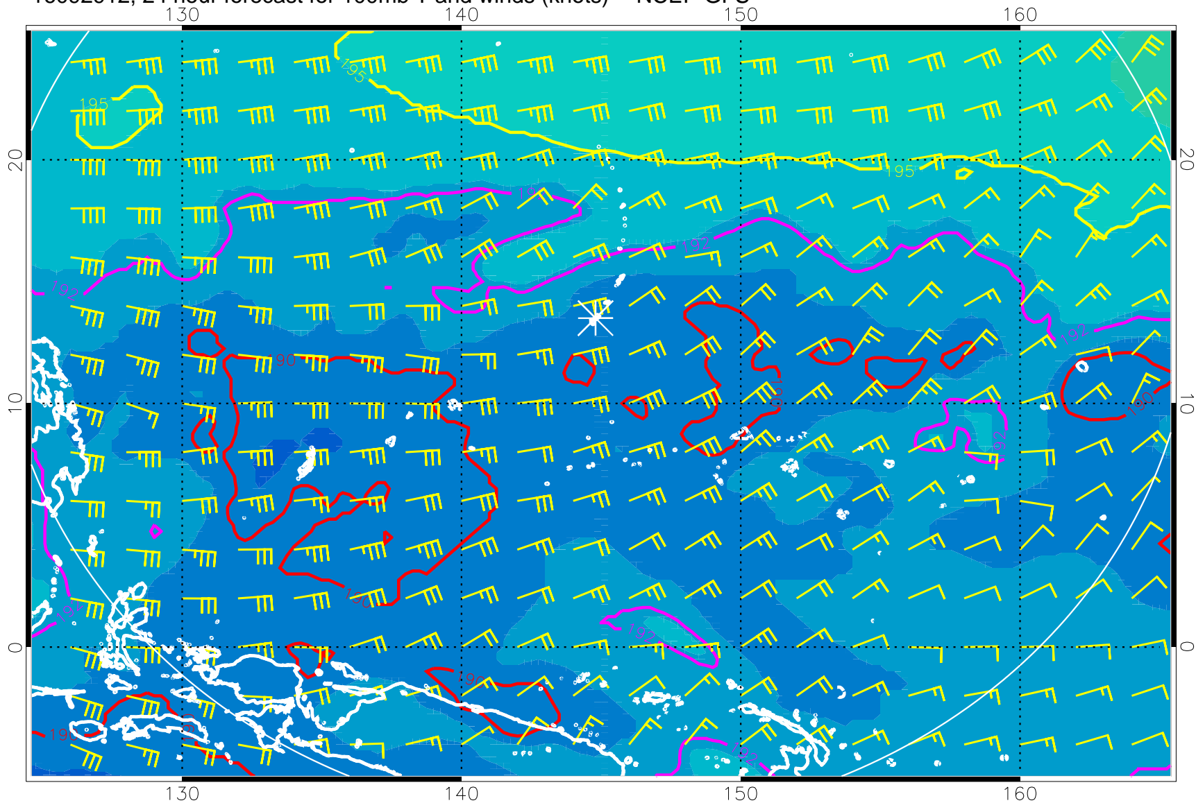
16092912, 24 hour forecast for 100mb T and winds (knots) -- NCEP GFS
