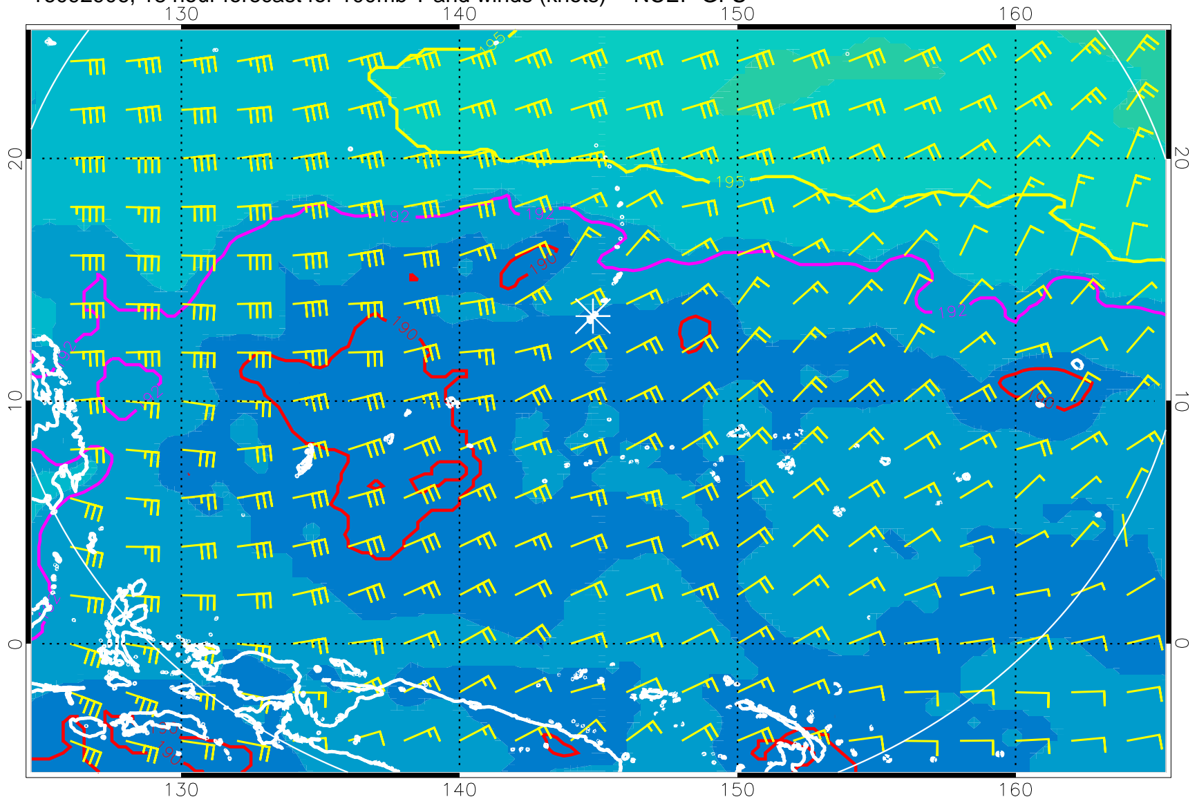
16092906, 18 hour forecast for 100mb T and winds (knots) -- NCEP GFS
