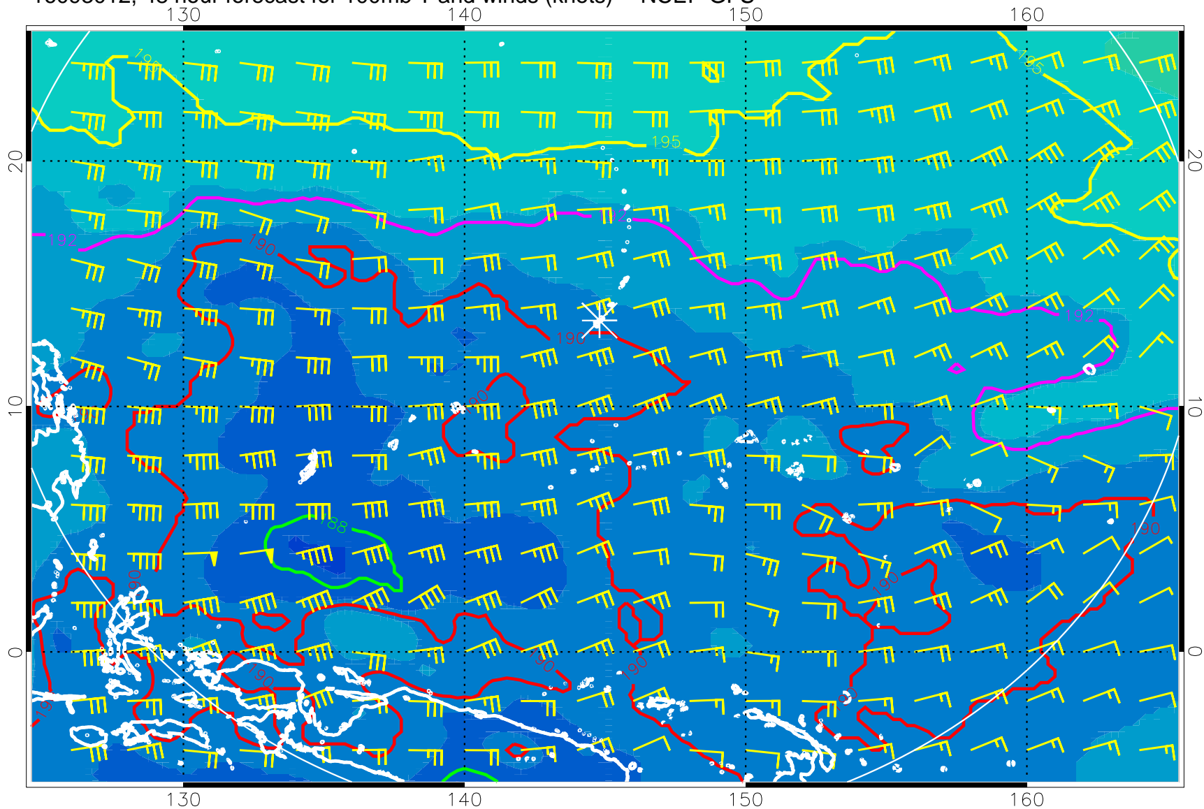
16093012, 48 hour forecast for 100mb T and winds (knots) -- NCEP GFS
