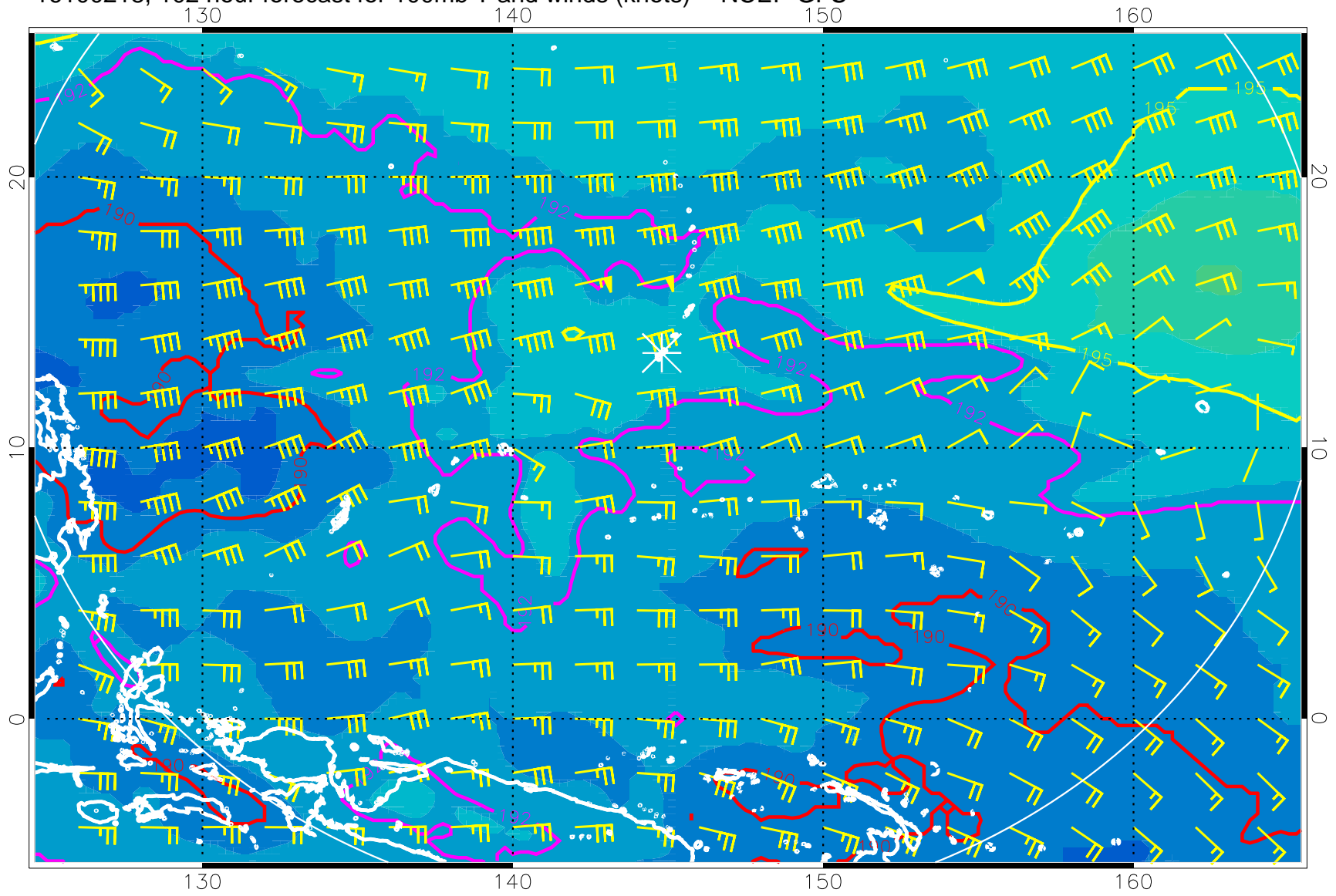
16100218, 102 hour forecast for 100mb T and winds (knots) -- NCEP GFS
