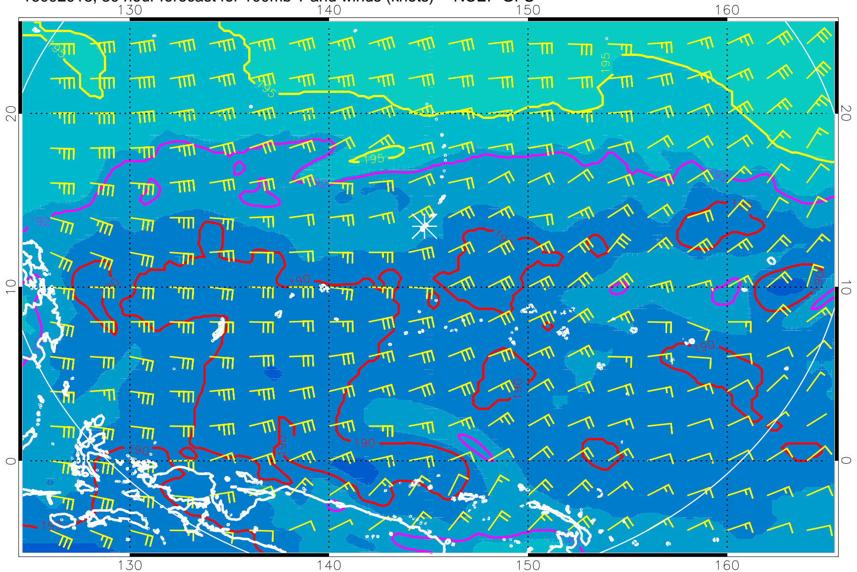
16092918, 30 hour forecast for 100mb T and winds (knots) -- NCEP GFS
