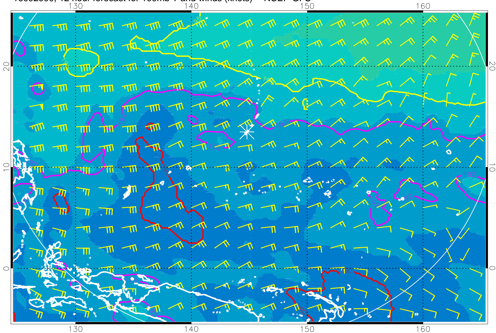
16092900, 12 hour forecast for 100mb T and winds (knots) -- NCEP GFS
