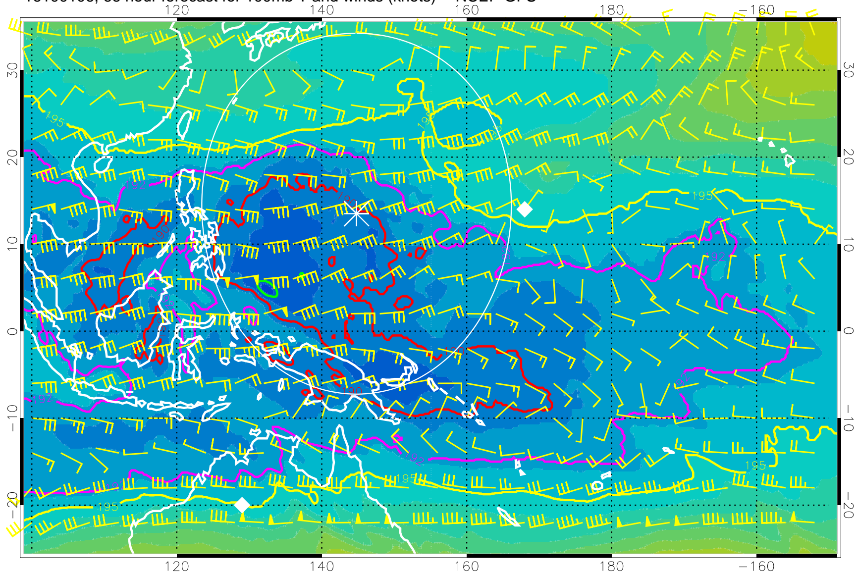
16100106, 66 hour forecast for 100mb T and winds (knots) -- NCEP GFS
