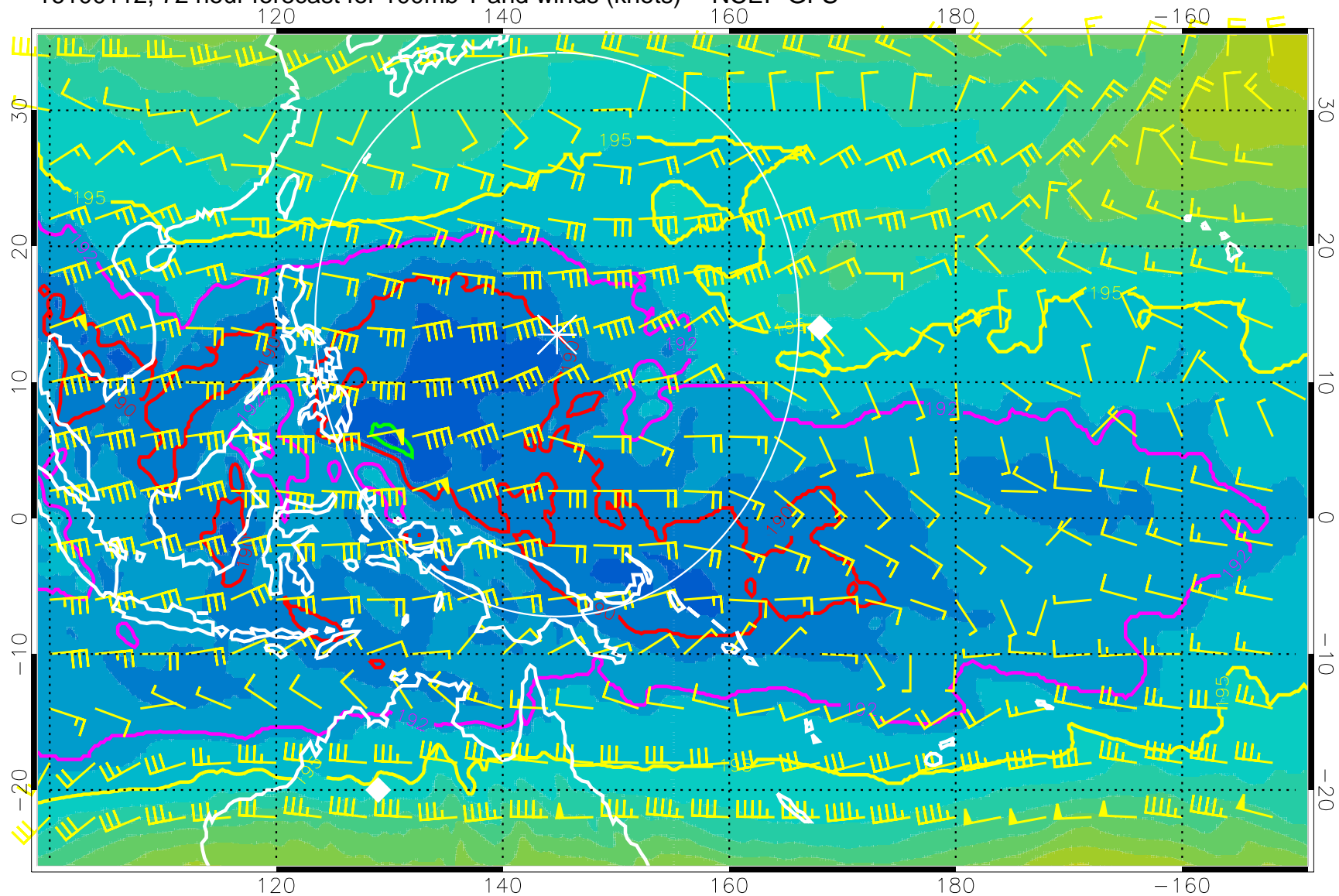
16100112, 72 hour forecast for 100mb T and winds (knots) -- NCEP GFS
