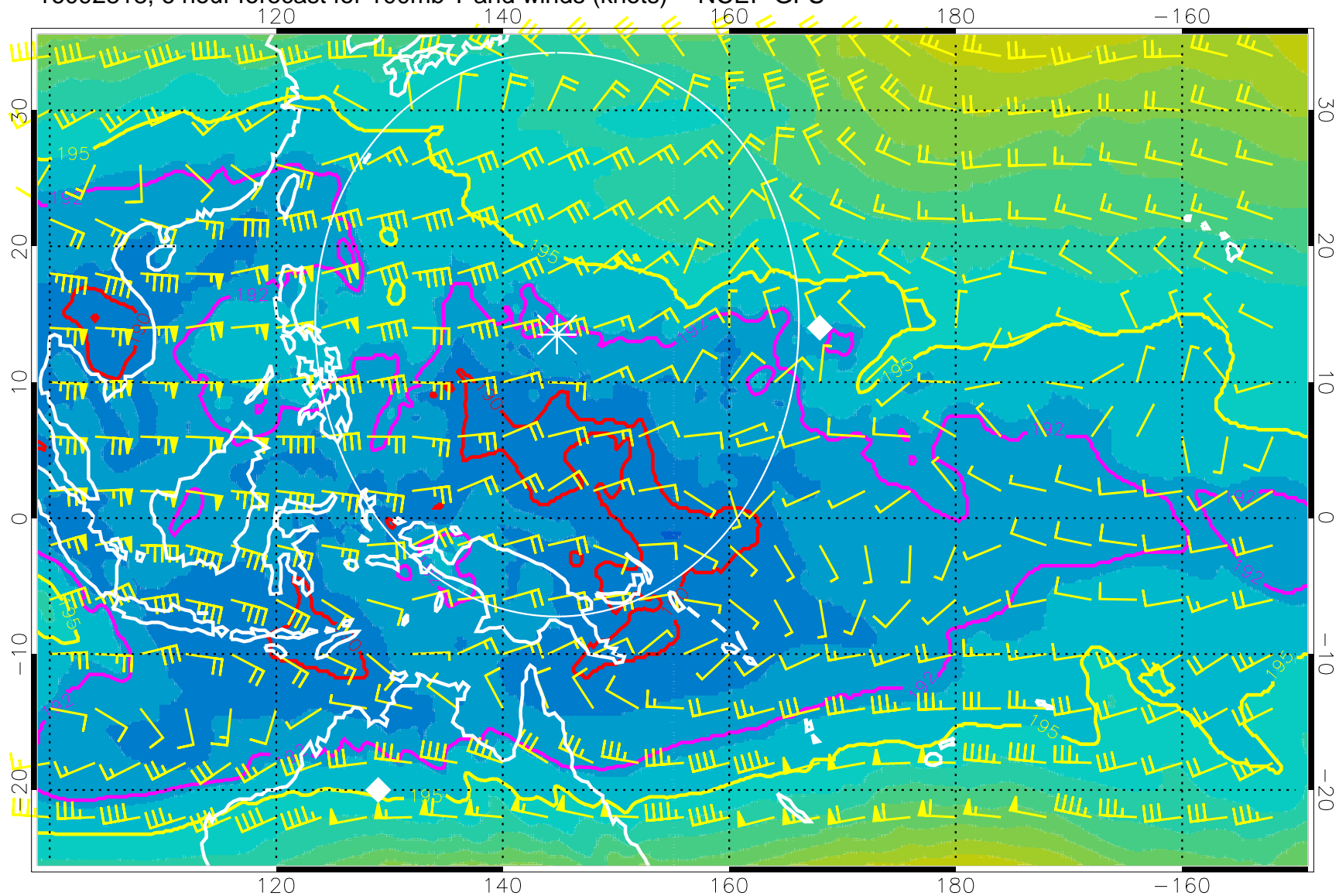
16092818, 6 hour forecast for 100mb T and winds (knots) -- NCEP GFS
