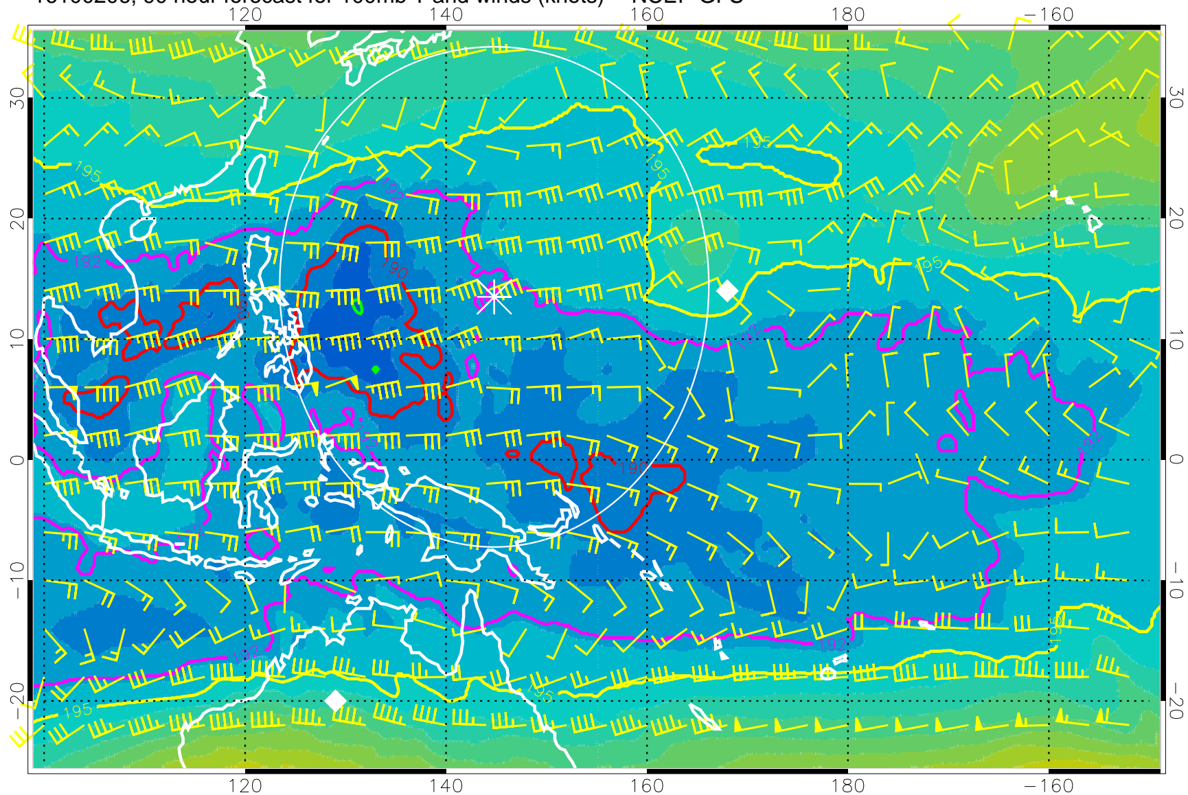
16100206, 90 hour forecast for 100mb T and winds (knots) -- NCEP GFS
