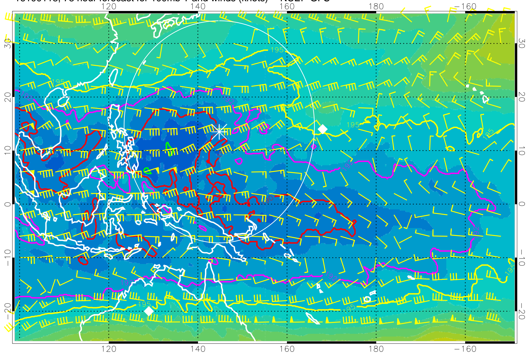
16100118, 78 hour forecast for 100mb T and winds (knots) -- NCEP GFS
