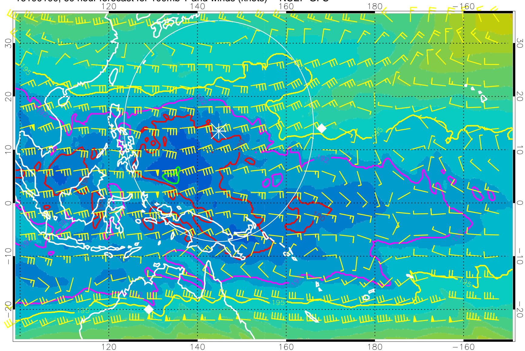
16100100, 60 hour forecast for 100mb T and winds (knots) -- NCEP GFS
