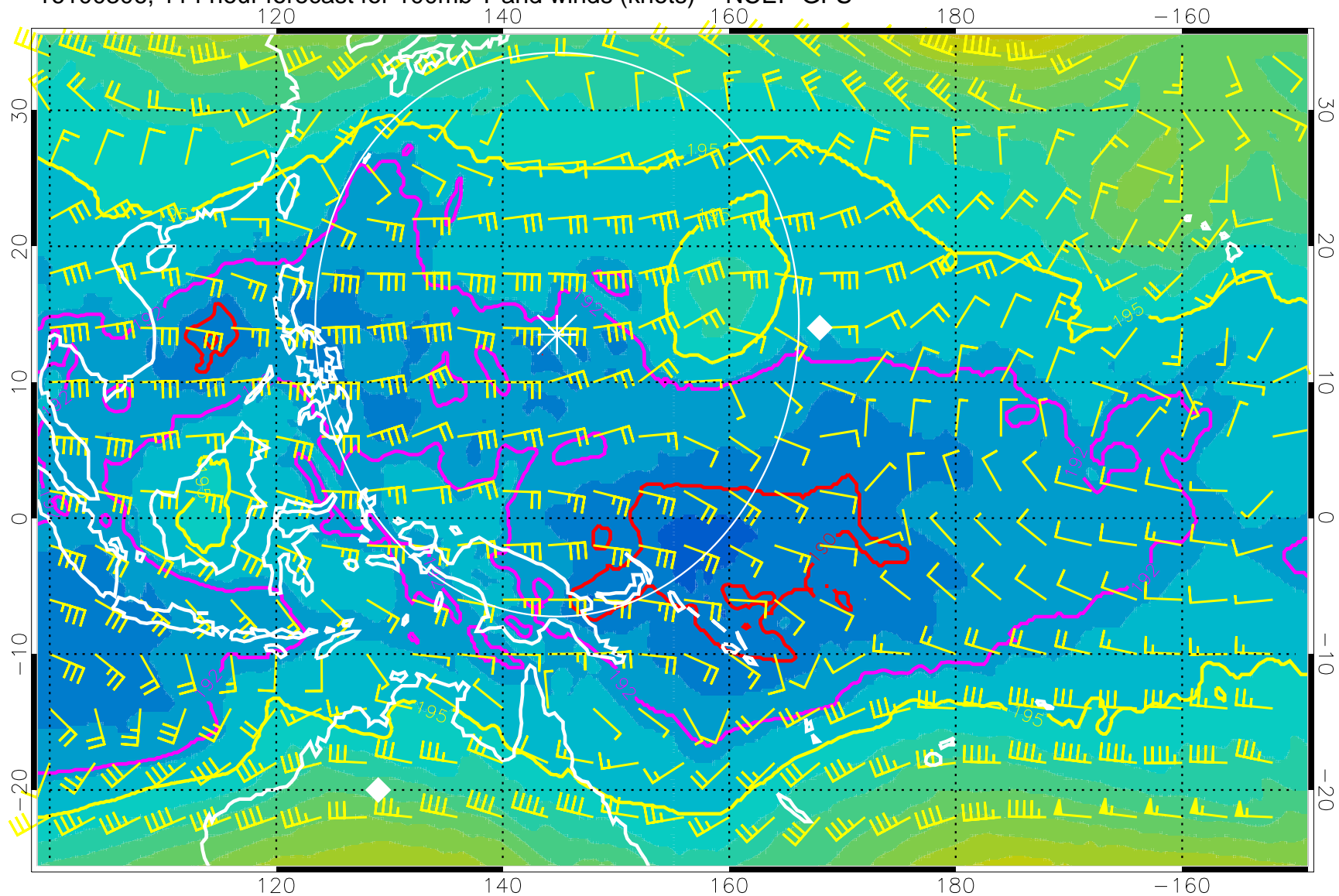
16100306, 114 hour forecast for 100mb T and winds (knots) -- NCEP GFS
