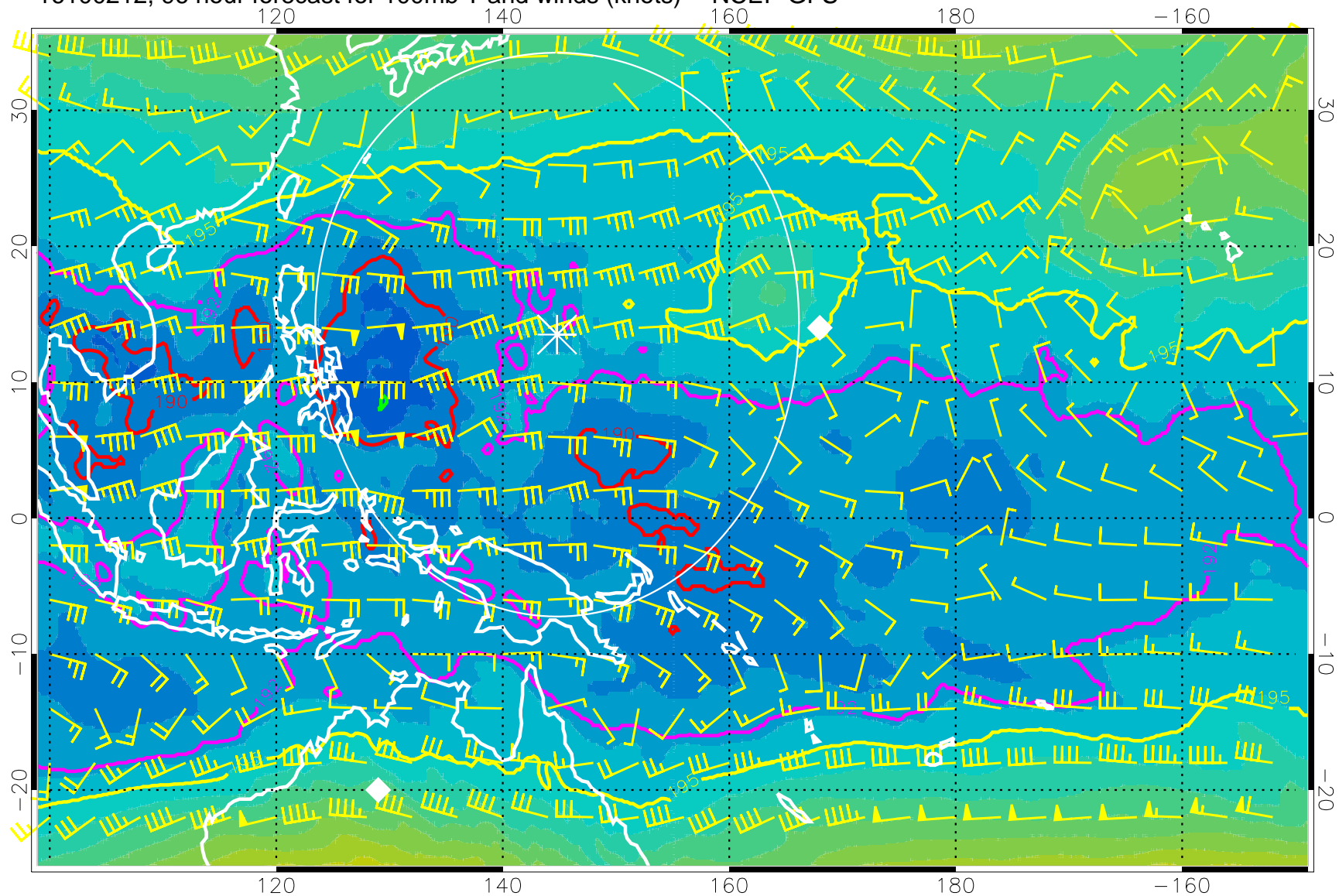
16100212, 96 hour forecast for 100mb T and winds (knots) -- NCEP GFS
