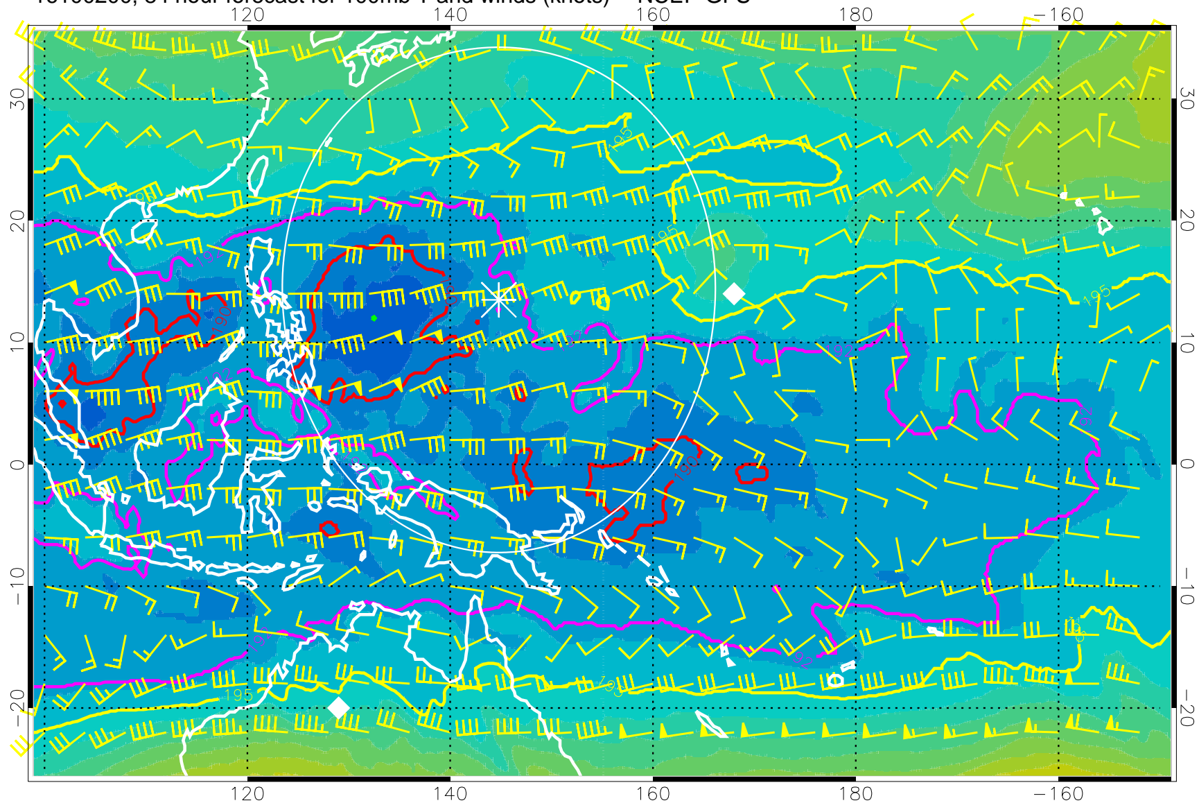
16100200, 84 hour forecast for 100mb T and winds (knots) -- NCEP GFS
