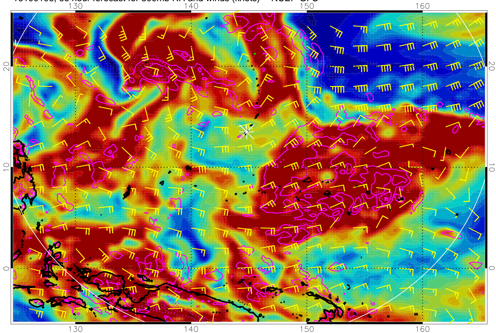
16100106, 66 hour forecast for 300mb RH and winds (knots) -- NCEP GFS
