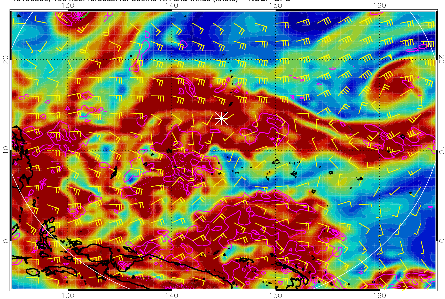
16100300, 108 hour forecast for 300mb RH and winds (knots) -- NCEP GFS
