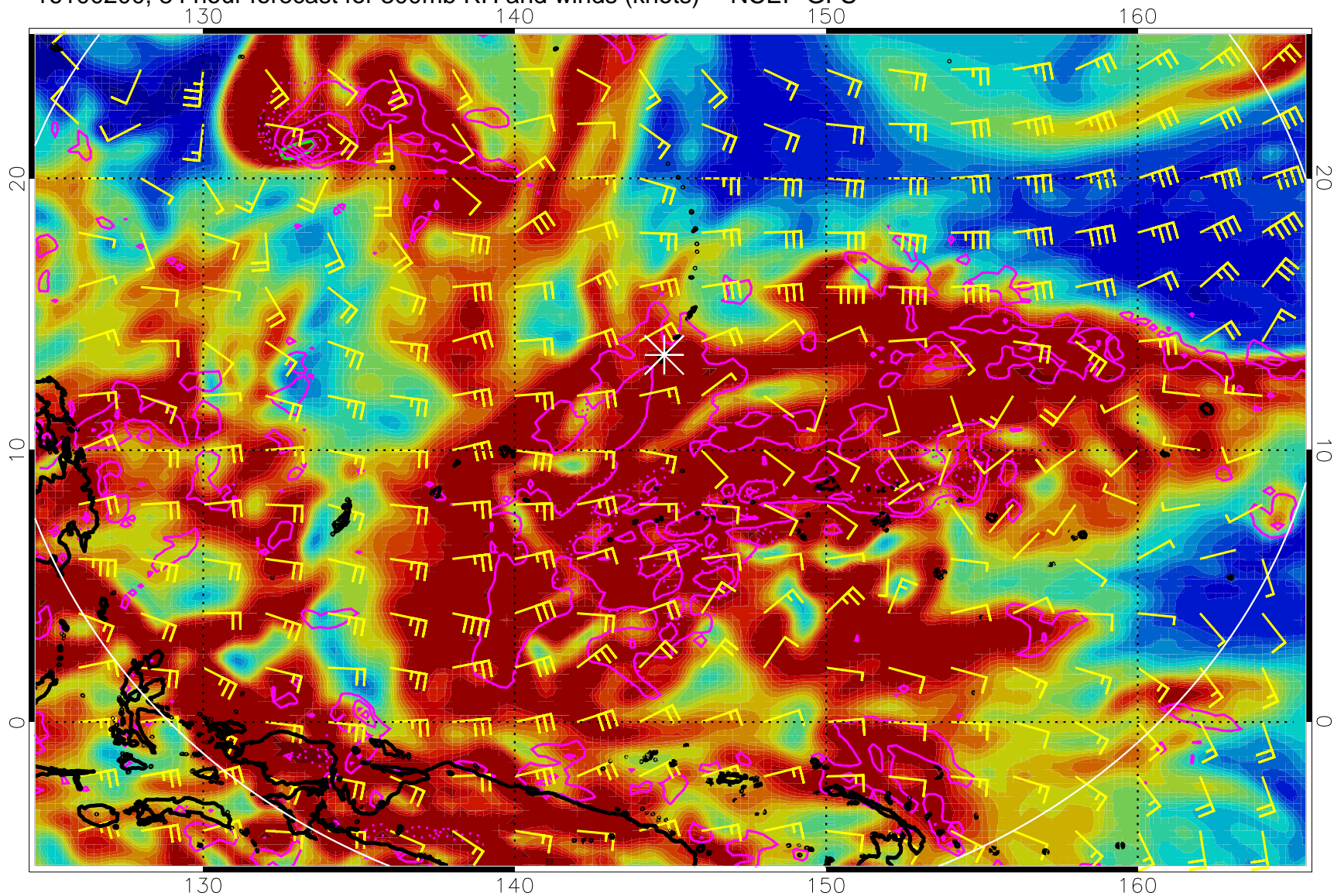
16100200, 84 hour forecast for 300mb RH and winds (knots) -- NCEP GFS
