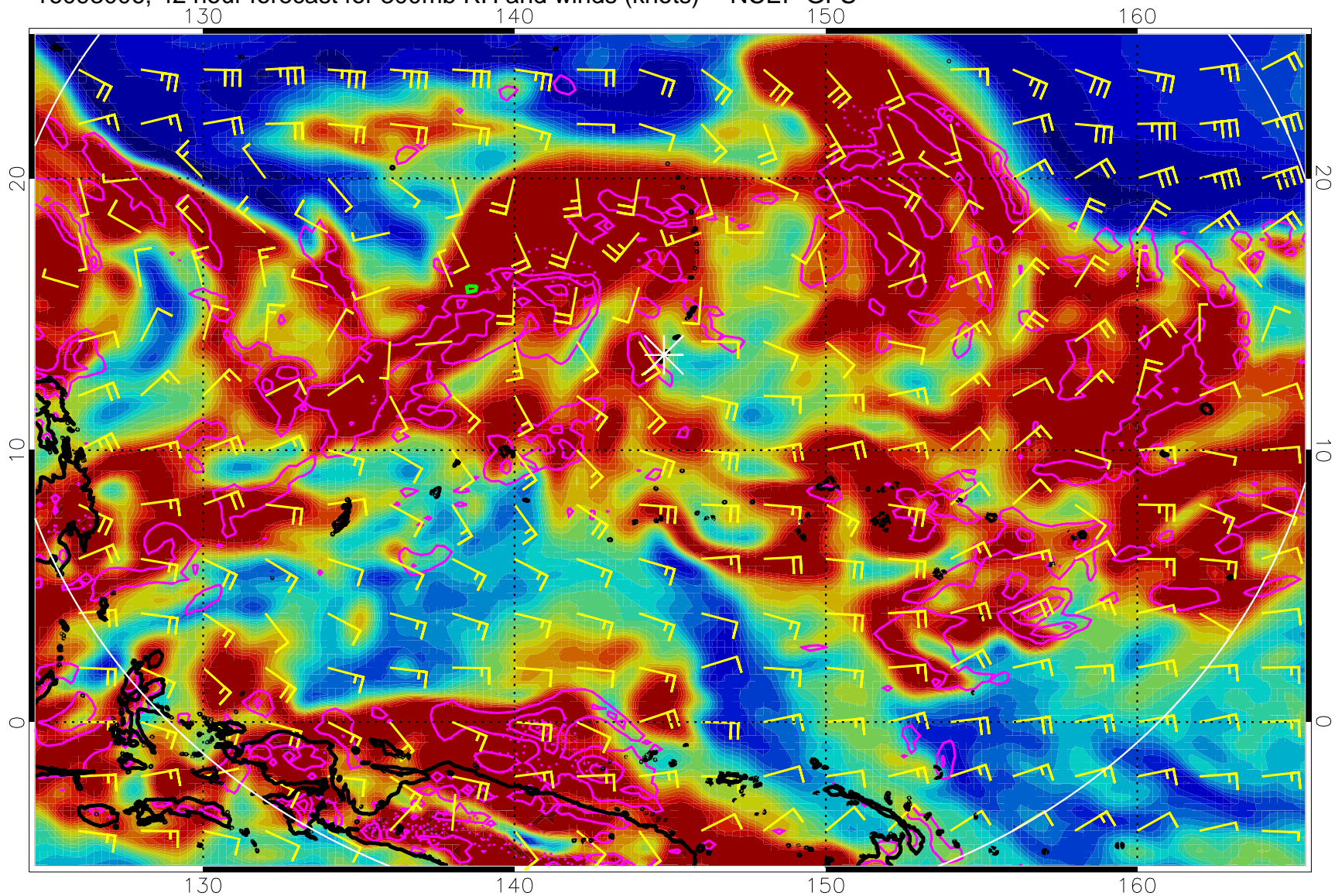
16093006, 42 hour forecast for 300mb RH and winds (knots) -- NCEP GFS
