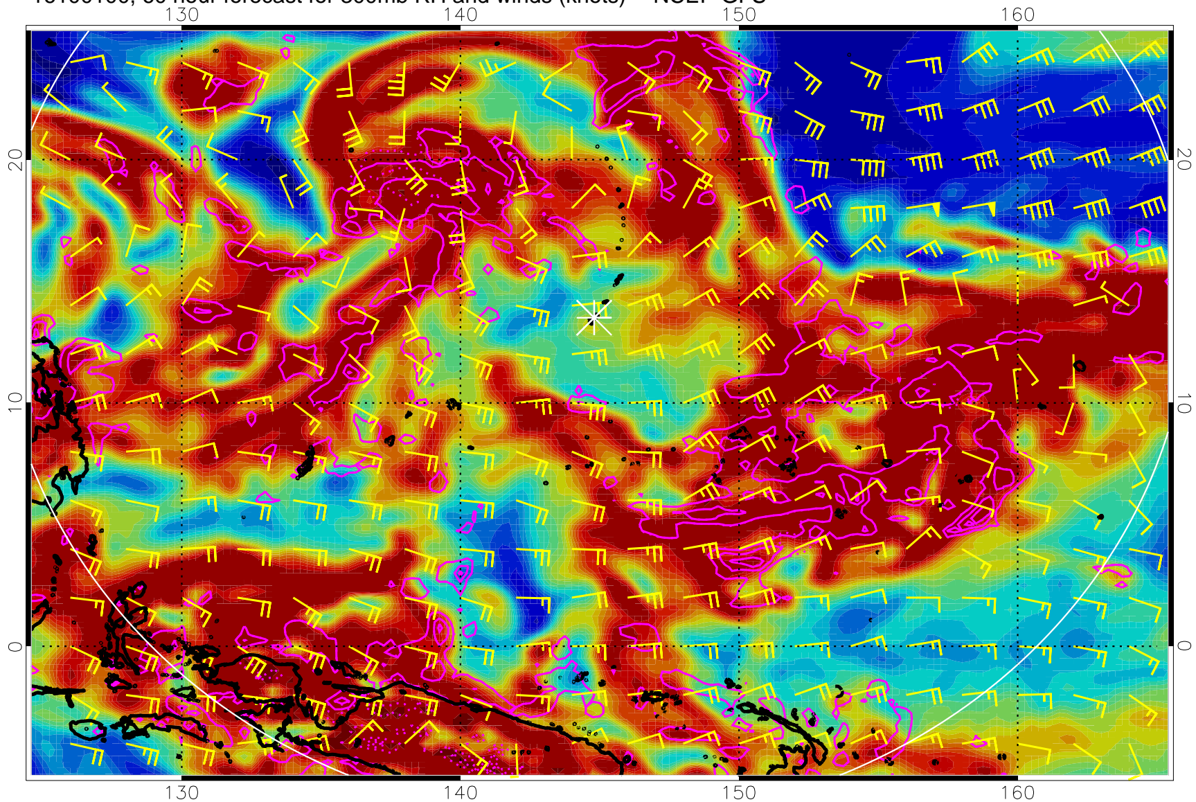
16100100, 60 hour forecast for 300mb RH and winds (knots) -- NCEP GFS
