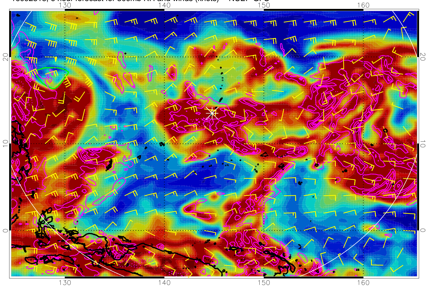
16092818, 6 hour forecast for 300mb RH and winds (knots) -- NCEP GFS
