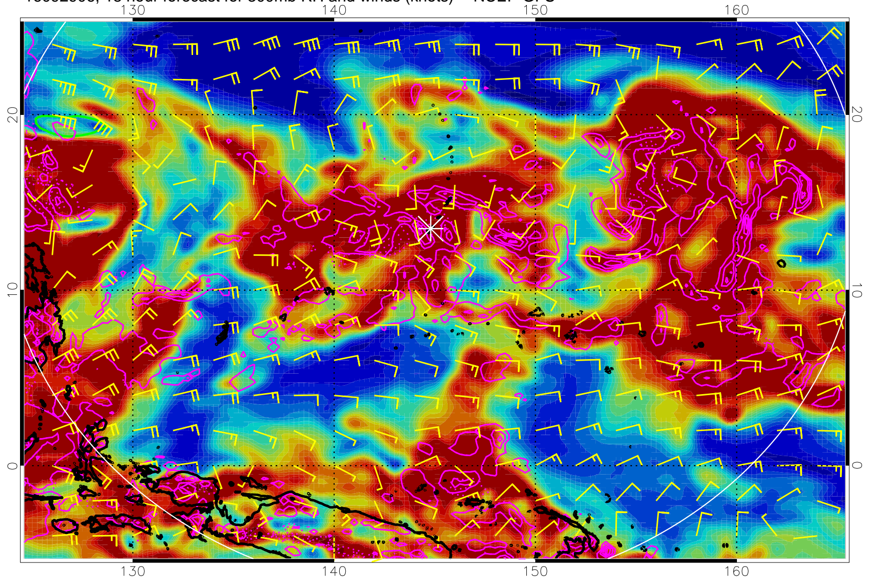
16092906, 18 hour forecast for 300mb RH and winds (knots) -- NCEP GFS
