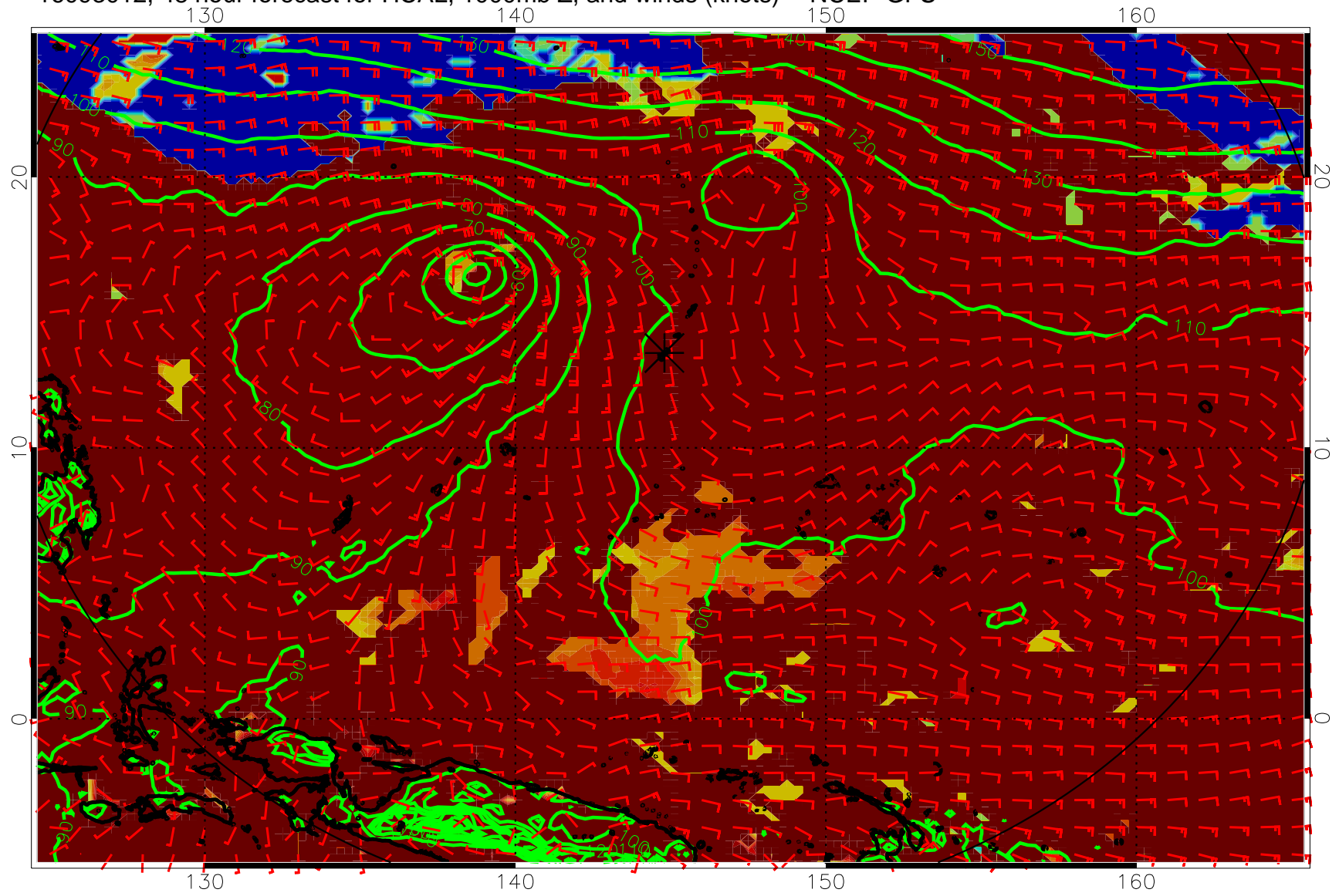
16093012, 48 hour forecast for HCAL, 1000mb Z, and winds (knots) -- NCEP GFS
