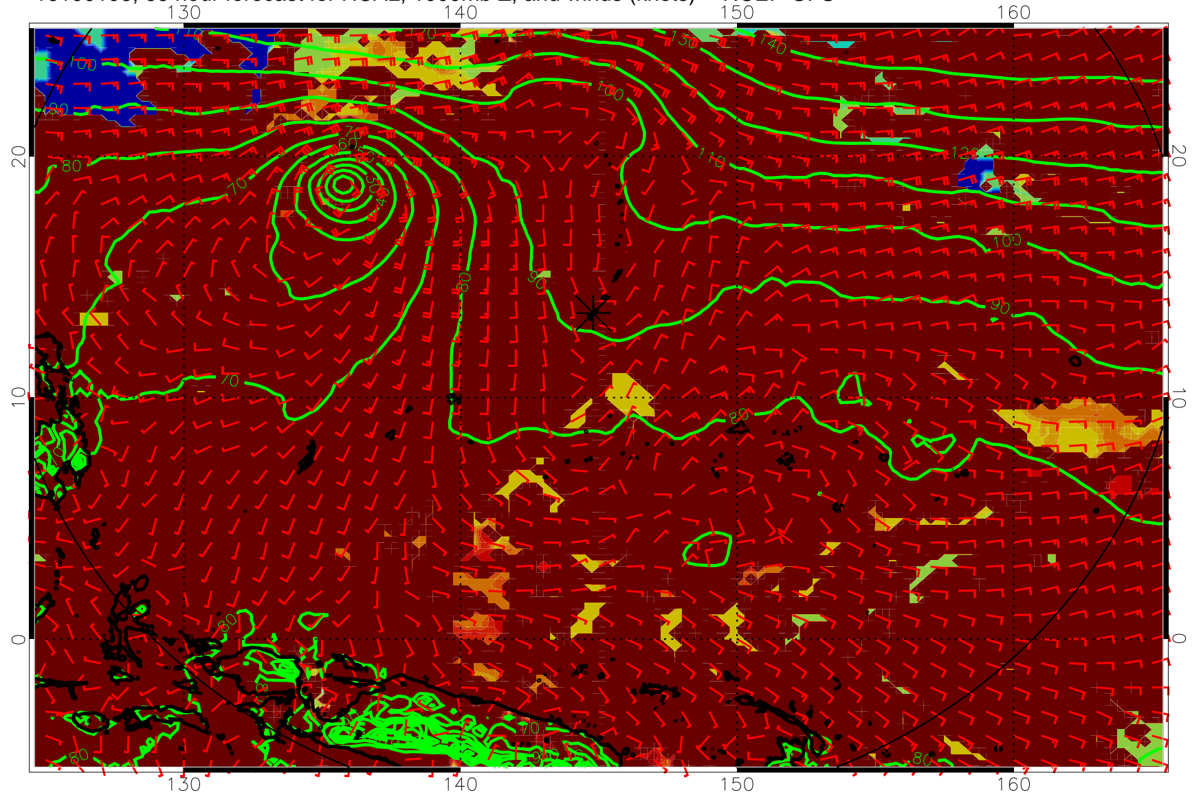
16100106, 66 hour forecast for HCAL, 1000mb Z, and winds (knots) -- NCEP GFS
