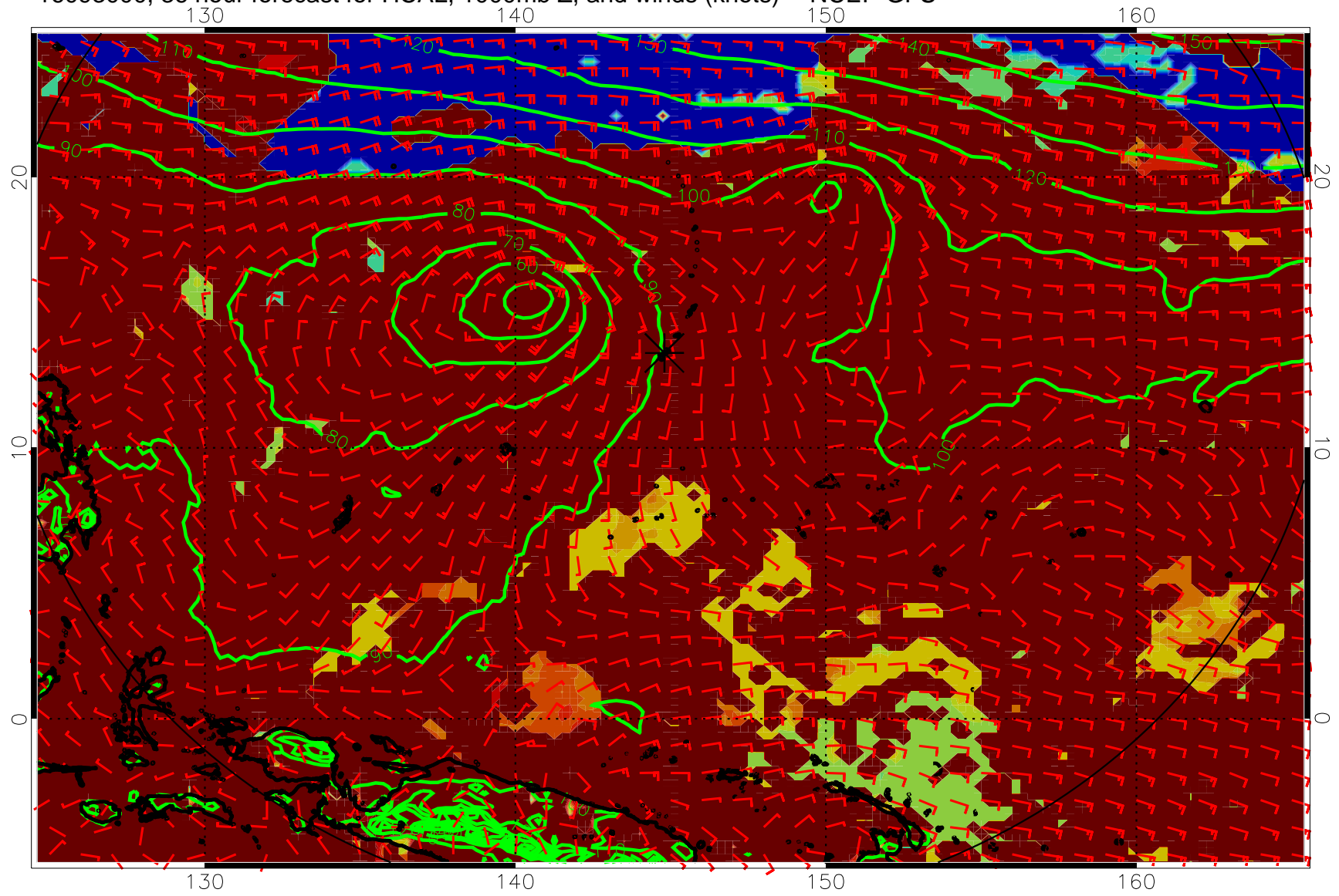
16093000, 36 hour forecast for HCAL, 1000mb Z, and winds (knots) -- NCEP GFS
