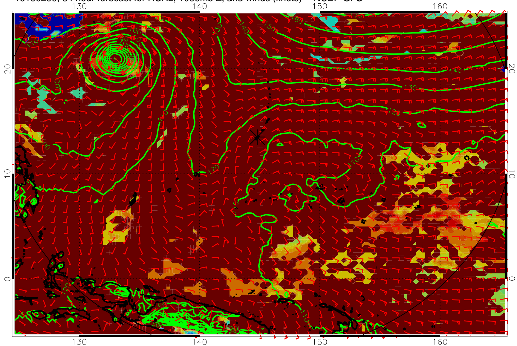
16100200, 84 hour forecast for HCAL, 1000mb Z, and winds (knots) -- NCEP GFS
