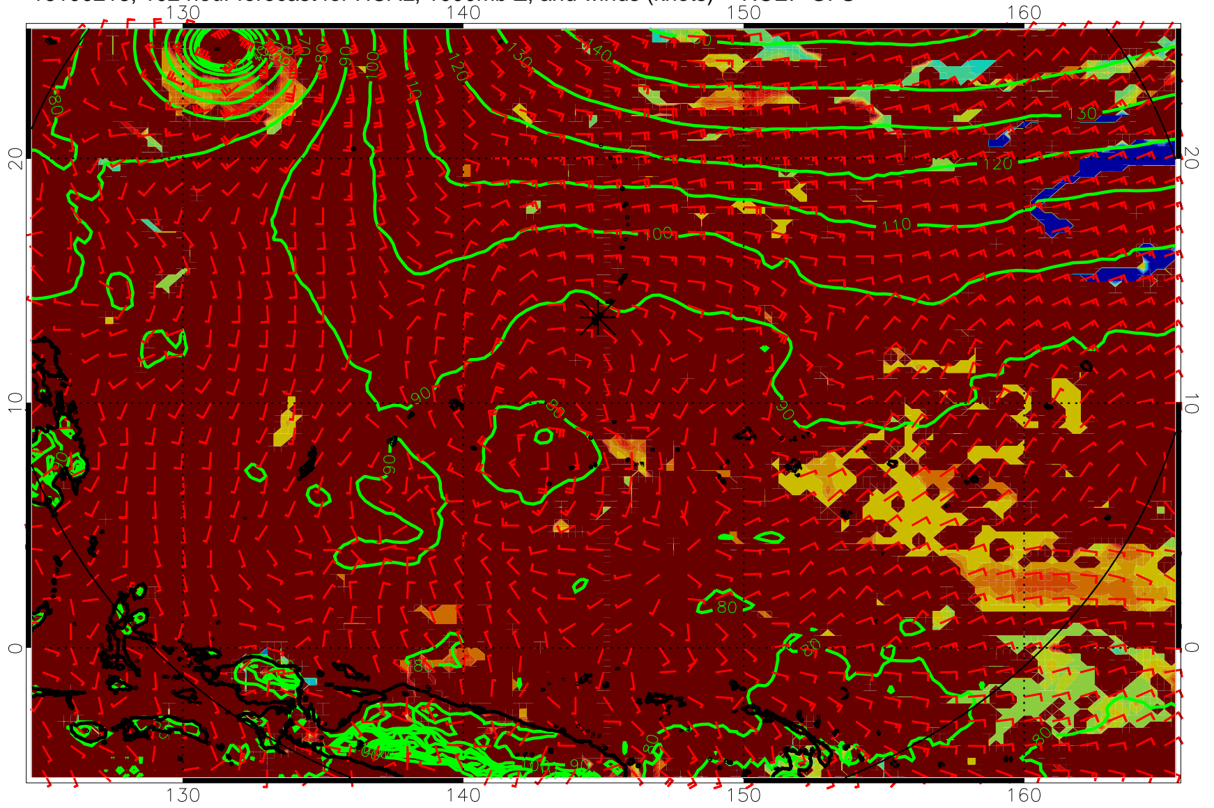
16100218, 102 hour forecast for HCAL, 1000mb Z, and winds (knots) -- NCEP GFS
