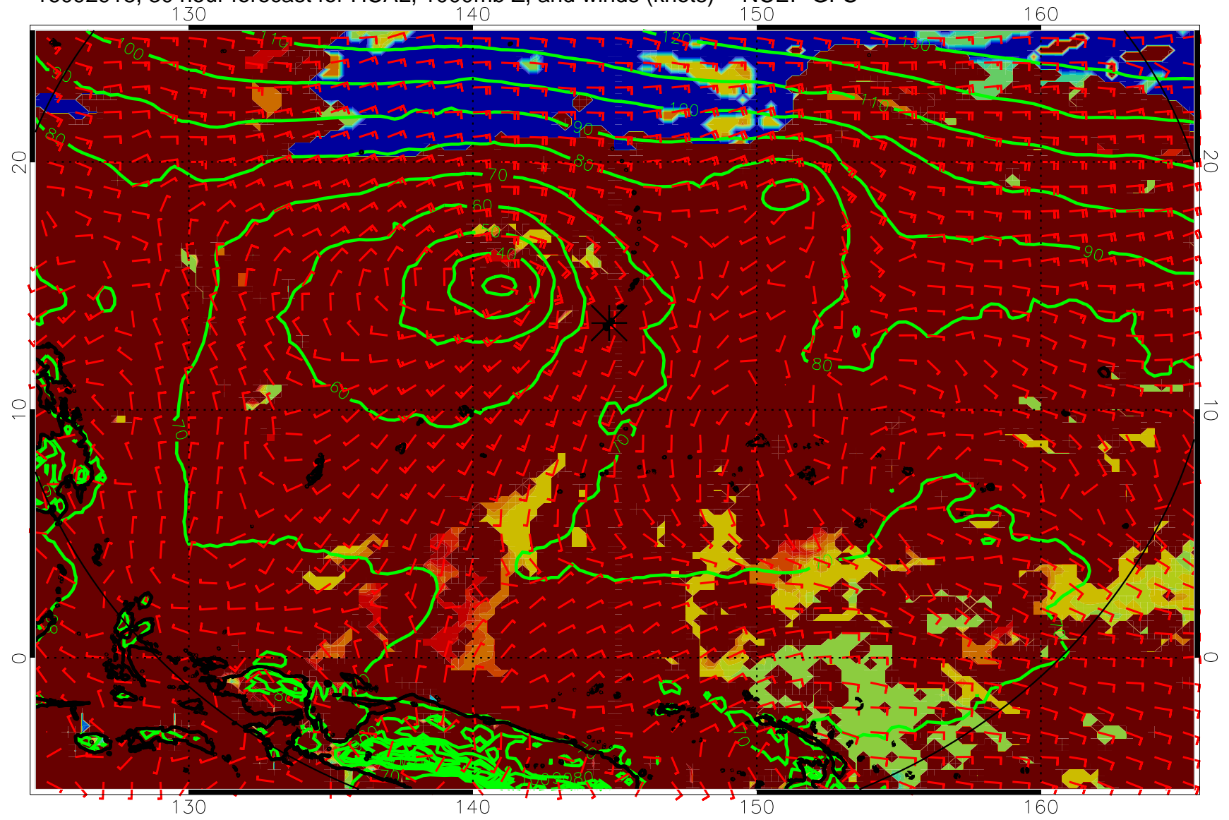
16092918, 30 hour forecast for HCAL, 1000mb Z, and winds (knots) -- NCEP GFS
