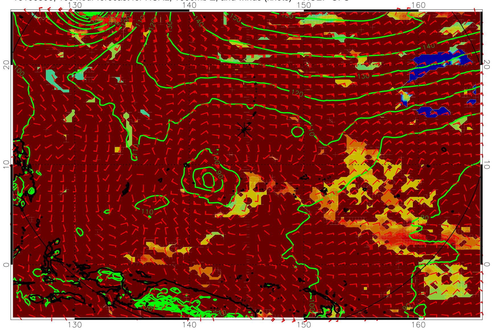
16100300, 108 hour forecast for HCAL, 1000mb Z, and winds (knots) -- NCEP GFS
