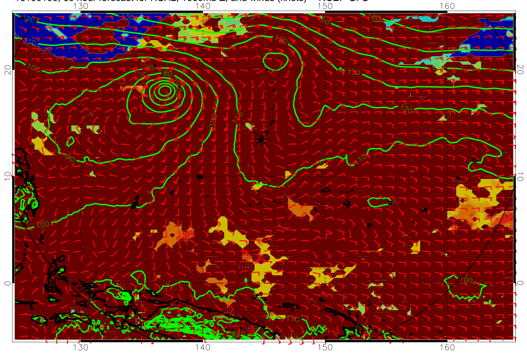
16100100, 60 hour forecast for HCAL, 1000mb Z, and winds (knots) -- NCEP GFS
