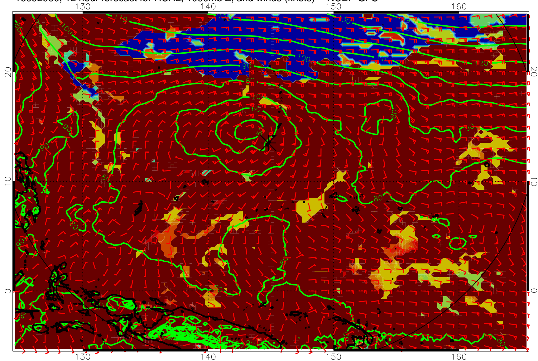
16092900, 12 hour forecast for HCAL, 1000mb Z, and winds (knots) -- NCEP GFS
