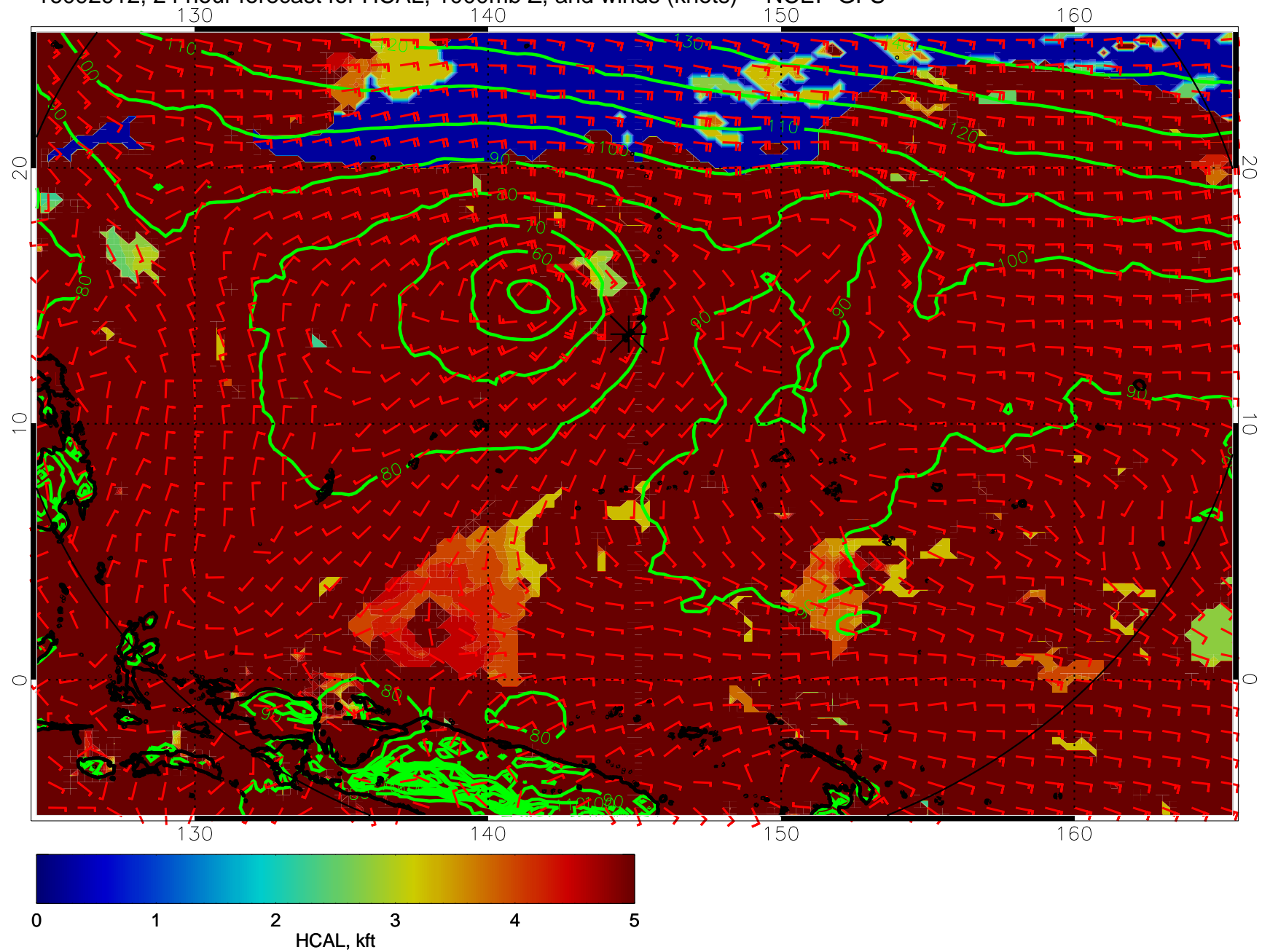
16092912, 24 hour forecast for HCAL, 1000mb Z, and winds (knots) -- NCEP GFS
