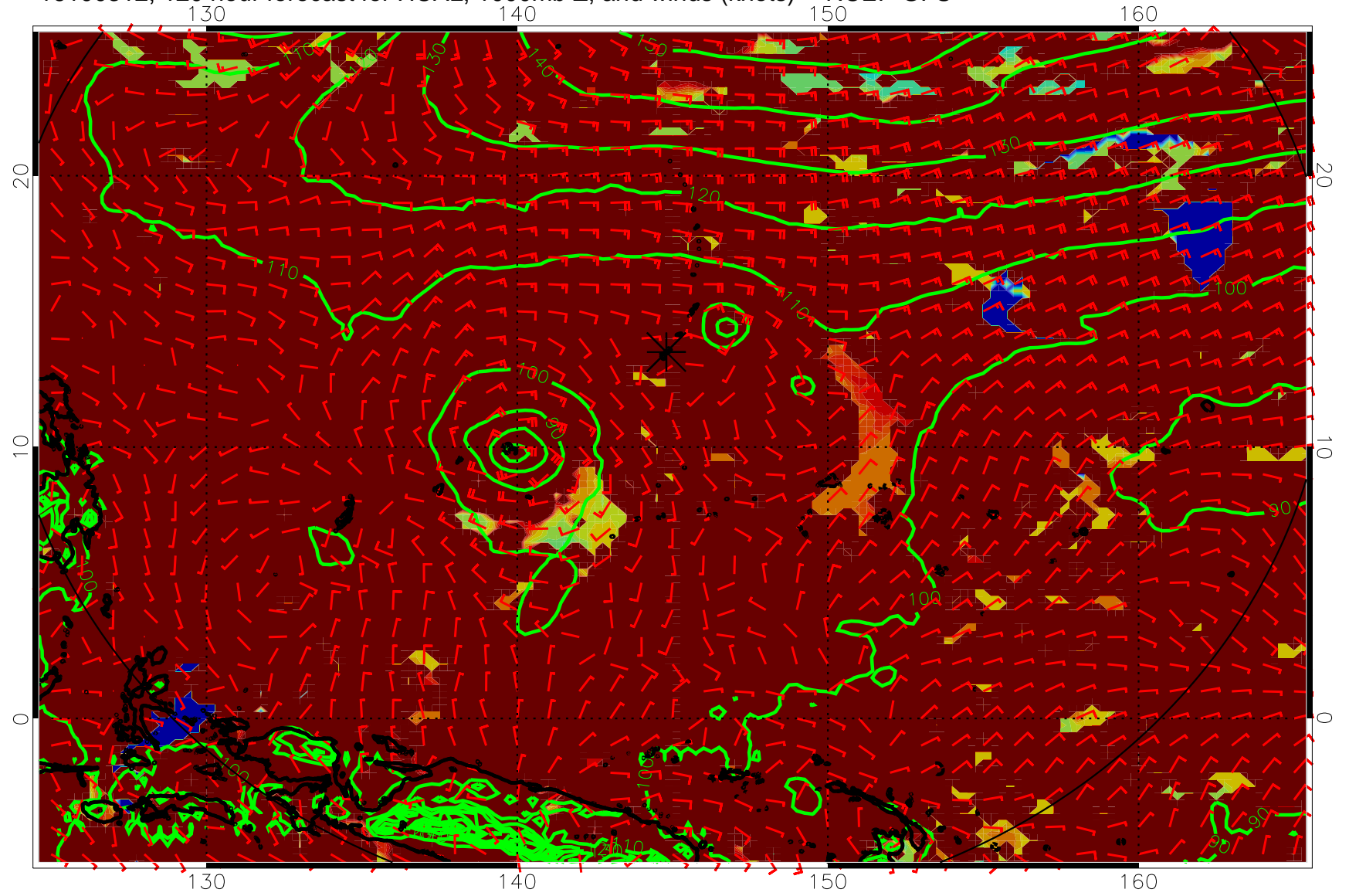
16100312, 120 hour forecast for HCAL, 1000mb Z, and winds (knots) -- NCEP GFS
