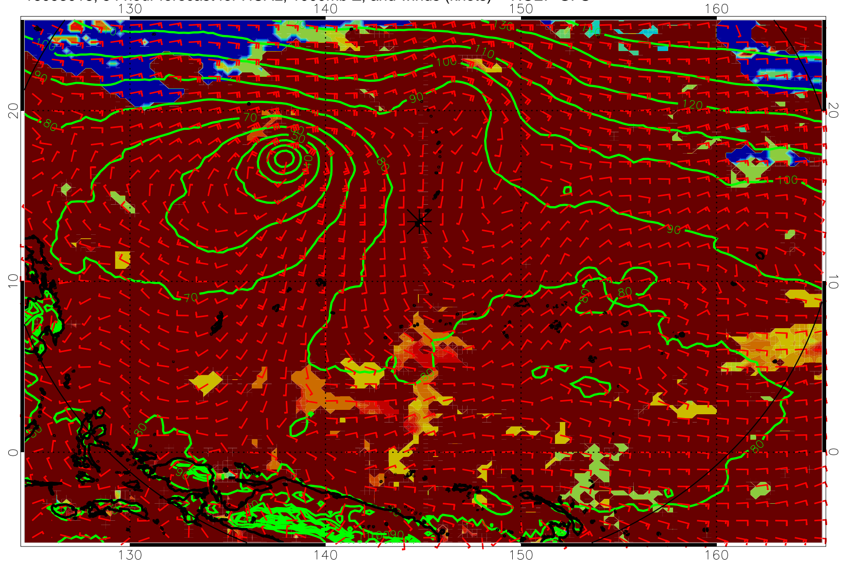
16093018, 54 hour forecast for HCAL, 1000mb Z, and winds (knots) -- NCEP GFS
