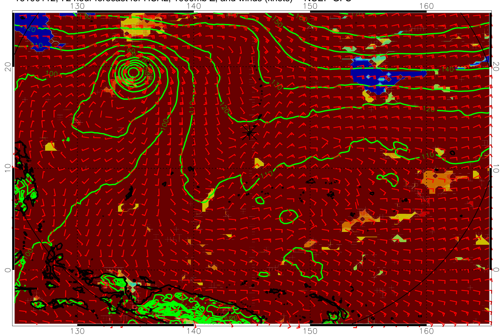
16100112, 72 hour forecast for HCAL, 1000mb Z, and winds (knots) -- NCEP GFS
