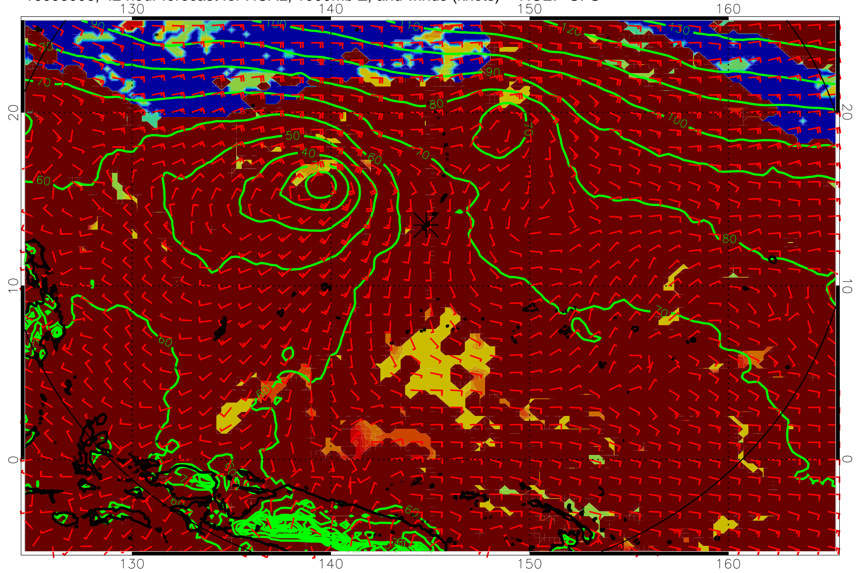
16093006, 42 hour forecast for HCAL, 1000mb Z, and winds (knots) -- NCEP GFS
