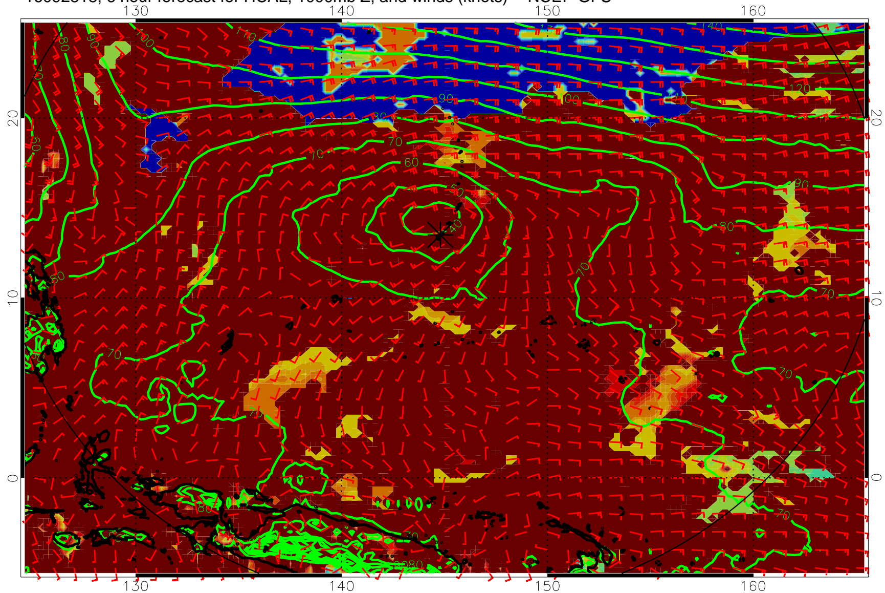
16092818, 6 hour forecast for HCAL, 1000mb Z, and winds (knots) -- NCEP GFS
