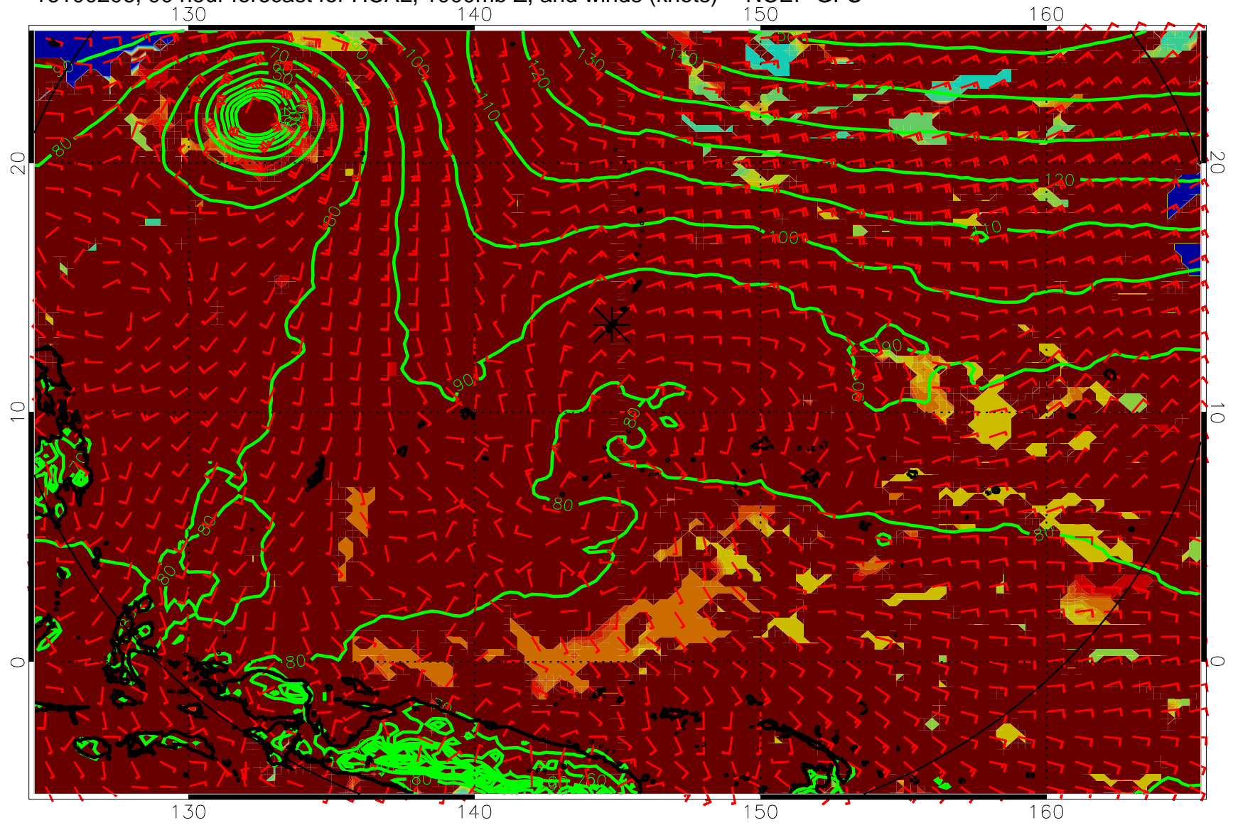
16100206, 90 hour forecast for HCAL, 1000mb Z, and winds (knots) -- NCEP GFS
