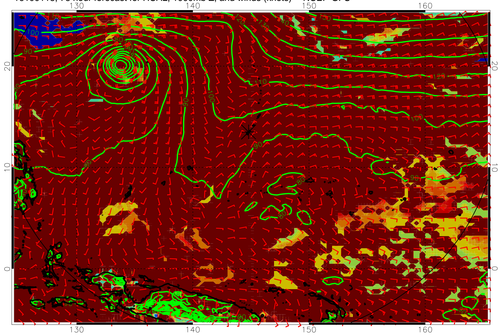
16100118, 78 hour forecast for HCAL, 1000mb Z, and winds (knots) -- NCEP GFS
