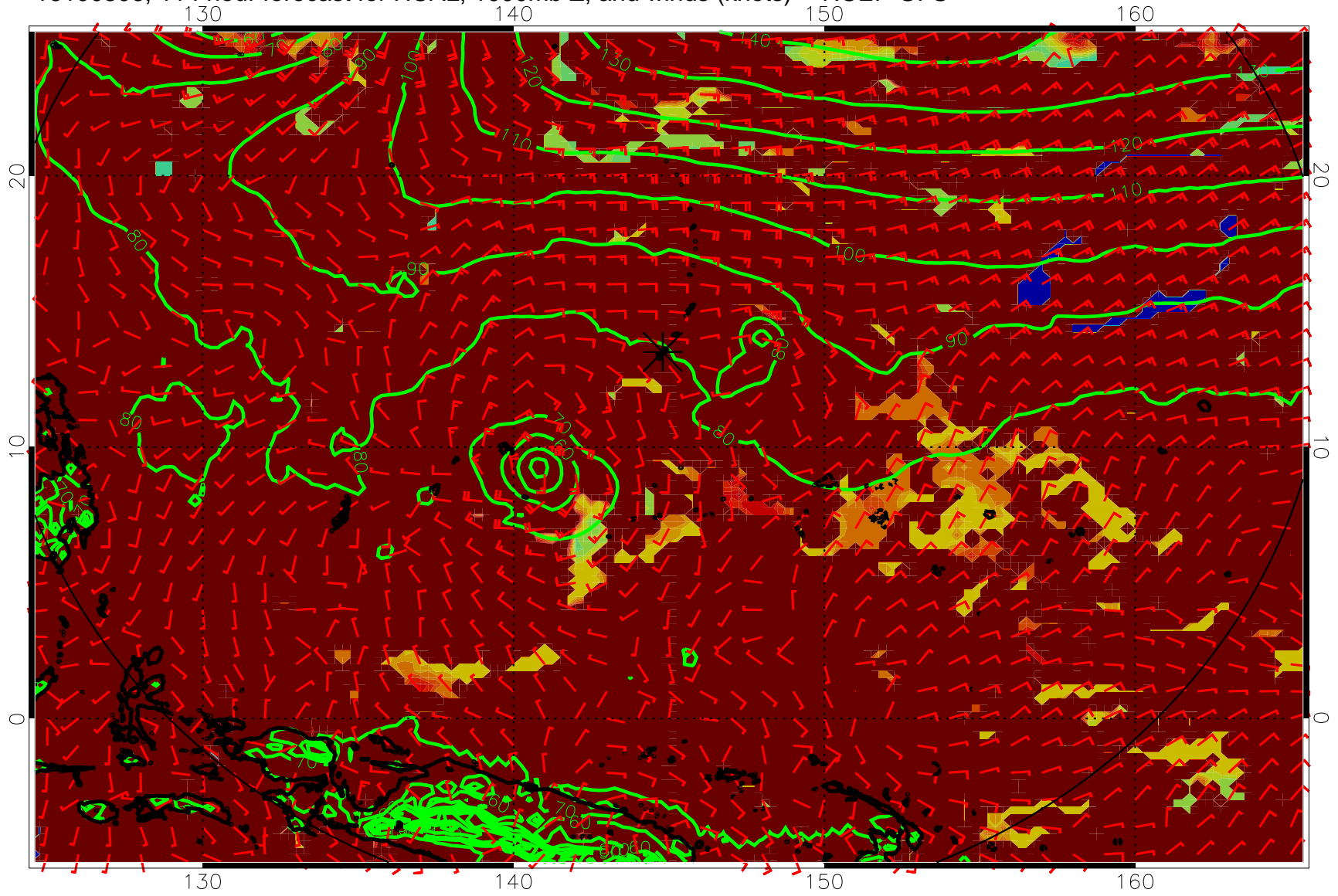
16100306, 114 hour forecast for HCAL, 1000mb Z, and winds (knots) -- NCEP GFS
