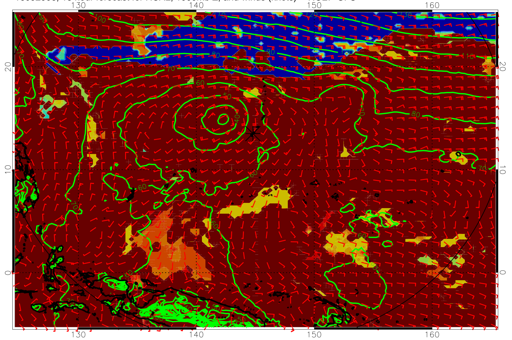
16092906, 18 hour forecast for HCAL, 1000mb Z, and winds (knots) -- NCEP GFS
