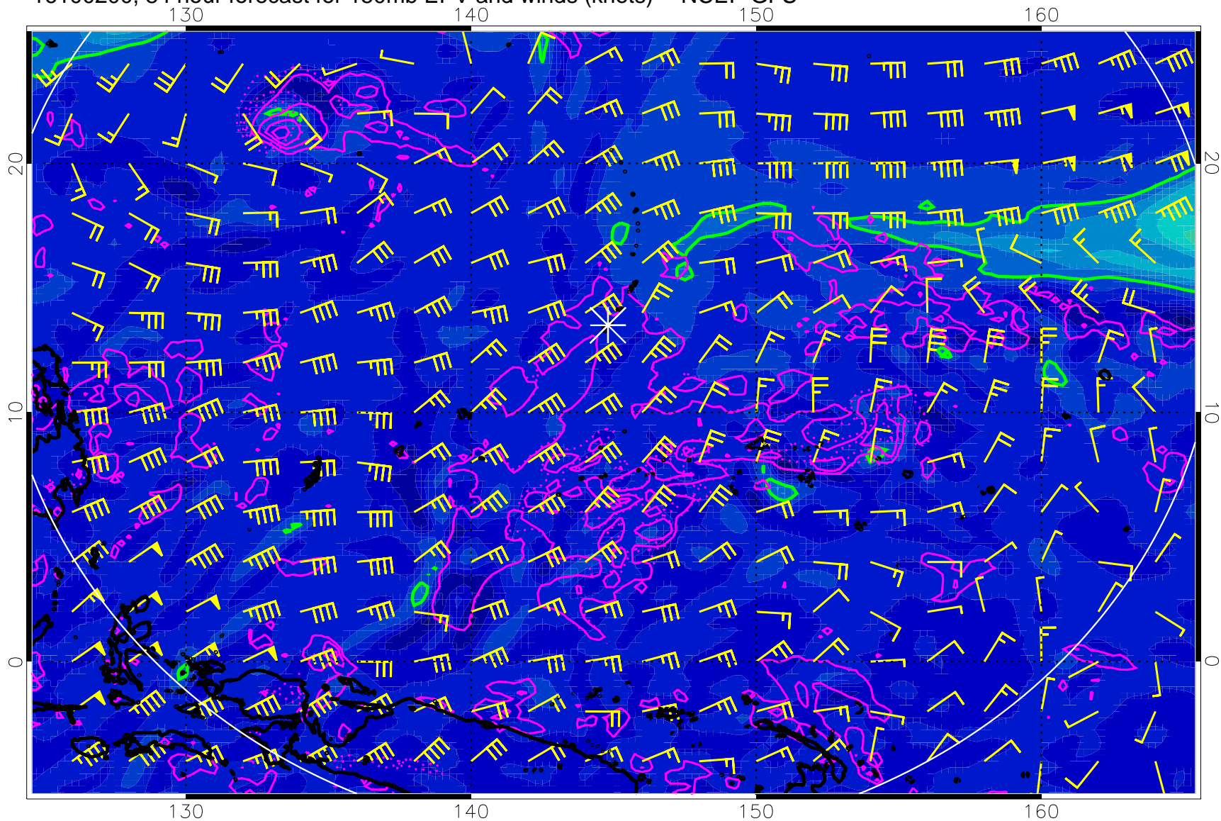
16100200, 84 hour forecast for 150mb EPV and winds (knots) -- NCEP GFS
