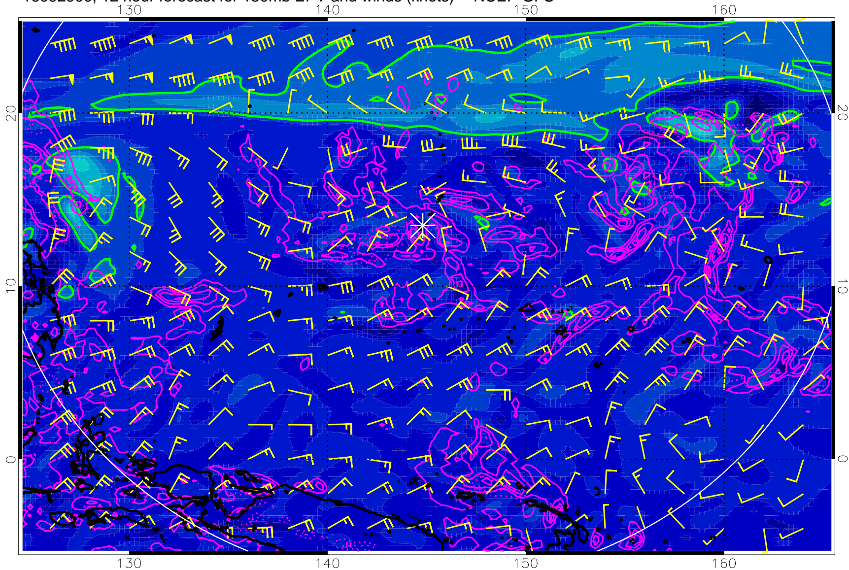
16092900, 12 hour forecast for 150mb EPV and winds (knots) -- NCEP GFS
