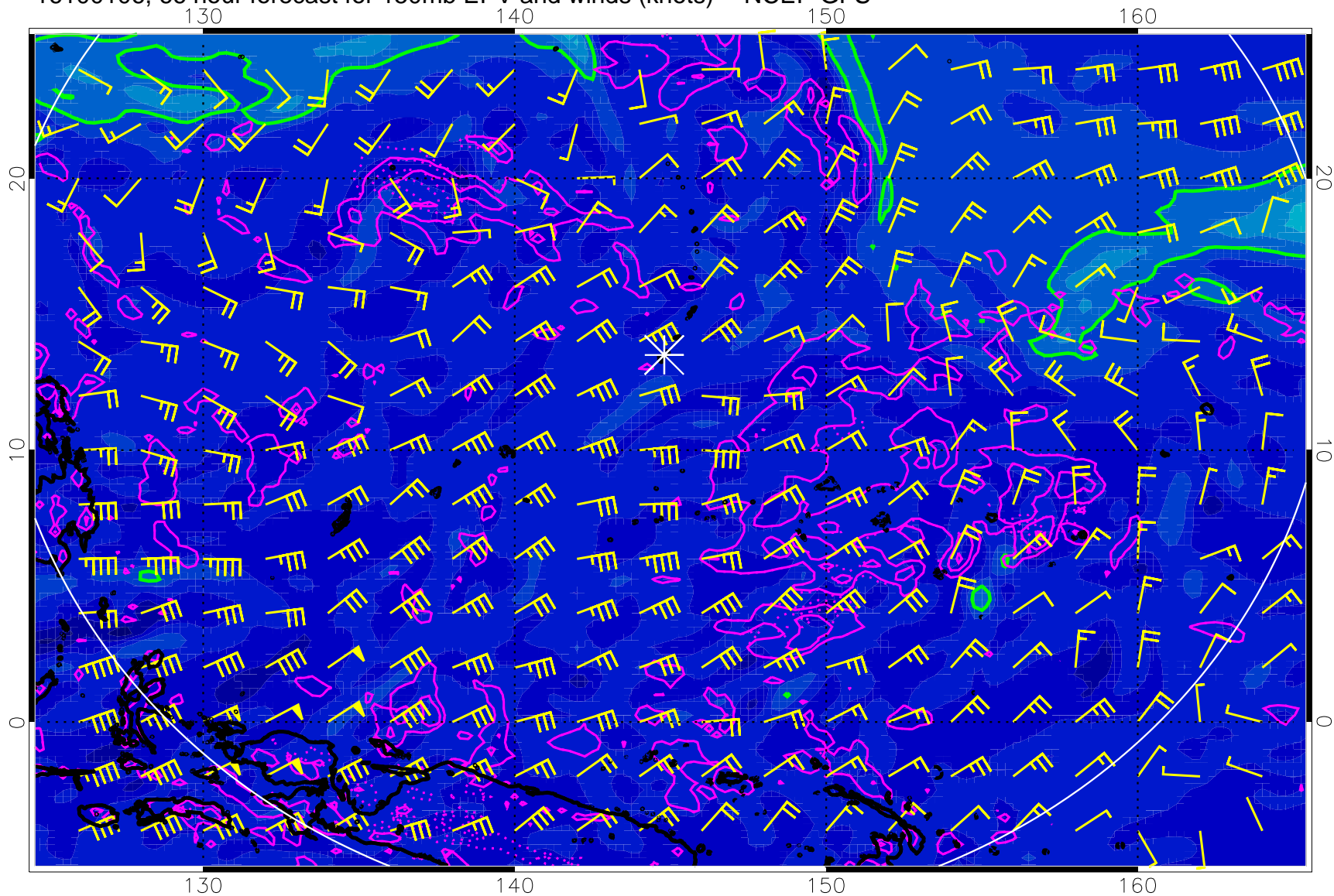
16100106, 66 hour forecast for 150mb EPV and winds (knots) -- NCEP GFS
