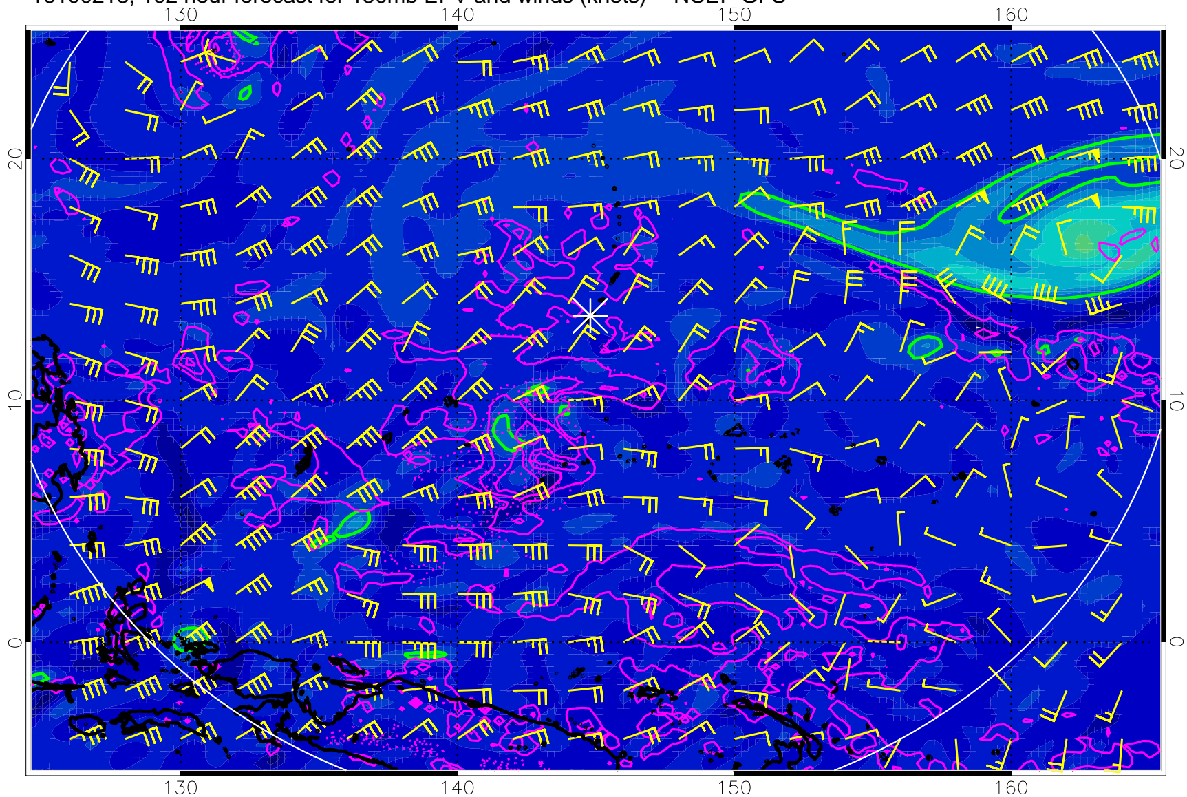
16100218, 102 hour forecast for 150mb EPV and winds (knots) -- NCEP GFS
