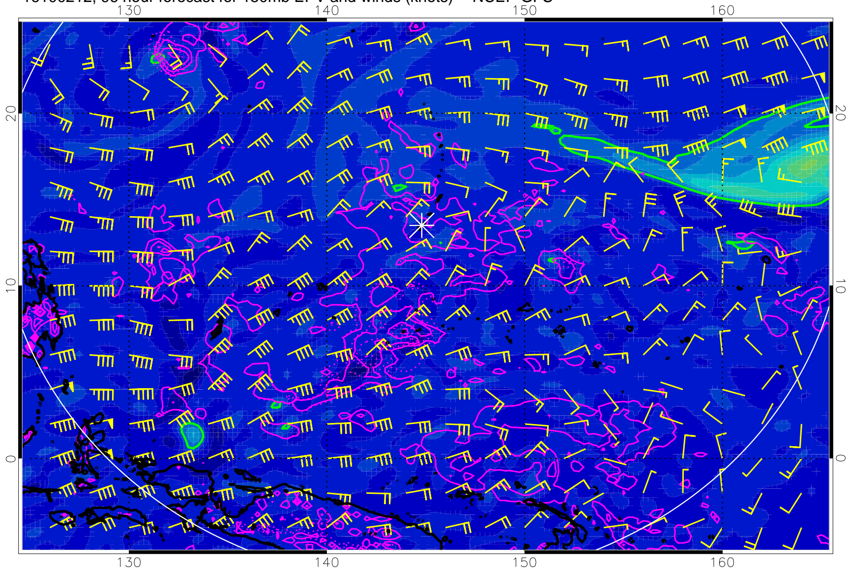
16100212, 96 hour forecast for 150mb EPV and winds (knots) -- NCEP GFS
