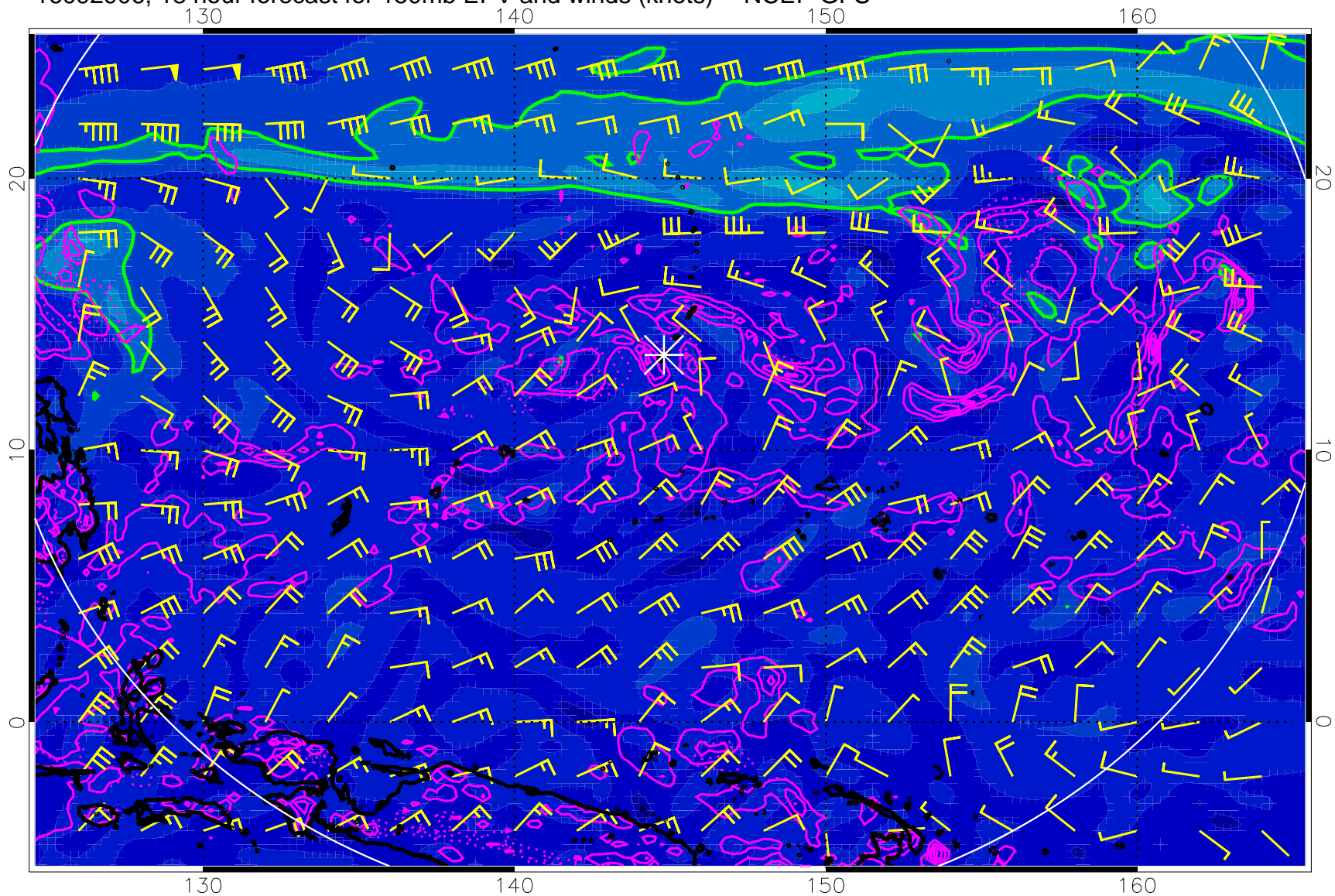
16092906, 18 hour forecast for 150mb EPV and winds (knots) -- NCEP GFS
