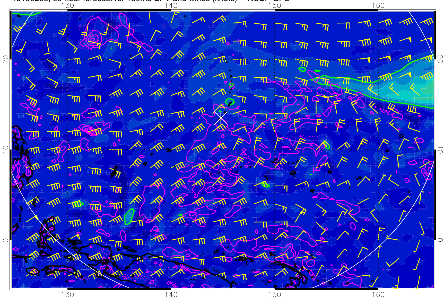
16100206, 90 hour forecast for 150mb EPV and winds (knots) -- NCEP GFS
