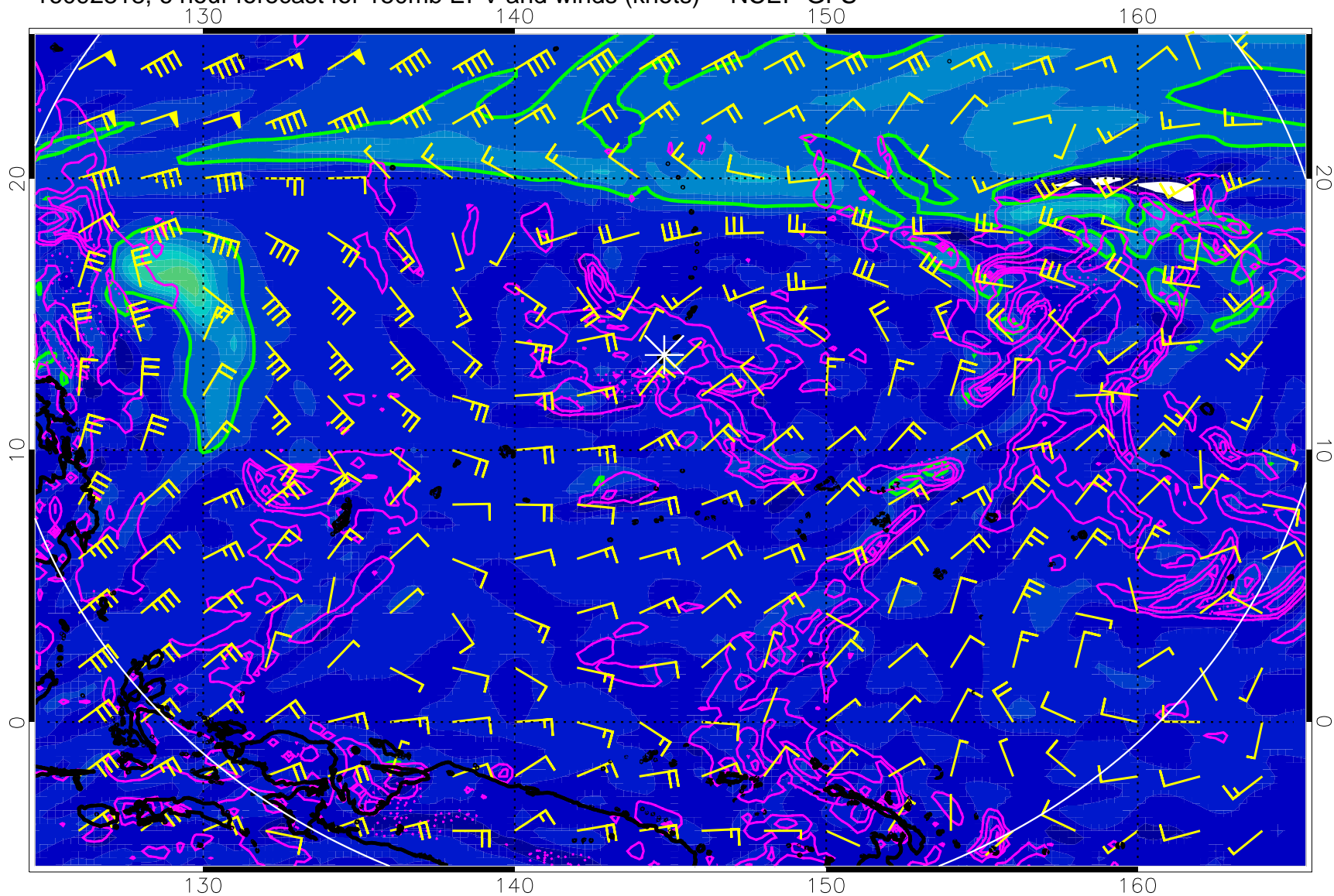
16092818, 6 hour forecast for 150mb EPV and winds (knots) -- NCEP GFS
