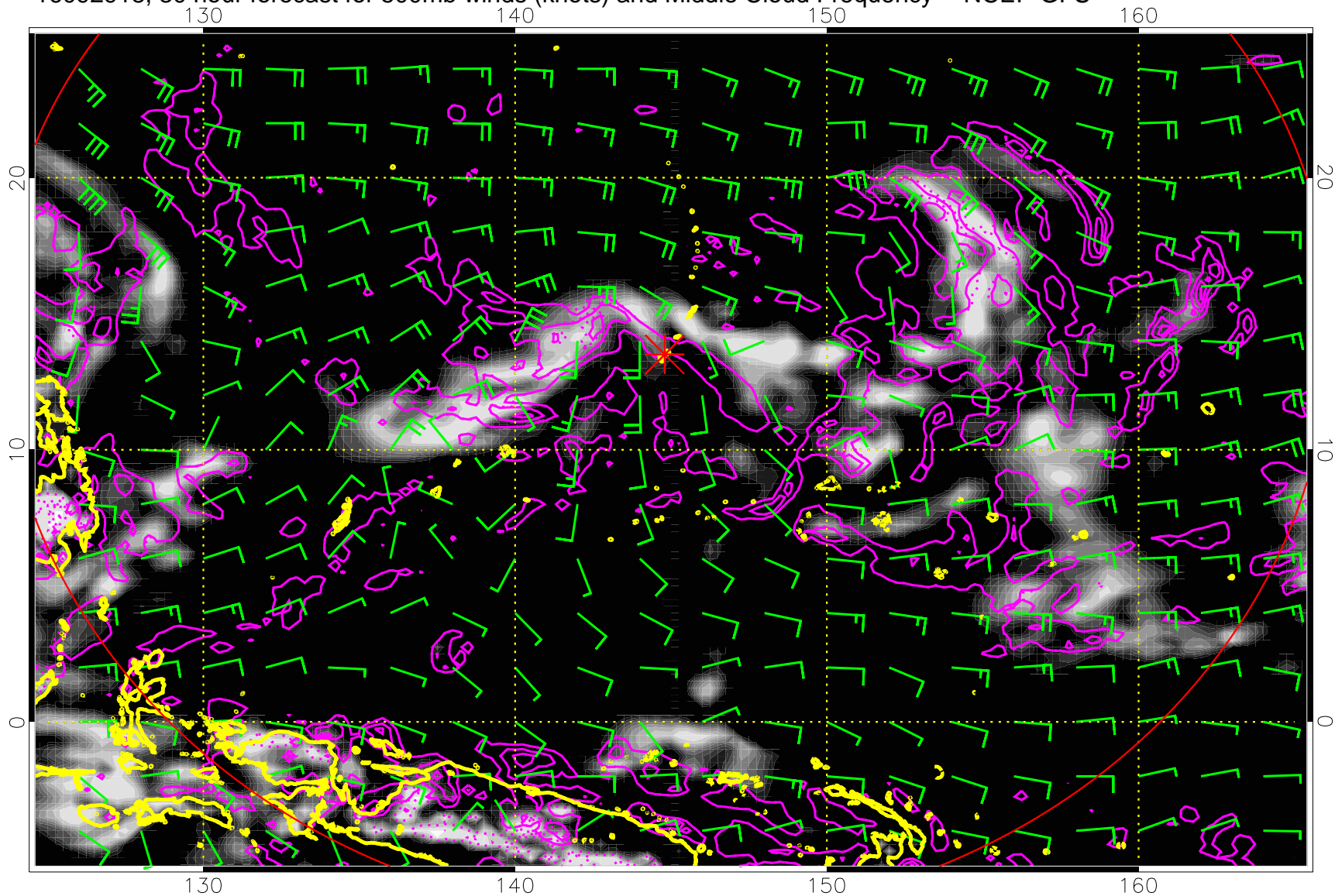
16092918, 30 hour forecast for 500mb winds (knots) and Middle Cloud Frequency -- NCEP GFS
