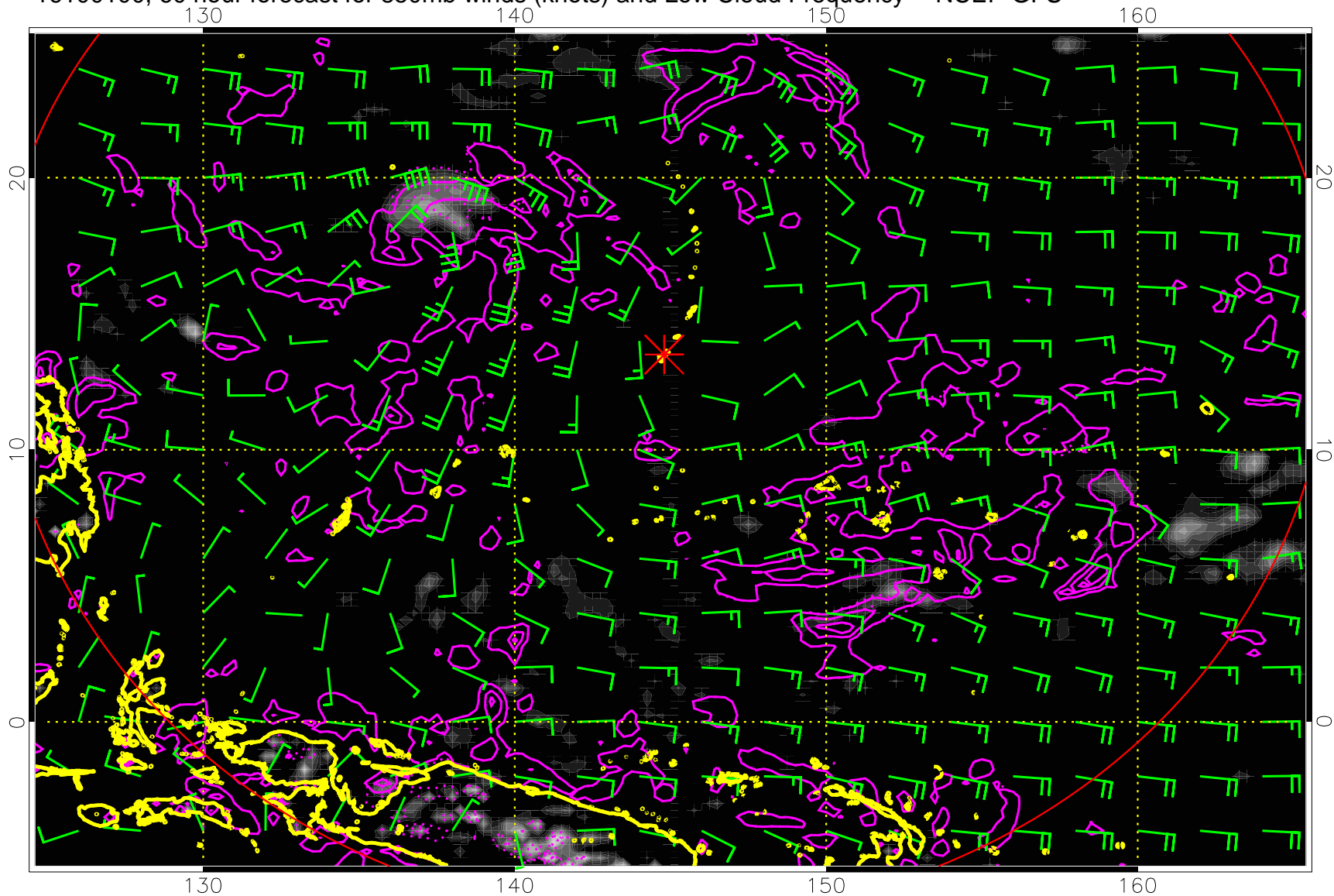
16100100, 60 hour forecast for 850mb winds (knots) and Low Cloud Frequency -- NCEP GFS
