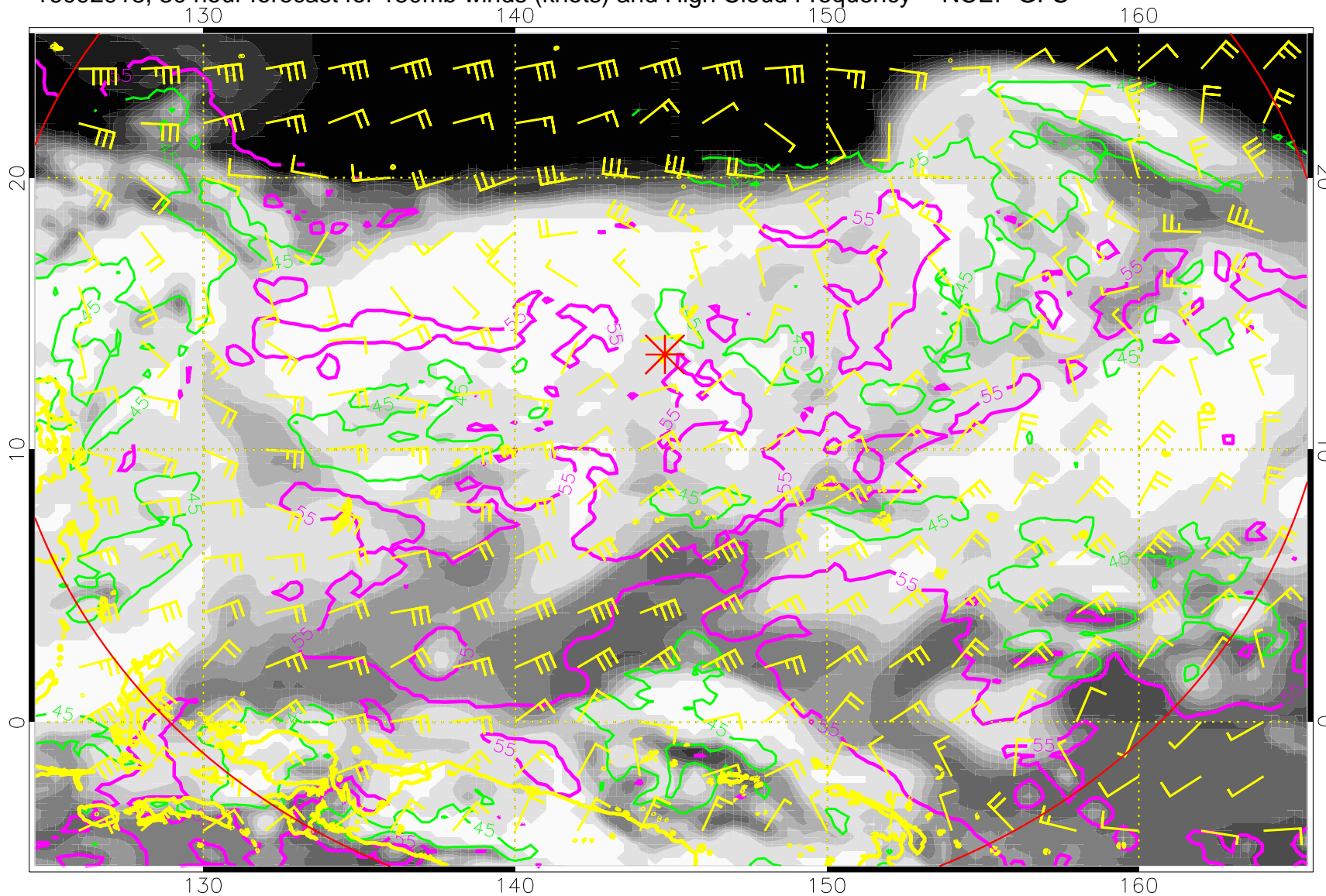
16092918, 30 hour forecast for 150mb winds (knots) and High Cloud Frequency -- NCEP GFS
