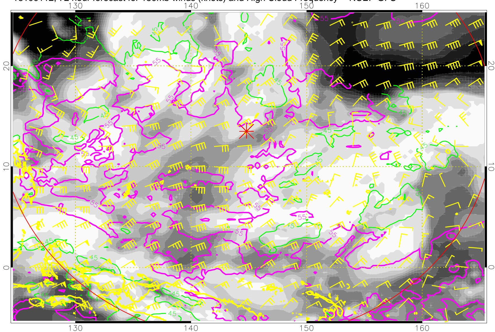
16100112, 72 hour forecast for 150mb winds (knots) and High Cloud Frequency -- NCEP GFS
