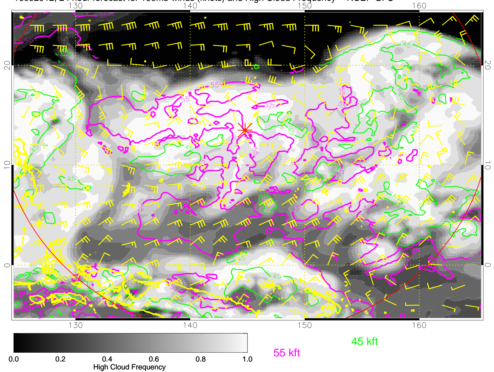
16092912, 24 hour forecast for 150mb winds (knots) and High Cloud Frequency -- NCEP GFS
