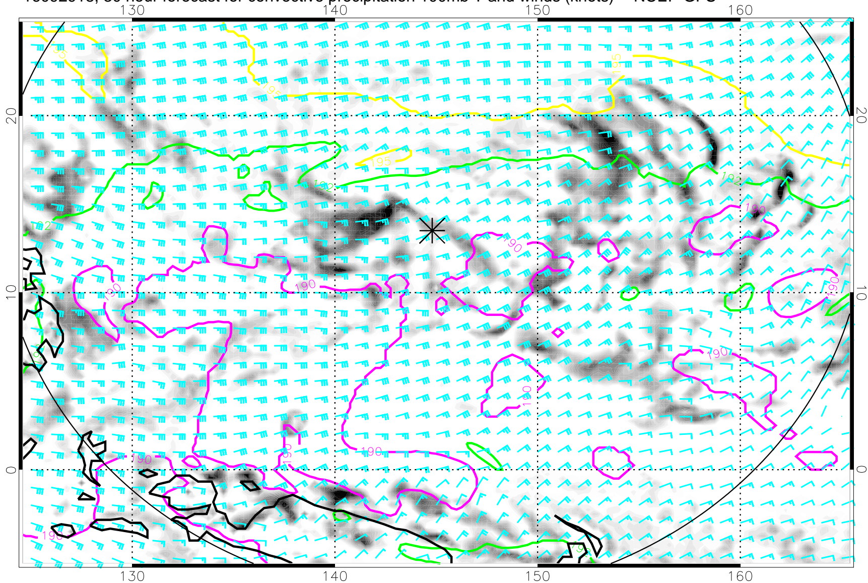
16092918, 30 hour forecast for convective precipitation 100mb T and winds (knots) -- NCEP GFS
