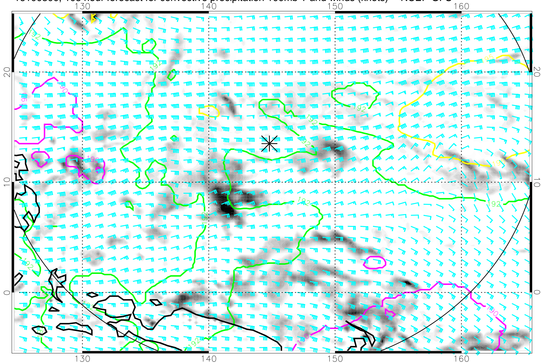
16100300, 108 hour forecast for convective precipitation 100mb T and winds (knots) -- NCEP GFS
