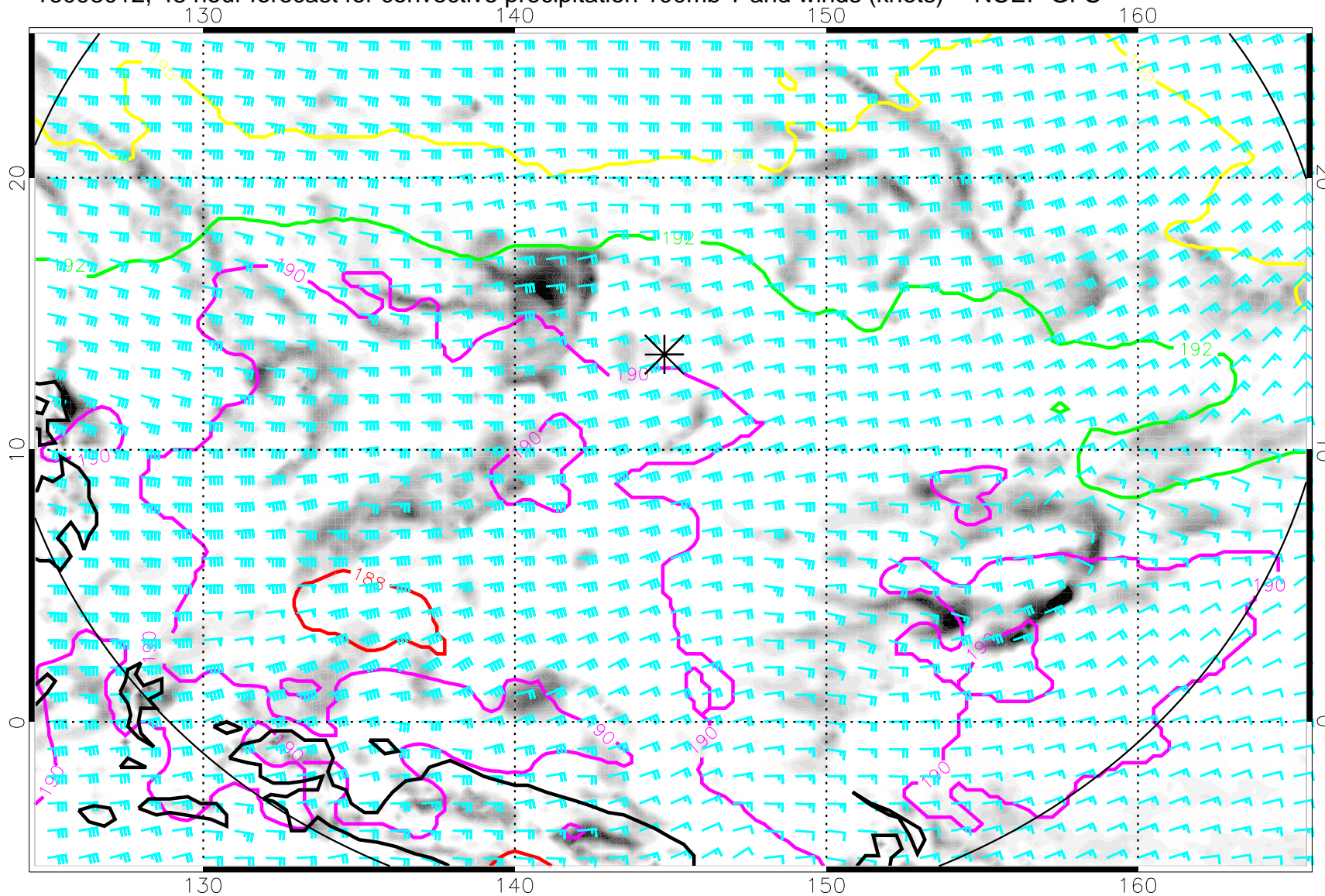
16093012, 48 hour forecast for convective precipitation 100mb T and winds (knots) -- NCEP GFS
