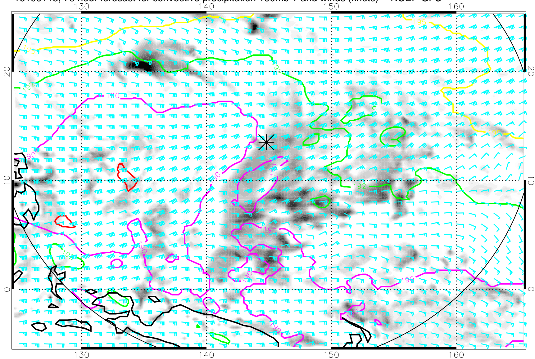
16100118, 78 hour forecast for convective precipitation 100mb T and winds (knots) -- NCEP GFS
