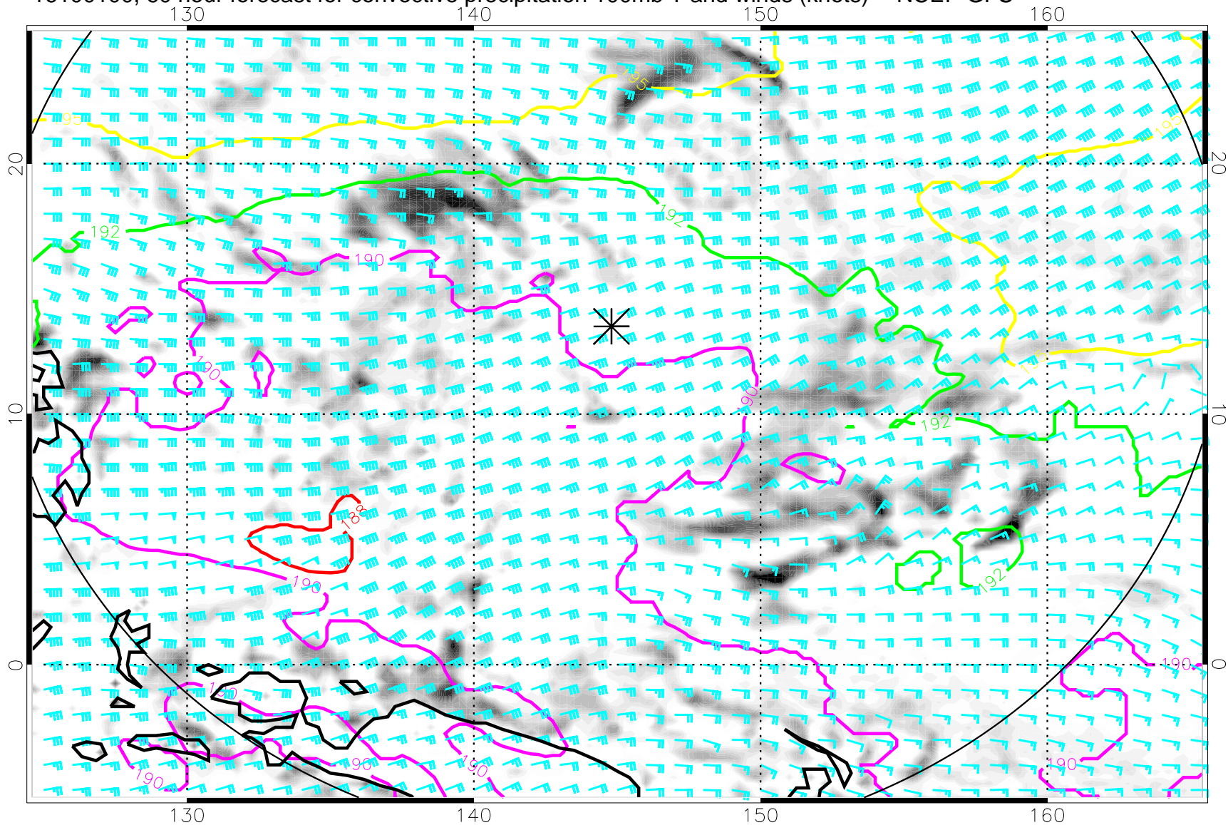
16100100, 60 hour forecast for convective precipitation 100mb T and winds (knots) -- NCEP GFS
