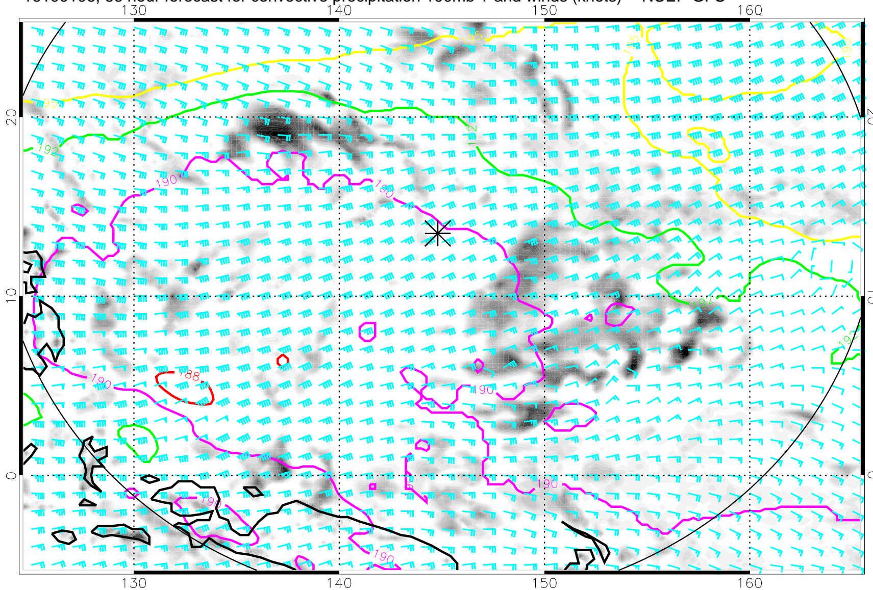
16100106, 66 hour forecast for convective precipitation 100mb T and winds (knots) -- NCEP GFS
