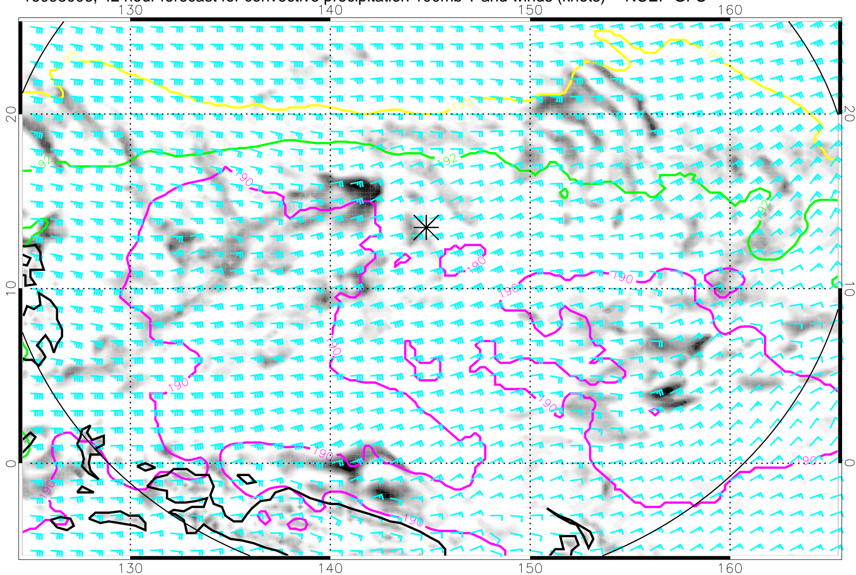
16093006, 42 hour forecast for convective precipitation 100mb T and winds (knots) -- NCEP GFS
