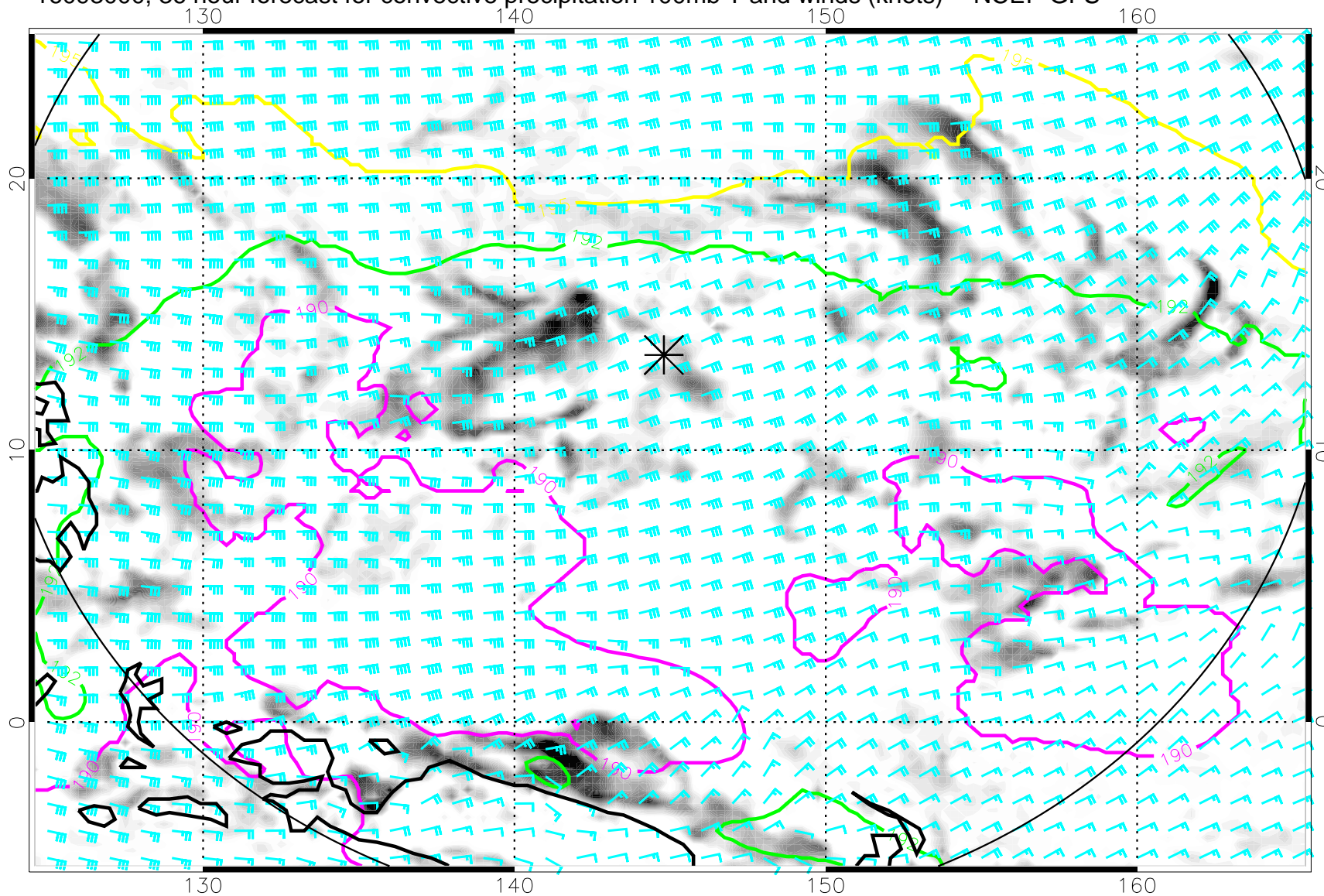
16093000, 36 hour forecast for convective precipitation 100mb T and winds (knots) -- NCEP GFS
