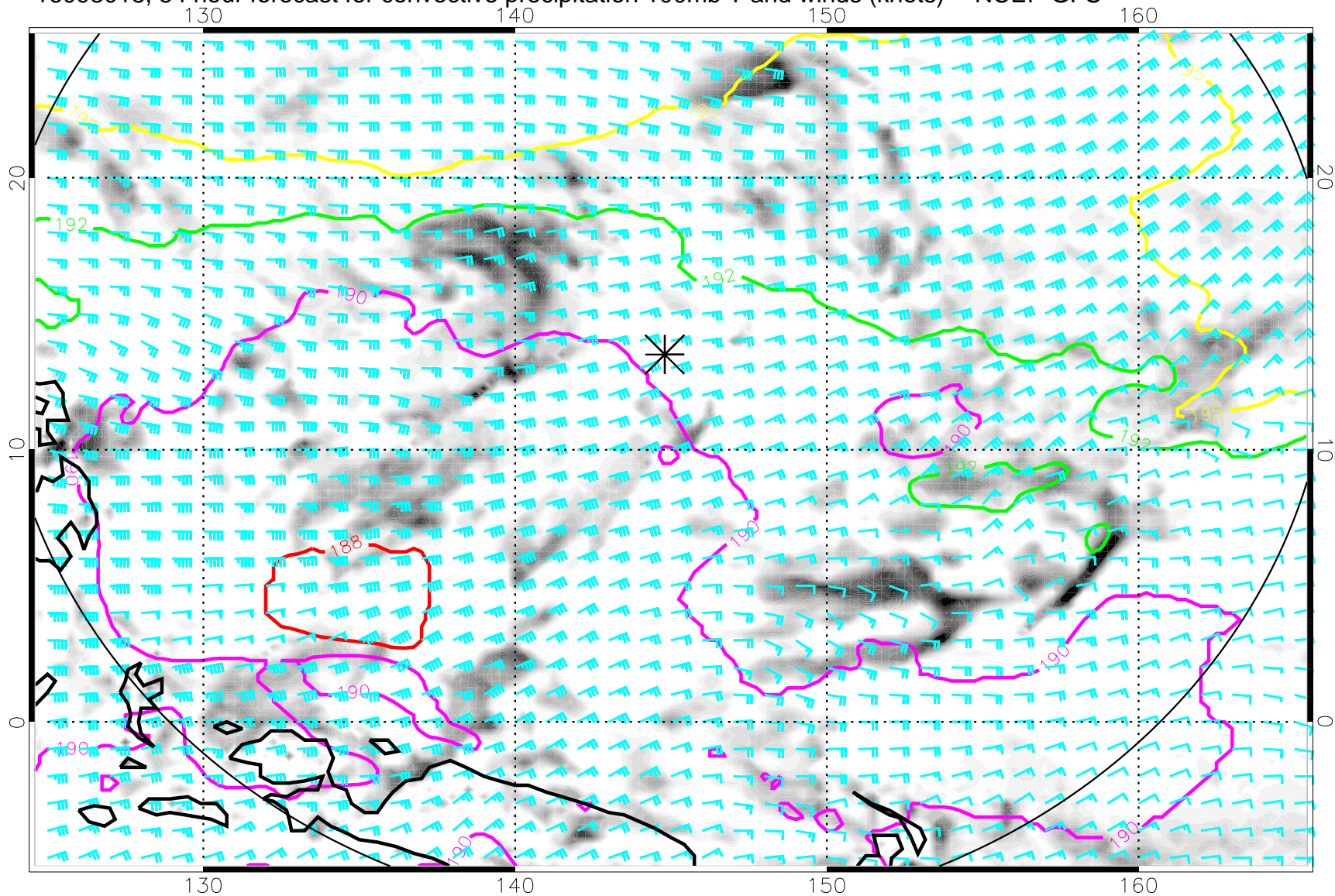
16093018, 54 hour forecast for convective precipitation 100mb T and winds (knots) -- NCEP GFS
