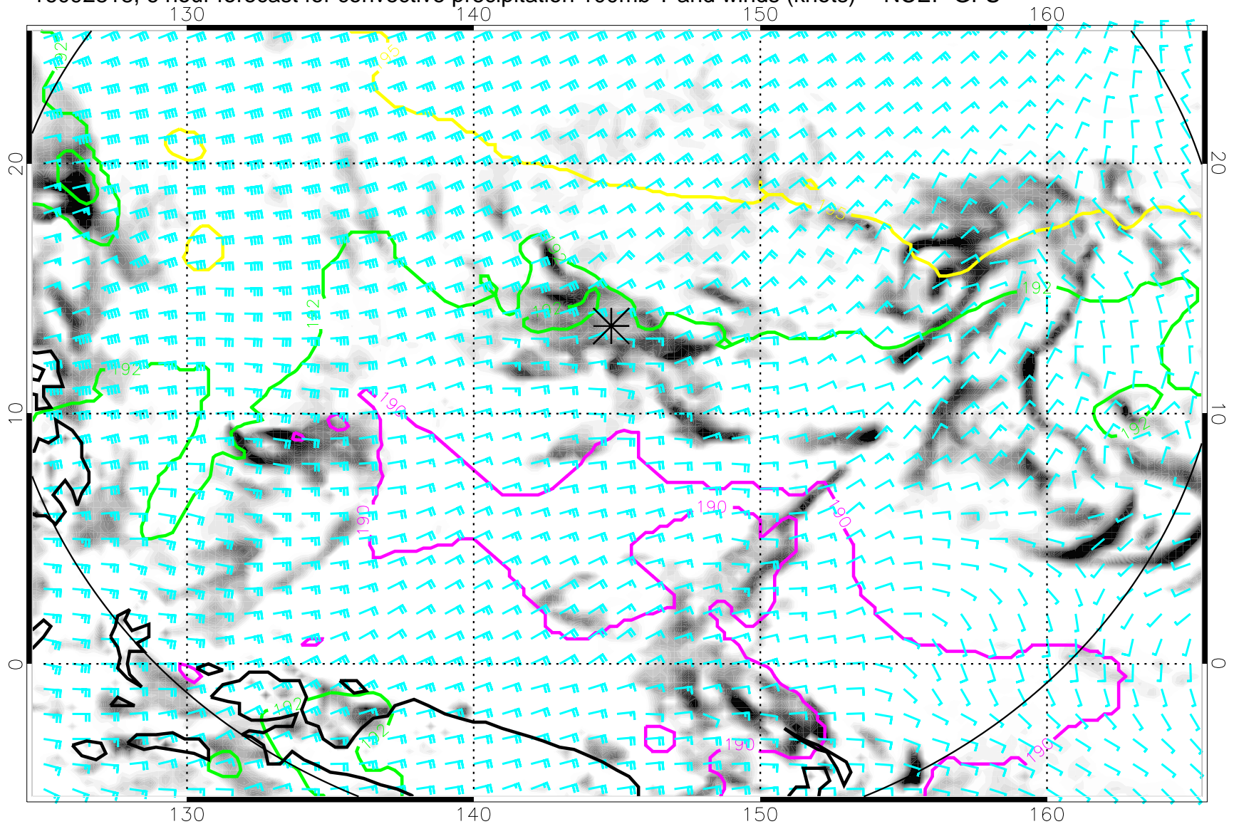
16092818, 6 hour forecast for convective precipitation 100mb T and winds (knots) -- NCEP GFS
