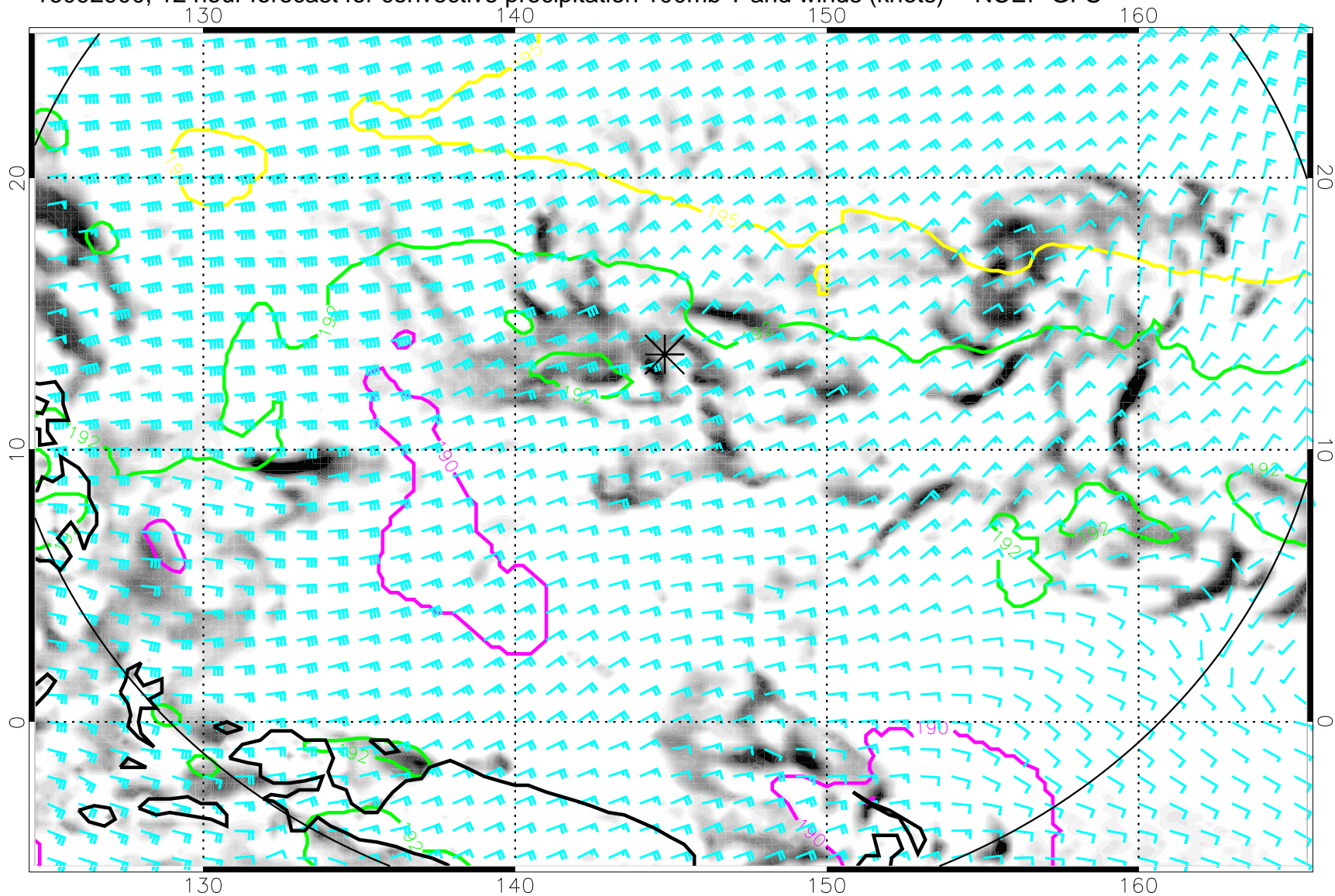
16092900, 12 hour forecast for convective precipitation 100mb T and winds (knots) -- NCEP GFS
