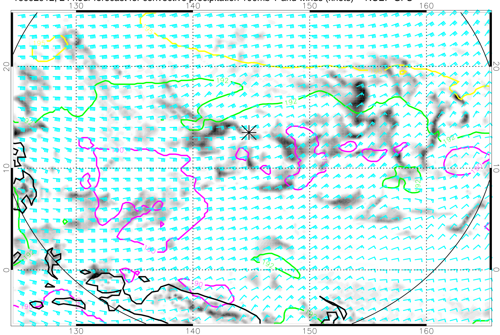
16092912, 24 hour forecast for convective precipitation 100mb T and winds (knots) -- NCEP GFS
