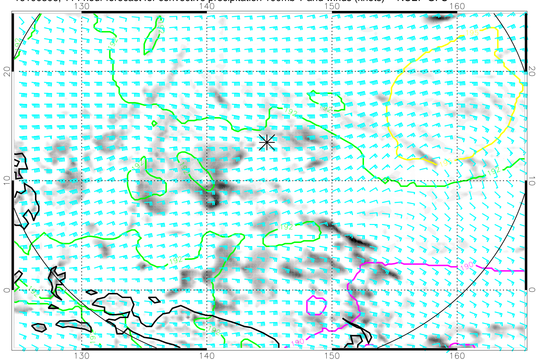
16100306, 114 hour forecast for convective precipitation 100mb T and winds (knots) -- NCEP GFS
