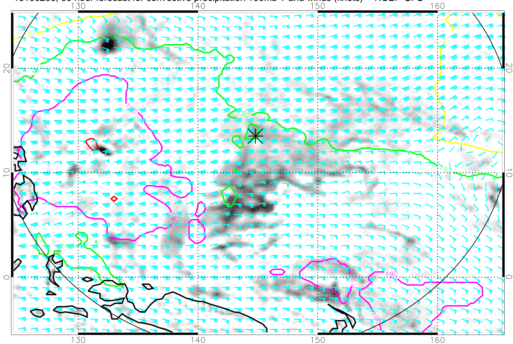
16100206, 90 hour forecast for convective precipitation 100mb T and winds (knots) -- NCEP GFS
