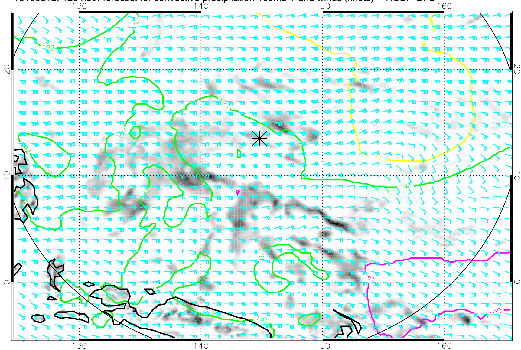
16100312, 120 hour forecast for convective precipitation 100mb T and winds (knots) -- NCEP GFS
