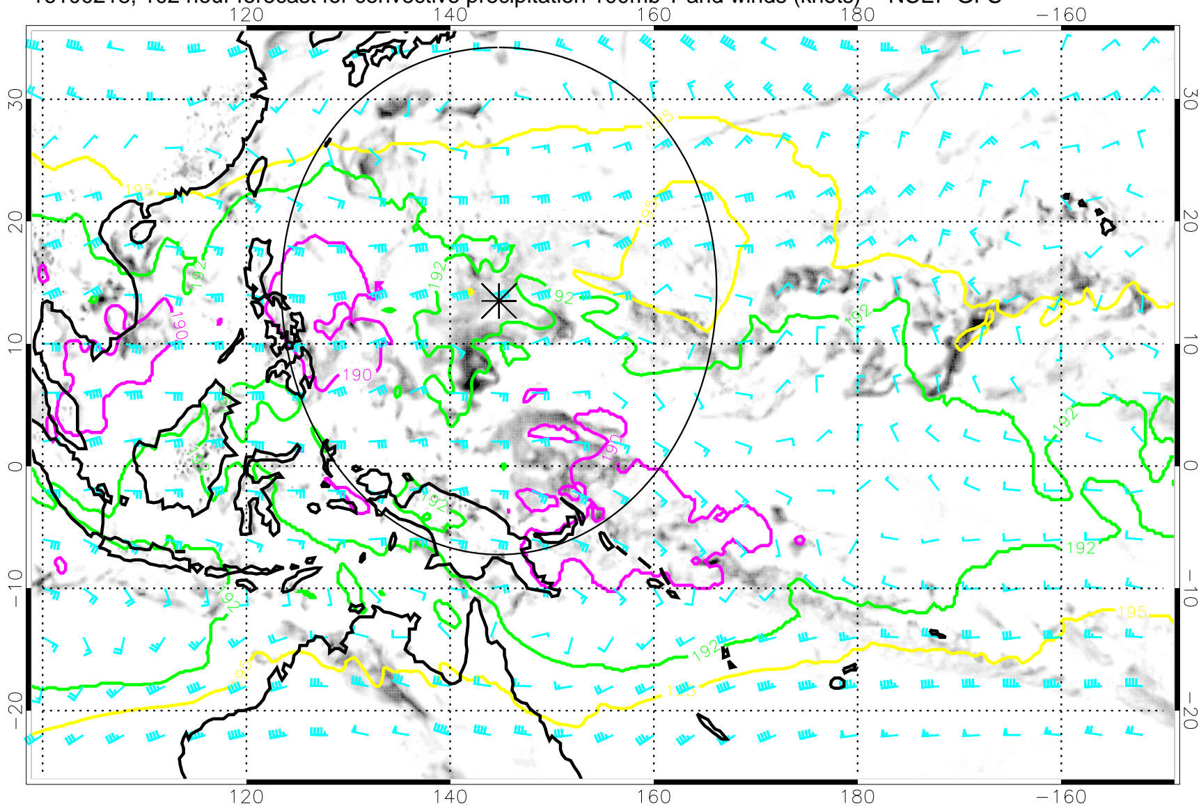
16100218, 102 hour forecast for convective precipitation 100mb T and winds (knots) -- NCEP GFS
