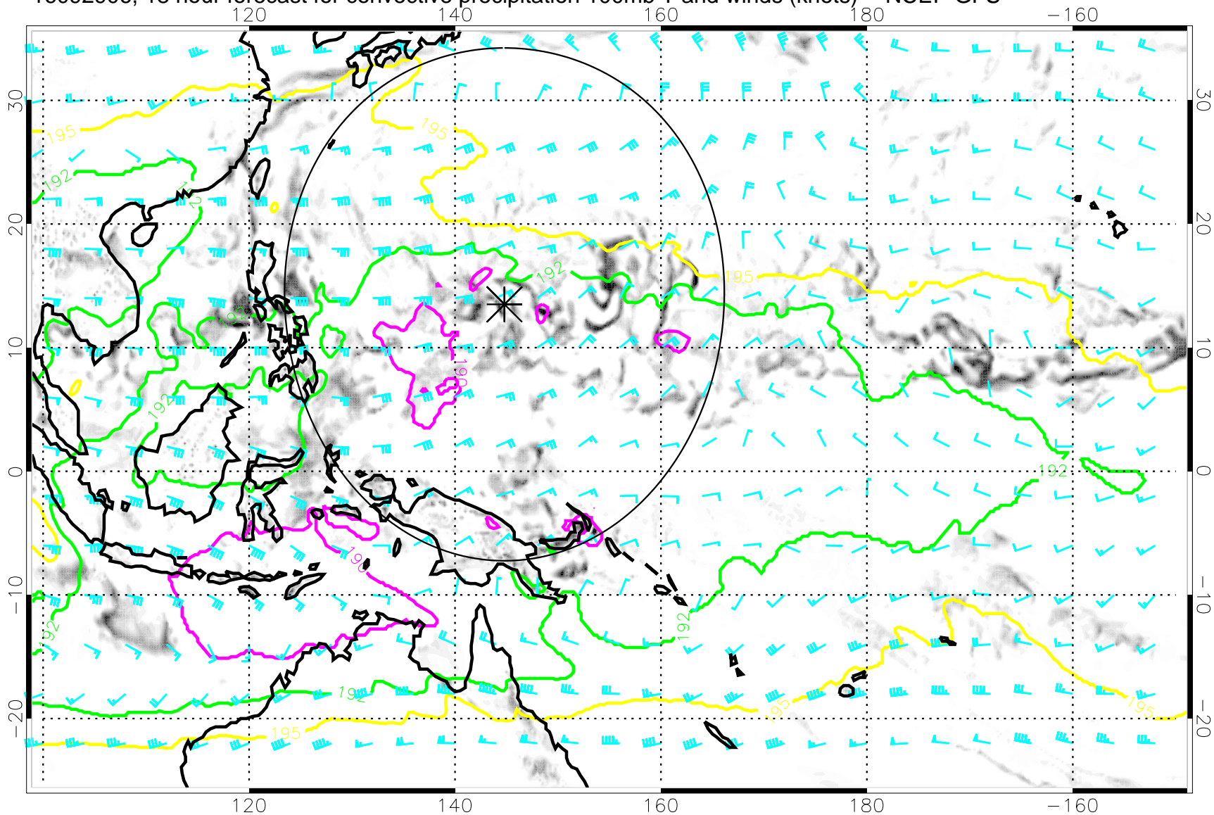
16092906, 18 hour forecast for convective precipitation 100mb T and winds (knots) -- NCEP GFS
