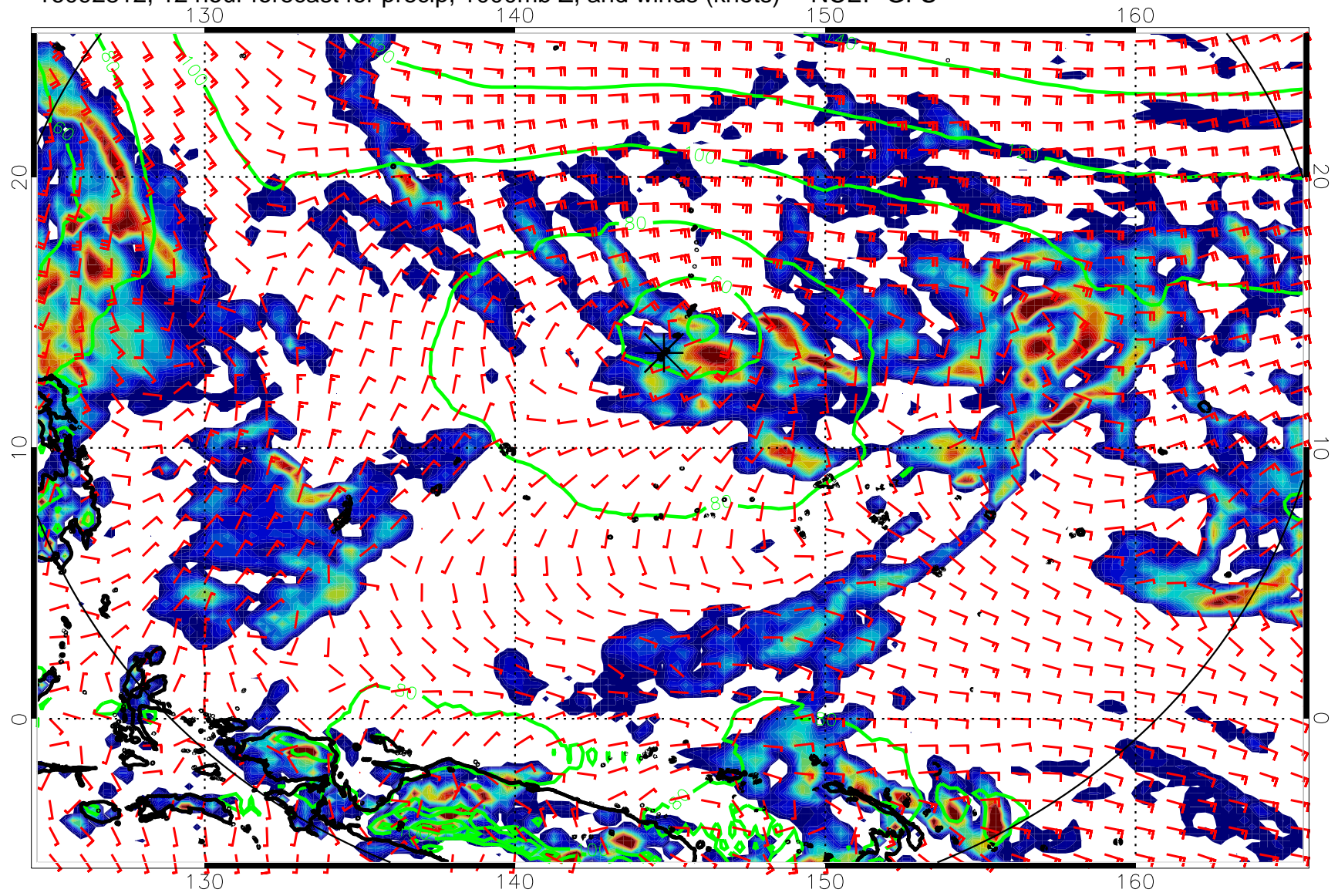
16092812, 12 hour forecast for precip, 1000mb Z, and winds (knots) -- NCEP GFS
