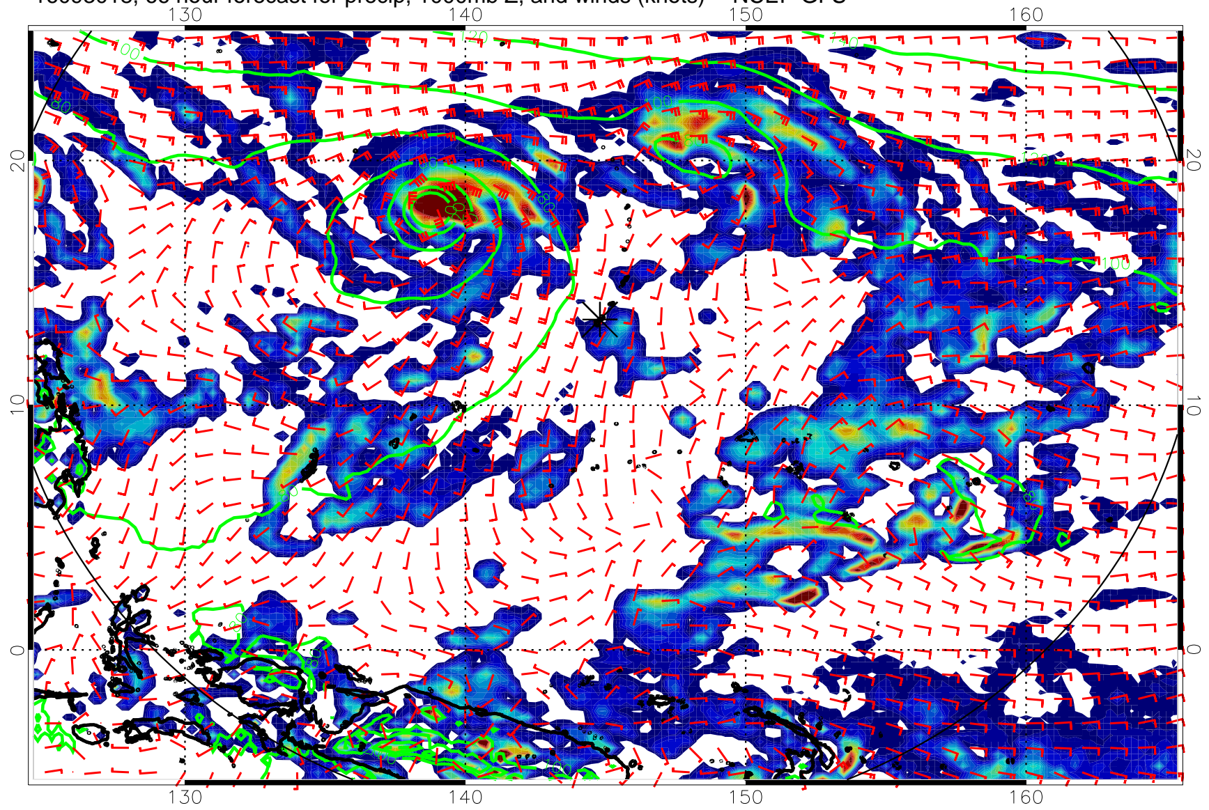
16093018, 66 hour forecast for precip, 1000mb Z, and winds (knots) -- NCEP GFS
