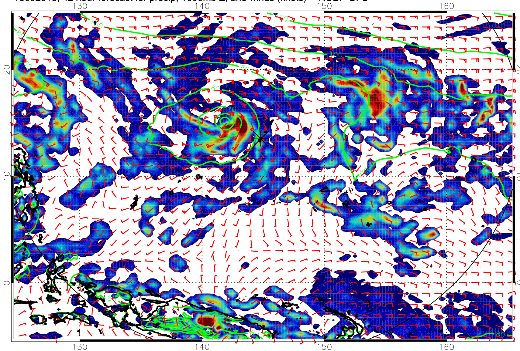
16092918, 42 hour forecast for precip, 1000mb Z, and winds (knots) -- NCEP GFS
