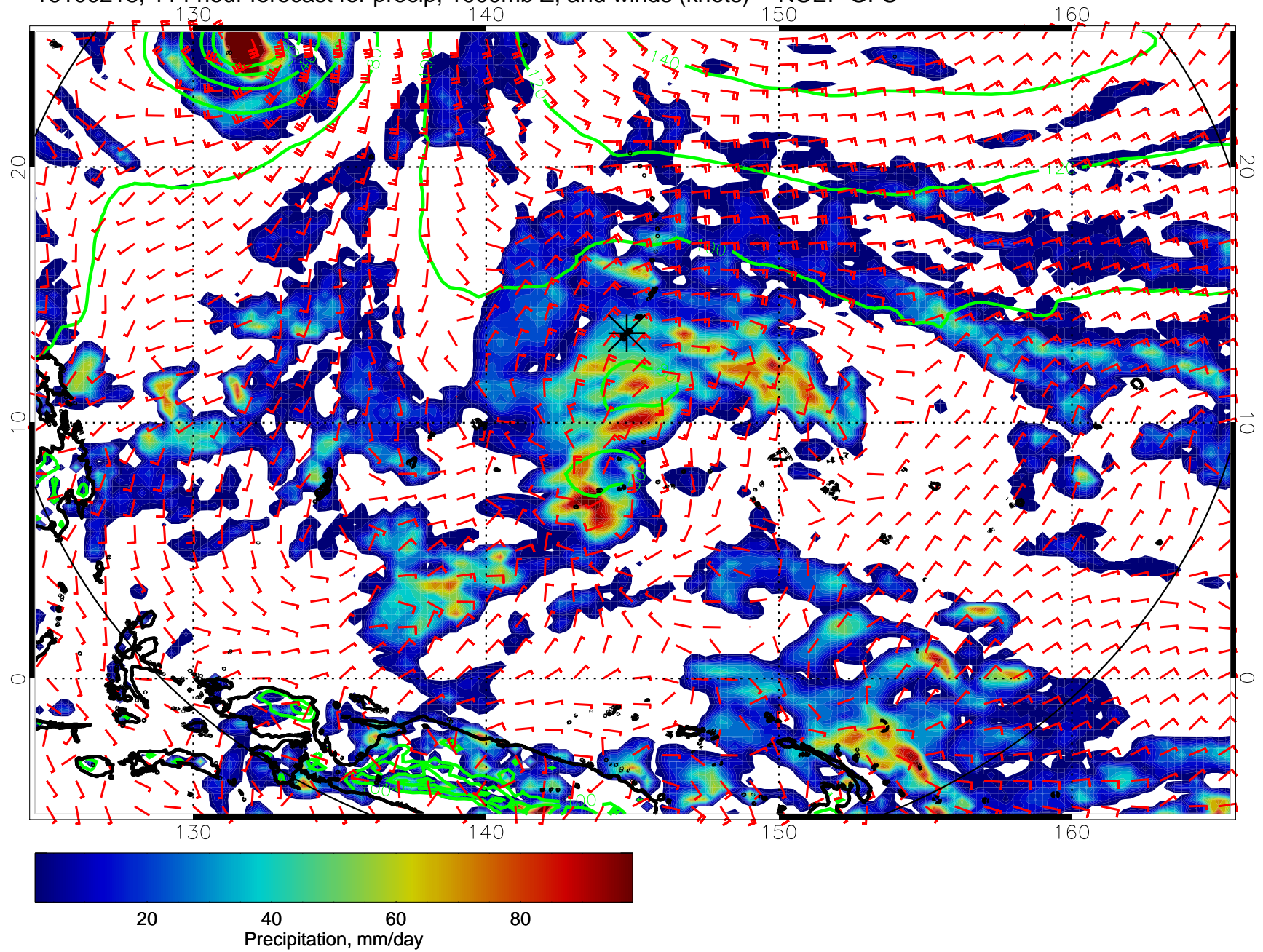
16100218, 114 hour forecast for precip, 1000mb Z, and winds (knots) -- NCEP GFS
