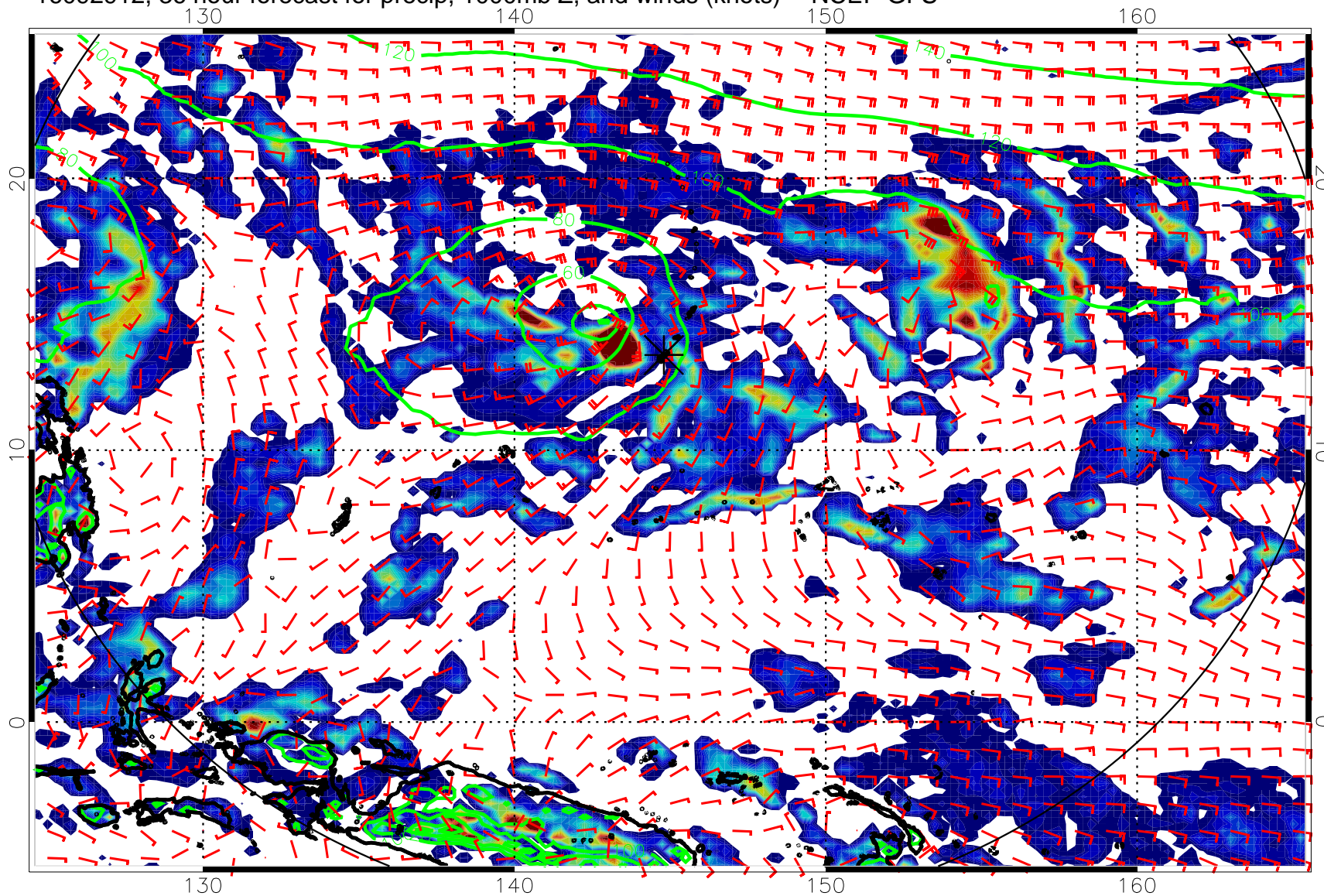
16092912, 36 hour forecast for precip, 1000mb Z, and winds (knots) -- NCEP GFS
