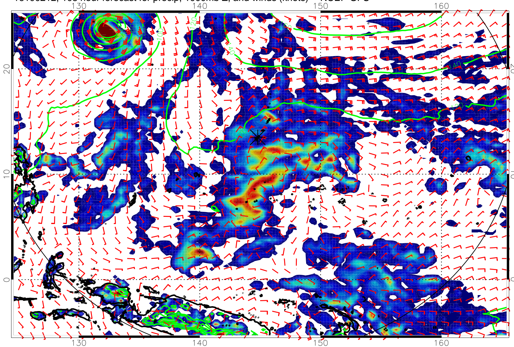
16100212, 108 hour forecast for precip, 1000mb Z, and winds (knots) -- NCEP GFS
