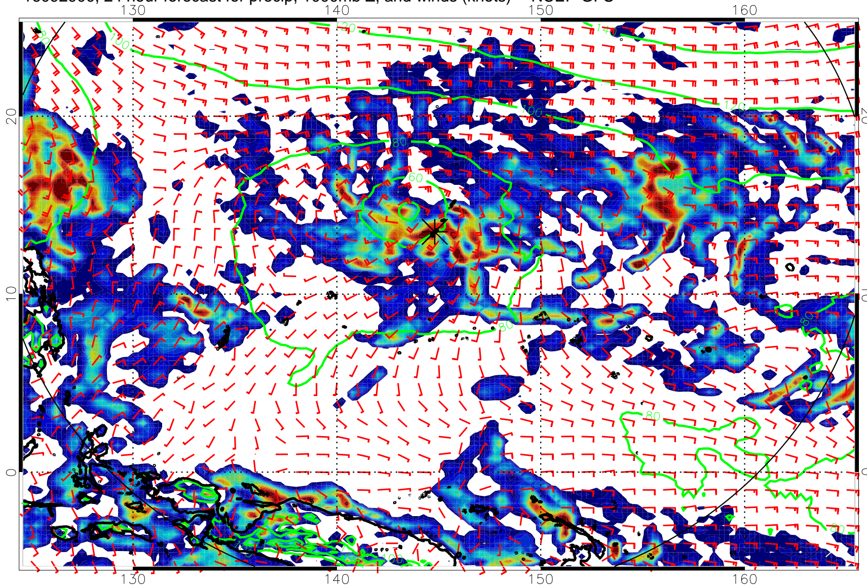
16092900, 24 hour forecast for precip, 1000mb Z, and winds (knots) -- NCEP GFS
