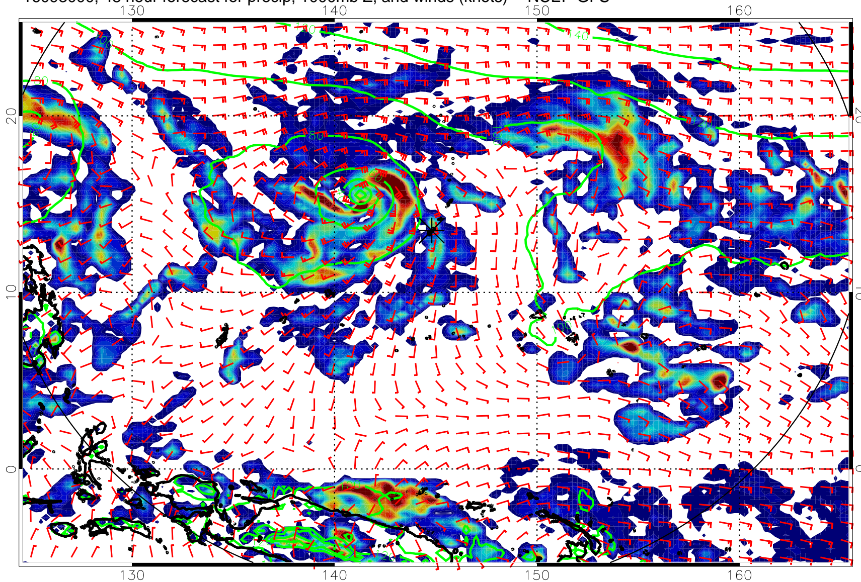
16093000, 48 hour forecast for precip, 1000mb Z, and winds (knots) -- NCEP GFS
