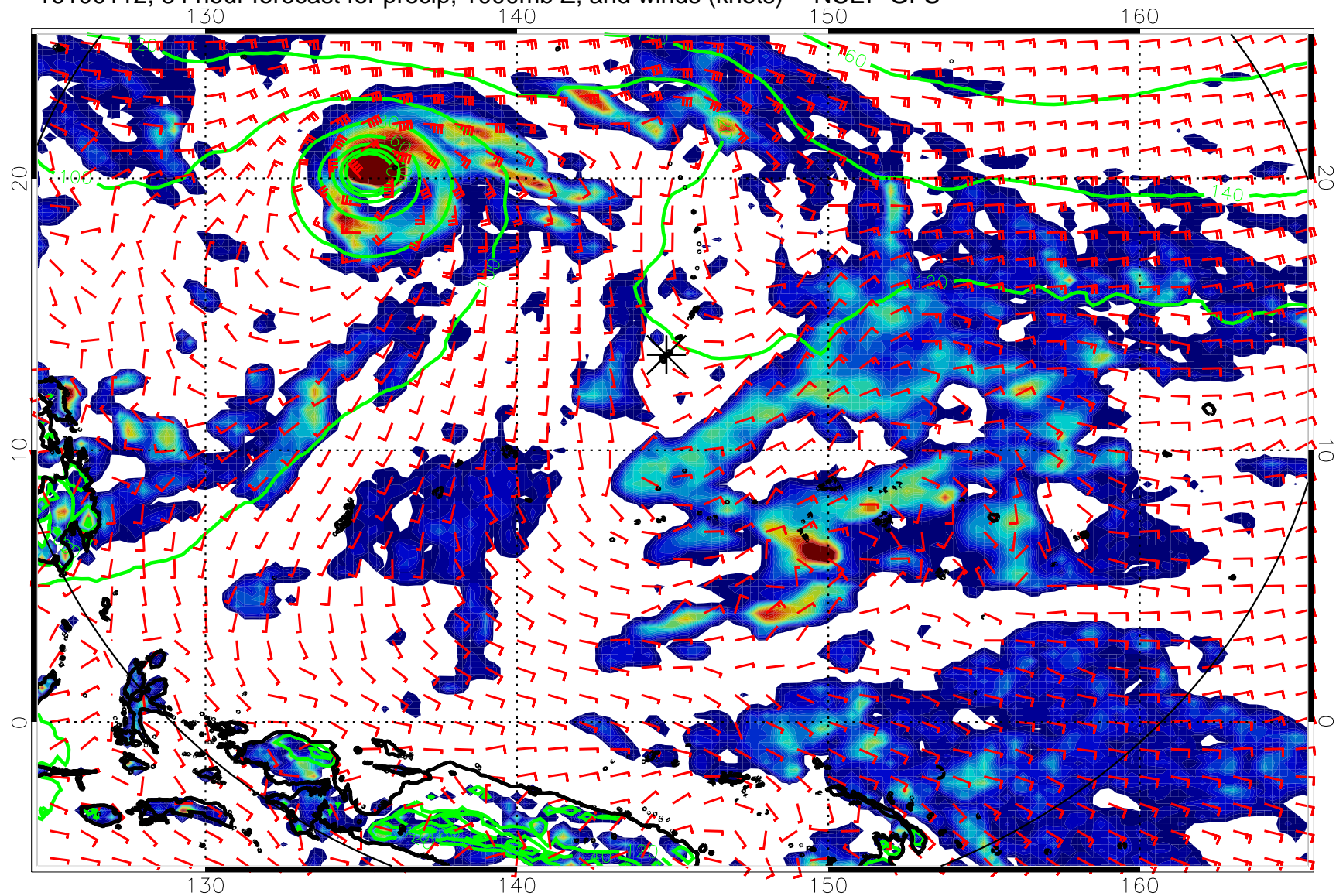
16100112, 84 hour forecast for precip, 1000mb Z, and winds (knots) -- NCEP GFS
