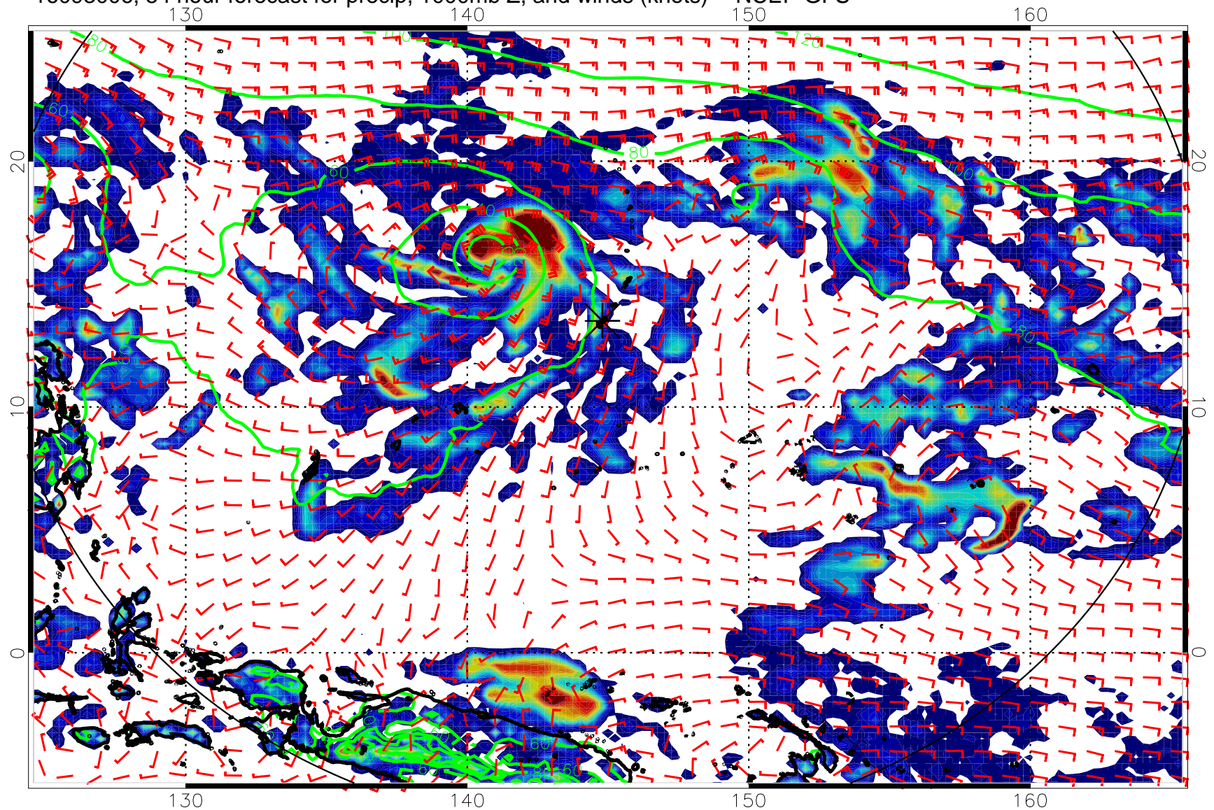
16093006, 54 hour forecast for precip, 1000mb Z, and winds (knots) -- NCEP GFS
