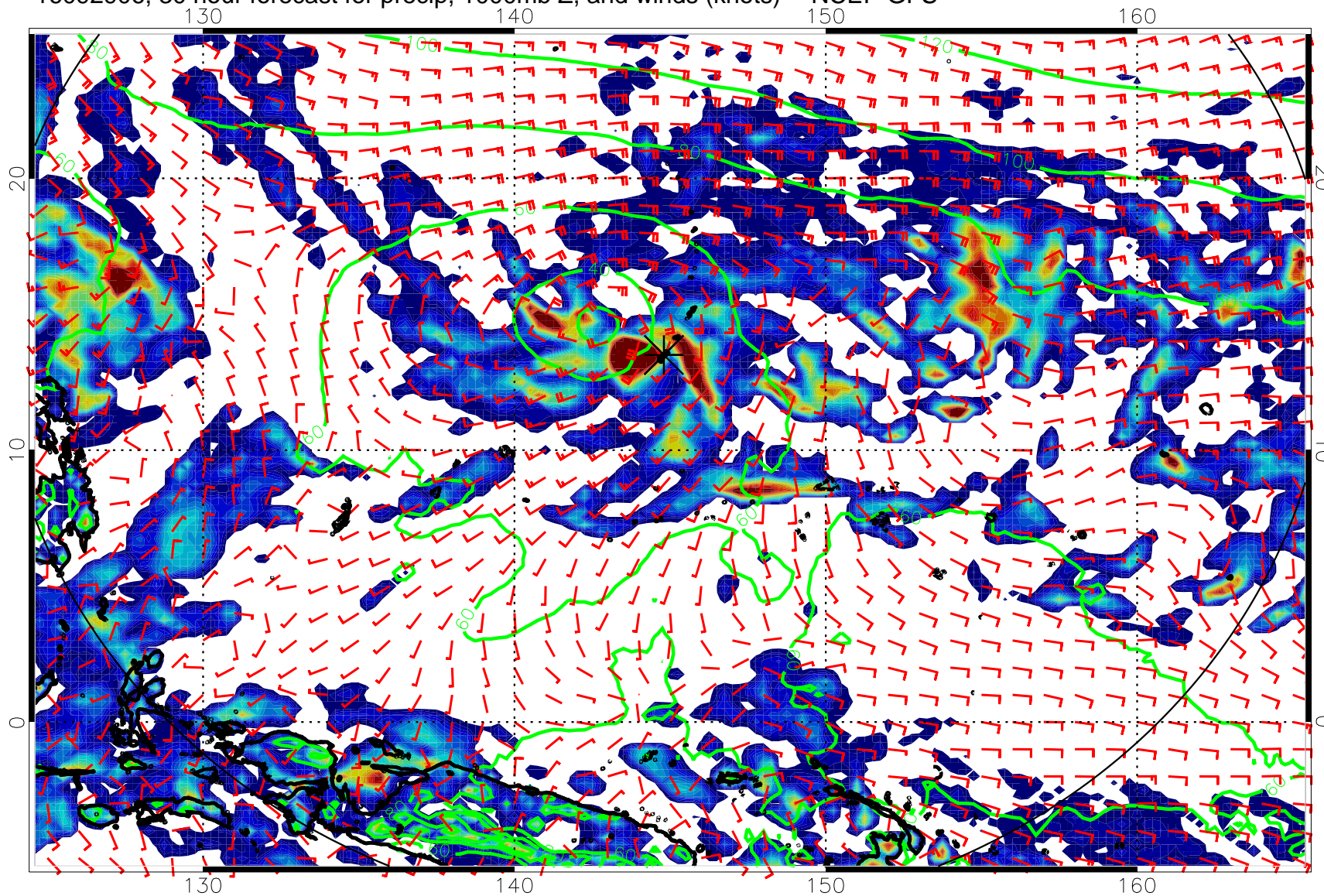
16092906, 30 hour forecast for precip, 1000mb Z, and winds (knots) -- NCEP GFS
