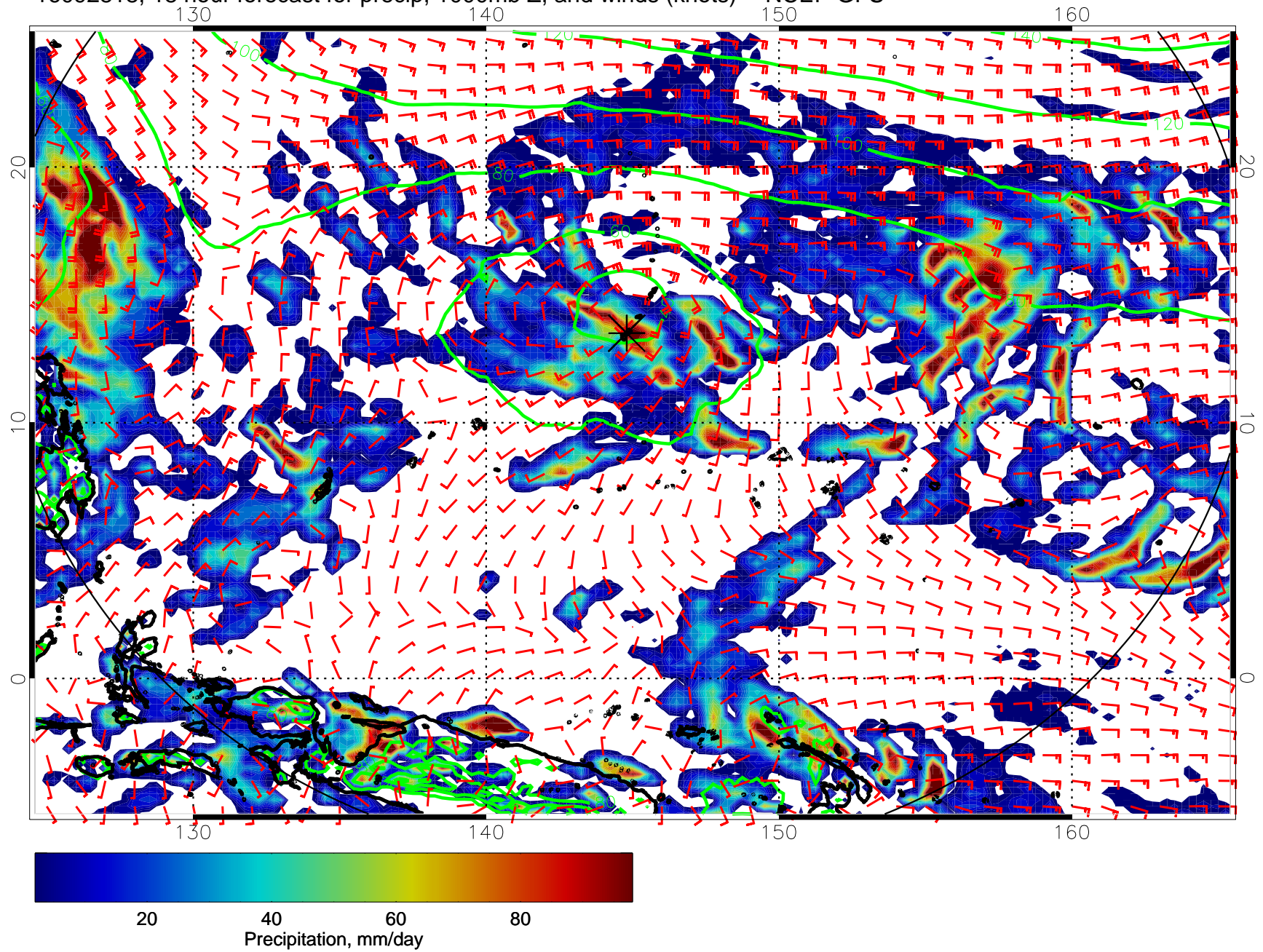
16092818, 18 hour forecast for precip, 1000mb Z, and winds (knots) -- NCEP GFS
