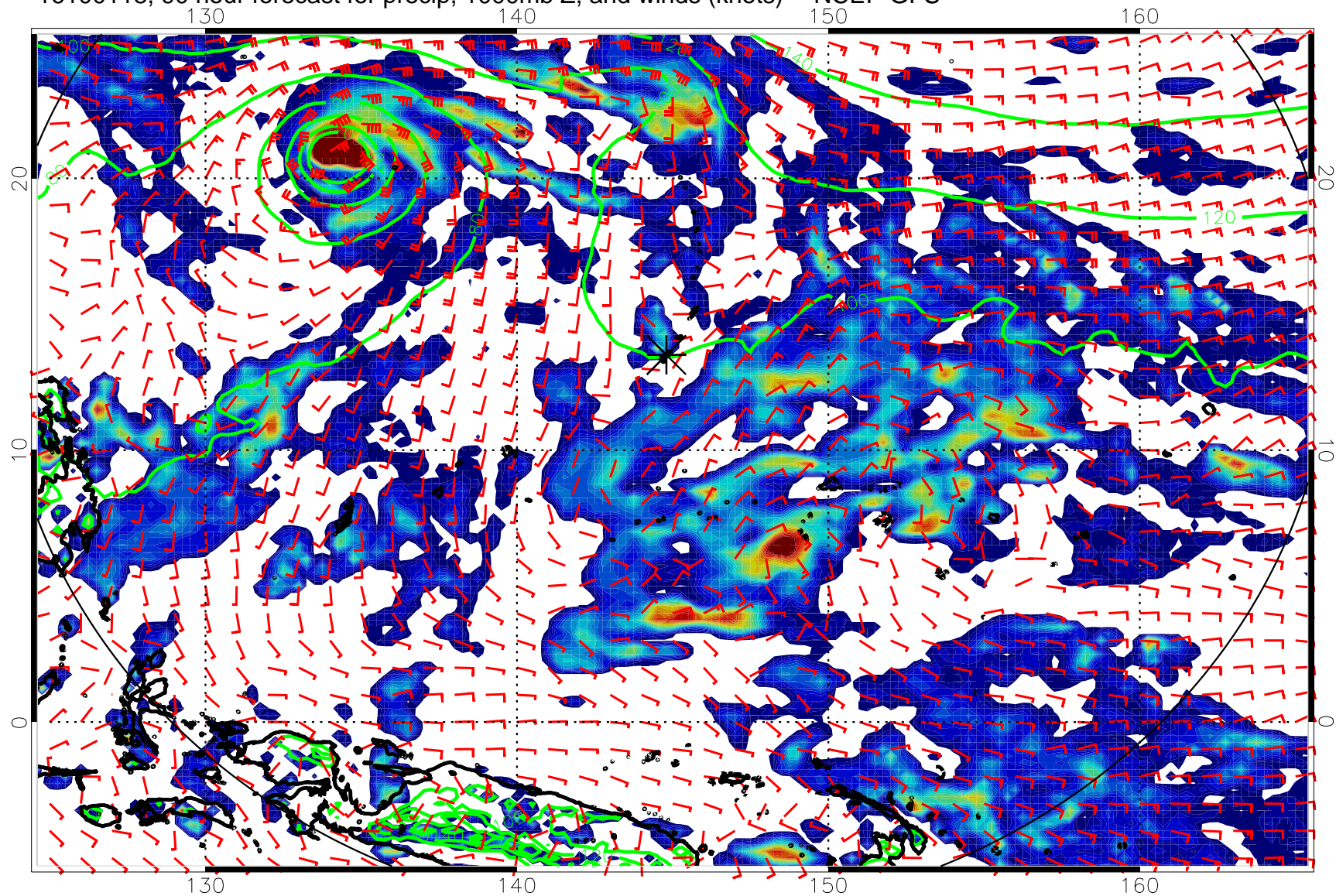
16100118, 90 hour forecast for precip, 1000mb Z, and winds (knots) -- NCEP GFS
