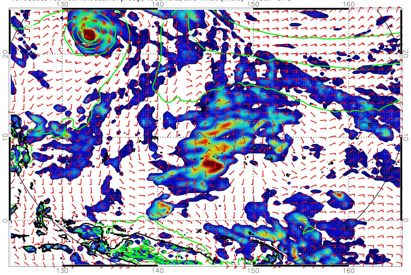
16100206, 102 hour forecast for precip, 1000mb Z, and winds (knots) -- NCEP GFS
