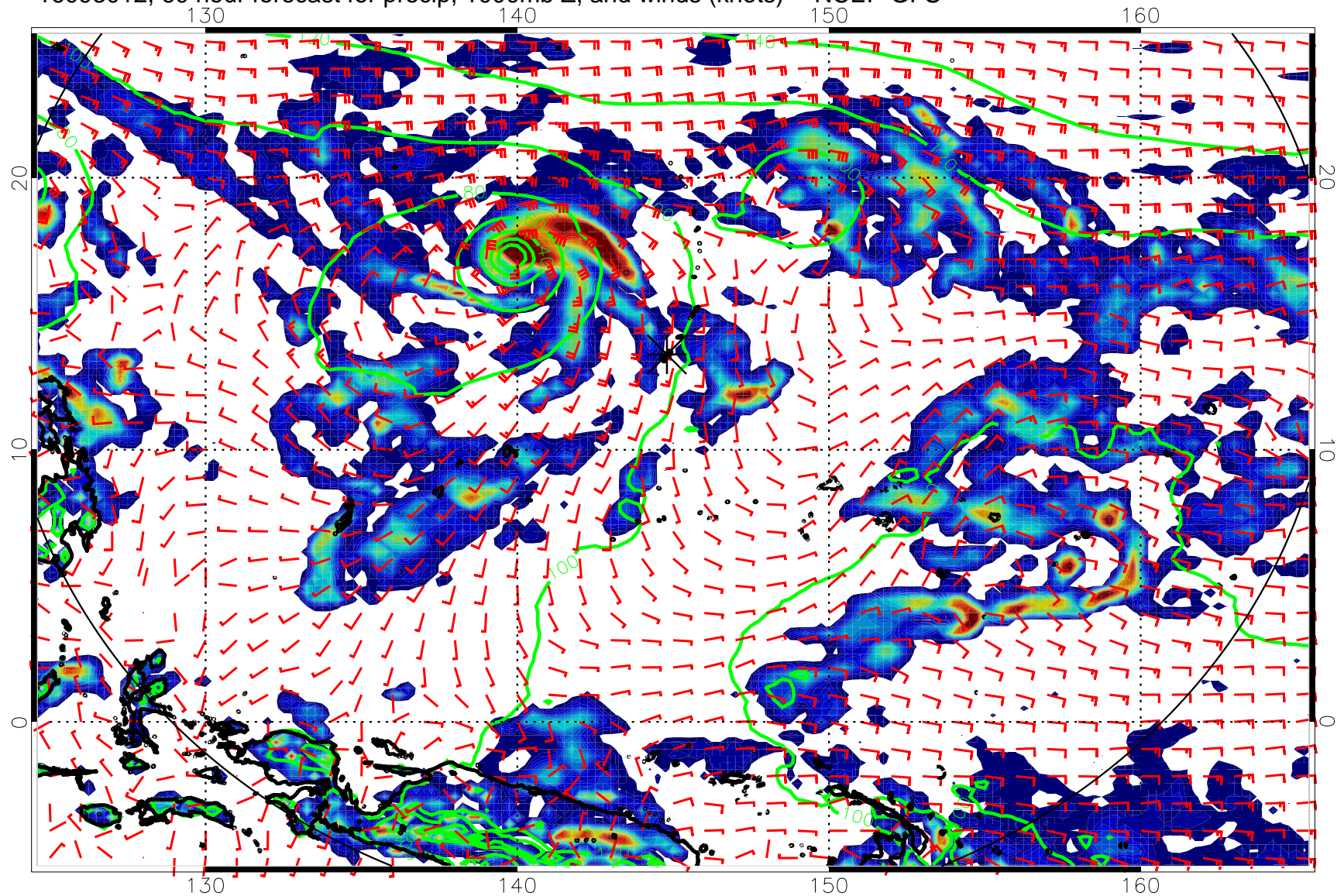
16093012, 60 hour forecast for precip, 1000mb Z, and winds (knots) -- NCEP GFS
