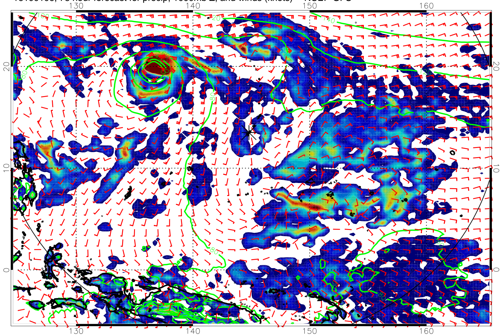
16100106, 78 hour forecast for precip, 1000mb Z, and winds (knots) -- NCEP GFS
