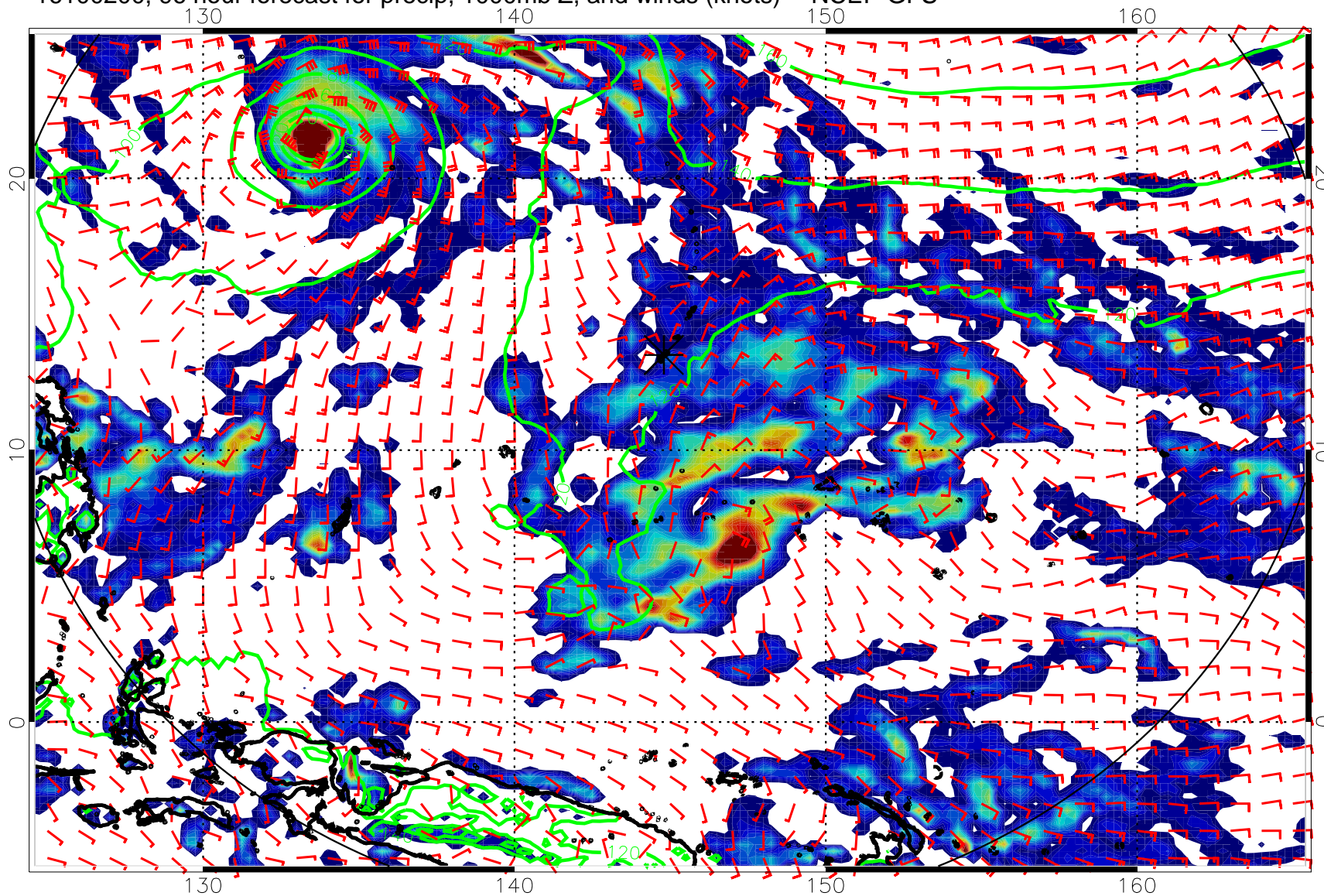
16100200, 96 hour forecast for precip, 1000mb Z, and winds (knots) -- NCEP GFS
