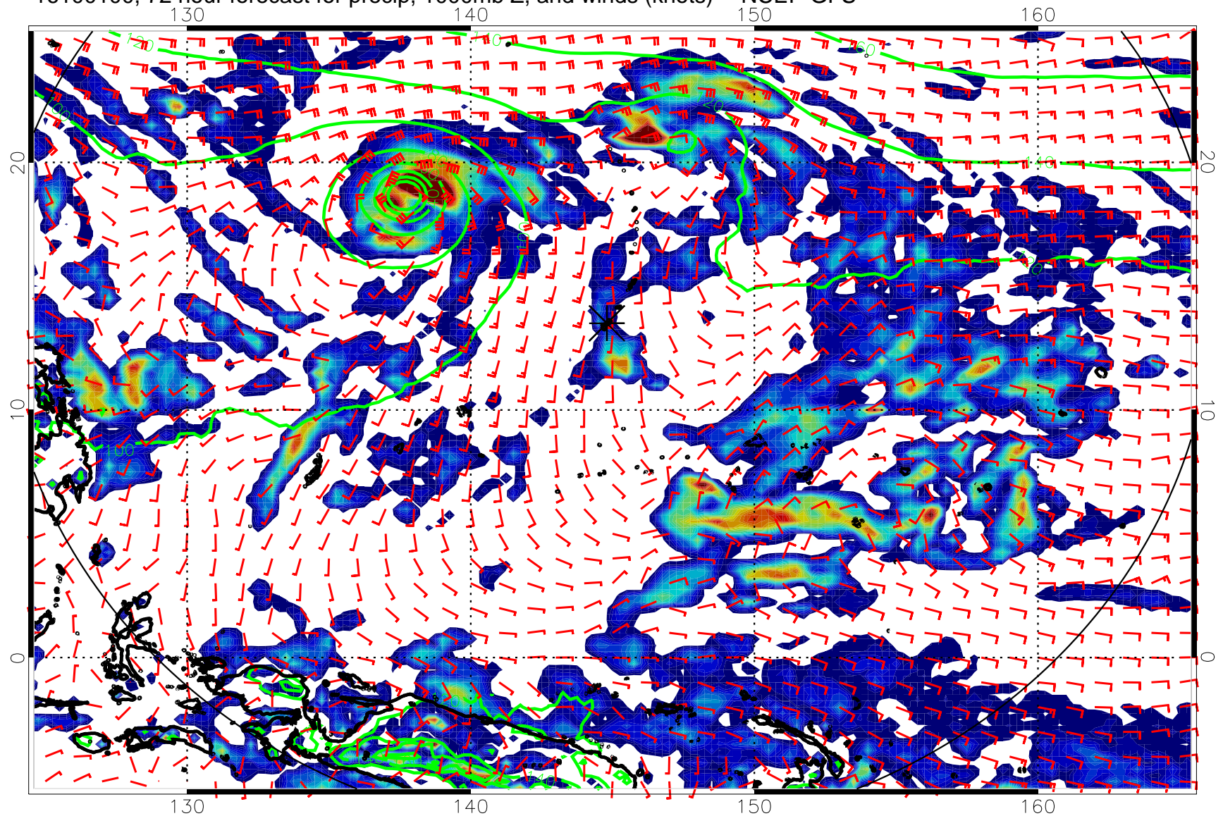
16100100, 72 hour forecast for precip, 1000mb Z, and winds (knots) -- NCEP GFS
