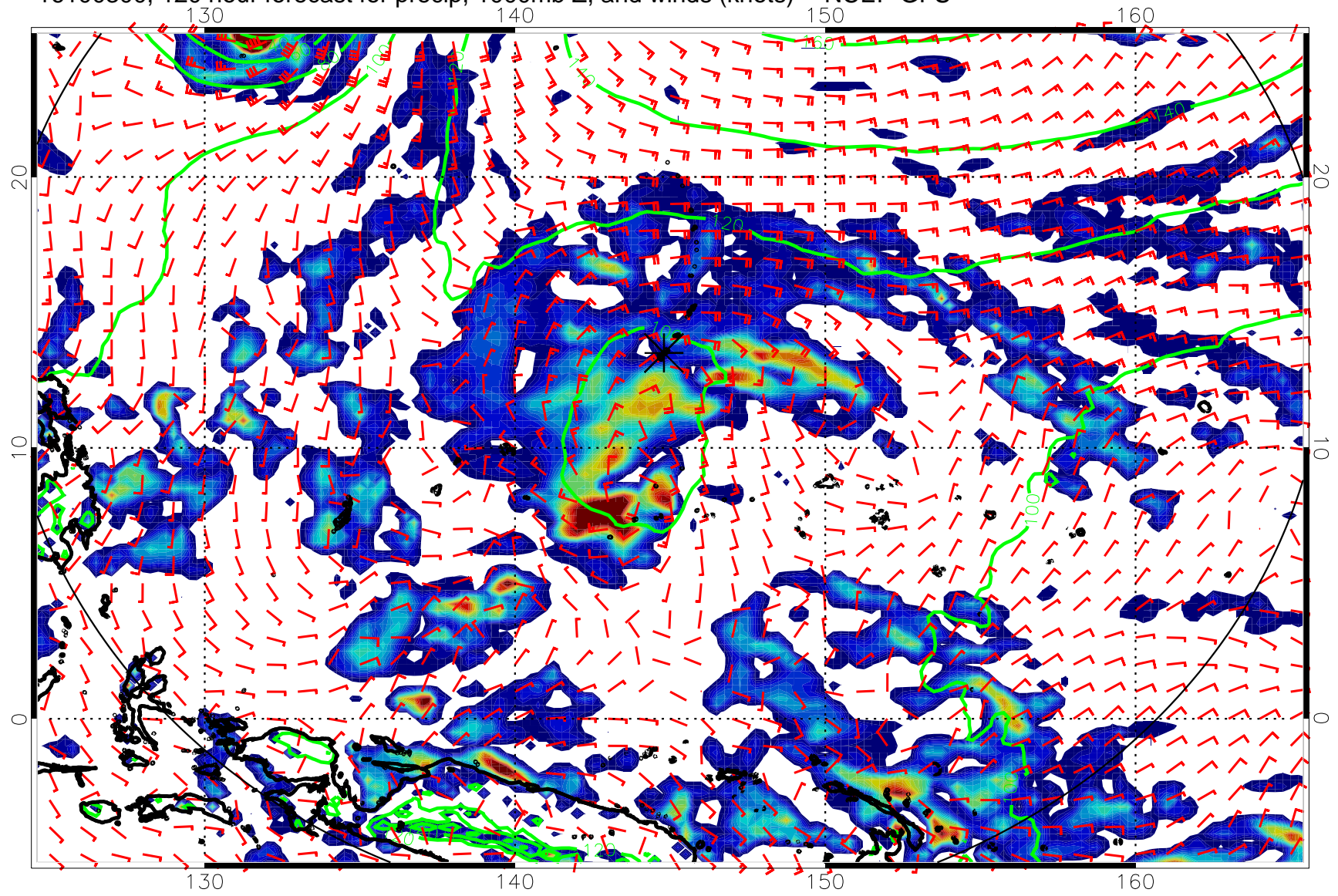
16100300, 120 hour forecast for precip, 1000mb Z, and winds (knots) -- NCEP GFS
