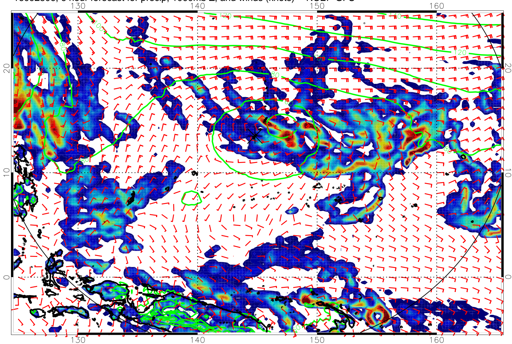
16092806, 6 hour forecast for precip, 1000mb Z, and winds (knots) -- NCEP GFS
