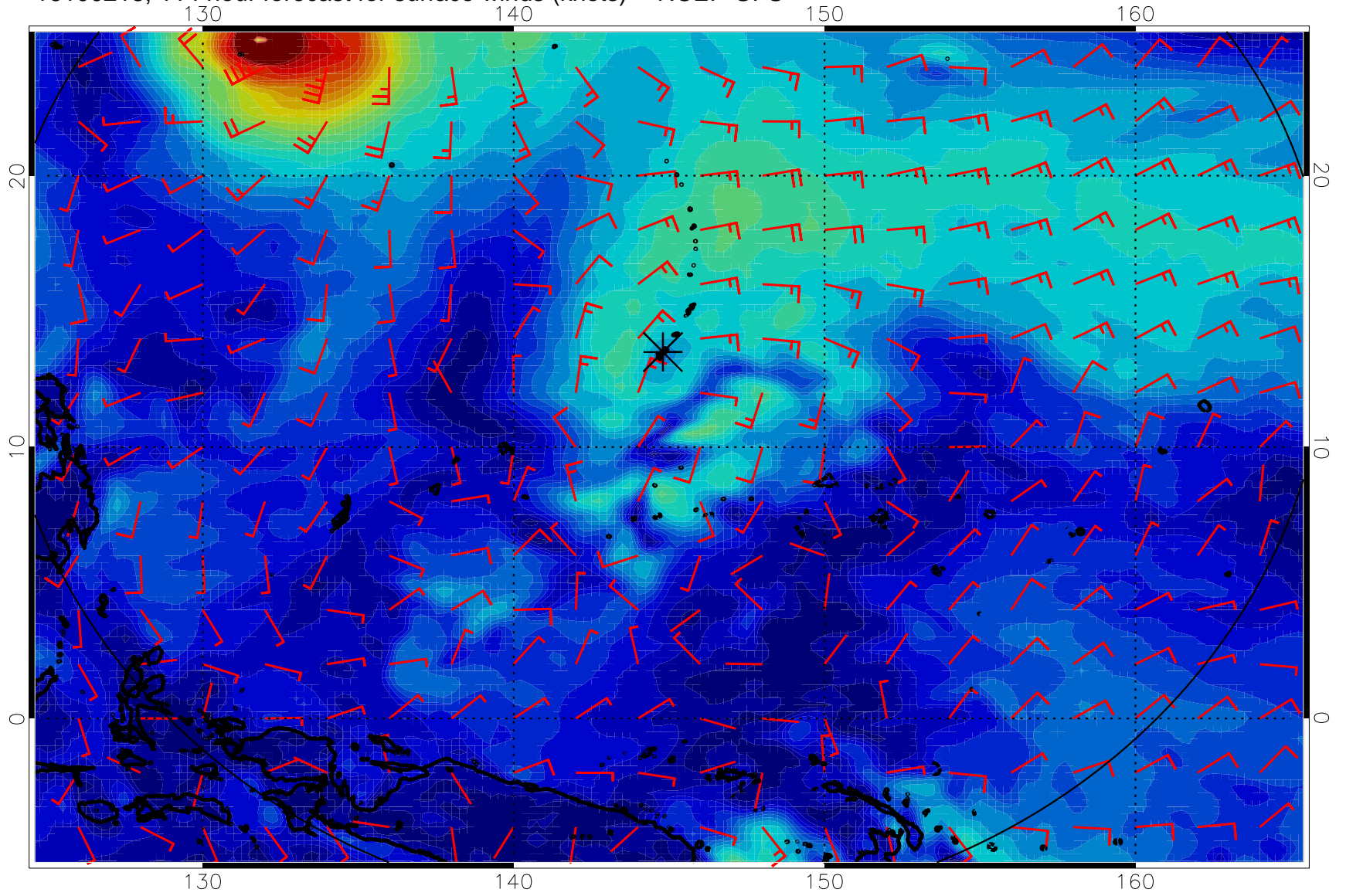
16100218, 114 hour forecast for surface winds (knots) -- NCEP GFS
