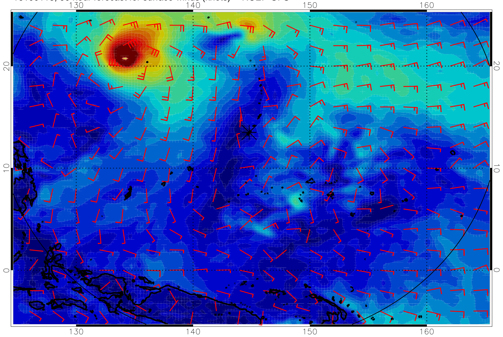
16100118, 90 hour forecast for surface winds (knots) -- NCEP GFS
