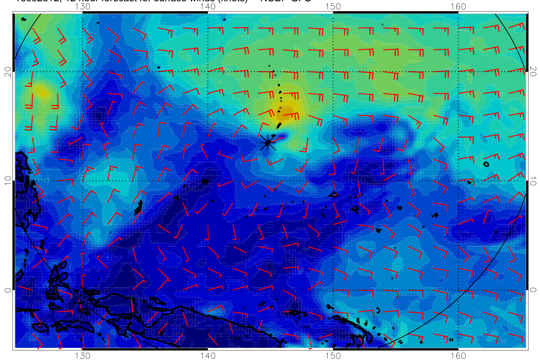
16092812, 12 hour forecast for surface winds (knots) -- NCEP GFS
