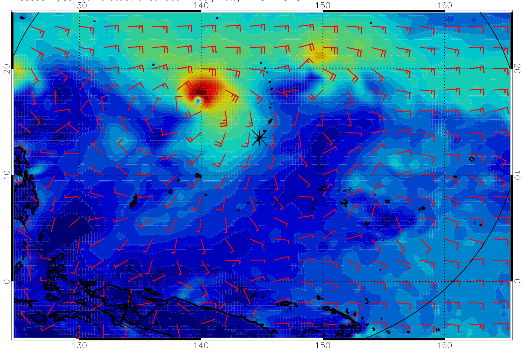
16093012, 60 hour forecast for surface winds (knots) -- NCEP GFS
