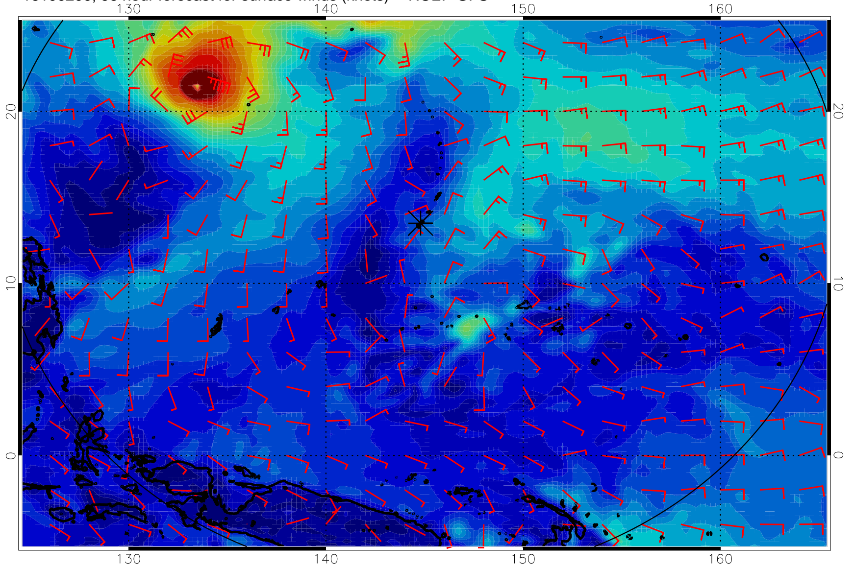
16100200, 96 hour forecast for surface winds (knots) -- NCEP GFS
