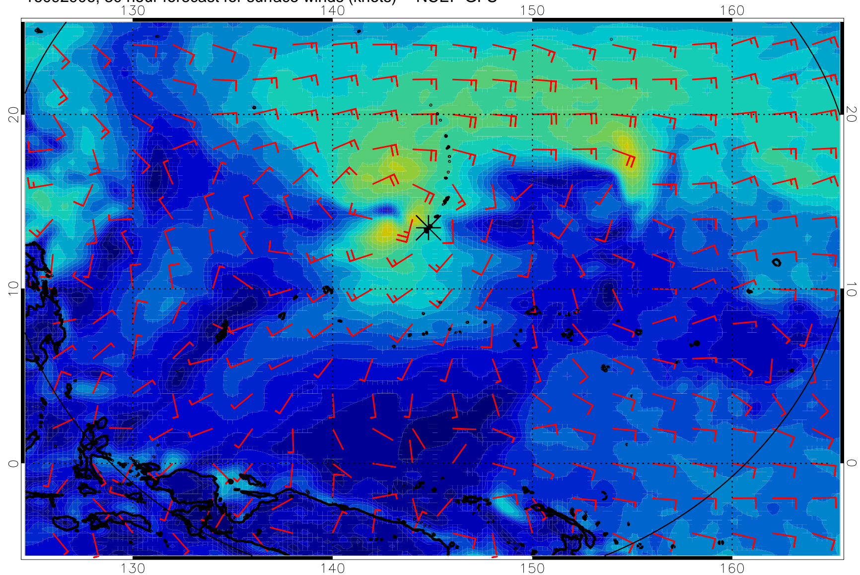
16092906, 30 hour forecast for surface winds (knots) -- NCEP GFS
