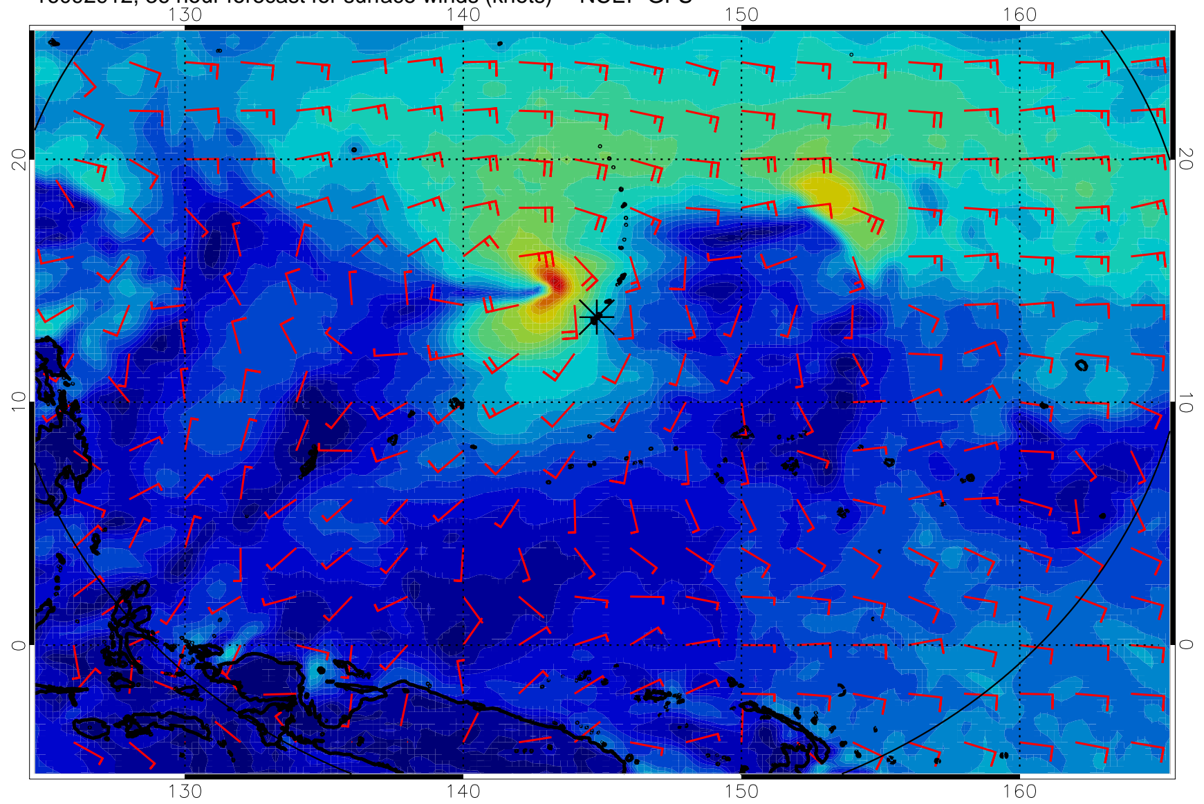
16092912, 36 hour forecast for surface winds (knots) -- NCEP GFS
