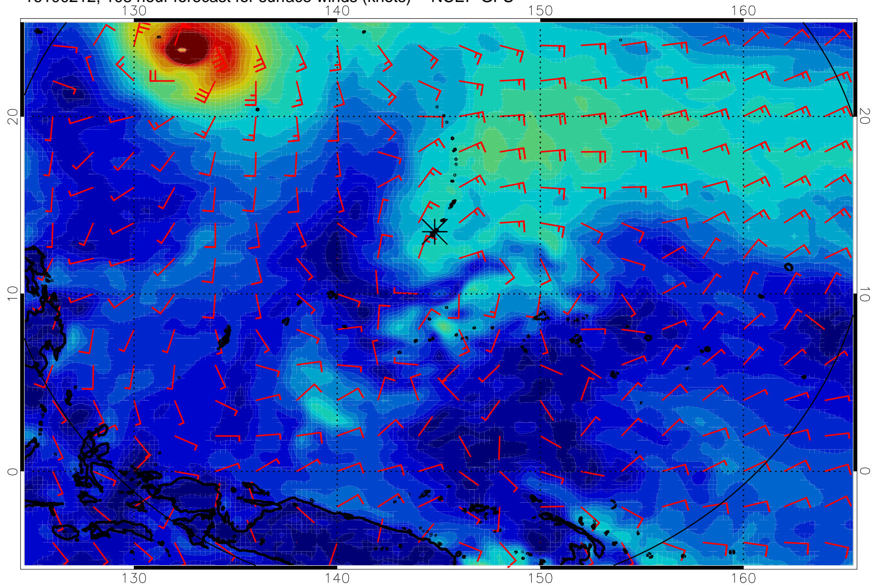
16100212, 108 hour forecast for surface winds (knots) -- NCEP GFS
