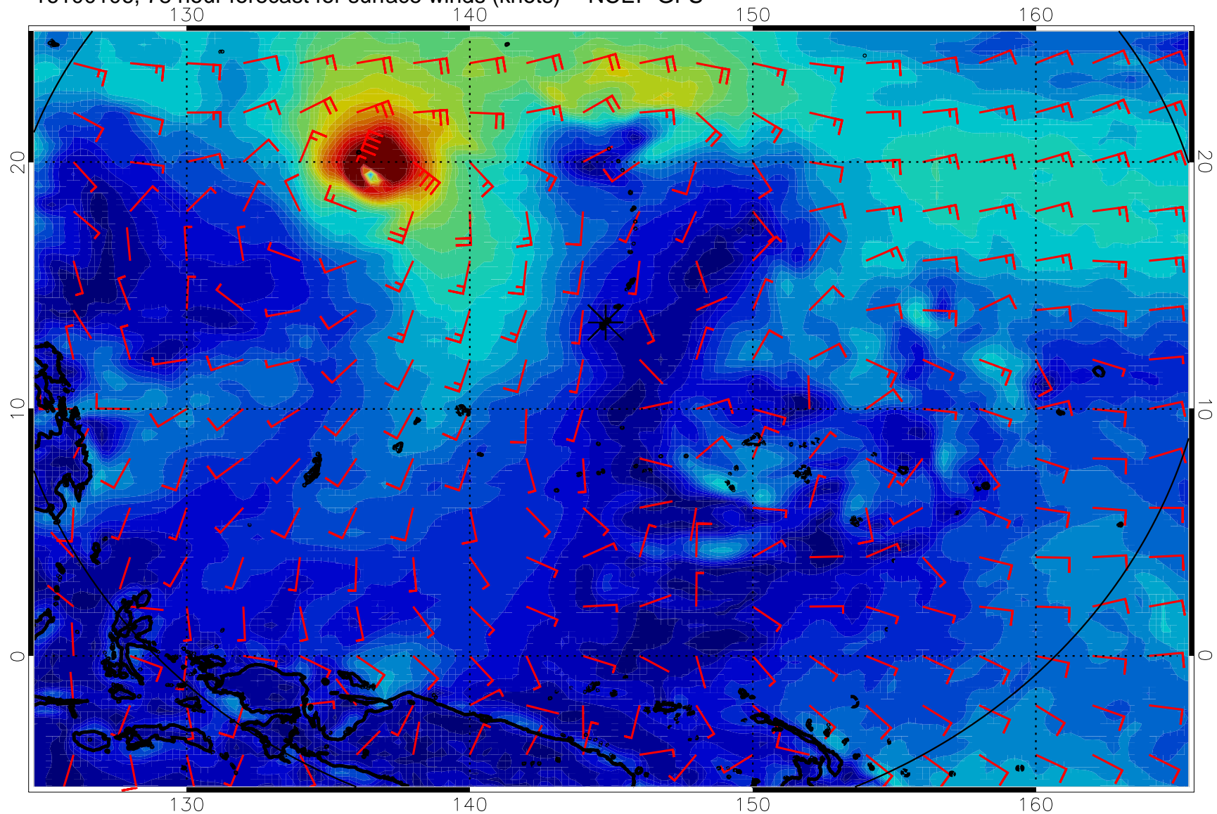
16100106, 78 hour forecast for surface winds (knots) -- NCEP GFS
