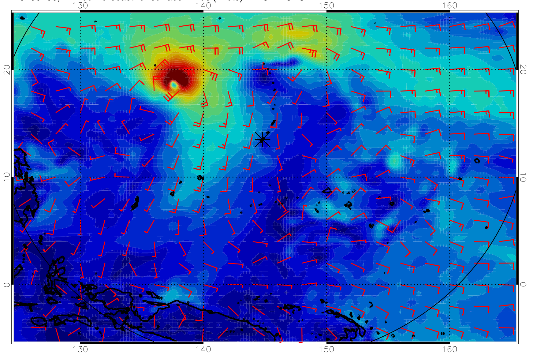
16100100, 72 hour forecast for surface winds (knots) -- NCEP GFS
