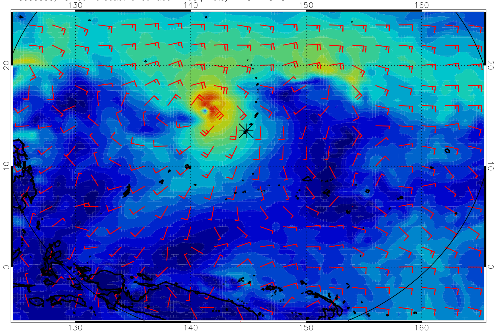
16093000, 48 hour forecast for surface winds (knots) -- NCEP GFS
