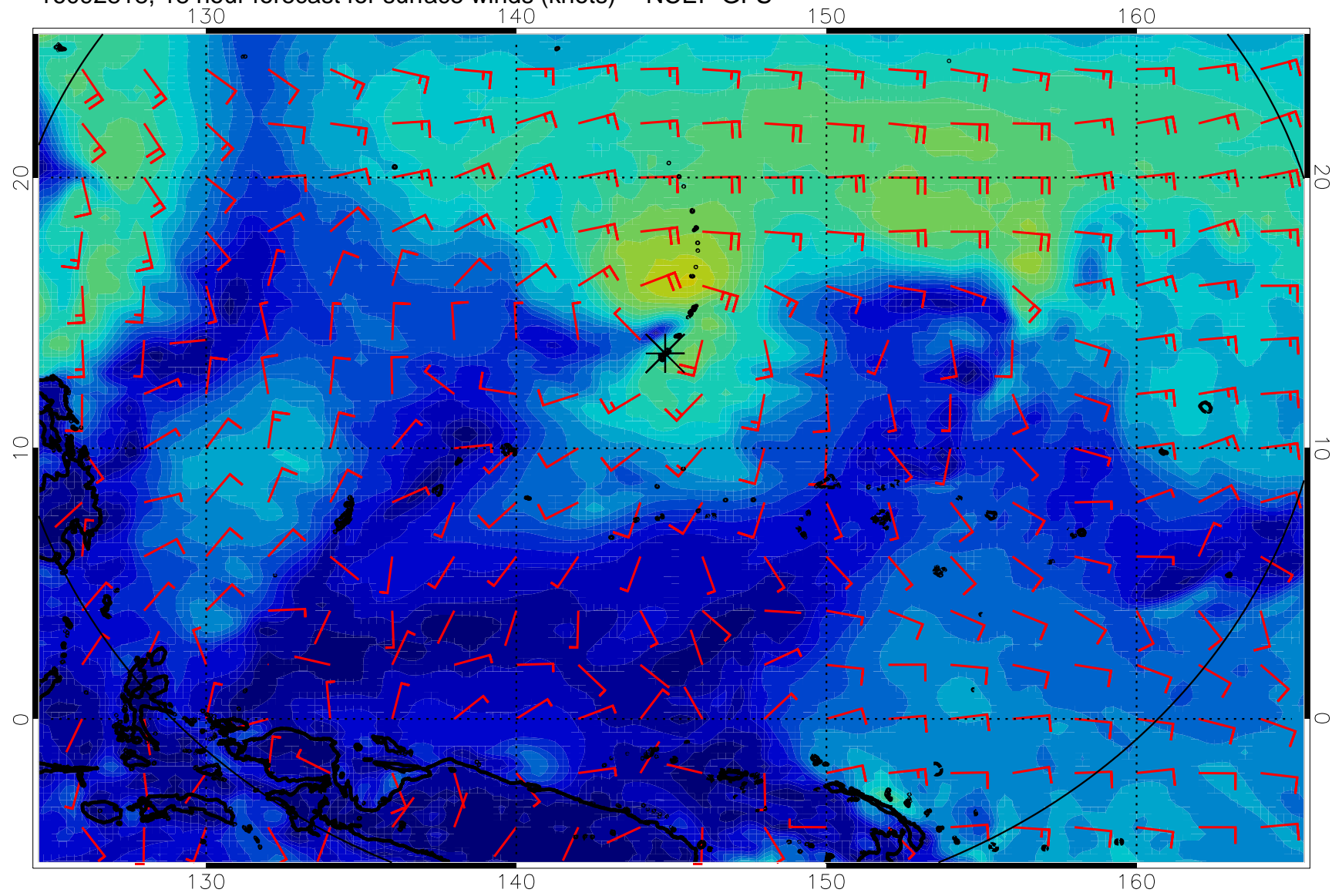
16092818, 18 hour forecast for surface winds (knots) -- NCEP GFS
