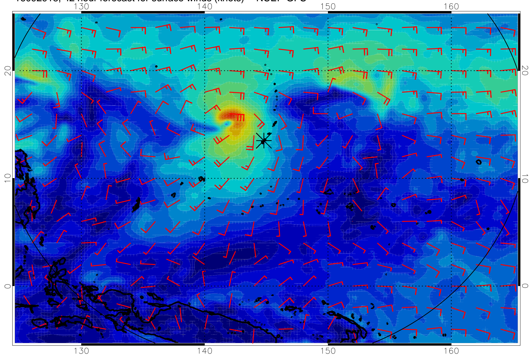
16092918, 42 hour forecast for surface winds (knots) -- NCEP GFS
