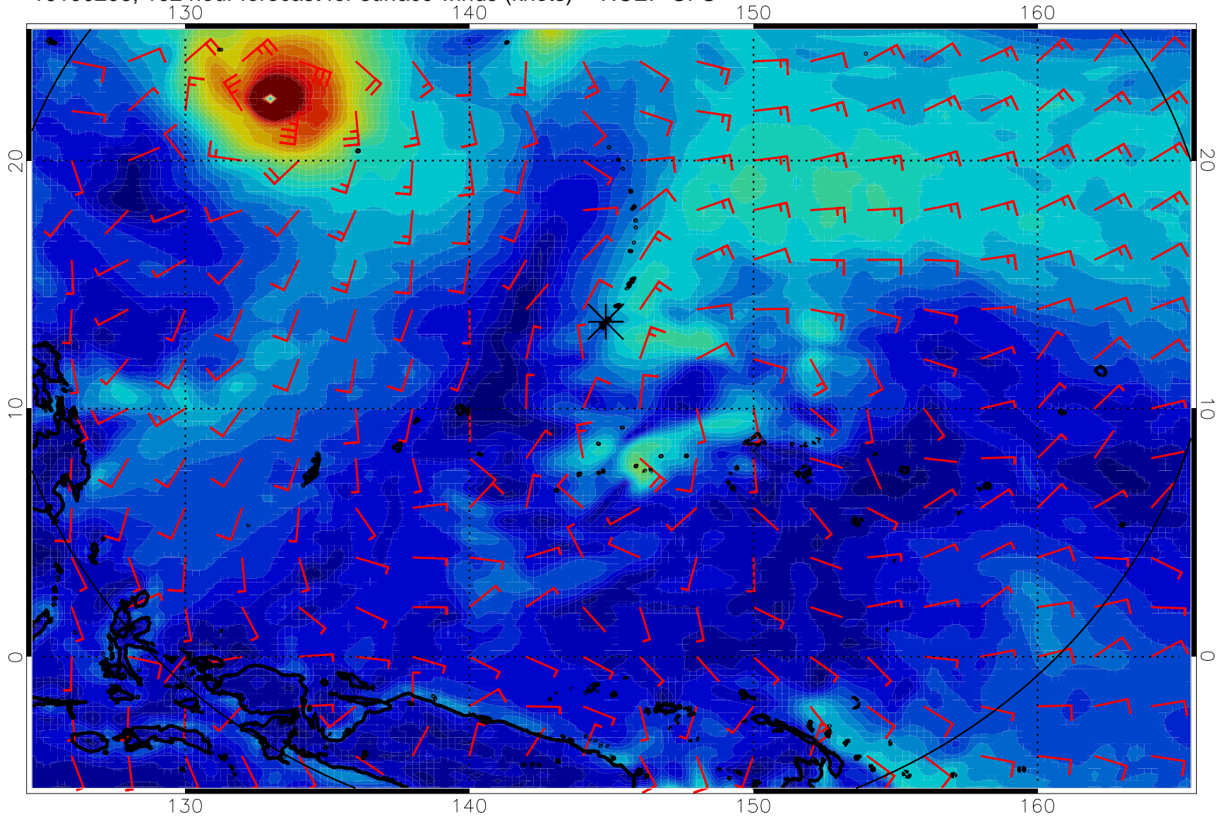
16100206, 102 hour forecast for surface winds (knots) -- NCEP GFS
