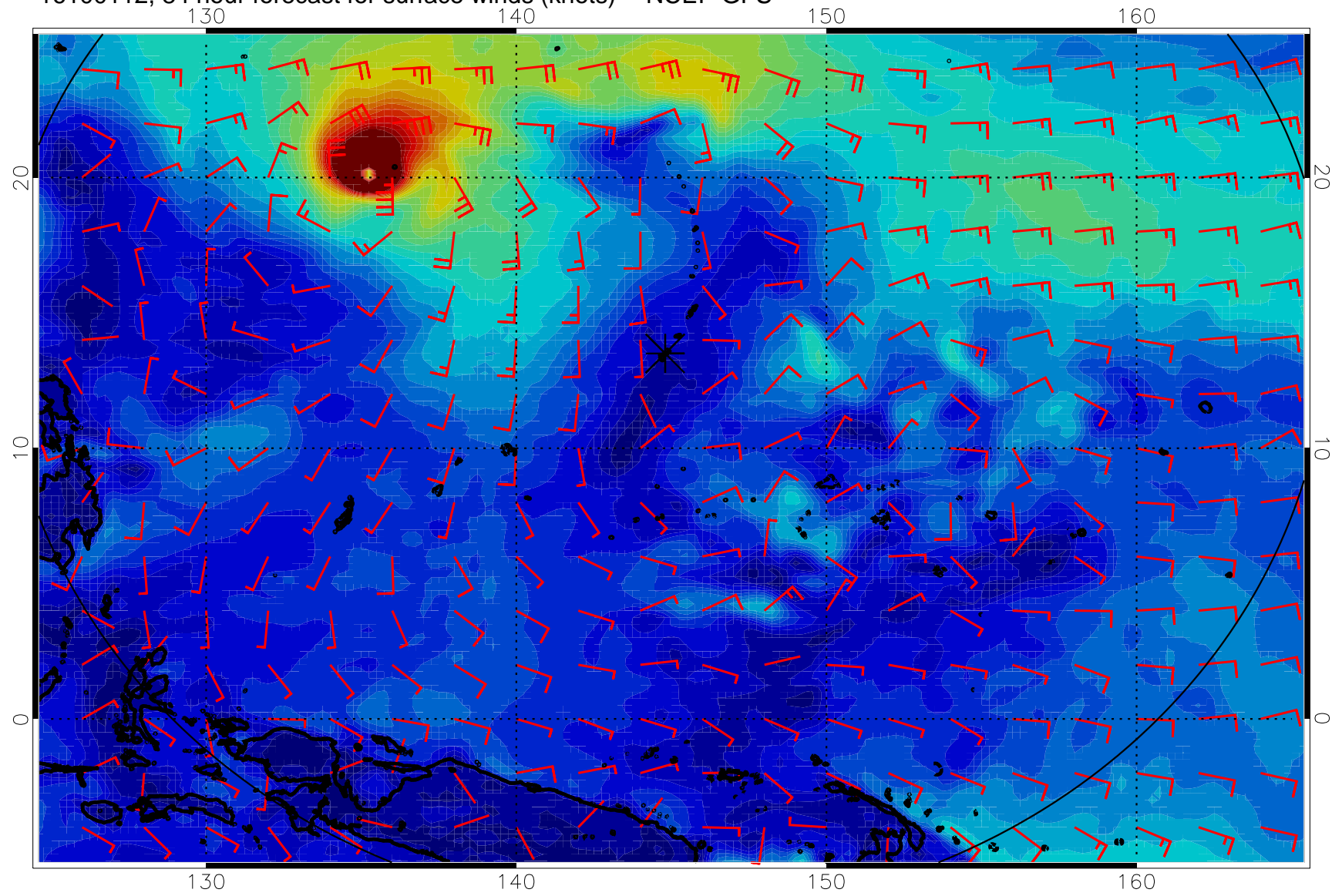
16100112, 84 hour forecast for surface winds (knots) -- NCEP GFS
