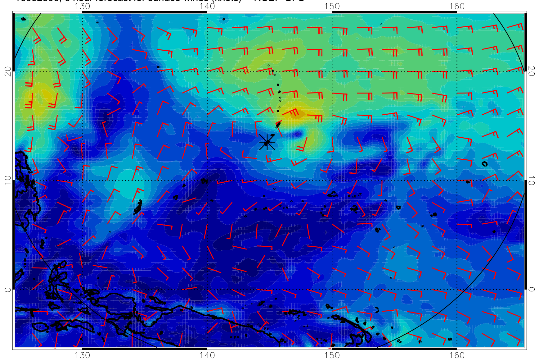
16092806, 6 hour forecast for surface winds (knots) -- NCEP GFS
