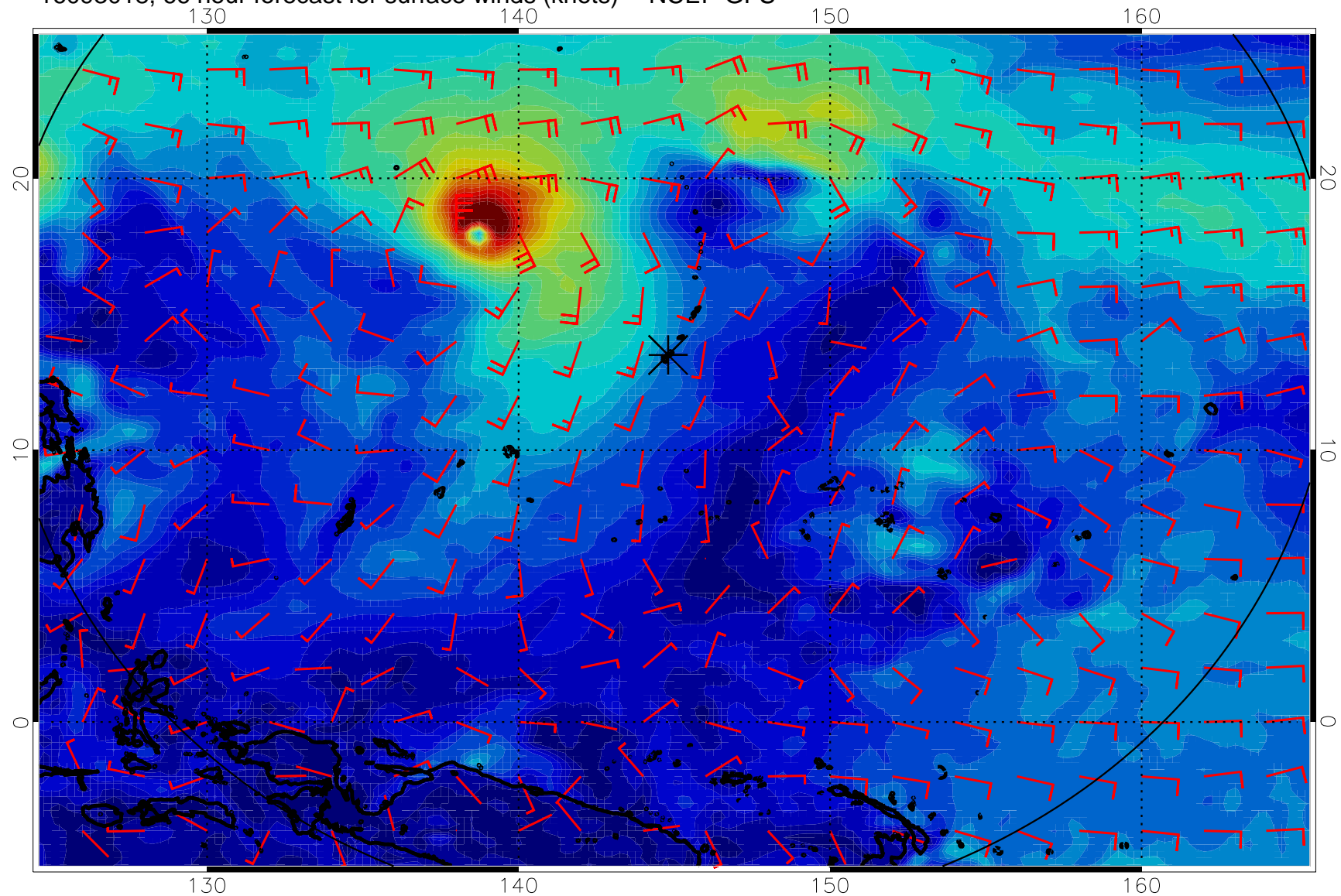
16093018, 66 hour forecast for surface winds (knots) -- NCEP GFS
