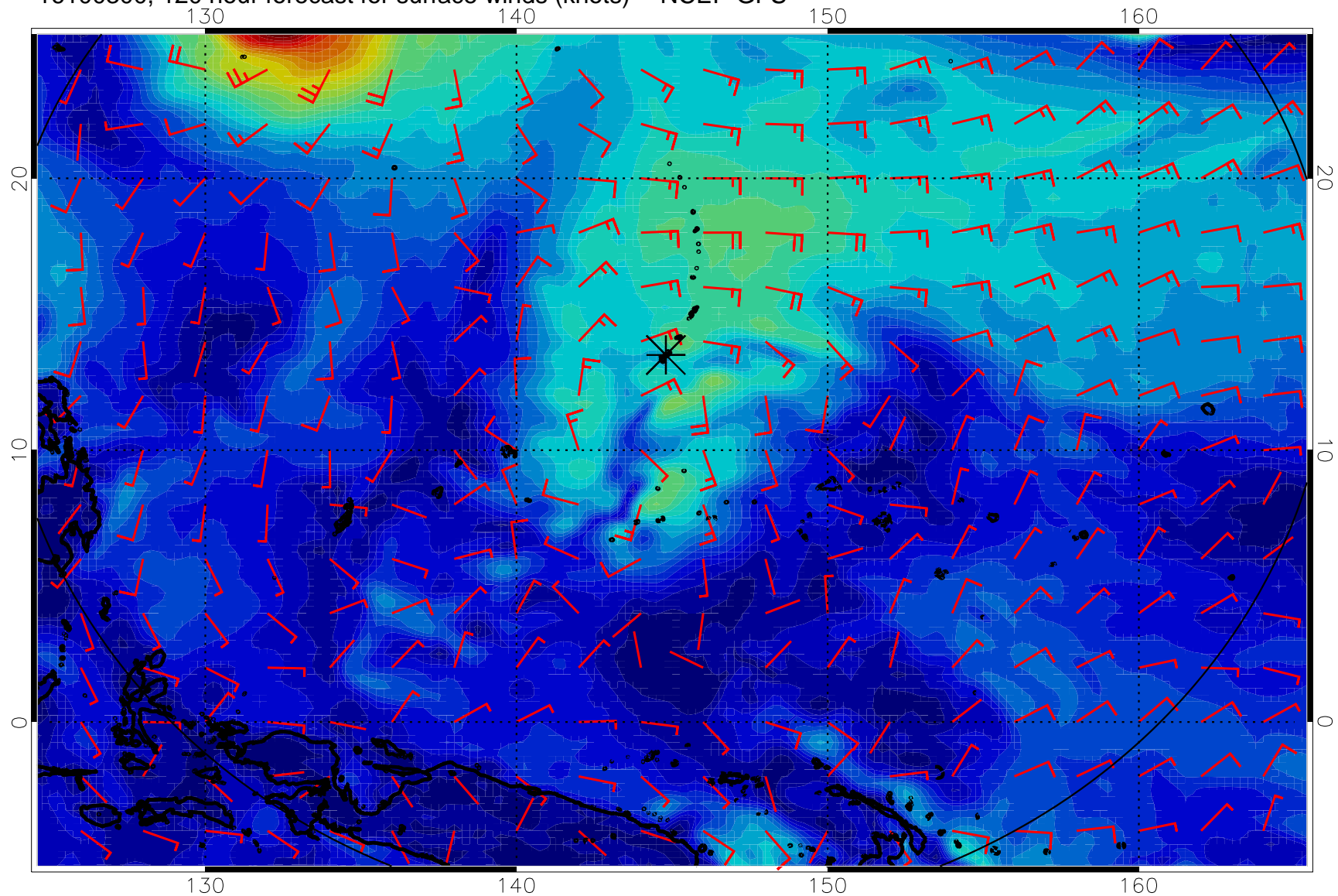
16100300, 120 hour forecast for surface winds (knots) -- NCEP GFS
