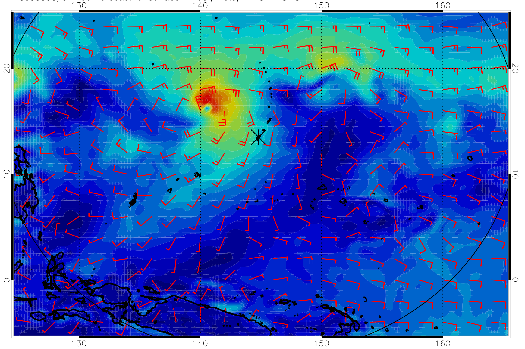
16093006, 54 hour forecast for surface winds (knots) -- NCEP GFS
