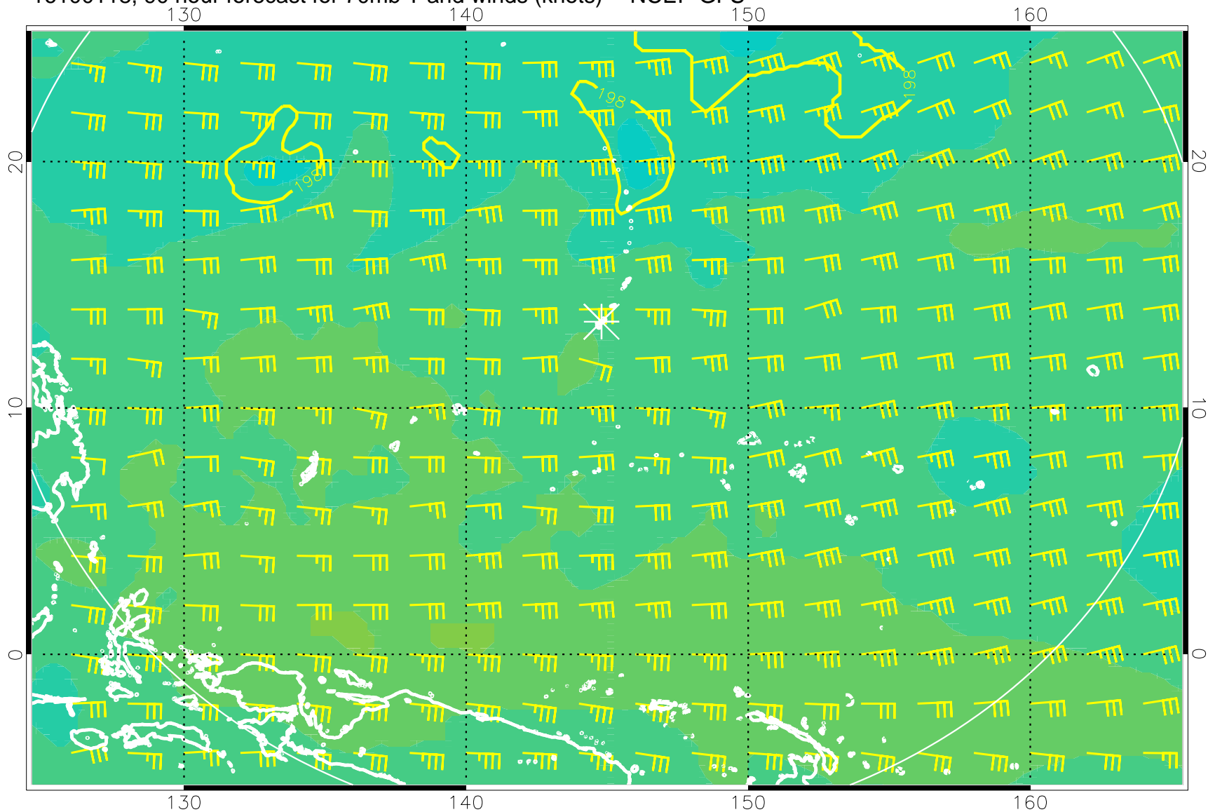
16100118, 90 hour forecast for 70mb T and winds (knots) -- NCEP GFS
