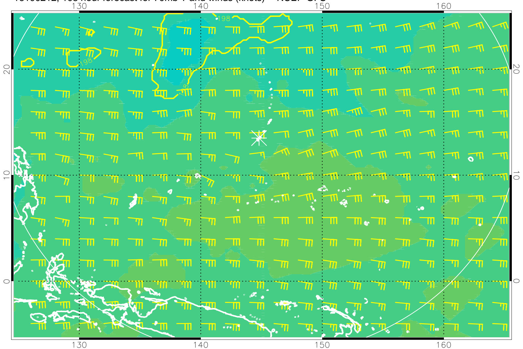
16100212, 108 hour forecast for 70mb T and winds (knots) -- NCEP GFS
