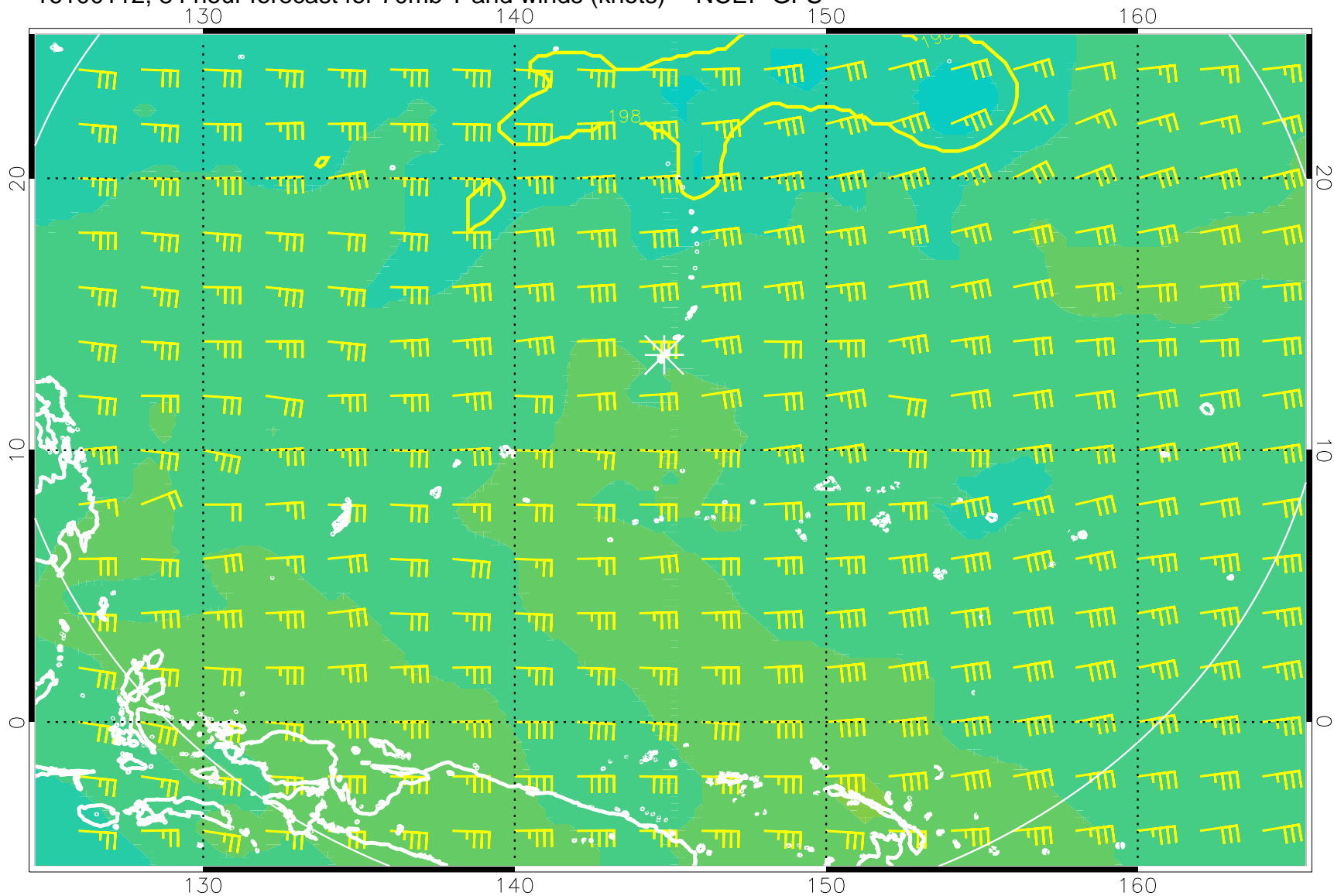
16100112, 84 hour forecast for 70mb T and winds (knots) -- NCEP GFS
