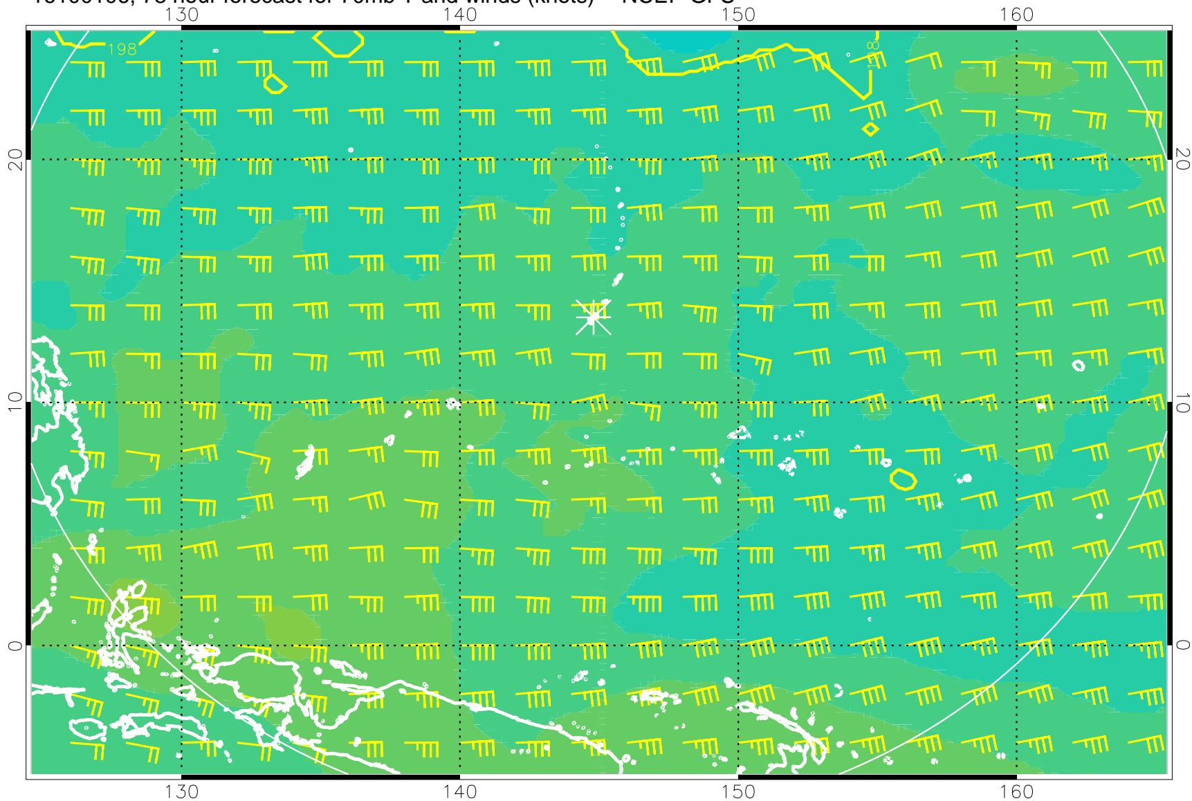
16100106, 78 hour forecast for 70mb T and winds (knots) -- NCEP GFS
