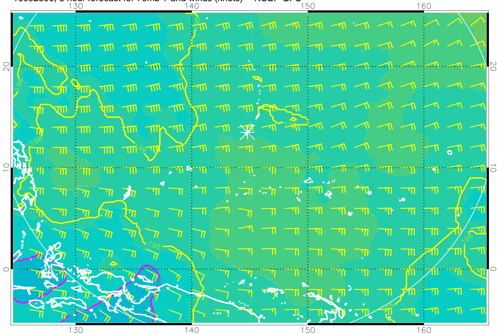
16092806, 6 hour forecast for 70mb T and winds (knots) -- NCEP GFS
