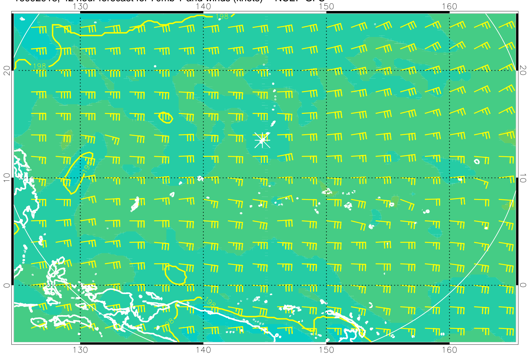
16092918, 42 hour forecast for 70mb T and winds (knots) -- NCEP GFS
