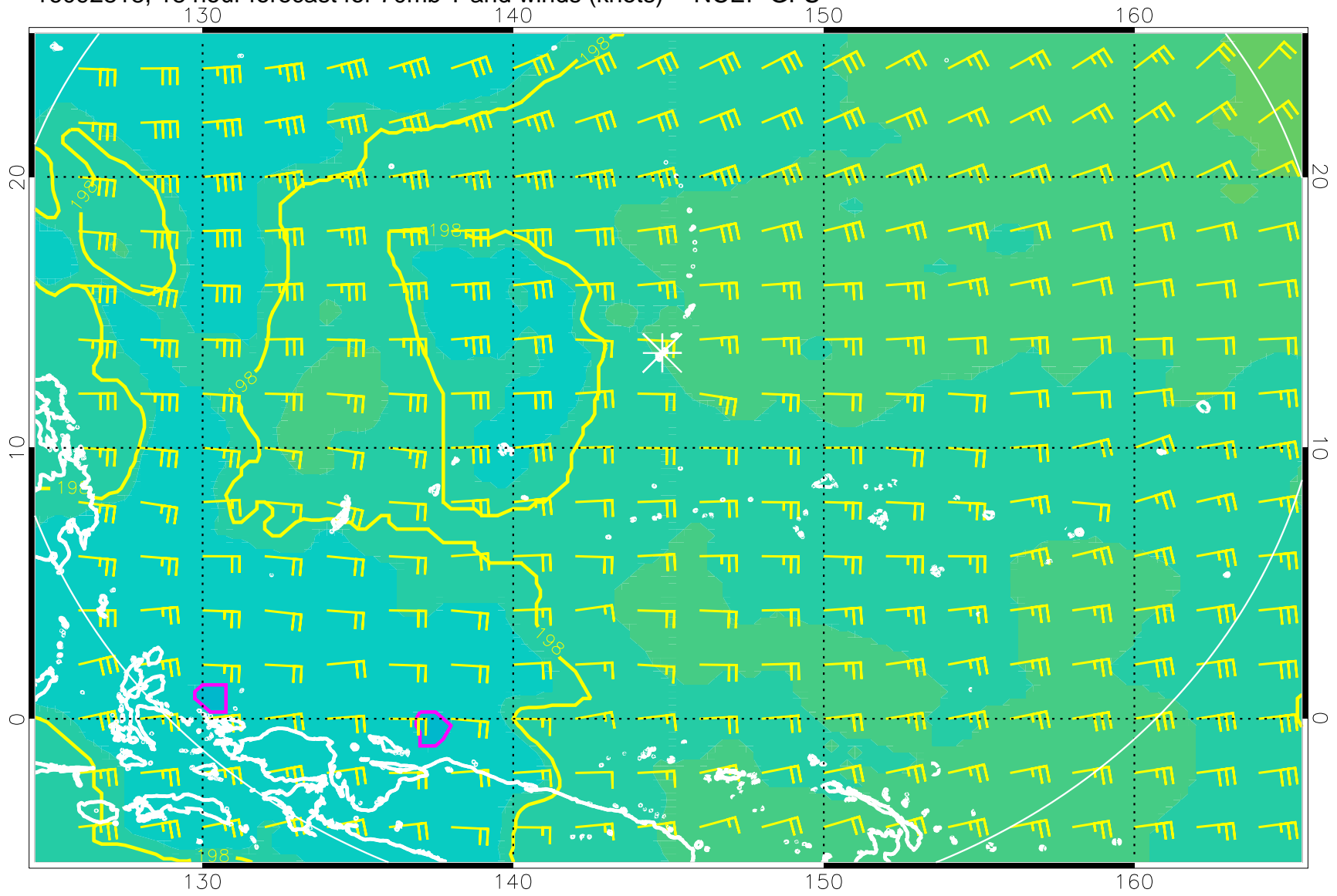
16092818, 18 hour forecast for 70mb T and winds (knots) -- NCEP GFS
