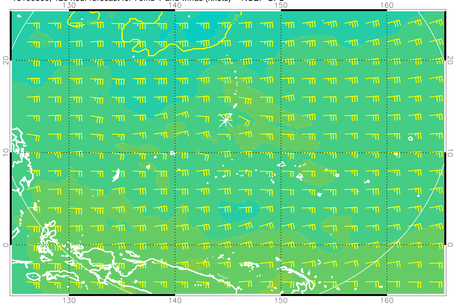
16100300, 120 hour forecast for 70mb T and winds (knots) -- NCEP GFS
