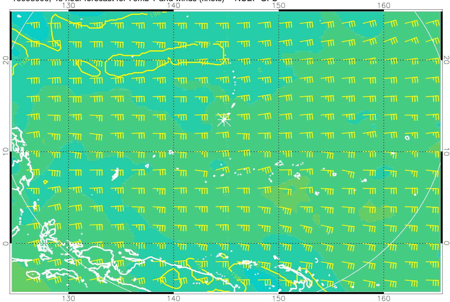
16093000, 48 hour forecast for 70mb T and winds (knots) -- NCEP GFS
