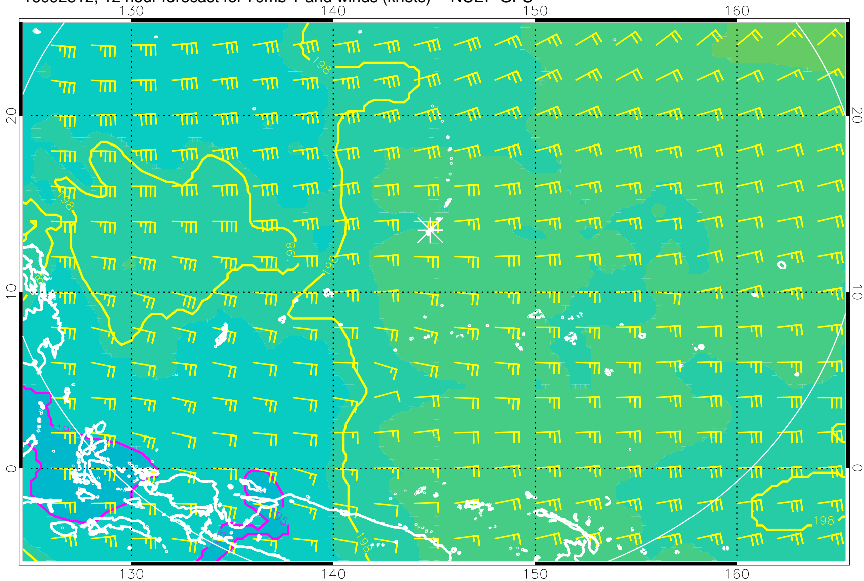
16092812, 12 hour forecast for 70mb T and winds (knots) -- NCEP GFS
