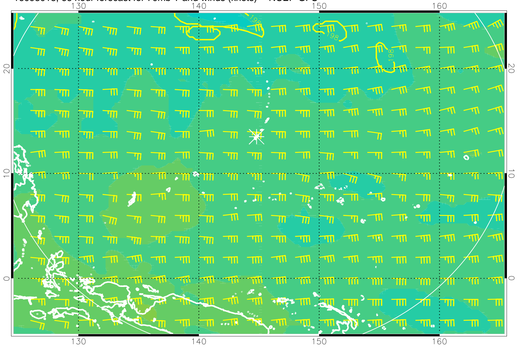
16093018, 66 hour forecast for 70mb T and winds (knots) -- NCEP GFS
