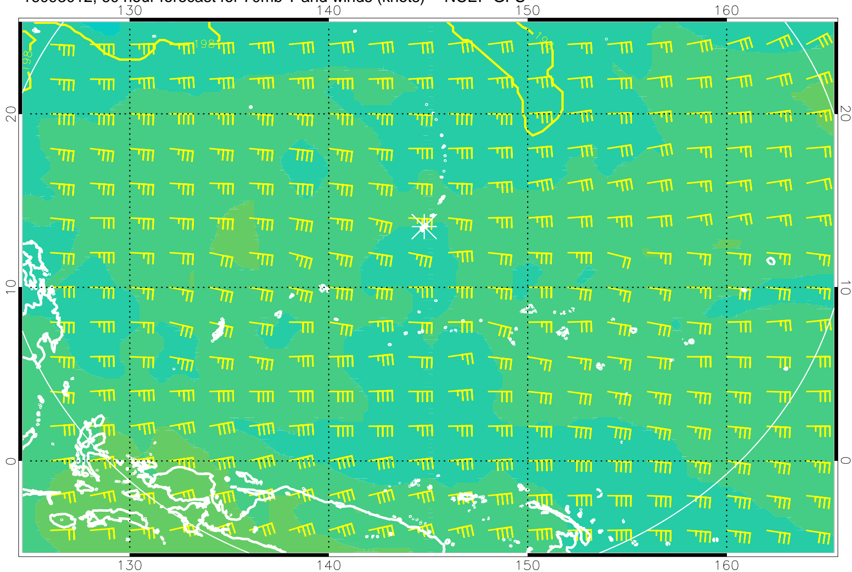
16093012, 60 hour forecast for 70mb T and winds (knots) -- NCEP GFS
