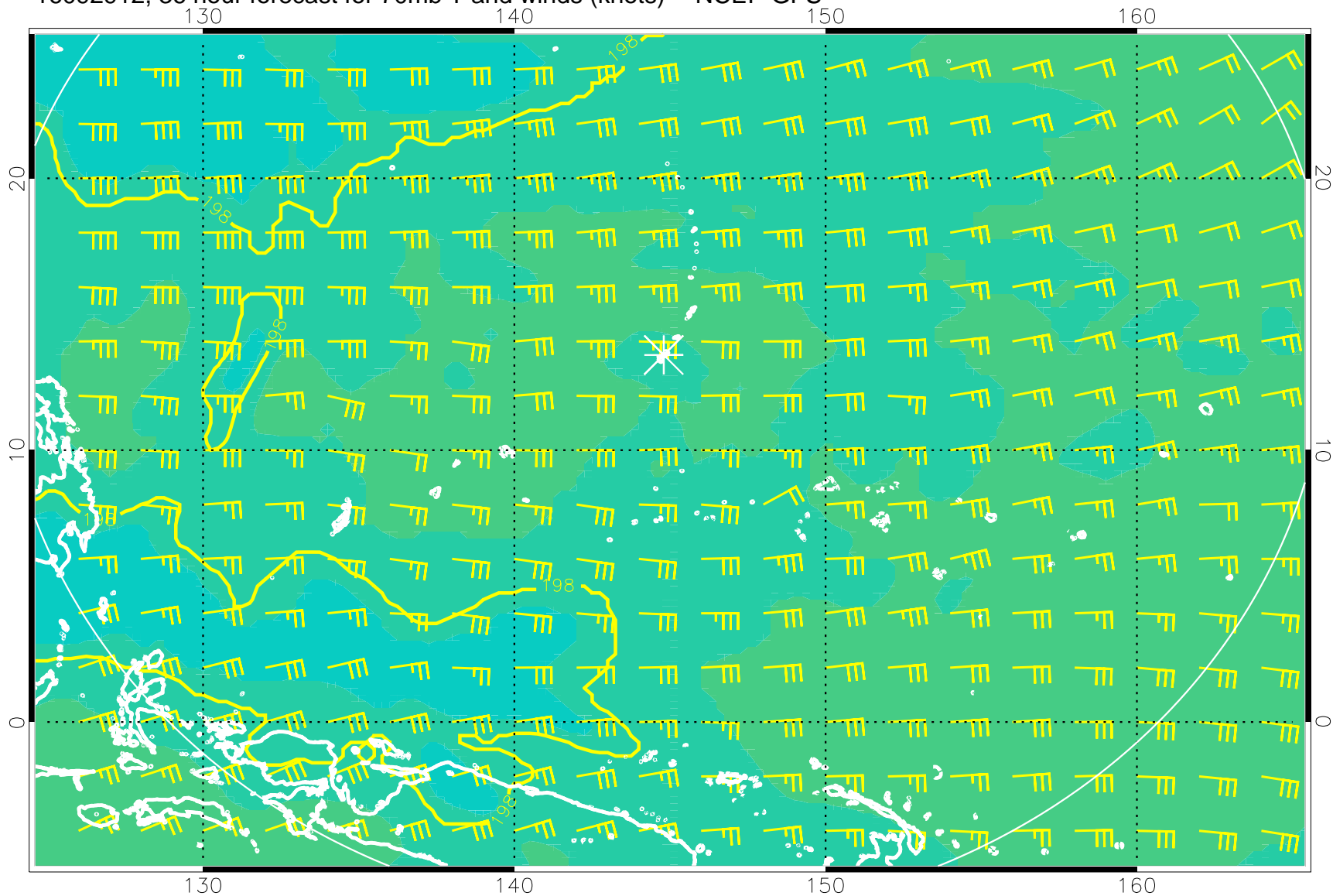
16092912, 36 hour forecast for 70mb T and winds (knots) -- NCEP GFS
