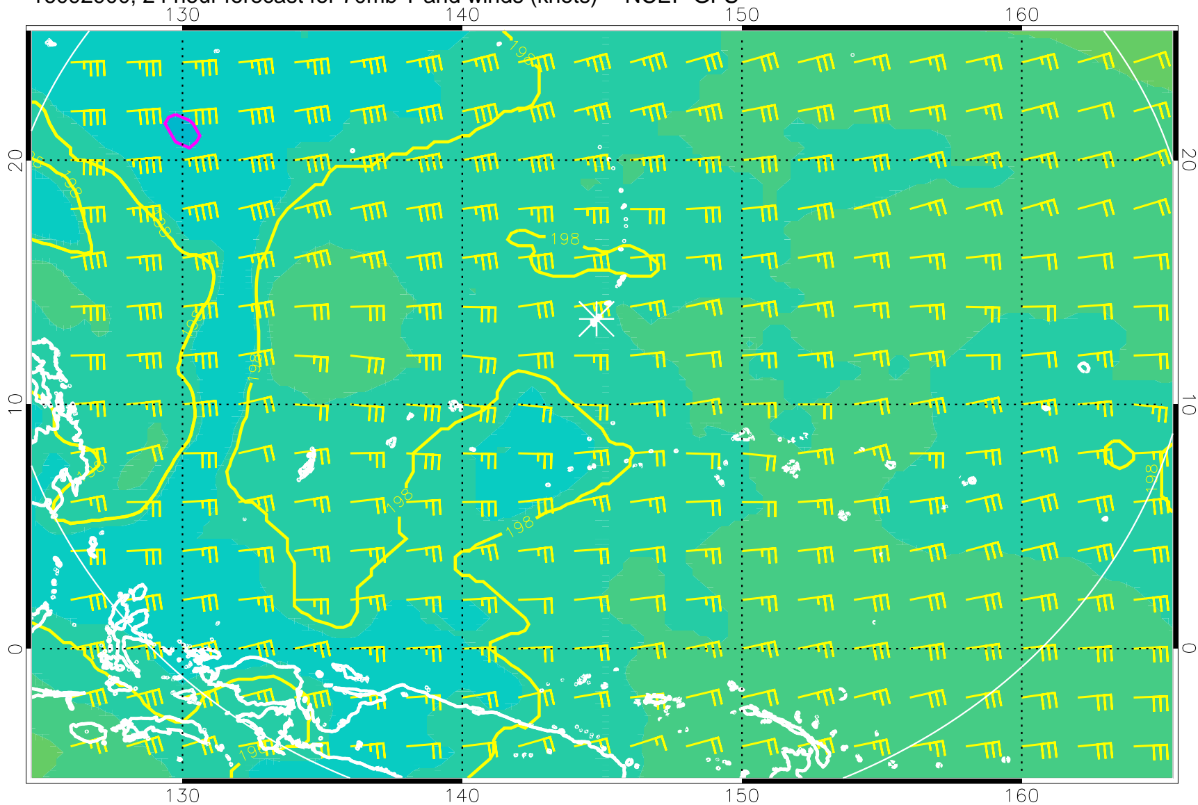
16092900, 24 hour forecast for 70mb T and winds (knots) -- NCEP GFS
