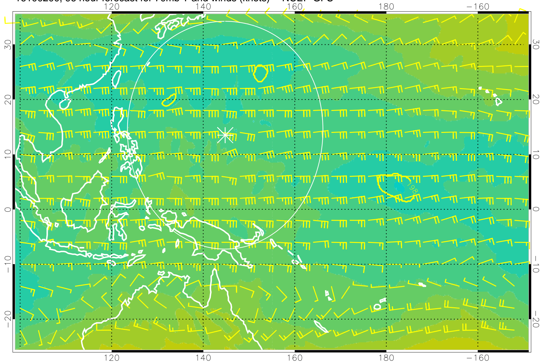
16100200, 96 hour forecast for 70mb T and winds (knots) -- NCEP GFS
