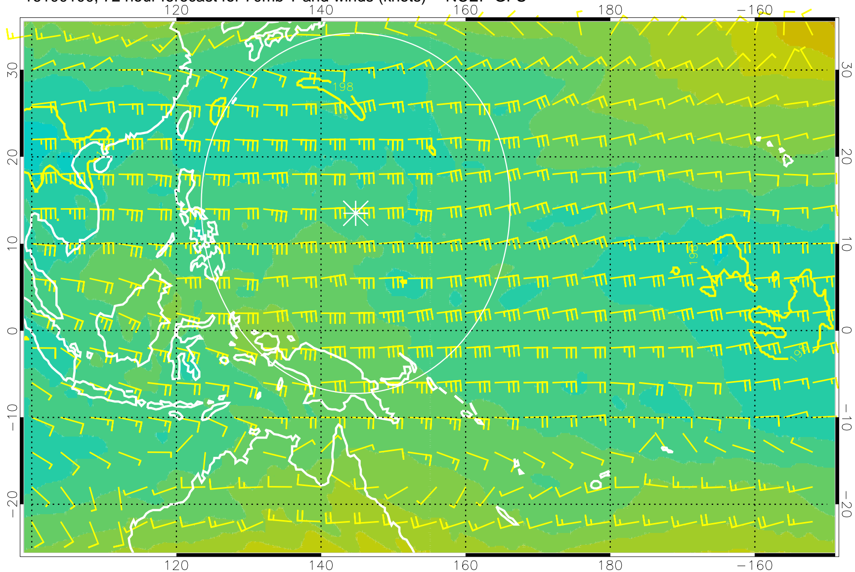
16100100, 72 hour forecast for 70mb T and winds (knots) -- NCEP GFS
