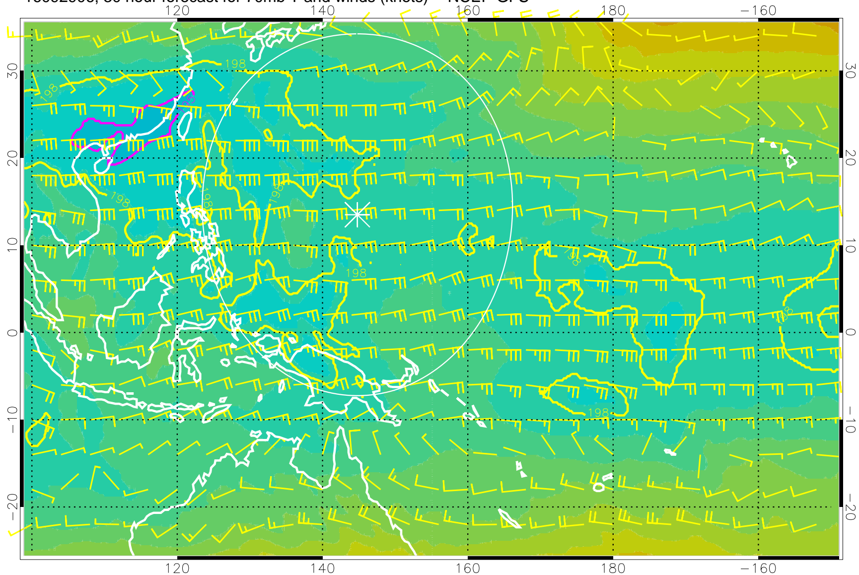
16092906, 30 hour forecast for 70mb T and winds (knots) -- NCEP GFS
