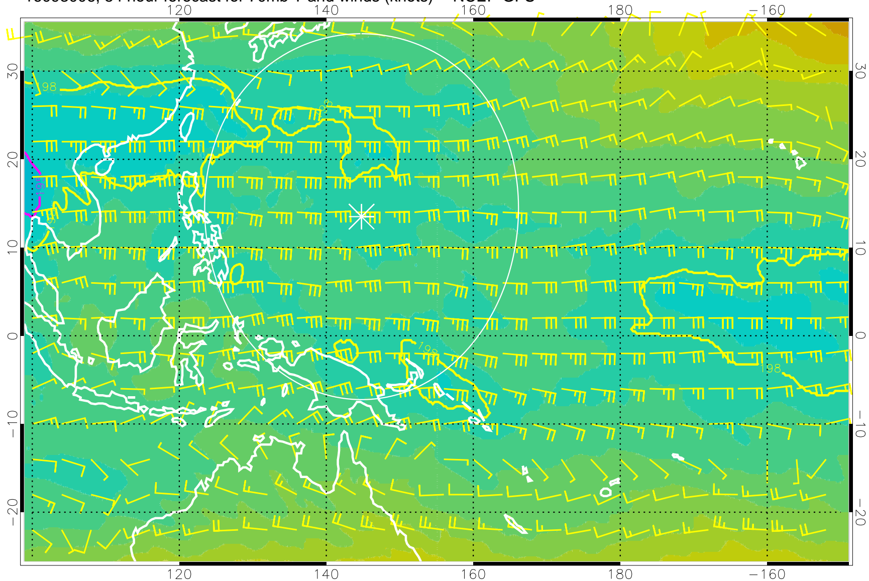
16093006, 54 hour forecast for 70mb T and winds (knots) -- NCEP GFS
