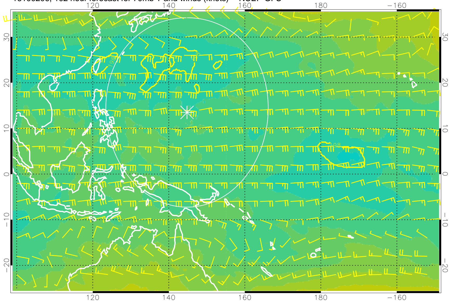
16100206, 102 hour forecast for 70mb T and winds (knots) -- NCEP GFS
