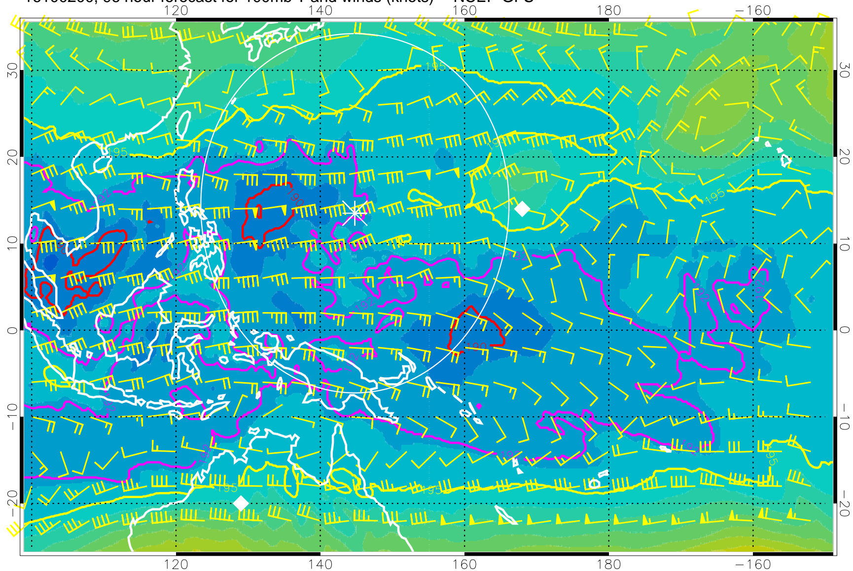
16100200, 96 hour forecast for 100mb T and winds (knots) -- NCEP GFS
