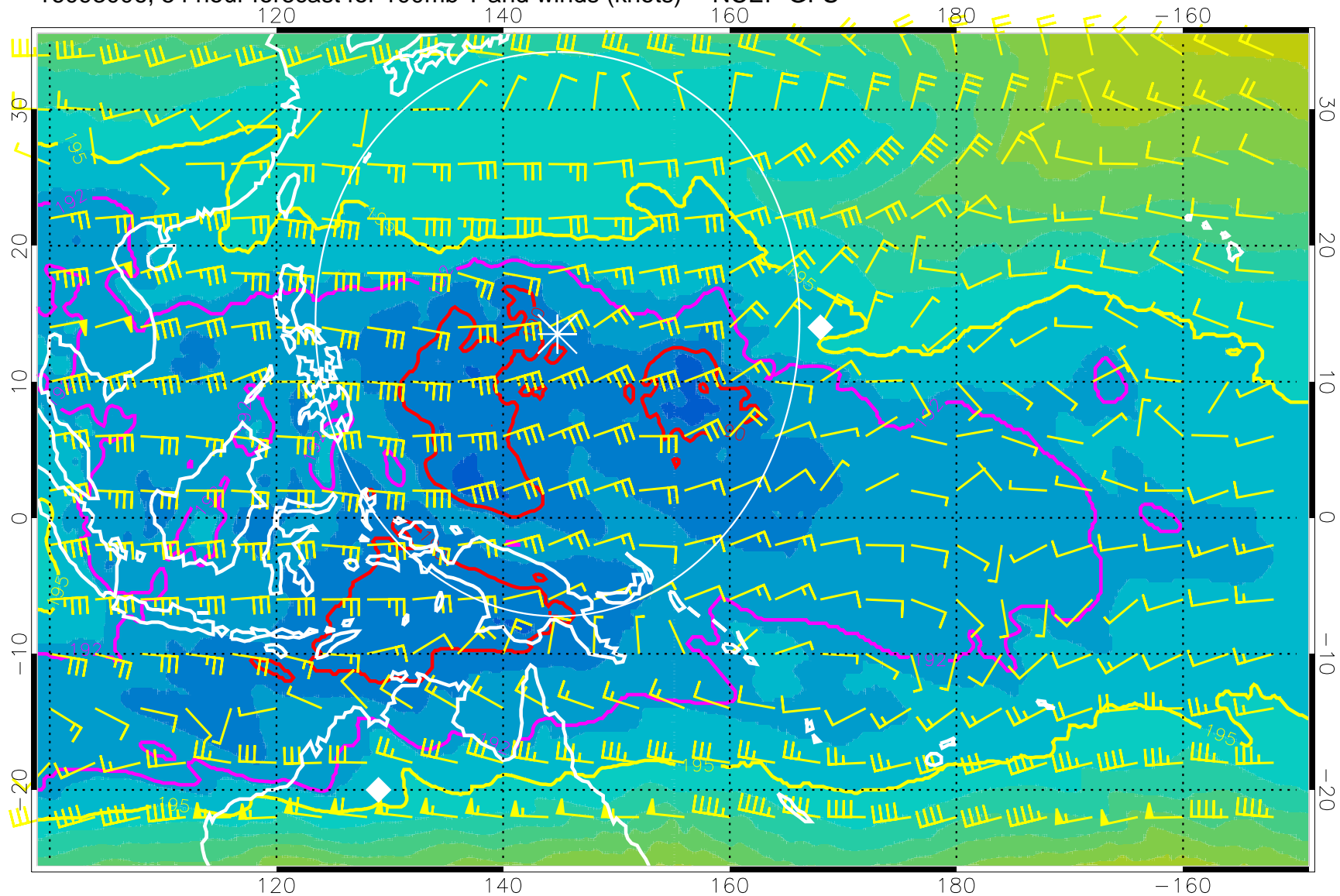
16093006, 54 hour forecast for 100mb T and winds (knots) -- NCEP GFS
