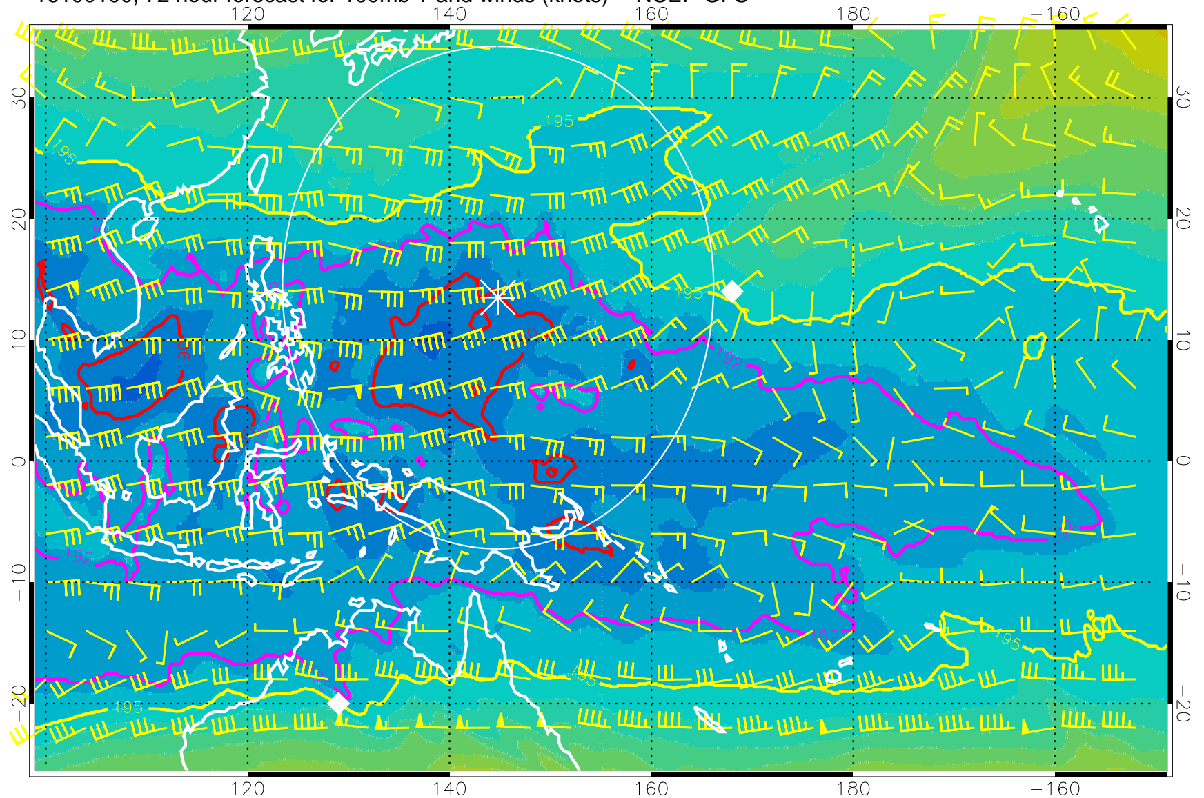
16100100, 72 hour forecast for 100mb T and winds (knots) -- NCEP GFS
