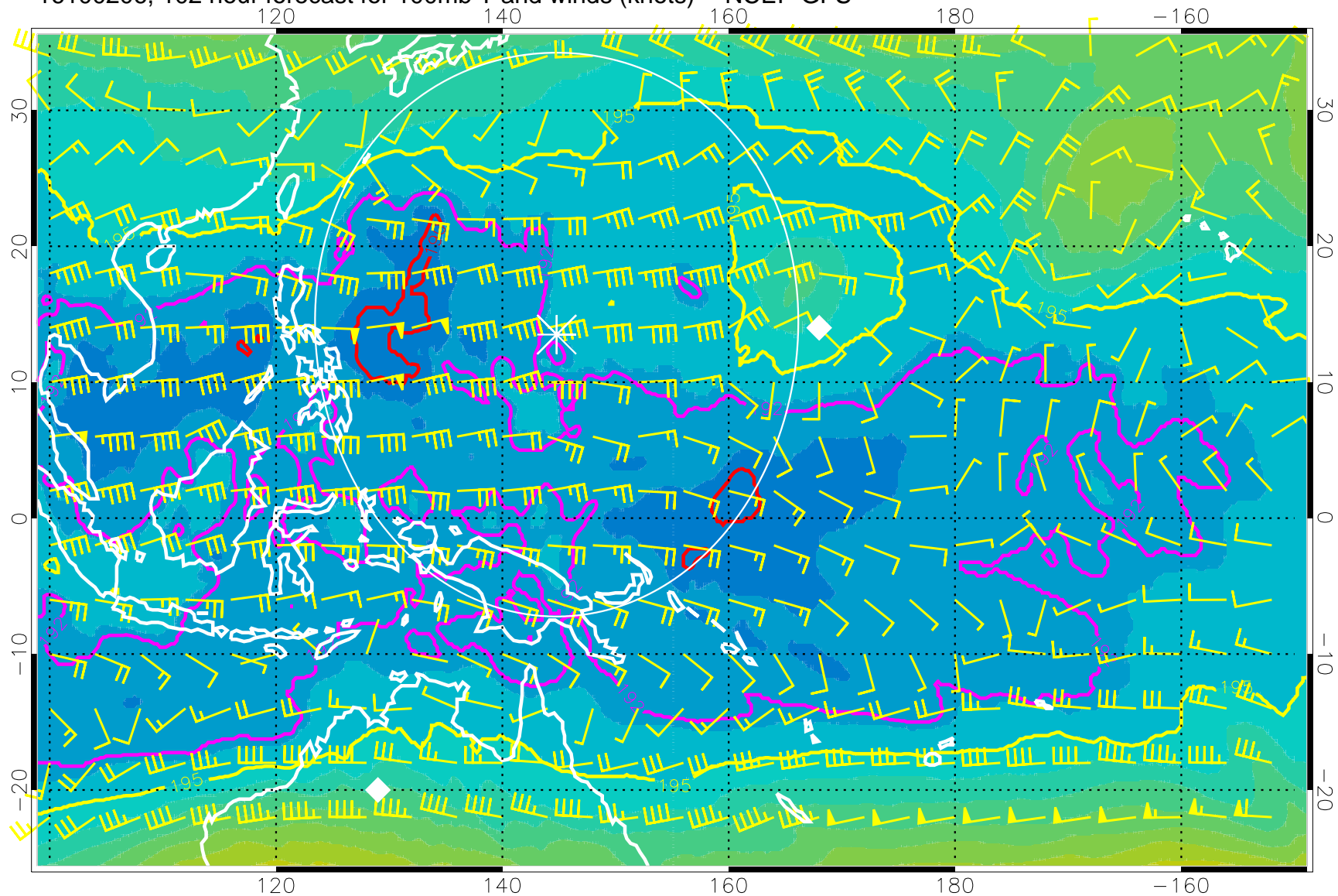
16100206, 102 hour forecast for 100mb T and winds (knots) -- NCEP GFS
