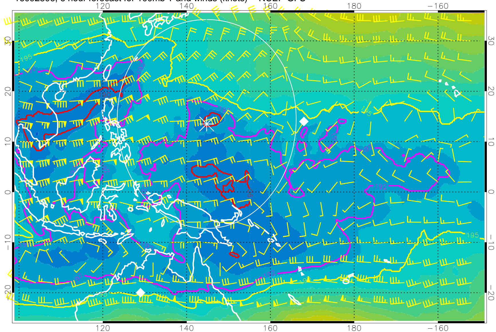
16092806, 6 hour forecast for 100mb T and winds (knots) -- NCEP GFS
