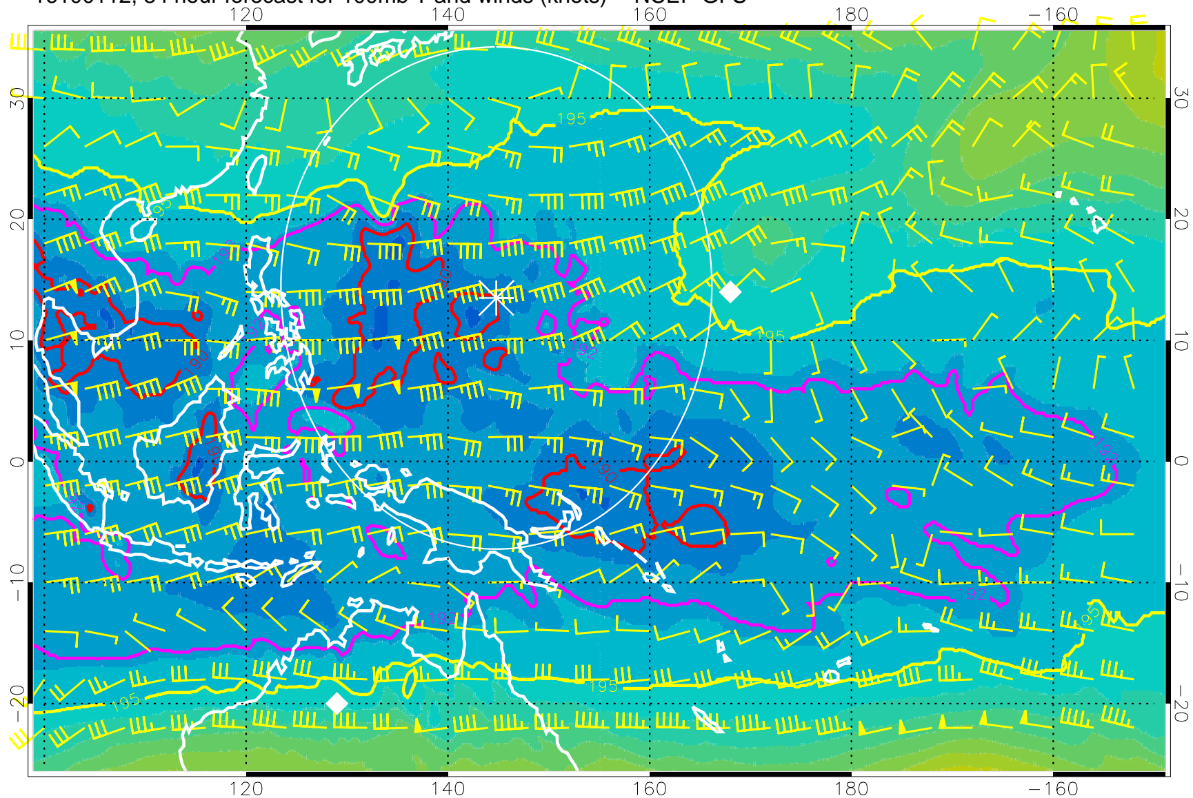
16100112, 84 hour forecast for 100mb T and winds (knots) -- NCEP GFS
