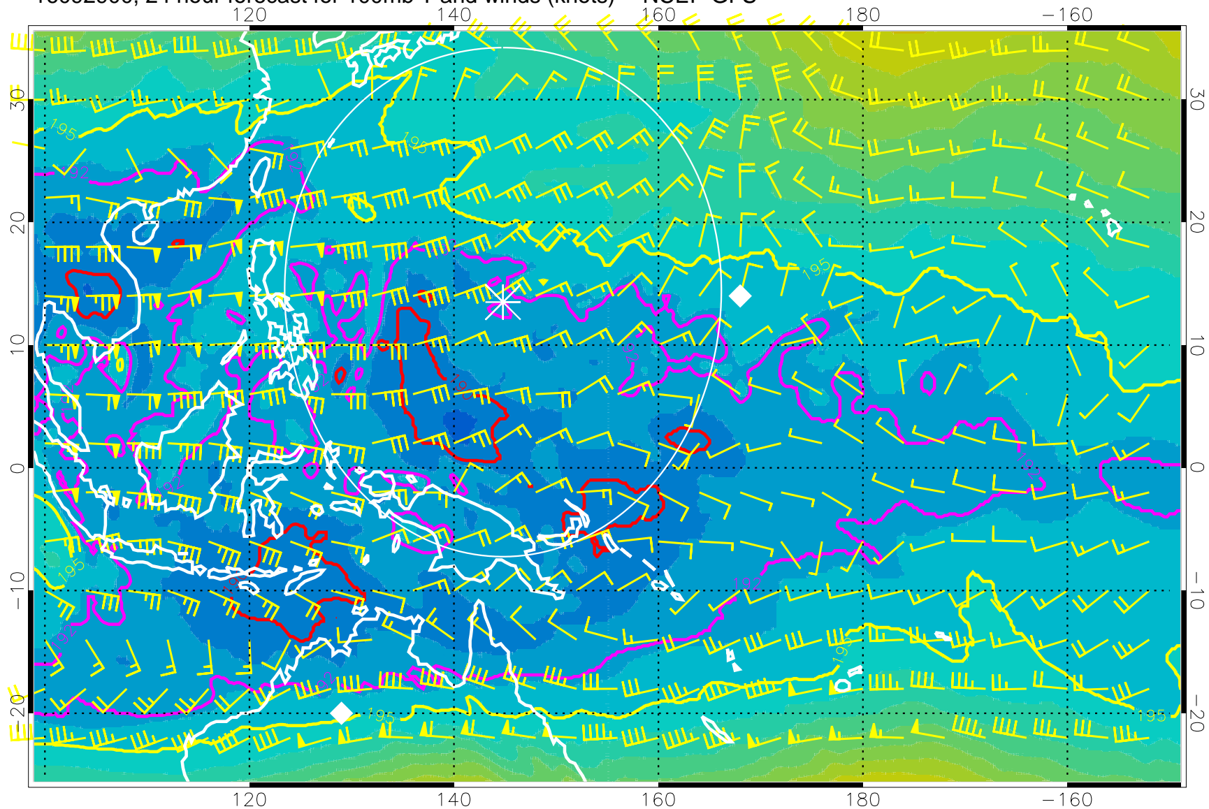
16092900, 24 hour forecast for 100mb T and winds (knots) -- NCEP GFS
