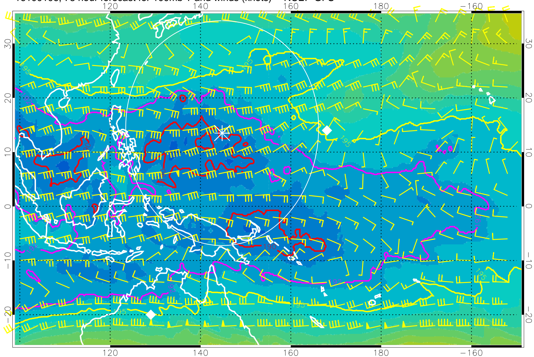
16100106, 78 hour forecast for 100mb T and winds (knots) -- NCEP GFS
