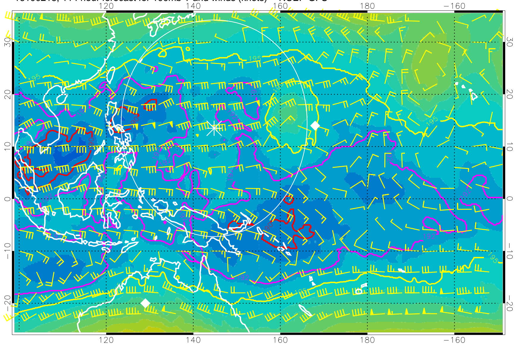
16100218, 114 hour forecast for 100mb T and winds (knots) -- NCEP GFS
