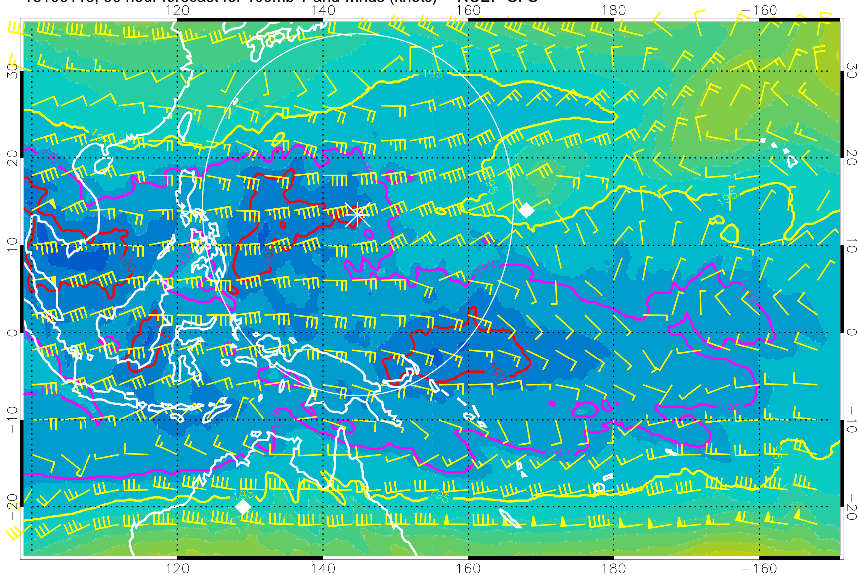
16100118, 90 hour forecast for 100mb T and winds (knots) -- NCEP GFS
