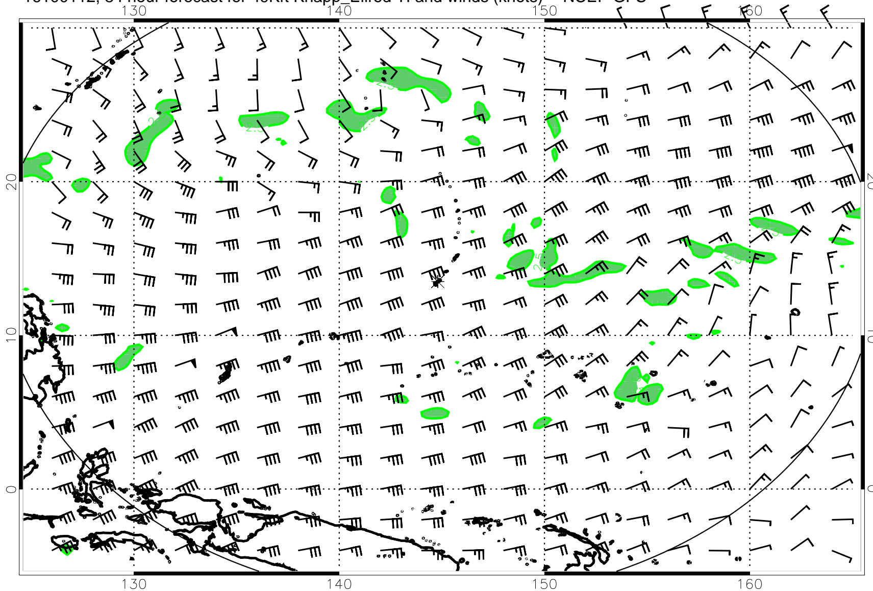
16100112, 84 hour forecast for 49Kft Knapp_Ellrod TI and winds (knots) -- NCEP GFS
