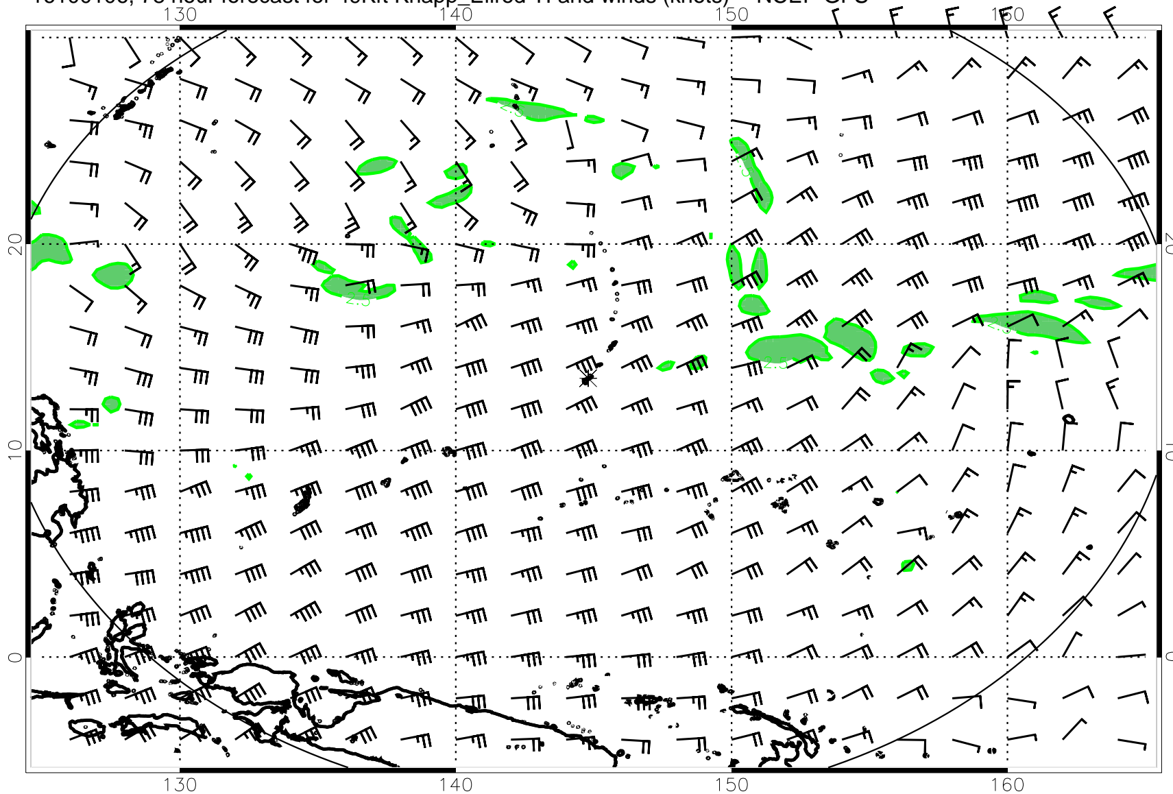
16100106, 78 hour forecast for 49Kft Knapp_Ellrod TI and winds (knots) -- NCEP GFS
