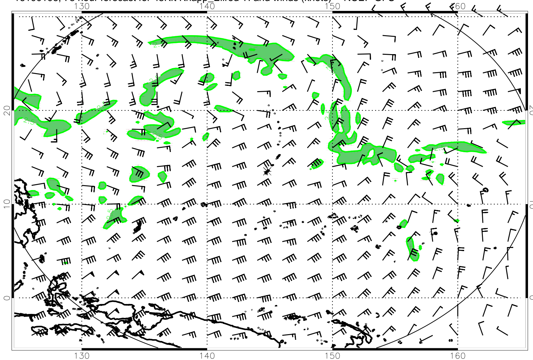
16100106, 78 hour forecast for 45Kft Knapp_Ellrod TI and winds (knots) -- NCEP GFS
