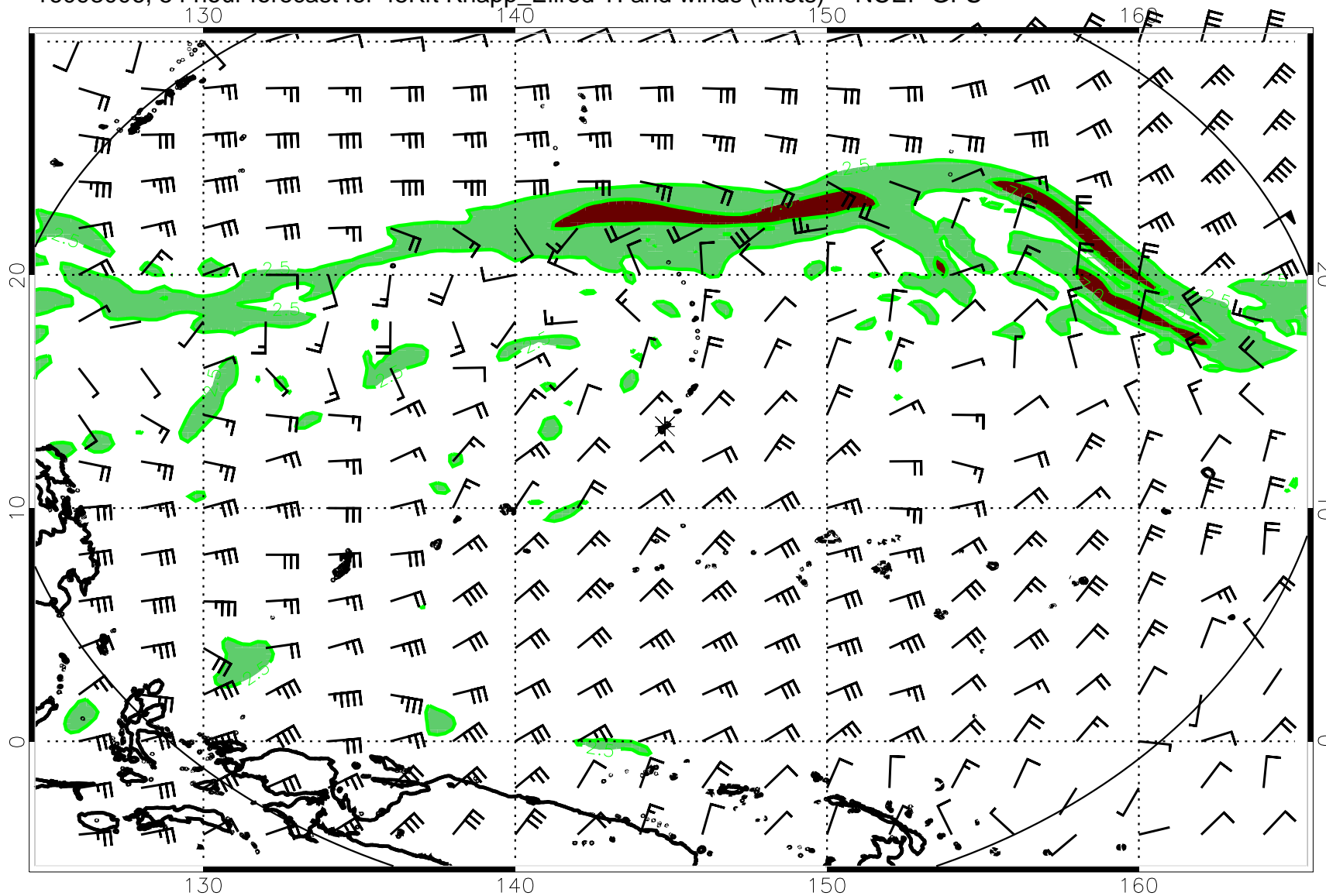
16093006, 54 hour forecast for 45Kft Knapp_Ellrod TI and winds (knots) -- NCEP GFS
