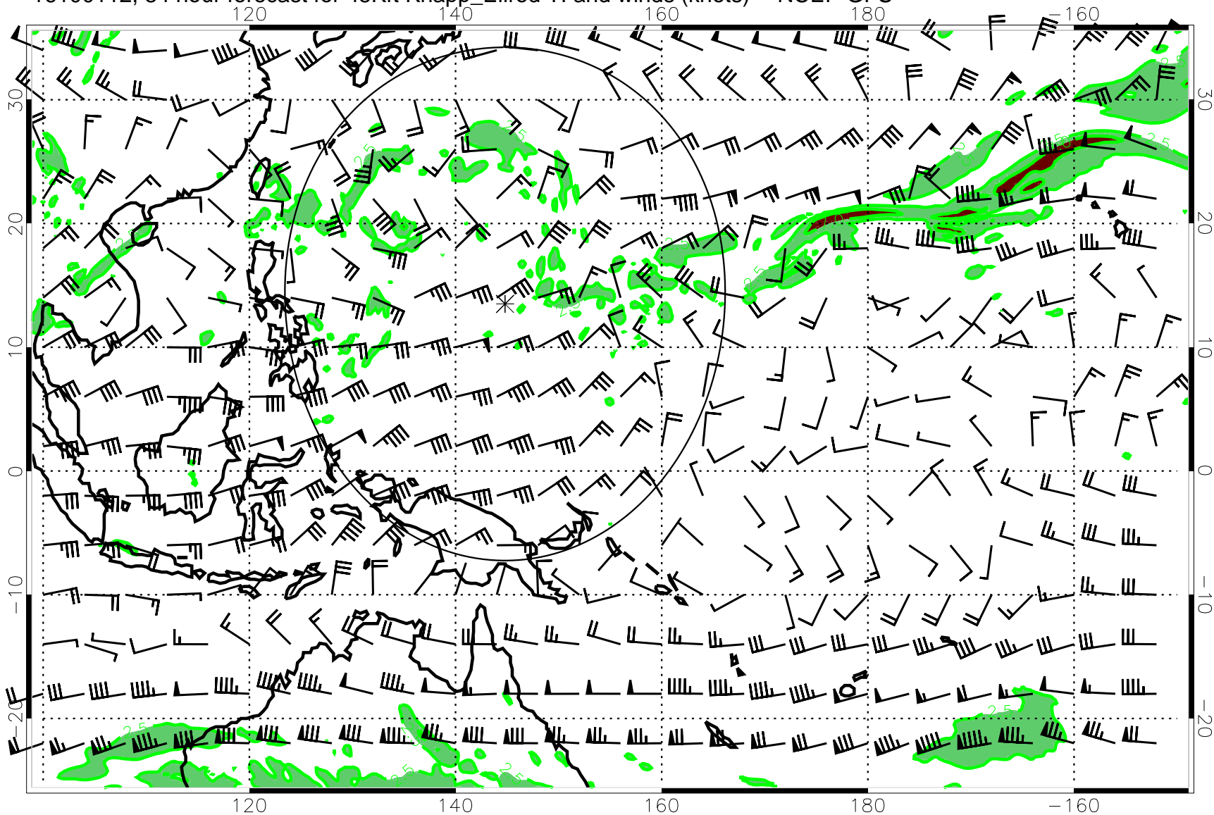
16100112, 84 hour forecast for 45Kft Knapp_Ellrod TI and winds (knots) -- NCEP GFS
