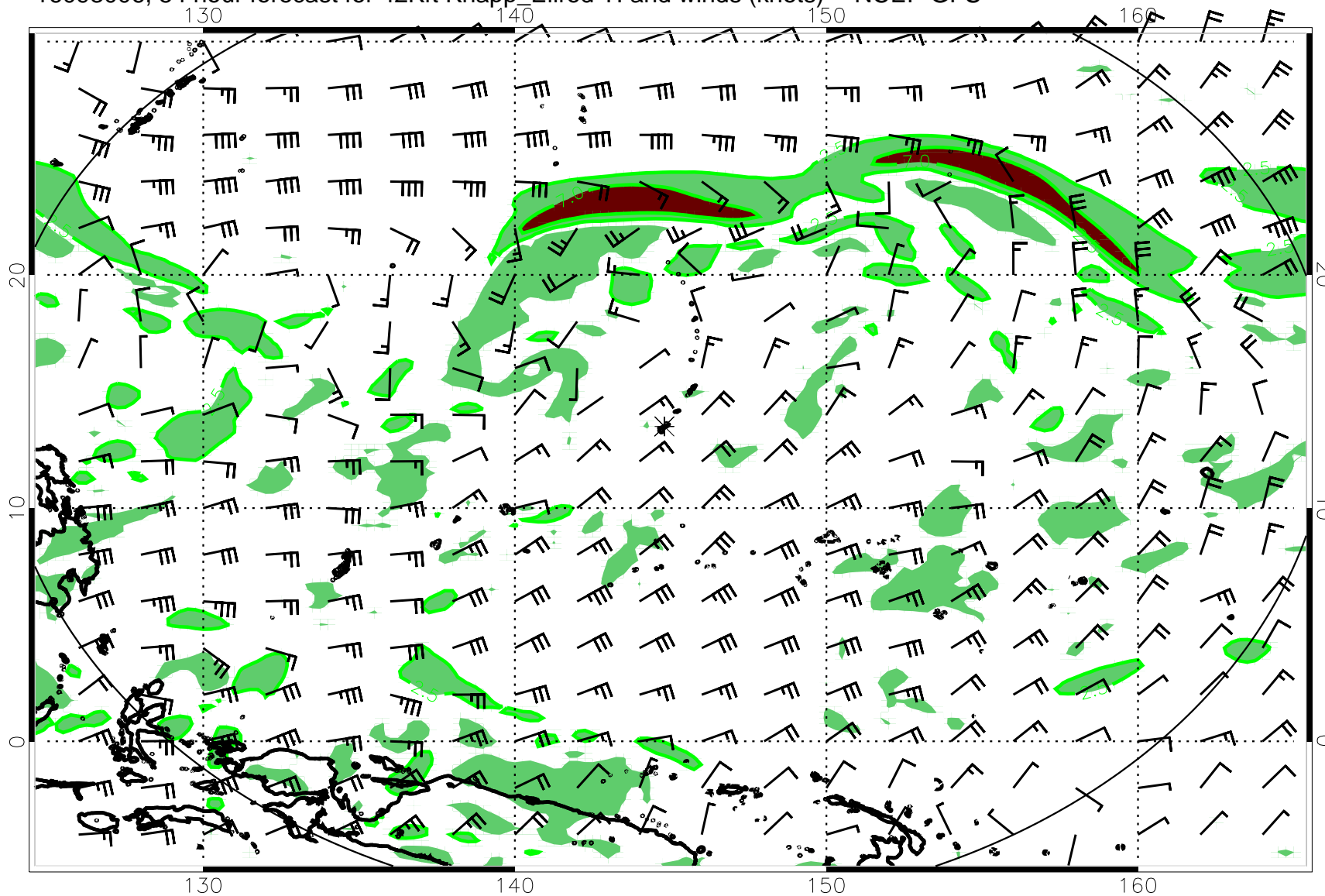
16093006, 54 hour forecast for 42Kft Knapp_Ellrod TI and winds (knots) -- NCEP GFS
