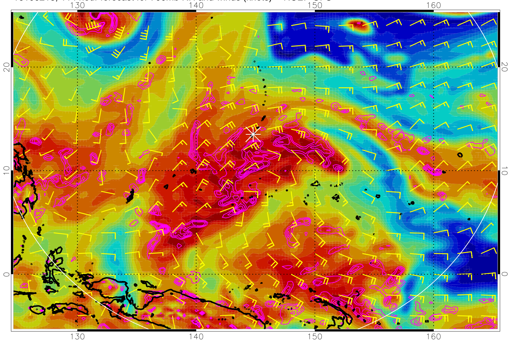
16100218, 114 hour forecast for 700mb RH and winds (knots) -- NCEP GFS
