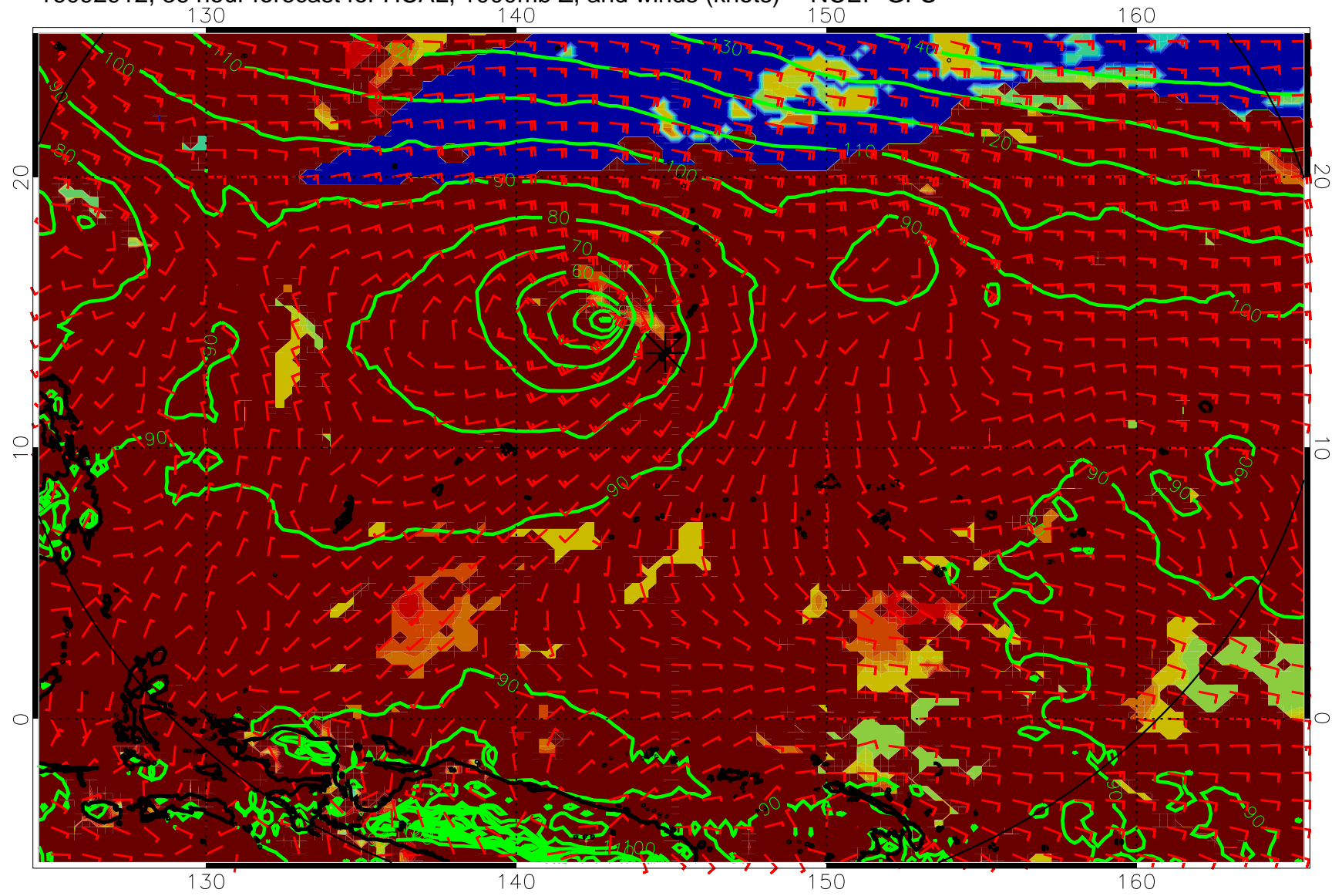
16092912, 36 hour forecast for HCAL, 1000mb Z, and winds (knots) -- NCEP GFS
