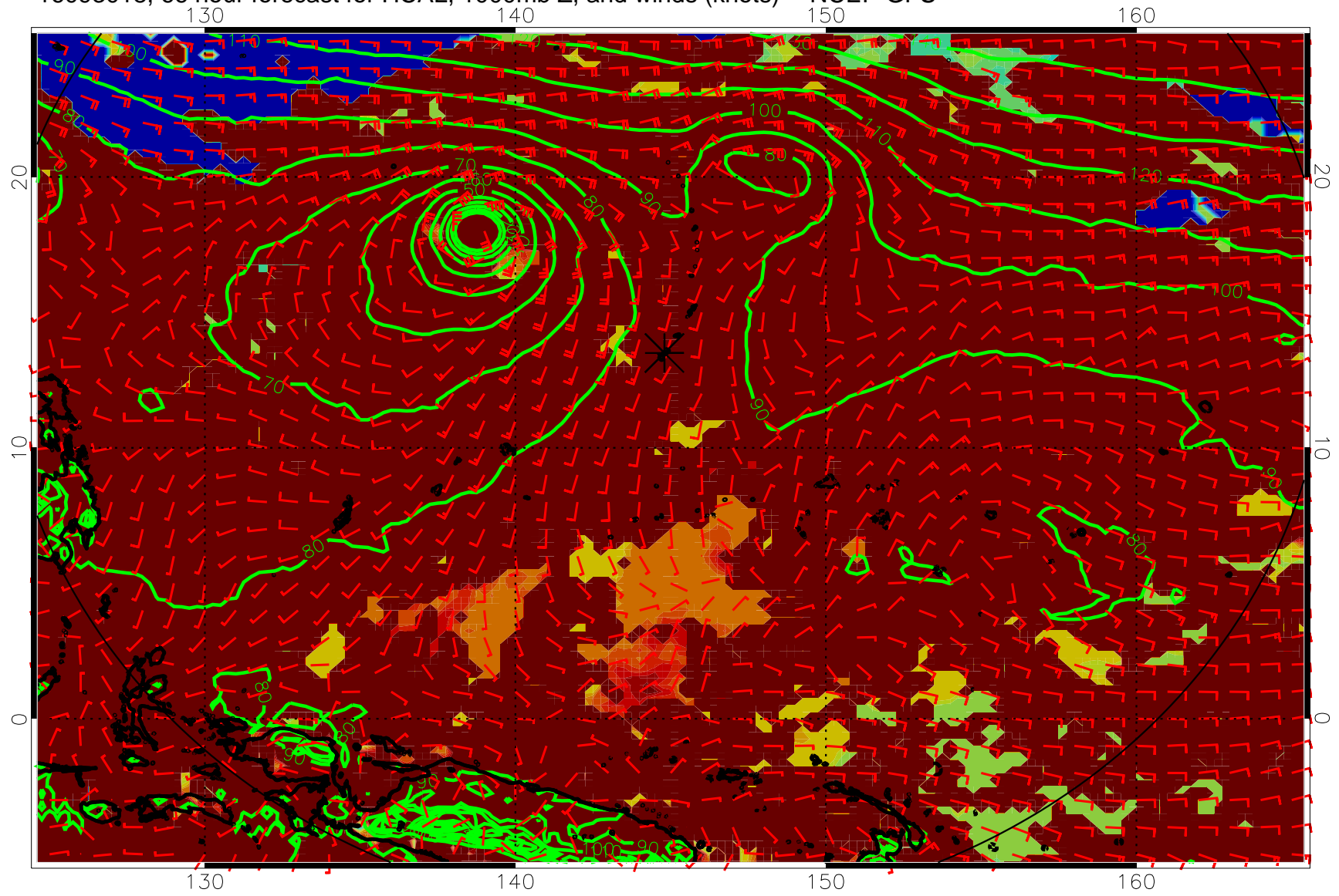
16093018, 66 hour forecast for HCAL, 1000mb Z, and winds (knots) -- NCEP GFS
