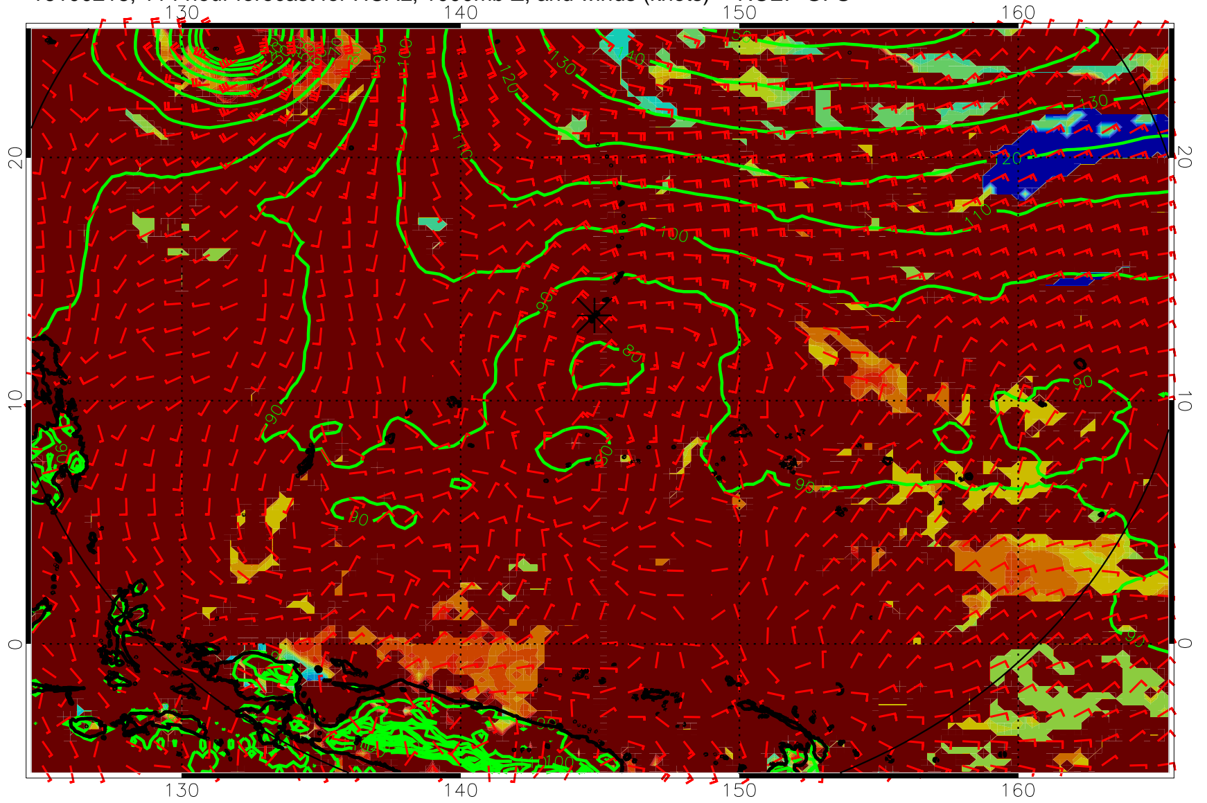
16100218, 114 hour forecast for HCAL, 1000mb Z, and winds (knots) -- NCEP GFS
