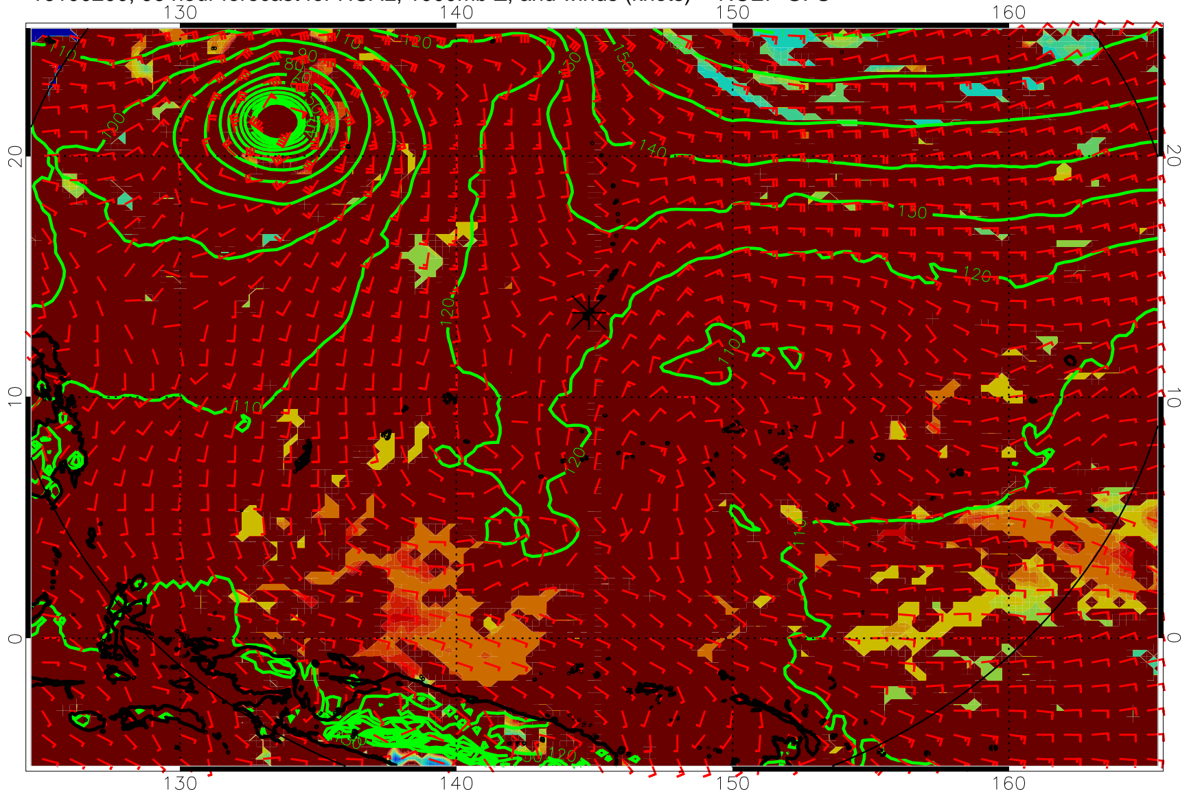
16100200, 96 hour forecast for HCAL, 1000mb Z, and winds (knots) -- NCEP GFS
