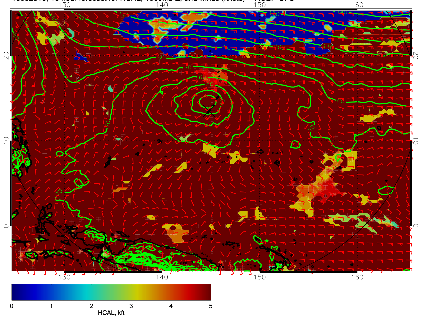
16092818, 18 hour forecast for HCAL, 1000mb Z, and winds (knots) -- NCEP GFS
