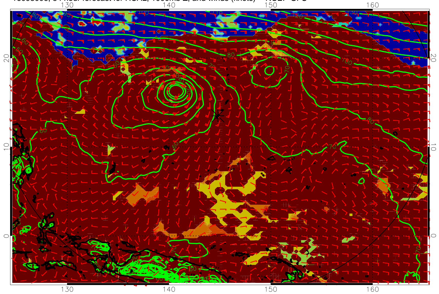
16093006, 54 hour forecast for HCAL, 1000mb Z, and winds (knots) -- NCEP GFS
