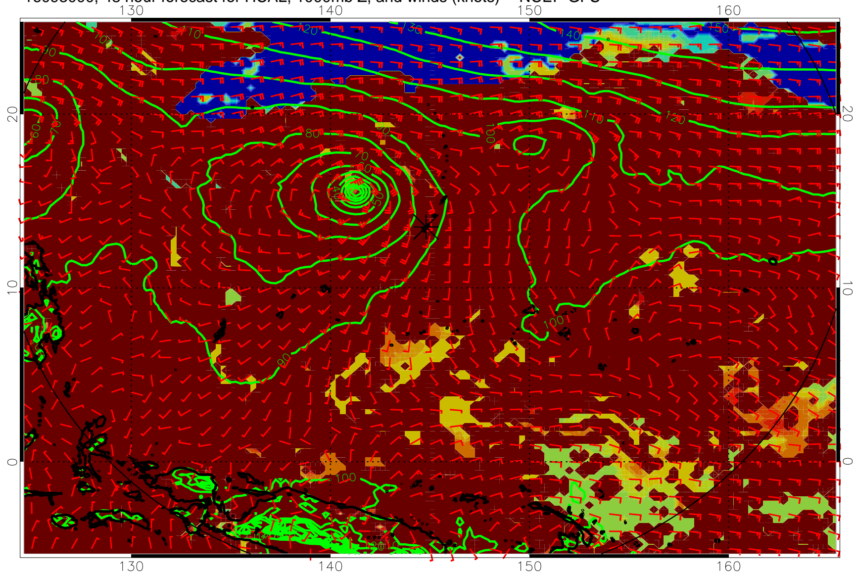
16093000, 48 hour forecast for HCAL, 1000mb Z, and winds (knots) -- NCEP GFS
