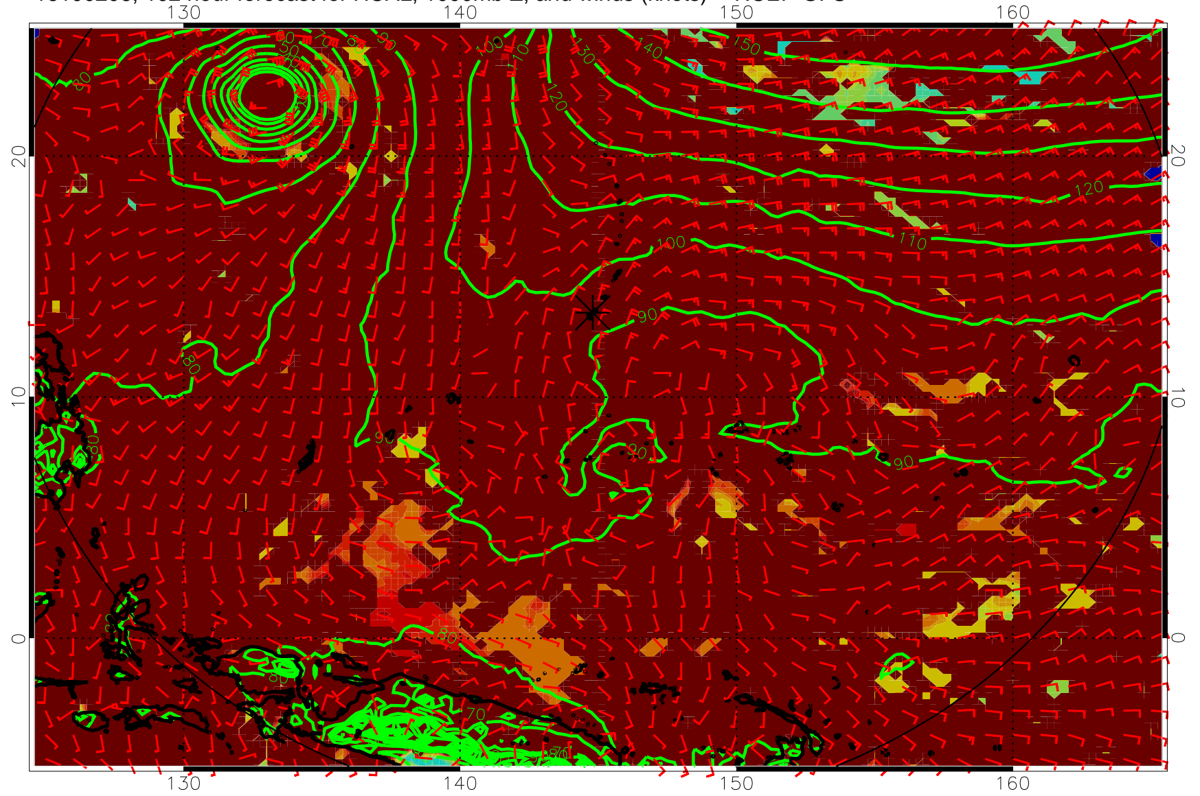
16100206, 102 hour forecast for HCAL, 1000mb Z, and winds (knots) -- NCEP GFS
