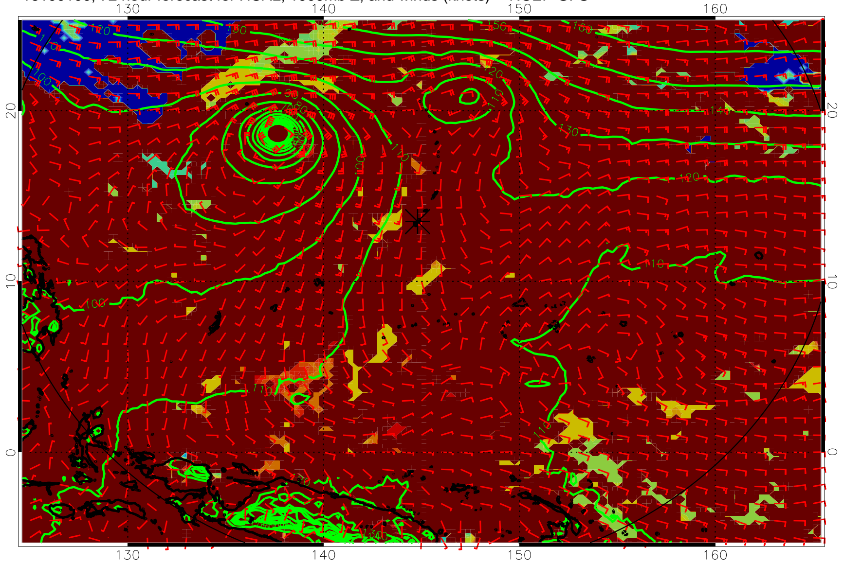
16100100, 72 hour forecast for HCAL, 1000mb Z, and winds (knots) -- NCEP GFS
