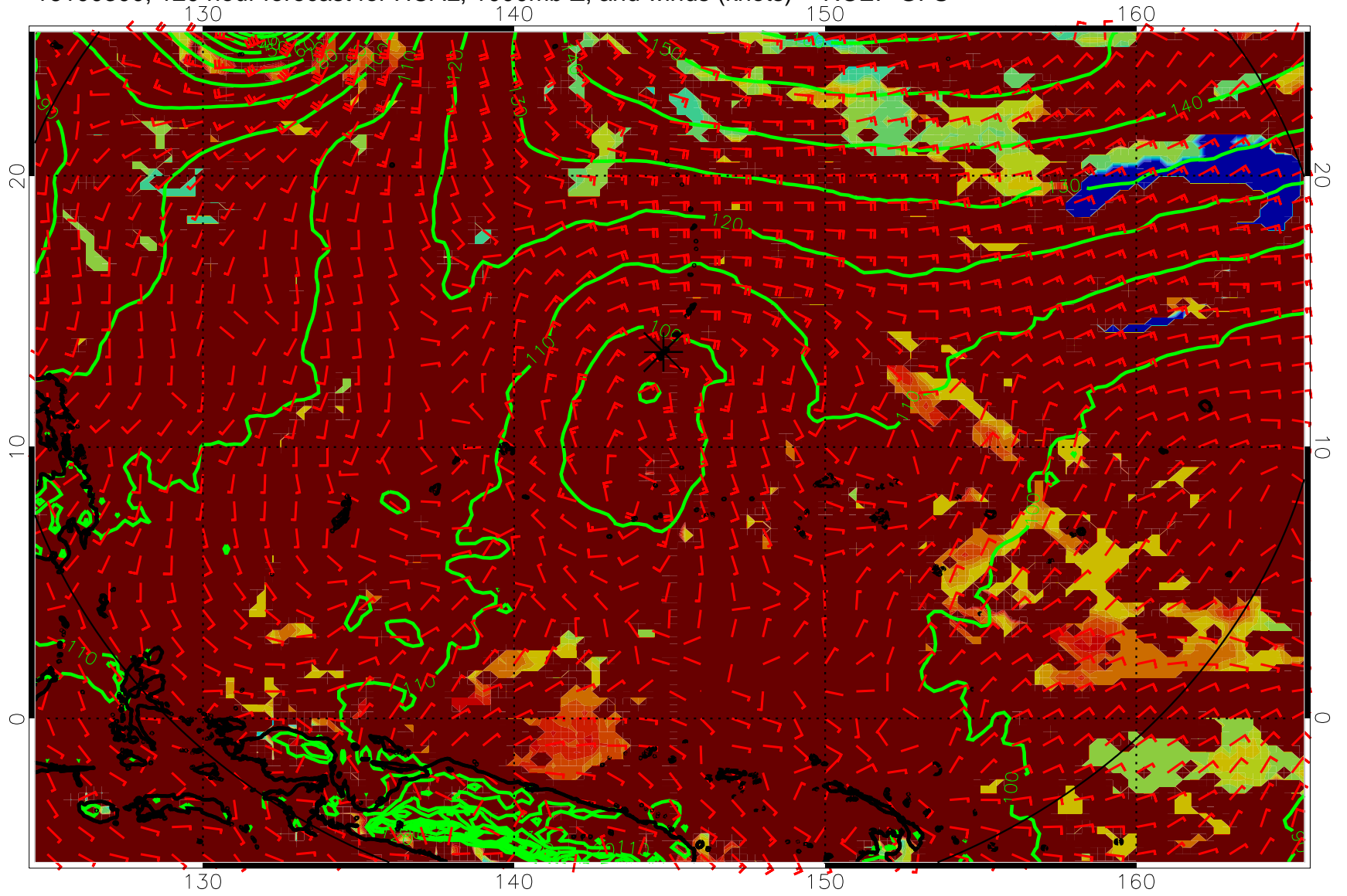
16100300, 120 hour forecast for HCAL, 1000mb Z, and winds (knots) -- NCEP GFS
