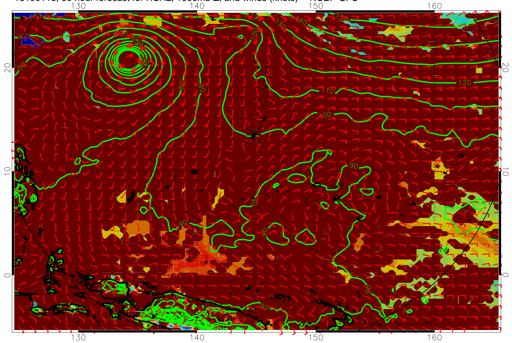
16100118, 90 hour forecast for HCAL, 1000mb Z, and winds (knots) -- NCEP GFS
