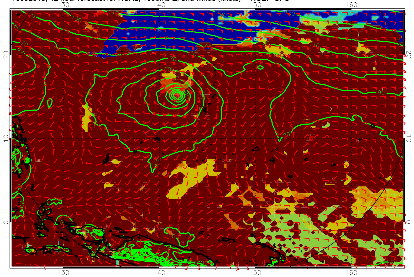
16092918, 42 hour forecast for HCAL, 1000mb Z, and winds (knots) -- NCEP GFS
