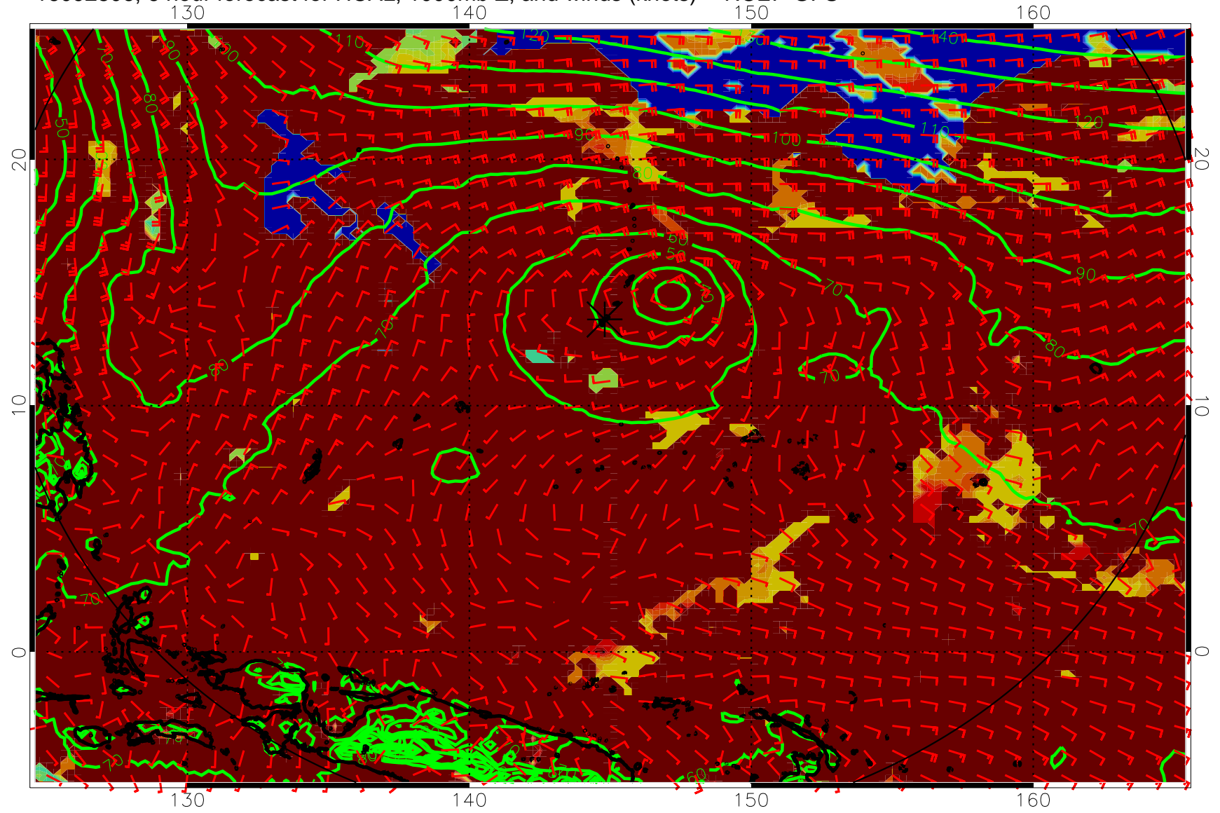
16092806, 6 hour forecast for HCAL, 1000mb Z, and winds (knots) -- NCEP GFS
