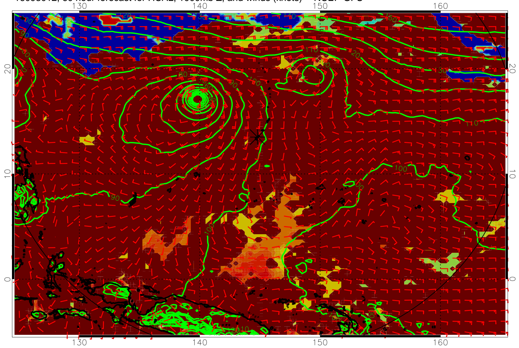
16093012, 60 hour forecast for HCAL, 1000mb Z, and winds (knots) -- NCEP GFS
