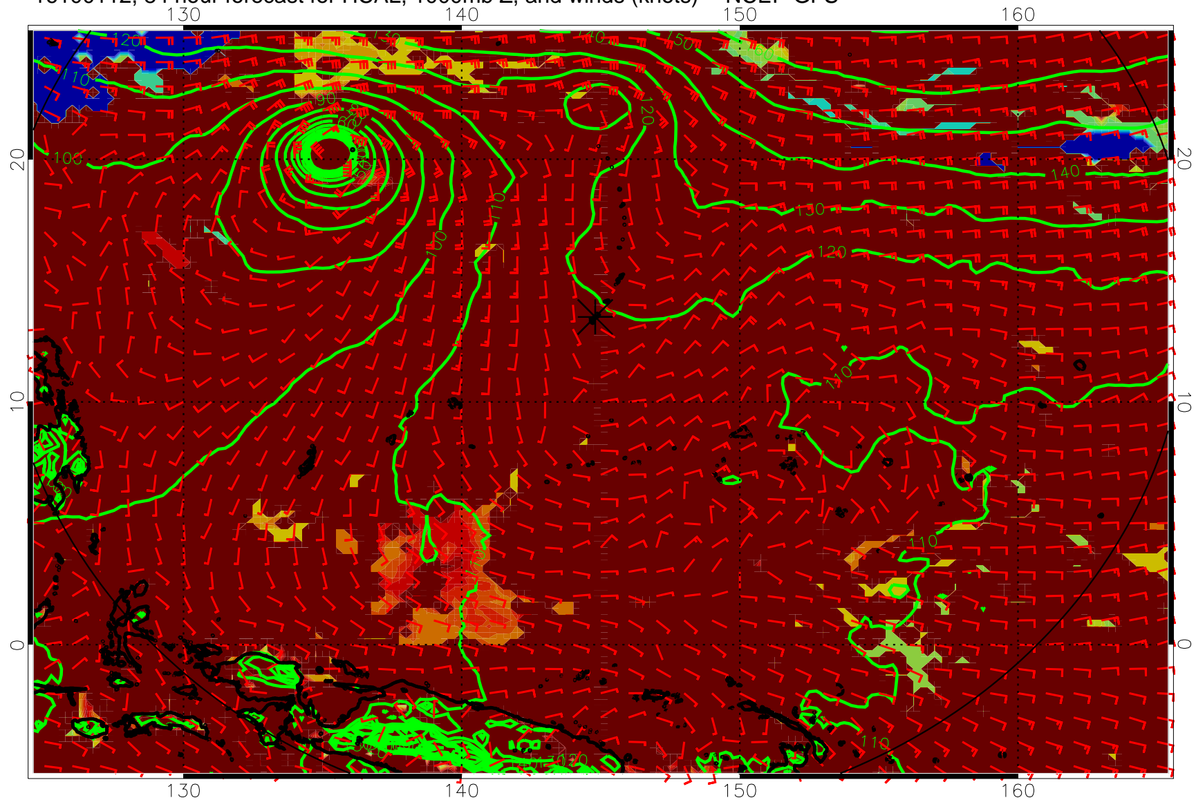
16100112, 84 hour forecast for HCAL, 1000mb Z, and winds (knots) -- NCEP GFS
