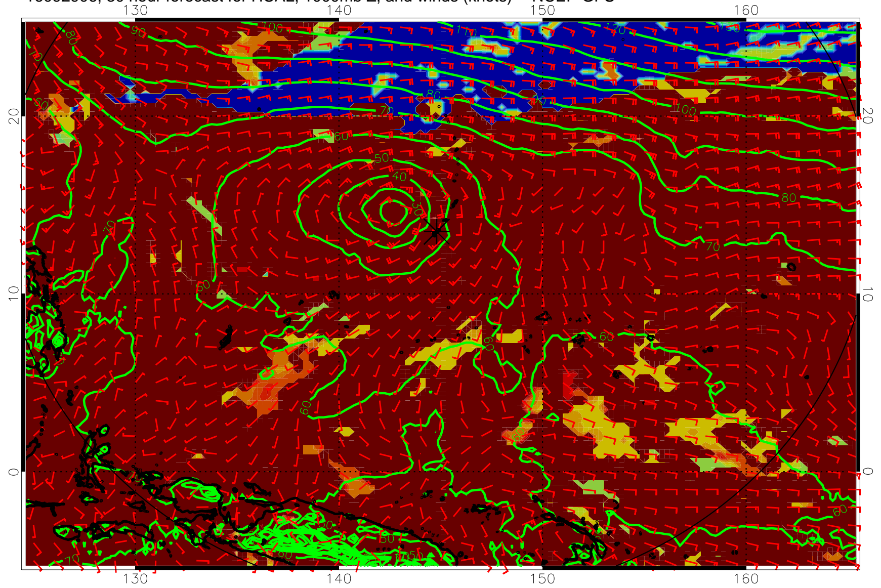
16092906, 30 hour forecast for HCAL, 1000mb Z, and winds (knots) -- NCEP GFS
