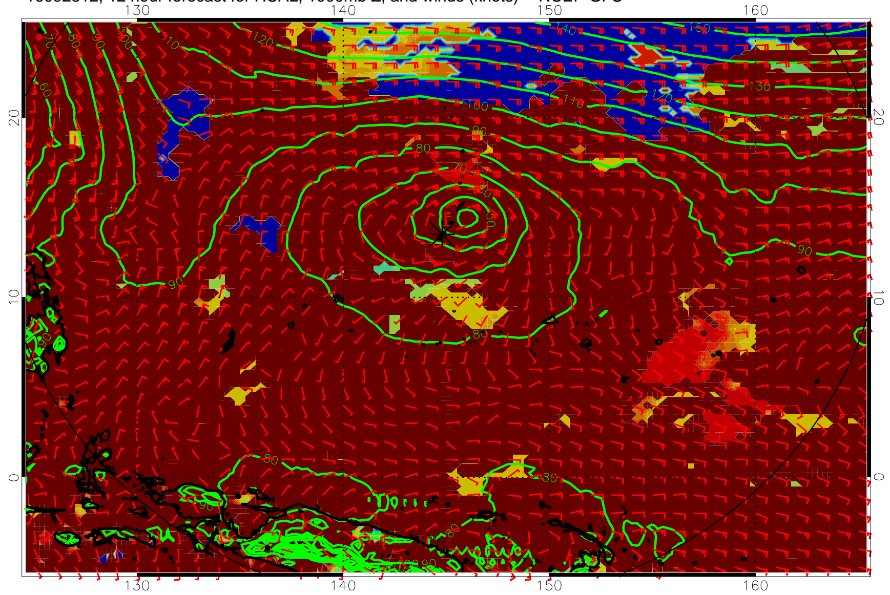
16092812, 12 hour forecast for HCAL, 1000mb Z, and winds (knots) -- NCEP GFS
