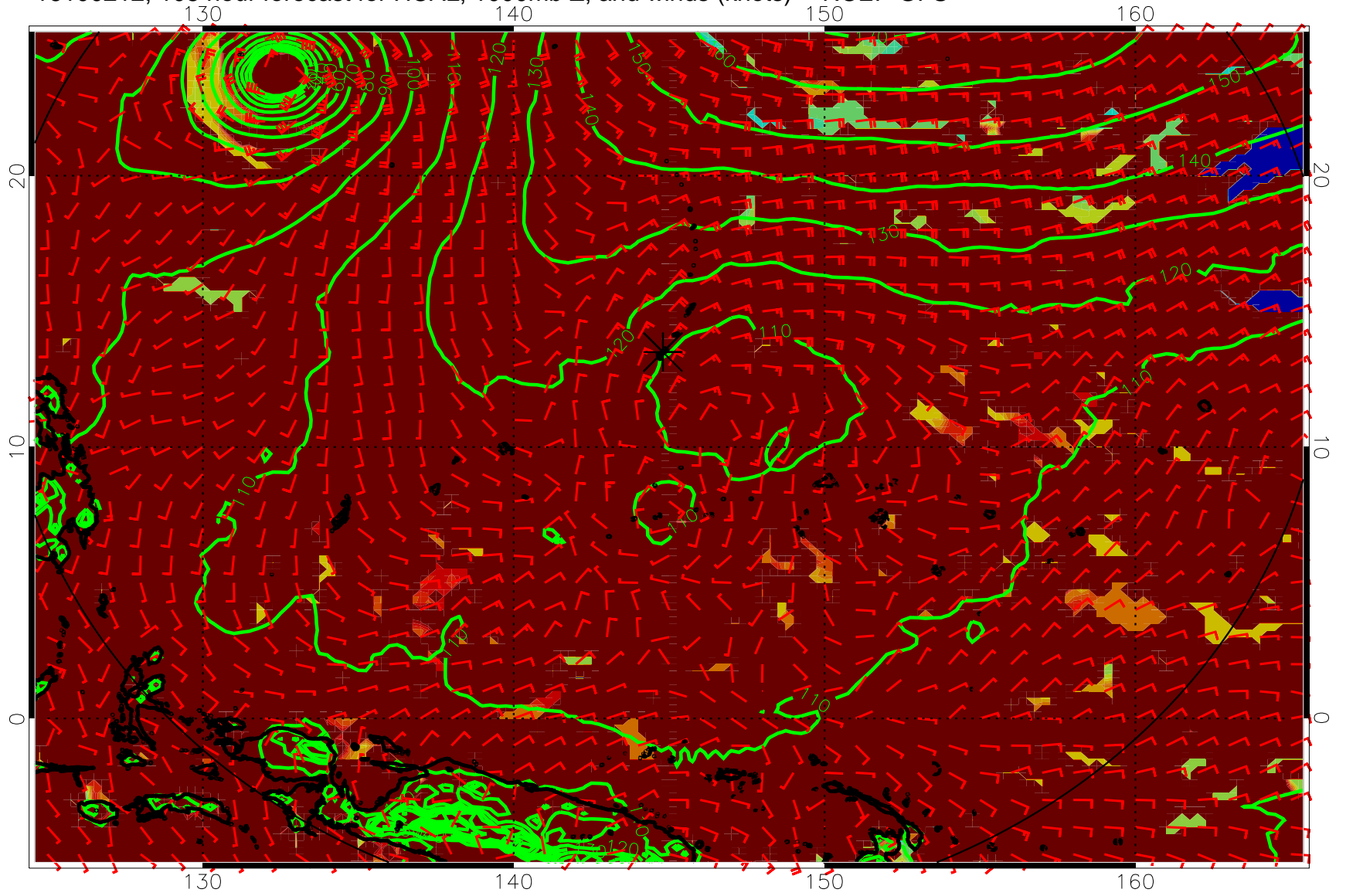
16100212, 108 hour forecast for HCAL, 1000mb Z, and winds (knots) -- NCEP GFS
