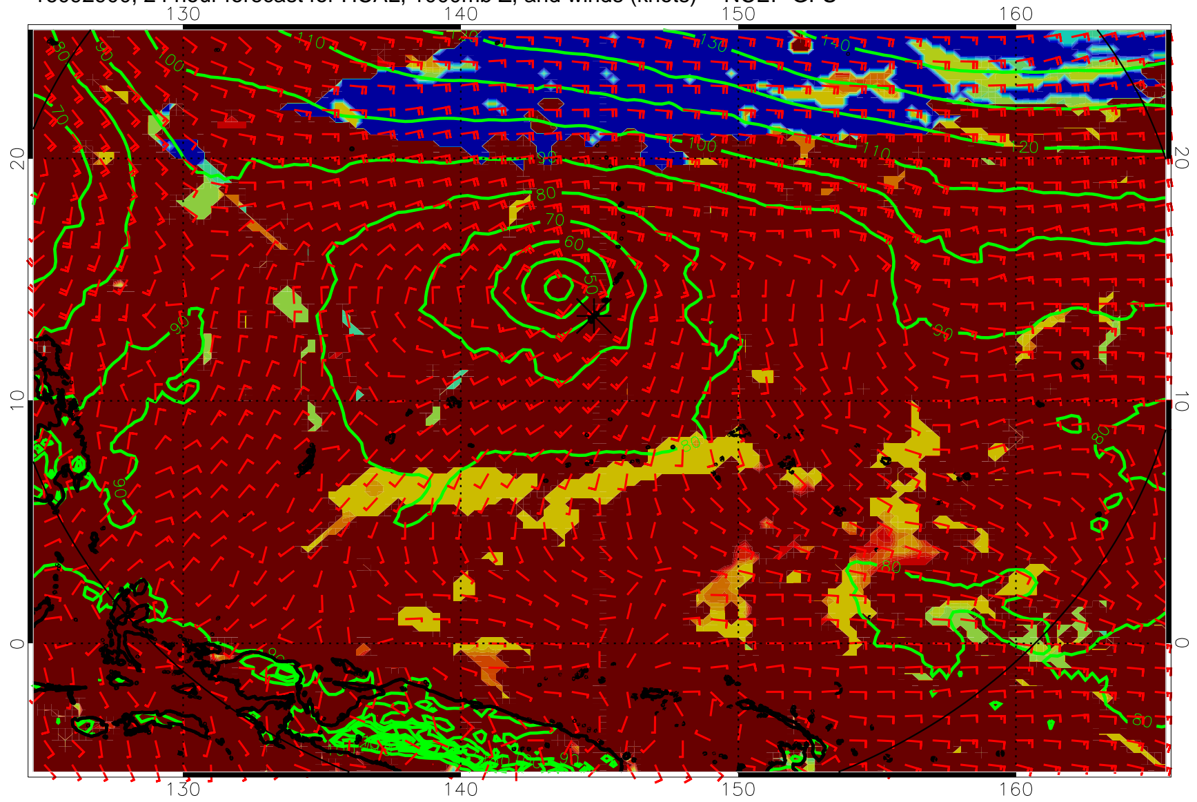
16092900, 24 hour forecast for HCAL, 1000mb Z, and winds (knots) -- NCEP GFS
