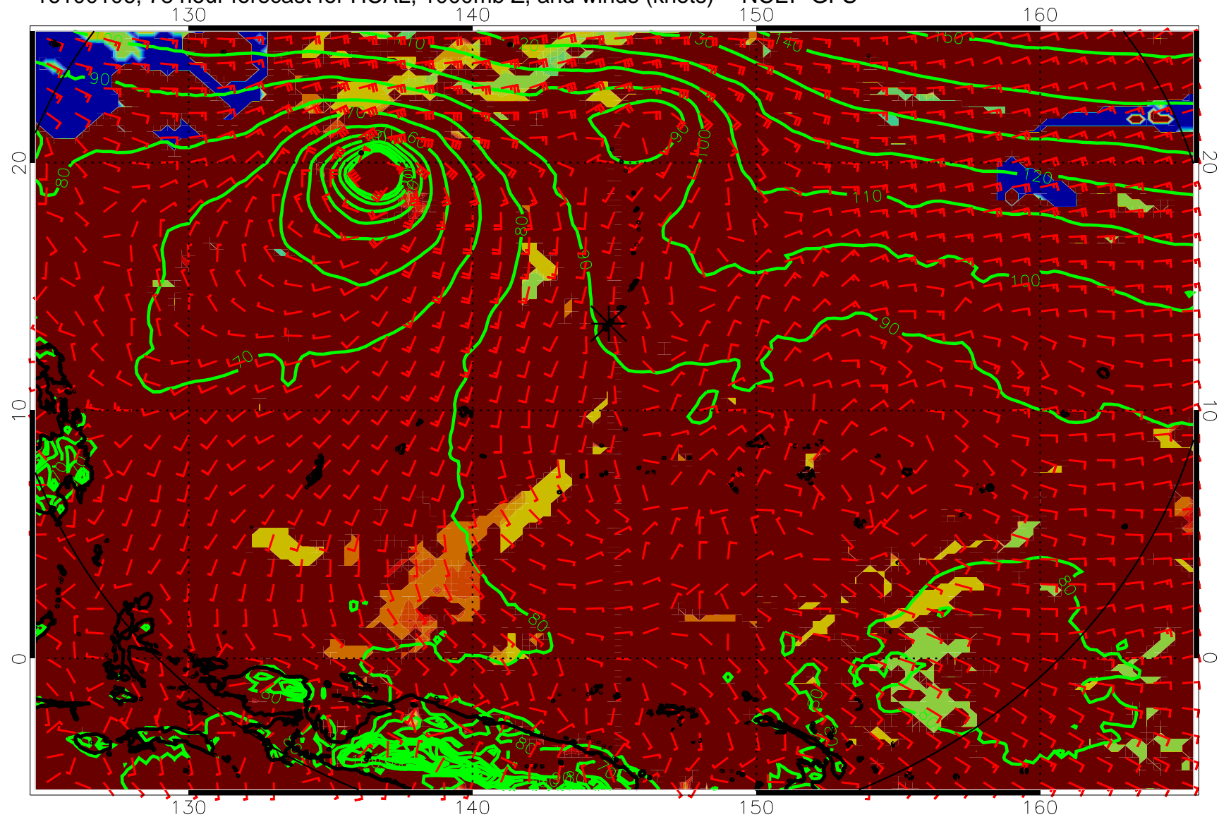
16100106, 78 hour forecast for HCAL, 1000mb Z, and winds (knots) -- NCEP GFS
