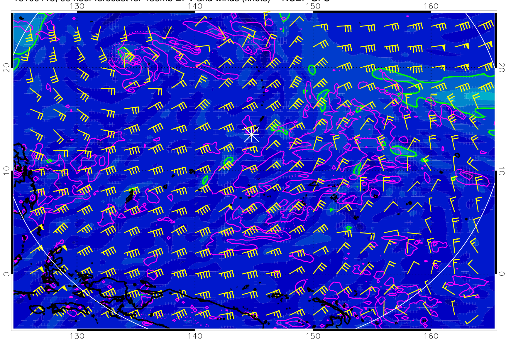
16100118, 90 hour forecast for 150mb EPV and winds (knots) -- NCEP GFS
