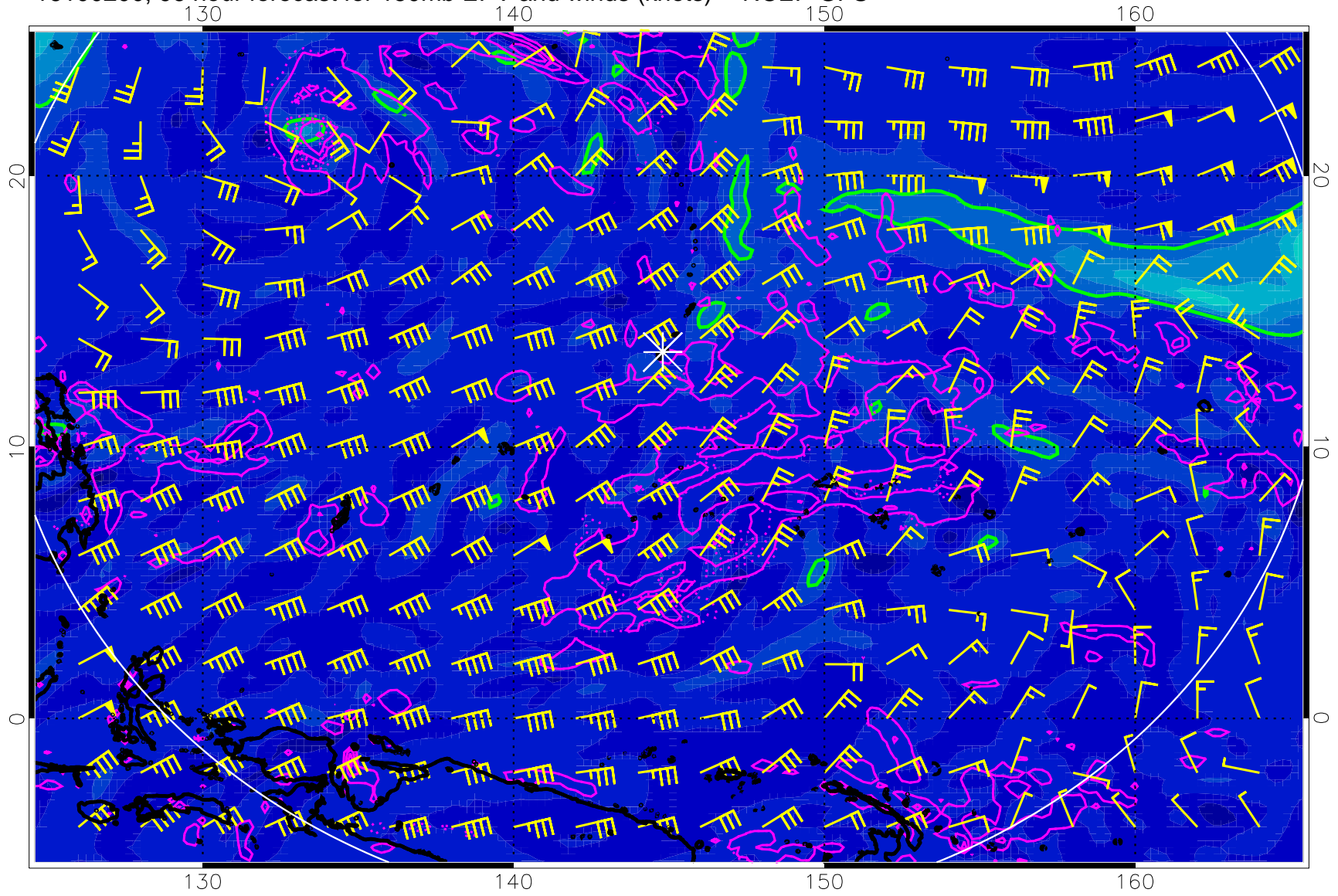
16100200, 96 hour forecast for 150mb EPV and winds (knots) -- NCEP GFS
