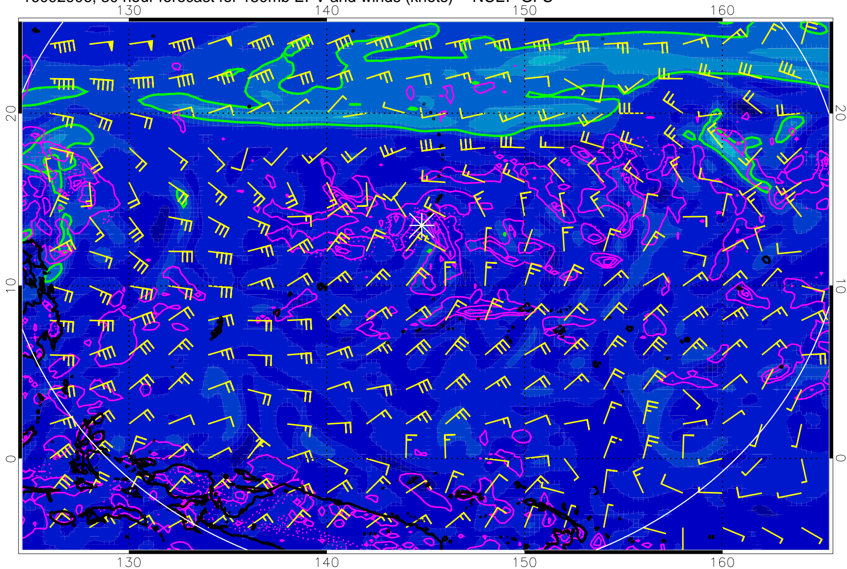
16092906, 30 hour forecast for 150mb EPV and winds (knots) -- NCEP GFS
