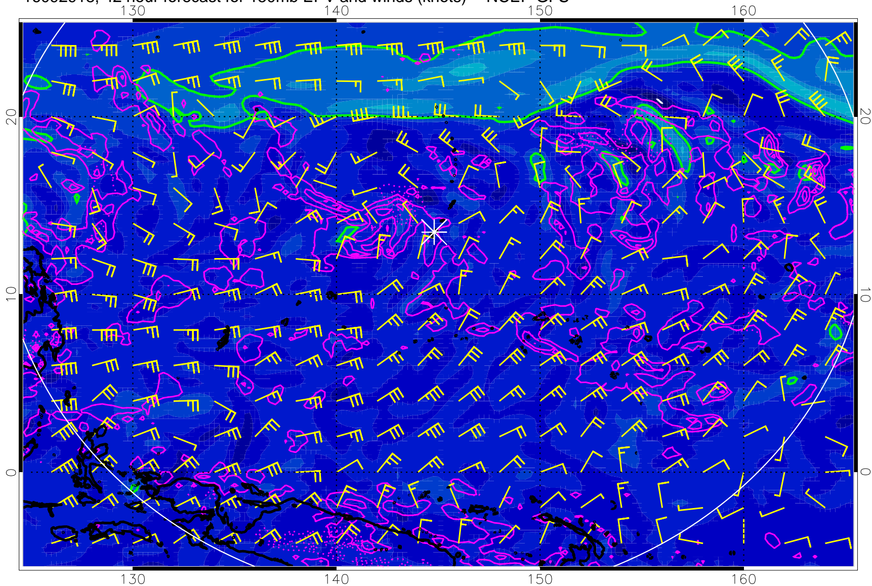
16092918, 42 hour forecast for 150mb EPV and winds (knots) -- NCEP GFS
