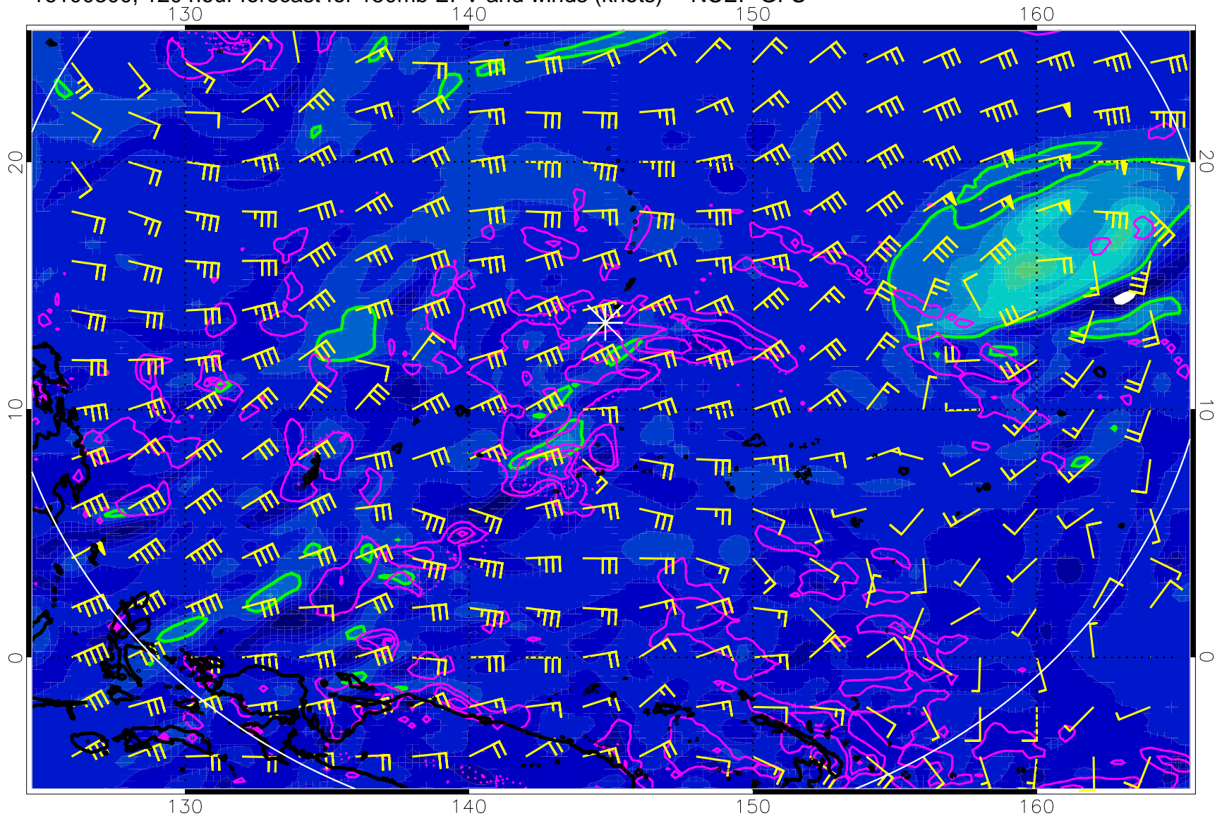
16100300, 120 hour forecast for 150mb EPV and winds (knots) -- NCEP GFS
