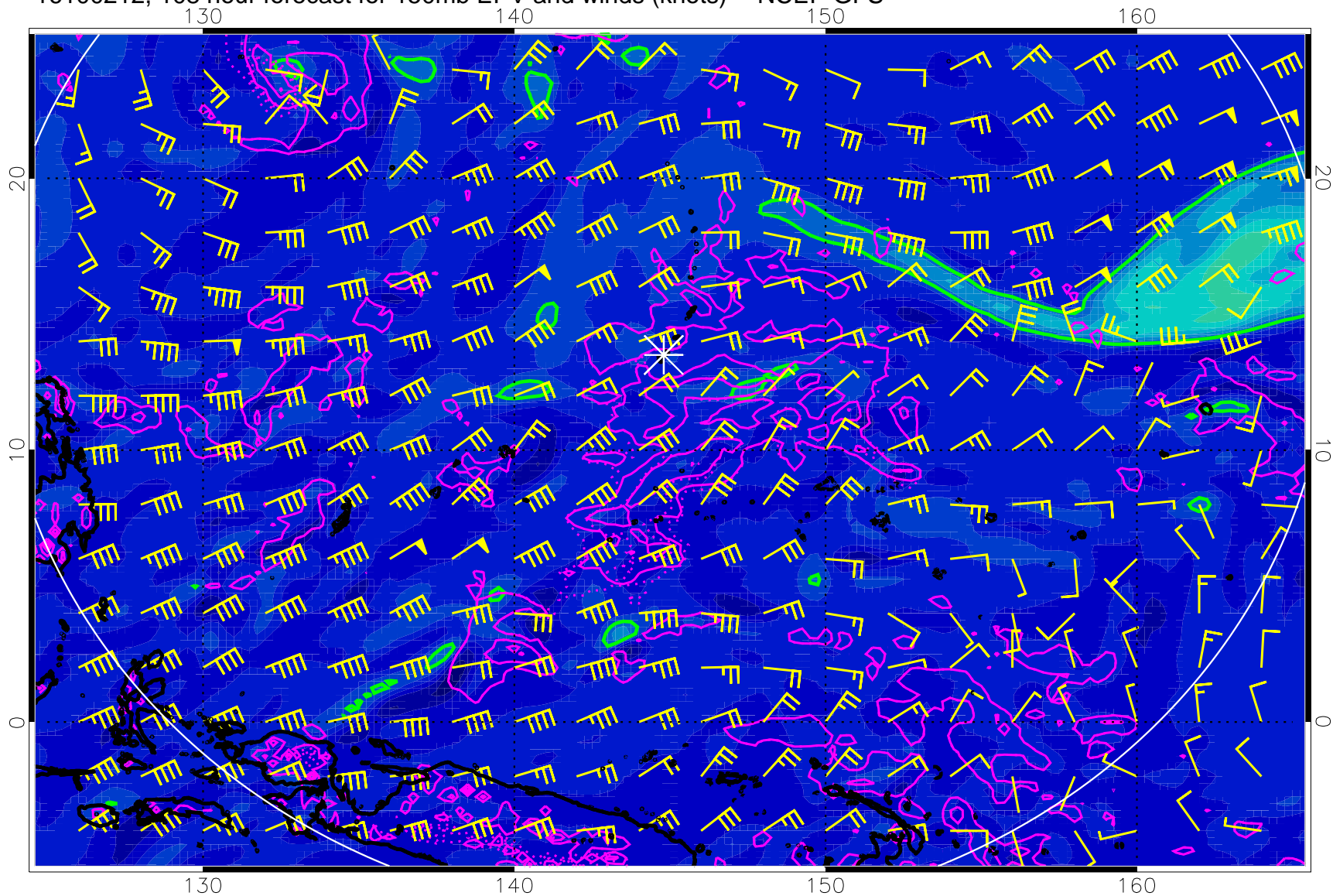
16100212, 108 hour forecast for 150mb EPV and winds (knots) -- NCEP GFS
