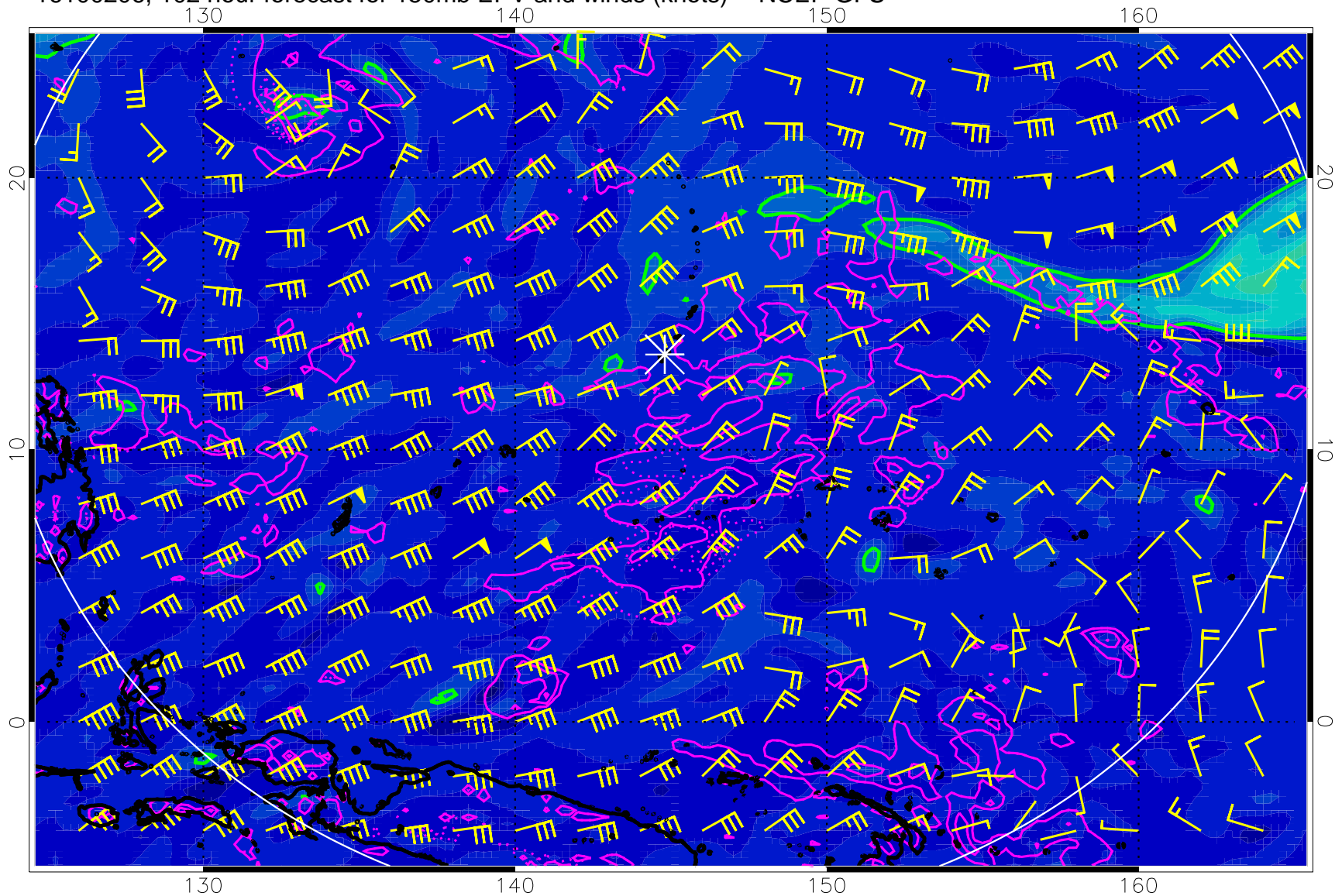
16100206, 102 hour forecast for 150mb EPV and winds (knots) -- NCEP GFS
