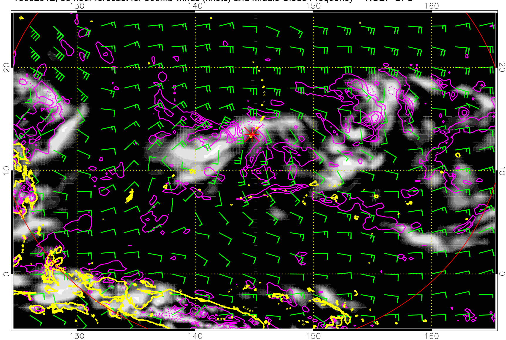
16092912, 36 hour forecast for 500mb winds (knots) and Middle Cloud Frequency -- NCEP GFS
