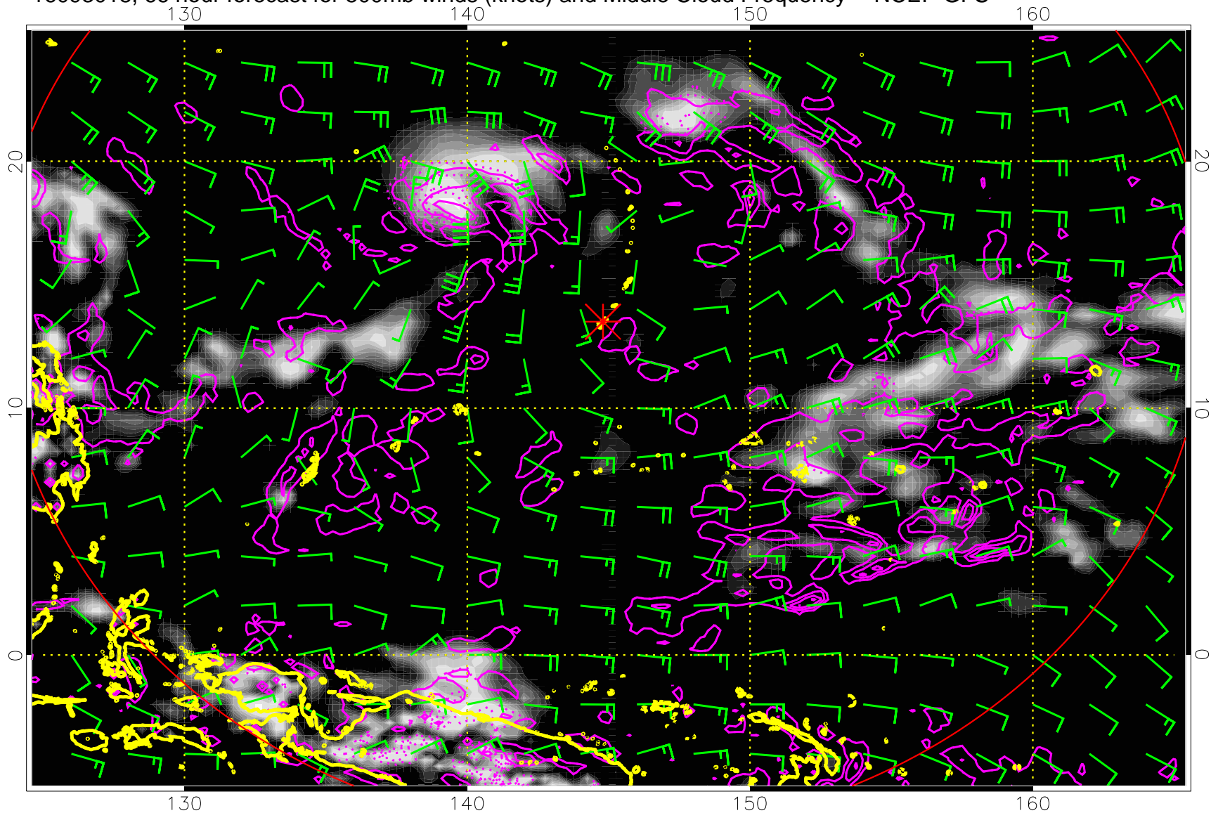
16093018, 66 hour forecast for 500mb winds (knots) and Middle Cloud Frequency -- NCEP GFS
