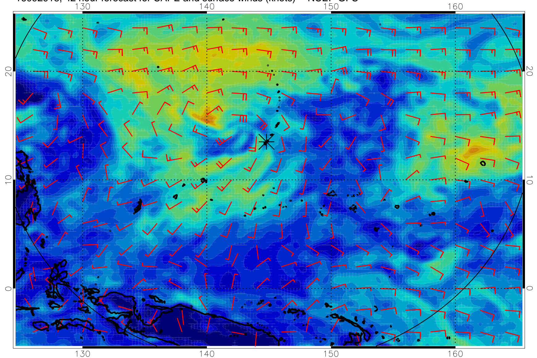
16092918, 42 hour forecast for CAPE and surface winds (knots) -- NCEP GFS
