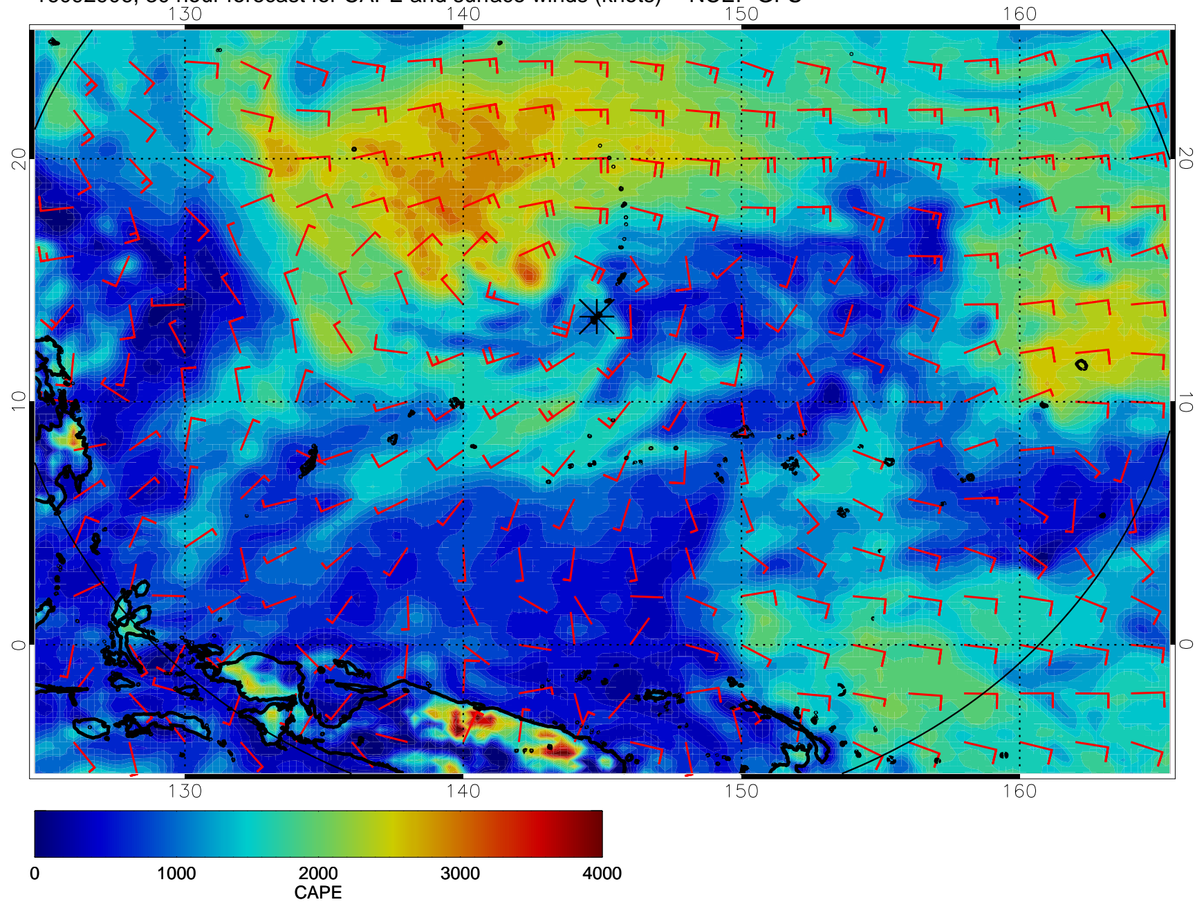
16092906, 30 hour forecast for CAPE and surface winds (knots) -- NCEP GFS
