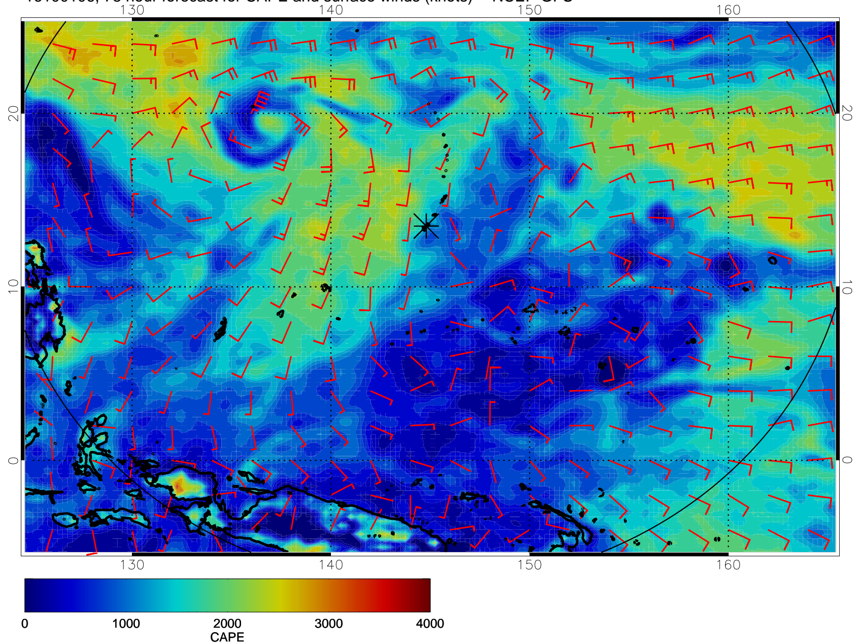
16100106, 78 hour forecast for CAPE and surface winds (knots) -- NCEP GFS
