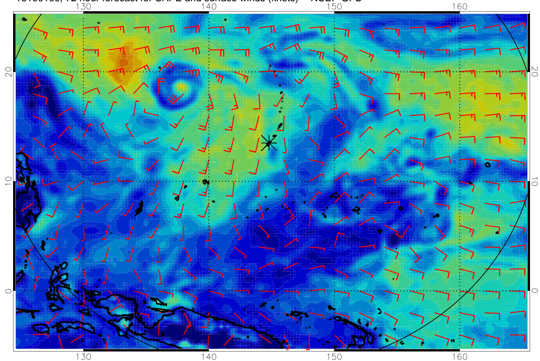
16100100, 72 hour forecast for CAPE and surface winds (knots) -- NCEP GFS
