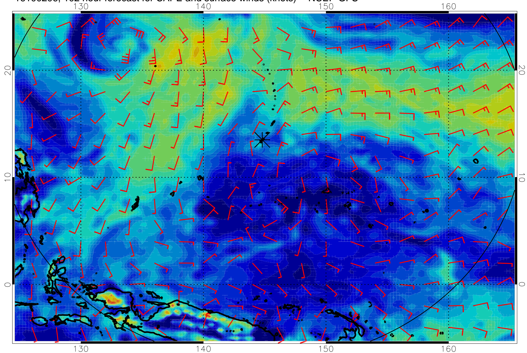
16100206, 102 hour forecast for CAPE and surface winds (knots) -- NCEP GFS
