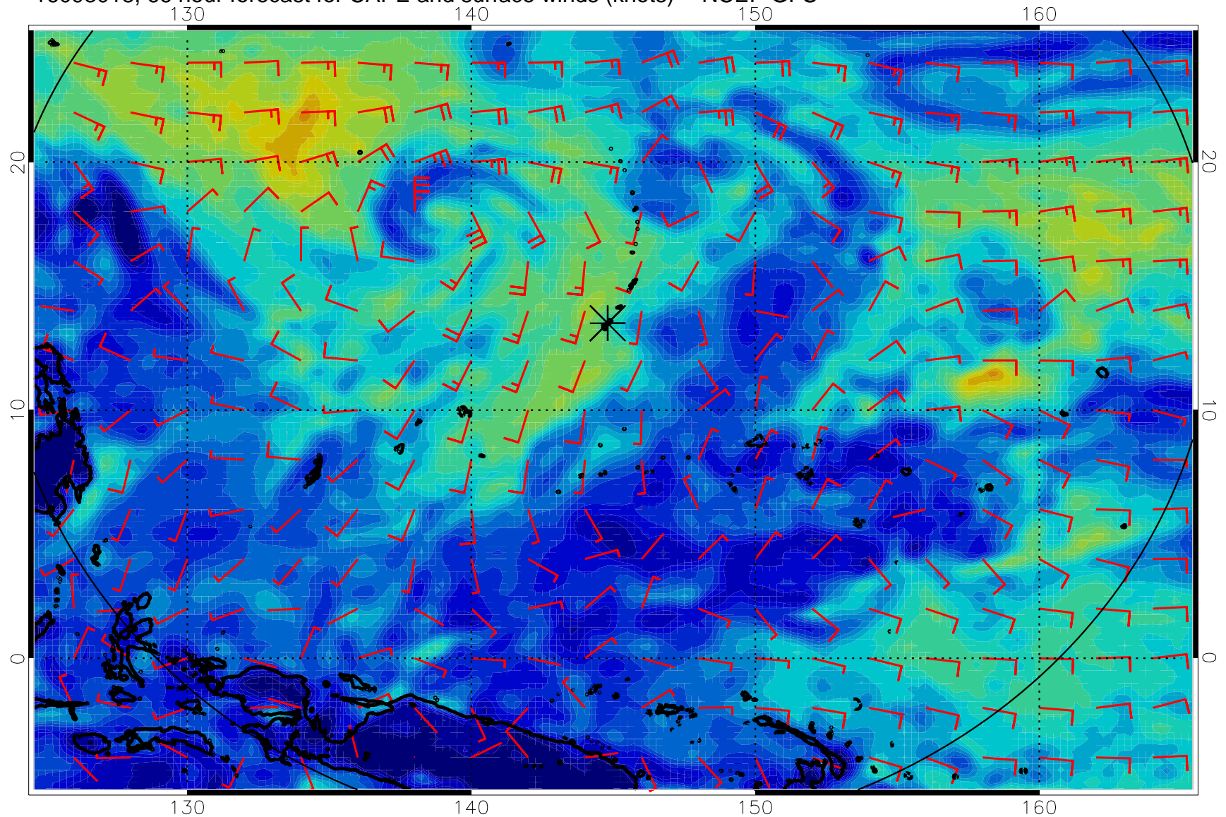
16093018, 66 hour forecast for CAPE and surface winds (knots) -- NCEP GFS
