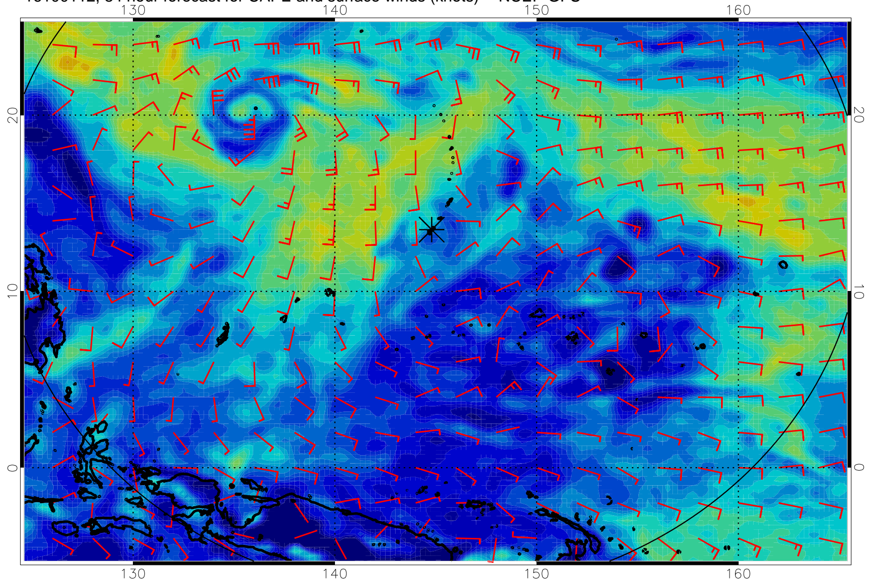
16100112, 84 hour forecast for CAPE and surface winds (knots) -- NCEP GFS
