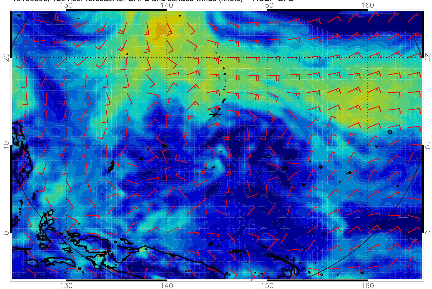
16100300, 120 hour forecast for CAPE and surface winds (knots) -- NCEP GFS
