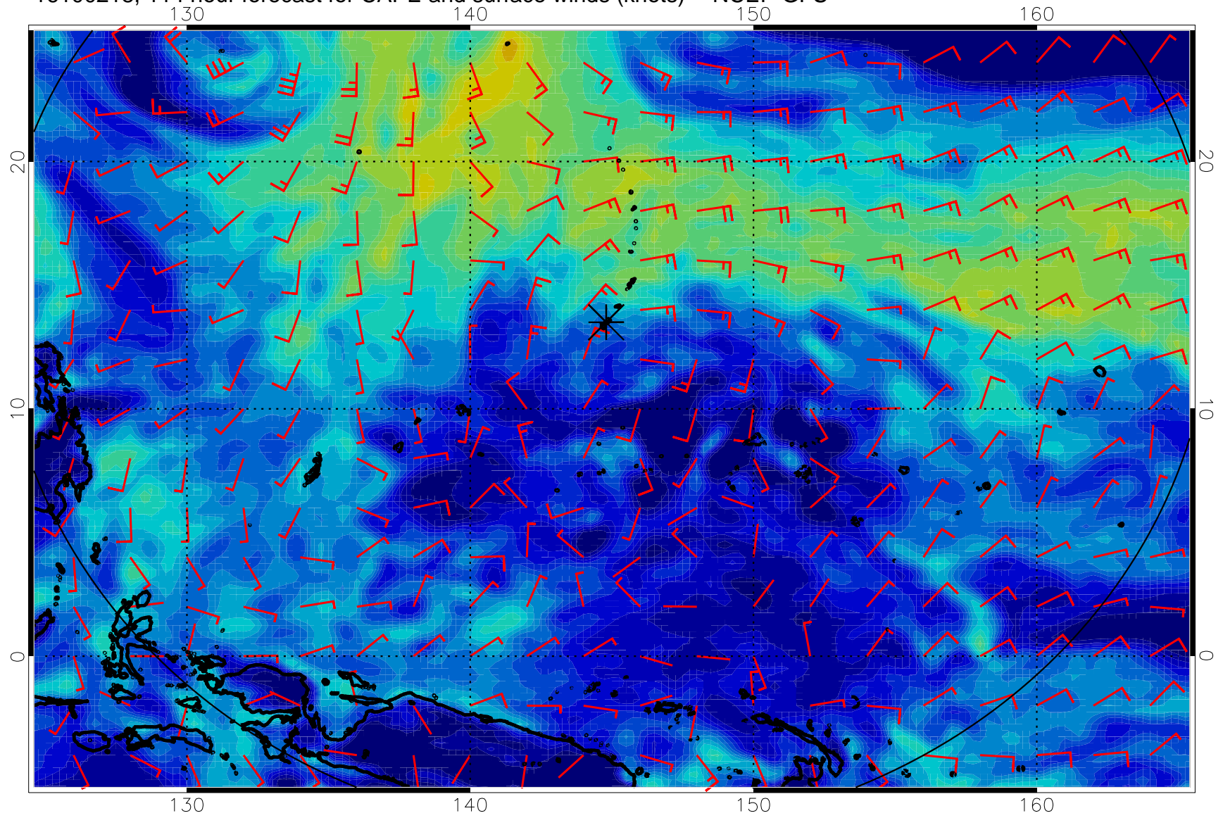
16100218, 114 hour forecast for CAPE and surface winds (knots) -- NCEP GFS
