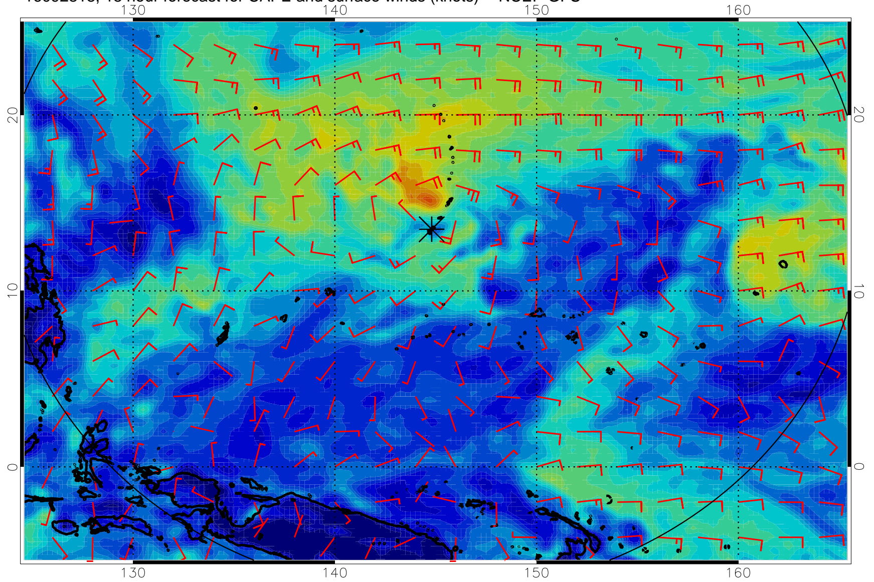
16092818, 18 hour forecast for CAPE and surface winds (knots) -- NCEP GFS
