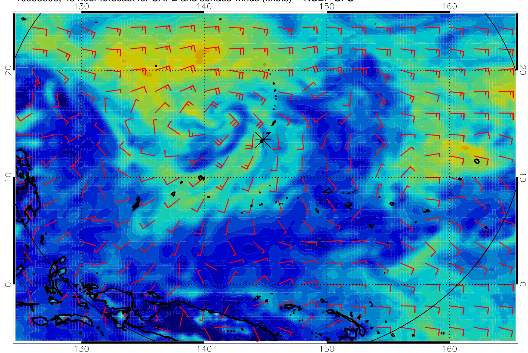
16093000, 48 hour forecast for CAPE and surface winds (knots) -- NCEP GFS
