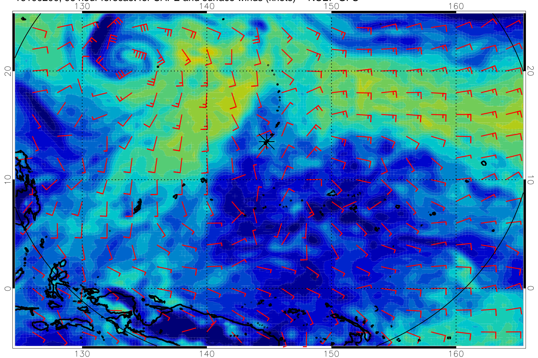
16100200, 96 hour forecast for CAPE and surface winds (knots) -- NCEP GFS
