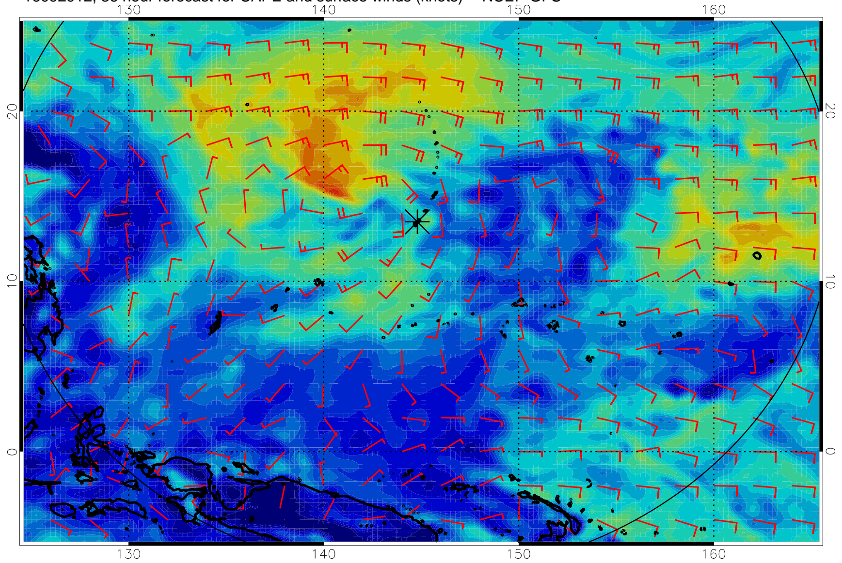
16092912, 36 hour forecast for CAPE and surface winds (knots) -- NCEP GFS
