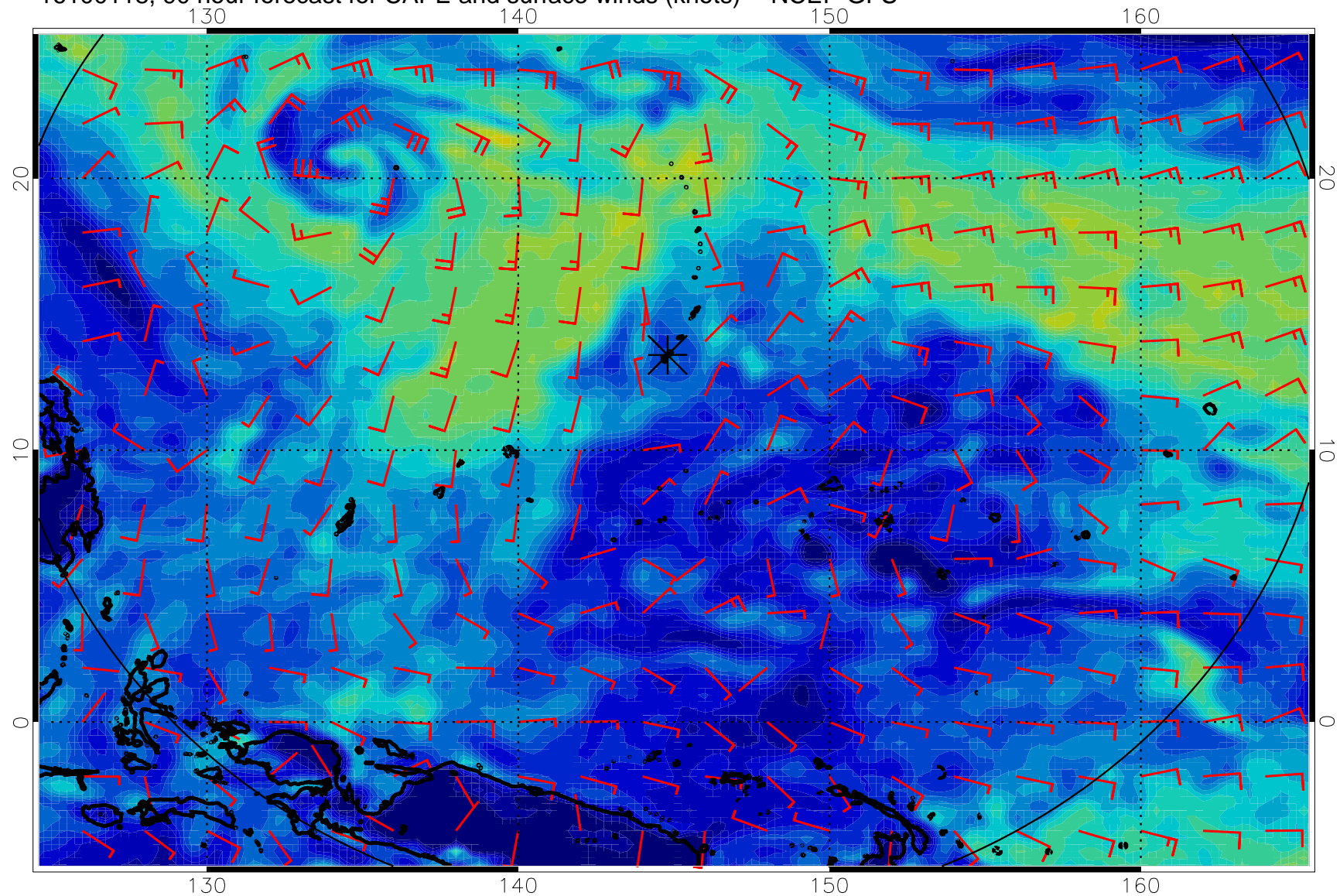
16100118, 90 hour forecast for CAPE and surface winds (knots) -- NCEP GFS
