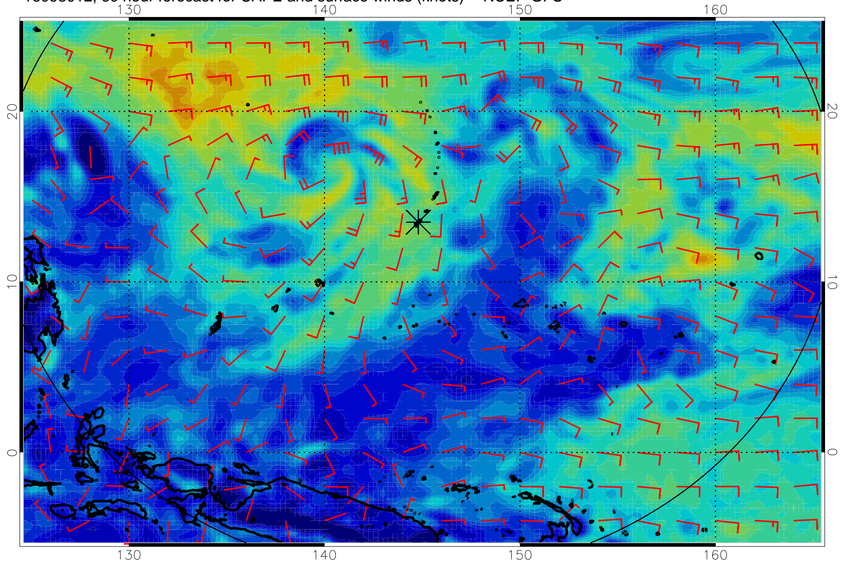
16093012, 60 hour forecast for CAPE and surface winds (knots) -- NCEP GFS
