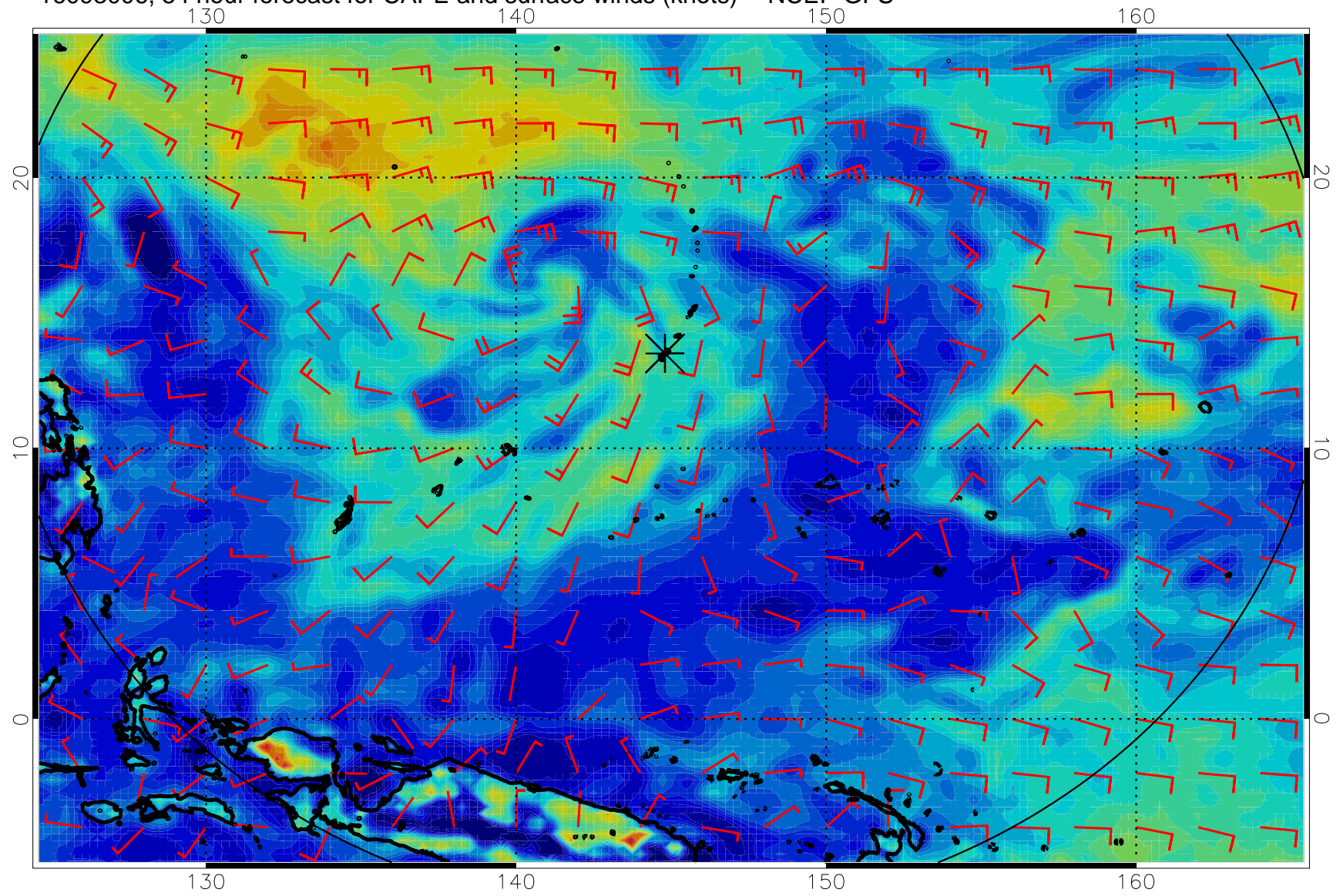
16093006, 54 hour forecast for CAPE and surface winds (knots) -- NCEP GFS
