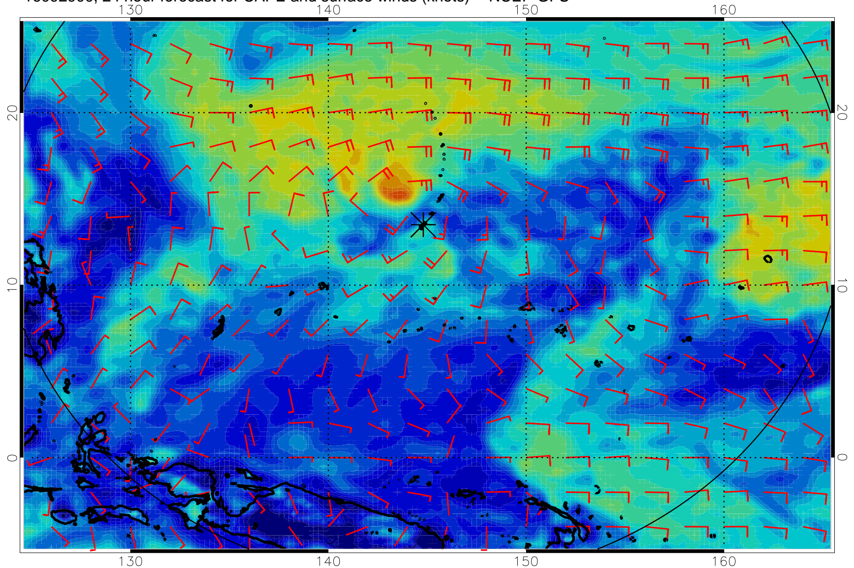
16092900, 24 hour forecast for CAPE and surface winds (knots) -- NCEP GFS
