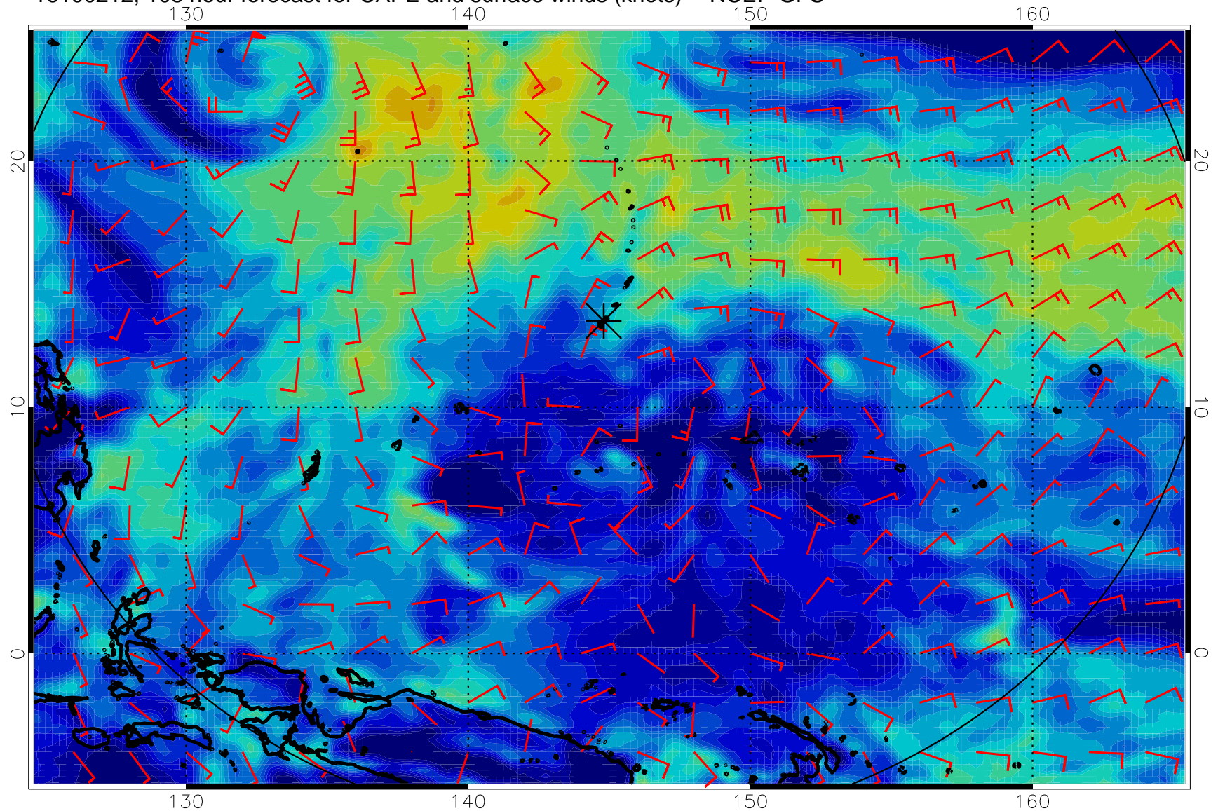
16100212, 108 hour forecast for CAPE and surface winds (knots) -- NCEP GFS
