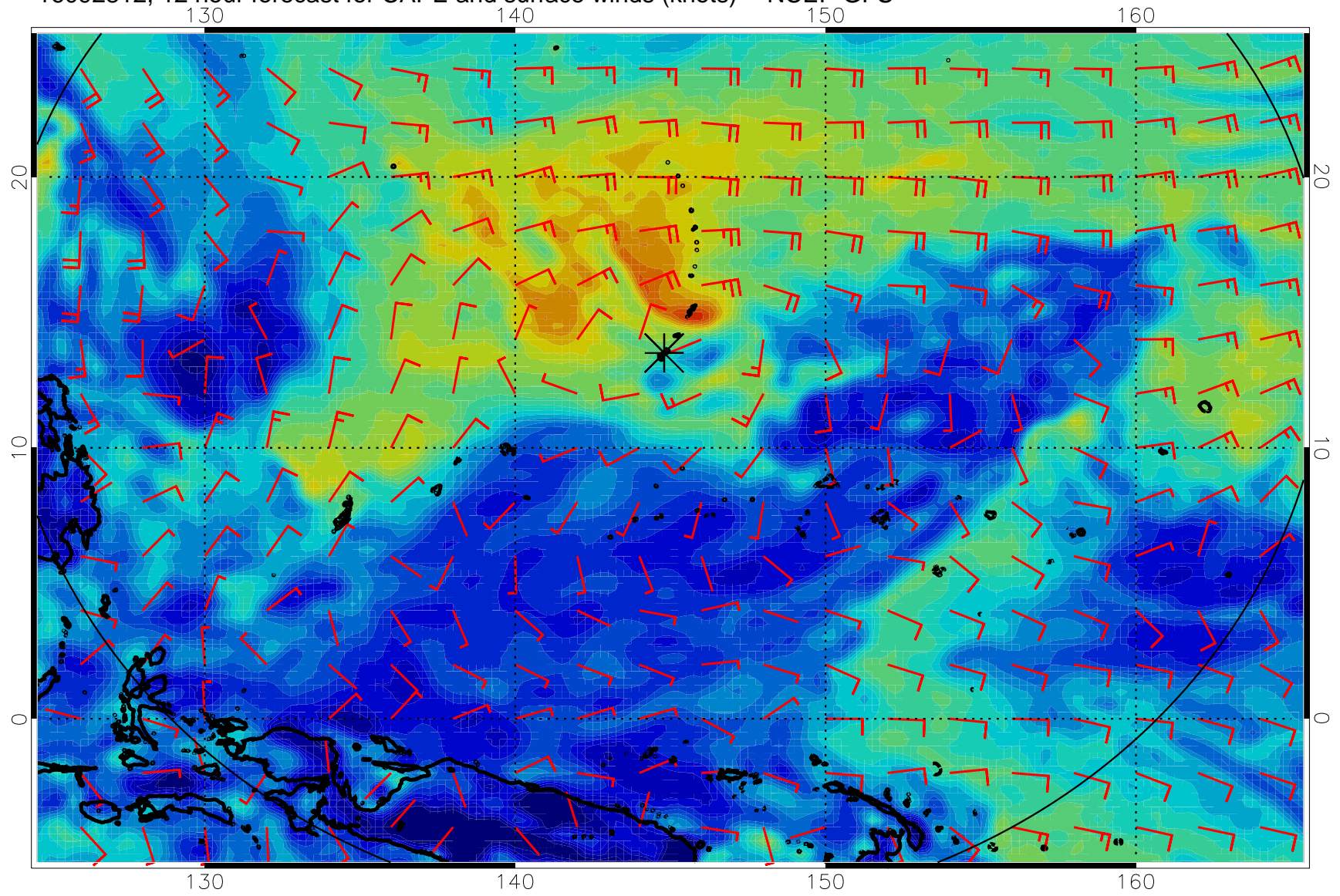
16092812, 12 hour forecast for CAPE and surface winds (knots) -- NCEP GFS
