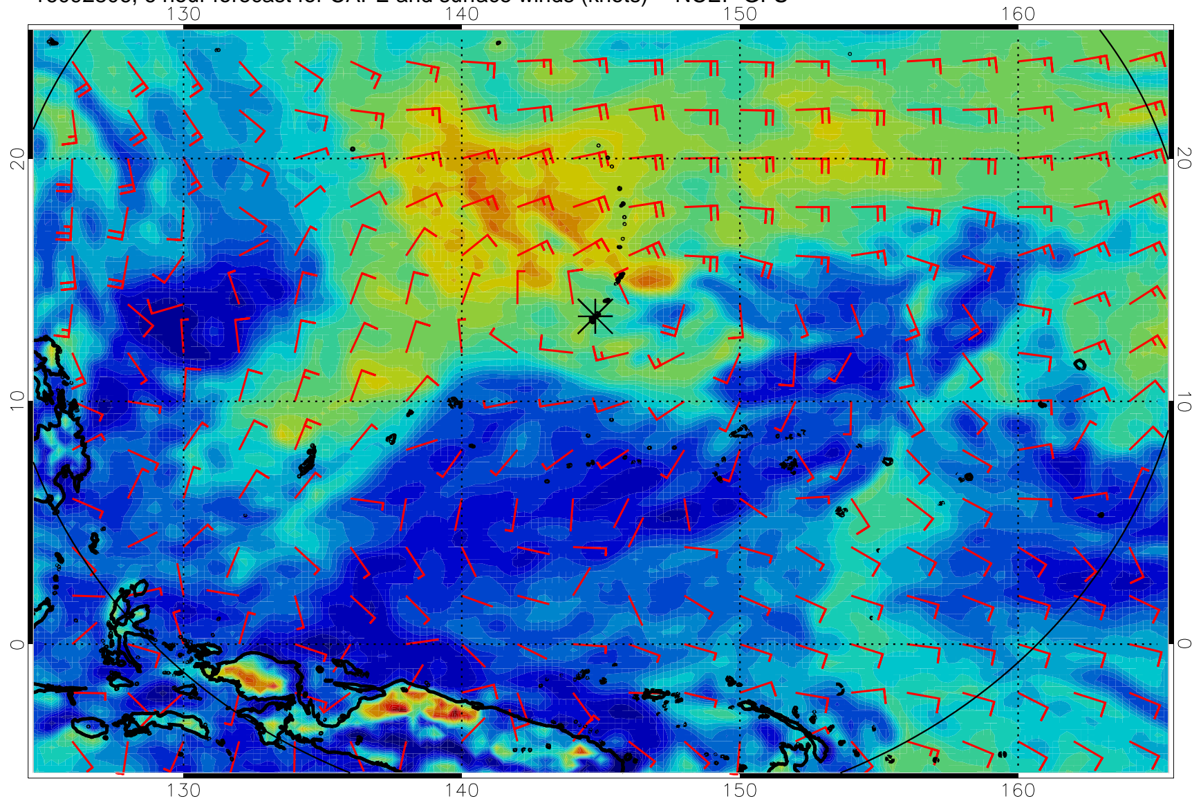
16092806, 6 hour forecast for CAPE and surface winds (knots) -- NCEP GFS
