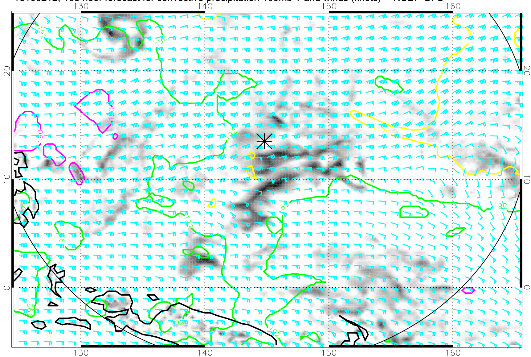
16100212, 108 hour forecast for convective precipitation 100mb T and winds (knots) -- NCEP GFS
