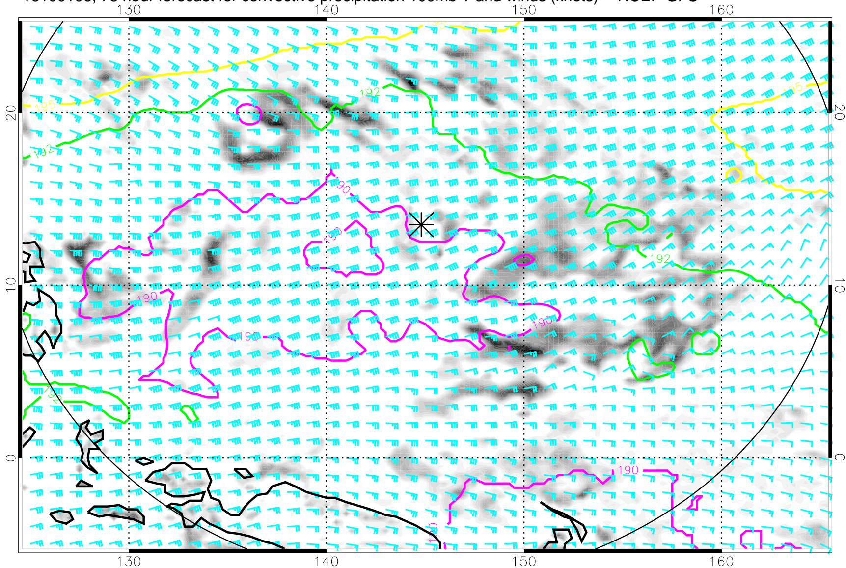
16100106, 78 hour forecast for convective precipitation 100mb T and winds (knots) -- NCEP GFS
