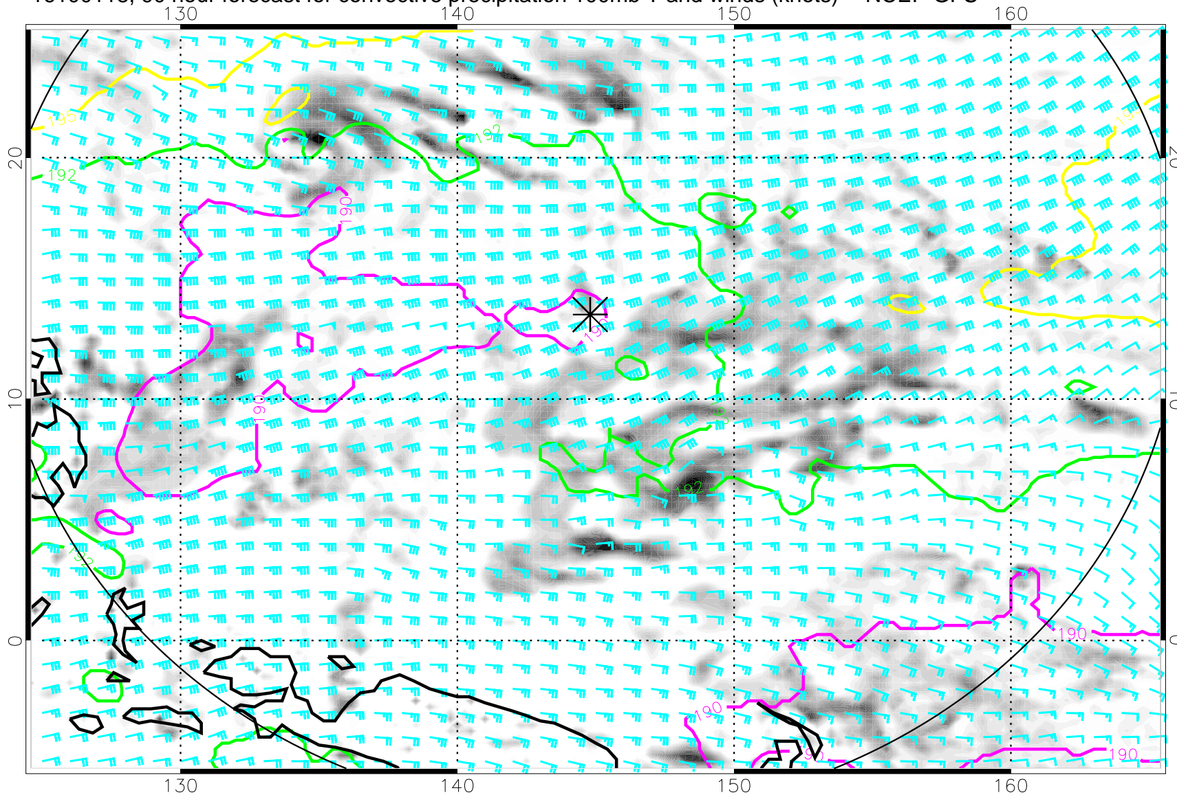
16100118, 90 hour forecast for convective precipitation 100mb T and winds (knots) -- NCEP GFS
