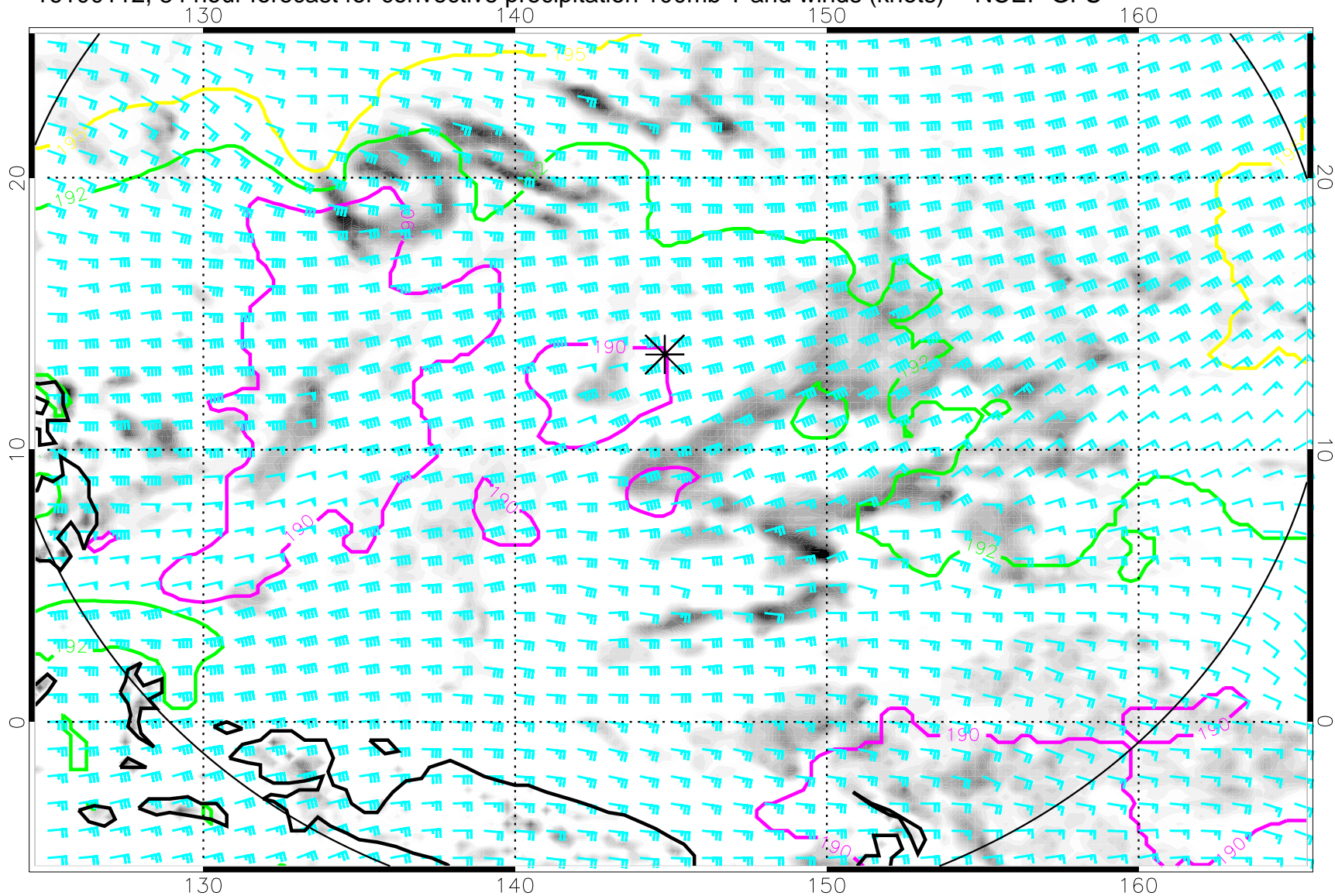
16100112, 84 hour forecast for convective precipitation 100mb T and winds (knots) -- NCEP GFS
