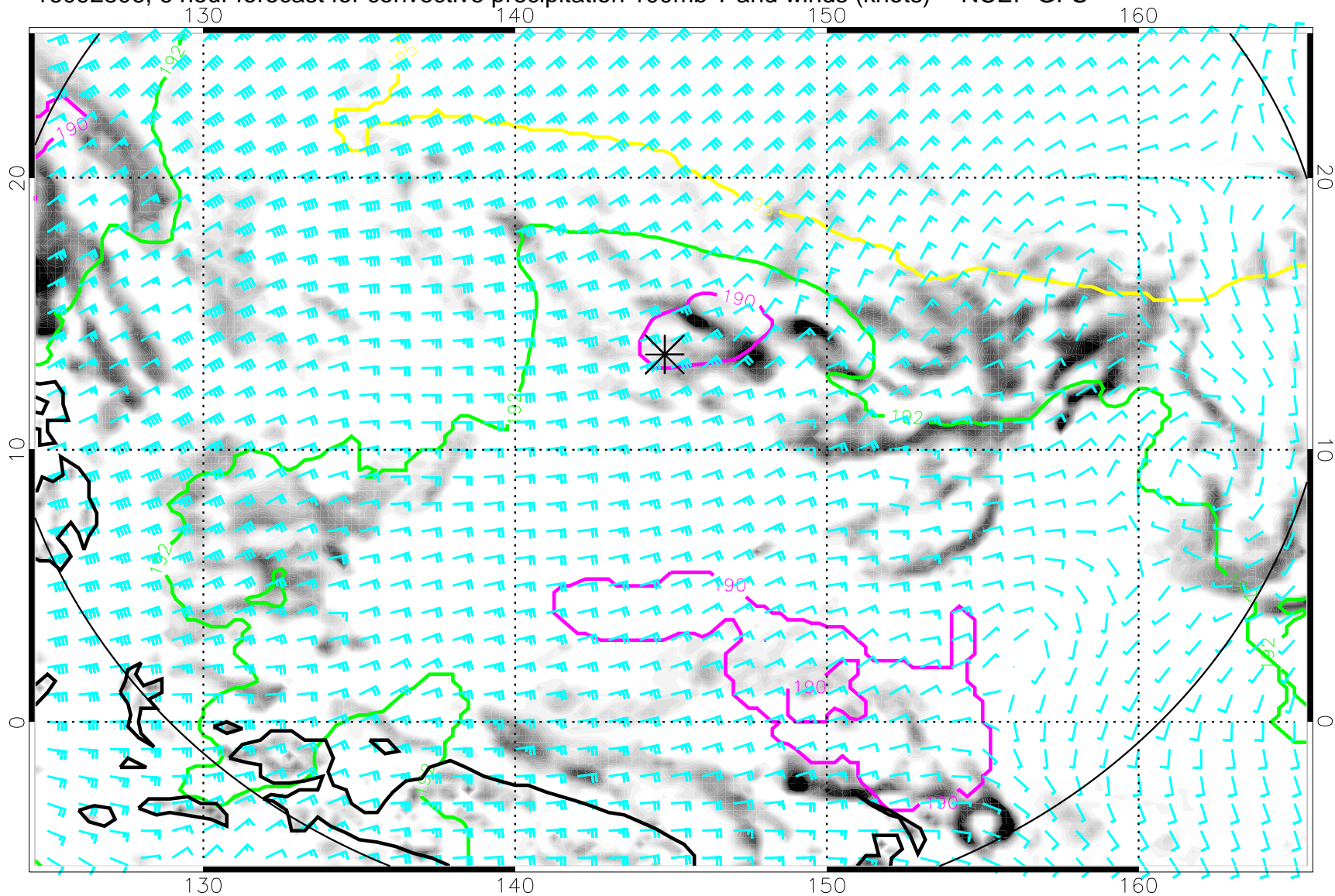
16092806, 6 hour forecast for convective precipitation 100mb T and winds (knots) -- NCEP GFS
