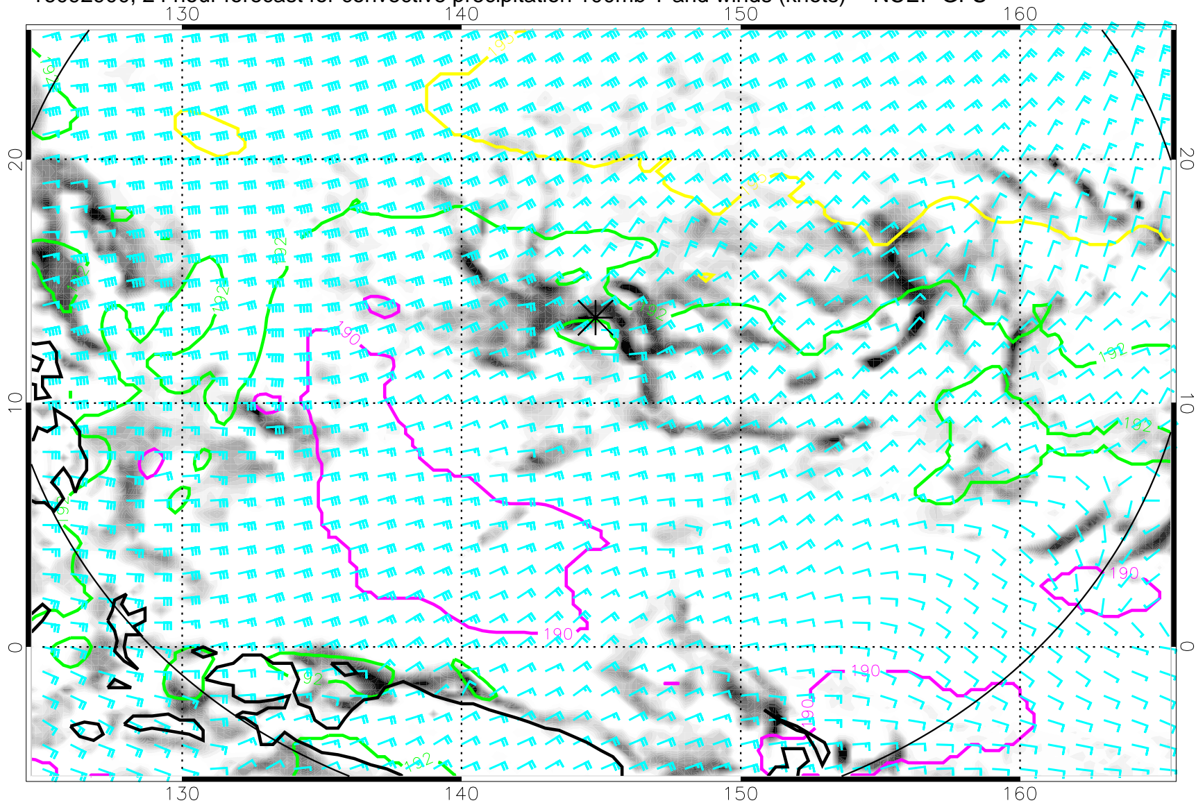
16092900, 24 hour forecast for convective precipitation 100mb T and winds (knots) -- NCEP GFS
