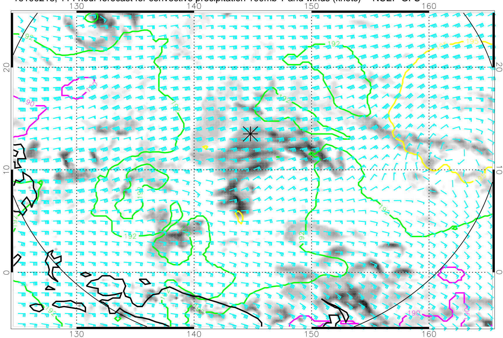
16100218, 114 hour forecast for convective precipitation 100mb T and winds (knots) -- NCEP GFS
