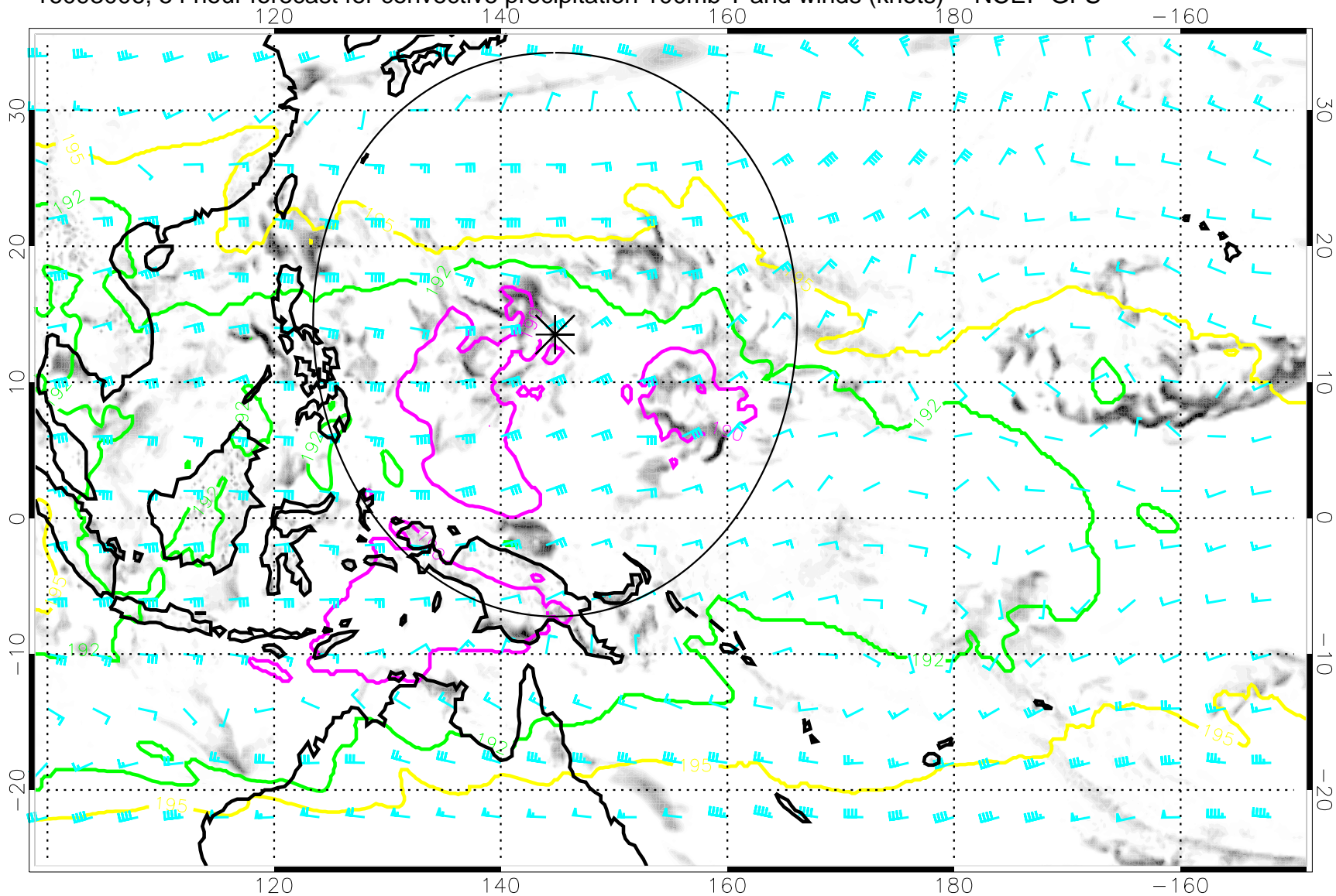
16093006, 54 hour forecast for convective precipitation 100mb T and winds (knots) -- NCEP GFS
