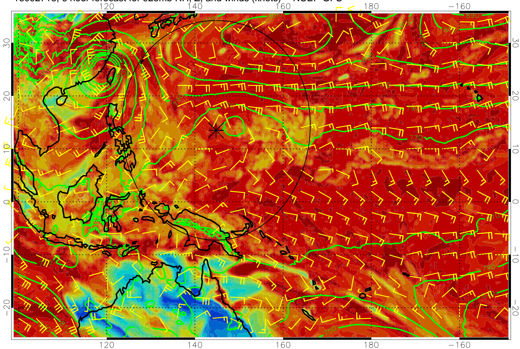
16092718, 6 hour forecast for 925mb RH, Z, and winds (knots) -- NCEP GFS
