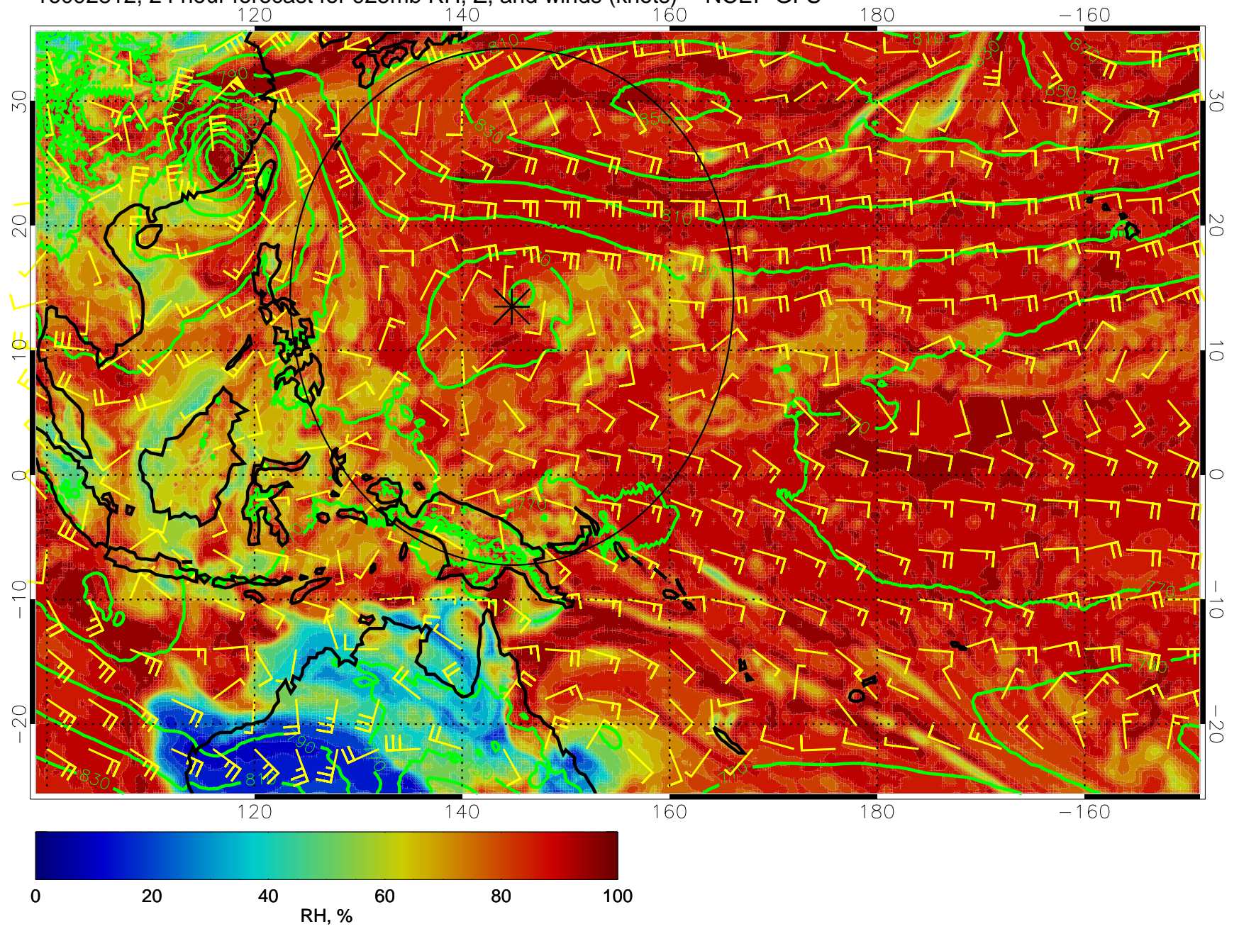
16092812, 24 hour forecast for 925mb RH, Z, and winds (knots) -- NCEP GFS
