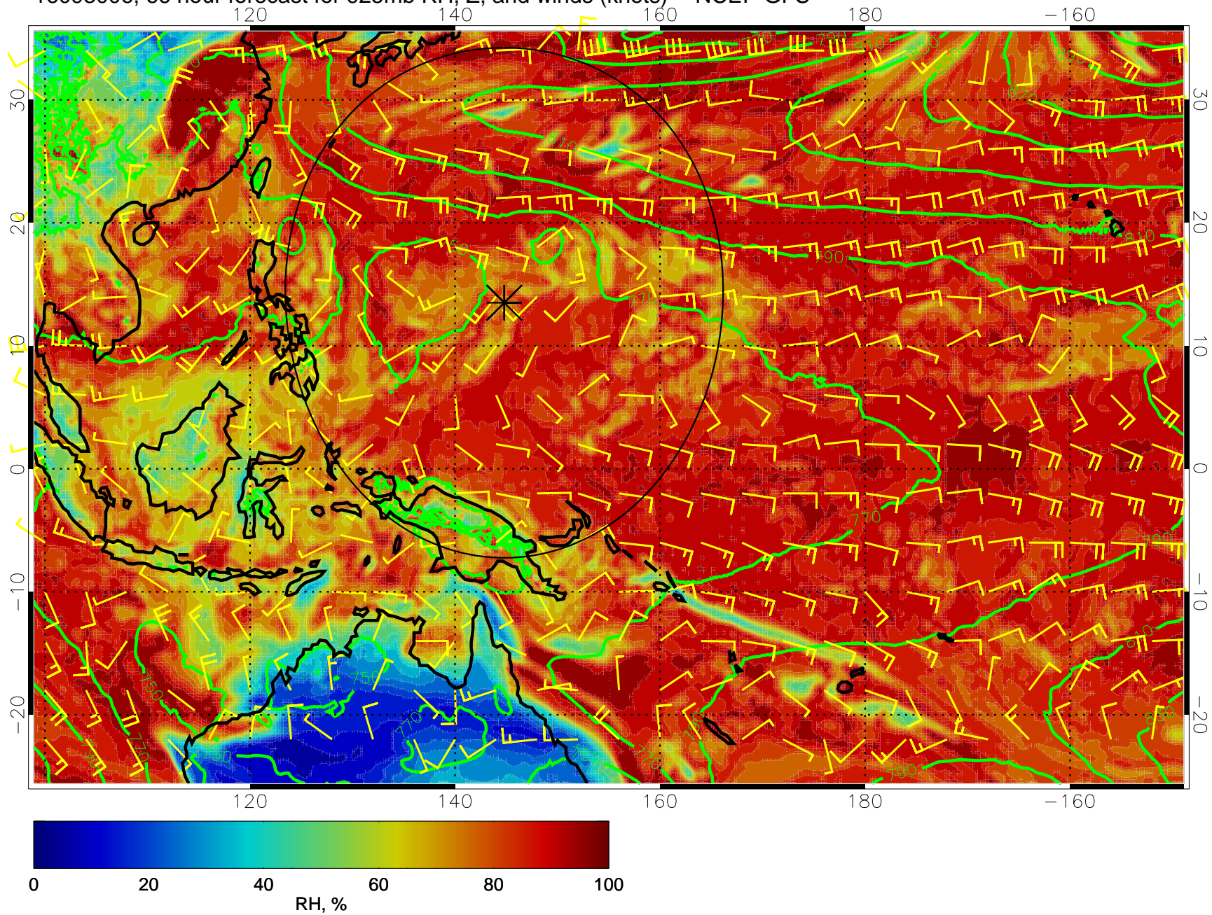
16093006, 66 hour forecast for 925mb RH, Z, and winds (knots) -- NCEP GFS
