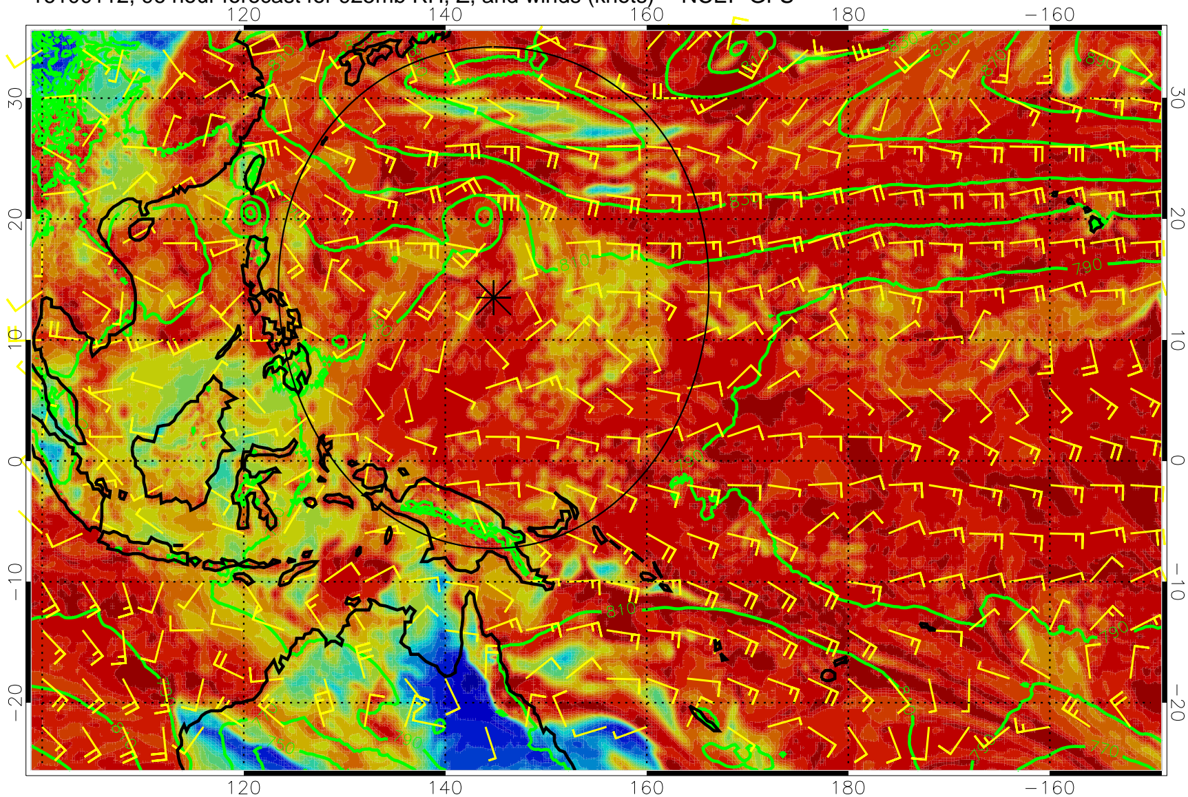
16100112, 96 hour forecast for 925mb RH, Z, and winds (knots) -- NCEP GFS
