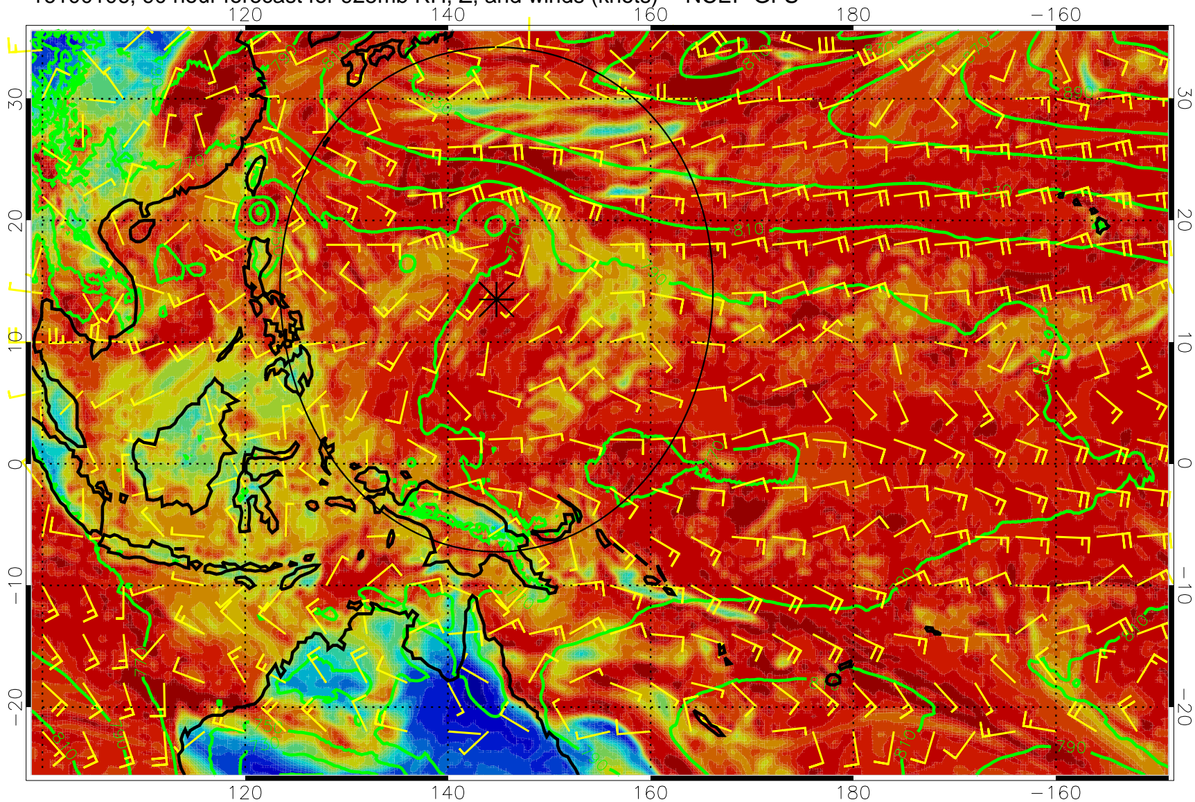
16100106, 90 hour forecast for 925mb RH, Z, and winds (knots) -- NCEP GFS
