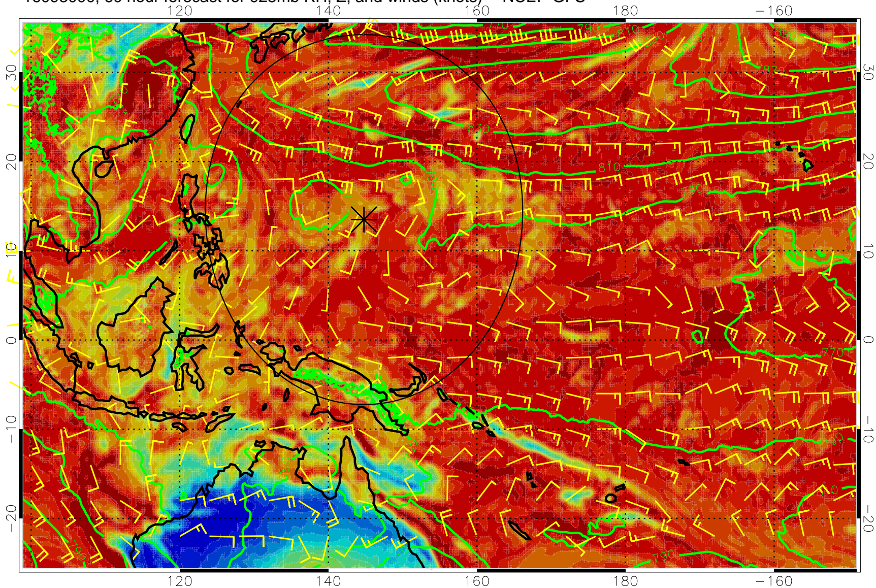
16093000, 60 hour forecast for 925mb RH, Z, and winds (knots) -- NCEP GFS
