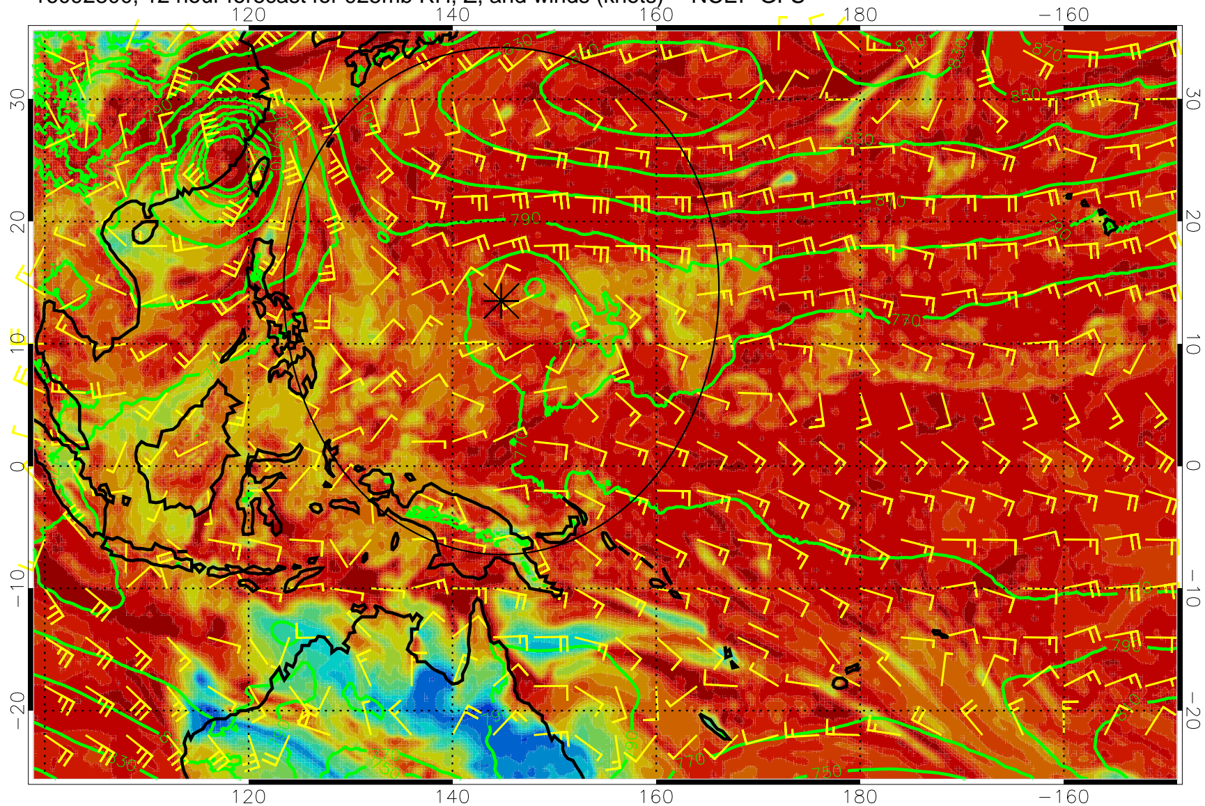
16092800, 12 hour forecast for 925mb RH, Z, and winds (knots) -- NCEP GFS
