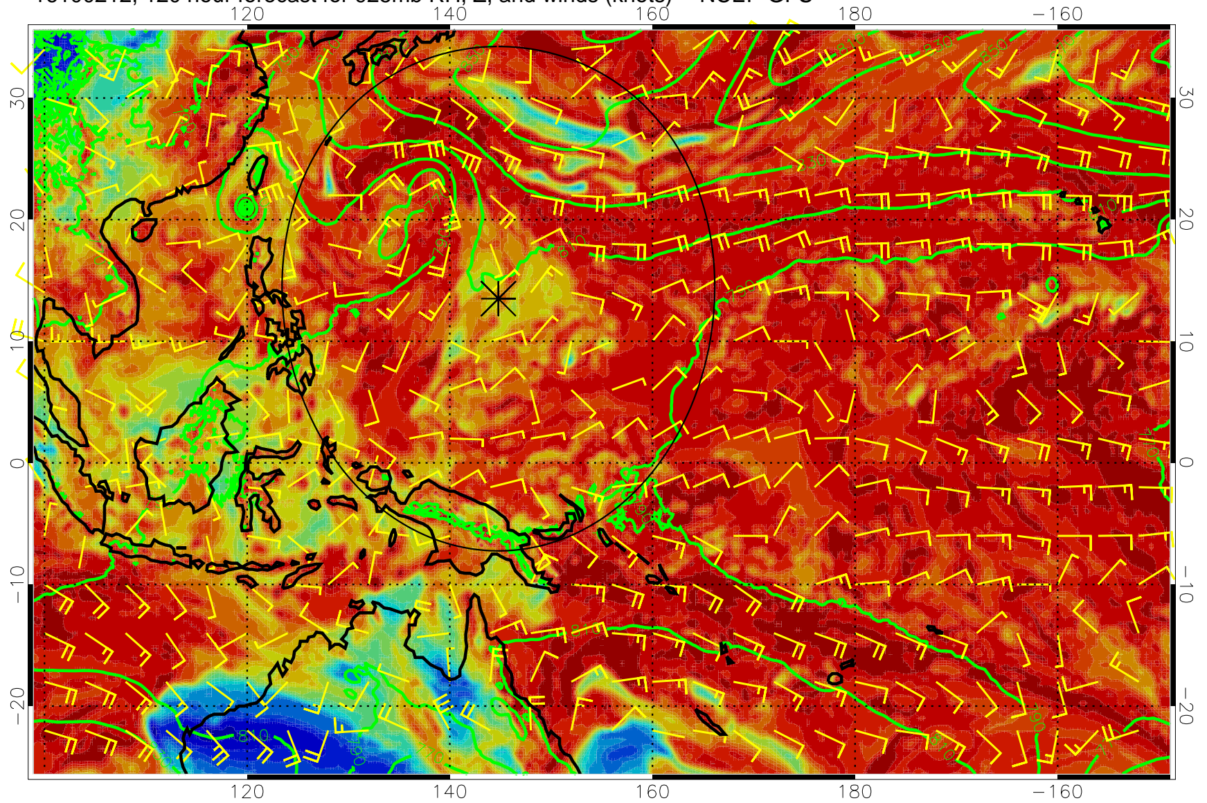
16100212, 120 hour forecast for 925mb RH, Z, and winds (knots) -- NCEP GFS
