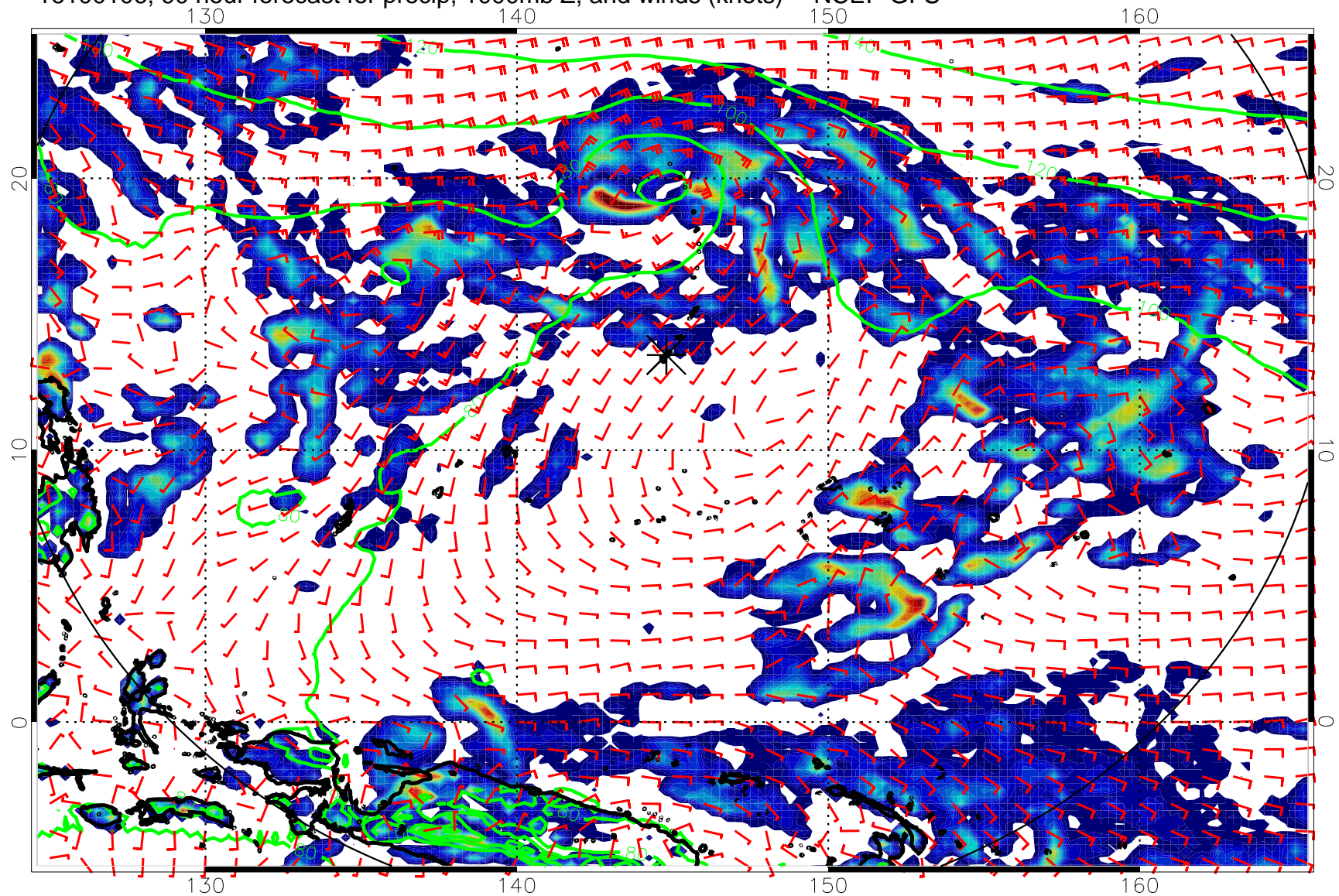
16100106, 90 hour forecast for precip, 1000mb Z, and winds (knots) -- NCEP GFS
