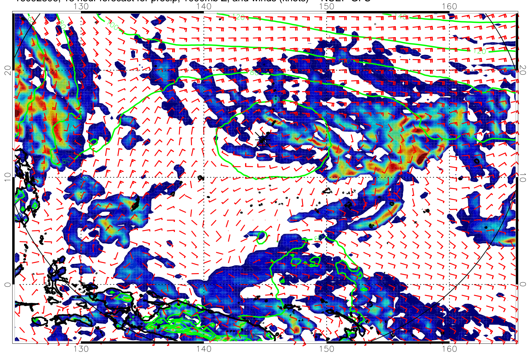
16092806, 18 hour forecast for precip, 1000mb Z, and winds (knots) -- NCEP GFS
