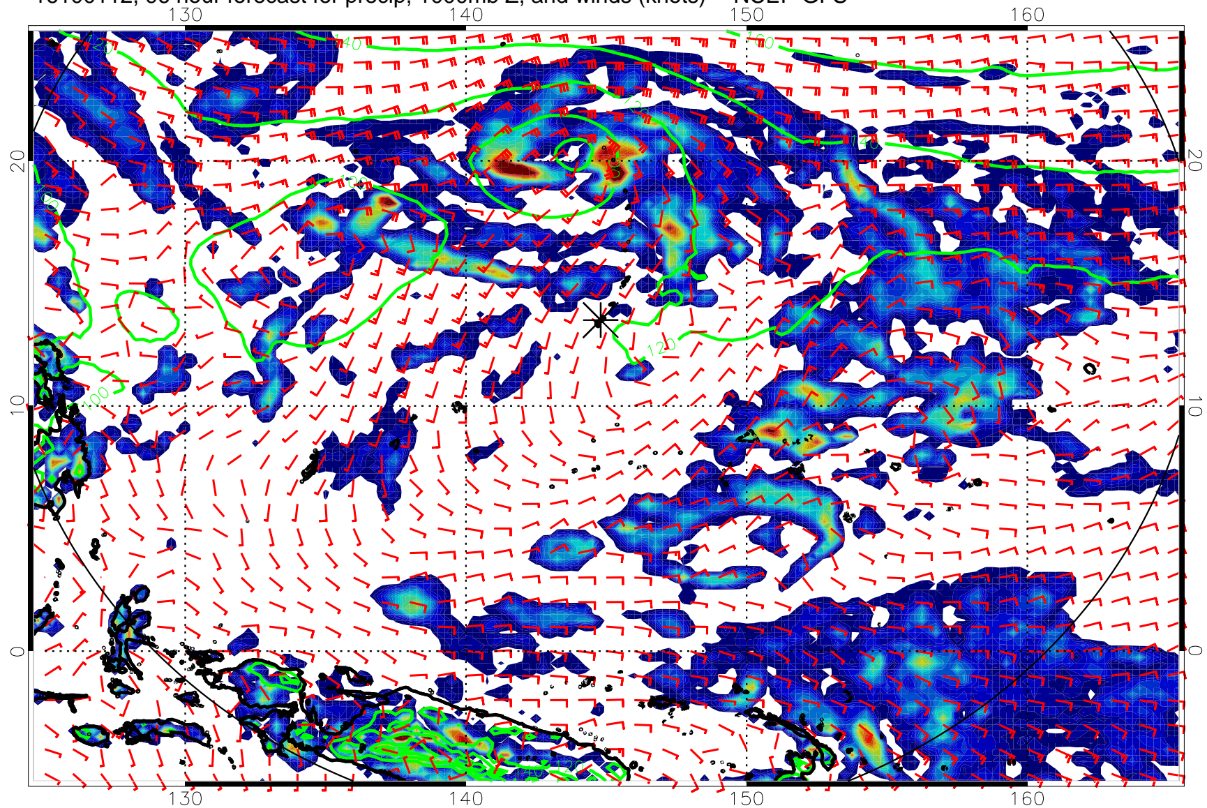
16100112, 96 hour forecast for precip, 1000mb Z, and winds (knots) -- NCEP GFS
