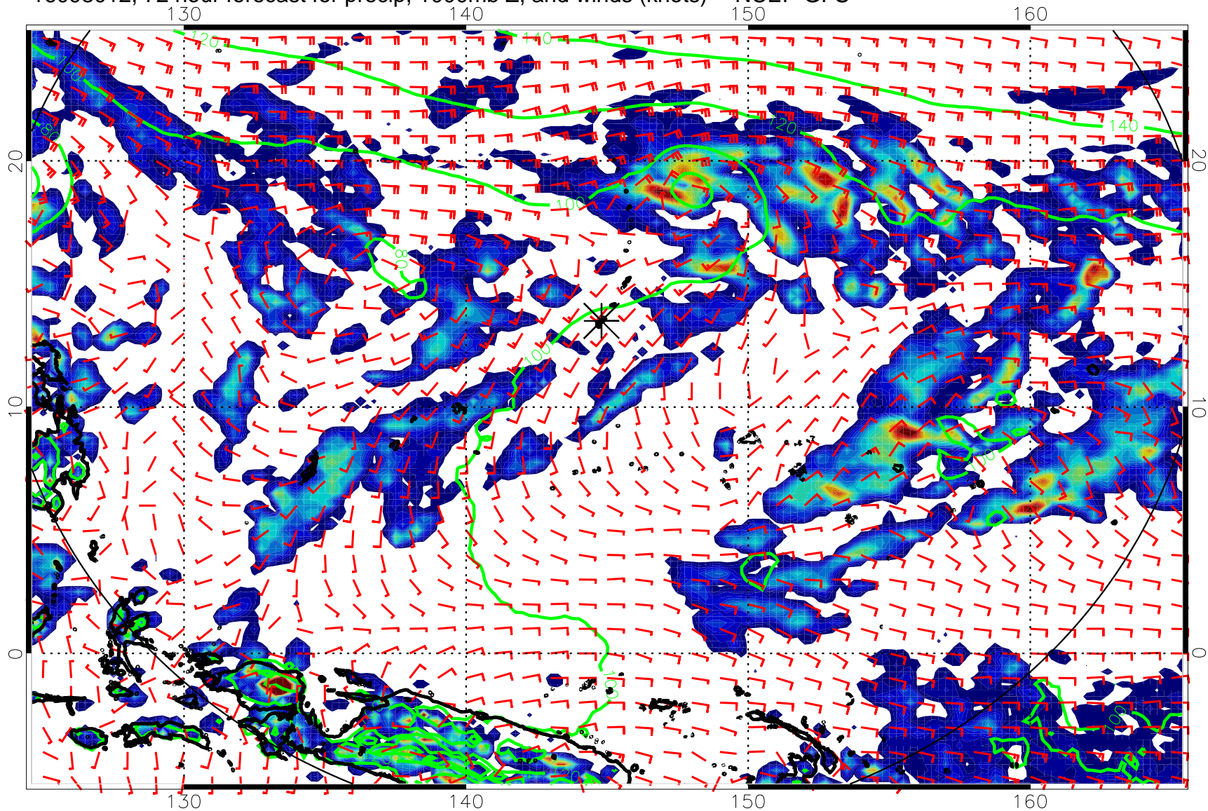
16093012, 72 hour forecast for precip, 1000mb Z, and winds (knots) -- NCEP GFS
