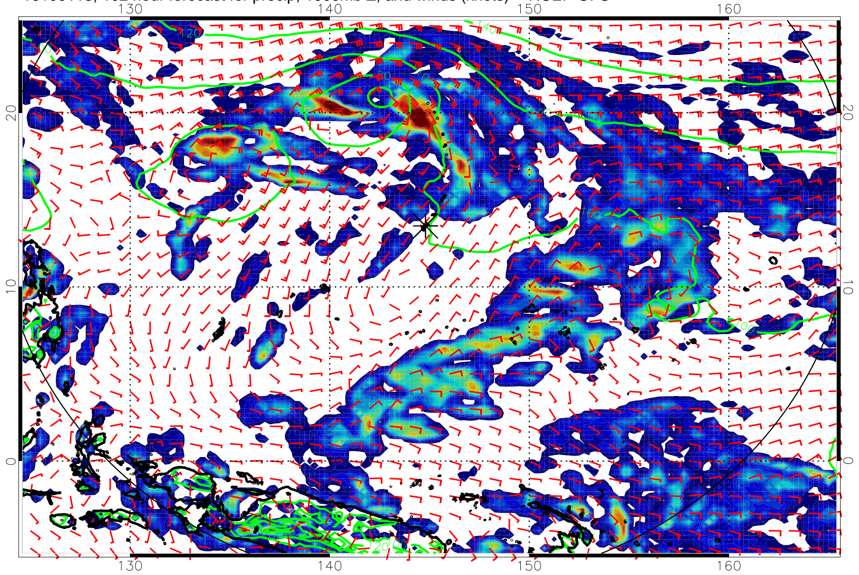
16100118, 102 hour forecast for precip, 1000mb Z, and winds (knots) -- NCEP GFS
