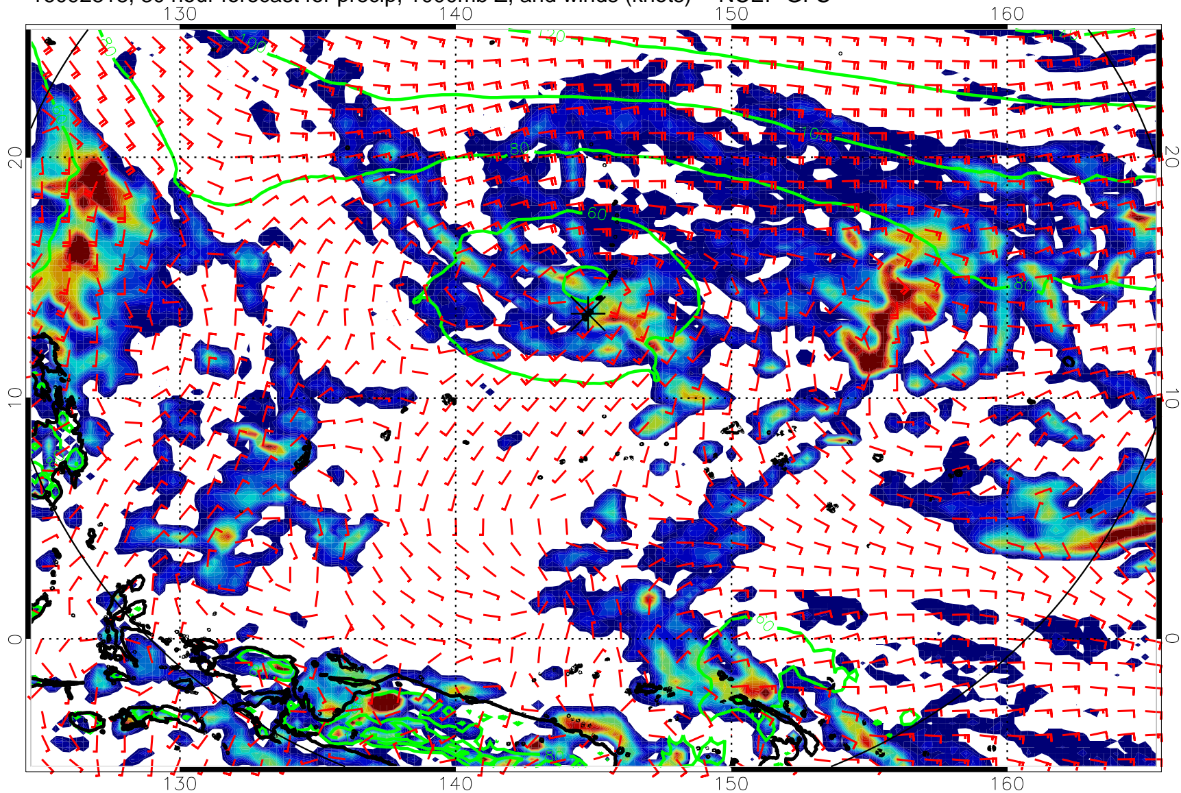
16092818, 30 hour forecast for precip, 1000mb Z, and winds (knots) -- NCEP GFS
