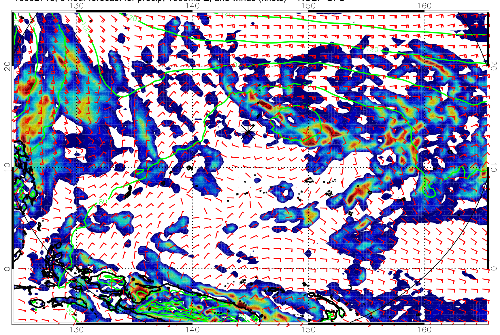
16092718, 6 hour forecast for precip, 1000mb Z, and winds (knots) -- NCEP GFS
