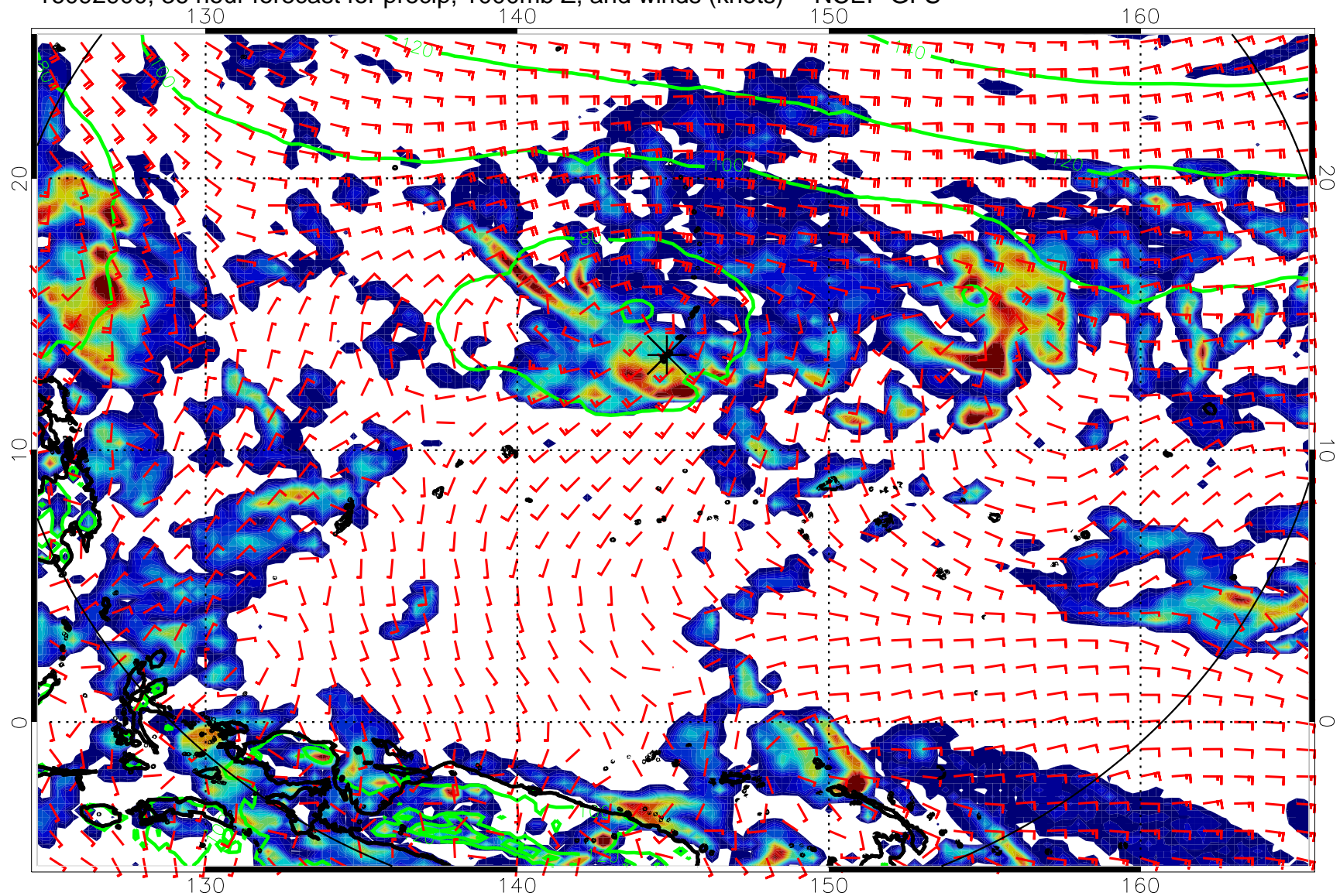
16092900, 36 hour forecast for precip, 1000mb Z, and winds (knots) -- NCEP GFS
