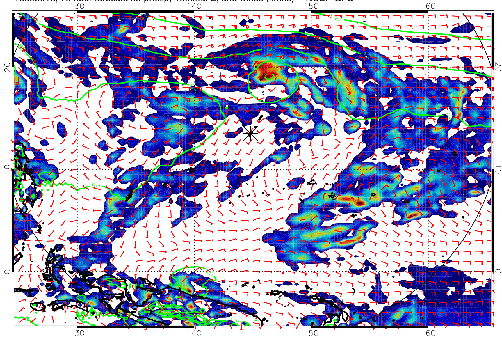
16093018, 78 hour forecast for precip, 1000mb Z, and winds (knots) -- NCEP GFS
