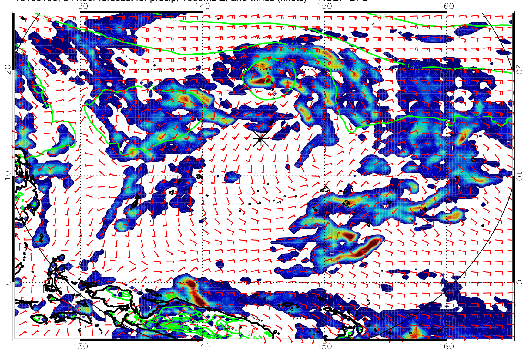
16100100, 84 hour forecast for precip, 1000mb Z, and winds (knots) -- NCEP GFS
