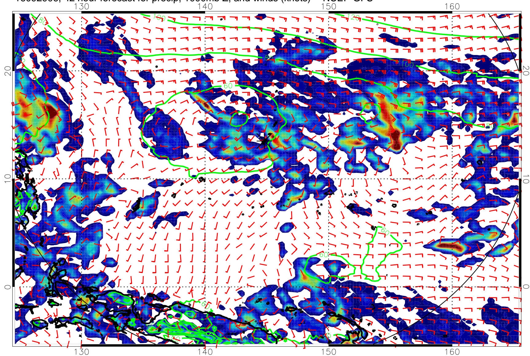
16092906, 42 hour forecast for precip, 1000mb Z, and winds (knots) -- NCEP GFS
