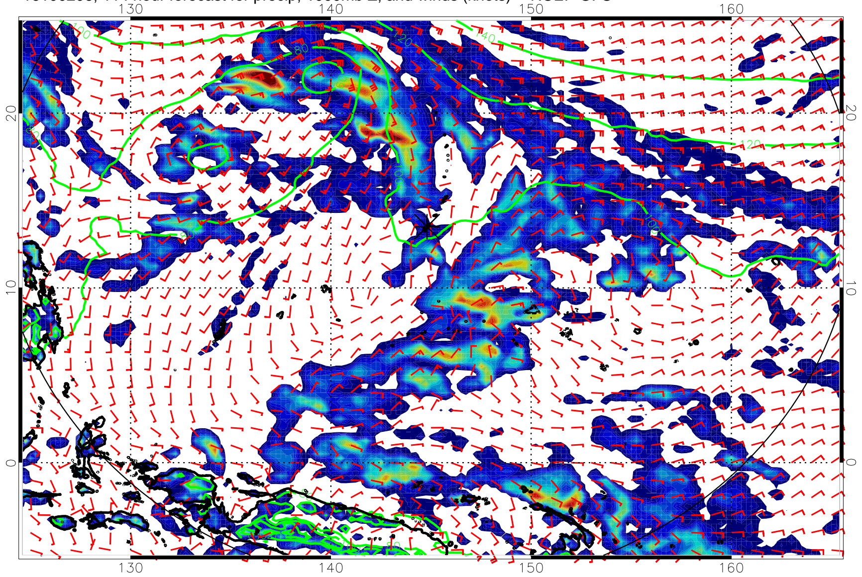
16100206, 114 hour forecast for precip, 1000mb Z, and winds (knots) -- NCEP GFS
