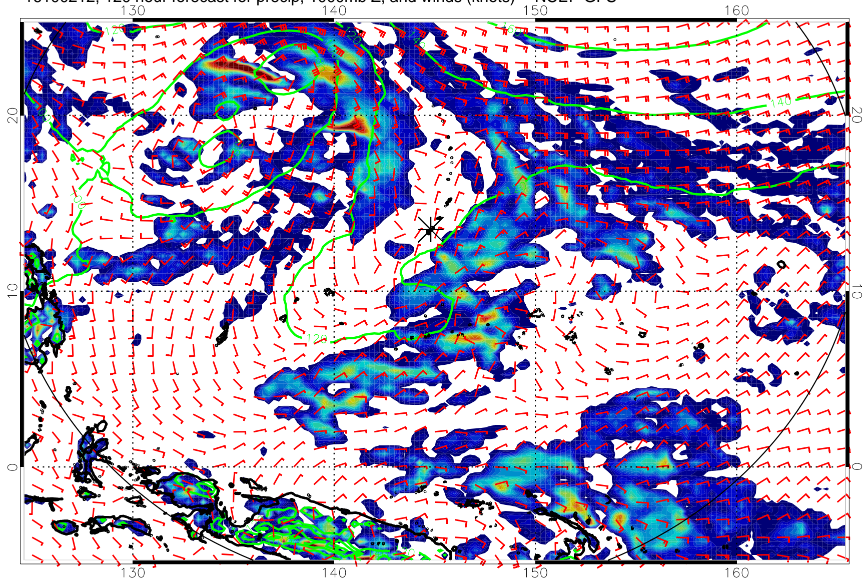
16100212, 120 hour forecast for precip, 1000mb Z, and winds (knots) -- NCEP GFS
