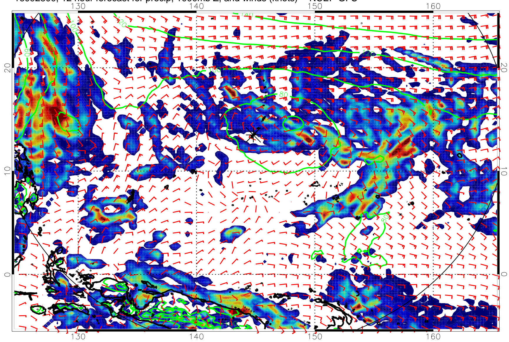
16092800, 12 hour forecast for precip, 1000mb Z, and winds (knots) -- NCEP GFS
