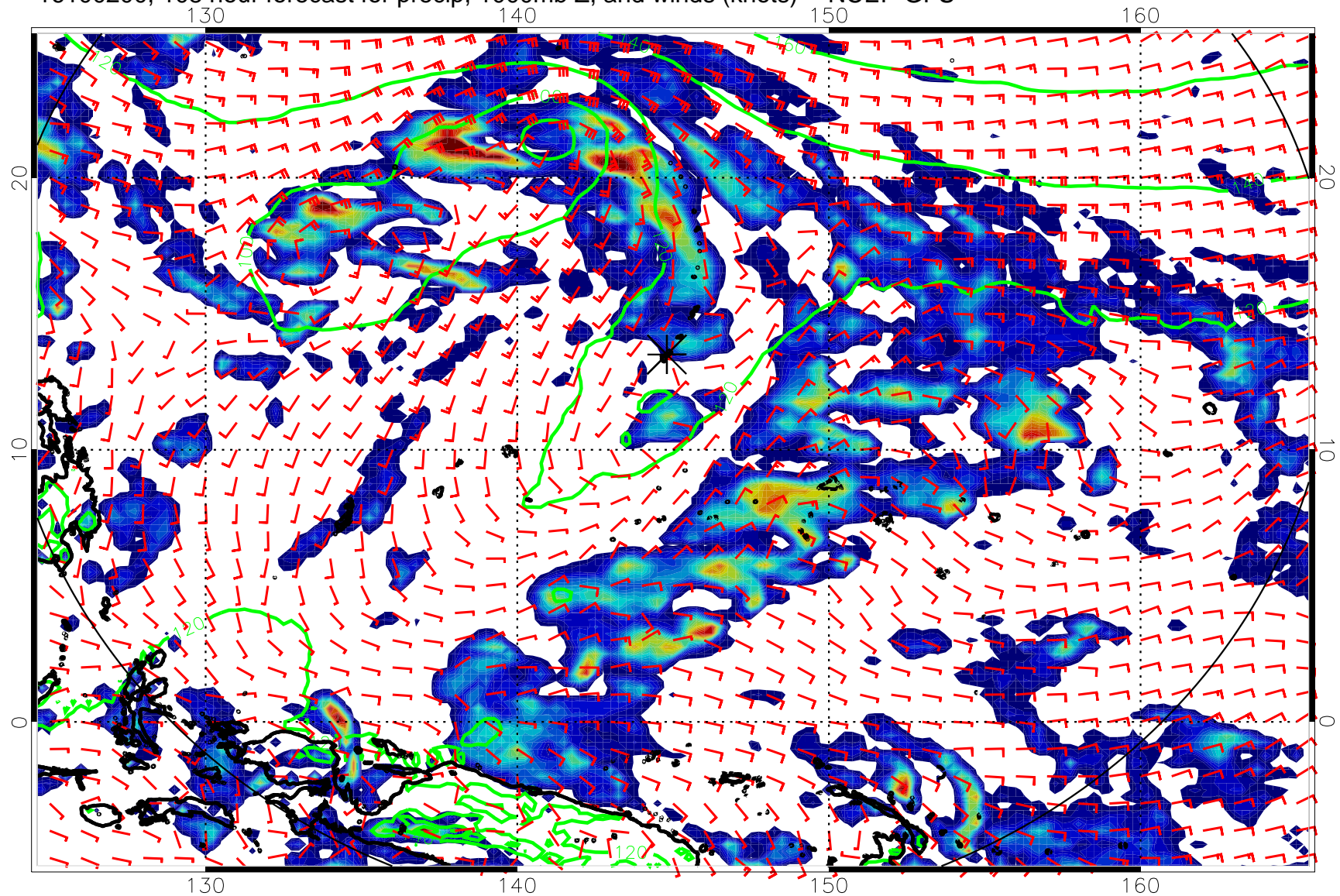
16100200, 108 hour forecast for precip, 1000mb Z, and winds (knots) -- NCEP GFS
