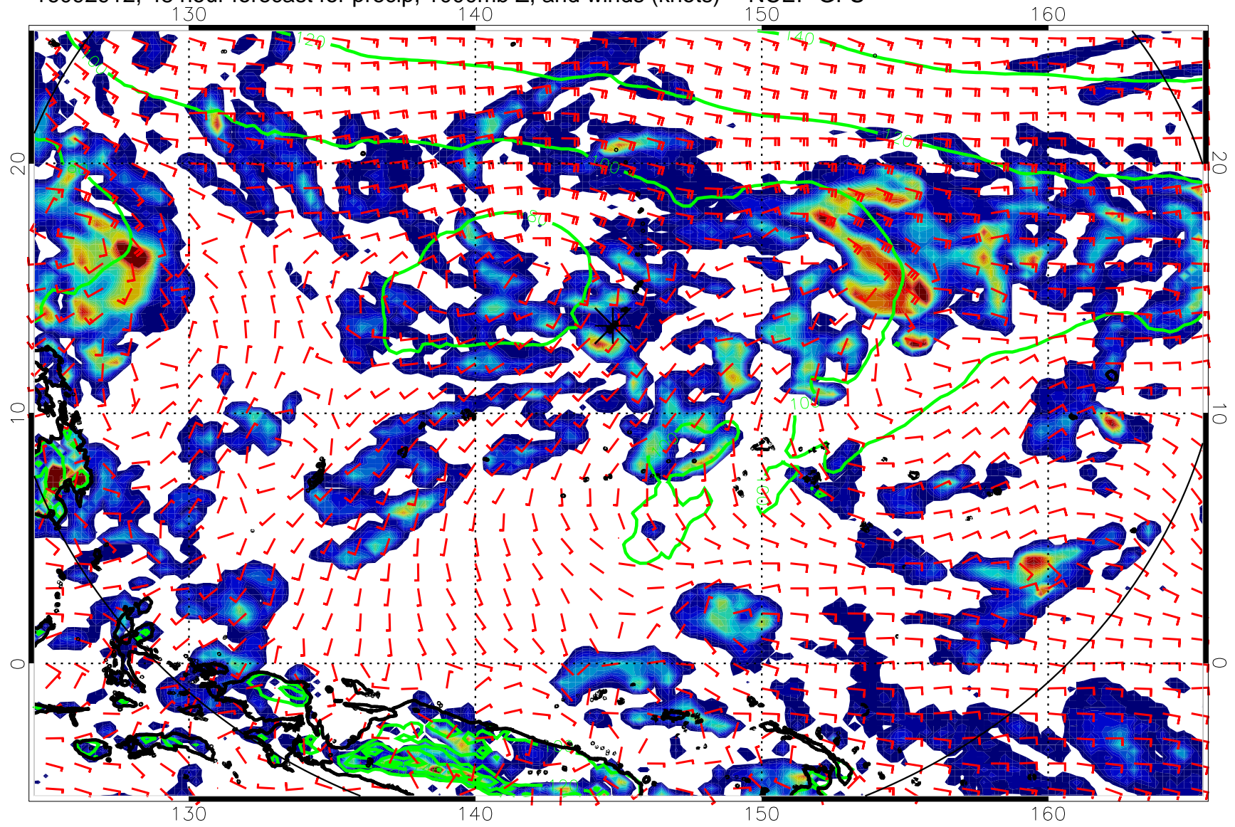
16092912, 48 hour forecast for precip, 1000mb Z, and winds (knots) -- NCEP GFS
