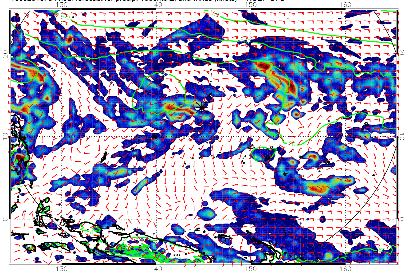
16092918, 54 hour forecast for precip, 1000mb Z, and winds (knots) -- NCEP GFS
