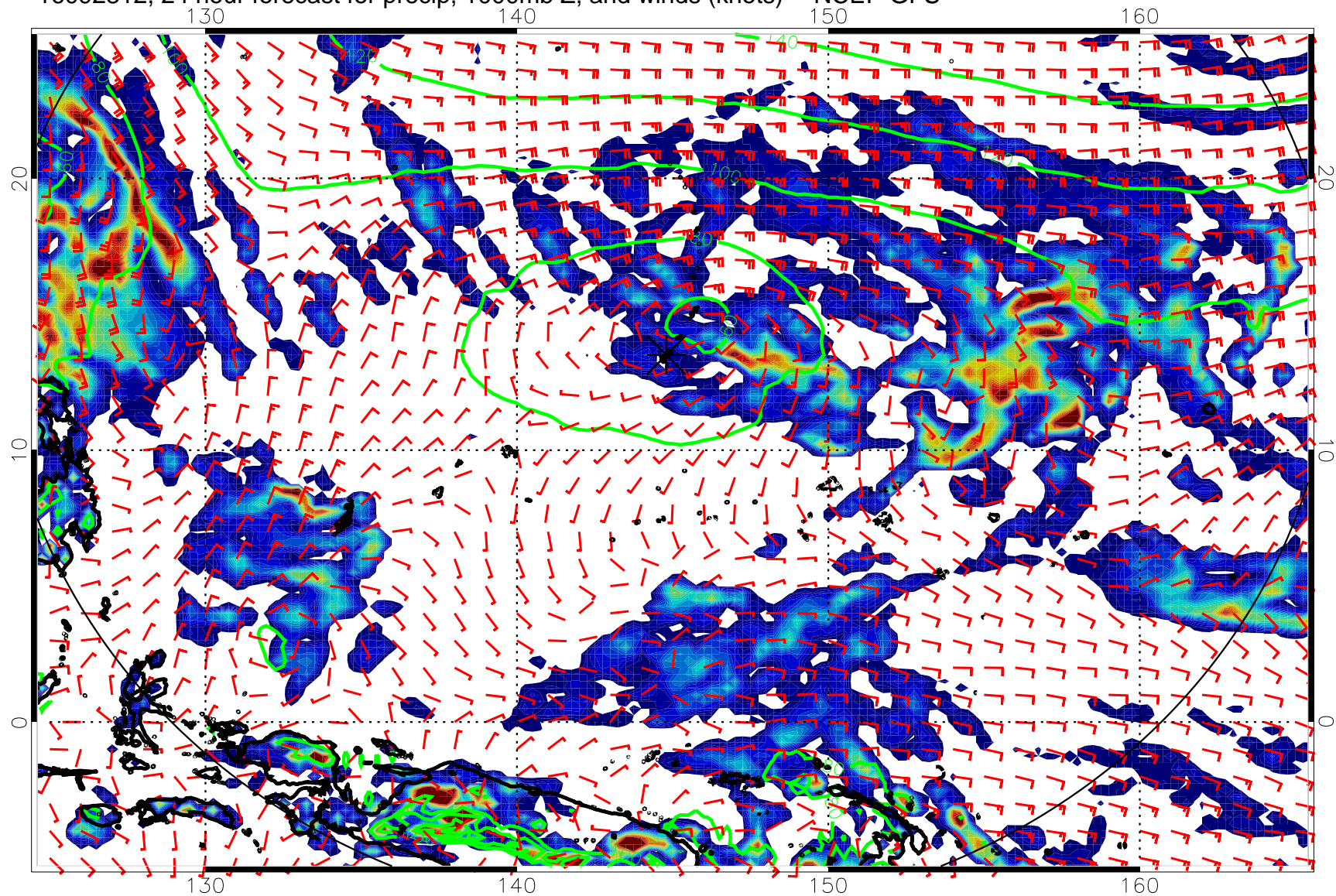
16092812, 24 hour forecast for precip, 1000mb Z, and winds (knots) -- NCEP GFS
