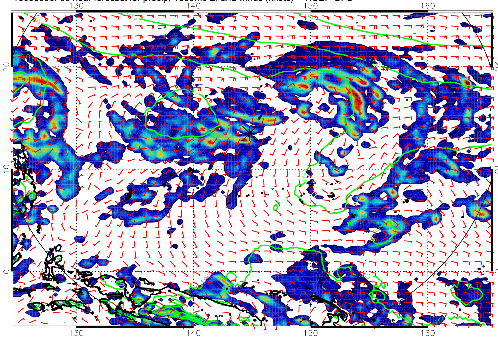
16093000, 60 hour forecast for precip, 1000mb Z, and winds (knots) -- NCEP GFS
