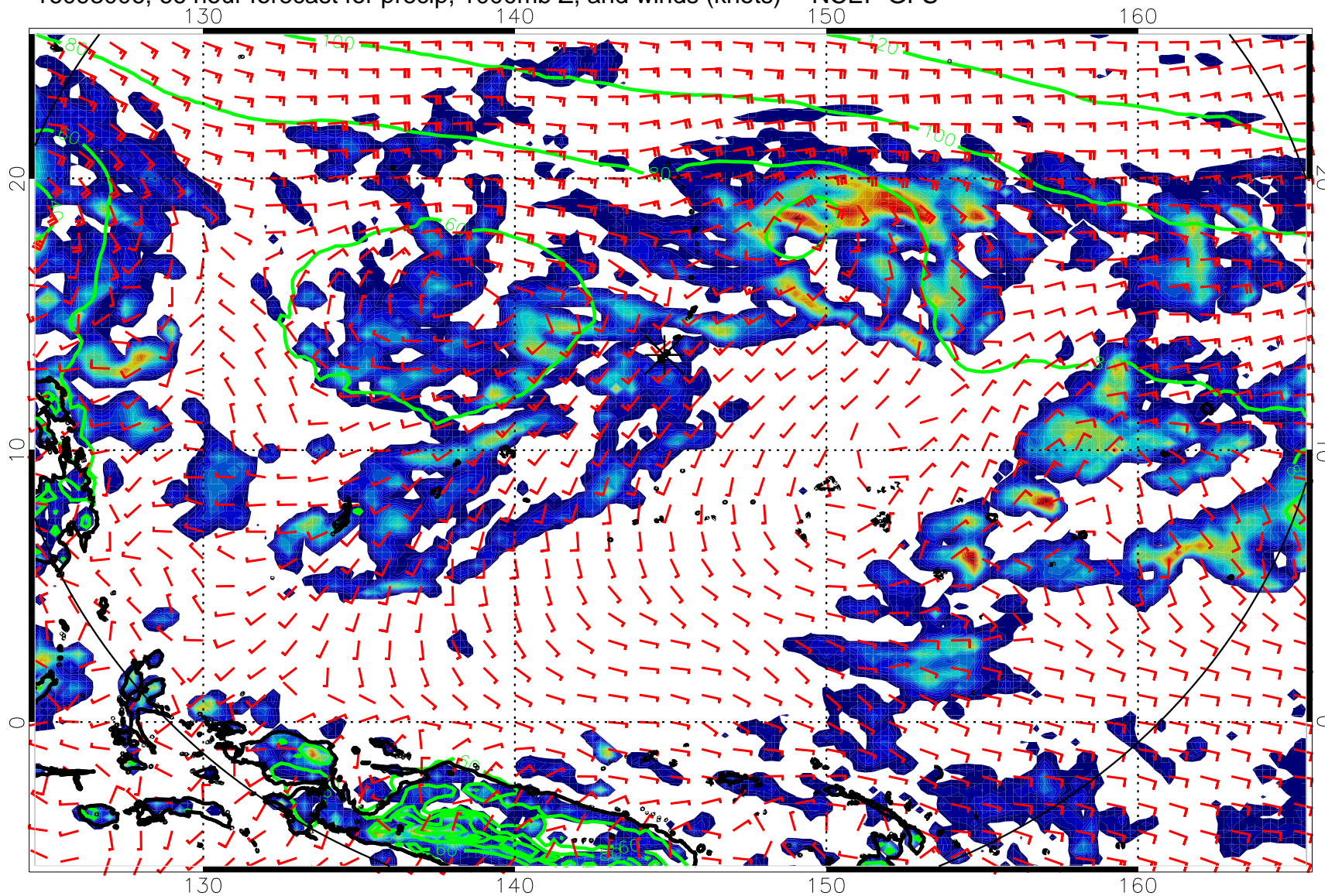
16093006, 66 hour forecast for precip, 1000mb Z, and winds (knots) -- NCEP GFS
