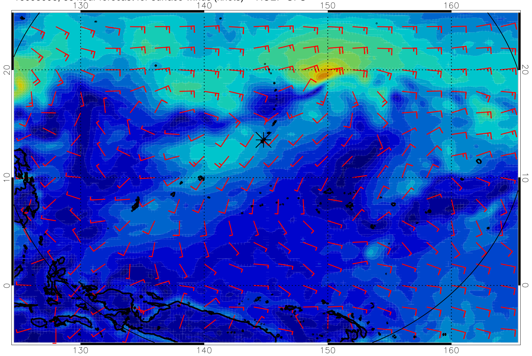
16093006, 66 hour forecast for surface winds (knots) -- NCEP GFS
