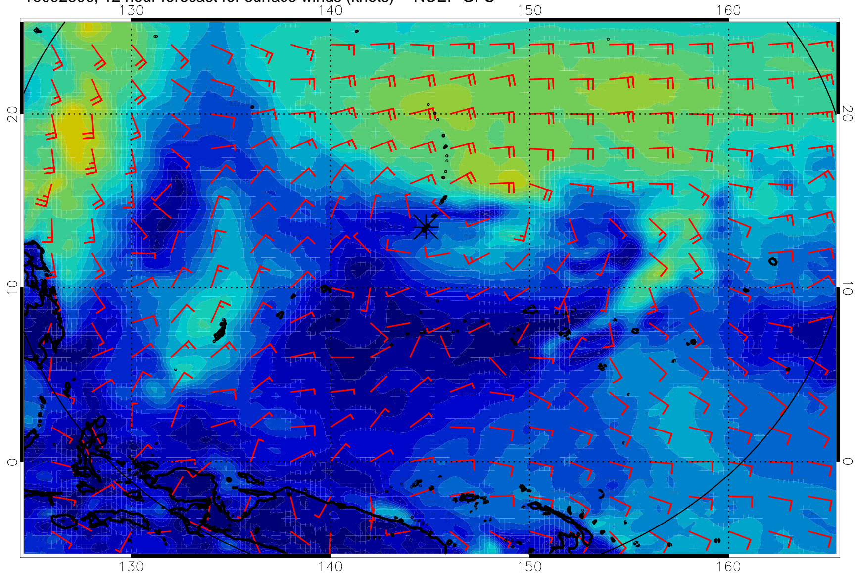
16092800, 12 hour forecast for surface winds (knots) -- NCEP GFS
