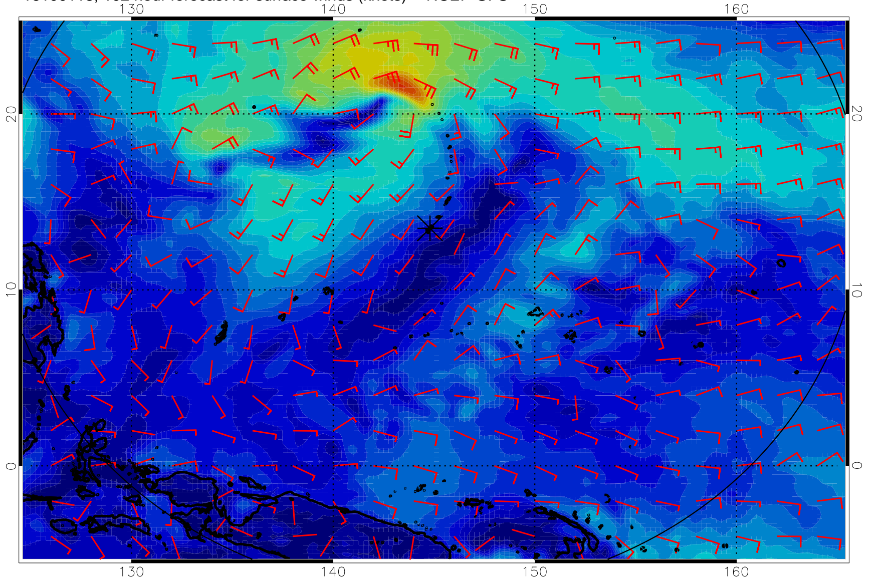
16100118, 102 hour forecast for surface winds (knots) -- NCEP GFS
