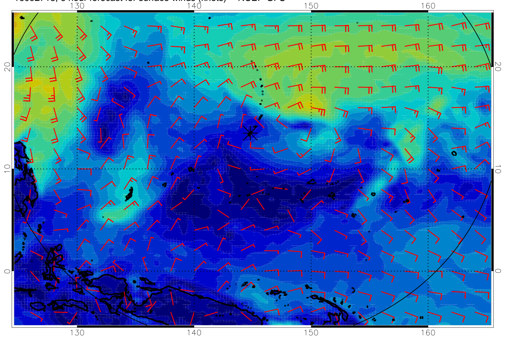
16092718, 6 hour forecast for surface winds (knots) -- NCEP GFS
