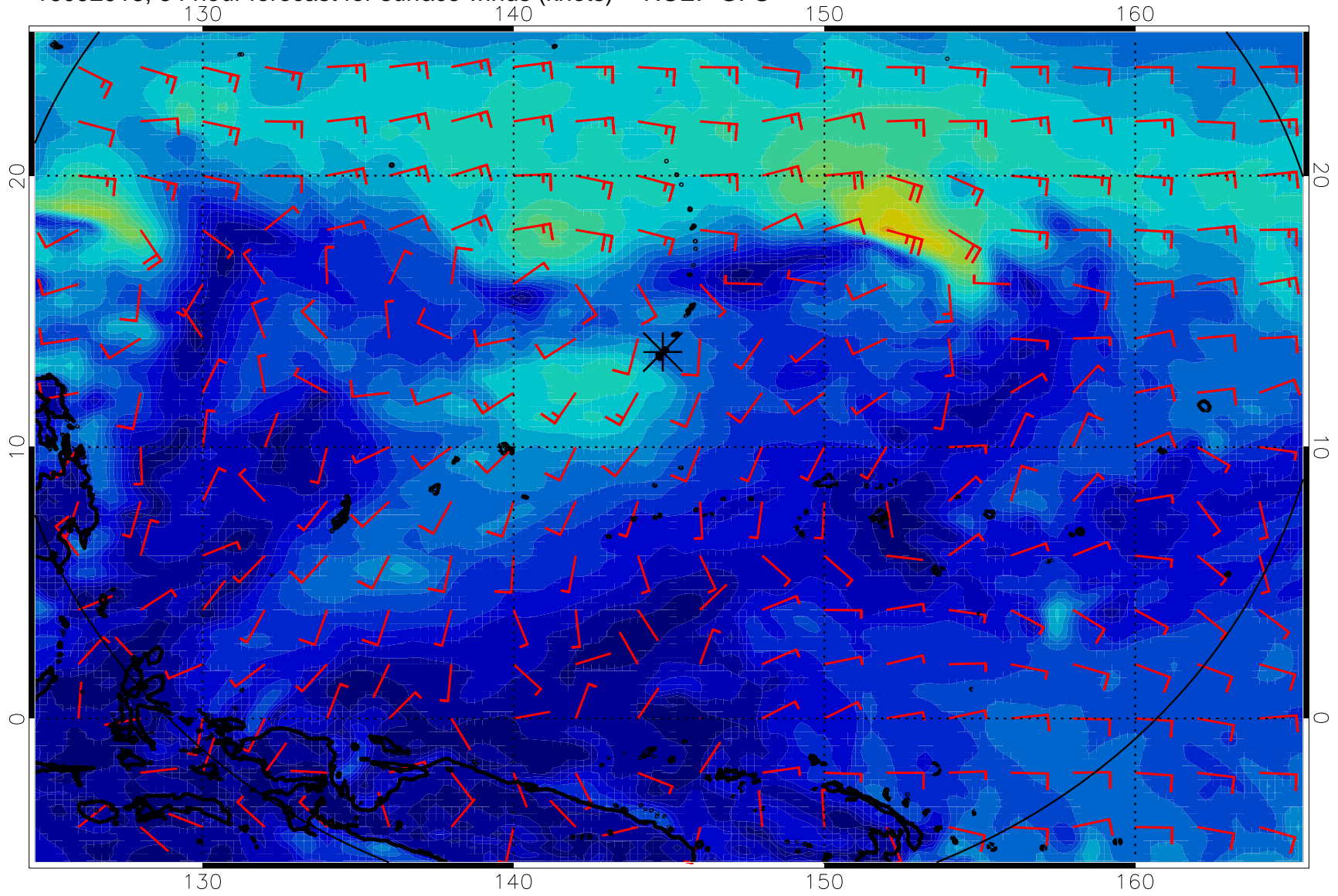
16092918, 54 hour forecast for surface winds (knots) -- NCEP GFS
