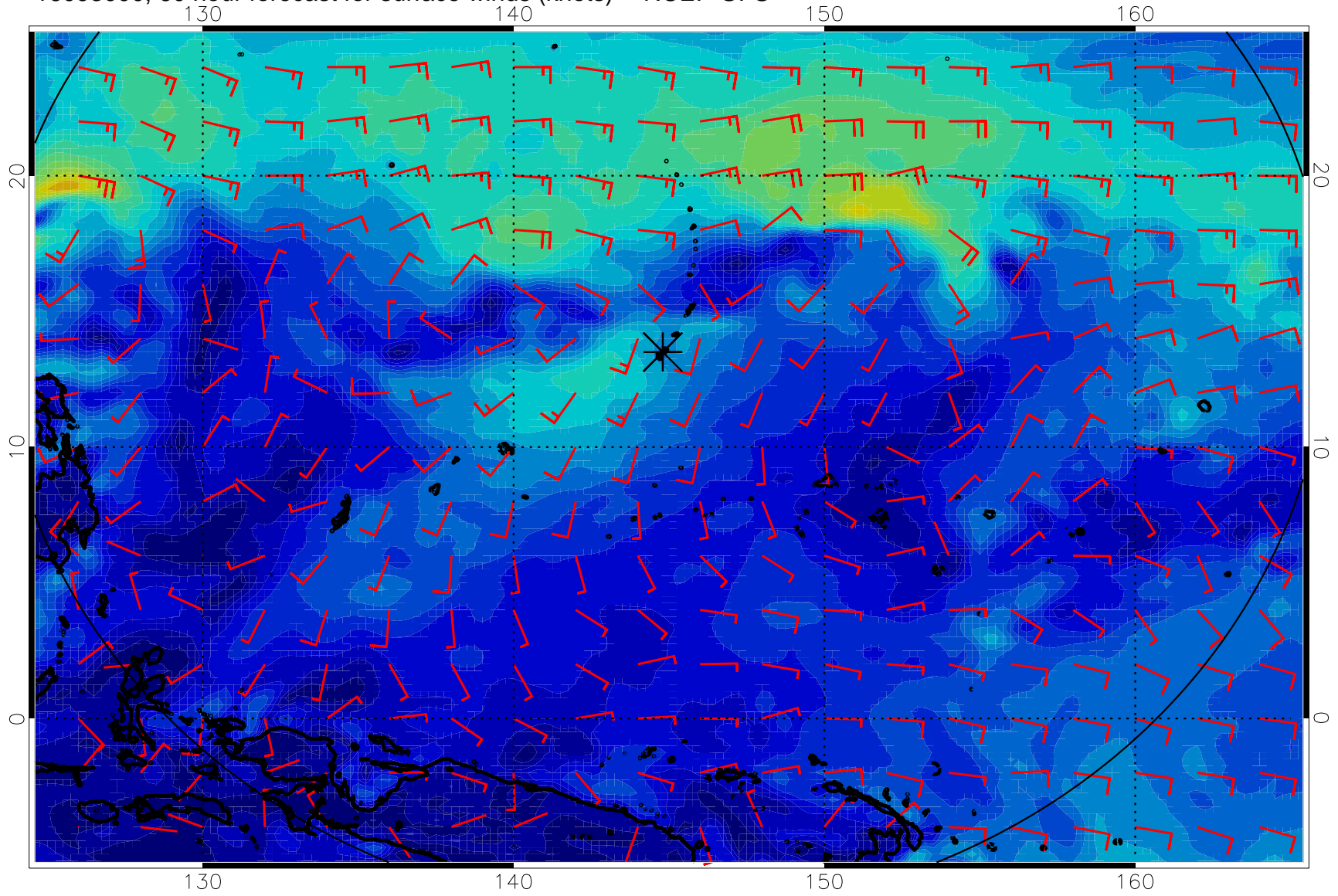
16093000, 60 hour forecast for surface winds (knots) -- NCEP GFS
