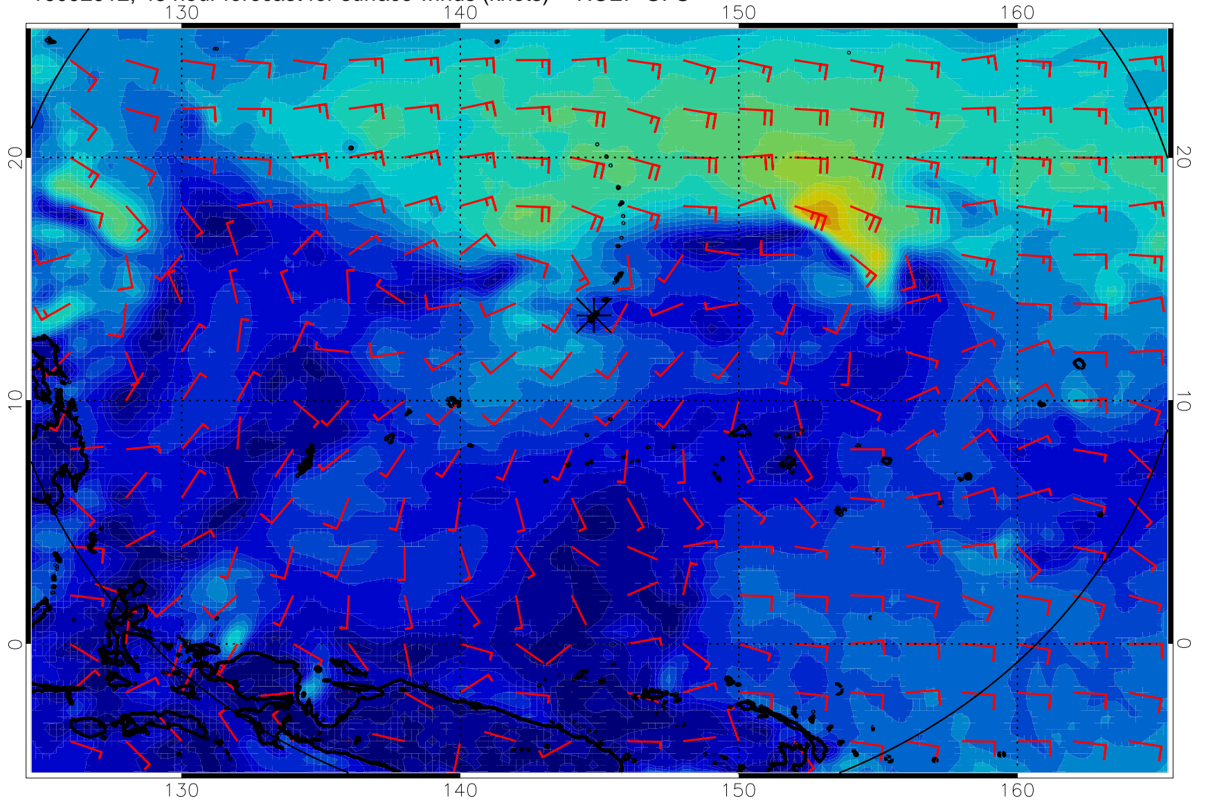
16092912, 48 hour forecast for surface winds (knots) -- NCEP GFS
