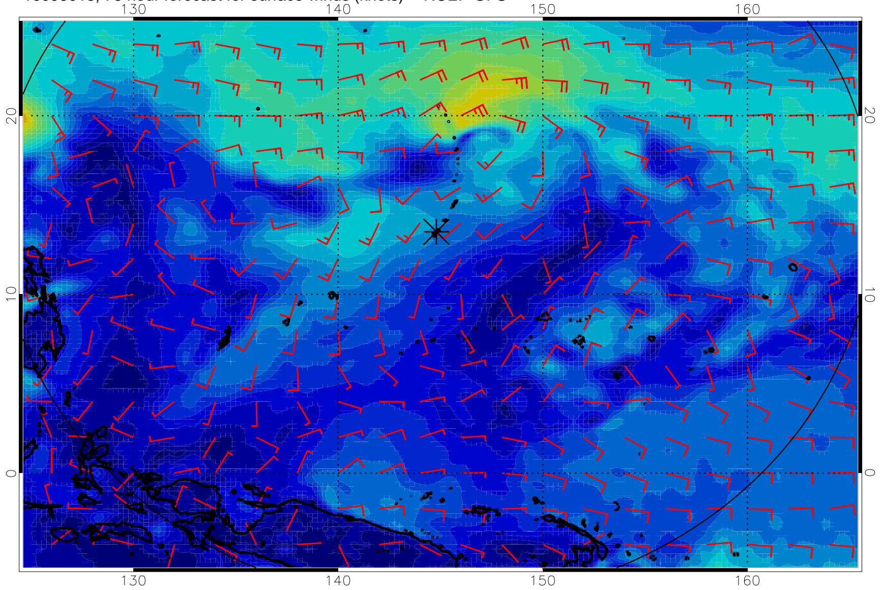
16093018, 78 hour forecast for surface winds (knots) -- NCEP GFS
