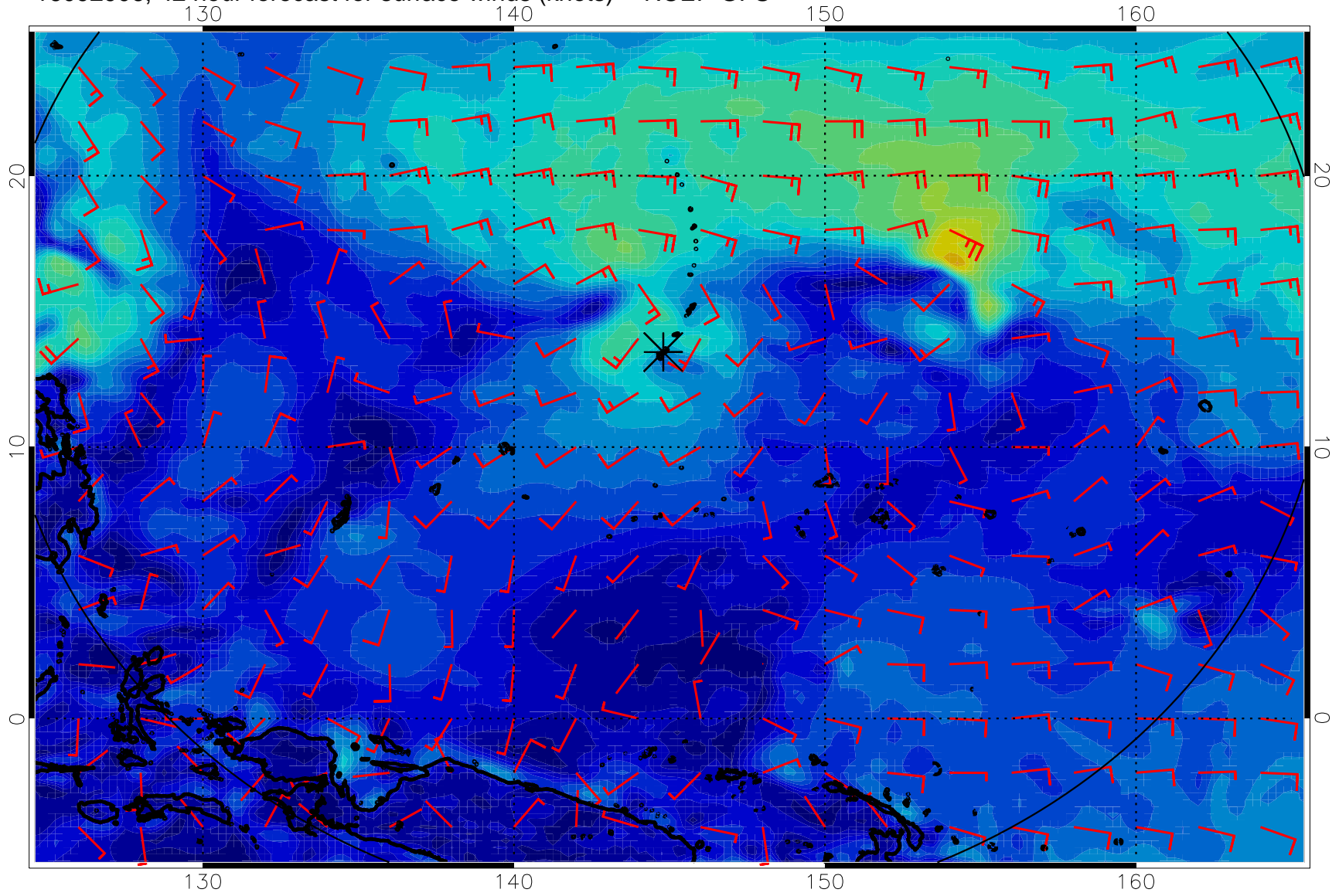
16092906, 42 hour forecast for surface winds (knots) -- NCEP GFS
