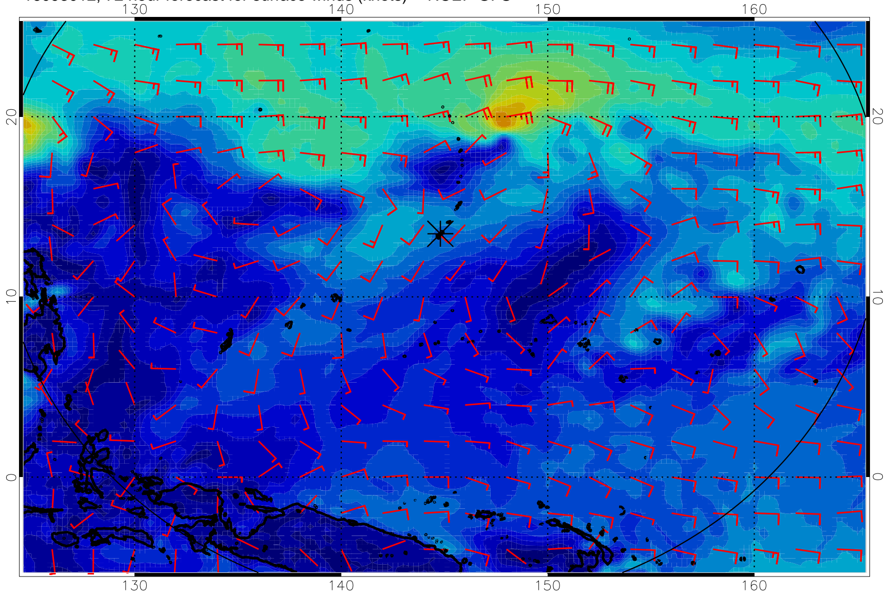
16093012, 72 hour forecast for surface winds (knots) -- NCEP GFS
