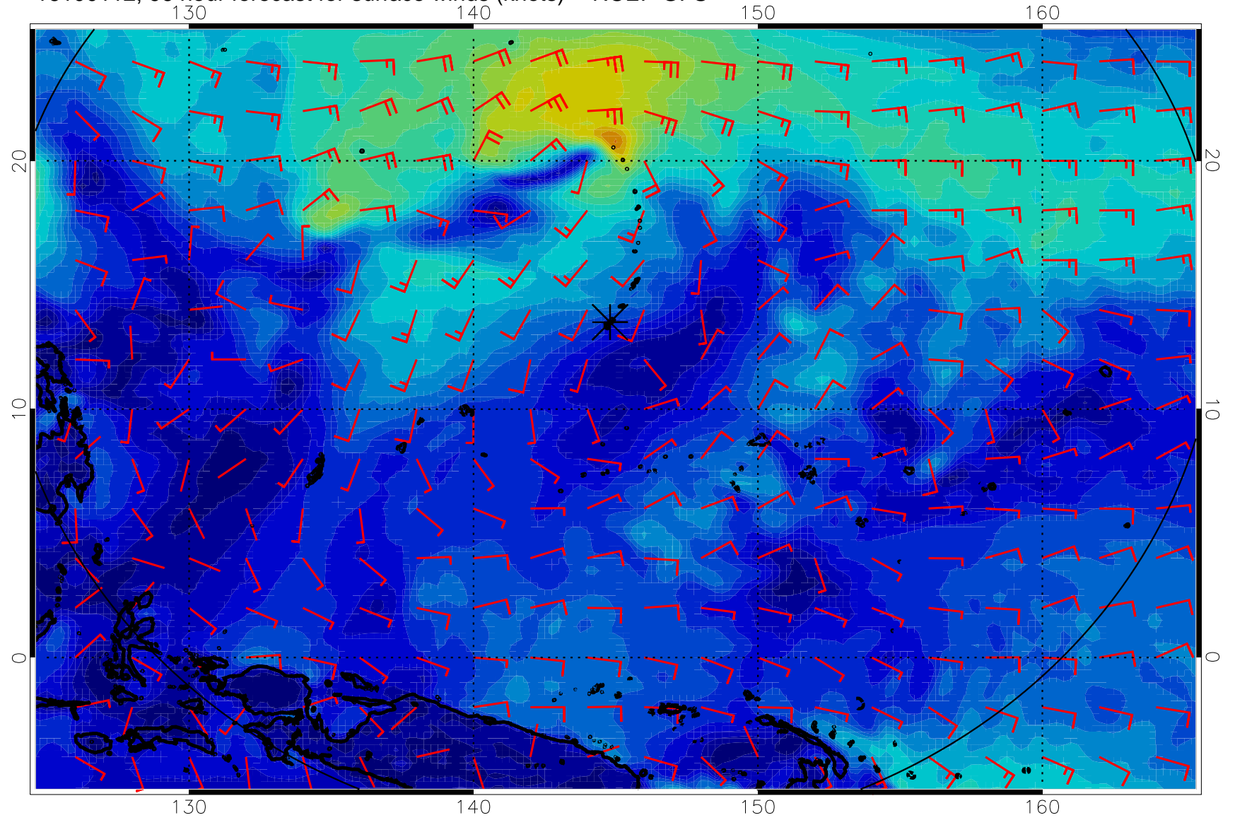
16100112, 96 hour forecast for surface winds (knots) -- NCEP GFS
