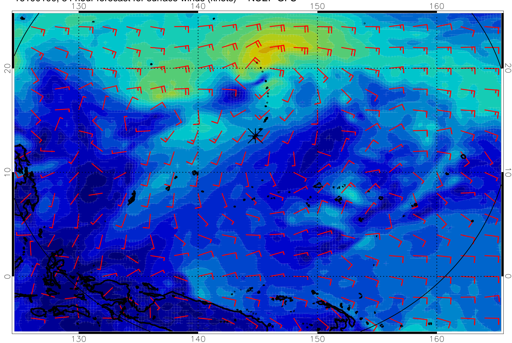
16100100, 84 hour forecast for surface winds (knots) -- NCEP GFS
