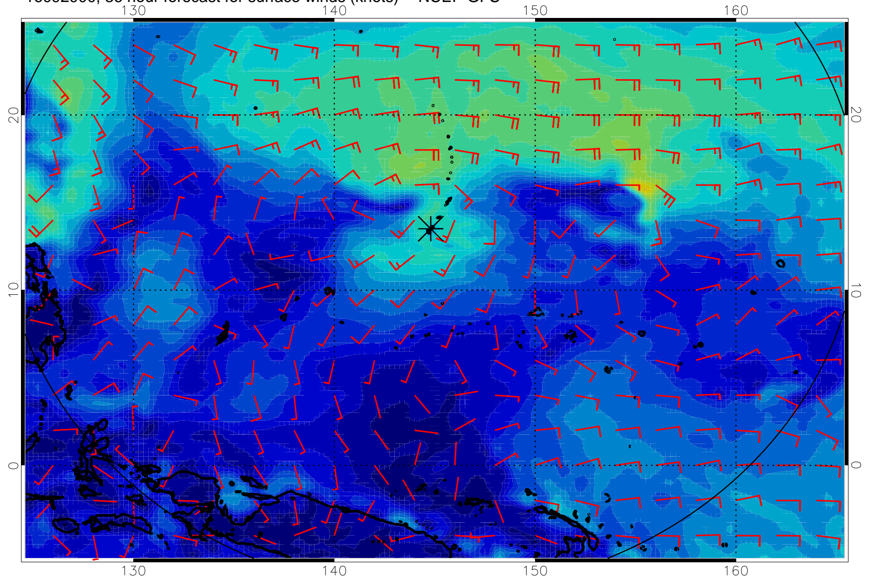
16092900, 36 hour forecast for surface winds (knots) -- NCEP GFS
