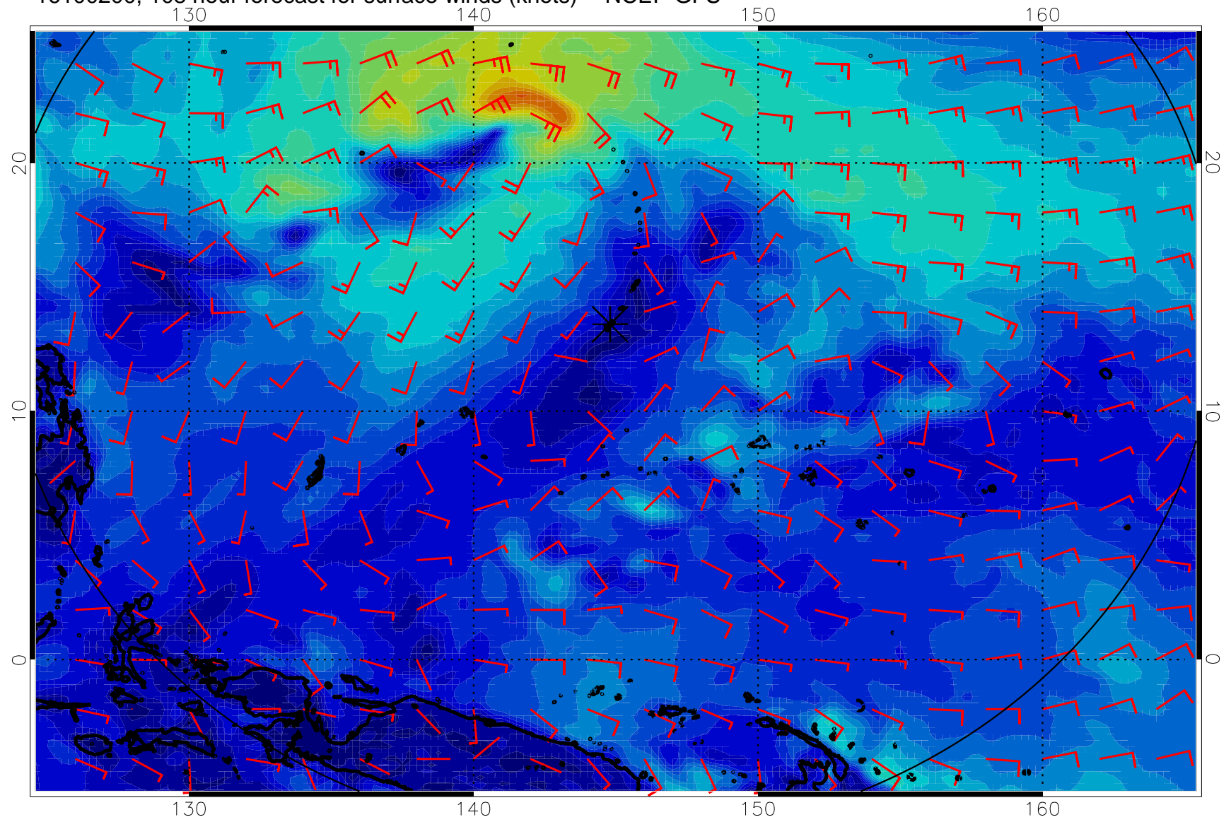
16100200, 108 hour forecast for surface winds (knots) -- NCEP GFS
