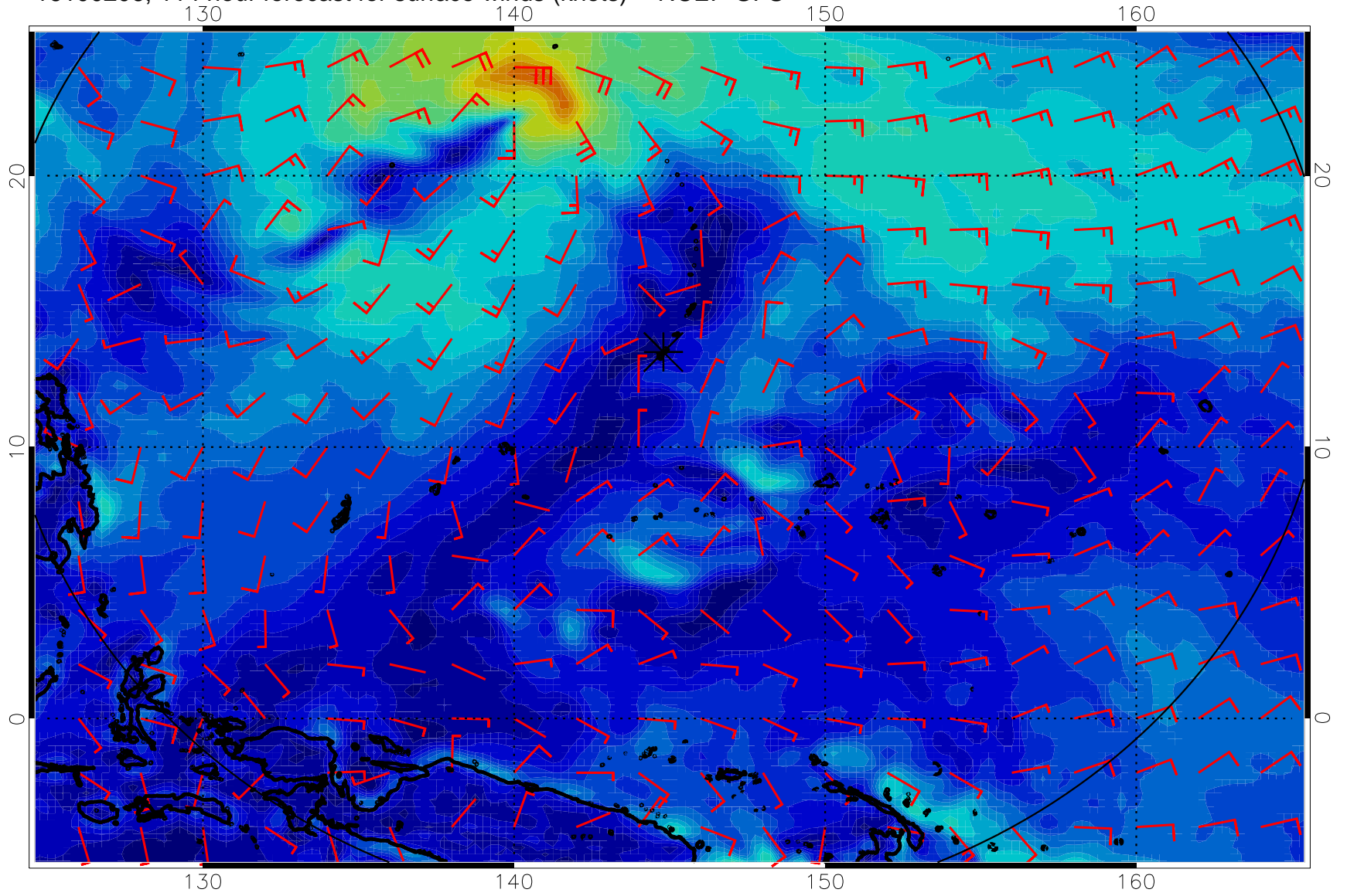
16100206, 114 hour forecast for surface winds (knots) -- NCEP GFS
