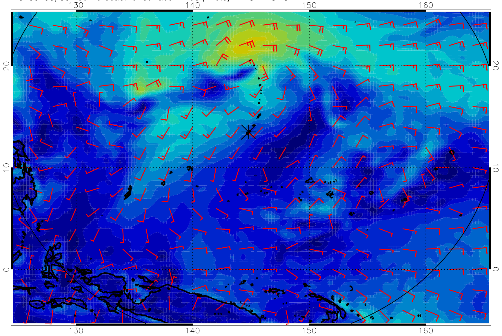
16100106, 90 hour forecast for surface winds (knots) -- NCEP GFS
