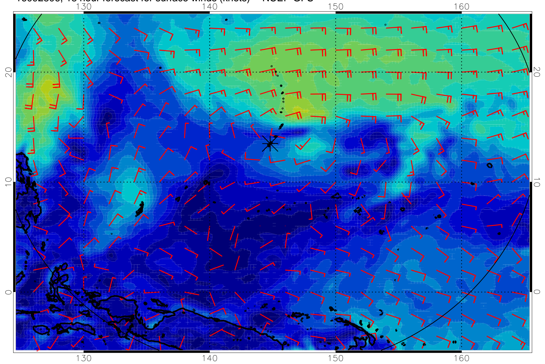
16092806, 18 hour forecast for surface winds (knots) -- NCEP GFS
