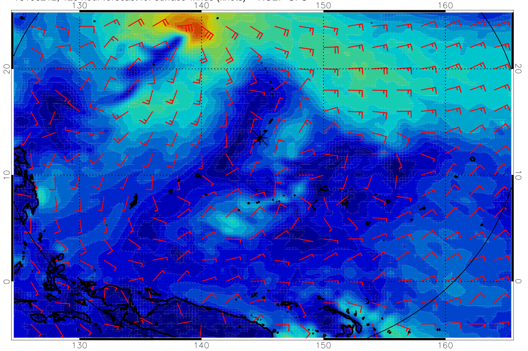
16100212, 120 hour forecast for surface winds (knots) -- NCEP GFS
