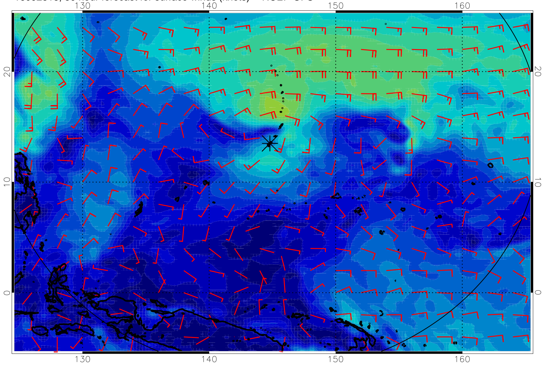
16092818, 30 hour forecast for surface winds (knots) -- NCEP GFS
