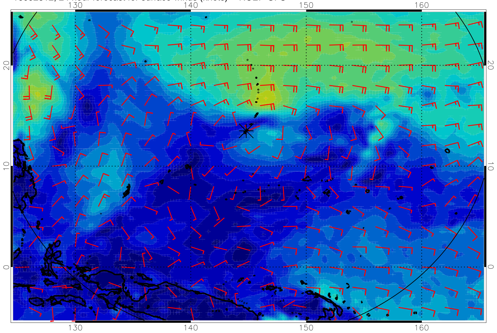
16092812, 24 hour forecast for surface winds (knots) -- NCEP GFS
