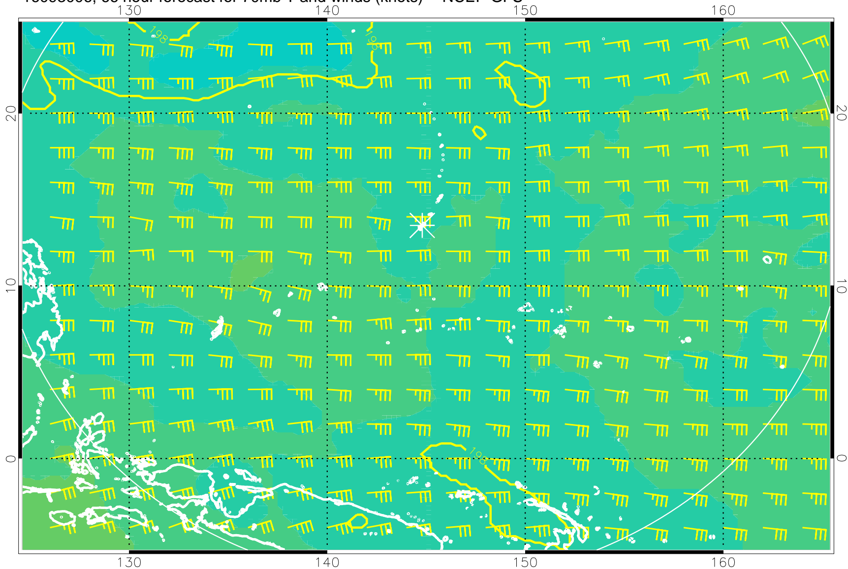
16093006, 66 hour forecast for 70mb T and winds (knots) -- NCEP GFS
