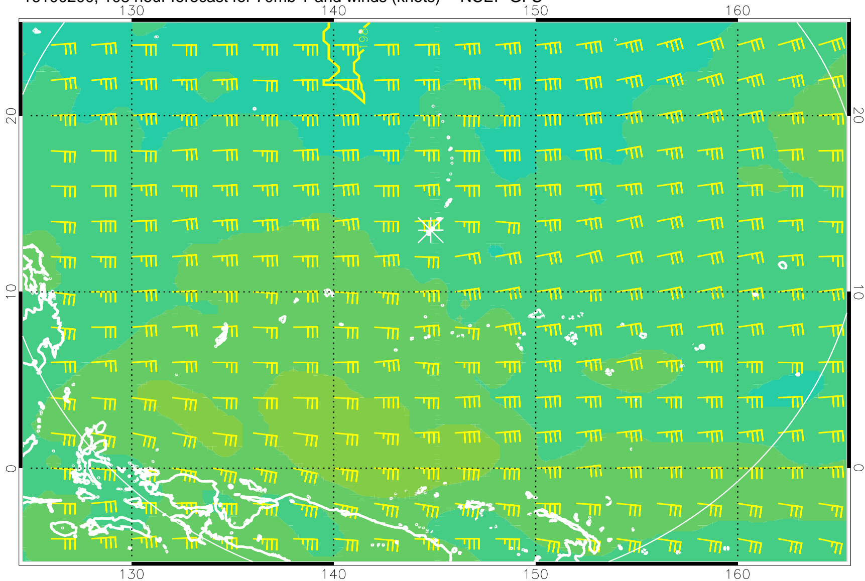
16100200, 108 hour forecast for 70mb T and winds (knots) -- NCEP GFS
