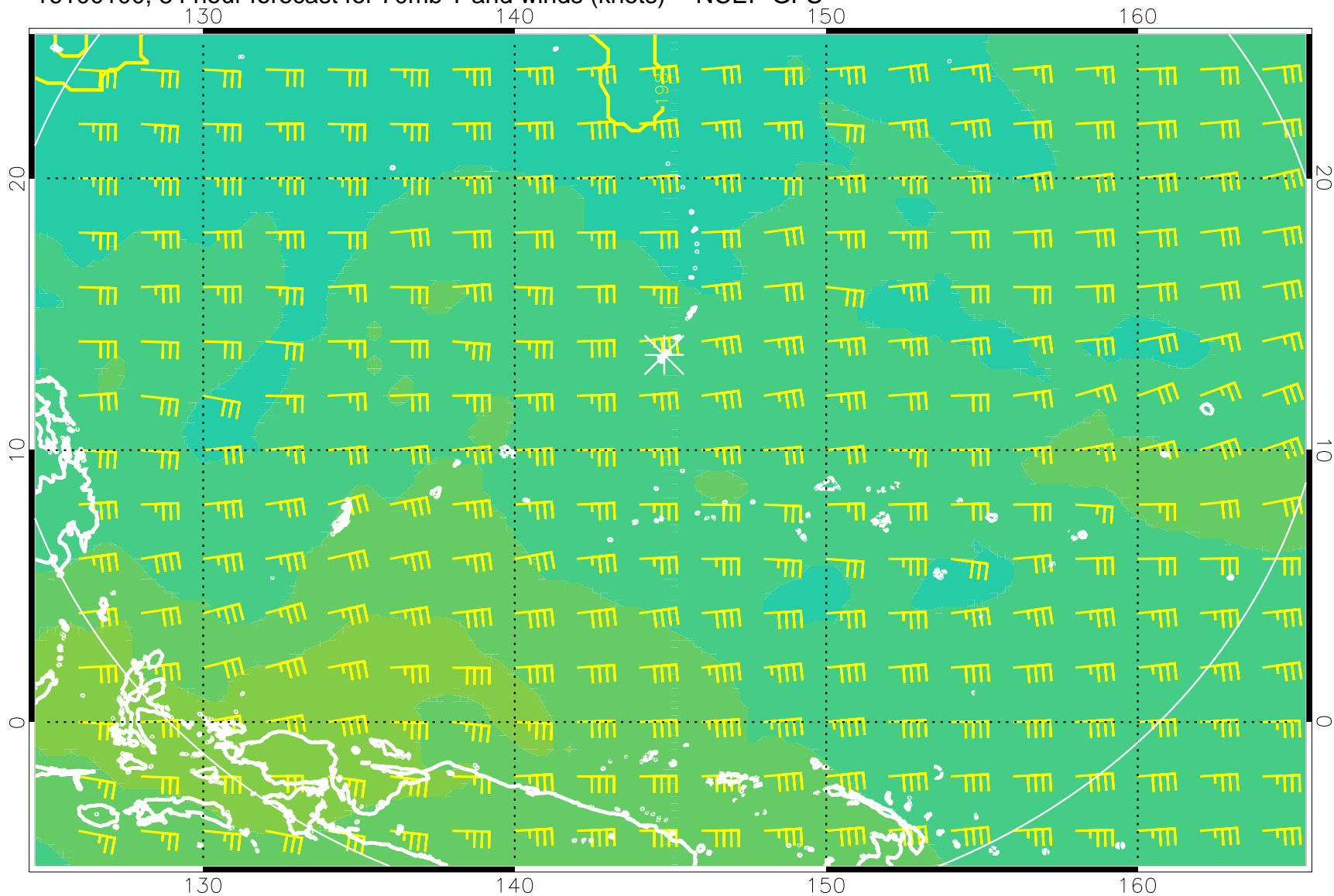
16100100, 84 hour forecast for 70mb T and winds (knots) -- NCEP GFS
