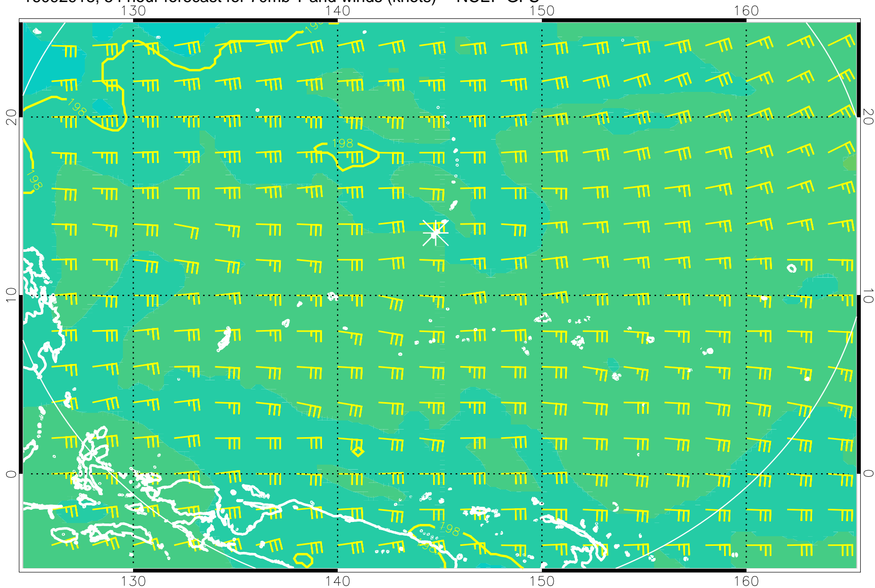
16092918, 54 hour forecast for 70mb T and winds (knots) -- NCEP GFS
