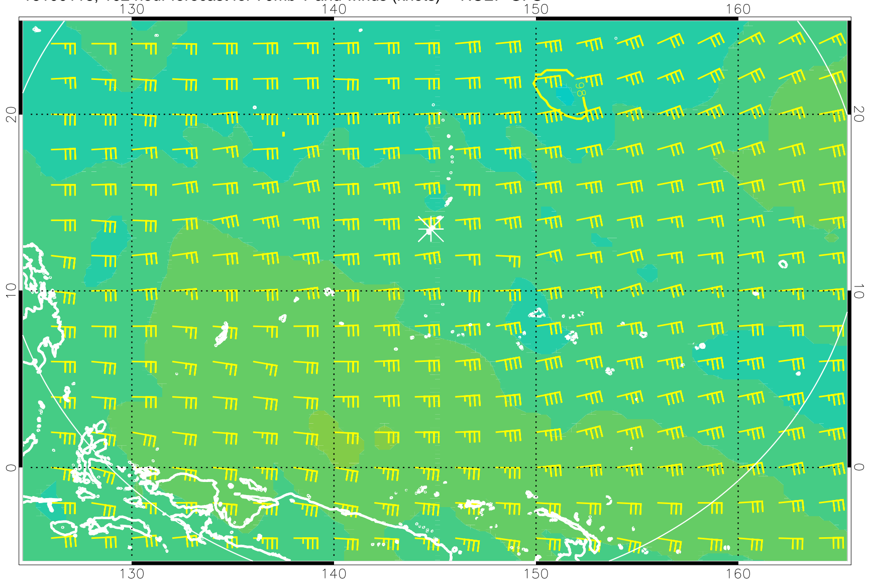
16100118, 102 hour forecast for 70mb T and winds (knots) -- NCEP GFS
