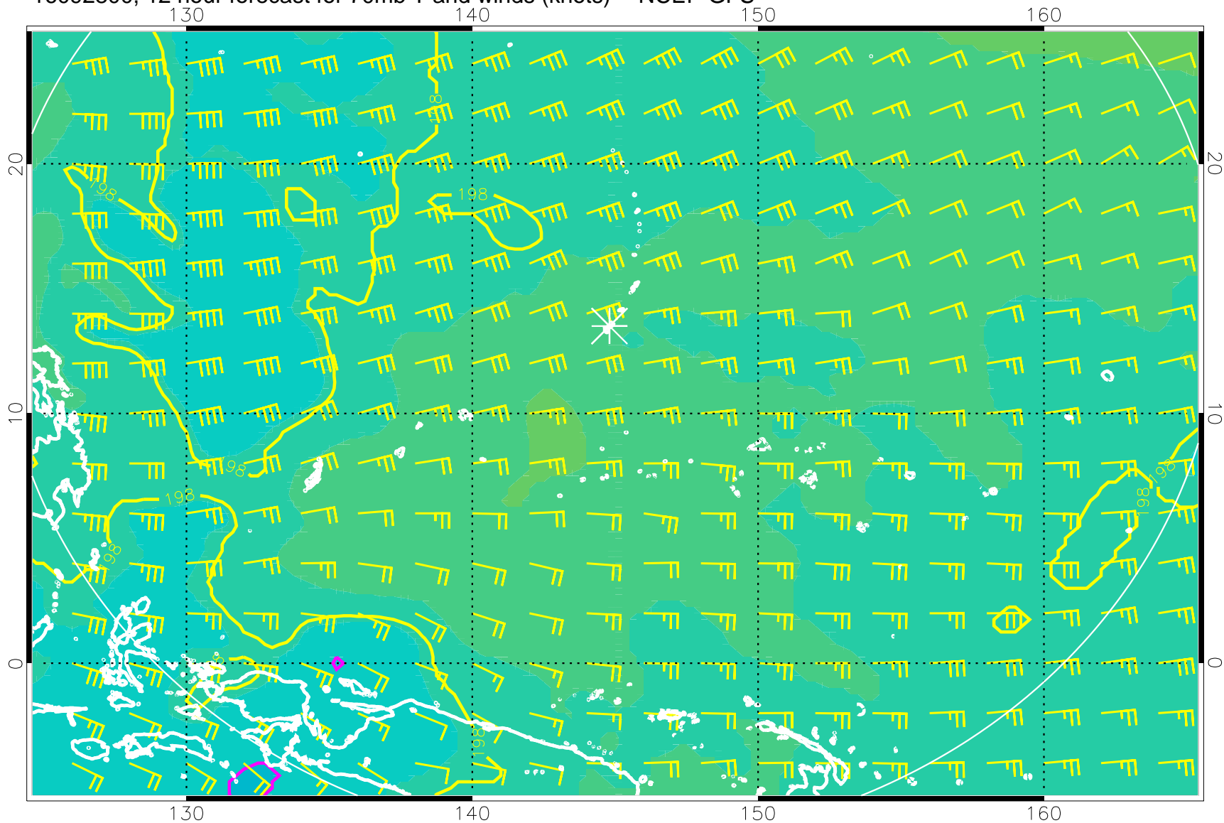
16092800, 12 hour forecast for 70mb T and winds (knots) -- NCEP GFS
