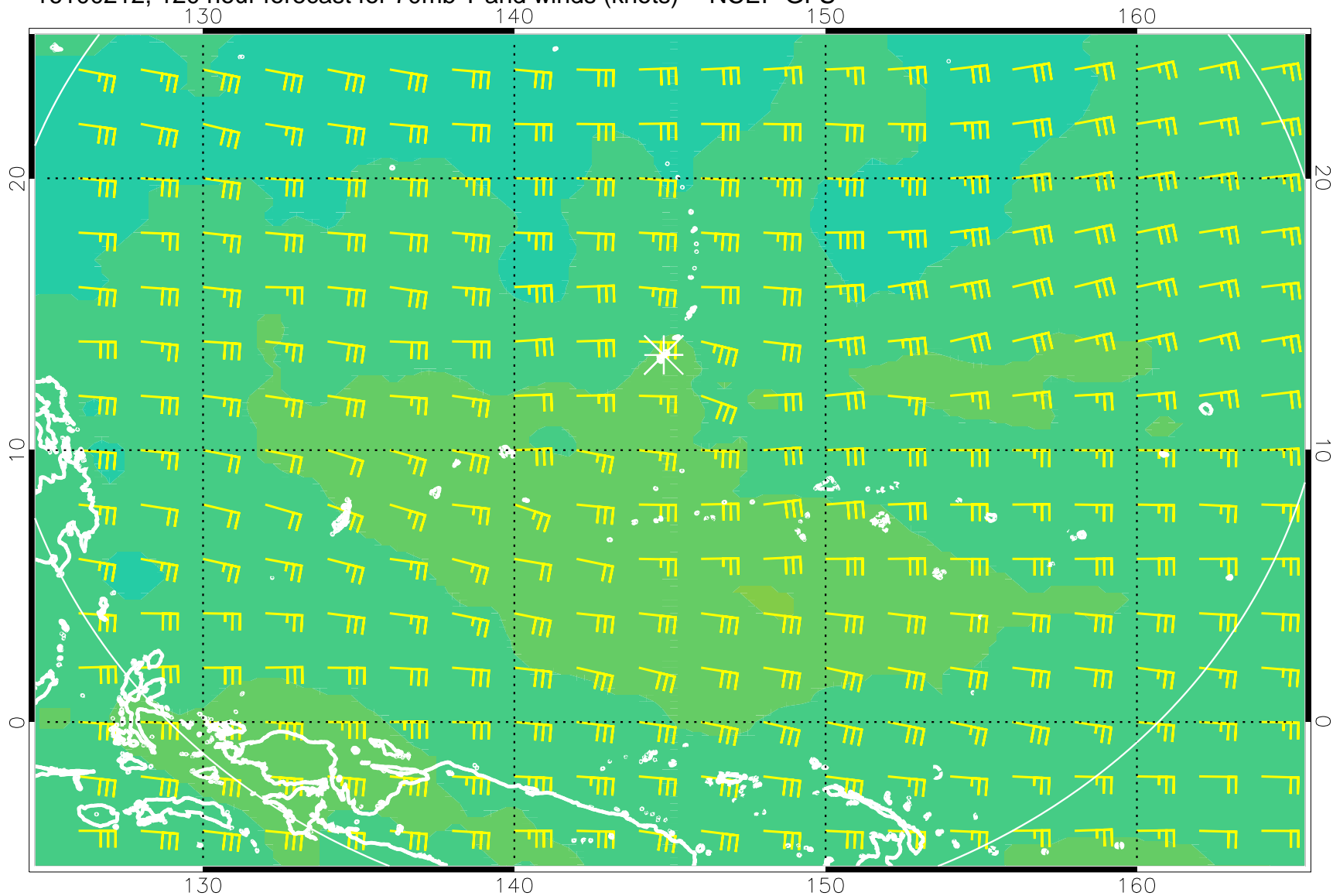
16100212, 120 hour forecast for 70mb T and winds (knots) -- NCEP GFS
