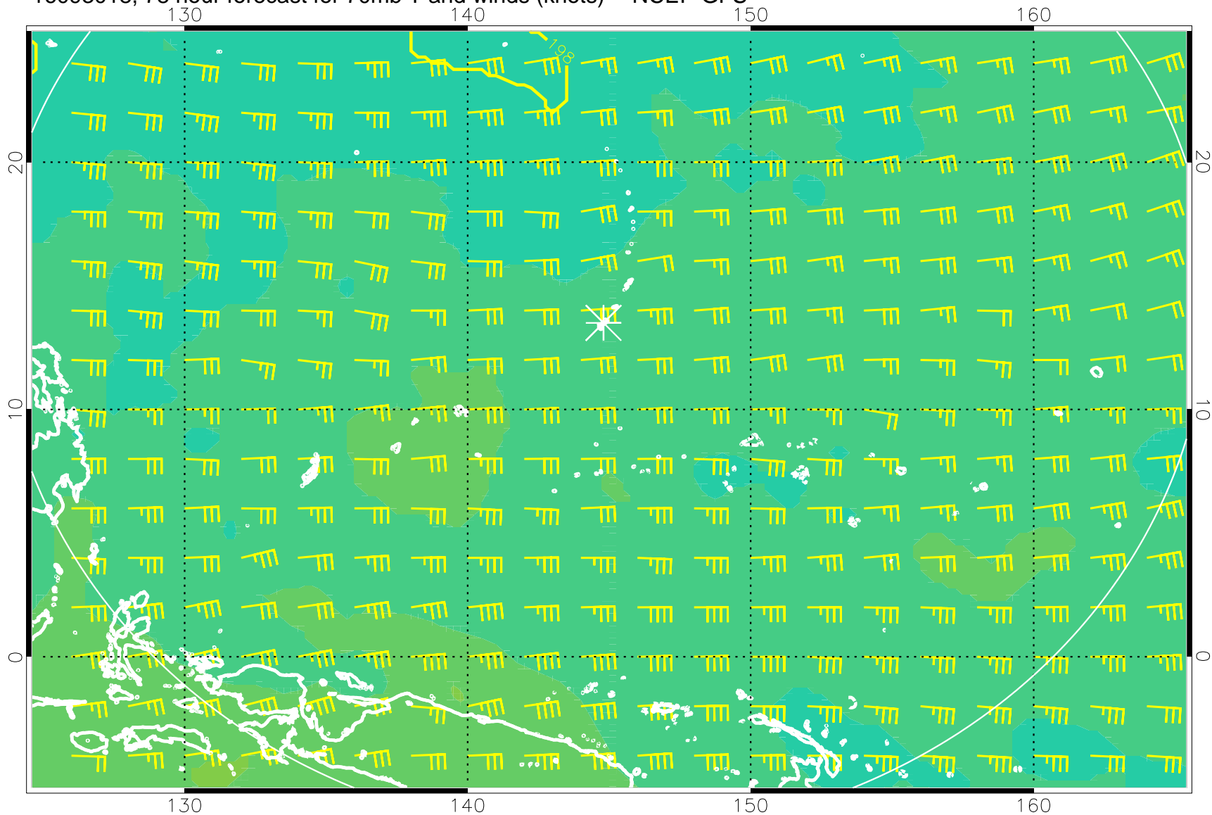
16093018, 78 hour forecast for 70mb T and winds (knots) -- NCEP GFS
