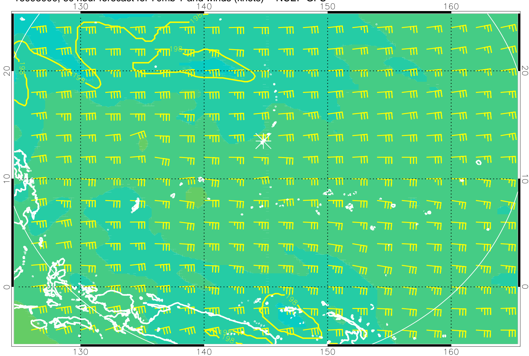
16093000, 60 hour forecast for 70mb T and winds (knots) -- NCEP GFS
