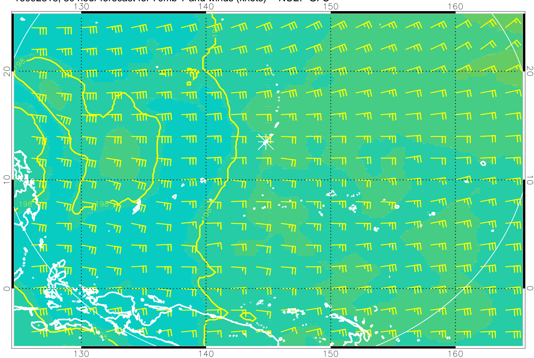
16092818, 30 hour forecast for 70mb T and winds (knots) -- NCEP GFS
