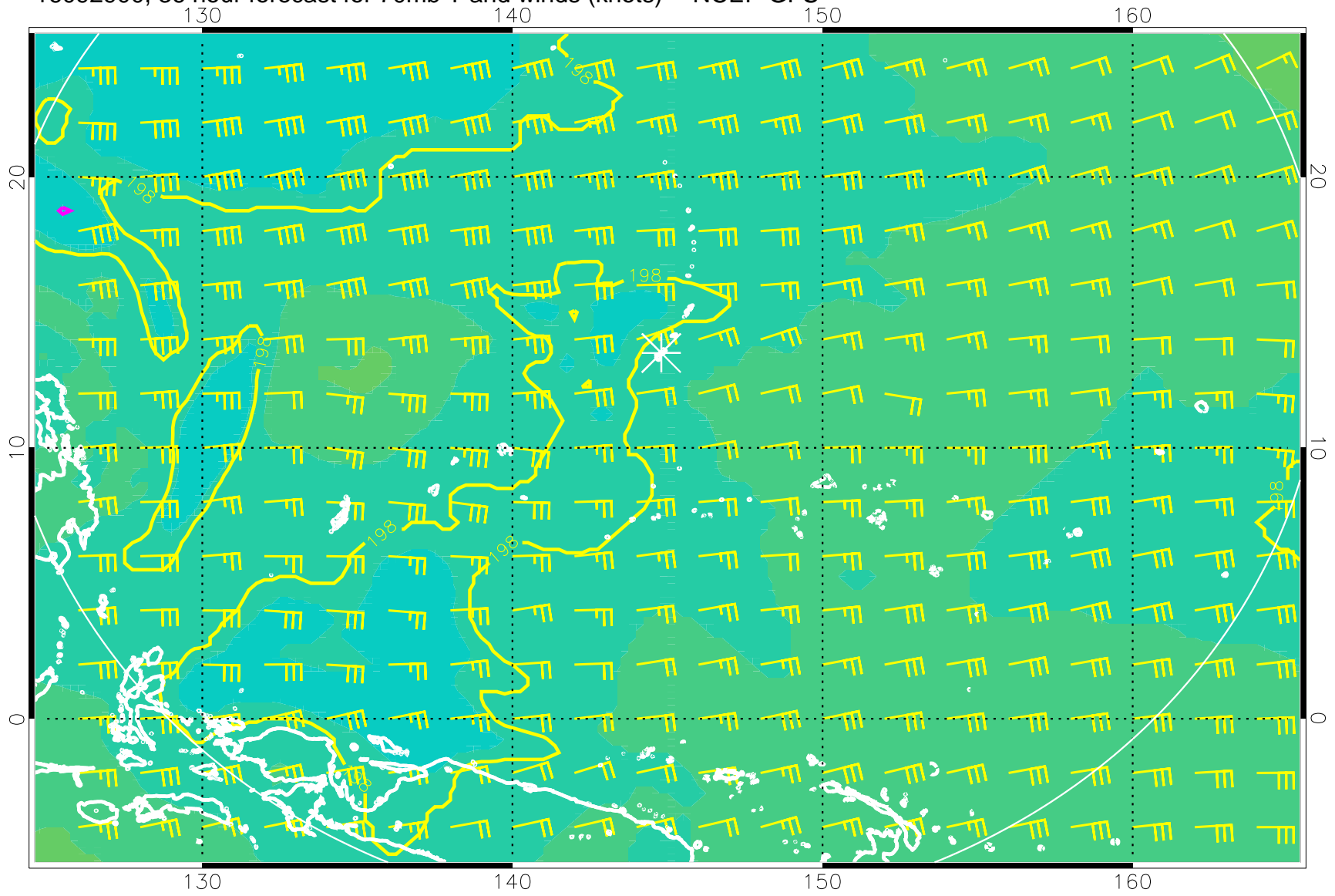
16092900, 36 hour forecast for 70mb T and winds (knots) -- NCEP GFS
