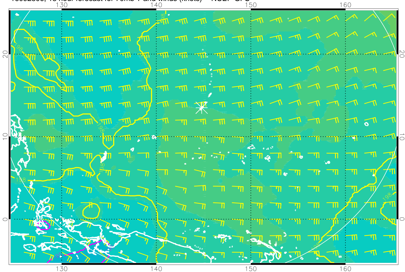
16092806, 18 hour forecast for 70mb T and winds (knots) -- NCEP GFS
