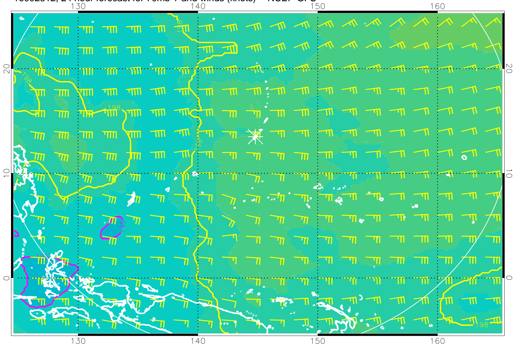
16092812, 24 hour forecast for 70mb T and winds (knots) -- NCEP GFS
