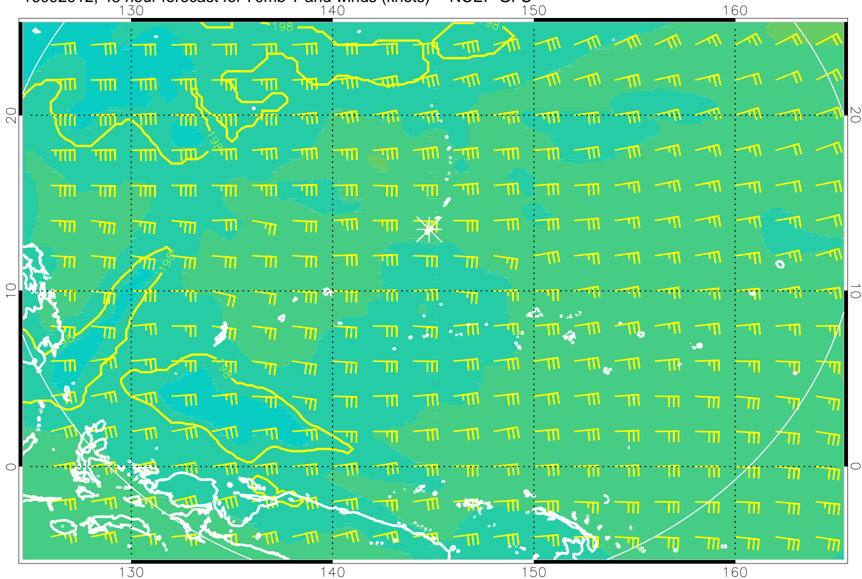
16092912, 48 hour forecast for 70mb T and winds (knots) -- NCEP GFS
