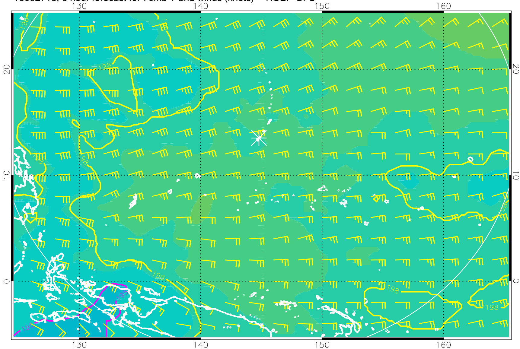
16092718, 6 hour forecast for 70mb T and winds (knots) -- NCEP GFS
