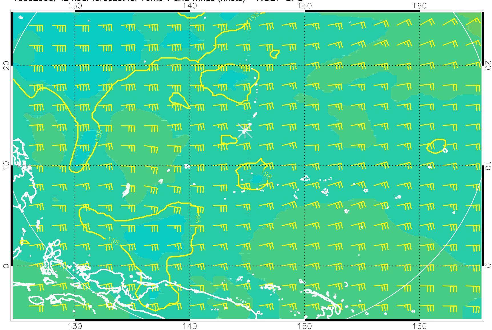
16092906, 42 hour forecast for 70mb T and winds (knots) -- NCEP GFS
