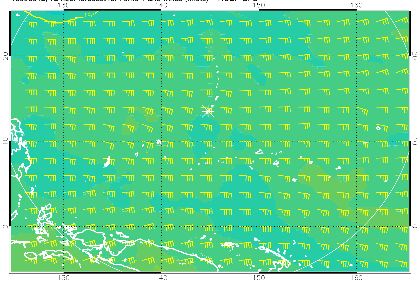
16093012, 72 hour forecast for 70mb T and winds (knots) -- NCEP GFS
