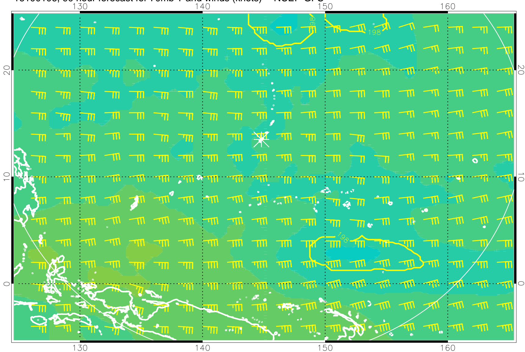
16100106, 90 hour forecast for 70mb T and winds (knots) -- NCEP GFS
