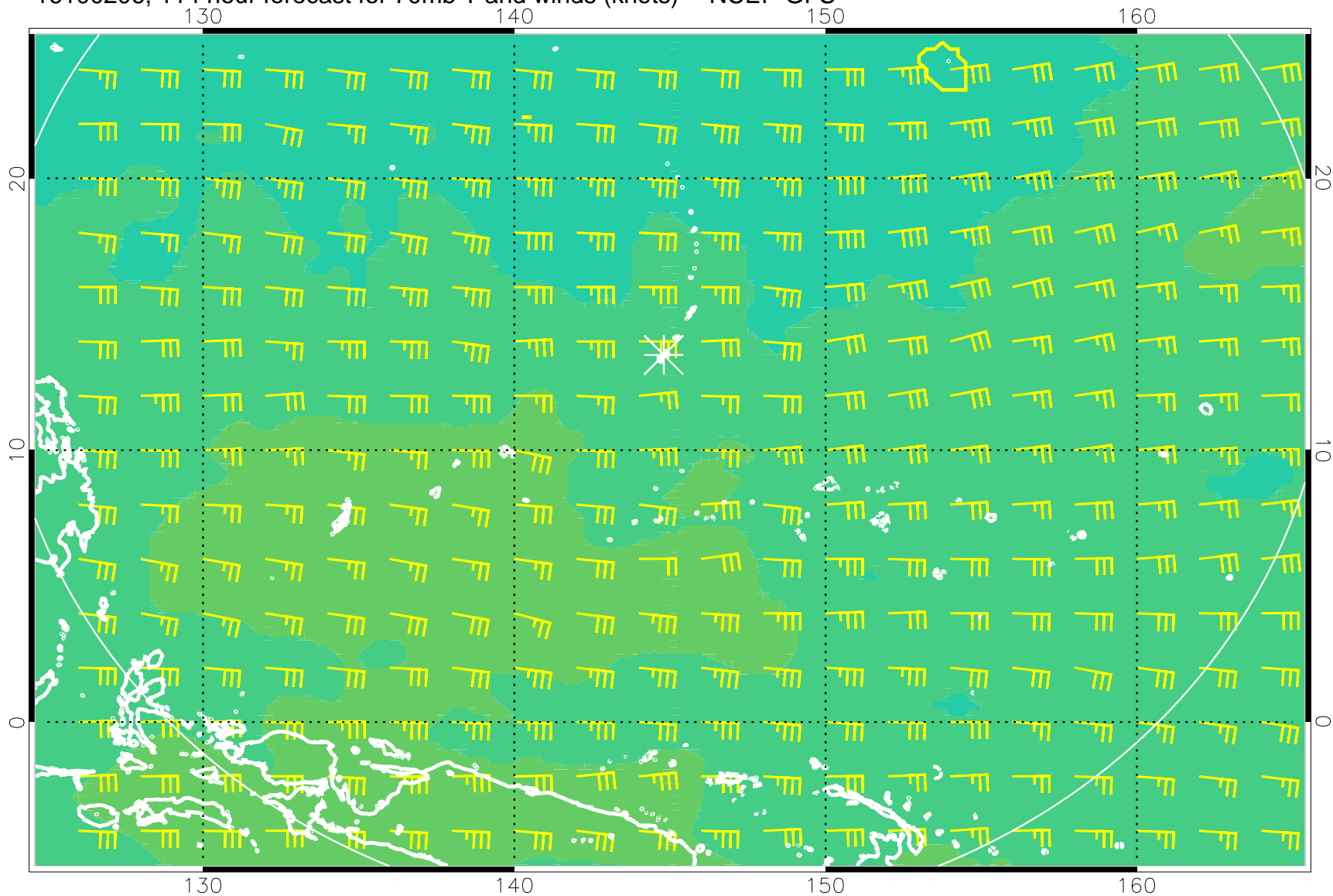
16100206, 114 hour forecast for 70mb T and winds (knots) -- NCEP GFS
