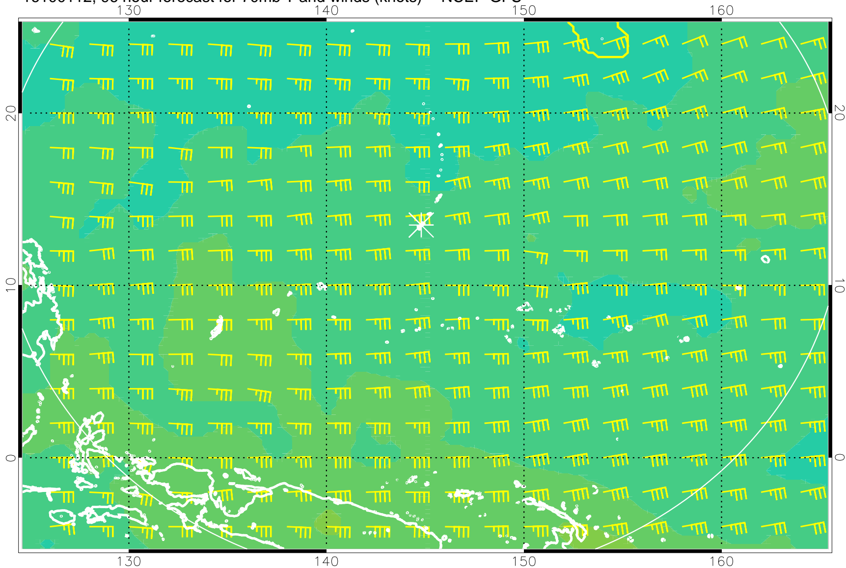
16100112, 96 hour forecast for 70mb T and winds (knots) -- NCEP GFS
