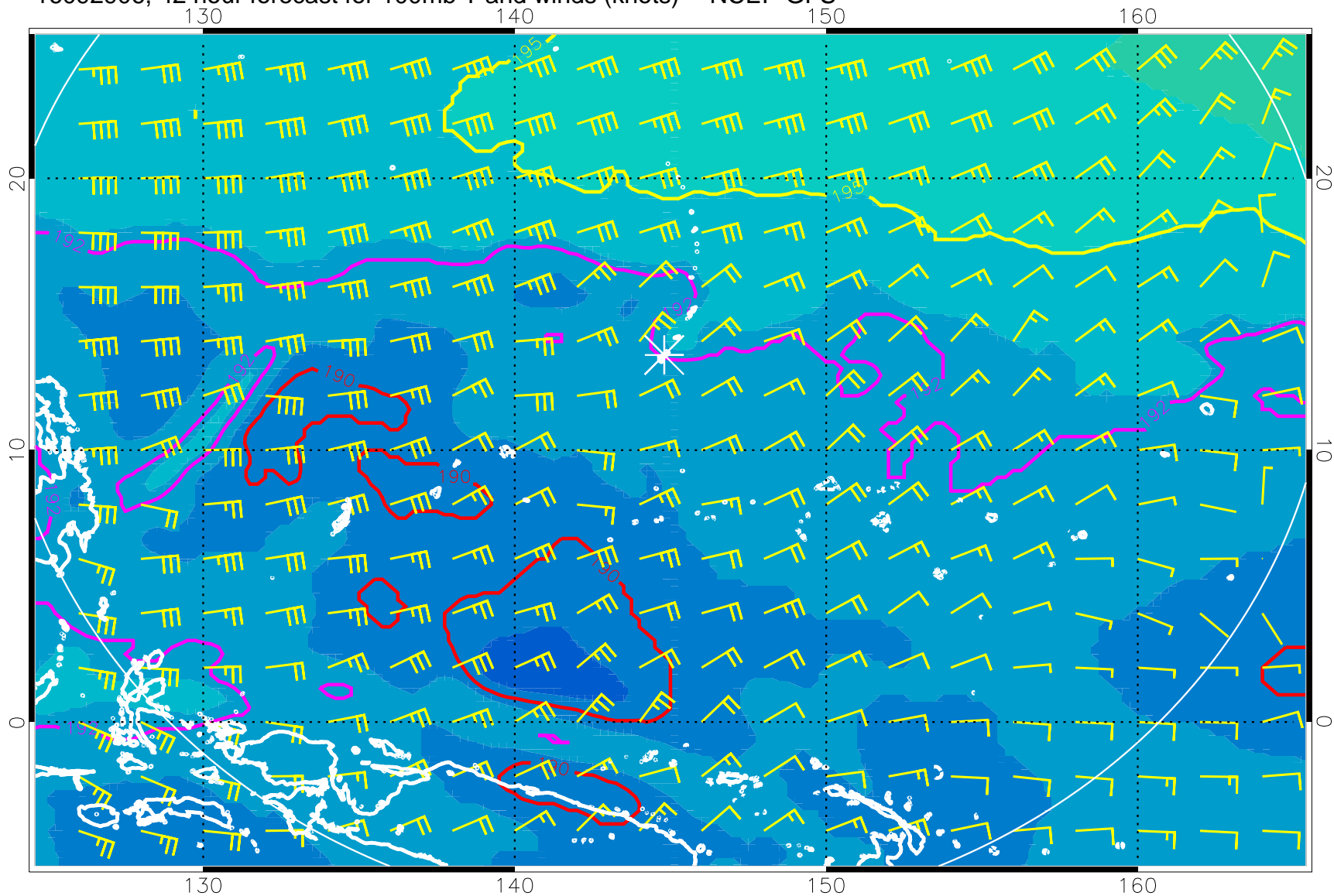
16092906, 42 hour forecast for 100mb T and winds (knots) -- NCEP GFS
