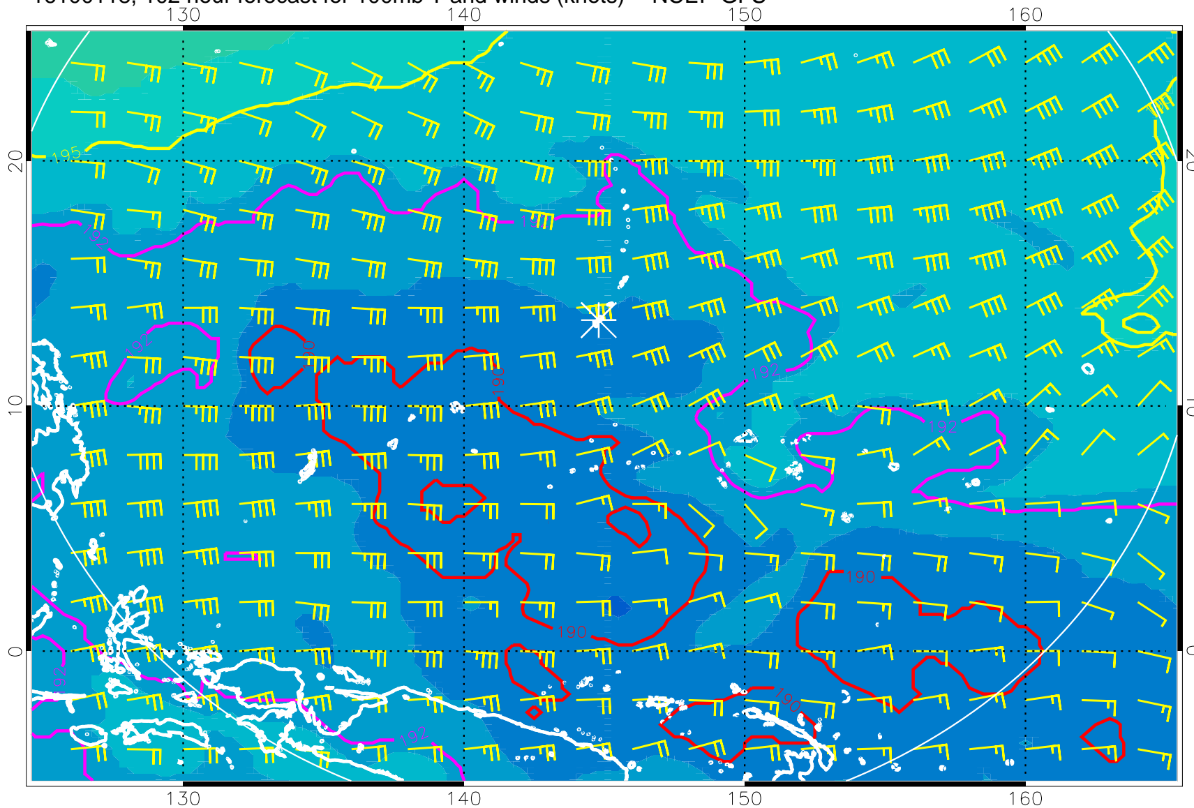
16100118, 102 hour forecast for 100mb T and winds (knots) -- NCEP GFS
