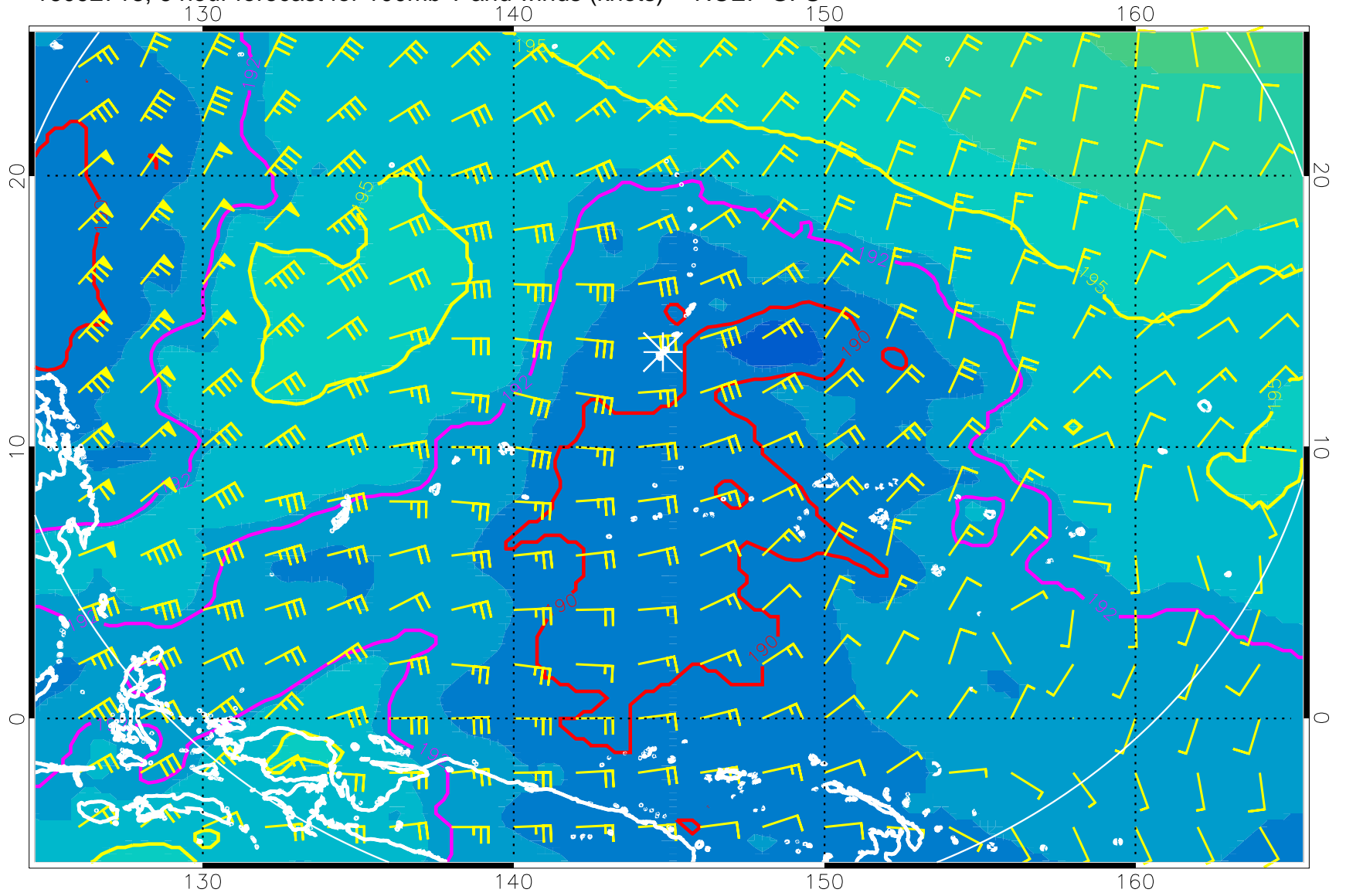
16092718, 6 hour forecast for 100mb T and winds (knots) -- NCEP GFS
