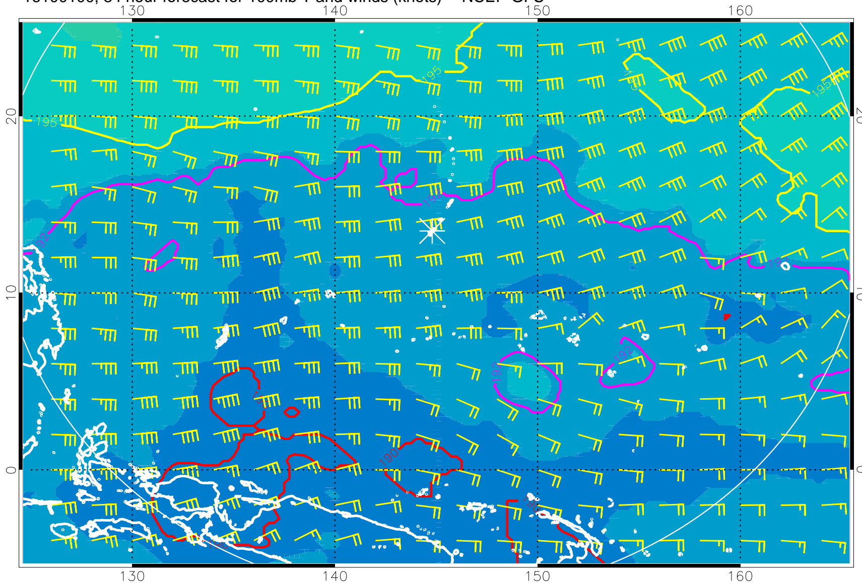
16100100, 84 hour forecast for 100mb T and winds (knots) -- NCEP GFS
