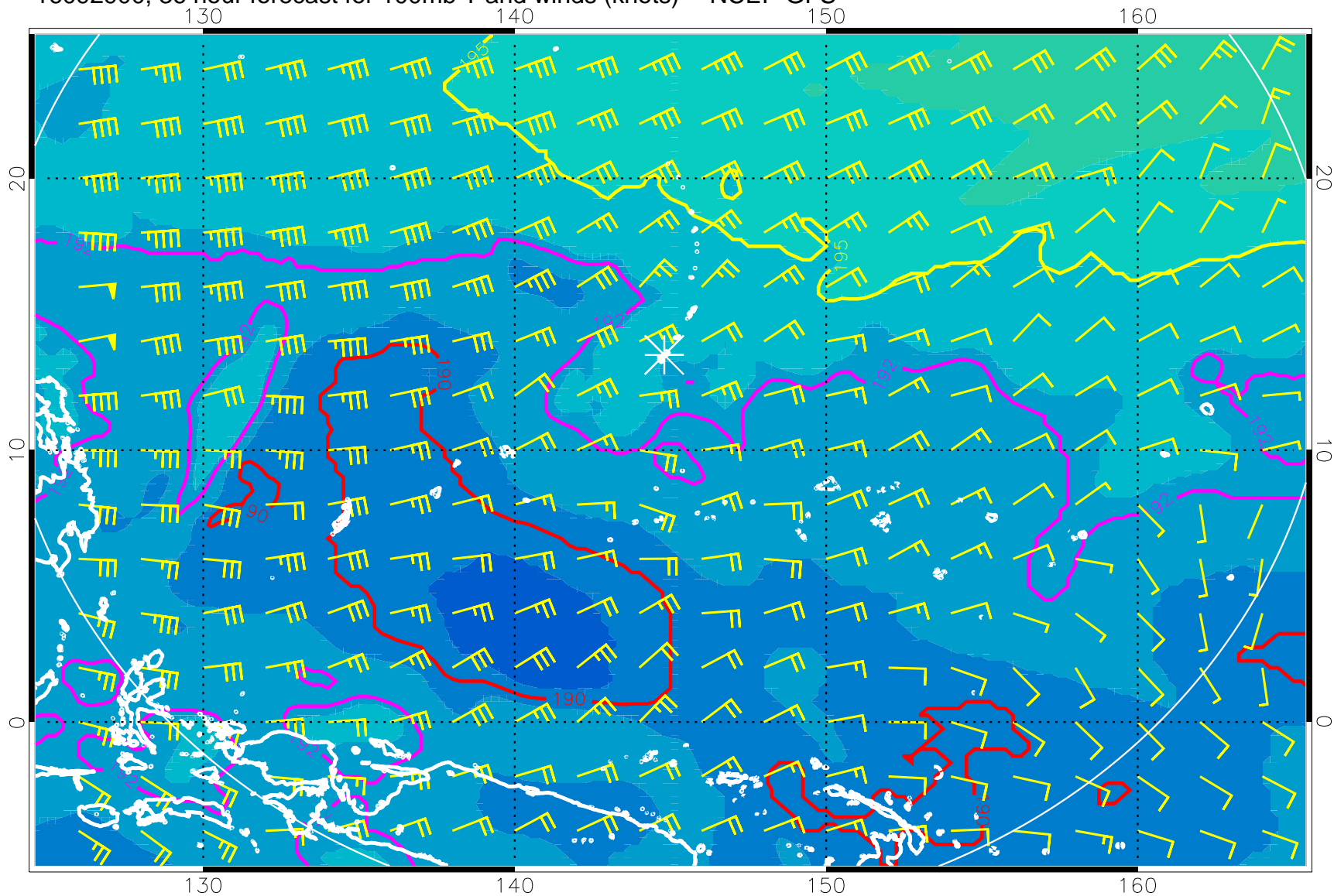
16092900, 36 hour forecast for 100mb T and winds (knots) -- NCEP GFS
