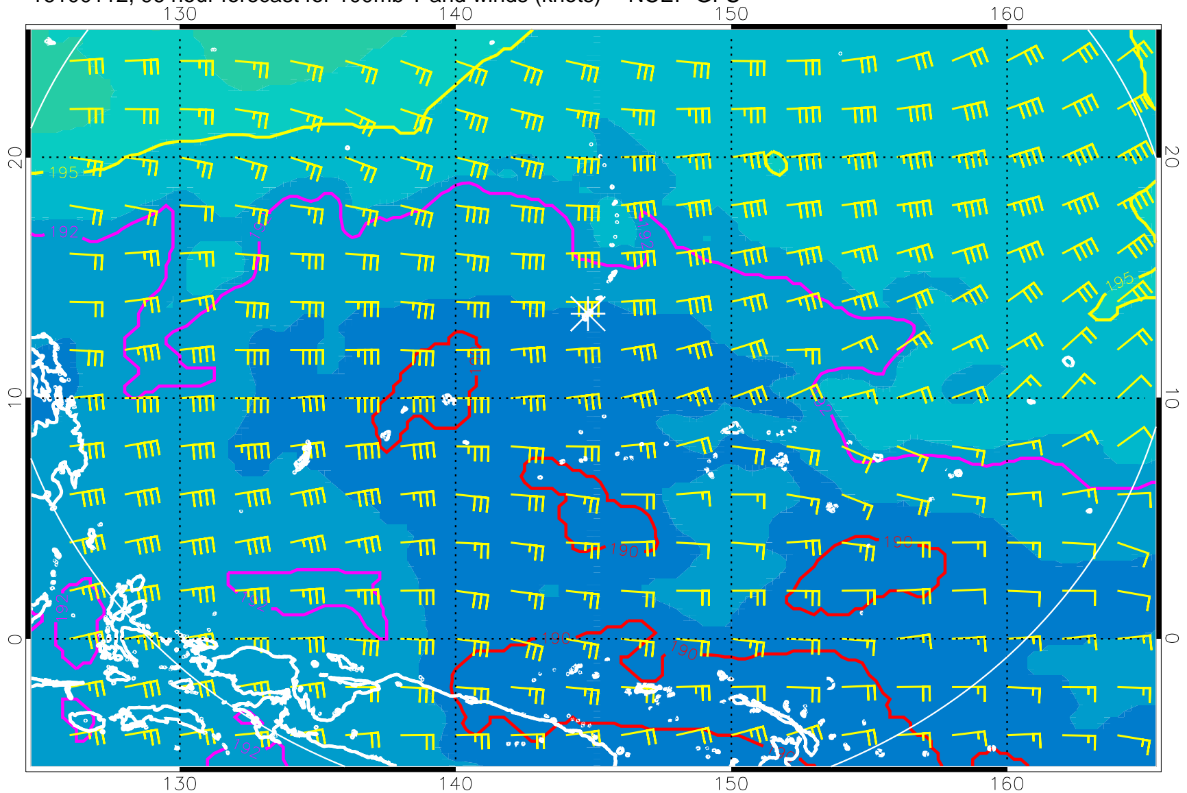
16100112, 96 hour forecast for 100mb T and winds (knots) -- NCEP GFS
