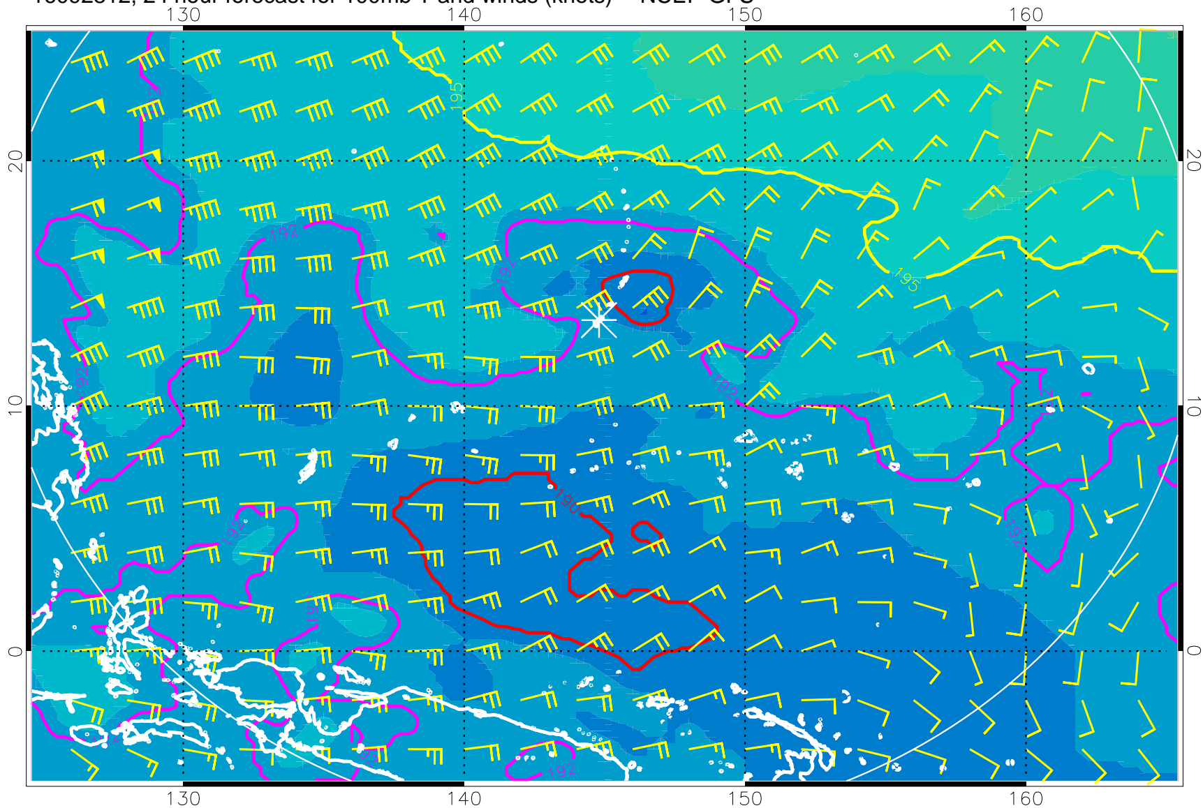
16092812, 24 hour forecast for 100mb T and winds (knots) -- NCEP GFS
