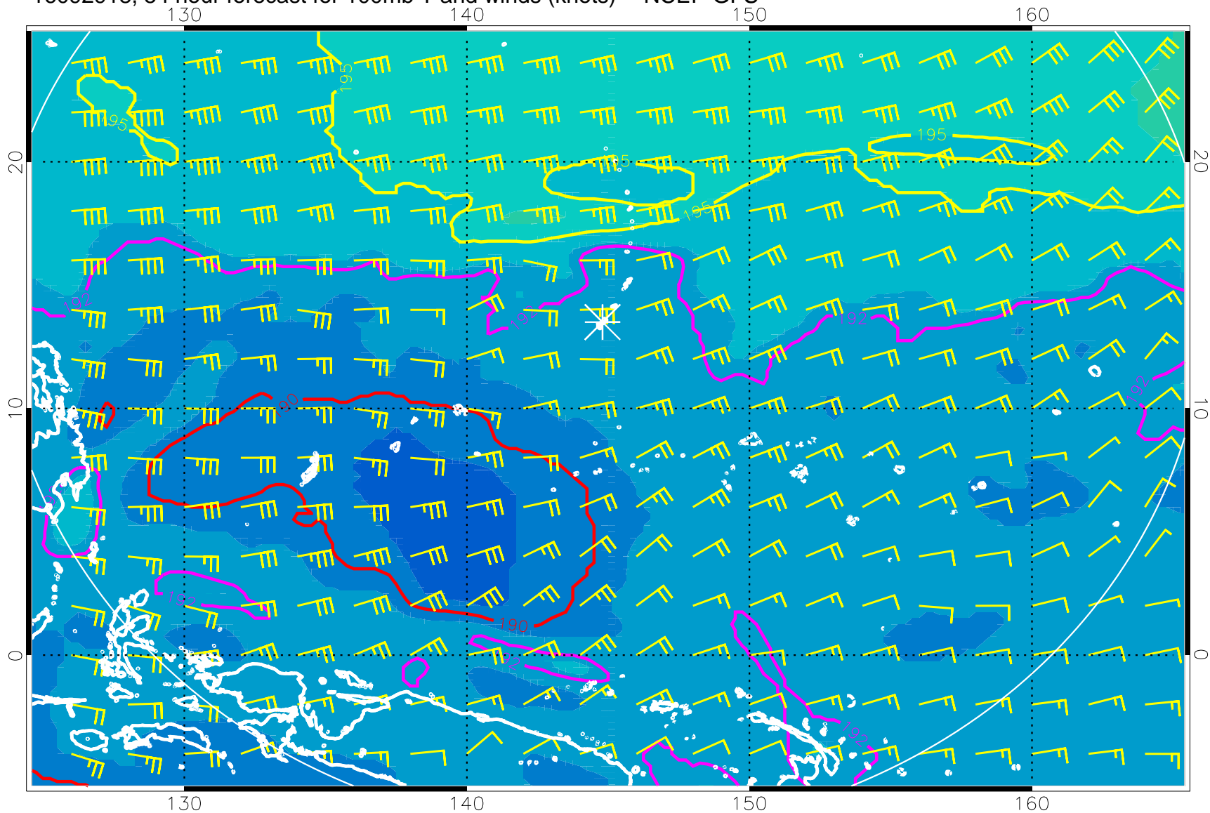
16092918, 54 hour forecast for 100mb T and winds (knots) -- NCEP GFS
