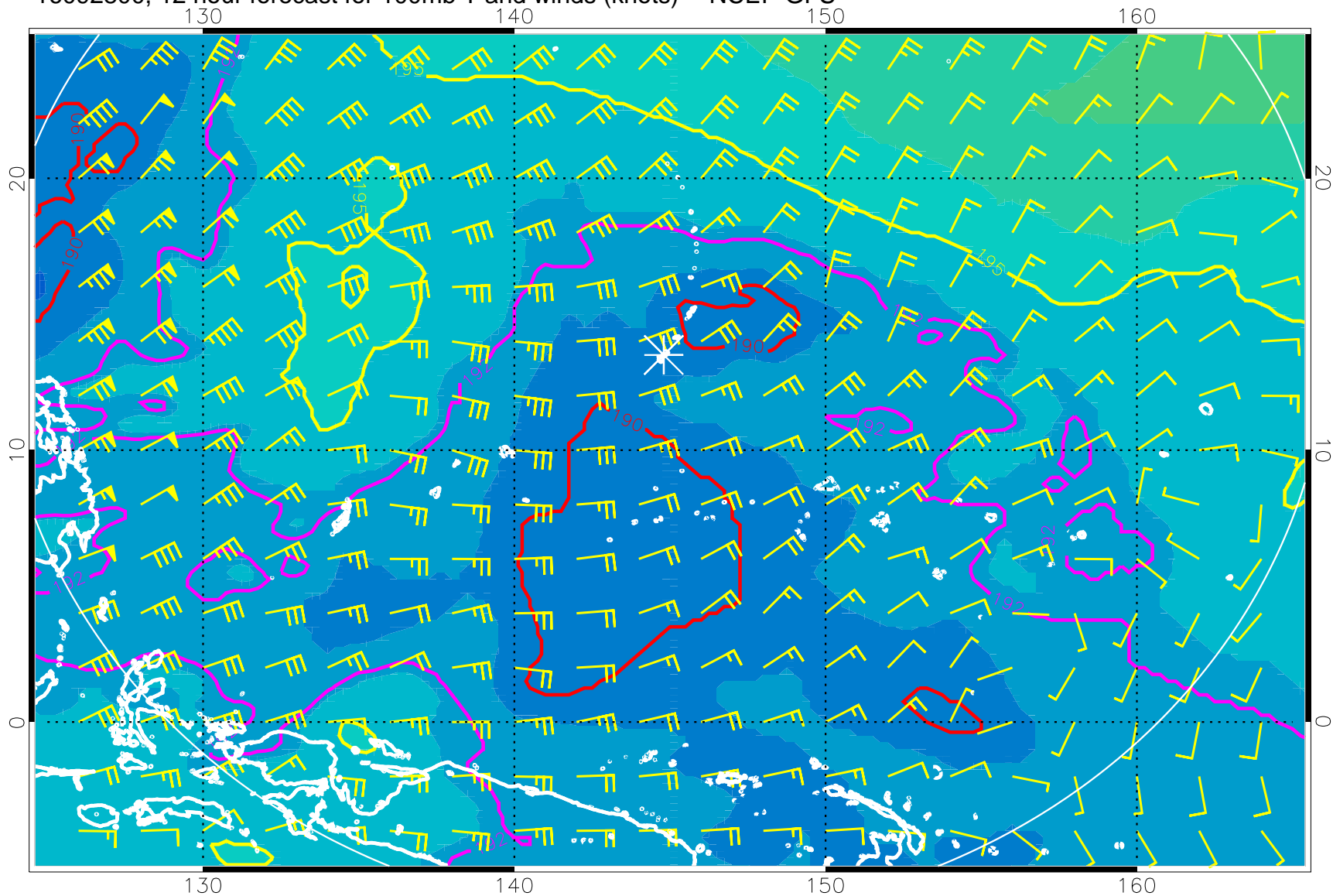
16092800, 12 hour forecast for 100mb T and winds (knots) -- NCEP GFS
