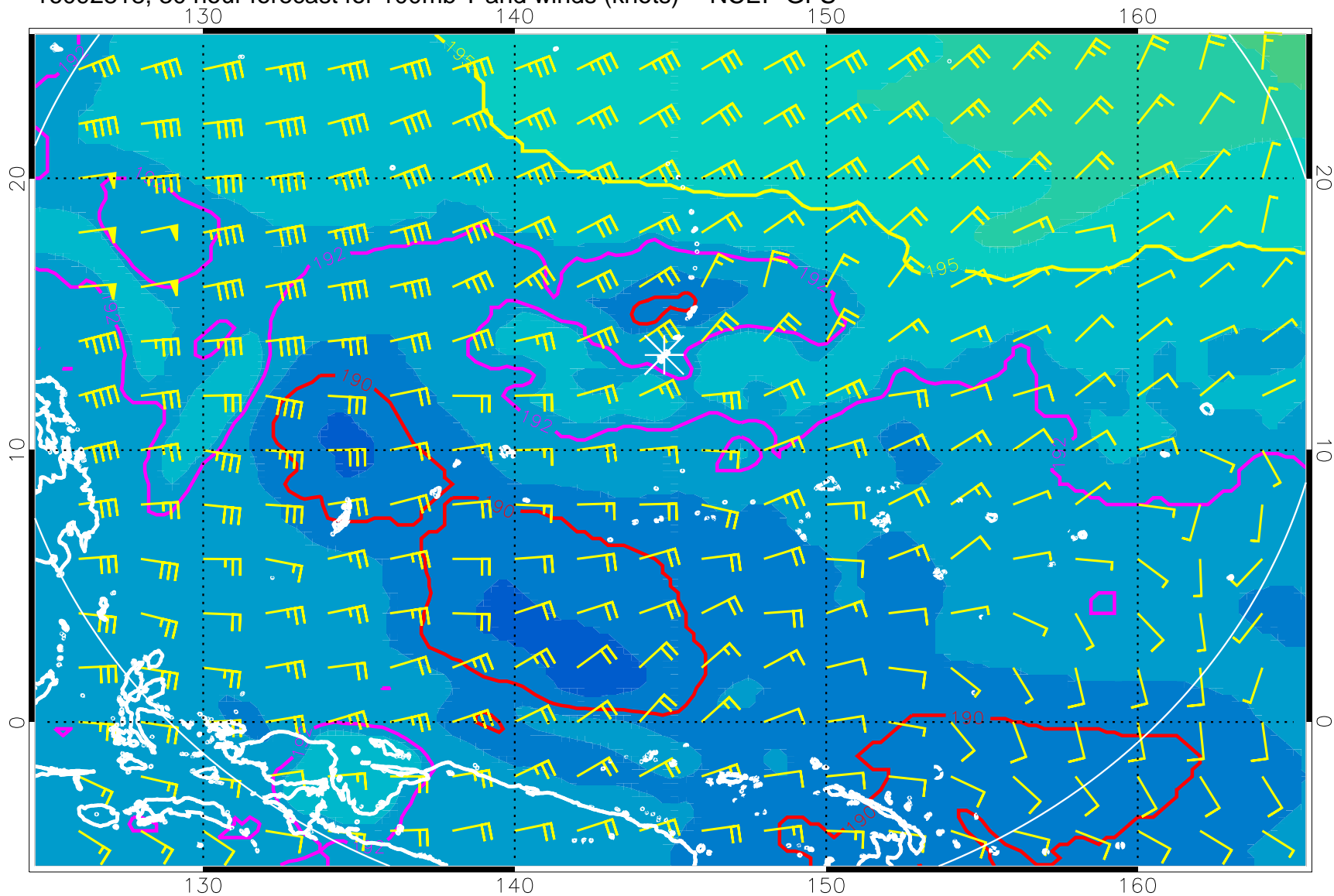
16092818, 30 hour forecast for 100mb T and winds (knots) -- NCEP GFS
