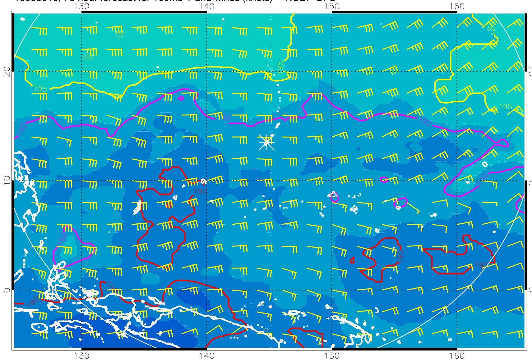
16093018, 78 hour forecast for 100mb T and winds (knots) -- NCEP GFS
