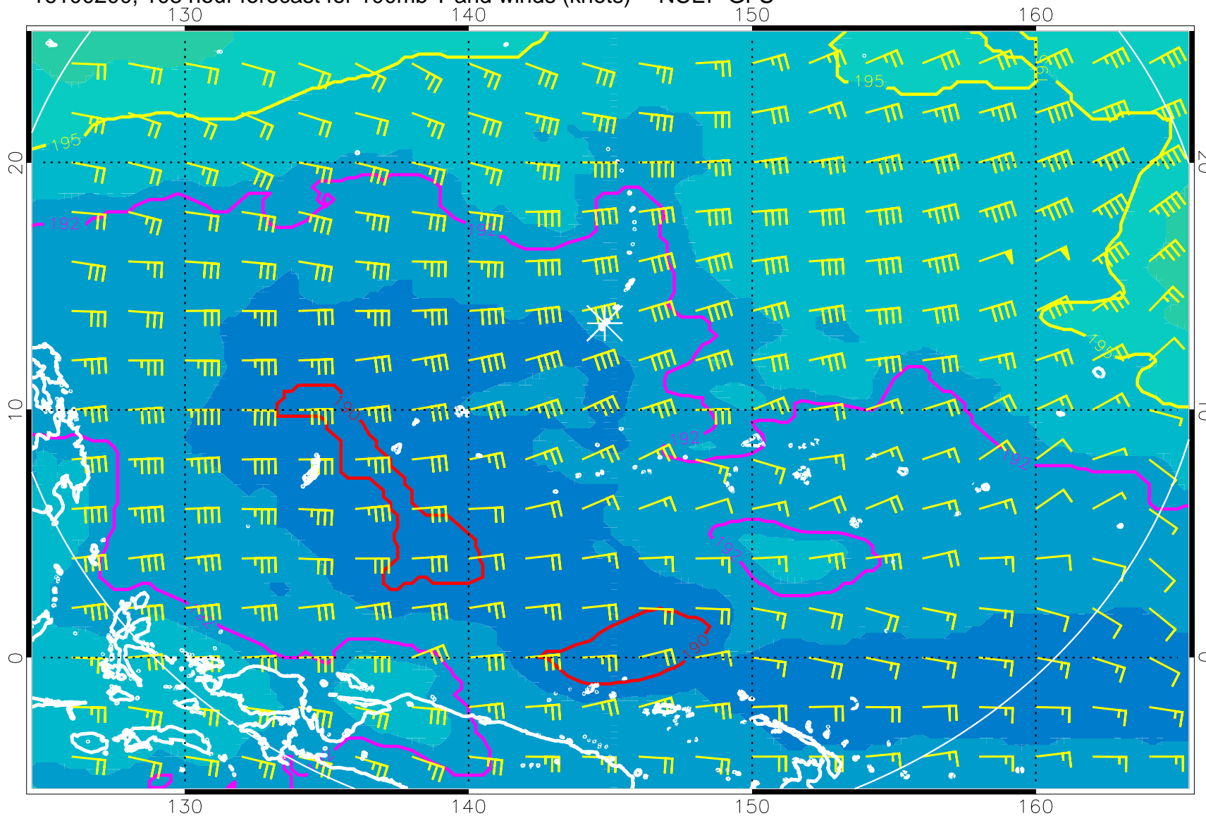
16100200, 108 hour forecast for 100mb T and winds (knots) -- NCEP GFS
