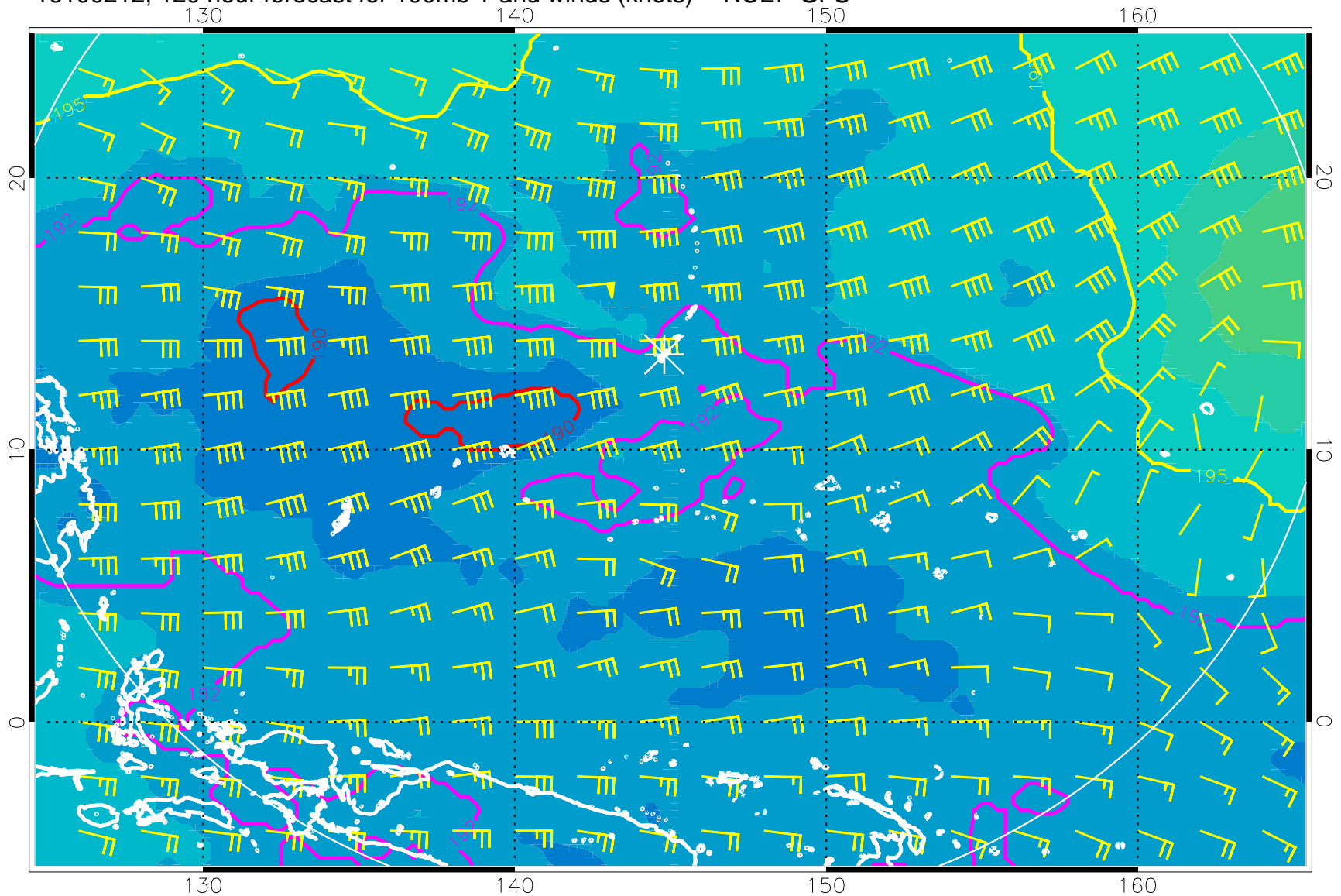
16100212, 120 hour forecast for 100mb T and winds (knots) -- NCEP GFS
