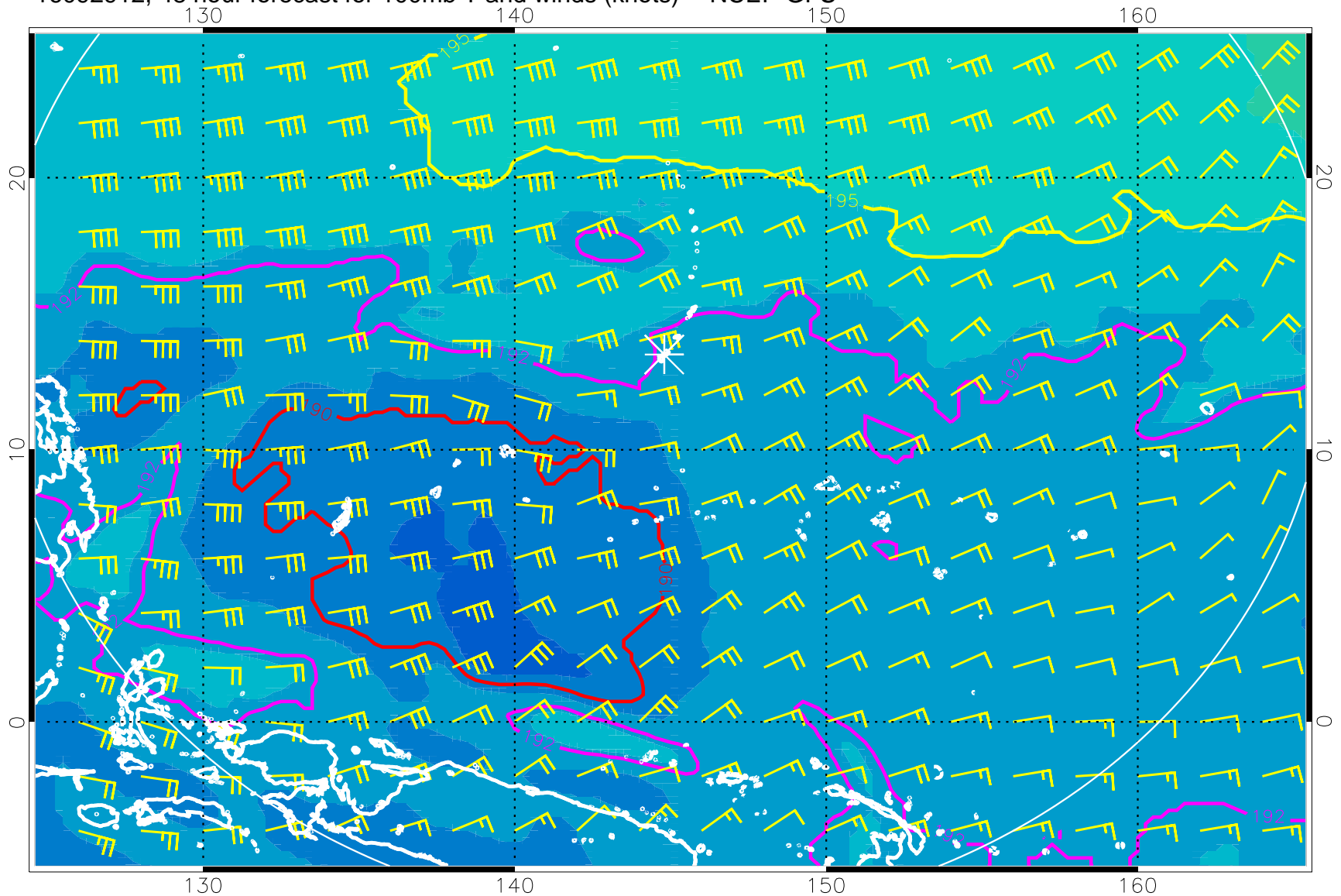
16092912, 48 hour forecast for 100mb T and winds (knots) -- NCEP GFS
