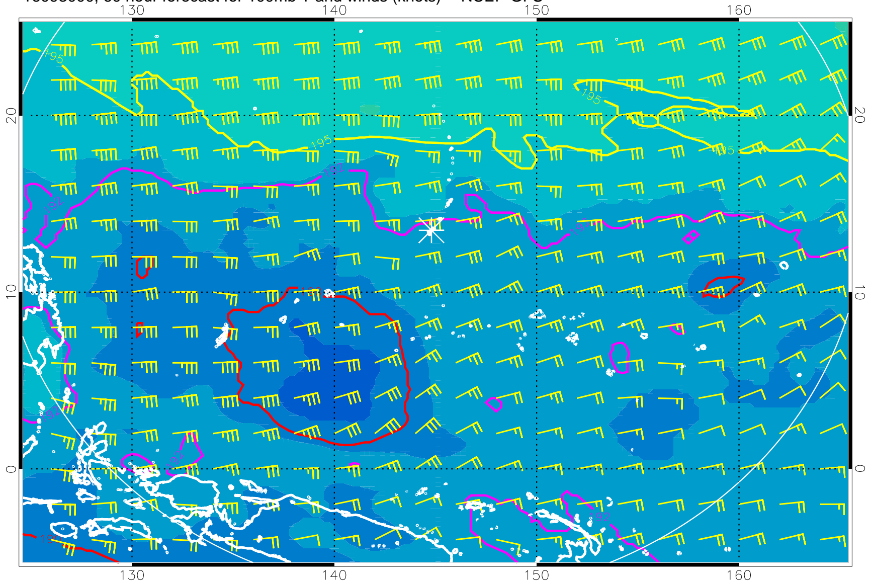
16093000, 60 hour forecast for 100mb T and winds (knots) -- NCEP GFS
