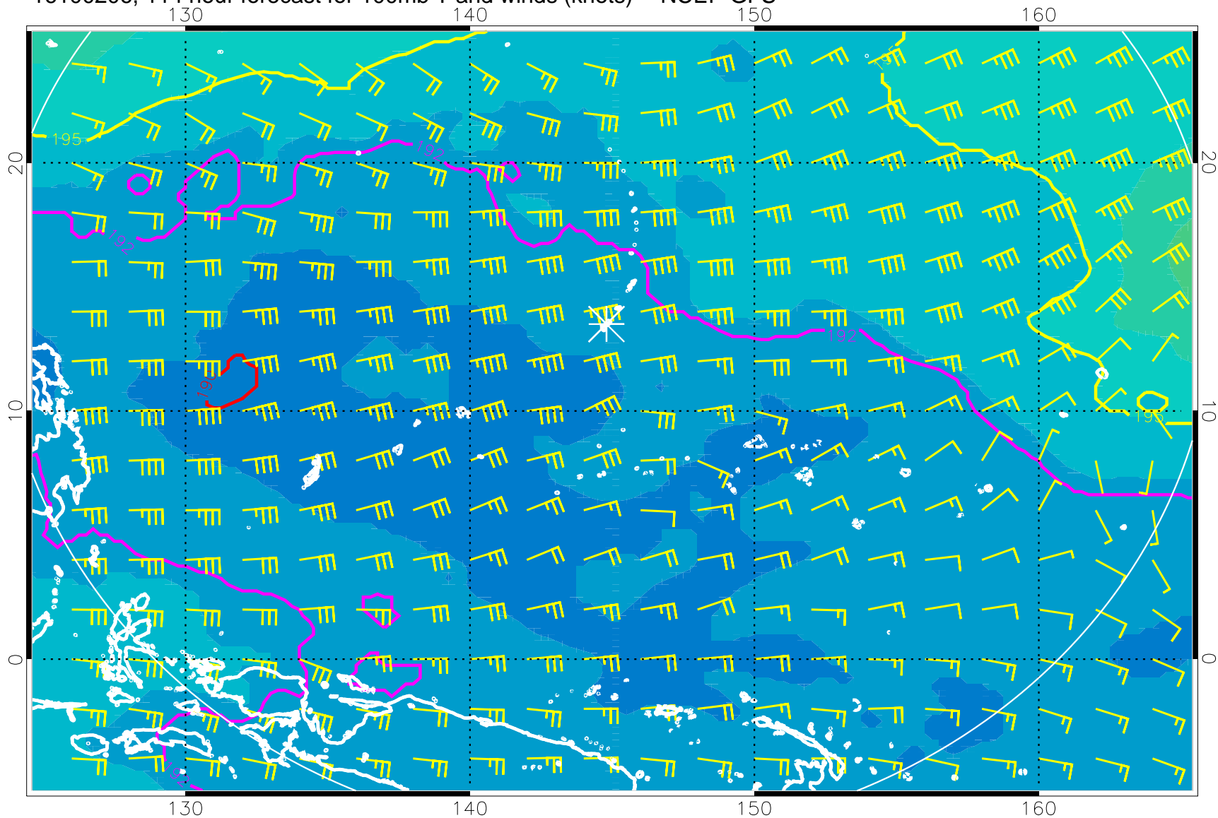
16100206, 114 hour forecast for 100mb T and winds (knots) -- NCEP GFS
