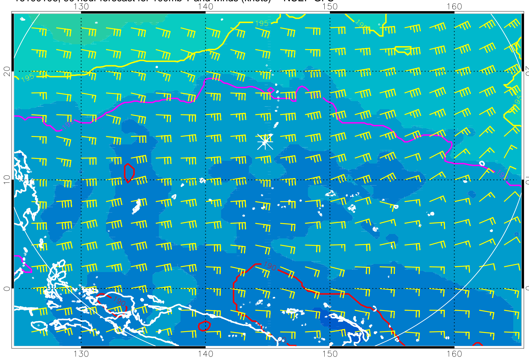
16100106, 90 hour forecast for 100mb T and winds (knots) -- NCEP GFS
