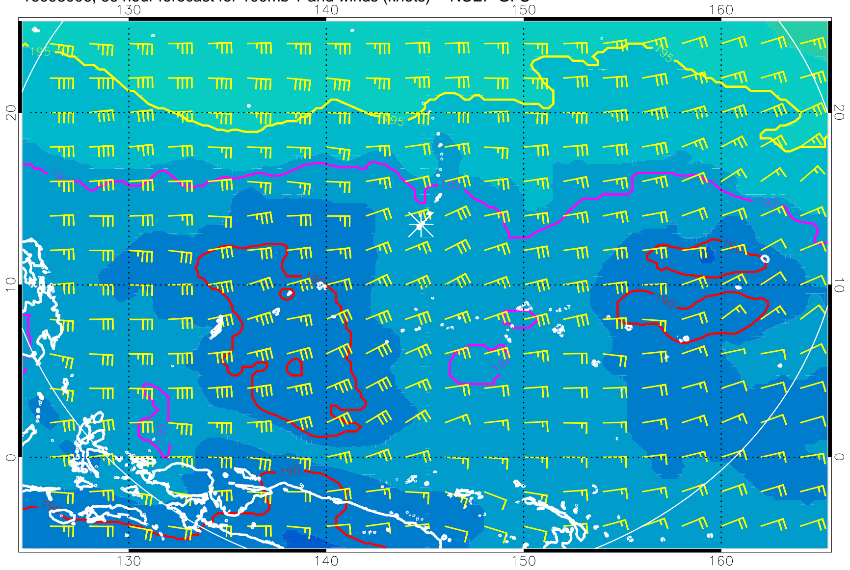
16093006, 66 hour forecast for 100mb T and winds (knots) -- NCEP GFS
