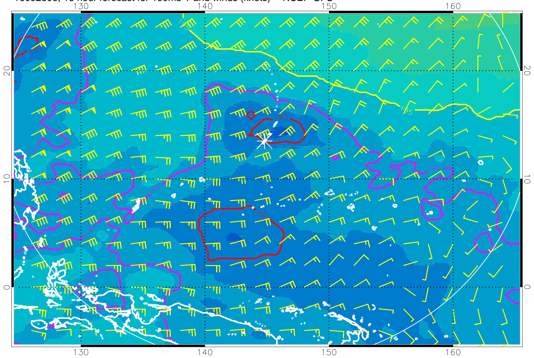
16092806, 18 hour forecast for 100mb T and winds (knots) -- NCEP GFS
