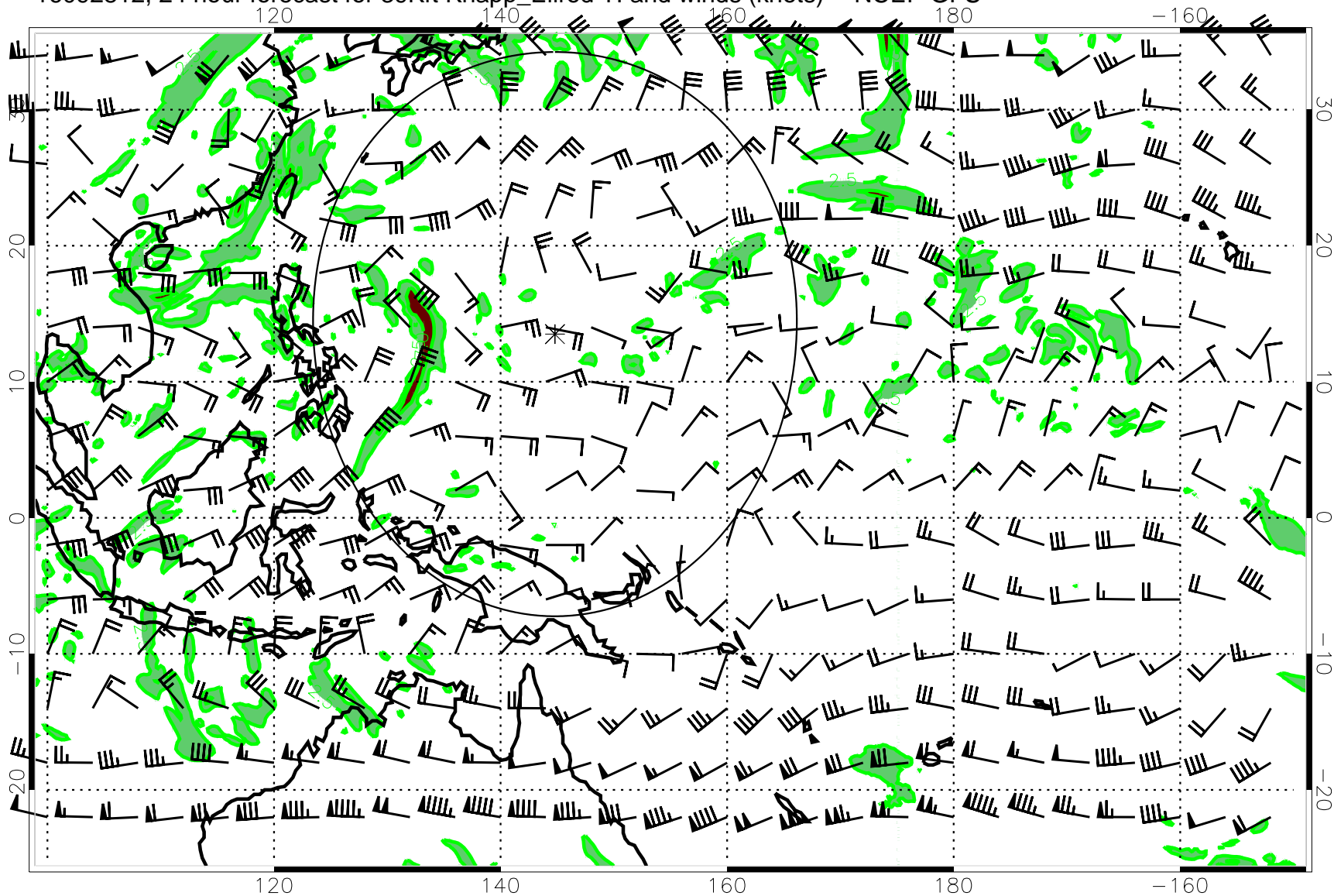
16092812, 24 hour forecast for 39Kft Knapp_Ellrod TI and winds (knots) -- NCEP GFS
