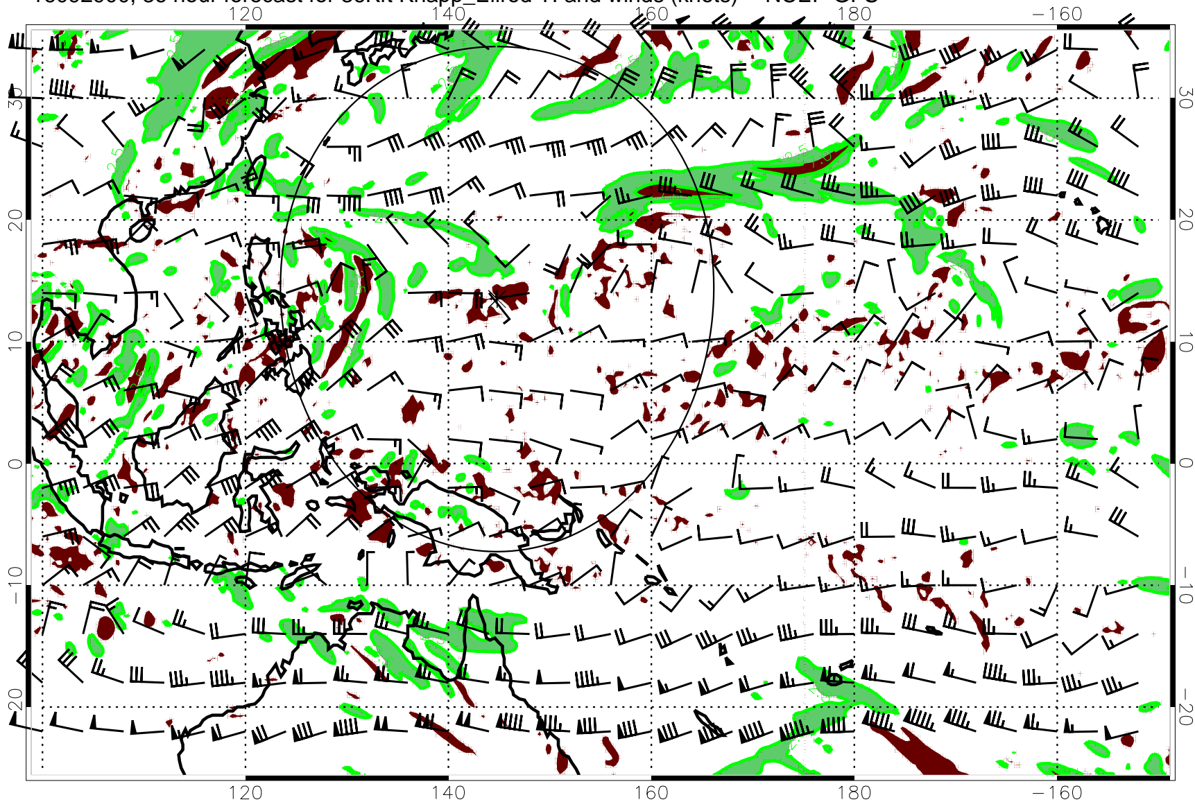
16092900, 36 hour forecast for 36Kft Knapp_Ellrod TI and winds (knots) -- NCEP GFS
