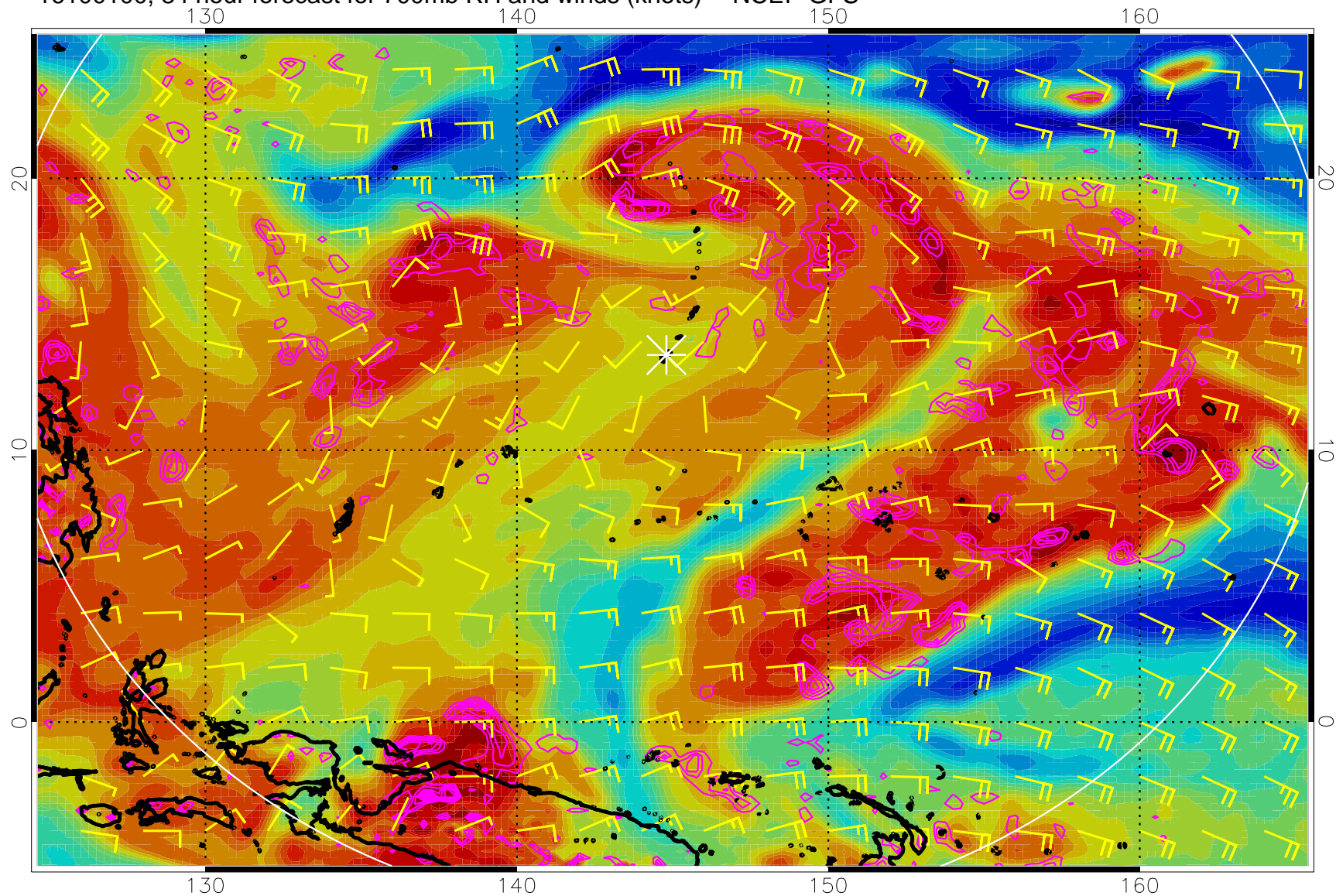
16100100, 84 hour forecast for 700mb RH and winds (knots) -- NCEP GFS
