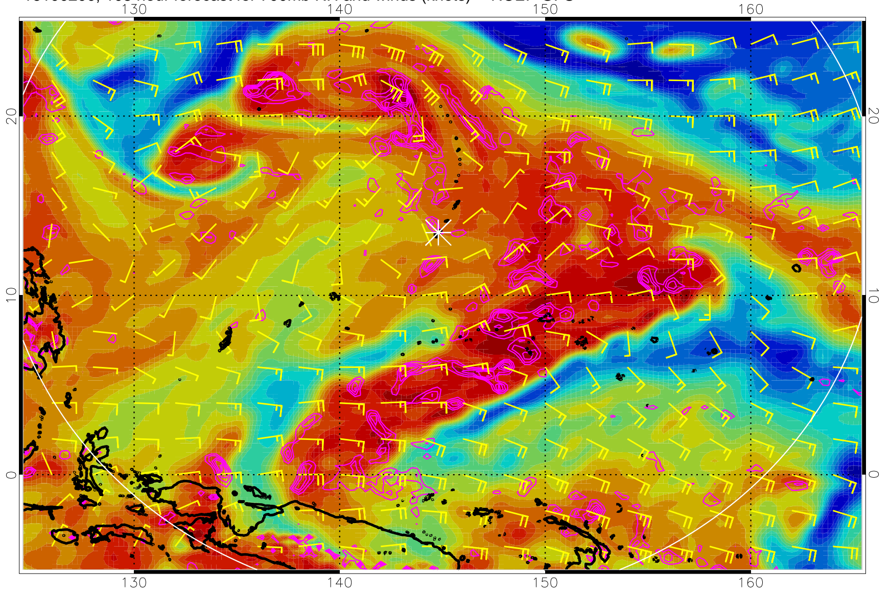
16100200, 108 hour forecast for 700mb RH and winds (knots) -- NCEP GFS
