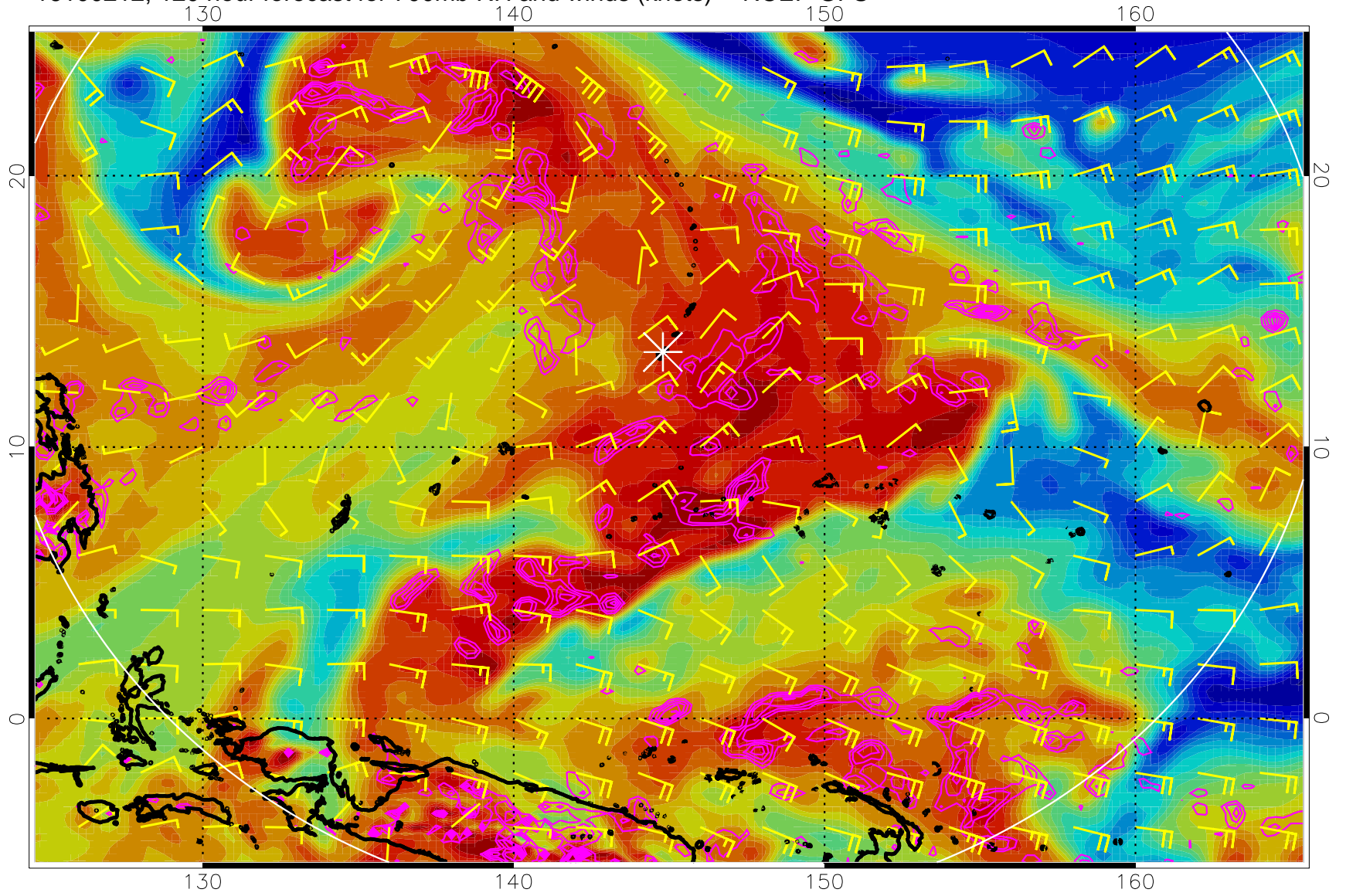
16100212, 120 hour forecast for 700mb RH and winds (knots) -- NCEP GFS
