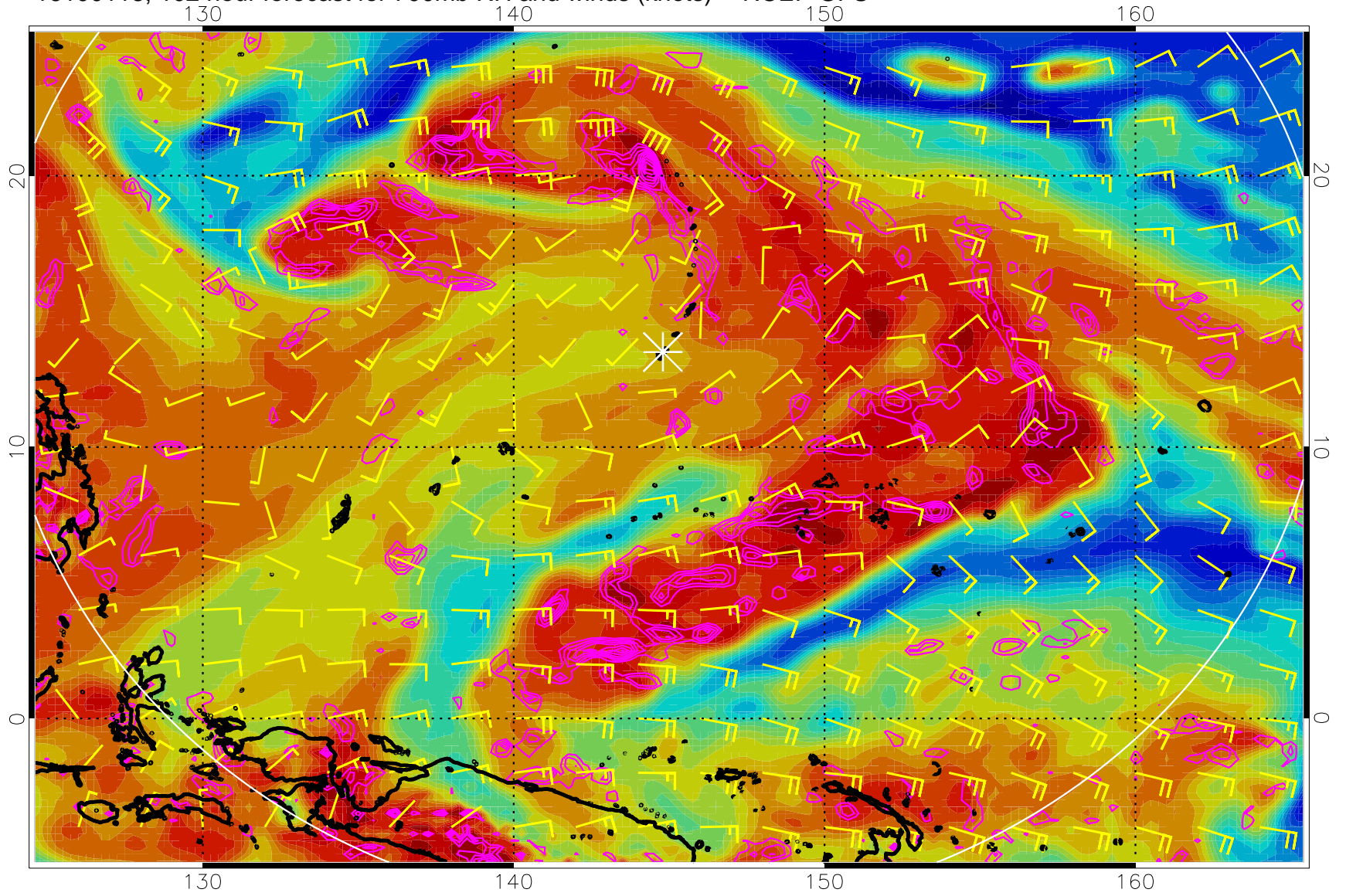
16100118, 102 hour forecast for 700mb RH and winds (knots) -- NCEP GFS
