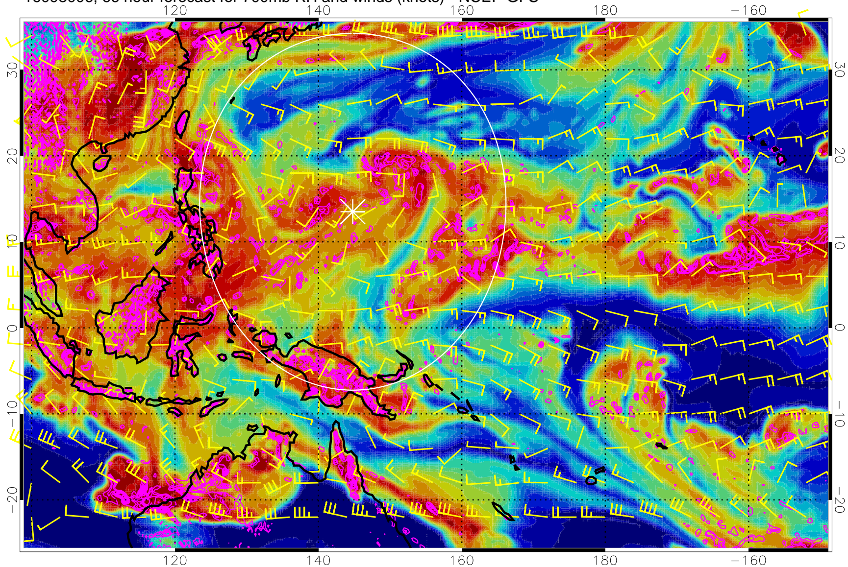
16093006, 66 hour forecast for 700mb RH and winds (knots) - NCEP GFS
