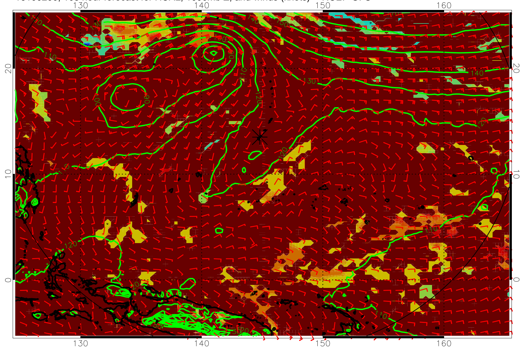
16100200, 108 hour forecast for HCAL, 1000mb Z, and winds (knots) -- NCEP GFS
