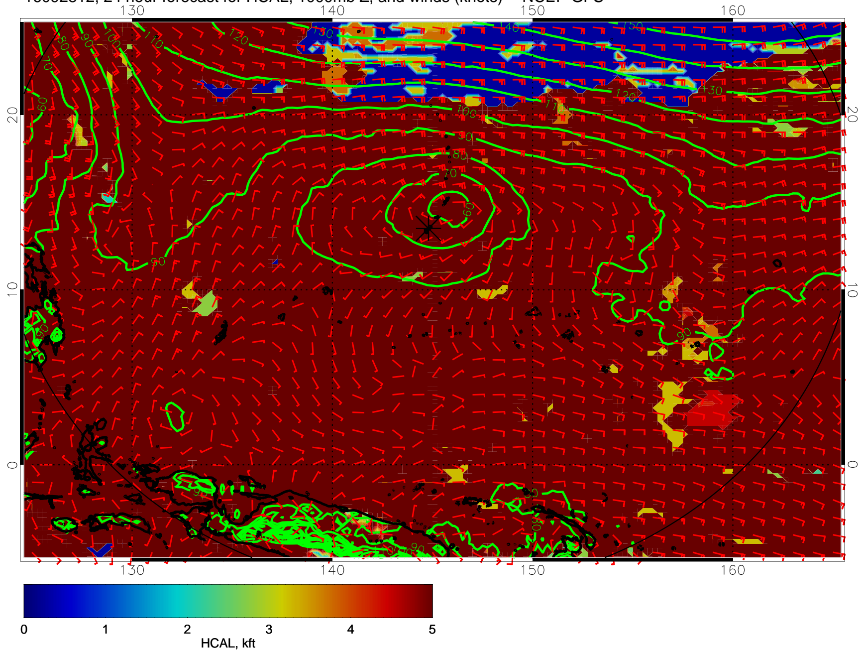
16092812, 24 hour forecast for HCAL, 1000mb Z, and winds (knots) -- NCEP GFS
