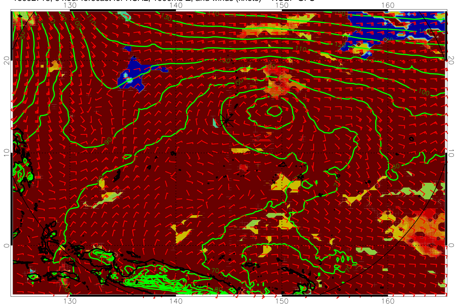
16092718, 6 hour forecast for HCAL, 1000mb Z, and winds (knots) -- NCEP GFS
