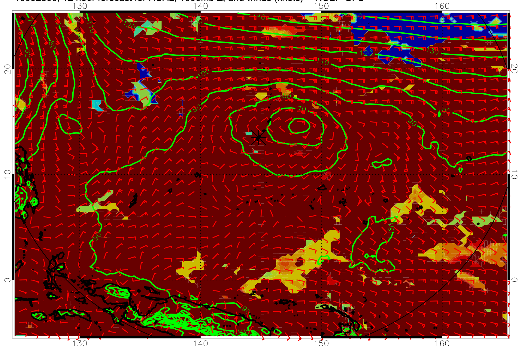
16092800, 12 hour forecast for HCAL, 1000mb Z, and winds (knots) -- NCEP GFS
