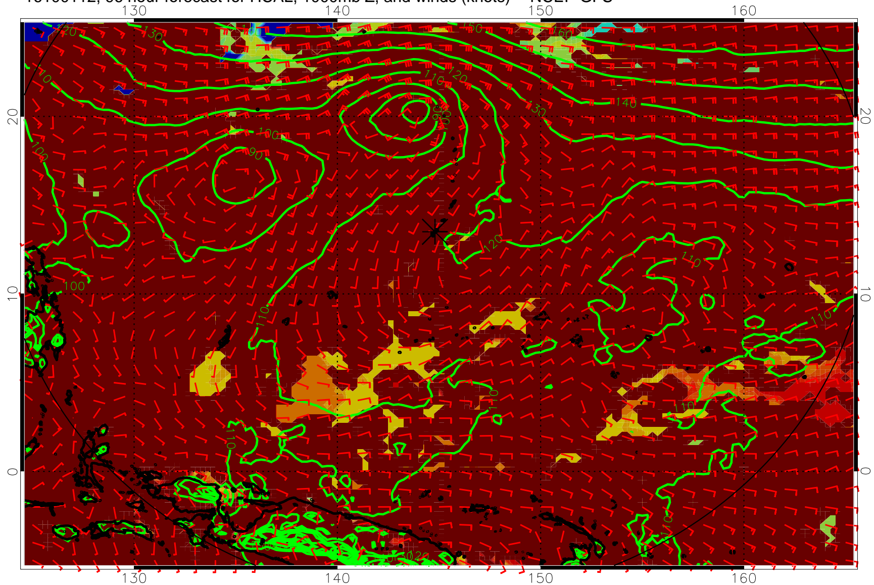
16100112, 96 hour forecast for HCAL, 1000mb Z, and winds (knots) -- NCEP GFS
