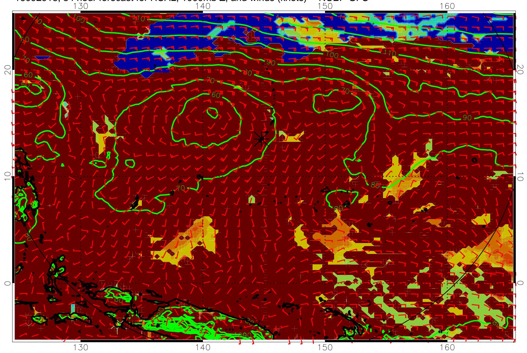
16092918, 54 hour forecast for HCAL, 1000mb Z, and winds (knots) -- NCEP GFS
