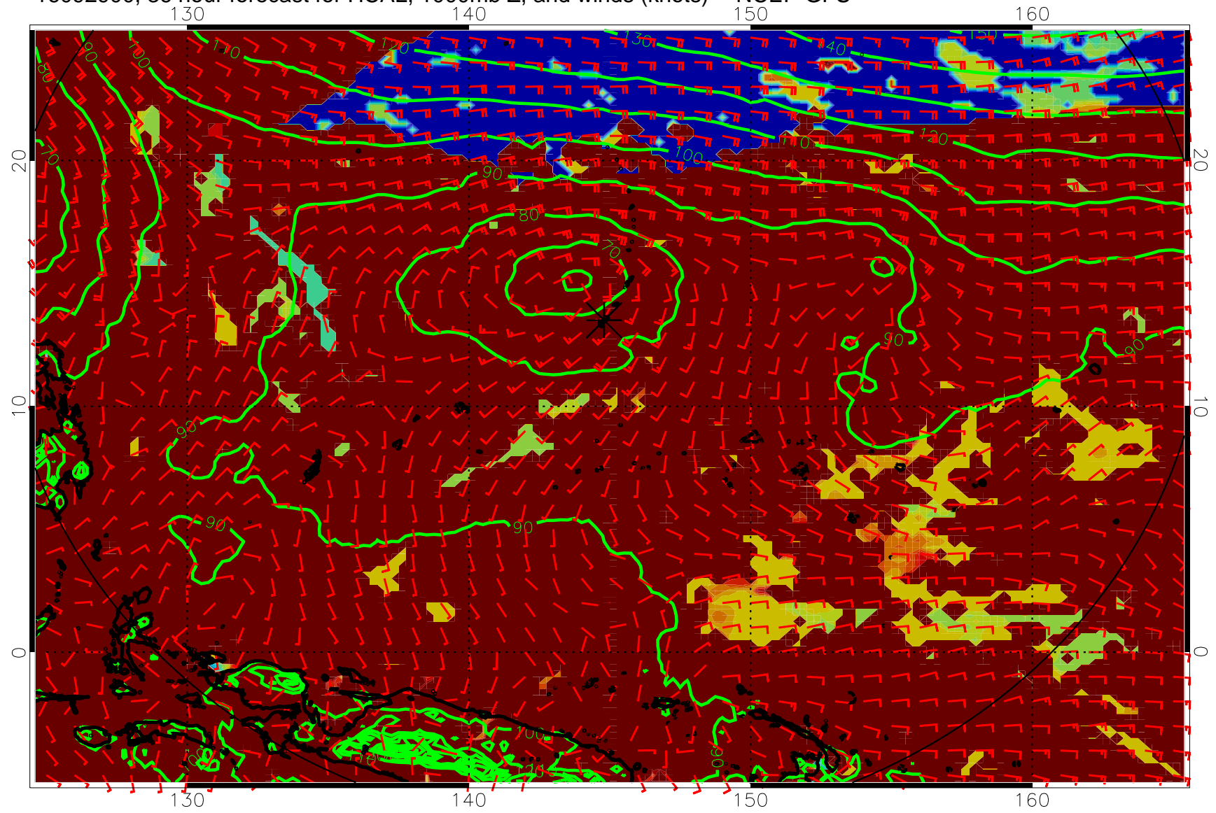
16092900, 36 hour forecast for HCAL, 1000mb Z, and winds (knots) -- NCEP GFS
