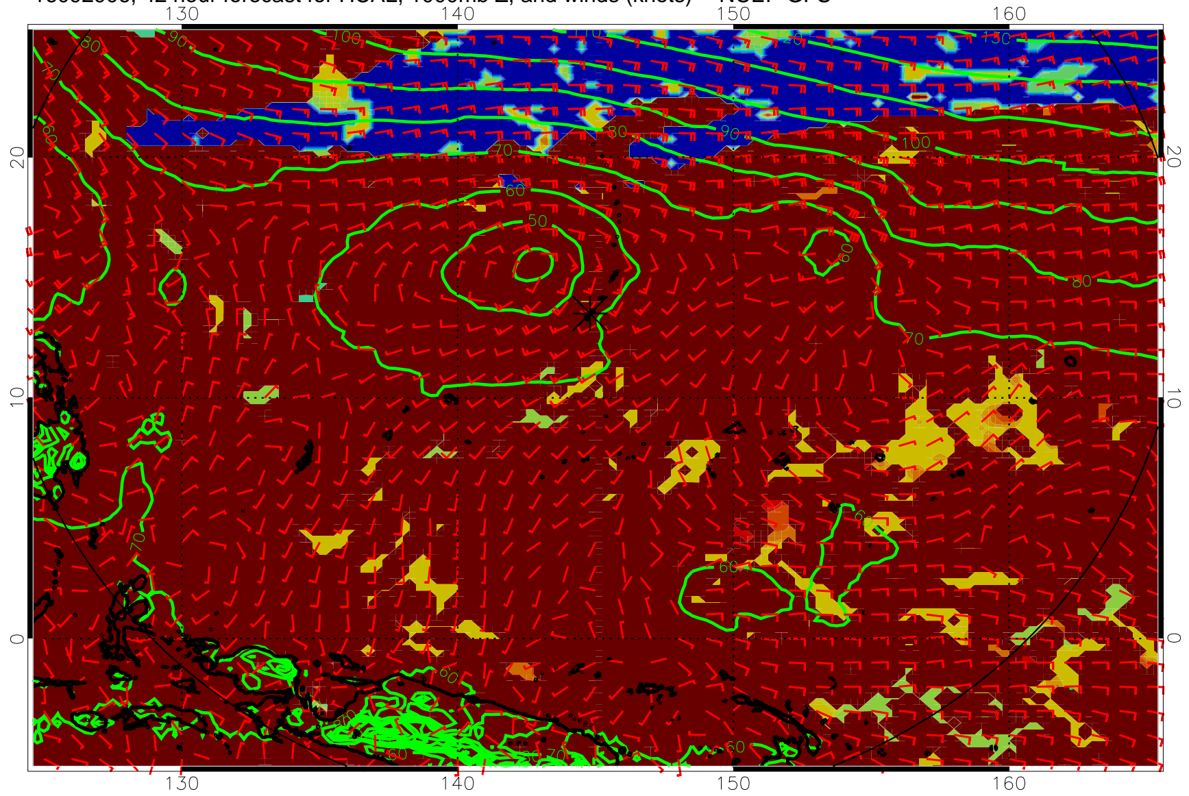
16092906, 42 hour forecast for HCAL, 1000mb Z, and winds (knots) -- NCEP GFS
