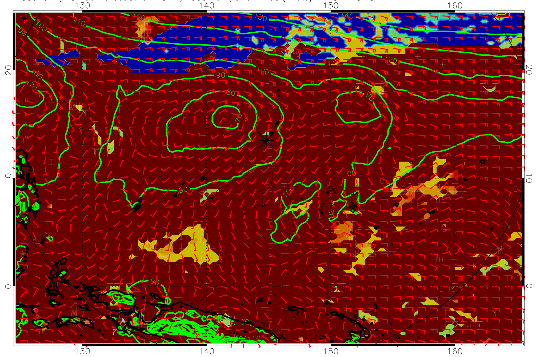
16092912, 48 hour forecast for HCAL, 1000mb Z, and winds (knots) -- NCEP GFS
