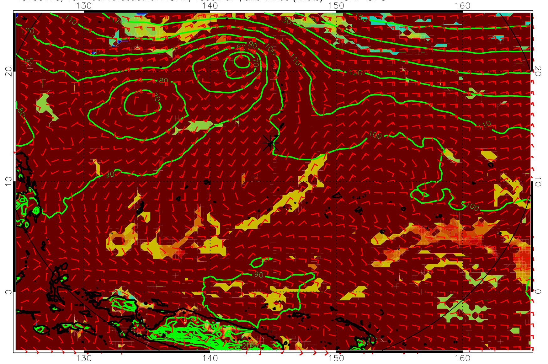
16100118, 102 hour forecast for HCAL, 1000mb Z, and winds (knots) -- NCEP GFS
