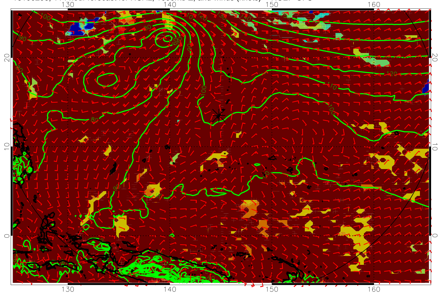
16100206, 114 hour forecast for HCAL, 1000mb Z, and winds (knots) -- NCEP GFS
