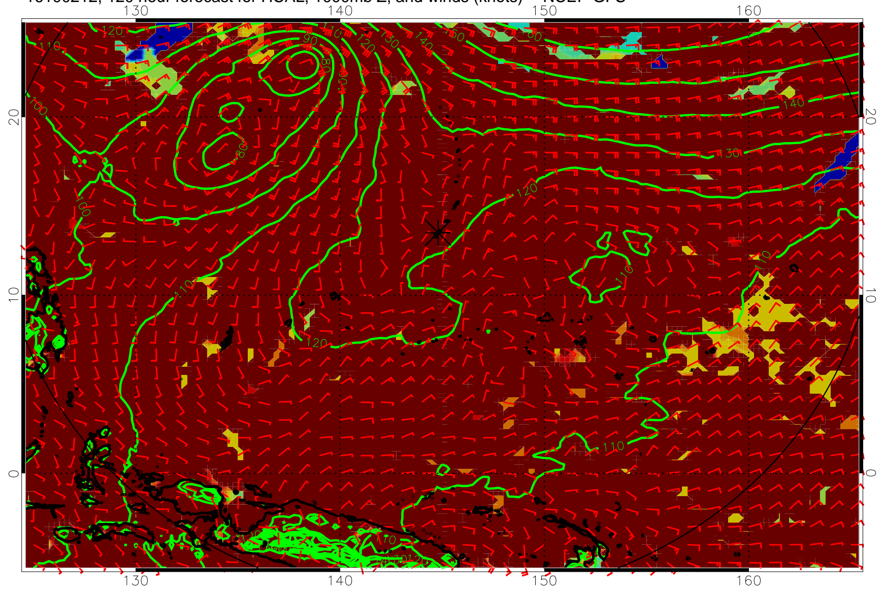
16100212, 120 hour forecast for HCAL, 1000mb Z, and winds (knots) -- NCEP GFS
