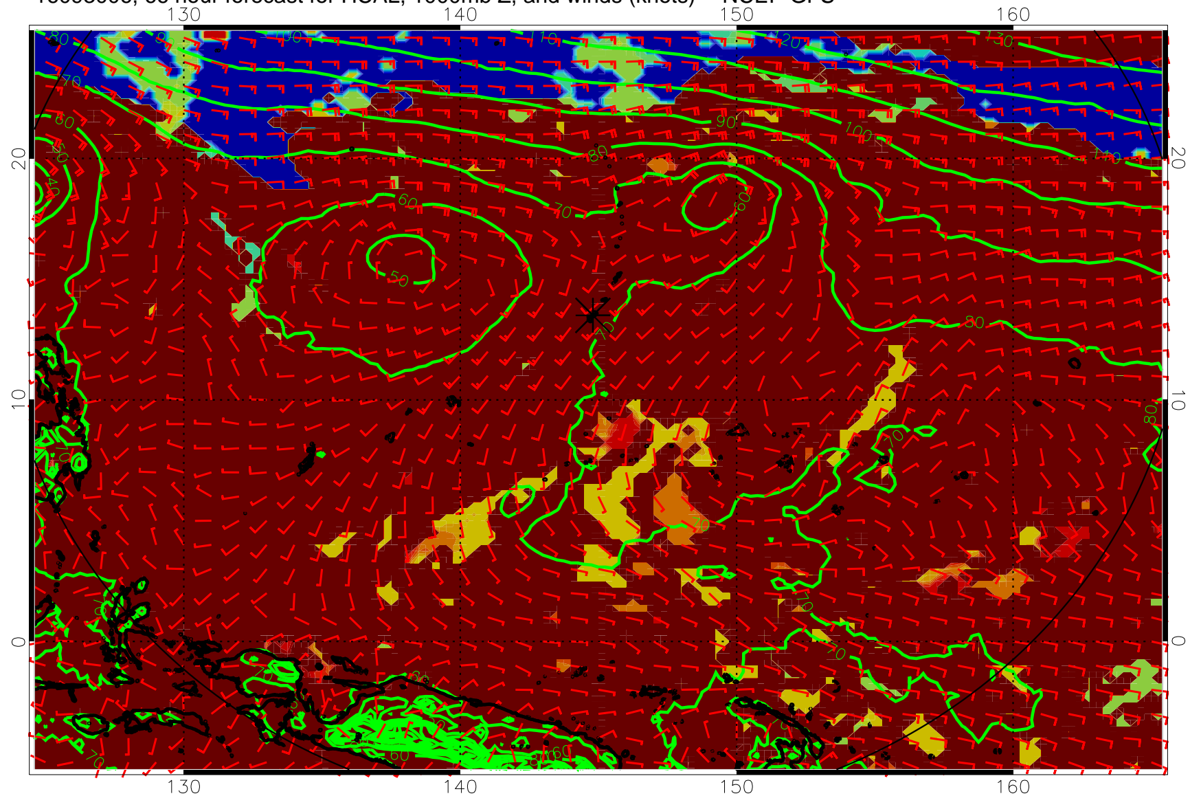
16093006, 66 hour forecast for HCAL, 1000mb Z, and winds (knots) -- NCEP GFS
