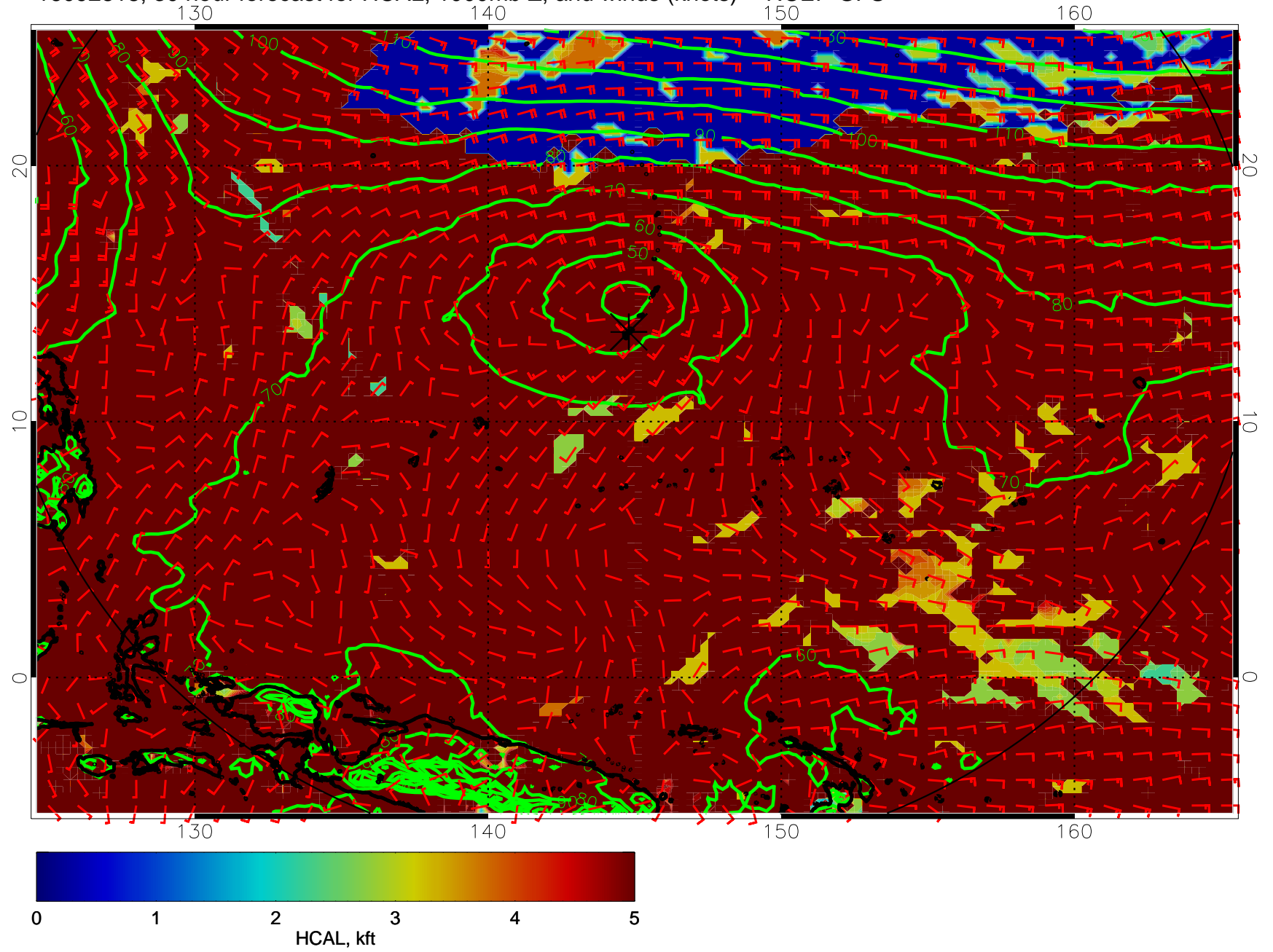
16092818, 30 hour forecast for HCAL, 1000mb Z, and winds (knots) -- NCEP GFS
