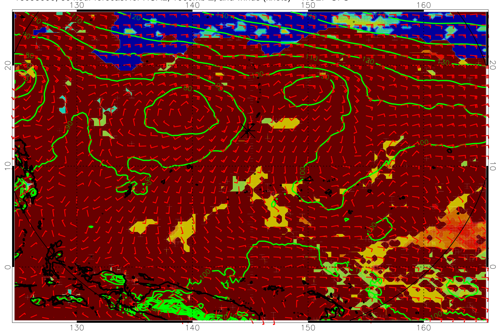
16093000, 60 hour forecast for HCAL, 1000mb Z, and winds (knots) -- NCEP GFS
