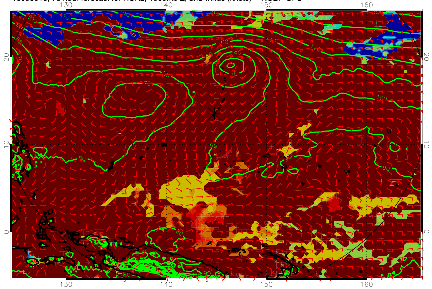
16093018, 78 hour forecast for HCAL, 1000mb Z, and winds (knots) -- NCEP GFS
