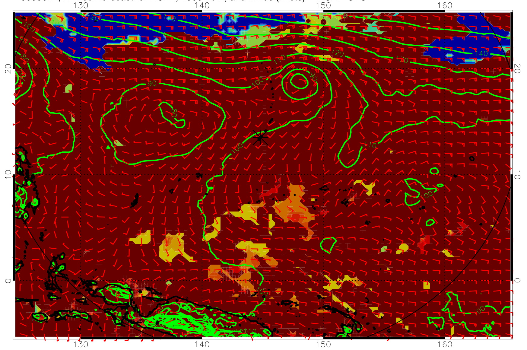
16093012, 72 hour forecast for HCAL, 1000mb Z, and winds (knots) -- NCEP GFS
