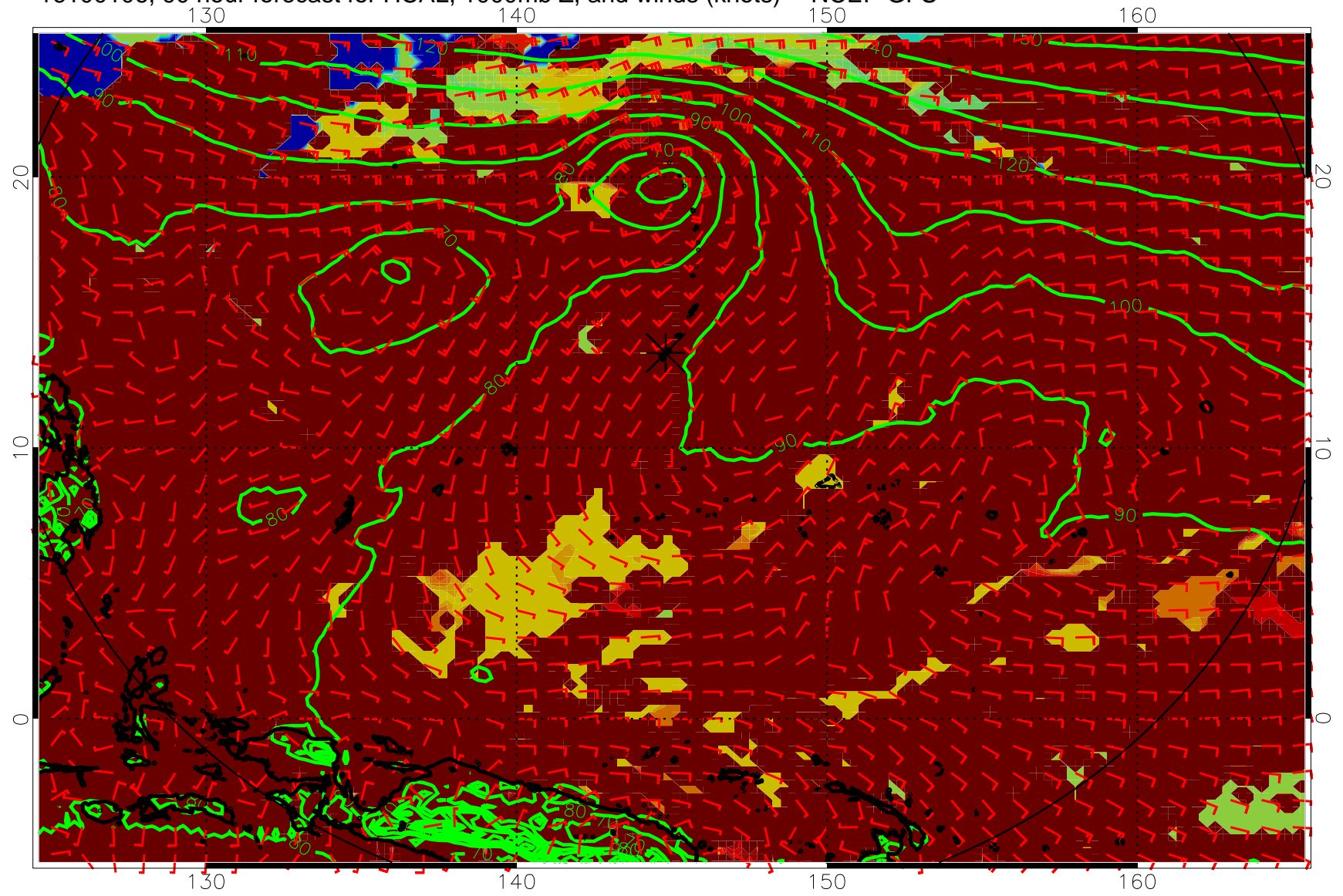
16100106, 90 hour forecast for HCAL, 1000mb Z, and winds (knots) -- NCEP GFS
