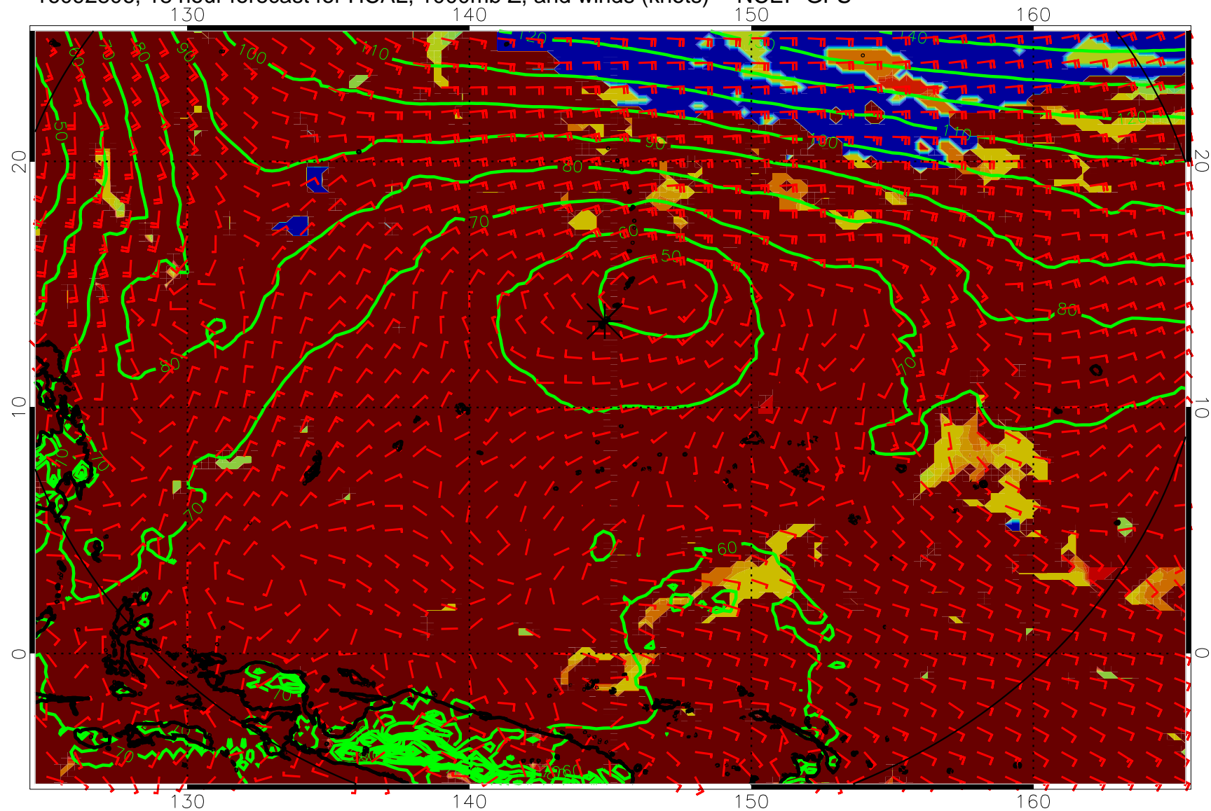
16092806, 18 hour forecast for HCAL, 1000mb Z, and winds (knots) -- NCEP GFS
