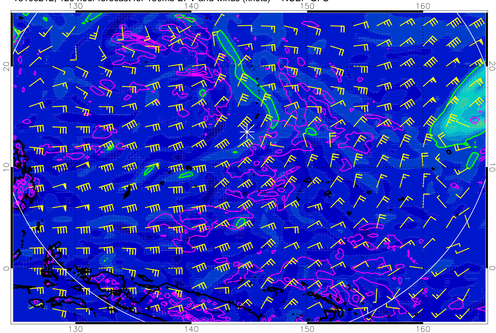
16100212, 120 hour forecast for 150mb EPV and winds (knots) -- NCEP GFS
