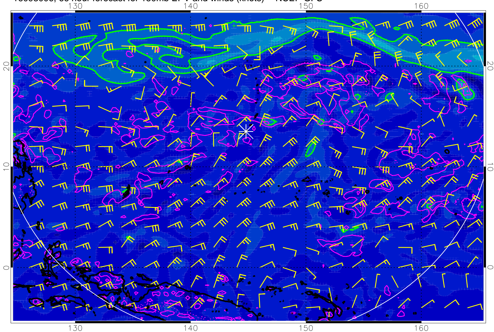
16093006, 66 hour forecast for 150mb EPV and winds (knots) -- NCEP GFS
