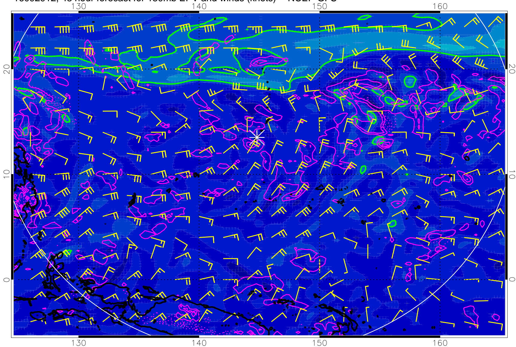
16092912, 48 hour forecast for 150mb EPV and winds (knots) -- NCEP GFS
