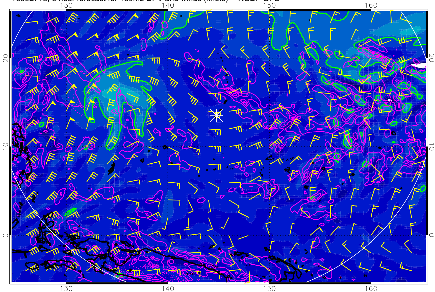
16092718, 6 hour forecast for 150mb EPV and winds (knots) -- NCEP GFS
