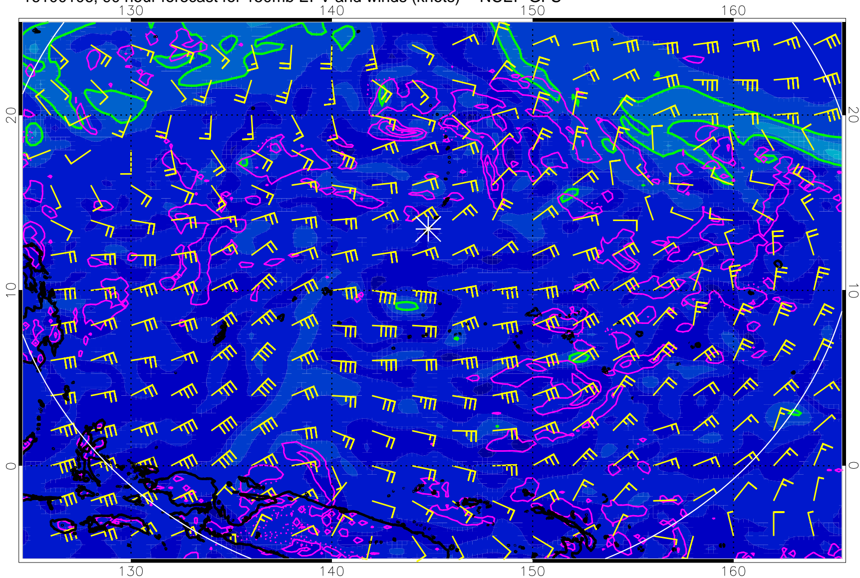
16100106, 90 hour forecast for 150mb EPV and winds (knots) -- NCEP GFS
