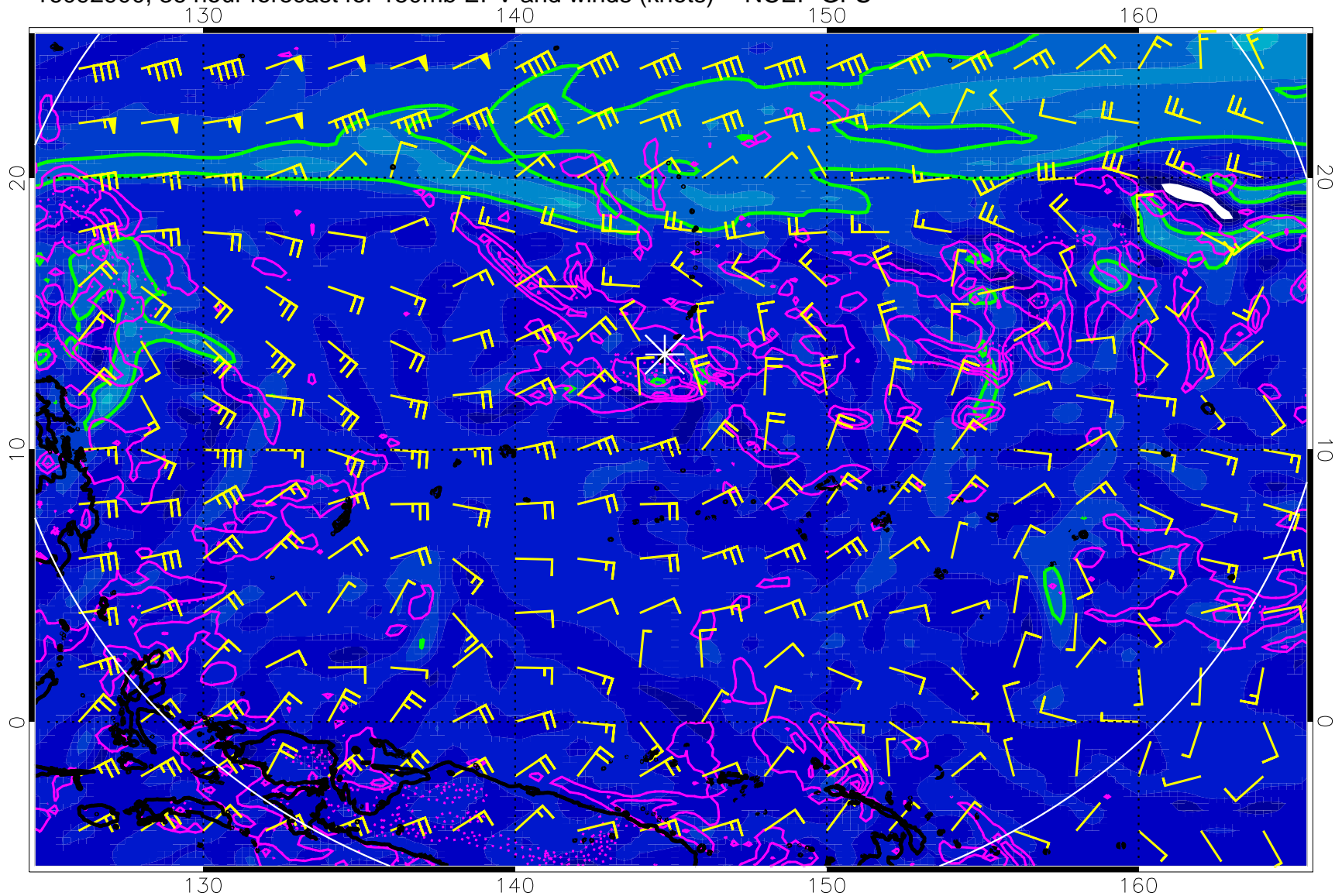
16092900, 36 hour forecast for 150mb EPV and winds (knots) -- NCEP GFS
