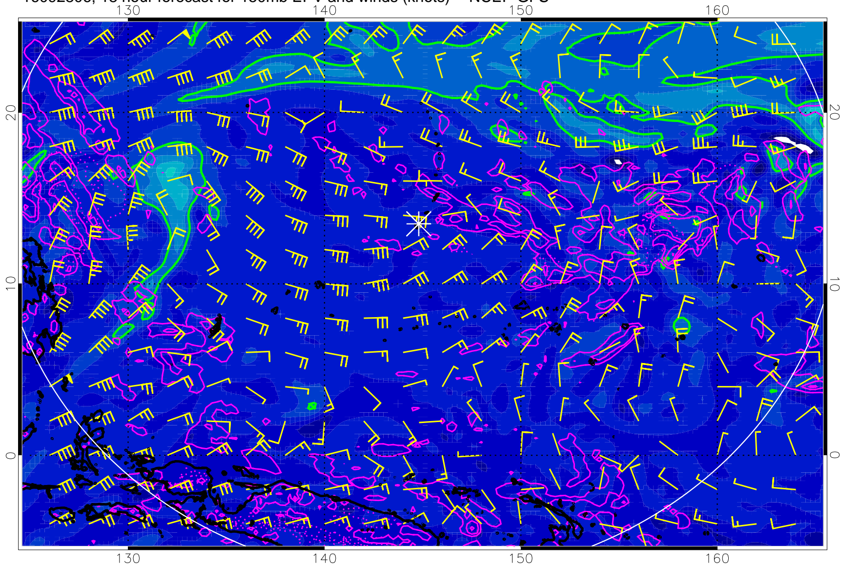
16092806, 18 hour forecast for 150mb EPV and winds (knots) -- NCEP GFS
