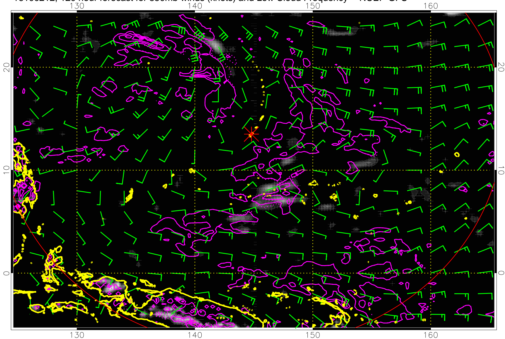
16100212, 120 hour forecast for 850mb winds (knots) and Low Cloud Frequency -- NCEP GFS
