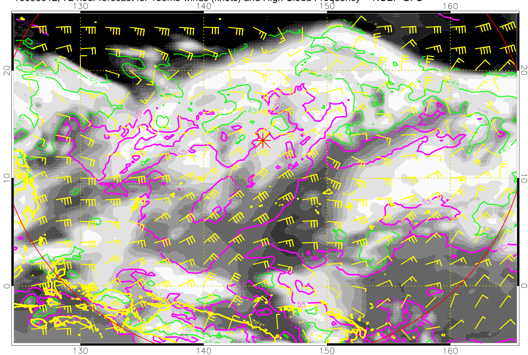
16093012, 72 hour forecast for 150mb winds (knots) and High Cloud Frequency -- NCEP GFS
