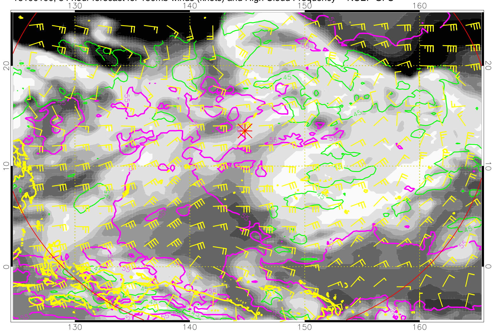
16100100, 84 hour forecast for 150mb winds (knots) and High Cloud Frequency -- NCEP GFS
