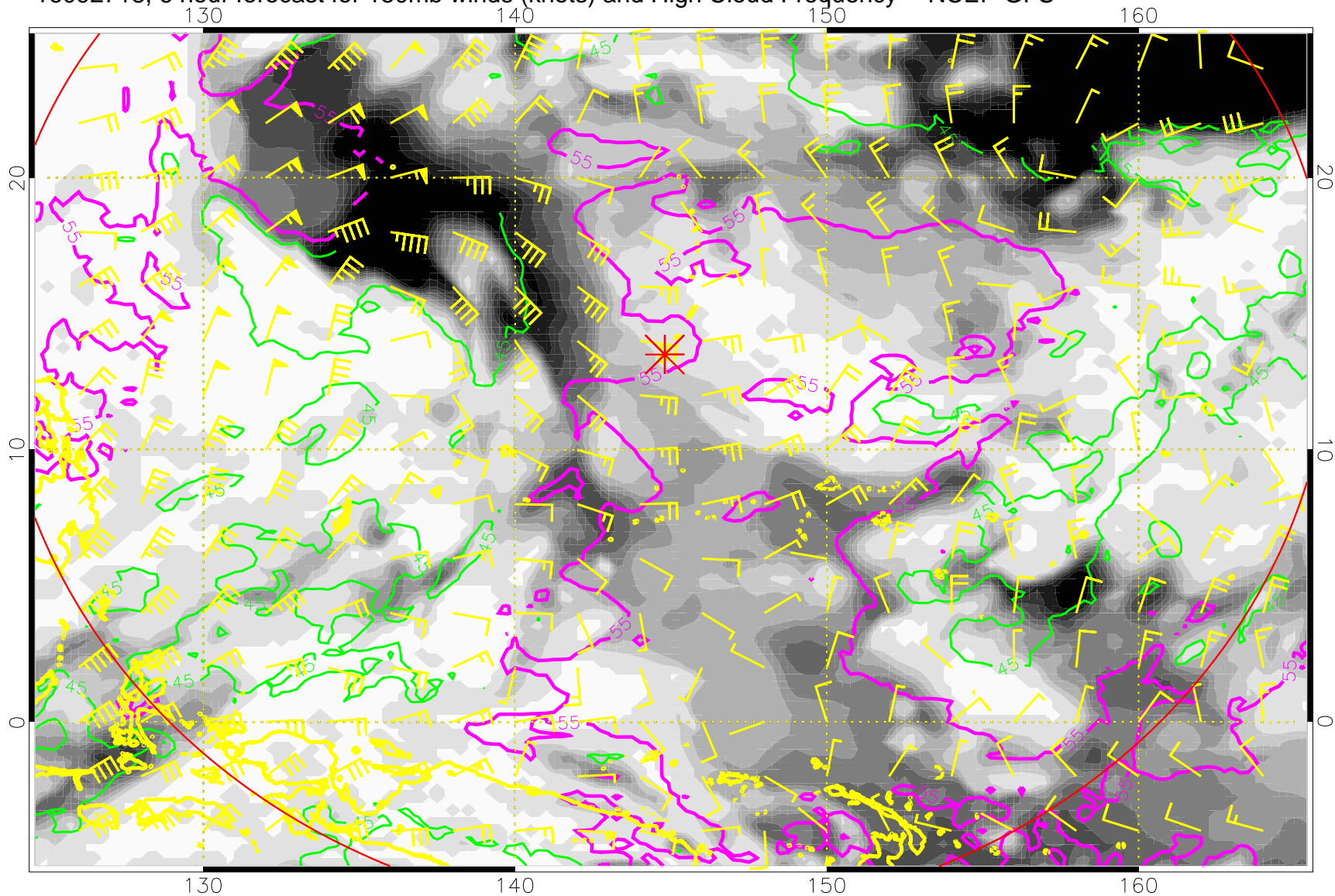
16092718, 6 hour forecast for 150mb winds (knots) and High Cloud Frequency -- NCEP GFS
