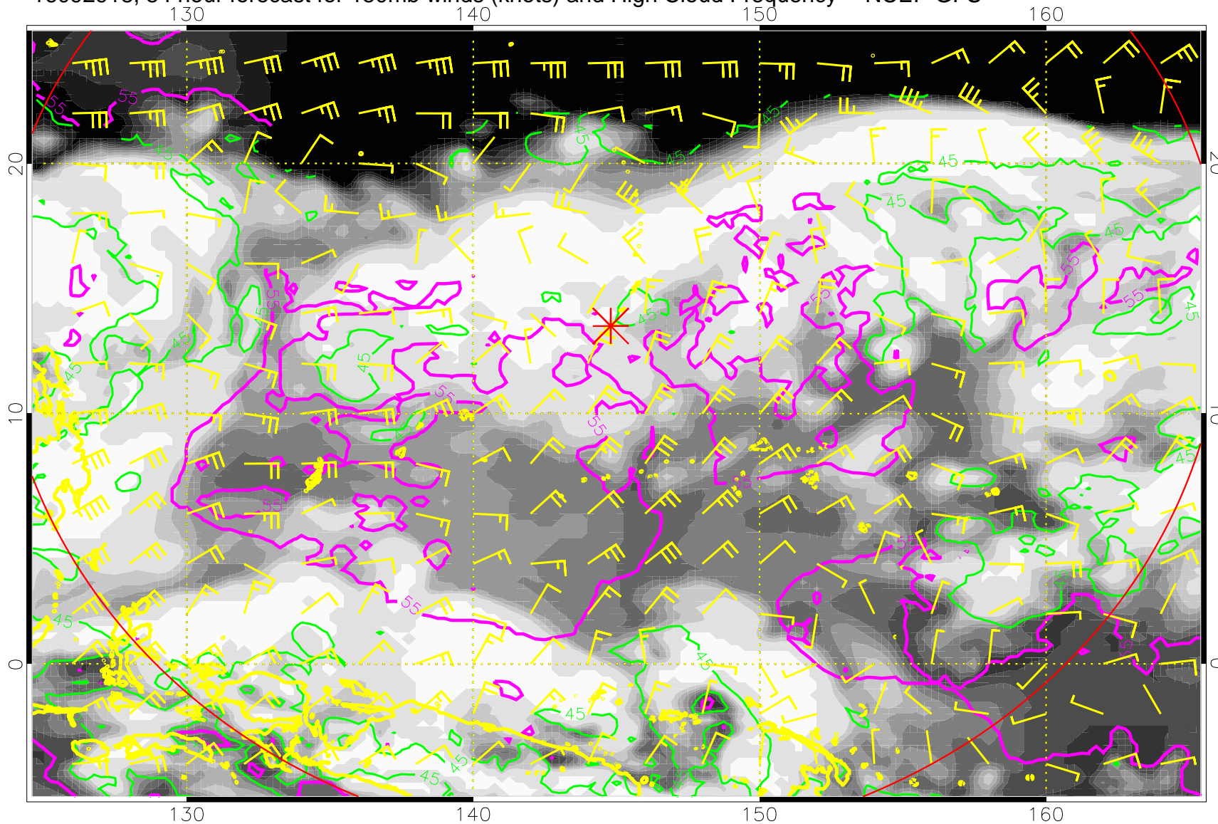
16092918, 54 hour forecast for 150mb winds (knots) and High Cloud Frequency -- NCEP GFS
