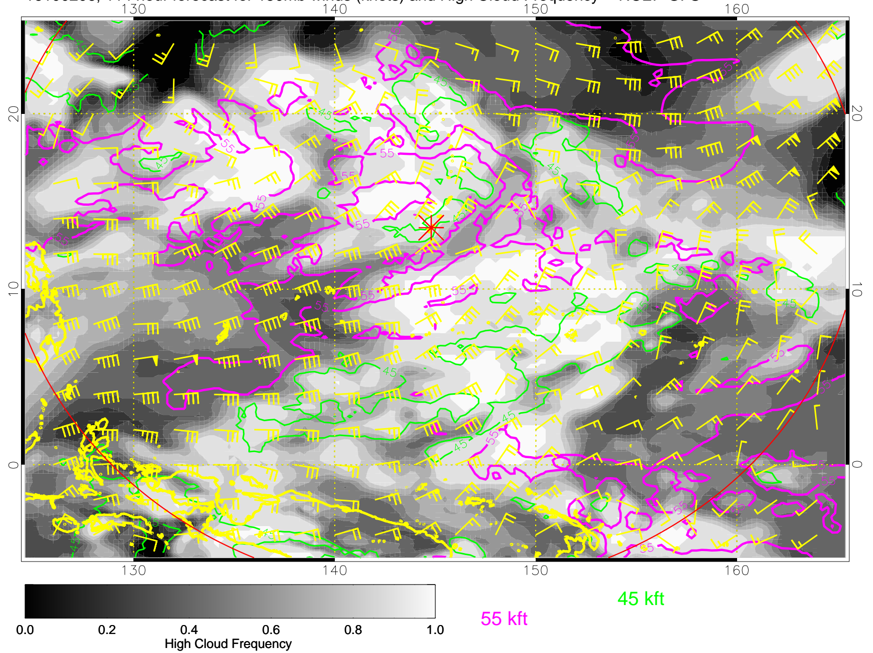
16100206, 114 hour forecast for 150mb winds (knots) and High Cloud Frequency -- NCEP GFS
