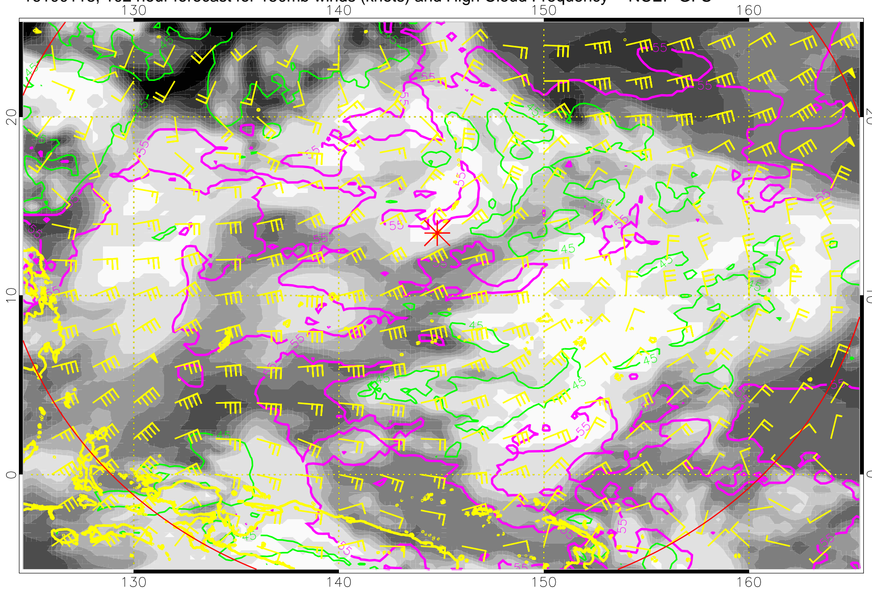
16100118, 102 hour forecast for 150mb winds (knots) and High Cloud Frequency -- NCEP GFS
