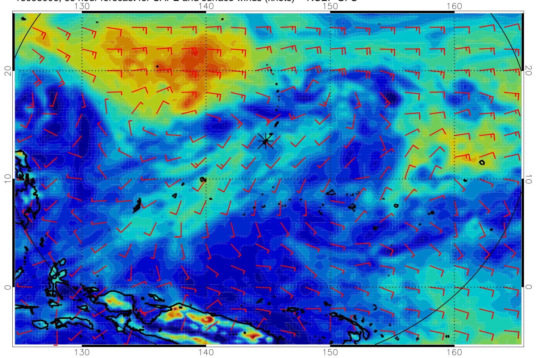
16093006, 66 hour forecast for CAPE and surface winds (knots) -- NCEP GFS
