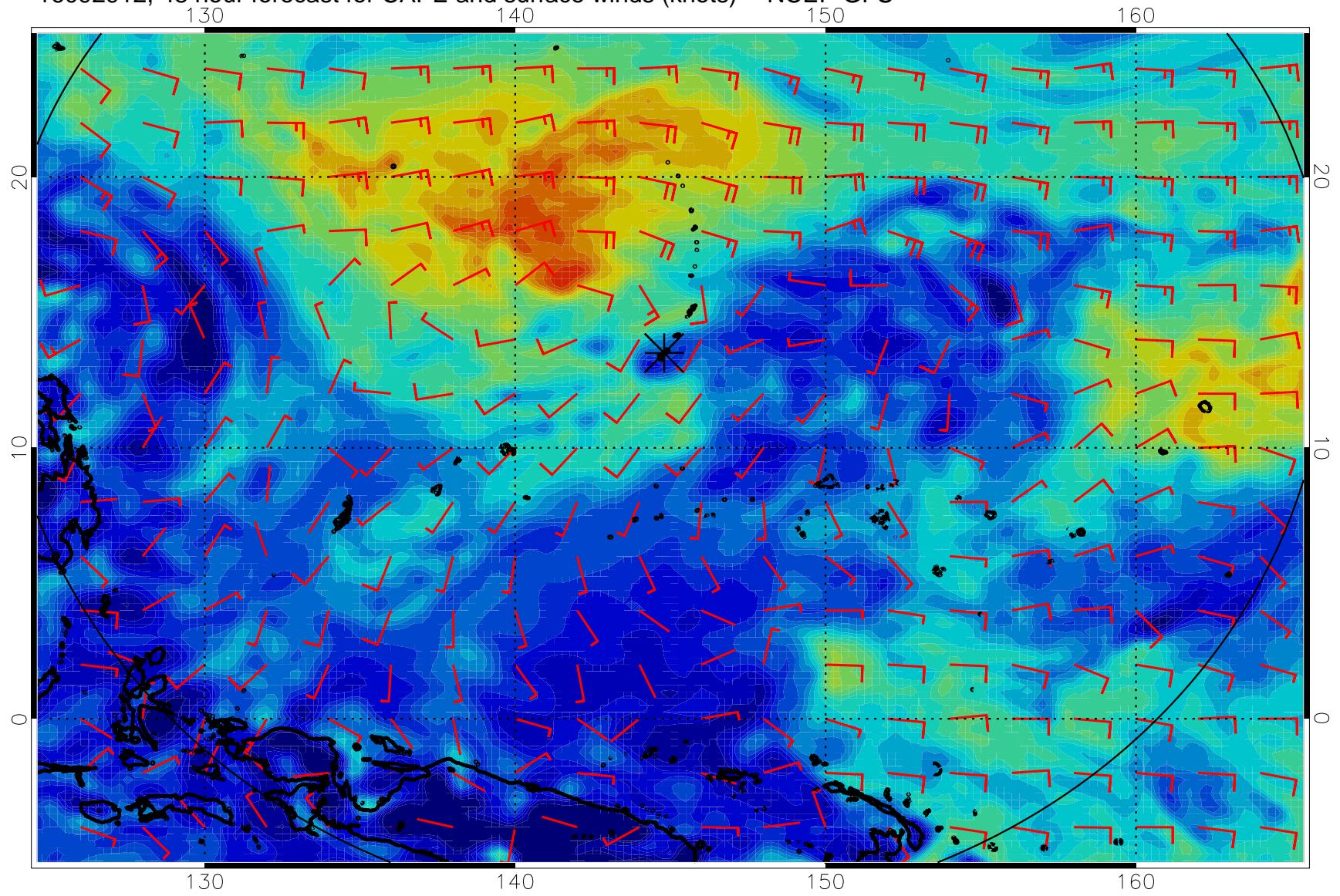
16092912, 48 hour forecast for CAPE and surface winds (knots) -- NCEP GFS
