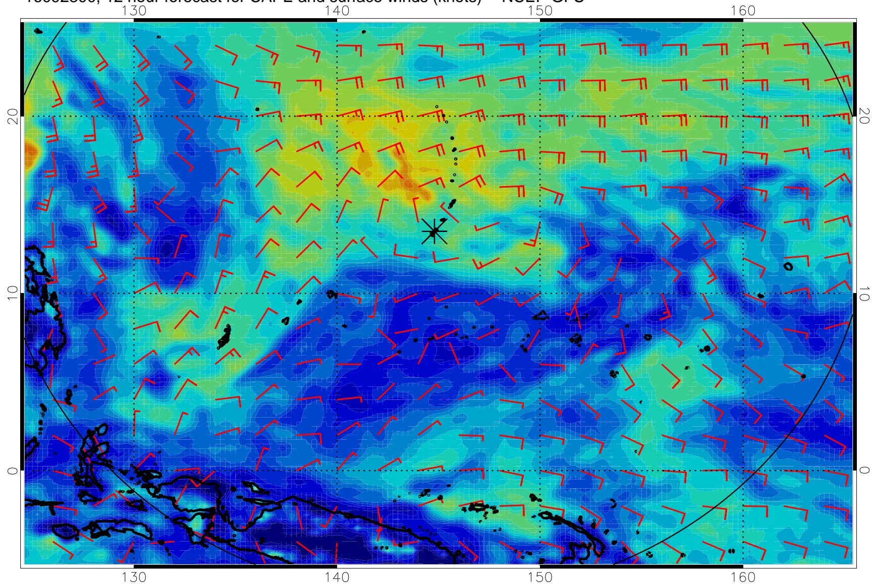
16092800, 12 hour forecast for CAPE and surface winds (knots) -- NCEP GFS
