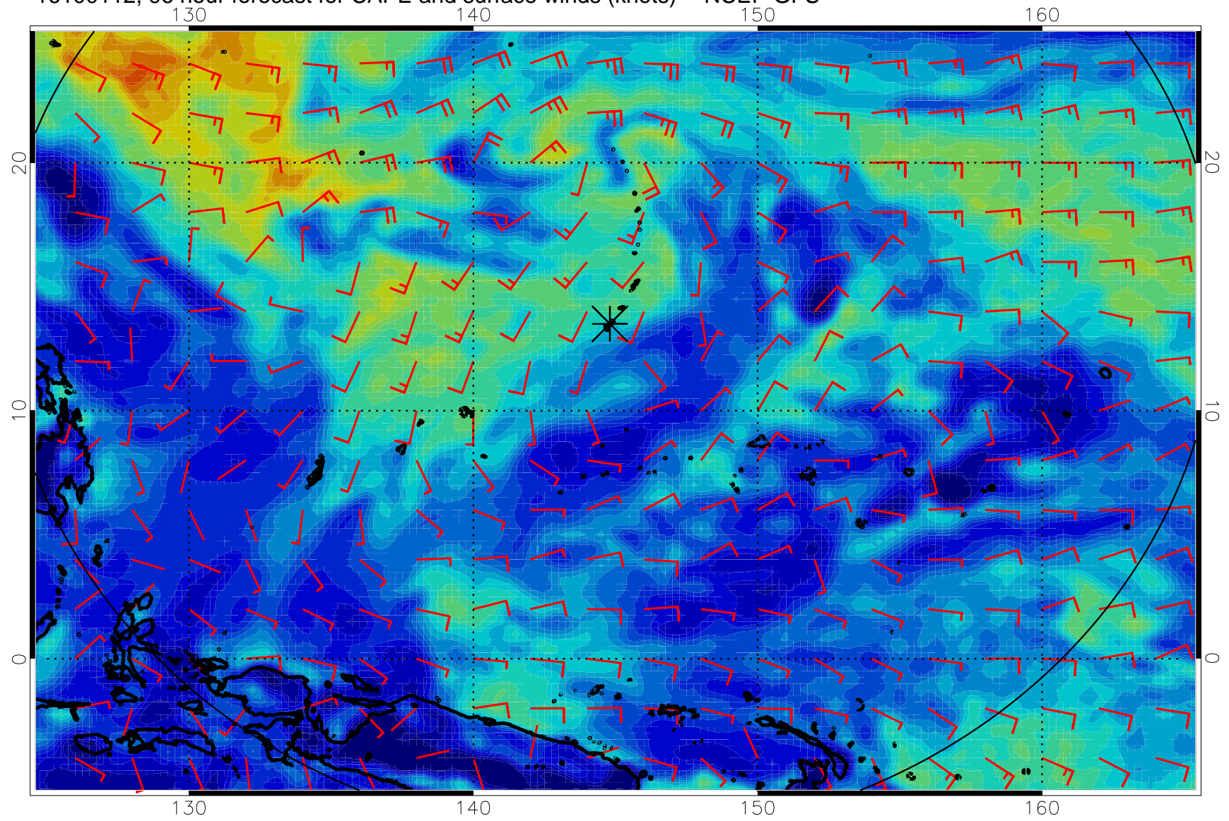
16100112, 96 hour forecast for CAPE and surface winds (knots) -- NCEP GFS
