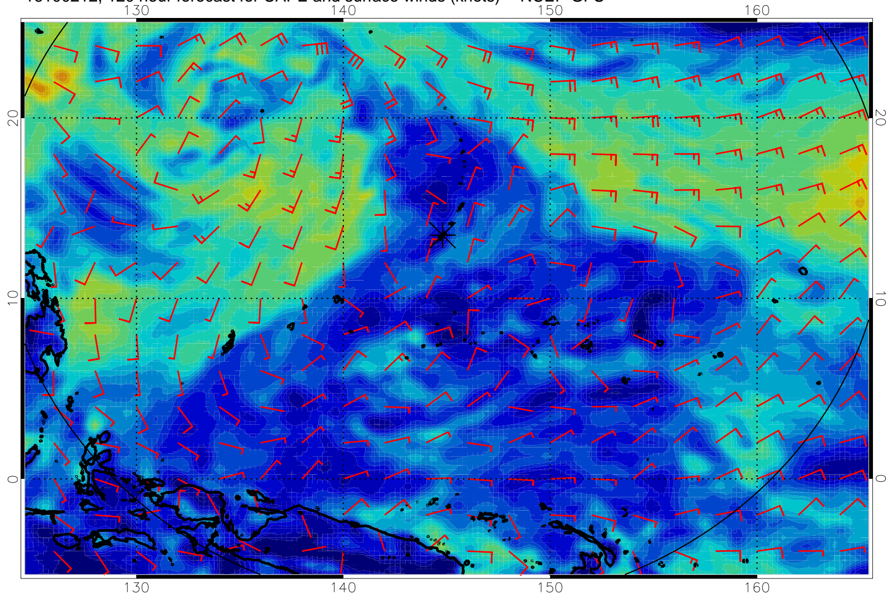
16100212, 120 hour forecast for CAPE and surface winds (knots) -- NCEP GFS
