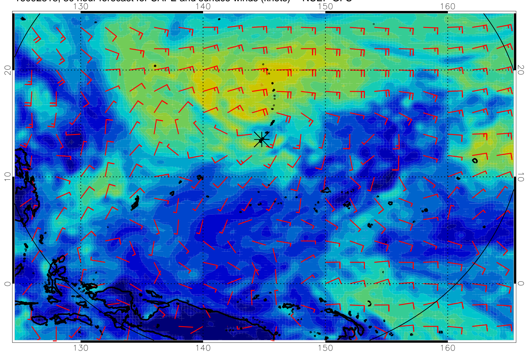
16092818, 30 hour forecast for CAPE and surface winds (knots) -- NCEP GFS
