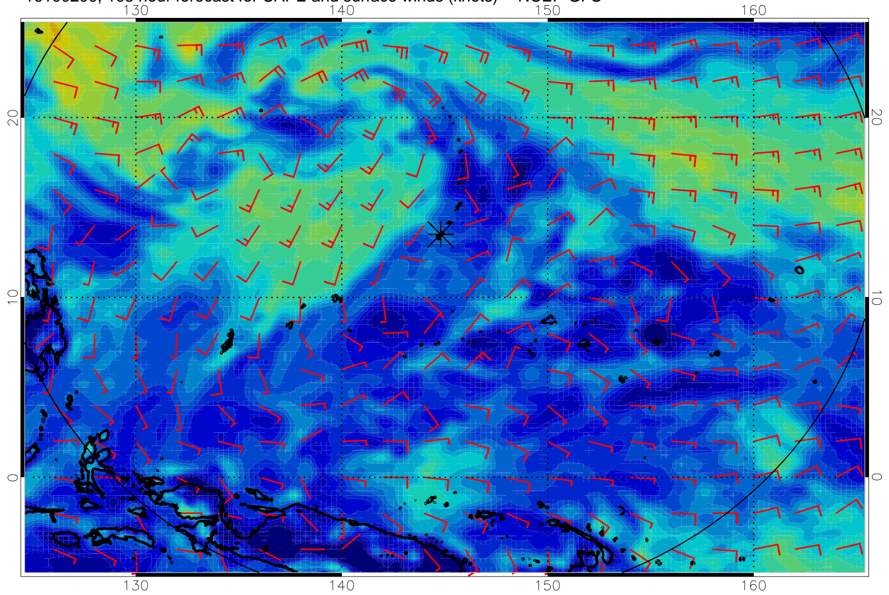
16100200, 108 hour forecast for CAPE and surface winds (knots) -- NCEP GFS
