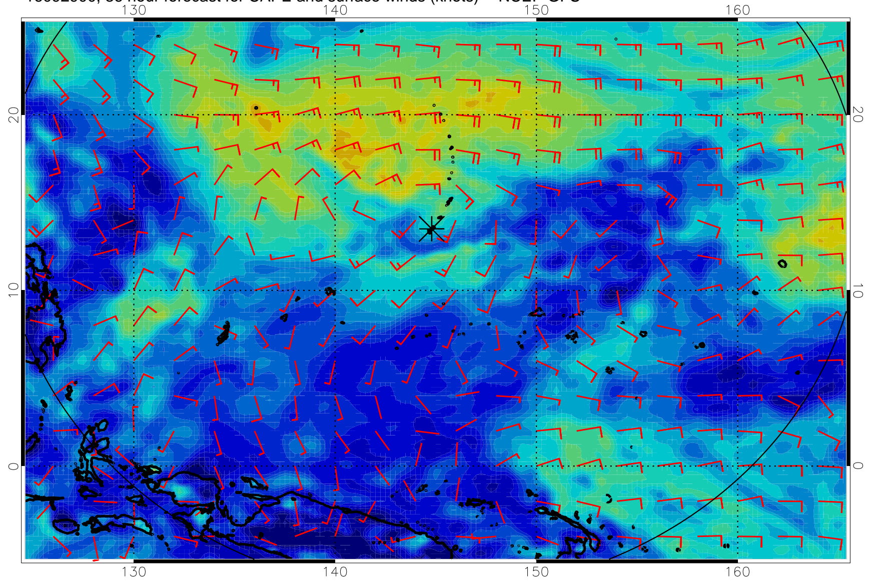
16092900, 36 hour forecast for CAPE and surface winds (knots) -- NCEP GFS
