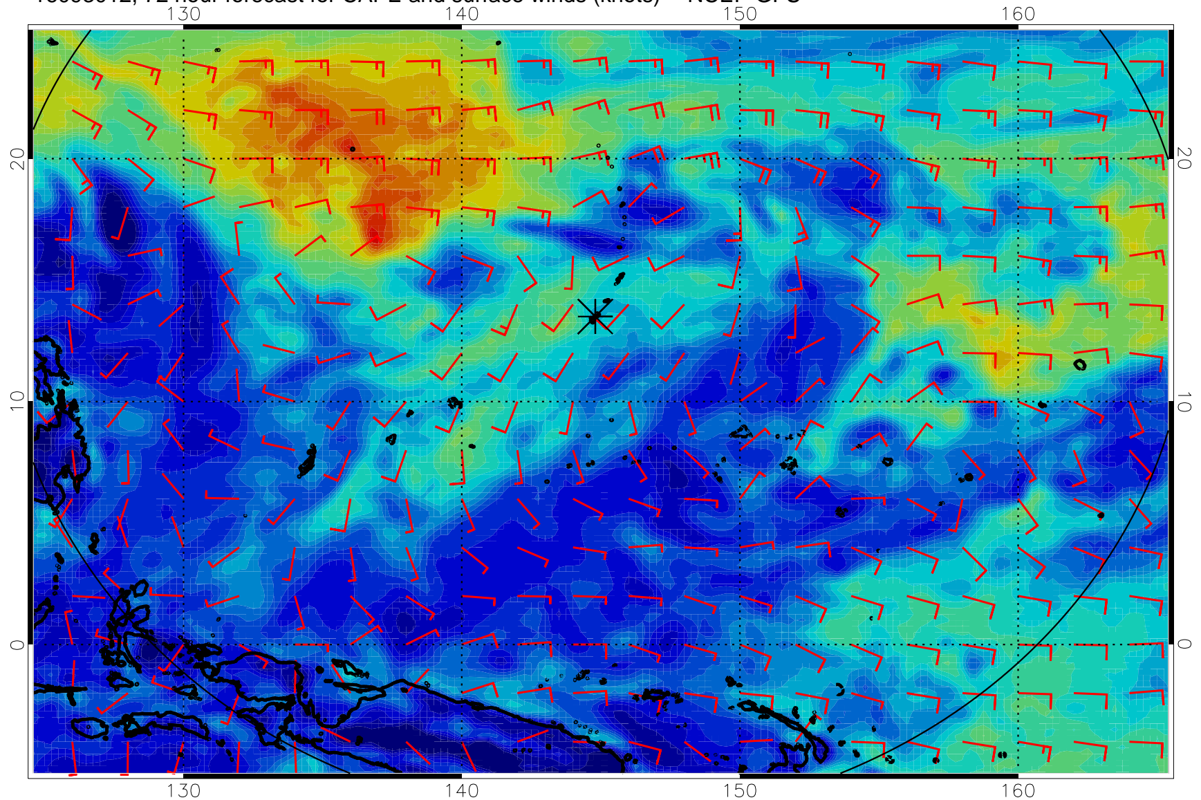
16093012, 72 hour forecast for CAPE and surface winds (knots) -- NCEP GFS
