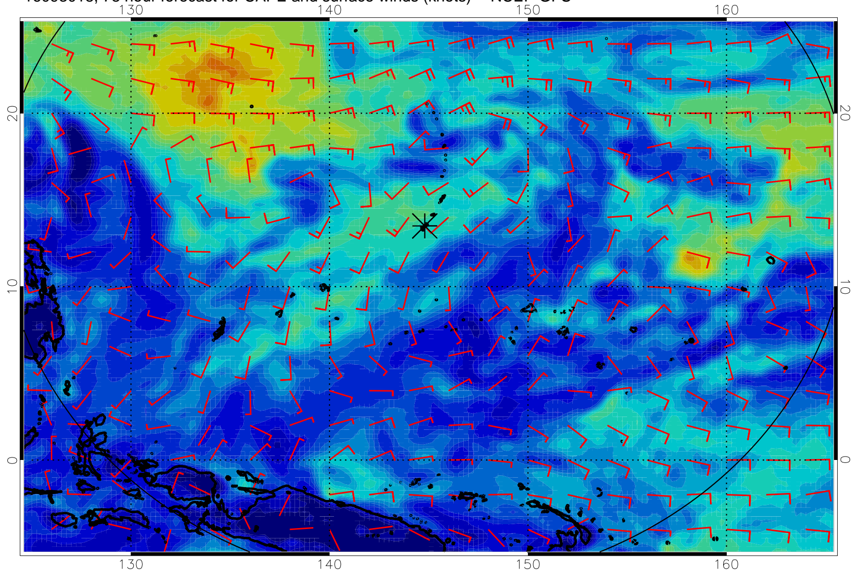
16093018, 78 hour forecast for CAPE and surface winds (knots) -- NCEP GFS
