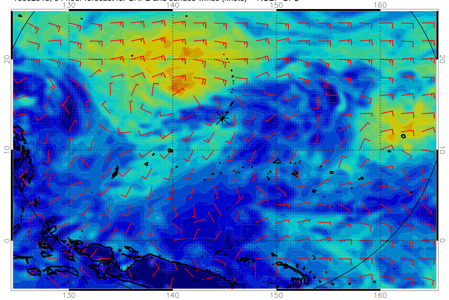
16092918, 54 hour forecast for CAPE and surface winds (knots) -- NCEP GFS
