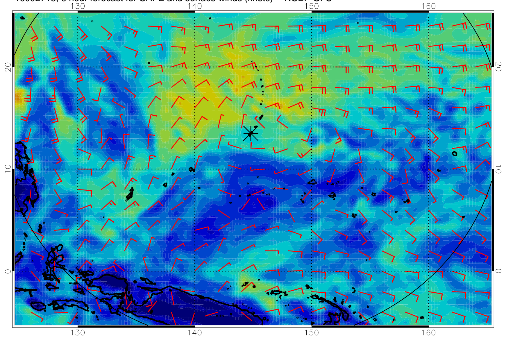
16092718, 6 hour forecast for CAPE and surface winds (knots) -- NCEP GFS
