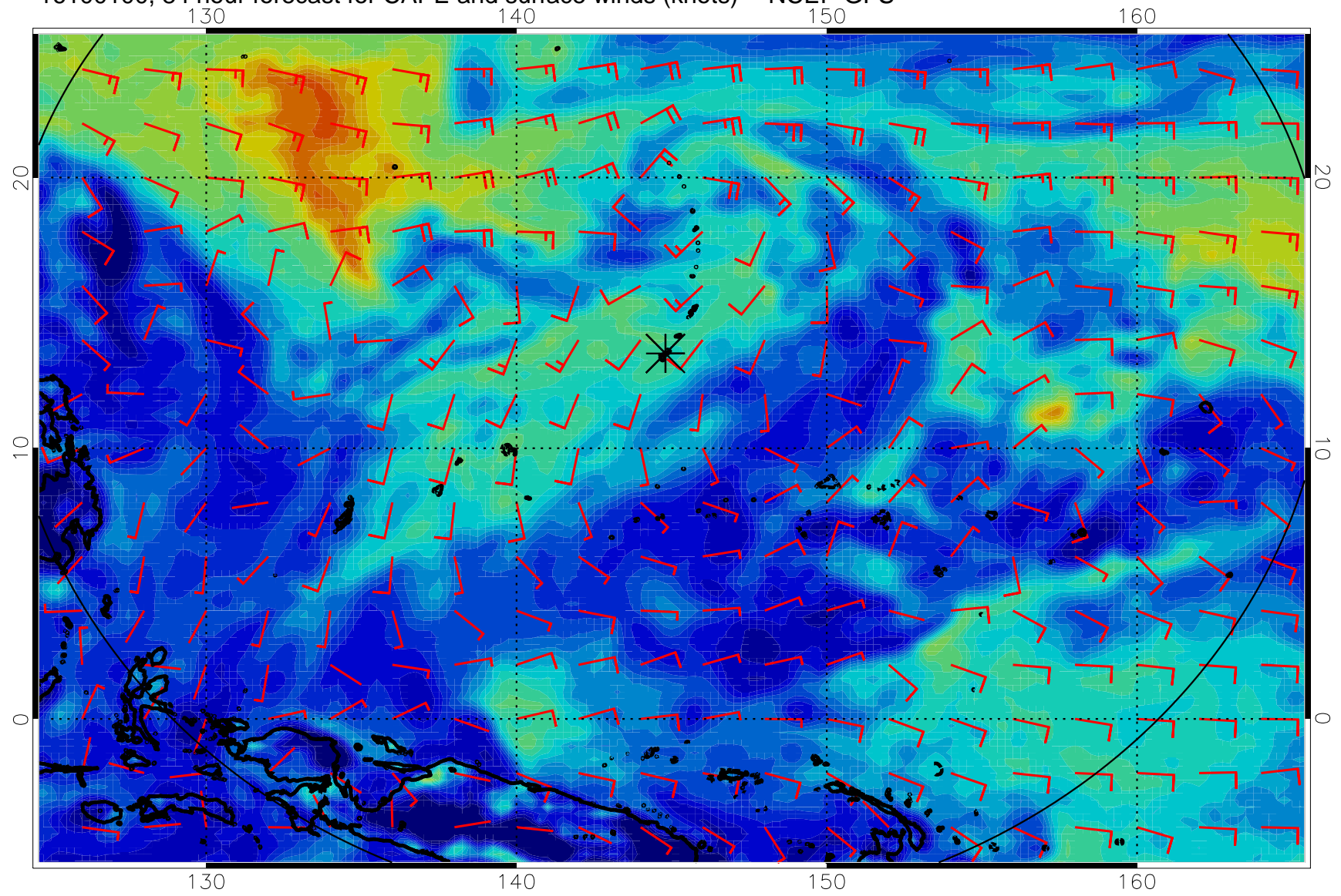
16100100, 84 hour forecast for CAPE and surface winds (knots) -- NCEP GFS
