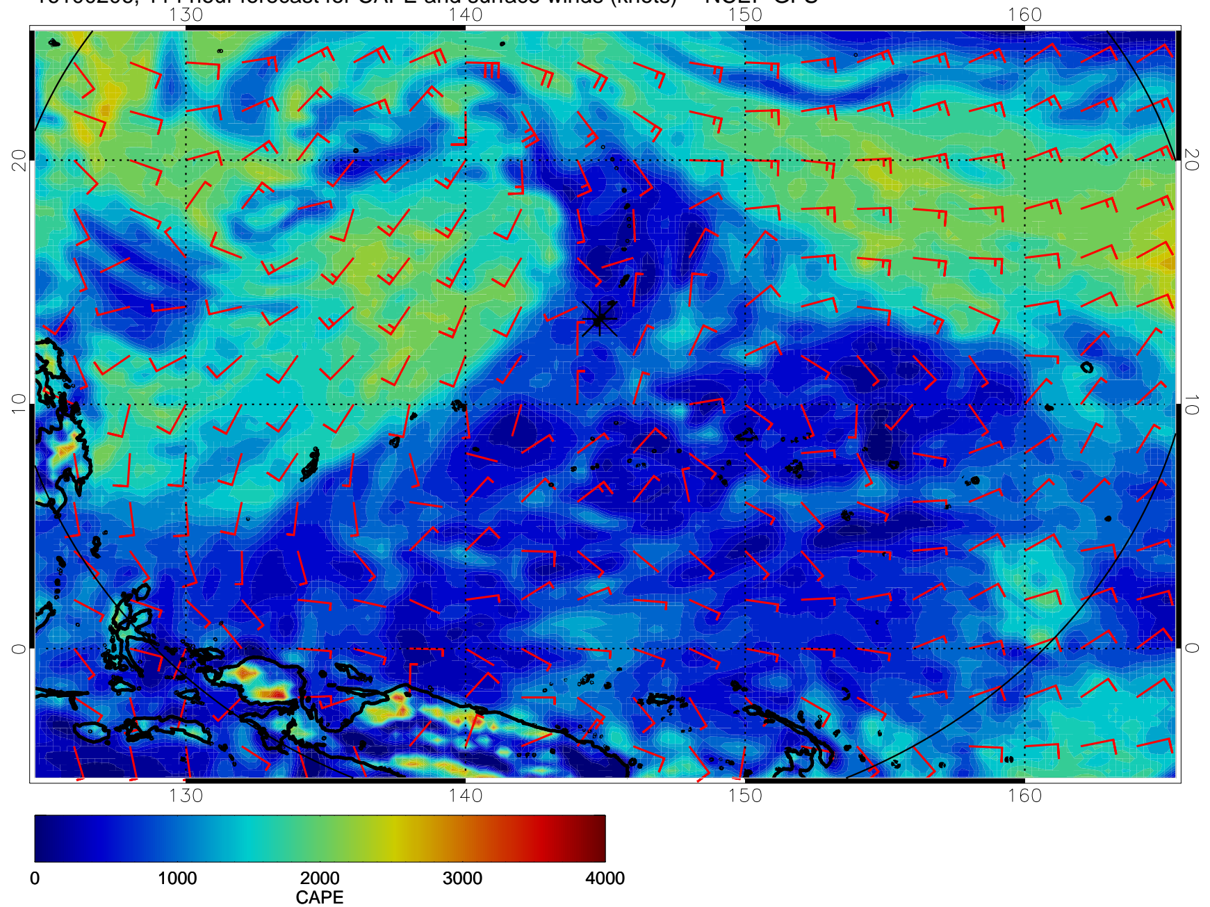
16100206, 114 hour forecast for CAPE and surface winds (knots) -- NCEP GFS
