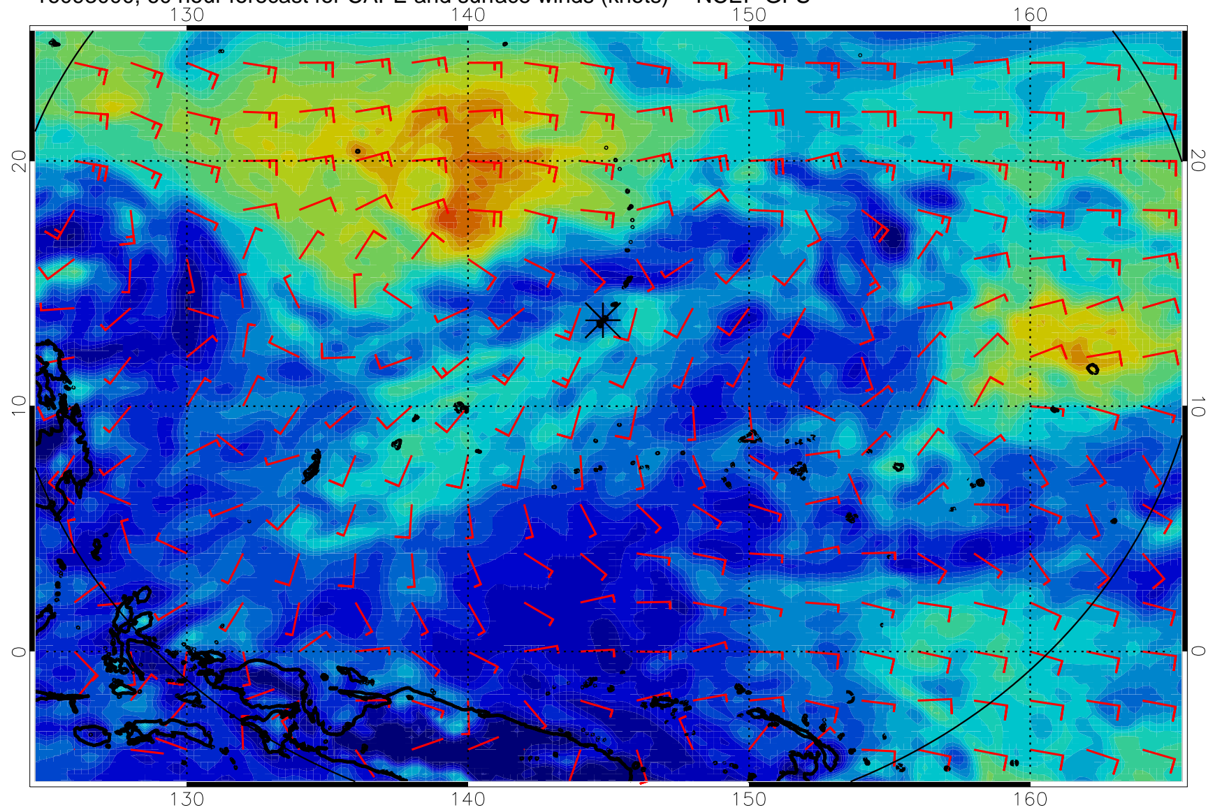
16093000, 60 hour forecast for CAPE and surface winds (knots) -- NCEP GFS
