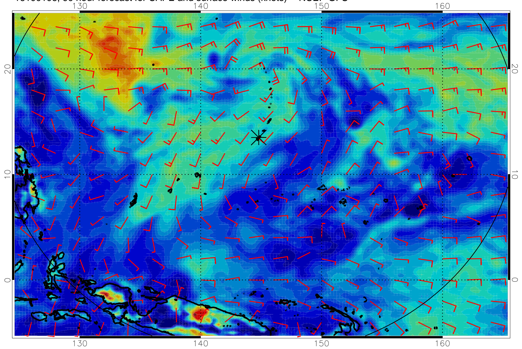
16100106, 90 hour forecast for CAPE and surface winds (knots) -- NCEP GFS
