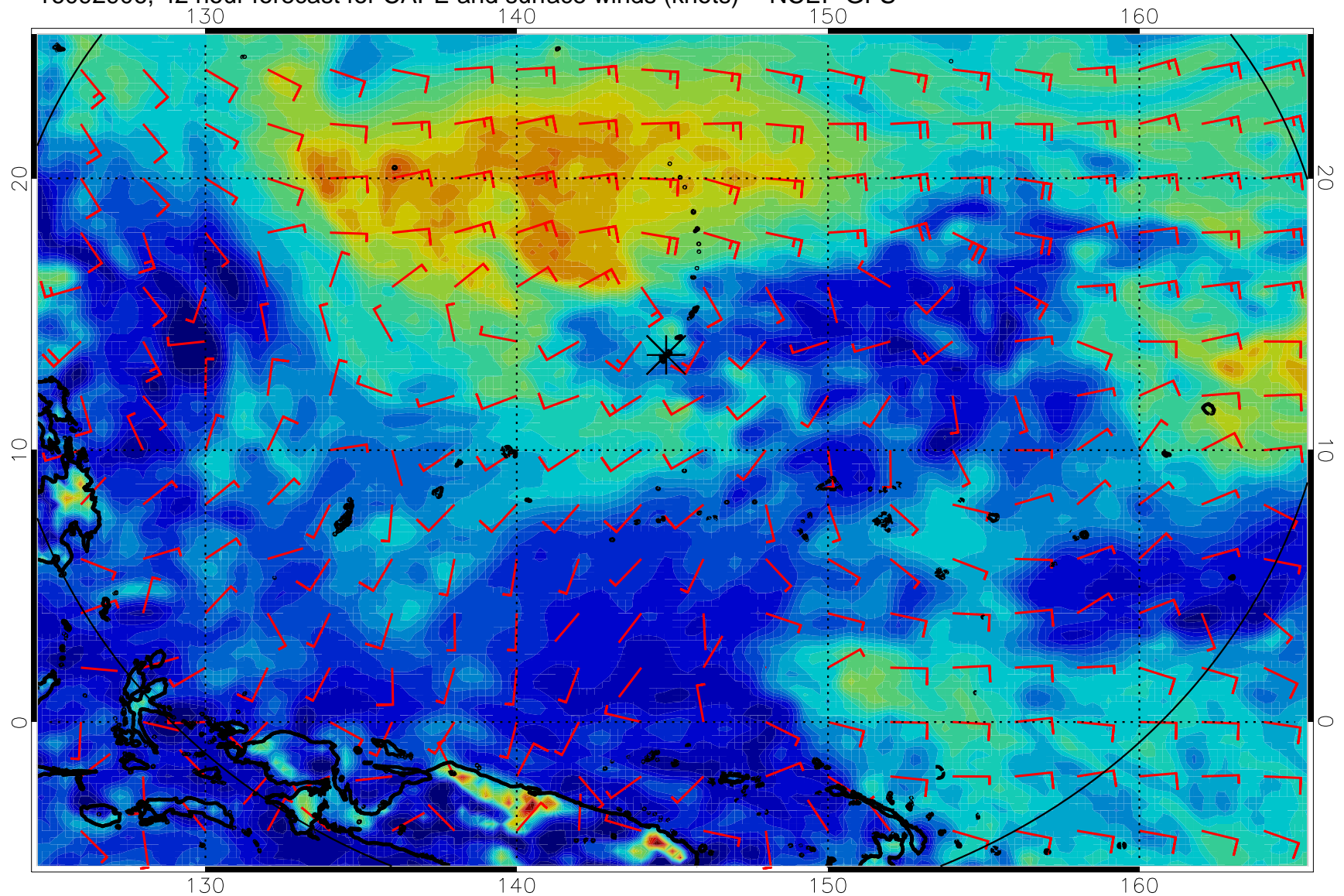
16092906, 42 hour forecast for CAPE and surface winds (knots) -- NCEP GFS
