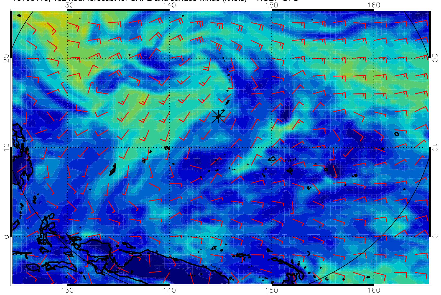
16100118, 102 hour forecast for CAPE and surface winds (knots) -- NCEP GFS
