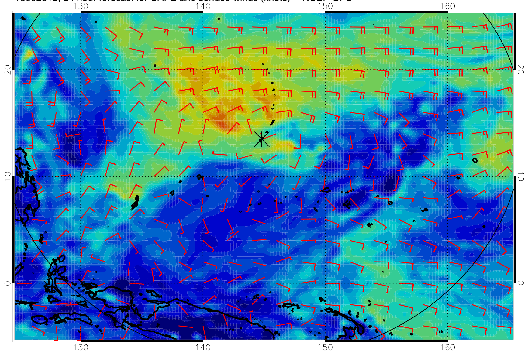
16092812, 24 hour forecast for CAPE and surface winds (knots) -- NCEP GFS
