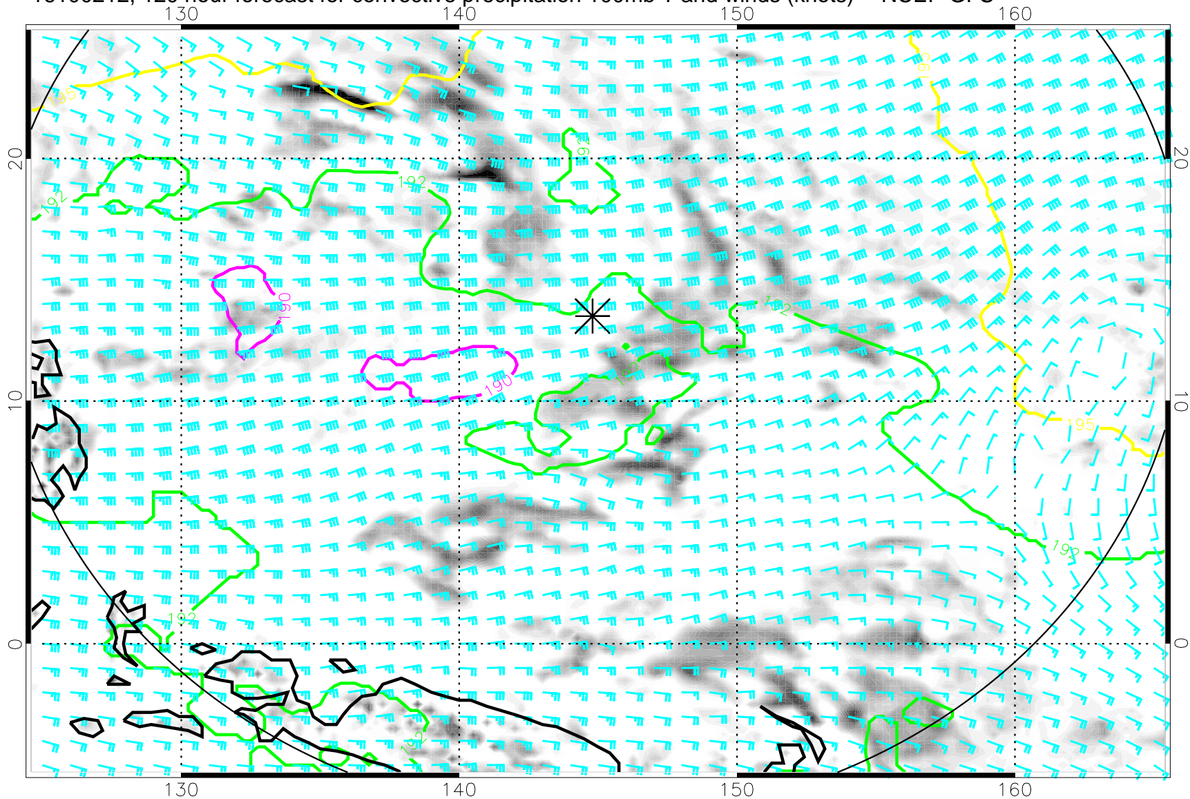
16100212, 120 hour forecast for convective precipitation 100mb T and winds (knots) -- NCEP GFS
