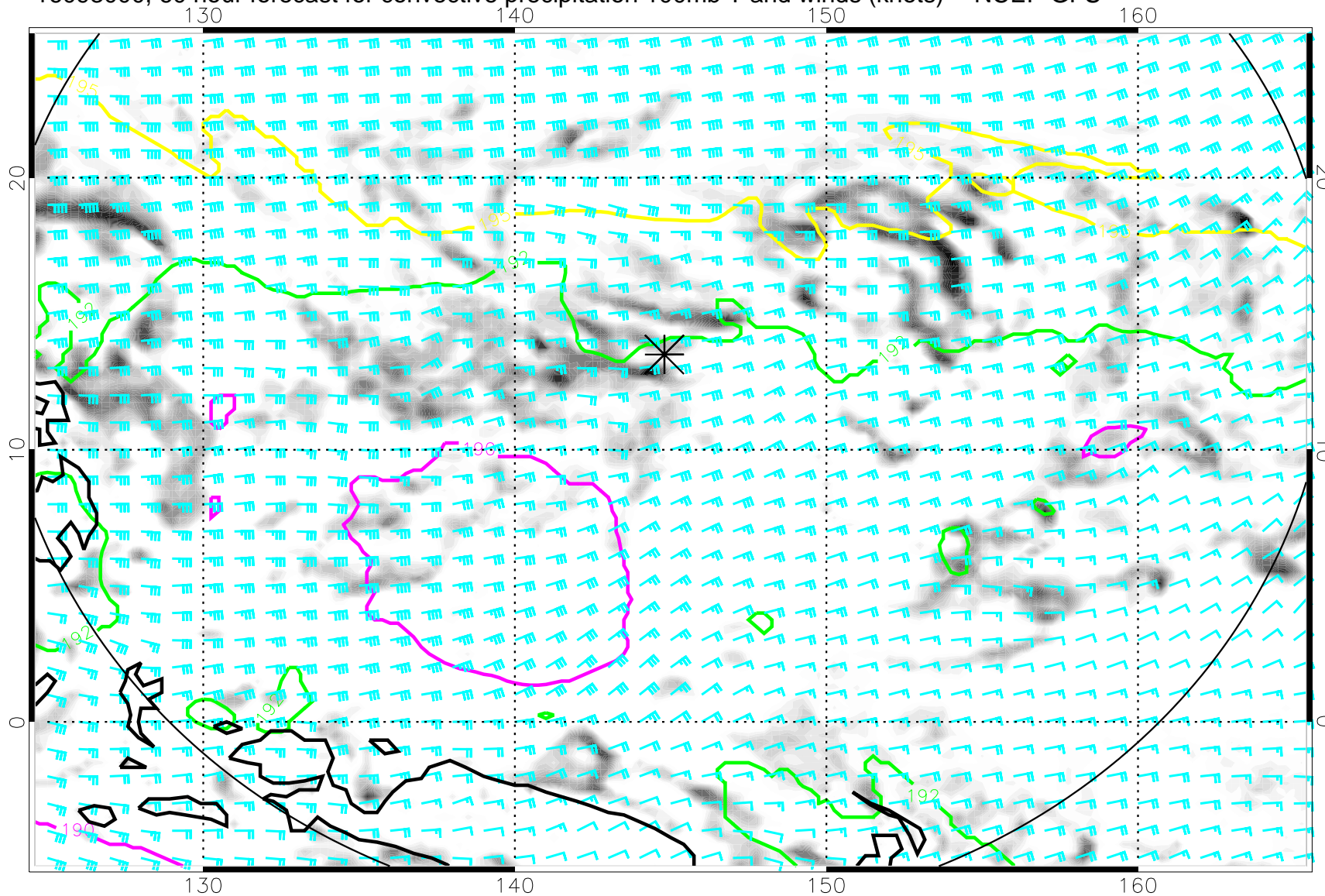
16093000, 60 hour forecast for convective precipitation 100mb T and winds (knots) -- NCEP GFS
