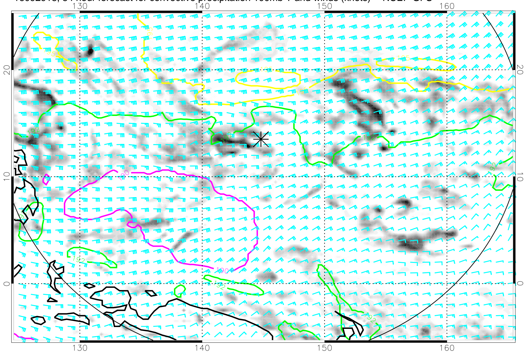
16092918, 54 hour forecast for convective precipitation 100mb T and winds (knots) -- NCEP GFS
