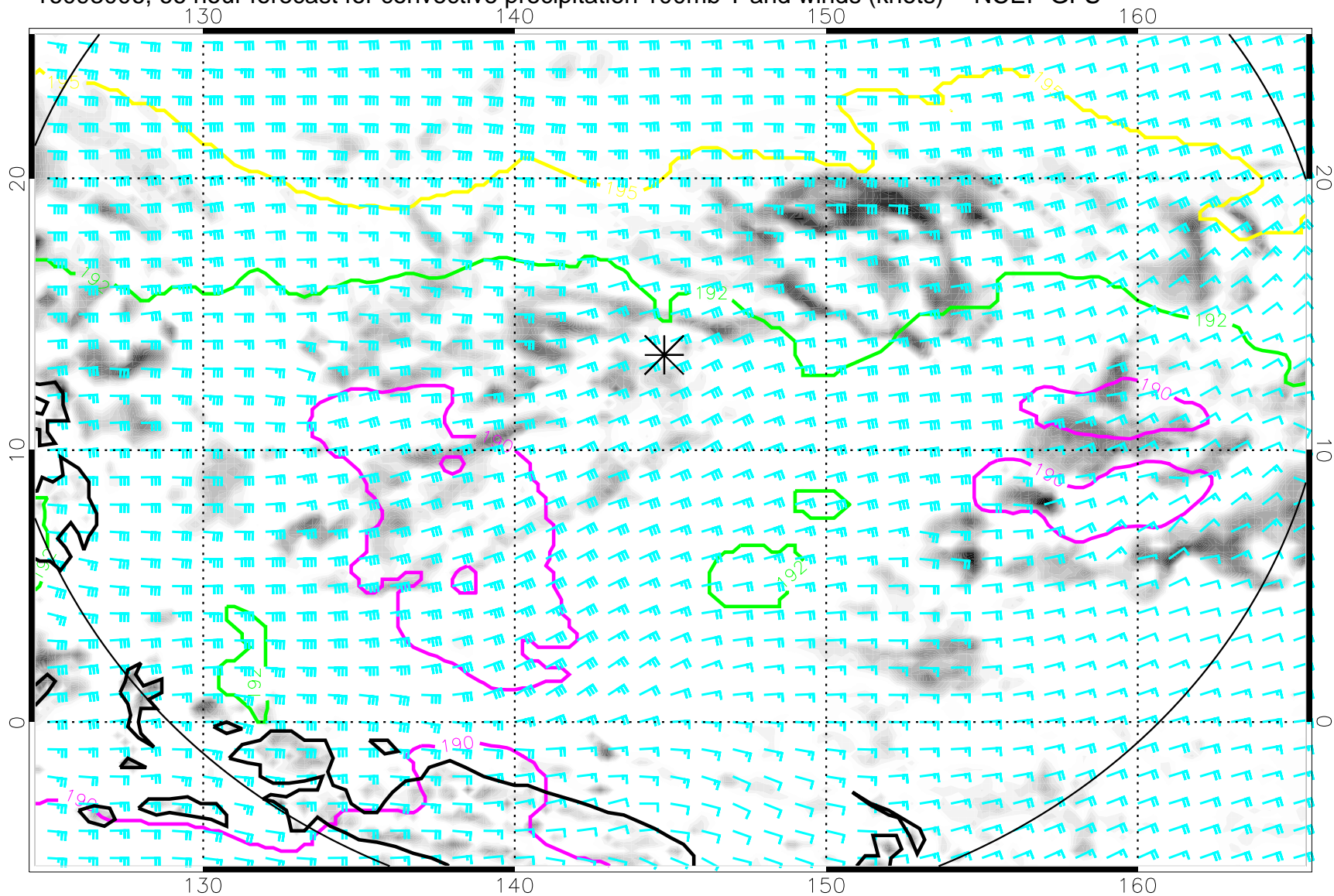
16093006, 66 hour forecast for convective precipitation 100mb T and winds (knots) -- NCEP GFS
