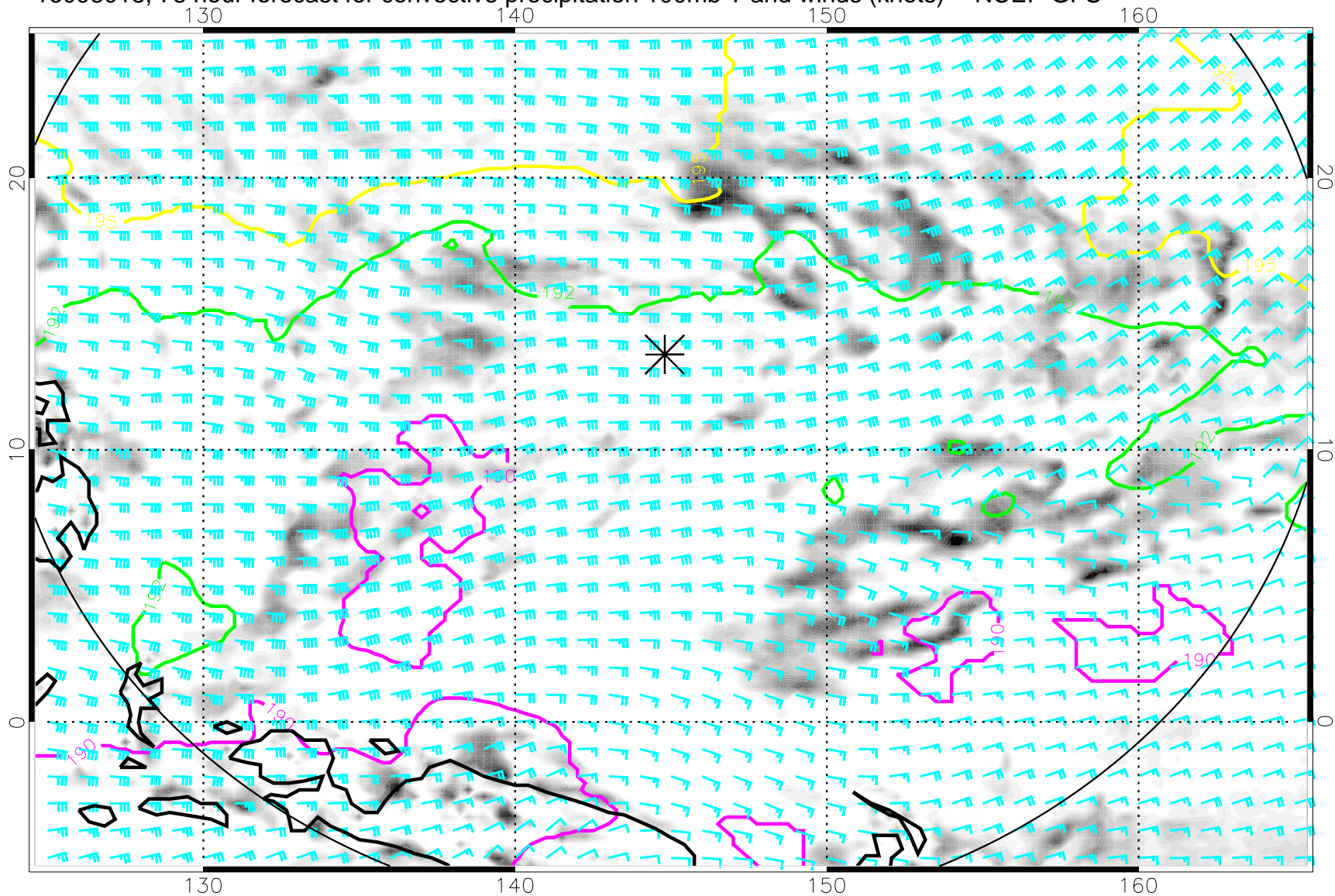
16093018, 78 hour forecast for convective precipitation 100mb T and winds (knots) -- NCEP GFS
