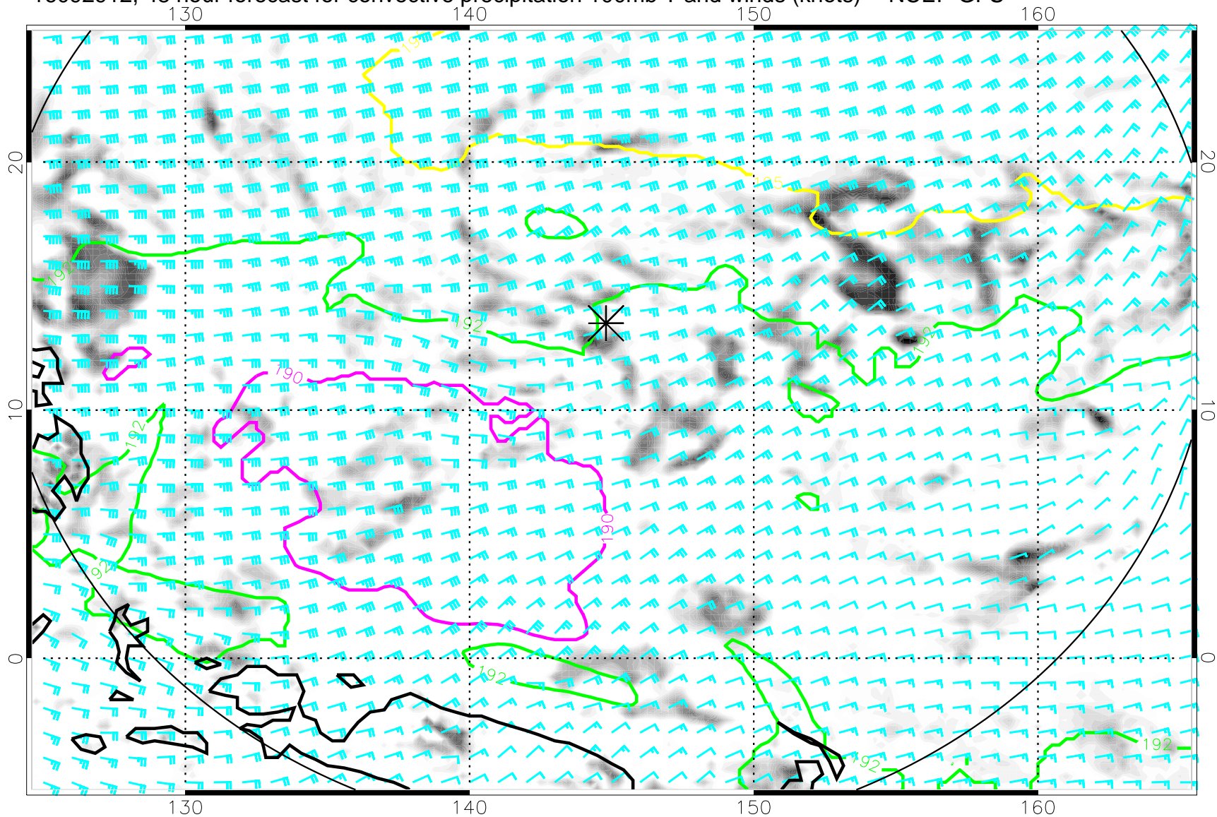
16092912, 48 hour forecast for convective precipitation 100mb T and winds (knots) -- NCEP GFS
