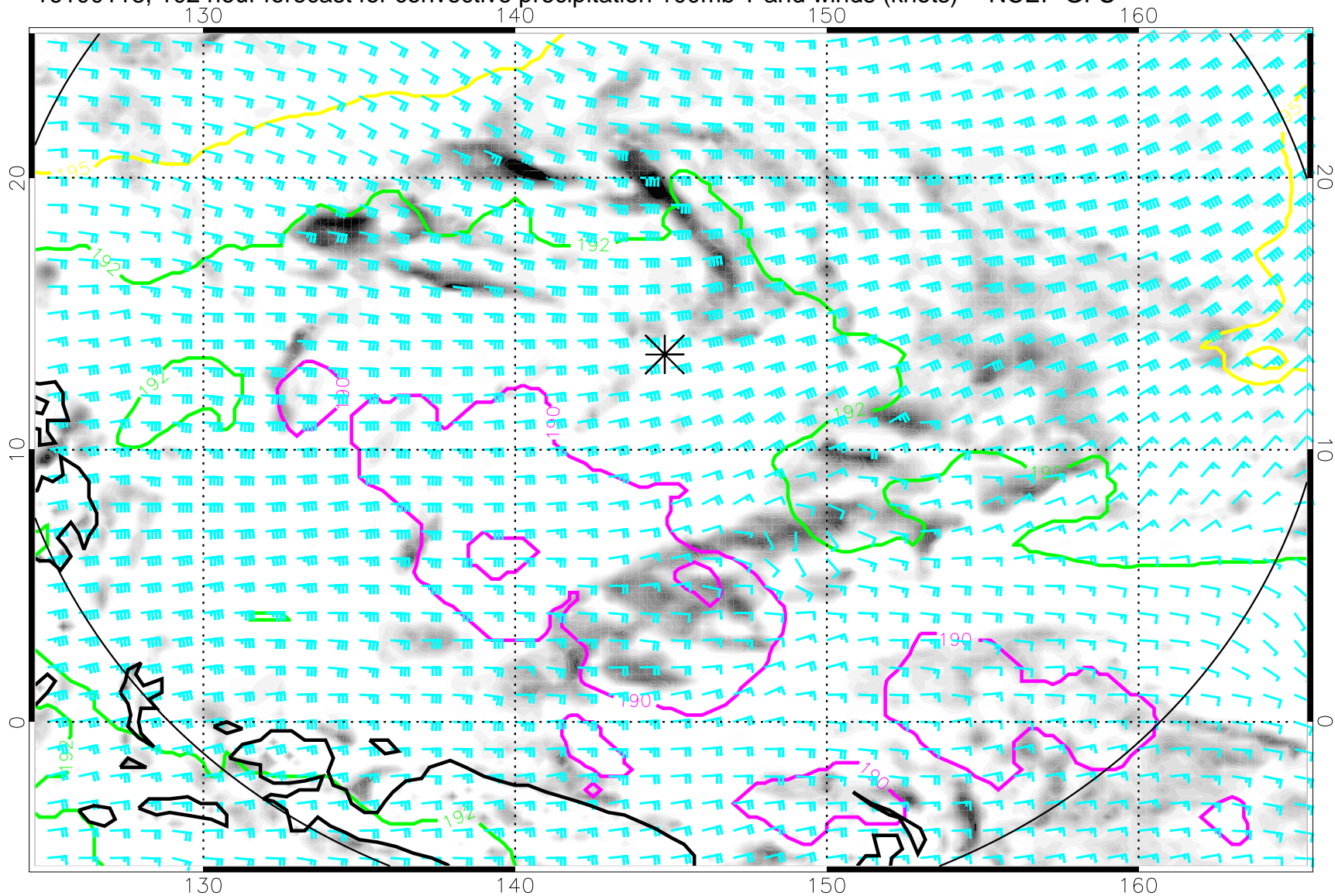
16100118, 102 hour forecast for convective precipitation 100mb T and winds (knots) -- NCEP GFS
