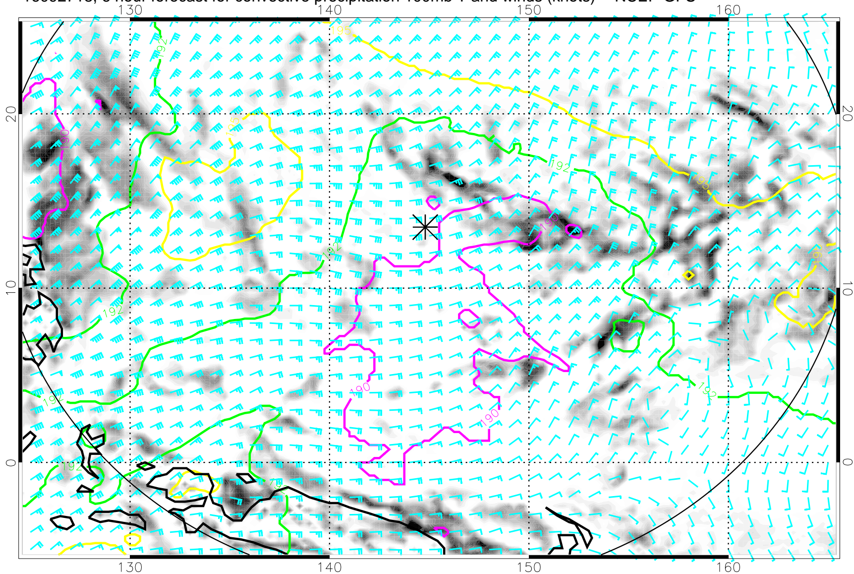
16092718, 6 hour forecast for convective precipitation 100mb T and winds (knots) -- NCEP GFS
