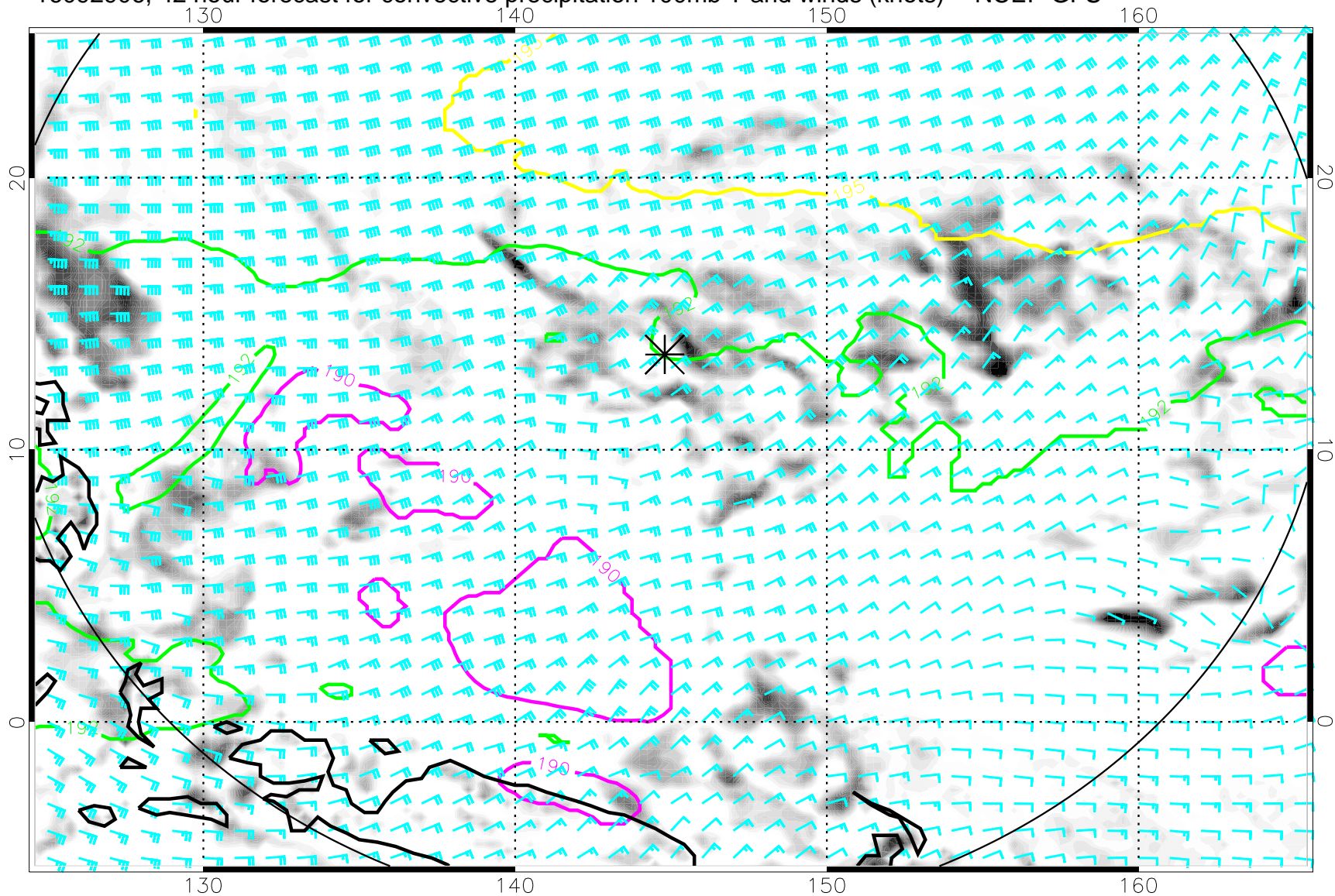
16092906, 42 hour forecast for convective precipitation 100mb T and winds (knots) -- NCEP GFS
