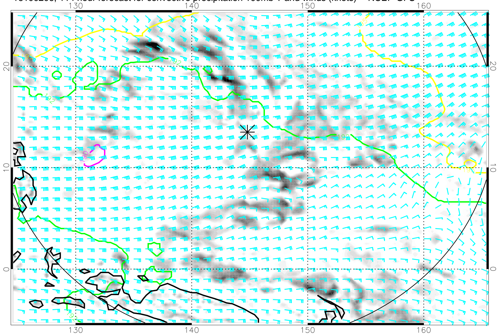
16100206, 114 hour forecast for convective precipitation 100mb T and winds (knots) -- NCEP GFS
