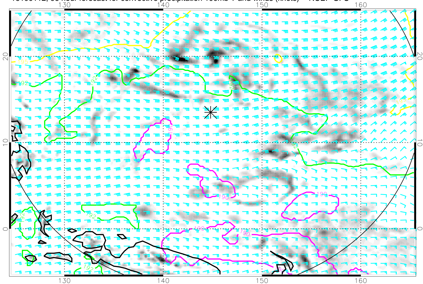
16100112, 96 hour forecast for convective precipitation 100mb T and winds (knots) -- NCEP GFS
