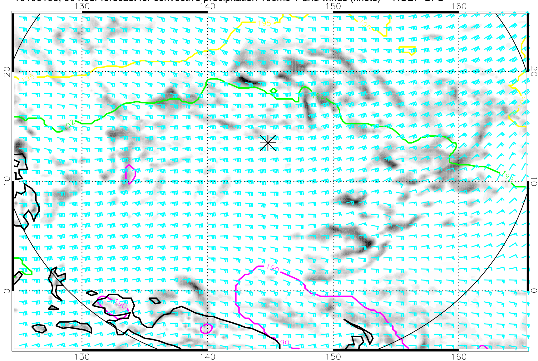
16100106, 90 hour forecast for convective precipitation 100mb T and winds (knots) -- NCEP GFS
