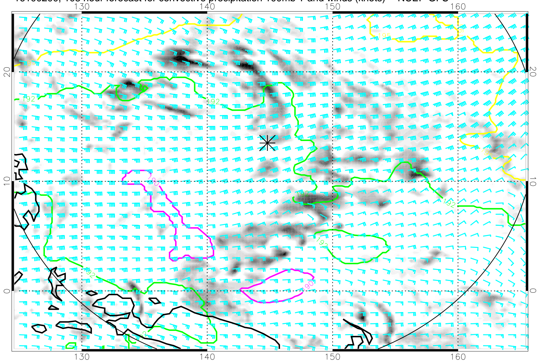
16100200, 108 hour forecast for convective precipitation 100mb T and winds (knots) -- NCEP GFS
