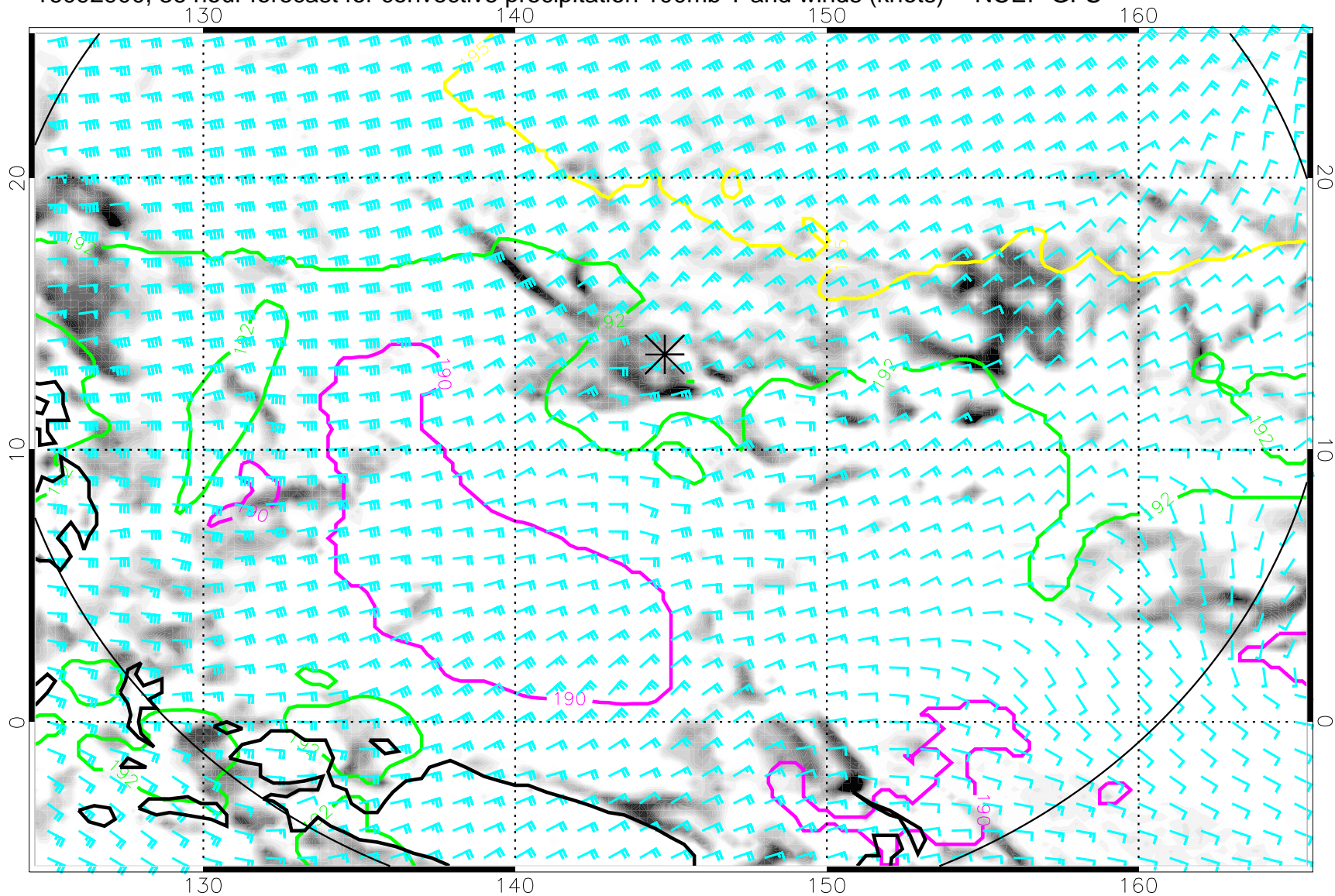
16092900, 36 hour forecast for convective precipitation 100mb T and winds (knots) -- NCEP GFS
