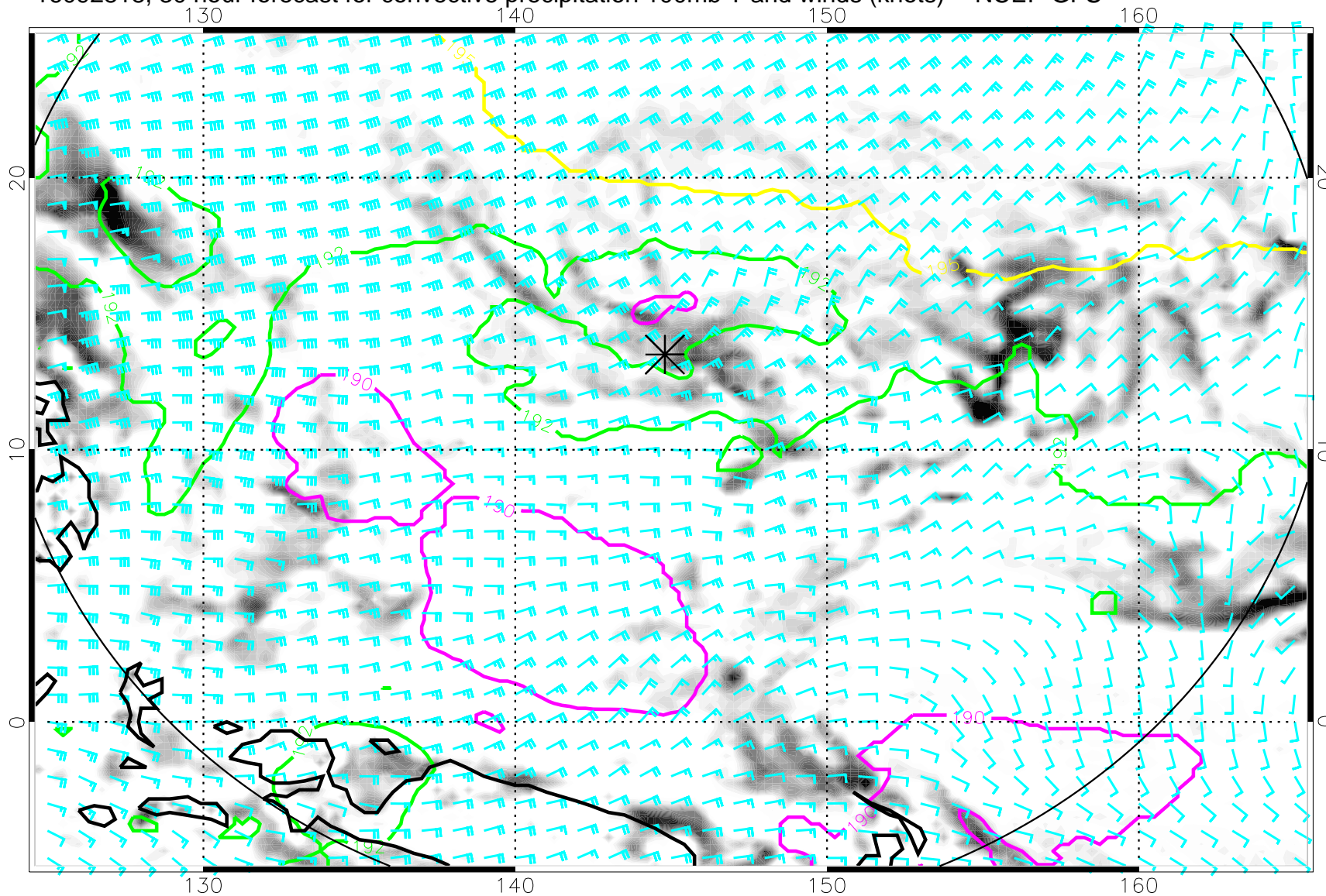
16092818, 30 hour forecast for convective precipitation 100mb T and winds (knots) -- NCEP GFS
