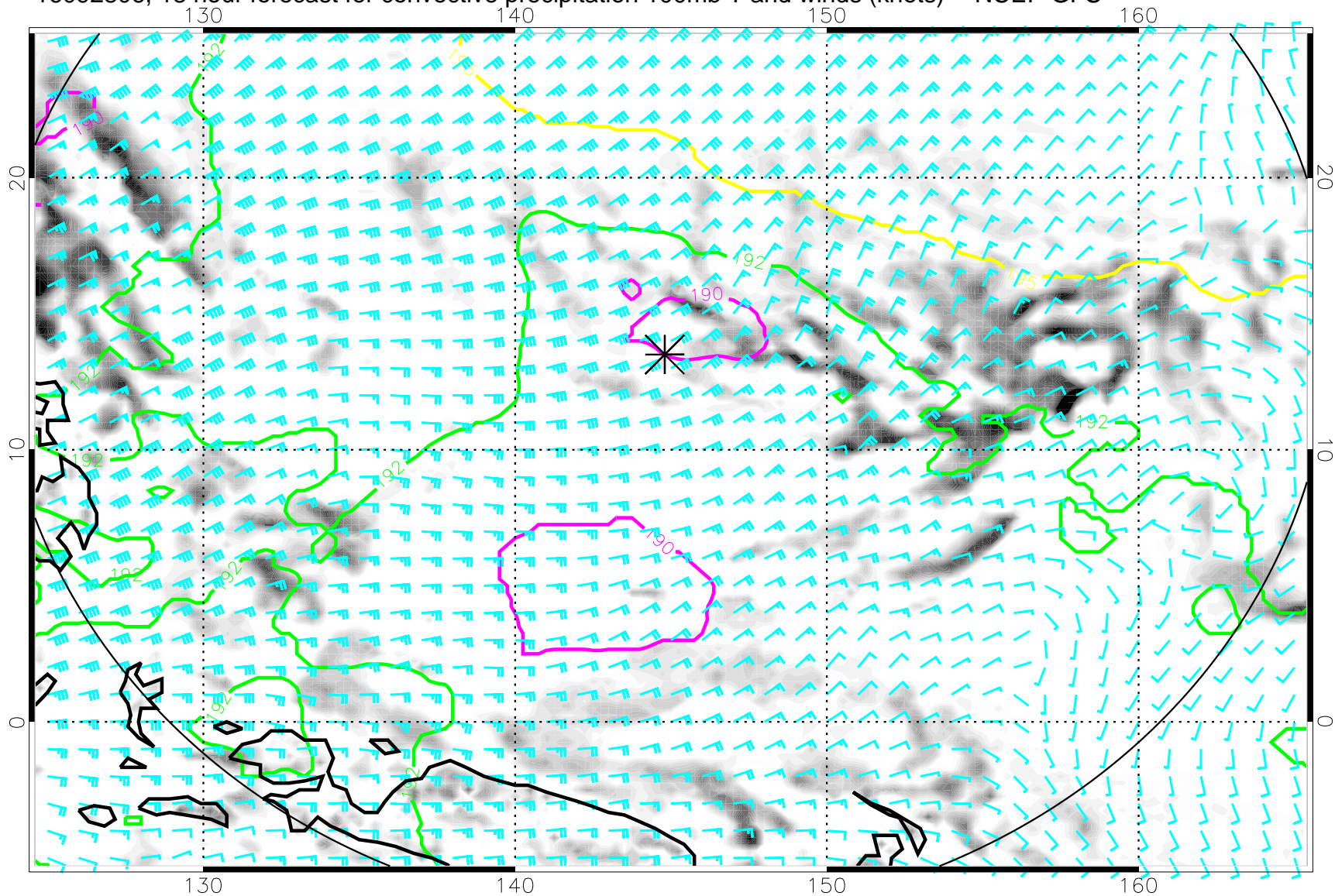
16092806, 18 hour forecast for convective precipitation 100mb T and winds (knots) -- NCEP GFS
