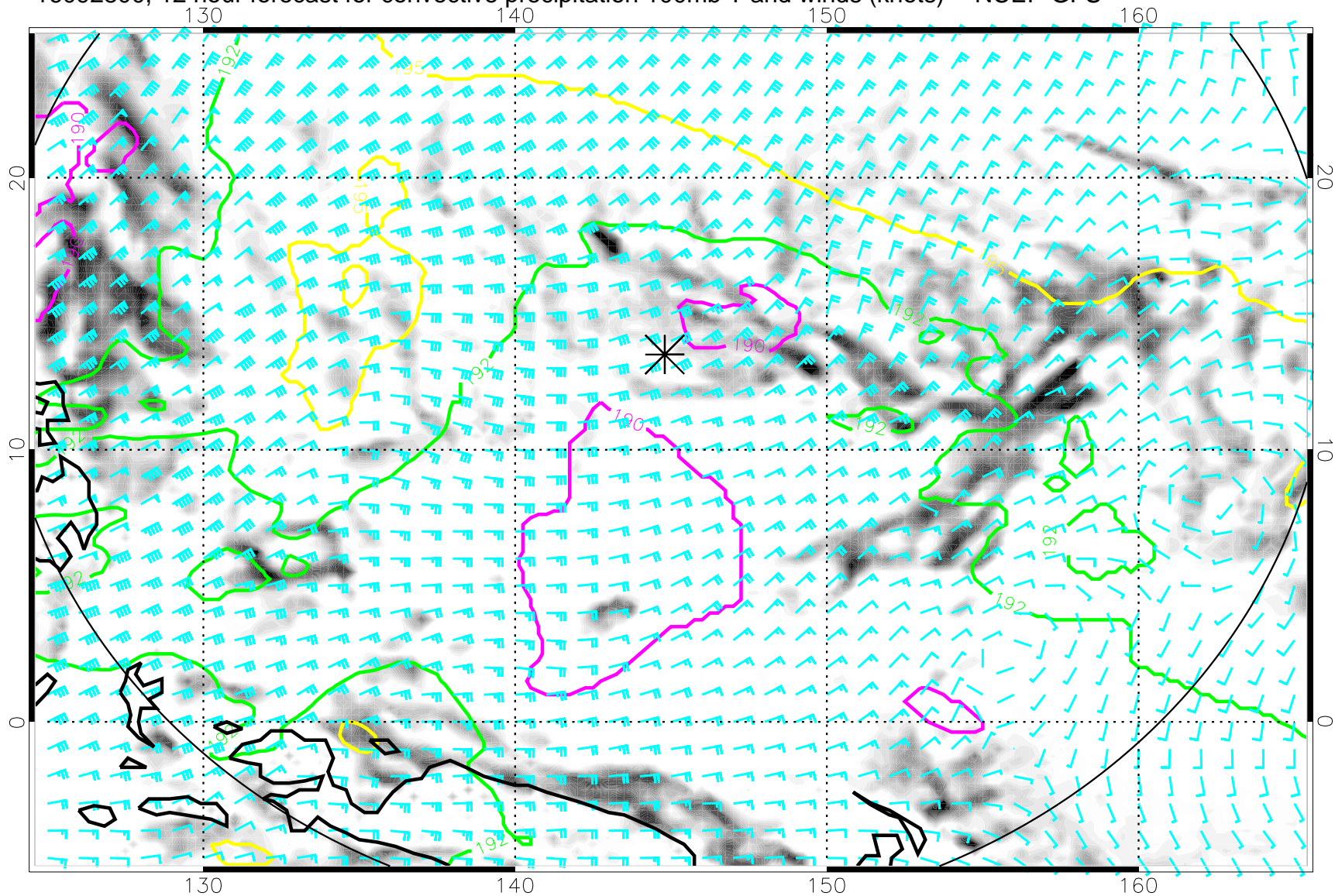
16092800, 12 hour forecast for convective precipitation 100mb T and winds (knots) -- NCEP GFS
